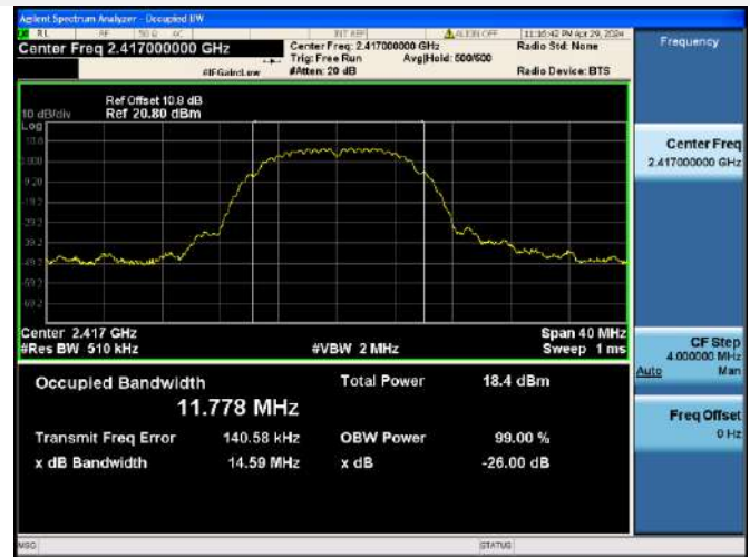
802.11b CHANNEL 2
