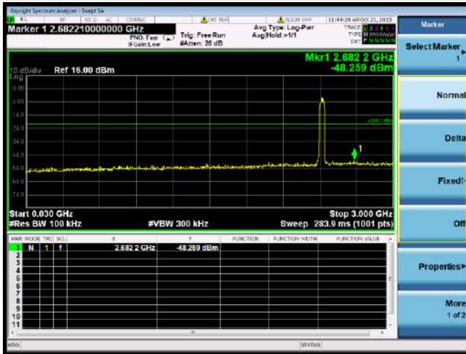
802.11n-40 MHz CHANNEL 3, SPURIOUS 30 MHz ~ 3 GHz
