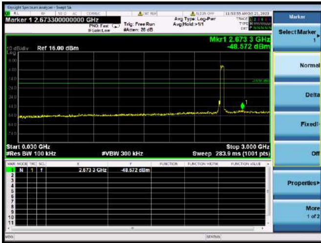
802.11n-40 MHz CHANNEL 6, SPURIOUS 30 MHz ~ 3 GHz
