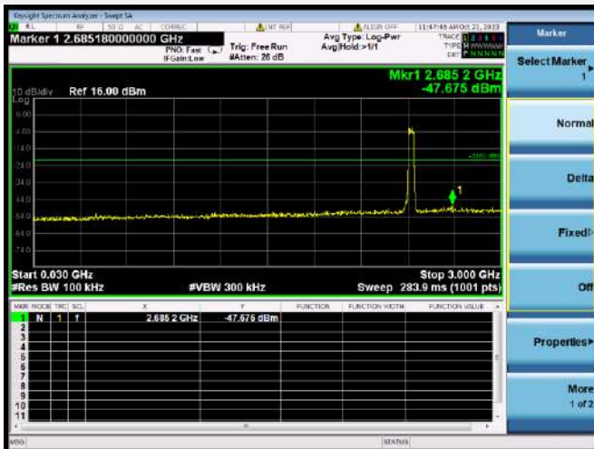
802.11n-40 MHz CHANNEL 4, SPURIOUS 30 MHz ~ 3 GHz
