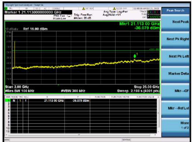
802.11n-40 MHz CHANNEL 4, SPURIOUS 2 GHz ~ 25 GHz
