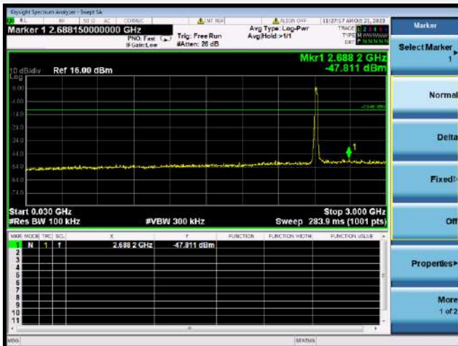
802.11n-20 MHz CHANNEL 2, SPURIOUS 30 MHz ~ 3 GHz
