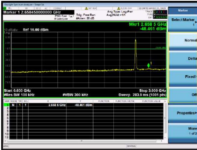
802.11n-20 MHz CHANNEL 1, SPURIOUS 30 MHz ~ 3 GHz
