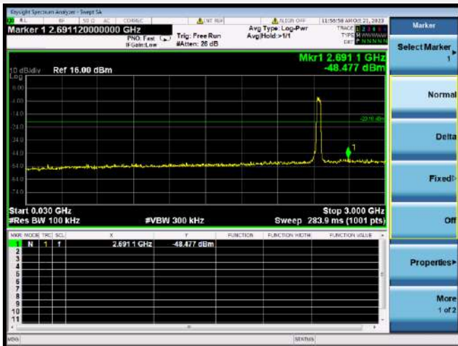
802.11n-40 MHz CHANNEL 8, SPURIOUS 30 MHz ~ 3 GHz
