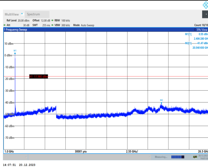
11AX40MIMO_Ant1_2422_106Tone_RU53_0~Reference
