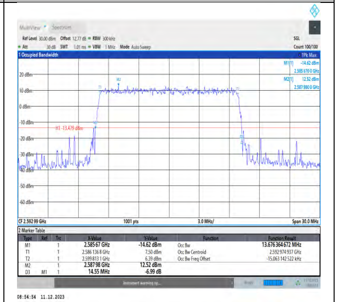
NTNV_N41_PC3_30_15_M_TID8_Ant1#1
