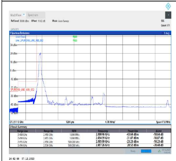
20MHz-20MHz_64QAM@64QAM-64QAM@64QAM_39750-39948_1RB#0@100RB#0-0RB#0@100RB#0
