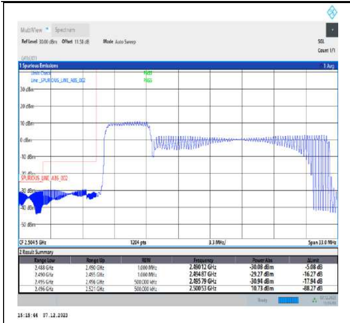
5MHz-20MHz_QPSK@QPSK-QPSK@QPSK_39683-39800_25RB#0@25RB#0-100RB#0@100RB#0
