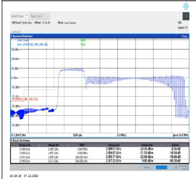
5MHz-20MHz_16QAM@16QAM-16QAM@16QAM_39683-39800_25RB#0@25RB#0-100RB#0@100RB#0
