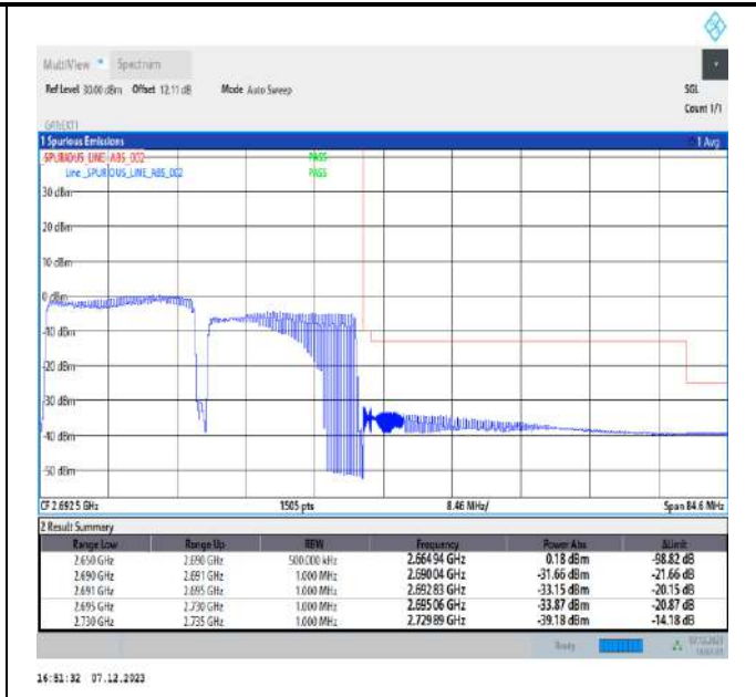
20MHz-20MHz_16QAM@16QAM-16QAM@16QAM_41292-41490_100RB#0@100RB#0-100RB#0@100RB#0
