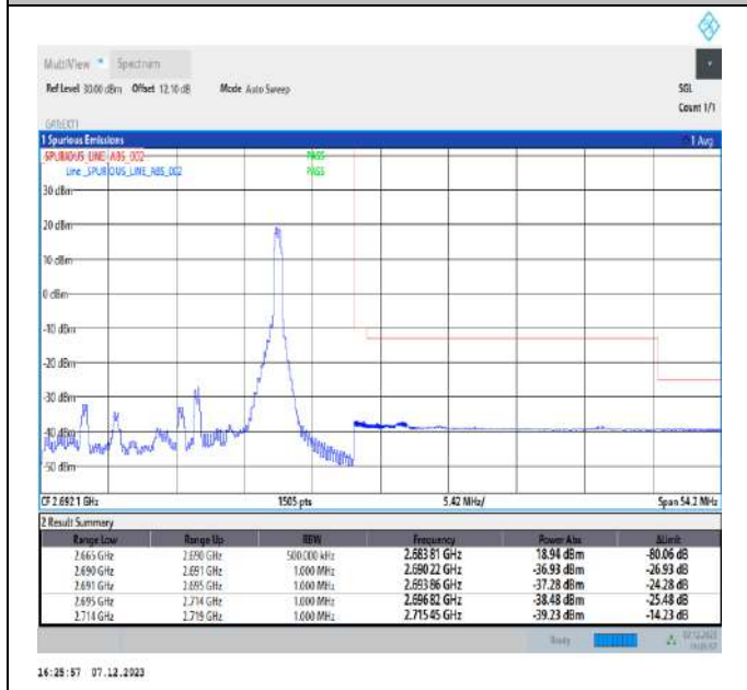
20MHz-5MHz_QPSK@QPSK-QPSK@QPSK_41440-41557_1RB#99@100RB#0-0RB#0@25RB#0
