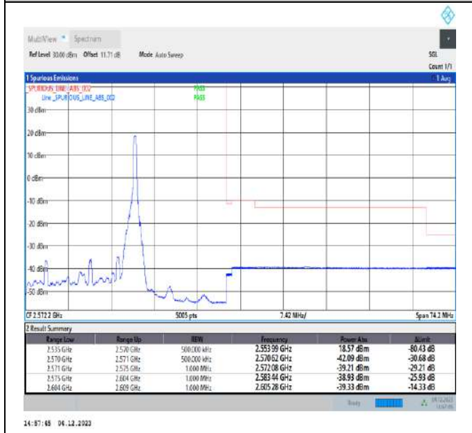
20MHz-15MHz_64QAM@64QAM-64QAM@64QAM_21201-21372_1RB#99@100RB#0-0RB#0@75RB#0
