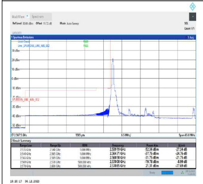
15MHz-15MHz_64QAM@64QAM-64QAM@64QAM_37825-37975_1RB#0@75RB#0-0RB#0@75RB#0
