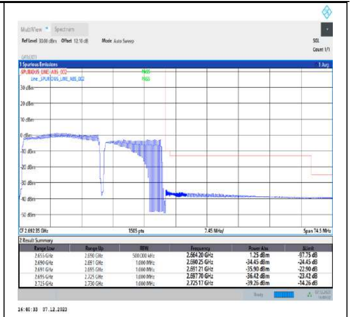
20MHz-15MHz_64QAM@64QAM-64QAM@64QAM_41341-41512_100RB#0@100RB#0-75RB#0@75RB#0
