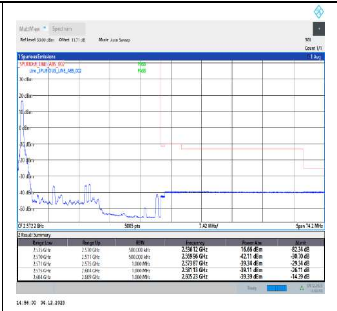
20MHz-15MHz_64QAM@64QAM-64QAM@64QAM_21201-21372_1RB#0@100RB#0-0RB#0@75RB#0
