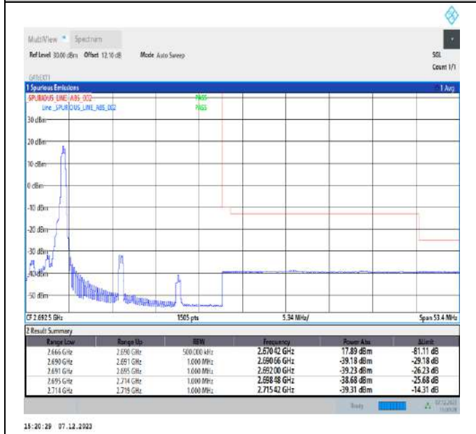
5MHz-20MHz_64QAM@64QAM-64QAM@64QAM_41373-41490_1RB#24@25RB#0-0RB#0@100RB#0
