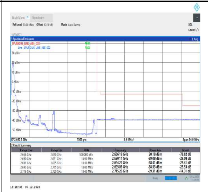
10MHz-15MHz_QPSK@QPSK-QPSK@QPSK_41395-41515_1RB#0@50RB#0-0RB#0@75RB#0
