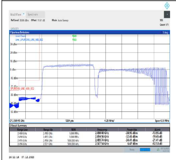
15MHz-20MHz_QPSK@QPSK-QPSK@QPSK_39728-39899_75RB#0@75RB#0-100RB#0@100RB#0
