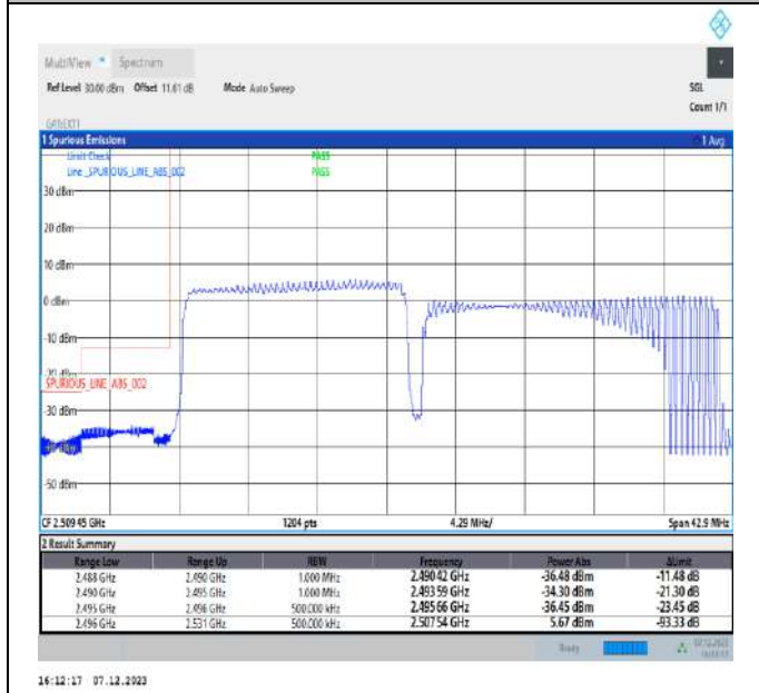
15MHz-20MHz_64QAM@64QAM-64QAM@64QAM_39728-39899_75RB#0@75RB#0-100RB#0@100RB#0
