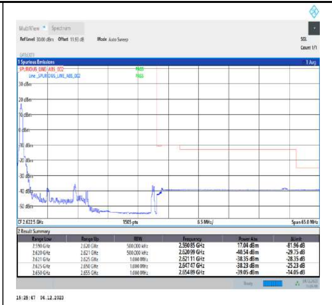
15MHz-15MHz_64QAM@64QAM-64QAM@64QAM_38025-38175_1RB#0@75RB#0-0RB#0@75RB#0
