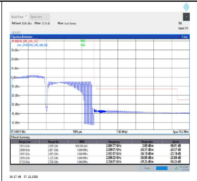
15MHz-20MHz_64QAM@64QAM-64QAM@64QAM_41319-41490_75RB#0@75RB#0-100RB#0@100RB#0
