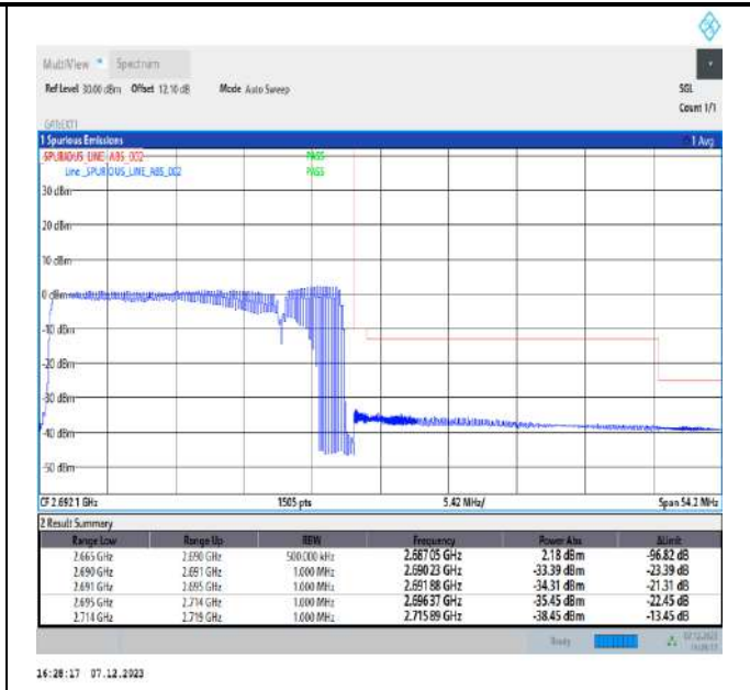
20MHz-5MHz_16QAM@16QAM-16QAM@16QAM_41440-41557_100RB#0@100RB#0-25RB#0@25RB#0
