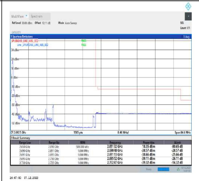
20MHz-20MHz_16QAM@16QAM-16QAM@16QAM_41292-41490_1RB#0@100RB#0-0RB#0@100RB#0
