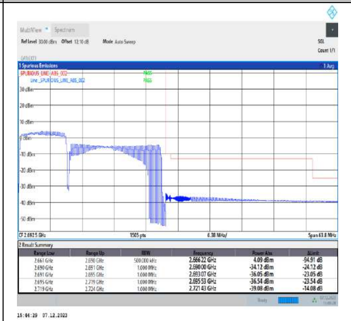
10MHz-20MHz_64QAM@64QAM-64QAM@64QAM_41346-41490_50RB#0@50RB#0-100RB#0@100RB#0
