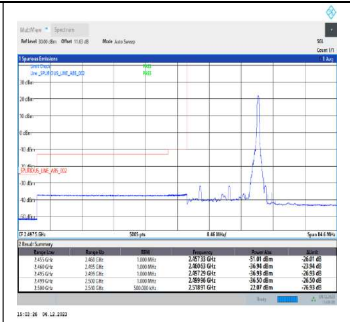
20MHz-20MHz_64QAM@64QAM-64QAM@64QAM_20850-21048_1RB#99@100RB#0-0RB#0@100RB#0
