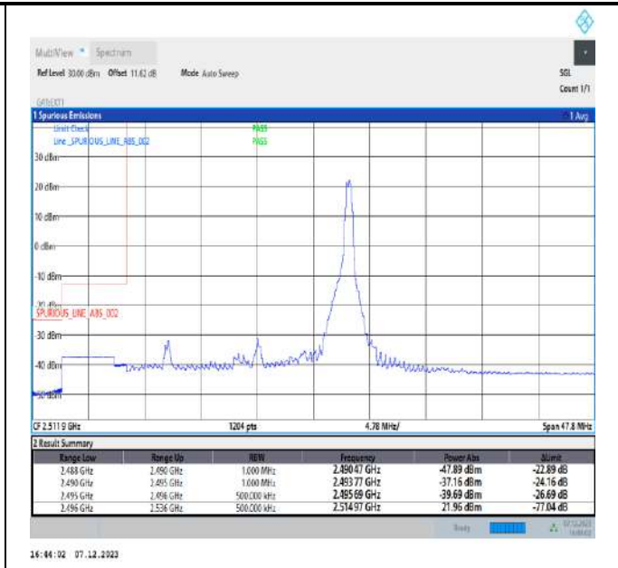
20MHz-20MHz_16QAM@16QAM-16QAM@16QAM_39750-39948_1RB#99@100RB#0-0RB#0@100RB#0
