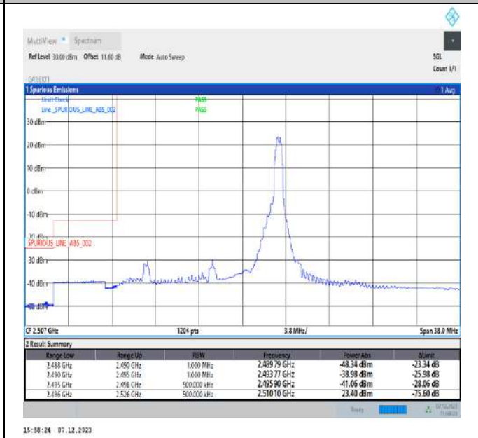
15MHz-15MHz_QPSK@QPSK-QPSK@QPSK_39725-39875_1RB#74@75RB#0-0RB#0@75RB#0
