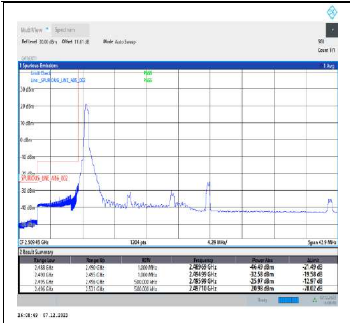
15MHz-20MHz_64QAM@64QAM-64QAM@64QAM_39728-39899_1RB#0@75RB#0-0RB#0@100RB#0
