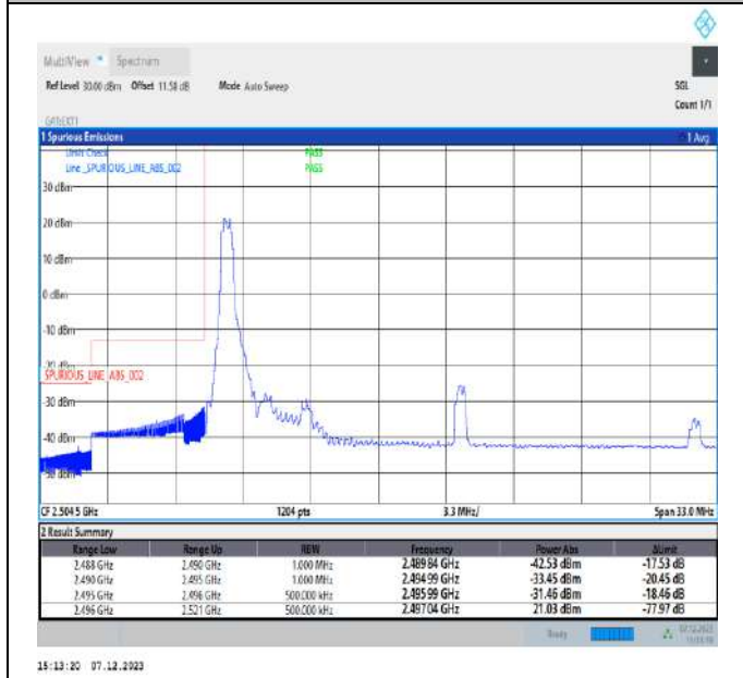
5MHz-20MHz_64QAM@64QAM-64QAM@64QAM_39683-39800_1RB#0@25RB#0-0RB#0@100RB#0
