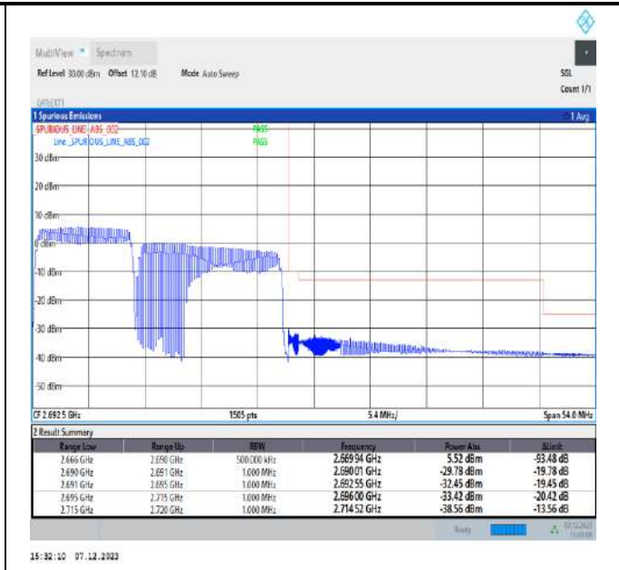
10MHz-15MHz_QPSK@QPSK-QPSK@QPSK_41395-41515_50RB#0@50RB#0-75RB#0@75RB#0
