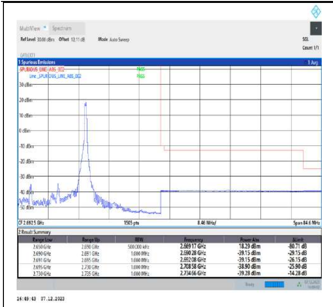
20MHz-20MHz_16QAM@16QAM-16QAM@16QAM_41292-41490_1RB#99@100RB#0-0RB#0@100RB#0
