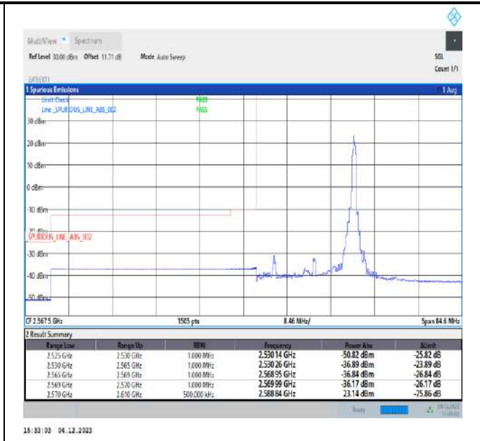
20MHz-20MHz_16QAM@16QAM-16QAM@16QAM_37850-38048_1RB#99@100RB#0-0RB#0@100RB#0
