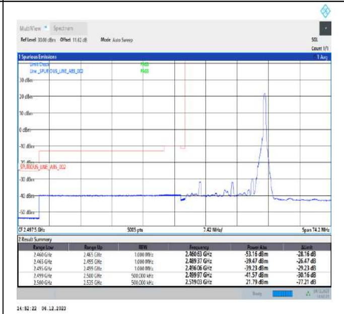
20MHz-15MHz_64QAM@64QAM-64QAM@64QAM_20850-21021_1RB#99@100RB#0-0RB#0@75RB#0
