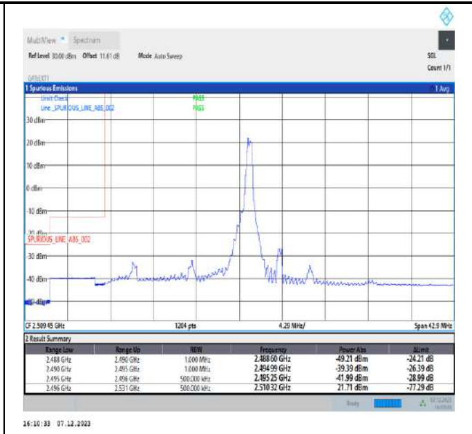
15MHz-20MHz_64QAM@64QAM-64QAM@64QAM_39728-39899_1RB#74@75RB#0-0RB#0@100RB#0
