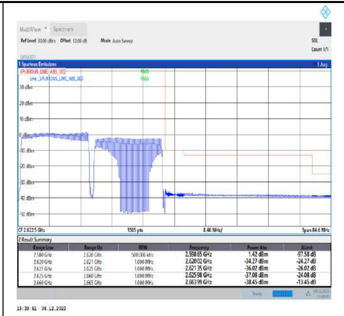
20MHz-20MHz_QPSK@QPSK-QPSK@QPSK_37952-38150_100RB#0@100RB#0-100RB#0@100RB#0
