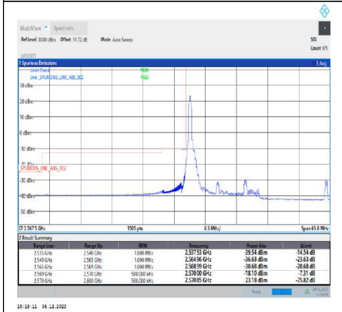
15MHz-15MHz_QPSK@QPSK-QPSK@QPSK_37825-37975_1RB#0@75RB#0-0RB#0@75RB#0
