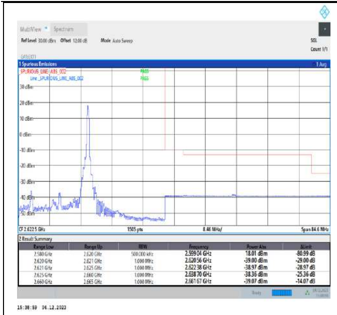
20MHz-20MHz_64QAM@64QAM-64QAM@64QAM_37952-38150_1RB#99@100RB#0-0RB#0@100RB#0
