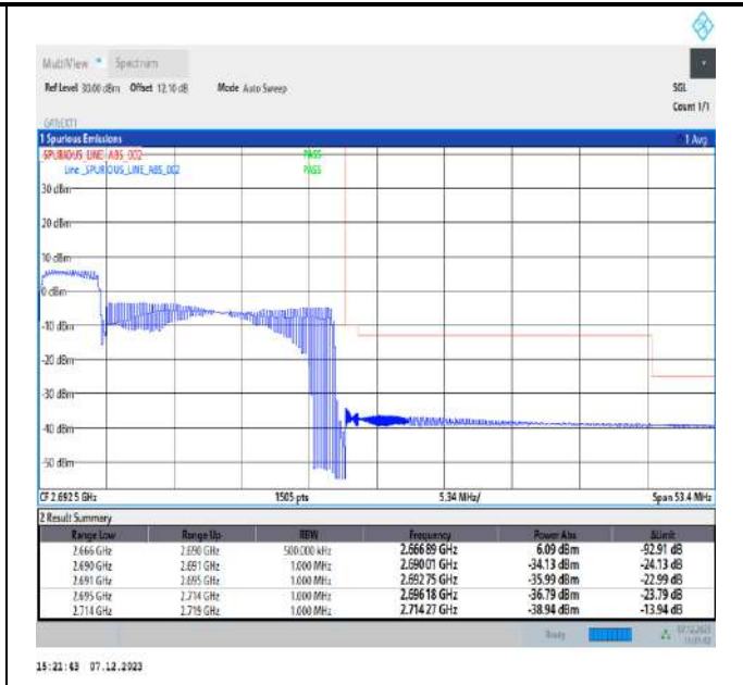
5MHz-20MHz_16QAM@16QAM-16QAM@16QAM_41373-41490_25RB#0@25RB#0-100RB#0@100RB#0
