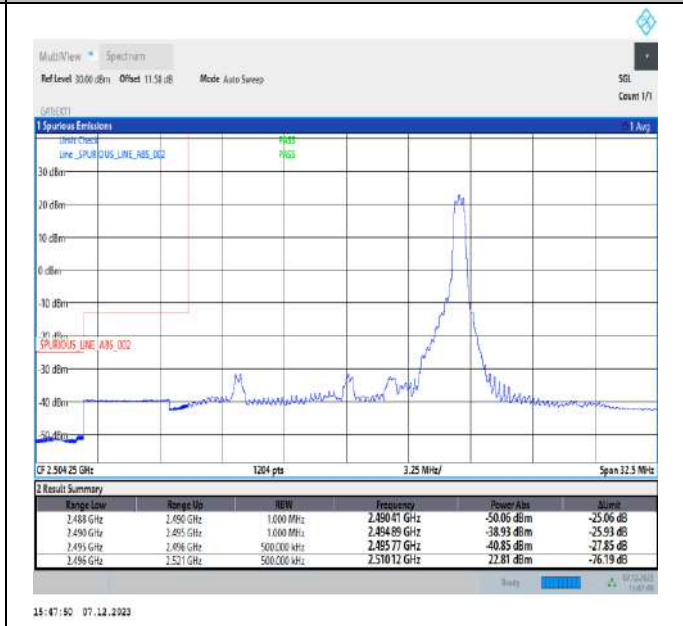
15MHz-10MHz_16QAM@16QAM-16QAM@16QAM_39725-39845_1RB#74@75RB#0-0RB#0@50RB#0
