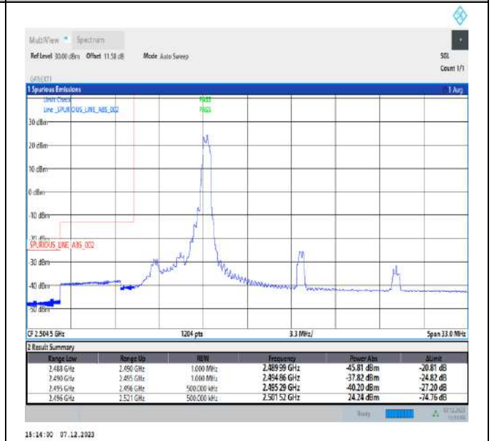
5MHz-20MHz_QPSK@QPSK-QPSK@QPSK_39683-39800_1RB#24@25RB#0-0RB#0@100RB#0
