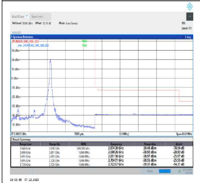
15MHz-15MHz_QPSK@QPSK-QPSK@QPSK_41365-41515_1RB#74@75RB#0-0RB#0@75RB#0
