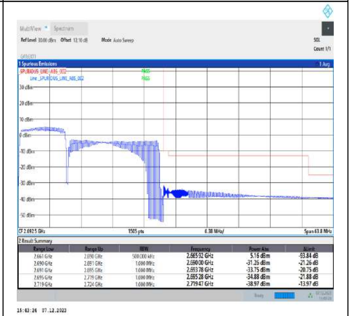
10MHz-20MHz_QPSK@QPSK-QPSK@QPSK_41346-41490_50RB#0@50RB#0-100RB#0@100RB#0
