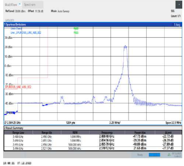
15MHz-10MHz_64QAM@64QAM-64QAM@64QAM_39725-39845_1RB#74@75RB#0-0RB#0@50RB#0
