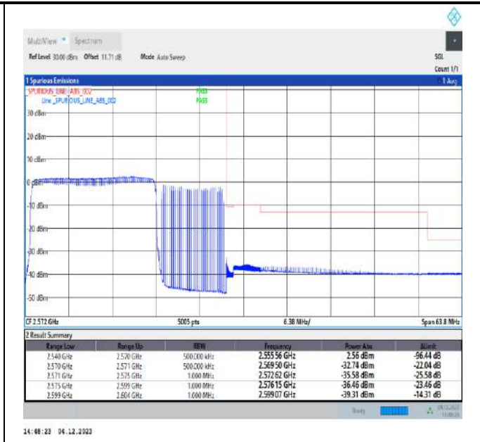
20MHz-10MHz_64QAM@64QAM-64QAM@64QAM_21251-21395_100RB#0@100RB#0-50RB#0@50RB#0
