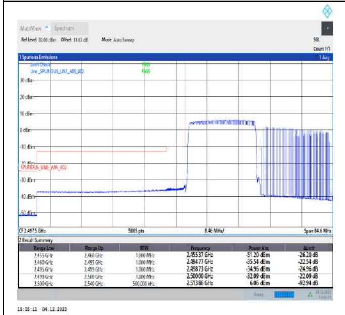
20MHz-20MHz_64QAM@64QAM-64QAM@64QAM_20850-21048_100RB#0@100RB#0-100RB#0@100RB#0
