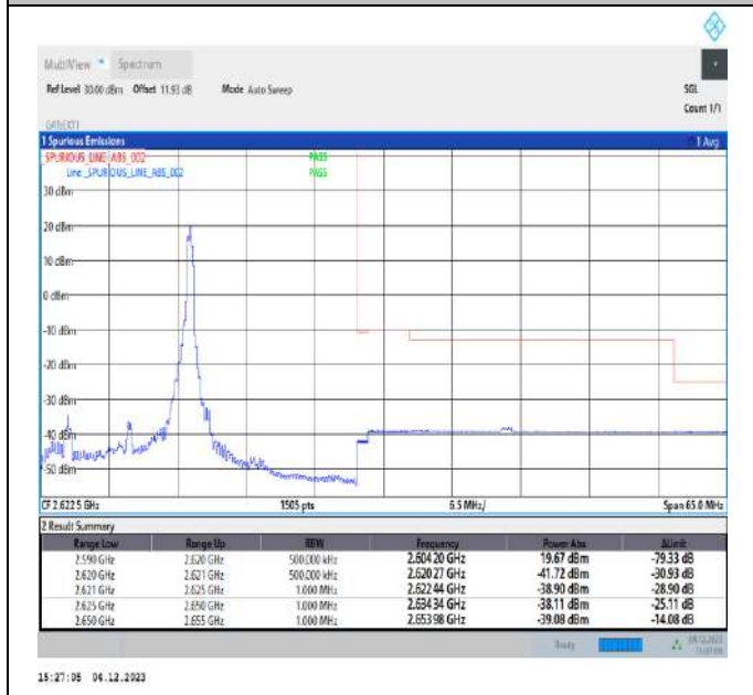
15MHz-15MHz_16QAM@16QAM-16QAM@16QAM_38025-38175_1RB#74@75RB#0-0RB#0@75RB#0
