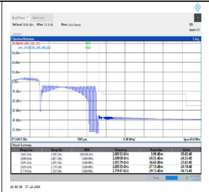
10MHz-20MHz_16QAM@16QAM-16QAM@16QAM_41346-41490_50RB#0@50RB#0-100RB#0@100RB#0
