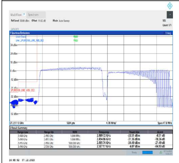
20MHz-20MHz_16QAM@16QAM-16QAM@16QAM_39750-39948_100RB#0@100RB#0-100RB#0@100RB#0
