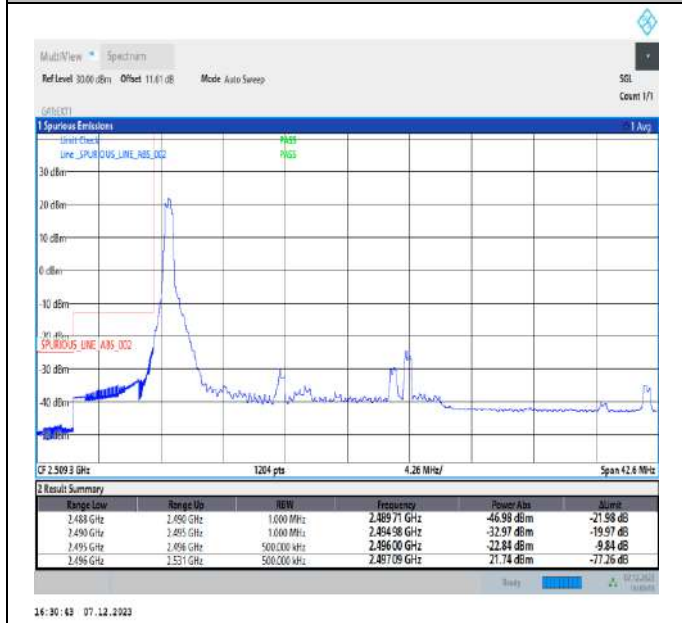
20MHz-15MHz_16QAM@16QAM-16QAM@16QAM_39750-39921_1RB#0@100RB#0-0RB#0@75RB#0
