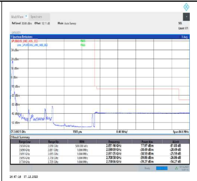
20MHz-20MHz_QPSK@QPSK-QPSK@QPSK_41292-41490_1RB#0@100RB#0-0RB#0@100RB#0
