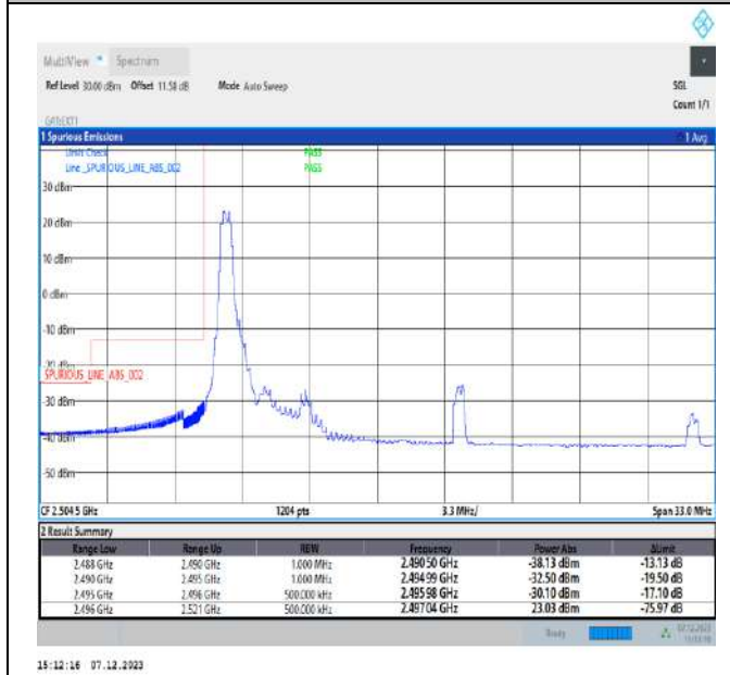
5MHz-20MHz_QPSK@QPSK-QPSK@QPSK_39683-39800_1RB#0@25RB#0-0RB#0@100RB#0
