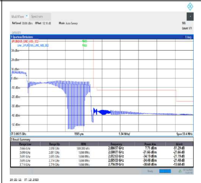
5MHz-20MHz_QPSK@QPSK-QPSK@QPSK_41373-41490_25RB#0@25RB#0-100RB#0@100RB#0
