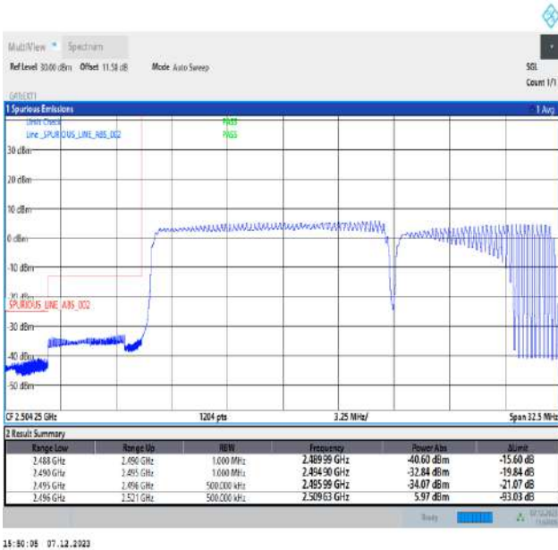
15MHz-10MHz_64QAM@64QAM-64QAM@64QAM_39725-39845_75RB#0@75RB#0-50RB#0@50RB#0
