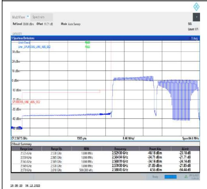
20MHz-20MHz_64QAM@64QAM-64QAM@64QAM_37850-38048_100RB#0@100RB#0-100RB#0@100RB#0
