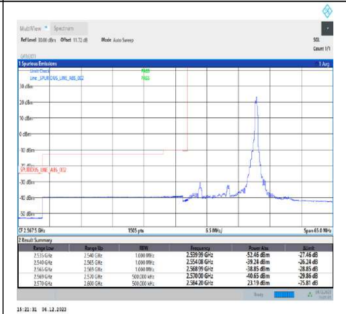
15MHz-15MHz_16QAM@16QAM-16QAM@16QAM_37825-37975_1RB#74@75RB#0-0RB#0@75RB#0
