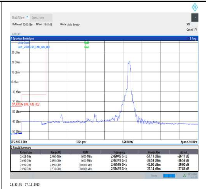
20MHz-15MHz_64QAM@64QAM-64QAM@64QAM_39750-39921_1RB#99@100RB#0-0RB#0@75RB#0
