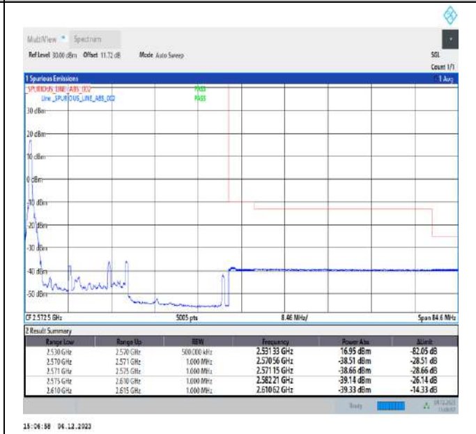
20MHz-20MHz_64QAM@64QAM-64QAM@64QAM_21152-21350_1RB#0@100RB#0-0RB#0@100RB#0
