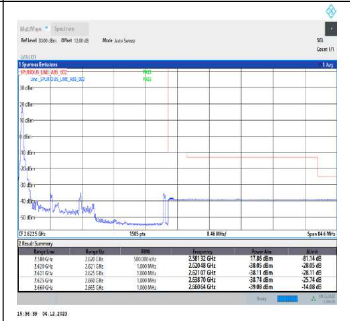
20MHz-20MHz_16QAM@16QAM-16QAM@16QAM_37952-38150_1RB#0@100RB#0-0RB#0@100RB#0
