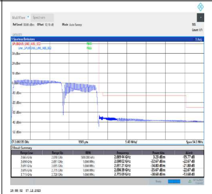
15MHz-10MHz_16QAM@16QAM-16QAM@16QAM_41417-41537_75RB#0@75RB#0-50RB#0@50RB#0
