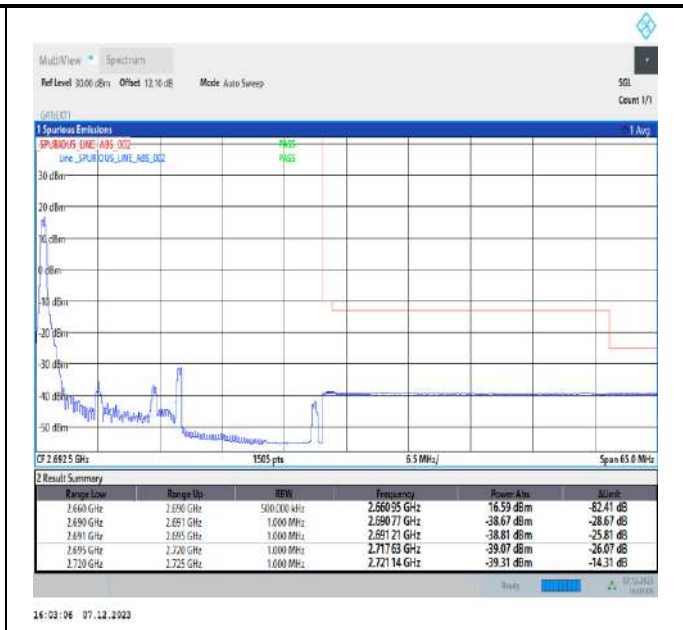
15MHz-15MHz_64QAM@64QAM-64QAM@64QAM_41365-41515_1RB#0@75RB#0-0RB#0@75RB#0
