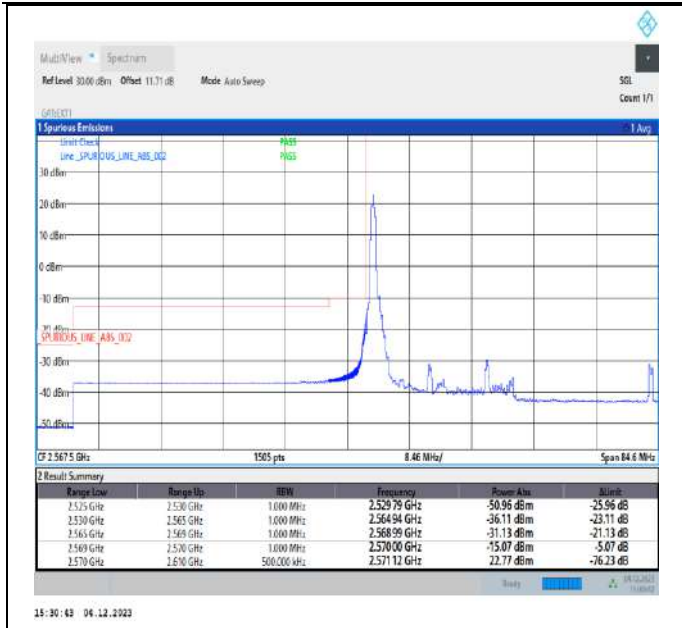
20MHz-20MHz_QPSK@QPSK-QPSK@QPSK_37850-38048_1RB#0@100RB#0-0RB#0@100RB#0
