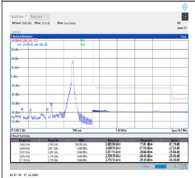
20MHz-5MHz_64QAM@64QAM-64QAM@64QAM_41440-41557_1RB#99@100RB#0-0RB#0@25RB#0
