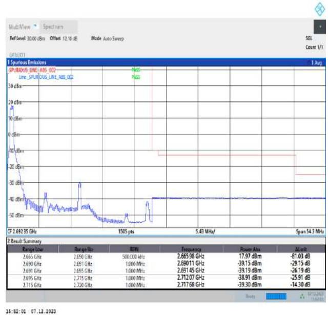
15MHz-10MHz_64QAM@64QAM-64QAM@64QAM_41417-41537_1RB#0@75RB#0-0RB#0@50RB#0
