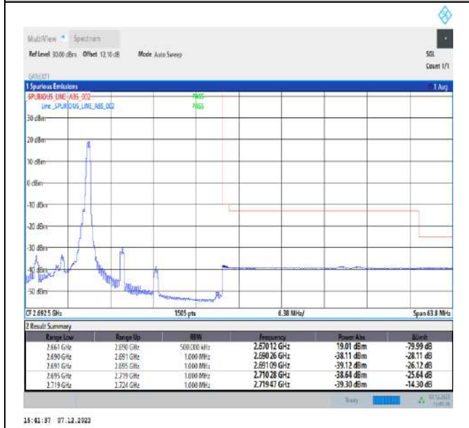
10MHz-20MHz_QPSK@QPSK-QPSK@QPSK_41346-41490_1RB#49@50RB#0-0RB#0@100RB#0
