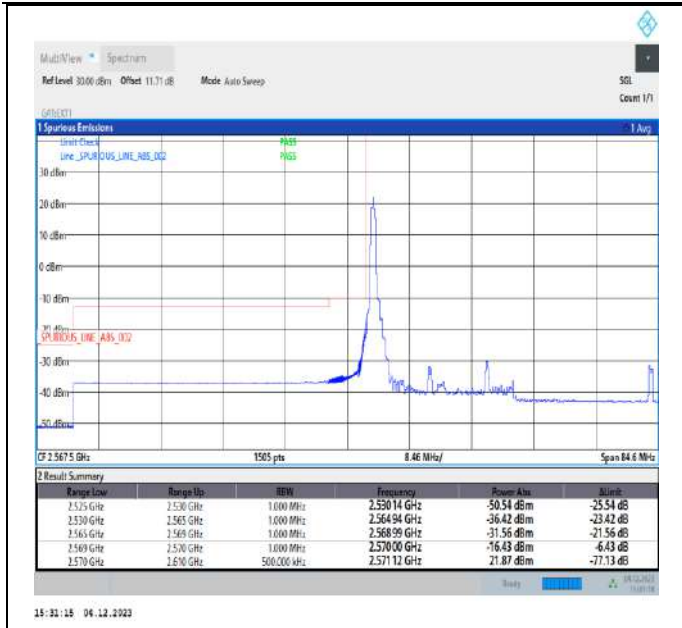
20MHz-20MHz_16QAM@16QAM-16QAM@16QAM_37850-38048_1RB#0@100RB#0-0RB#0@100RB#0
