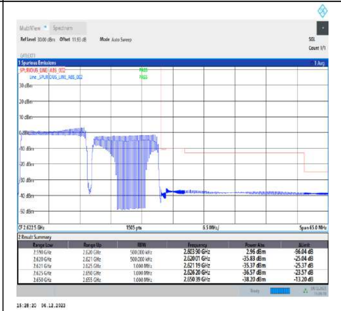
15MHz-15MHz_QPSK@QPSK-QPSK@QPSK_38025-38175_75RB#0@75RB#0-75RB#0@75RB#0
