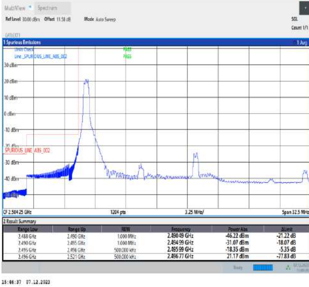
15MHz-10MHz_64QAM@64QAM-64QAM@64QAM_39725-39845_1RB#0@75RB#0-0RB#0@50RB#0
