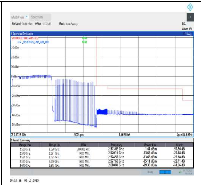
20MHz-20MHz_64QAM@64QAM-64QAM@64QAM_21152-21350_100RB#0@100RB#0-100RB#0@100RB#0
