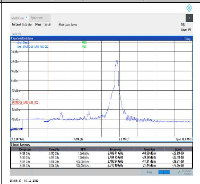
15MHz-15MHz_64QAM@64QAM-64QAM@64QAM_39725-39875_1RB#74@75RB#0-0RB#0@75RB#0
