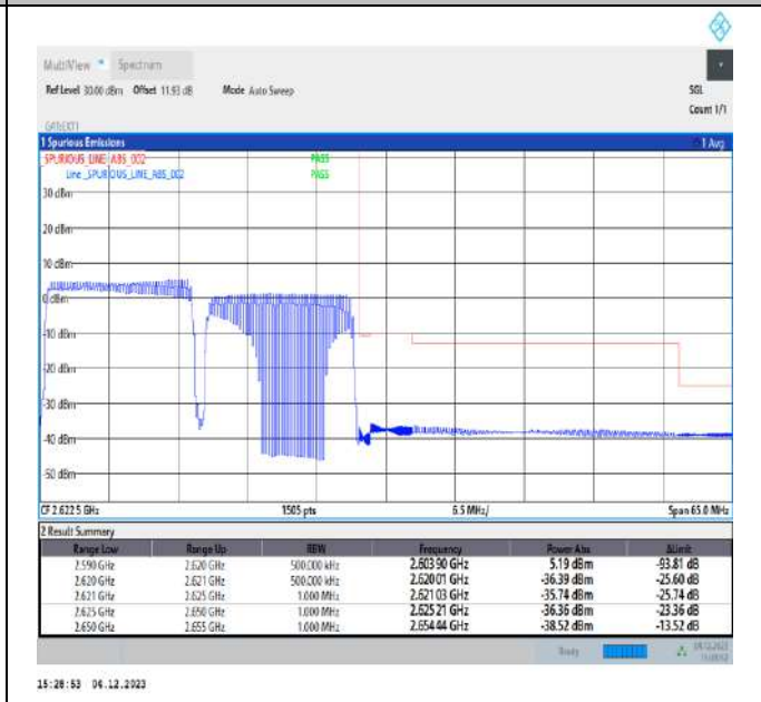
15MHz-15MHz_16QAM@16QAM-16QAM@16QAM_38025-38175_75RB#0@75RB#0-75RB#0@75RB#0
