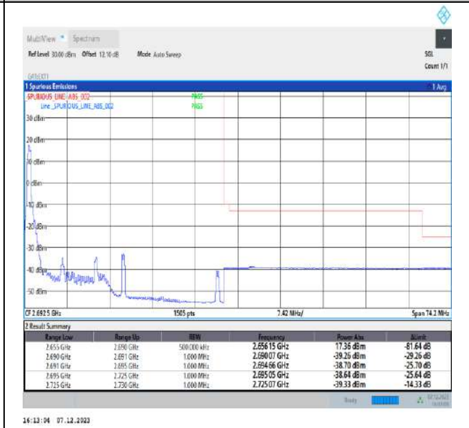
15MHz-20MHz_QPSK@QPSK-QPSK@QPSK_41319-41490_1RB#0@75RB#0-0RB#0@100RB#0
