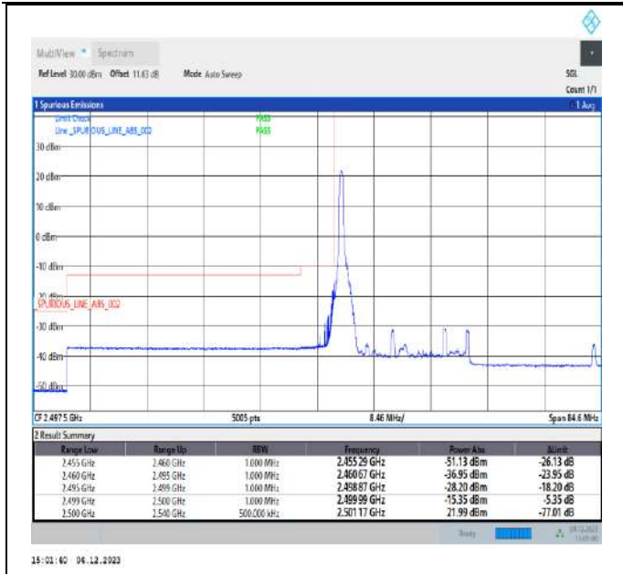
20MHz-20MHz_64QAM@64QAM-64QAM@64QAM_20850-21048_1RB#0@100RB#0-0RB#0@100RB#0
