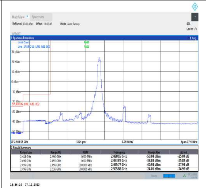
10MHz-20MHz_QPSK@QPSK-QPSK@QPSK_39705-39849_1RB#49@50RB#0-0RB#0@100RB#0
