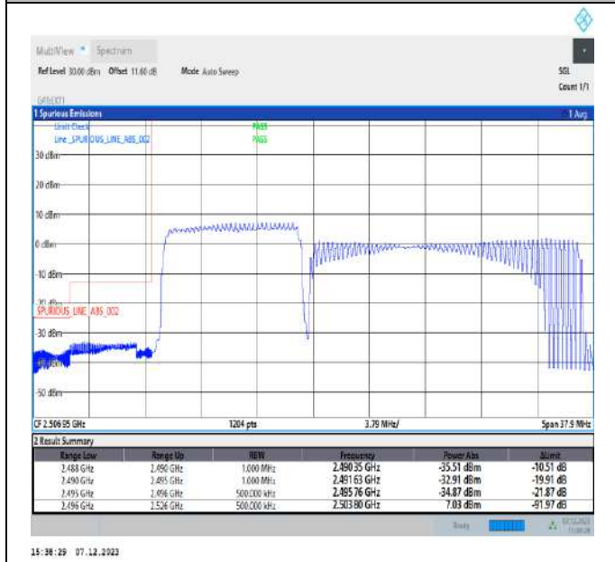
10MHz-20MHz_16QAM@16QAM-16QAM@16QAM_39705-39849_50RB#0@50RB#0-100RB#0@100RB#0
