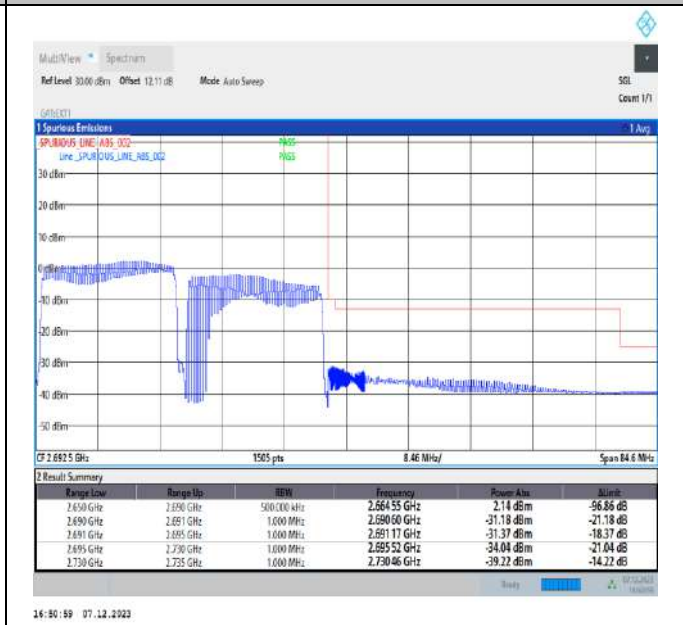
20MHz-20MHz_QPSK@QPSK-QPSK@QPSK_41292-41490_100RB#0@100RB#0-100RB#0@100RB#0
