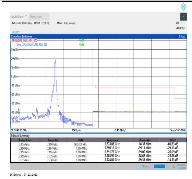
20MHz-15MHz_64QAM@64QAM-64QAM@64QAM_41341-41512_1RB#99@100RB#0-0RB#0@75RB#0
