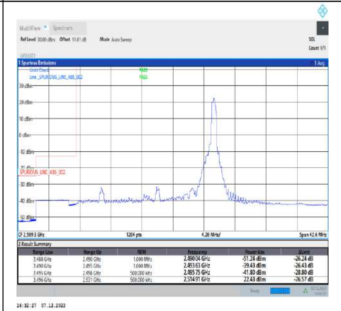
20MHz-15MHz_16QAM@16QAM-16QAM@16QAM_39750-39921_1RB#99@100RB#0-0RB#0@75RB#0
