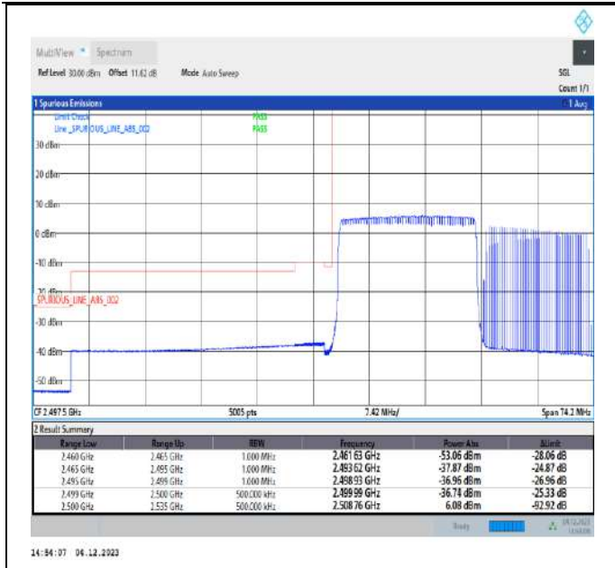
20MHz-15MHz_64QAM@64QAM-64QAM@64QAM_20850-21021_100RB#0@100RB#0-75RB#0@75RB#0
