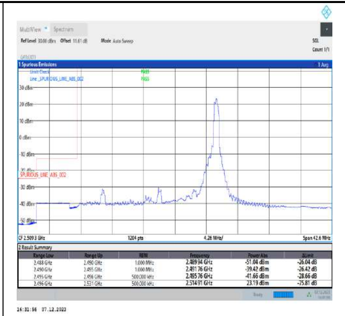
20MHz-15MHz_QPSK@QPSK-QPSK@QPSK_39750-39921_1RB#99@100RB#0-0RB#0@75RB#0
