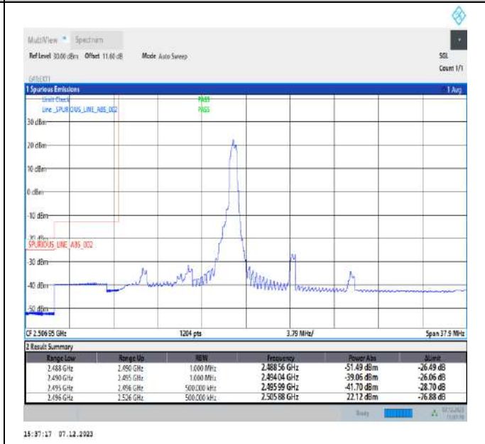
10MHz-20MHz_64QAM@64QAM-64QAM@64QAM_39705-39849_1RB#49@50RB#0-0RB#0@100RB#0
