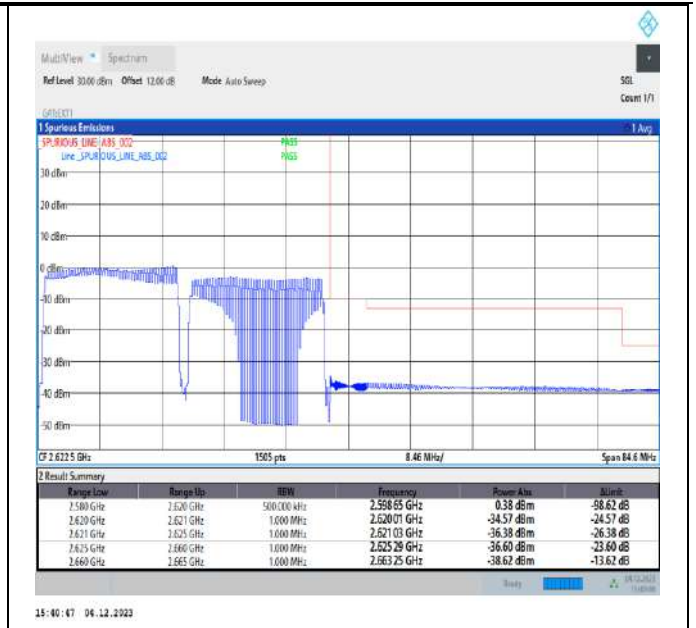
20MHz-20MHz_64QAM@64QAM-64QAM@64QAM_37952-38150_100RB#0@100RB#0-100RB#0@100RB#0
