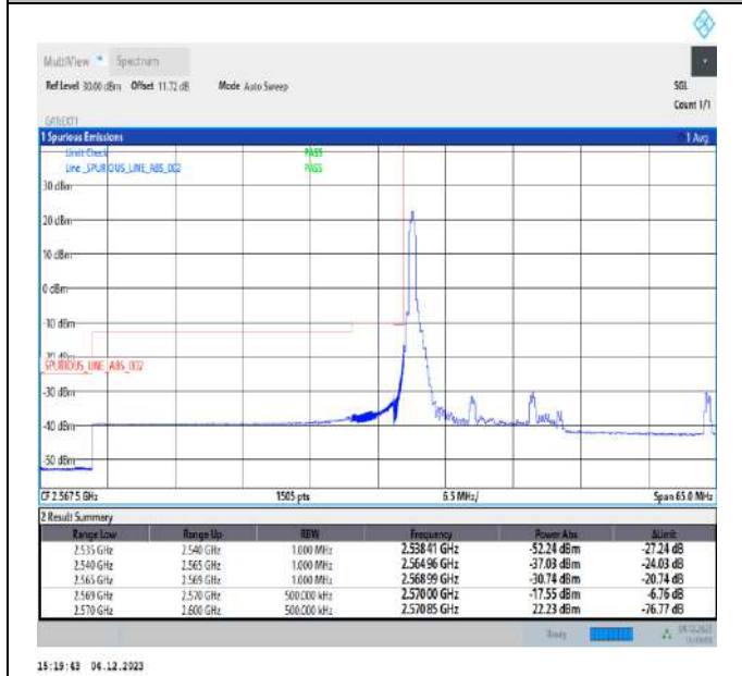
15MHz-15MHz_16QAM@16QAM-16QAM@16QAM_37825-37975_1RB#0@75RB#0-0RB#0@75RB#0
