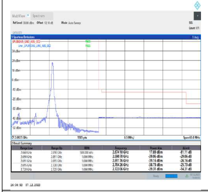
15MHz-15MHz_64QAM@64QAM-64QAM@64QAM_41365-41515_1RB#74@75RB#0-0RB#0@75RB#0
