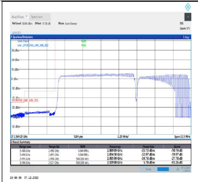
15MHz-10MHz_16QAM@16QAM-16QAM@16QAM_39725-39845_75RB#0@75RB#0-50RB#0@50RB#0
