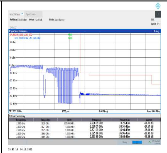
20MHz-20MHz_16QAM@16QAM-16QAM@16QAM_37952-38150_100RB#0@100RB#0-100RB#0@100RB#0
