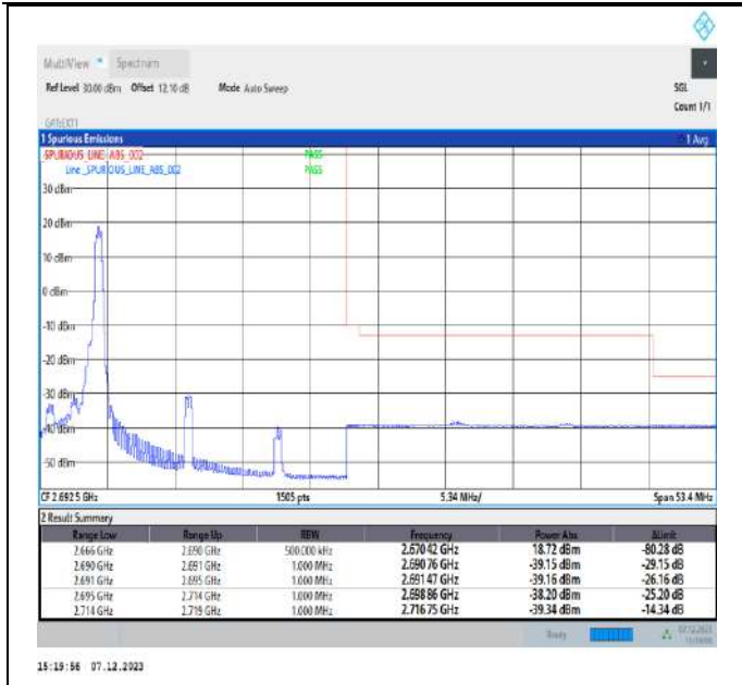
5MHz-20MHz_16QAM@16QAM-16QAM@16QAM_41373-41490_1RB#24@25RB#0-0RB#0@100RB#0
