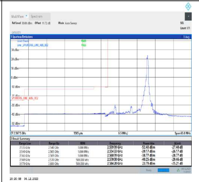
15MHz-15MHz_QPSK@QPSK-QPSK@QPSK_37825-37975_1RB#74@75RB#0-0RB#0@75RB#0
