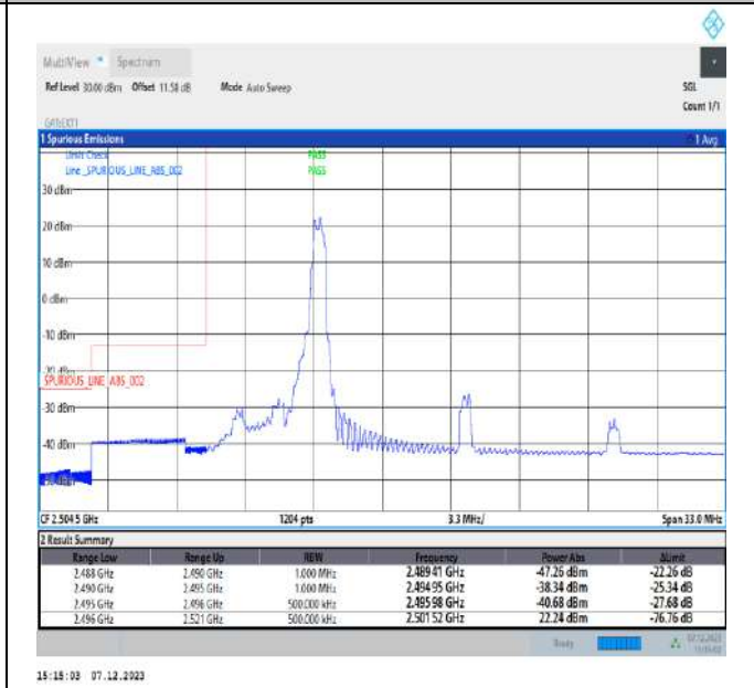
5MHz-20MHz_64QAM@64QAM-64QAM@64QAM_39683-39800_1RB#24@25RB#0-0RB#0@100RB#0
