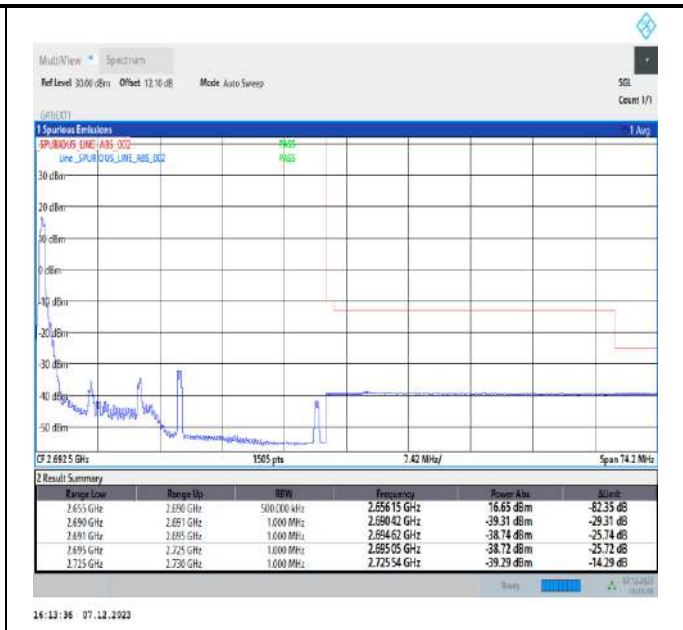
15MHz-20MHz_16QAM@16QAM-16QAM@16QAM_41319-41490_1RB#0@75RB#0-0RB#0@100RB#0
