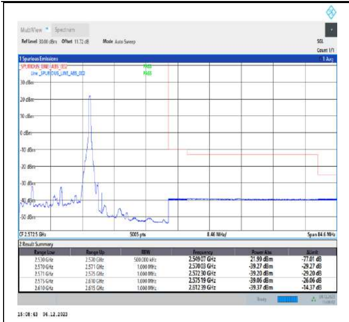
20MHz-20MHz_64QAM@64QAM-64QAM@64QAM_21152-21350_1RB#99@100RB#0-0RB#0@100RB#0
