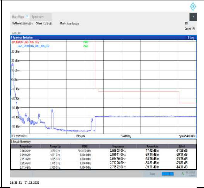
10MHz-15MHz_64QAM@64QAM-64QAM@64QAM_41395-41515_1RB#0@50RB#0-0RB#0@75RB#0
