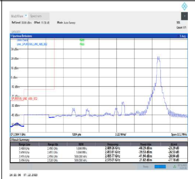
20MHz-5MHz_64QAM@64QAM-64QAM@64QAM_39750-39867_1RB#99@100RB#0-0RB#0@25RB#0
