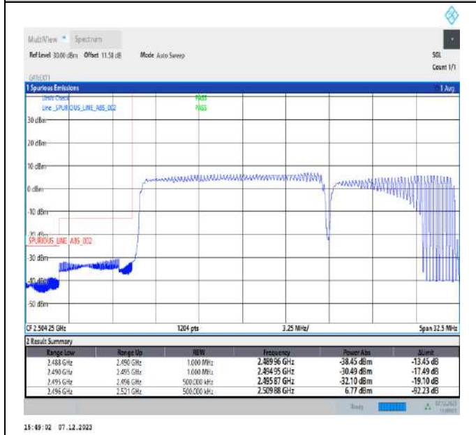
15MHz-10MHz_QPSK@QPSK-QPSK@QPSK_39725-39845_75RB#0@75RB#0-50RB#0@50RB#0
