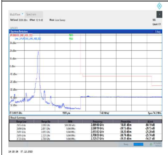
15MHz-20MHz_16QAM@16QAM-16QAM@16QAM_41319-41490_1RB#74@75RB#0-0RB#0@100RB#0
