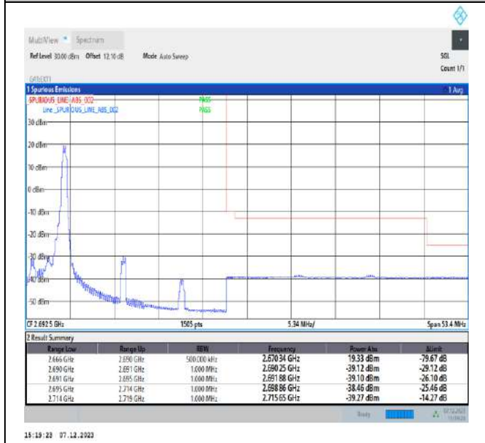
5MHz-20MHz_QPSK@QPSK-QPSK@QPSK_41373-41490_1RB#24@25RB#0-0RB#0@100RB#0
