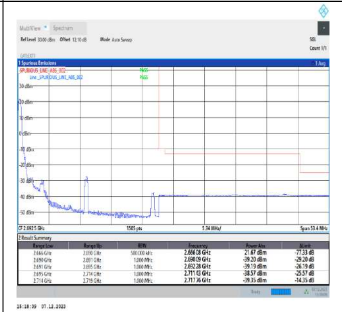
5MHz-20MHz_16QAM@16QAM-16QAM@16QAM_41373-41490_1RB#0@25RB#0-0RB#0@100RB#0
