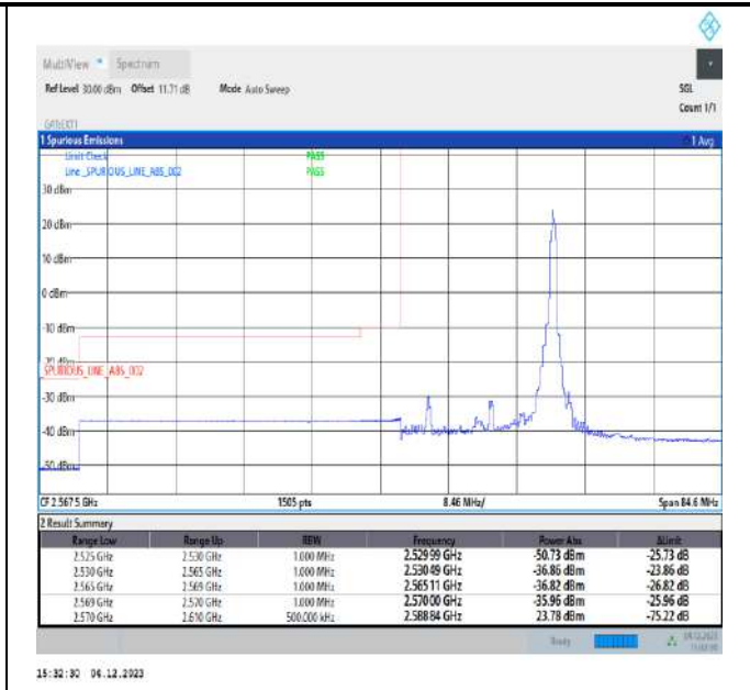
20MHz-20MHz_QPSK@QPSK-QPSK@QPSK_37850-38048_1RB#99@100RB#0-0RB#0@100RB#0
