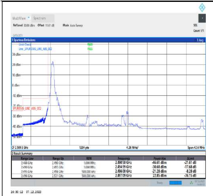
20MHz-15MHz_QPSK@QPSK-QPSK@QPSK_39750-39921_1RB#0@100RB#0-0RB#0@75RB#0
