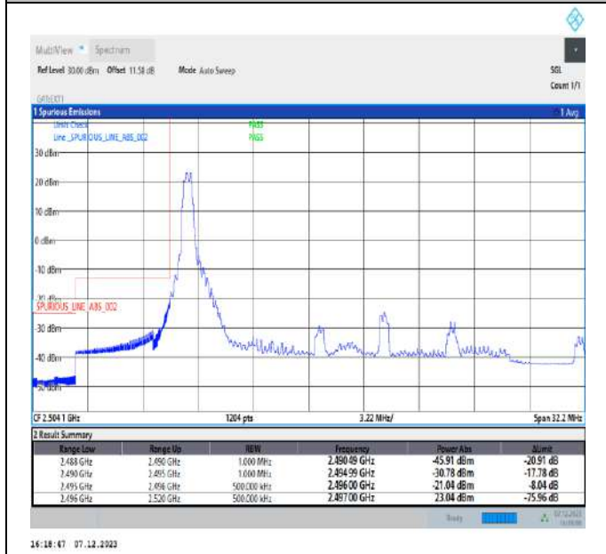
20MHz-5MHz_QPSK@QPSK-QPSK@QPSK_39750-39867_1RB#0@100RB#0-0RB#0@25RB#0
