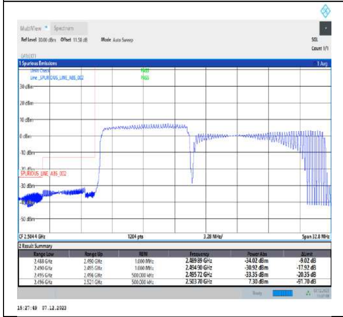
10MHz-15MHz_64QAM@64QAM-64QAM@64QAM_39703-39823_50RB#0@50RB#0-75RB#0@75RB#0
