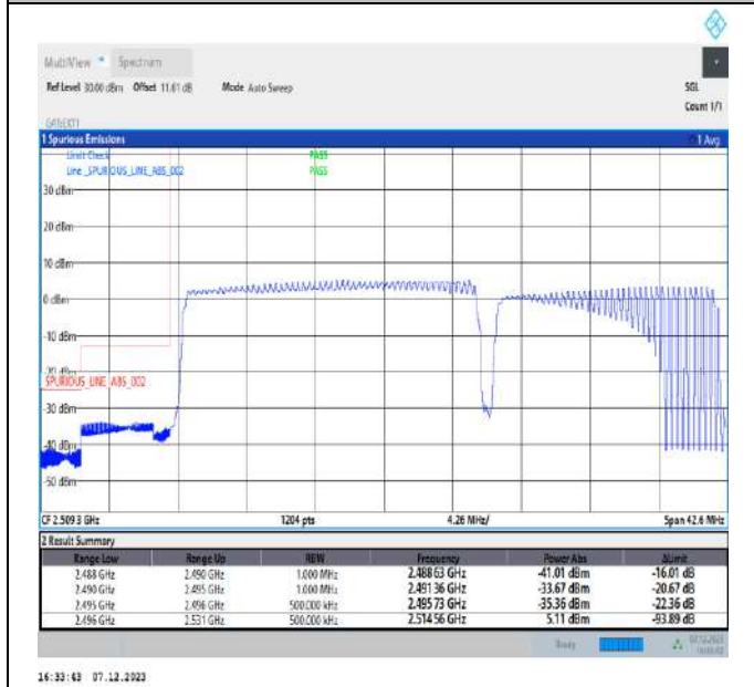
20MHz-15MHz_QPSK@QPSK-QPSK@QPSK_39750-39921_100RB#0@100RB#0-75RB#0@75RB#0
