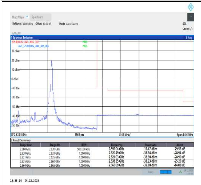
20MHz-20MHz_16QAM@16QAM-16QAM@16QAM_37952-38150_1RB#99@100RB#0-0RB#0@100RB#0
