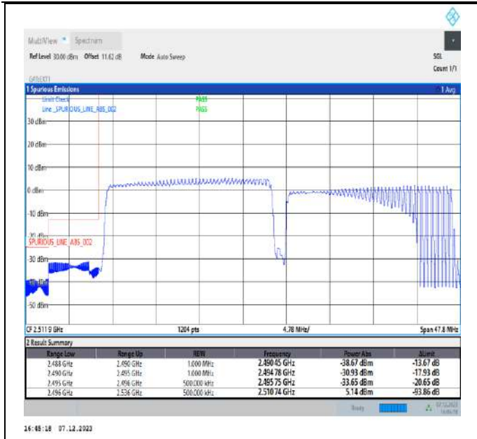
20MHz-20MHz_QPSK@QPSK-QPSK@QPSK_39750-39948_100RB#0@100RB#0-100RB#0@100RB#0
