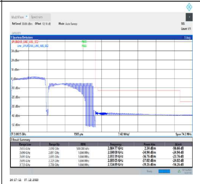
15MHz-20MHz_16QAM@16QAM-16QAM@16QAM_41319-41490_75RB#0@75RB#0-100RB#0@100RB#0
