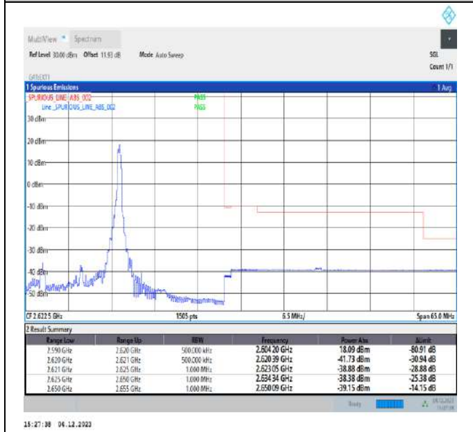
15MHz-15MHz_64QAM@64QAM-64QAM@64QAM_38025-38175_1RB#74@75RB#0-0RB#0@75RB#0
