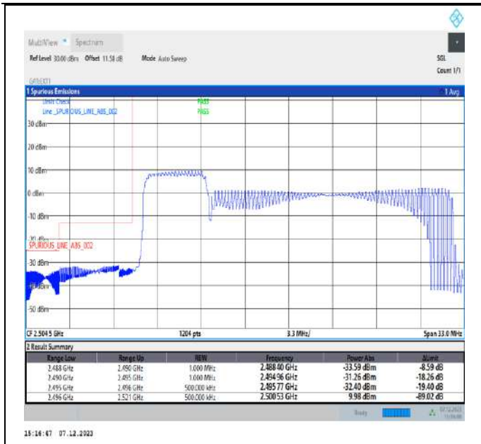
5MHz-20MHz_64QAM@64QAM-64QAM@64QAM_39683-39800_25RB#0@25RB#0-100RB#0@100RB#0
