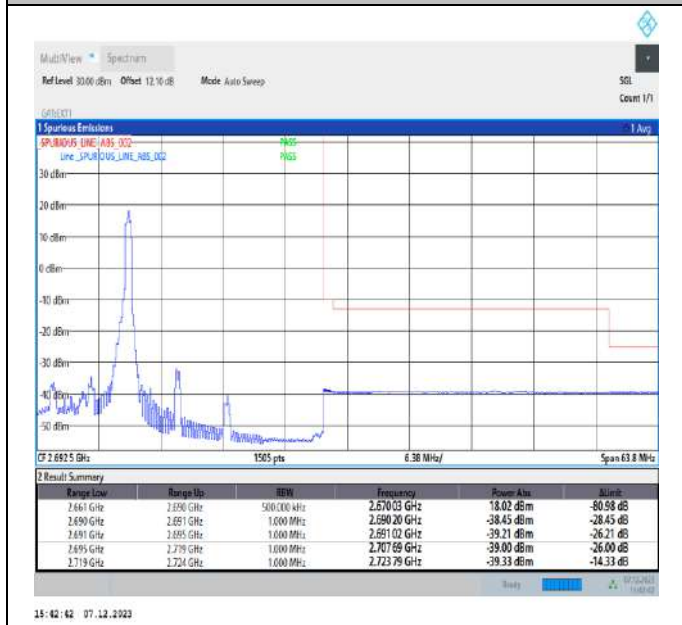
10MHz-20MHz_64QAM@64QAM-64QAM@64QAM_41346-41490_1RB#49@50RB#0-0RB#0@100RB#0
