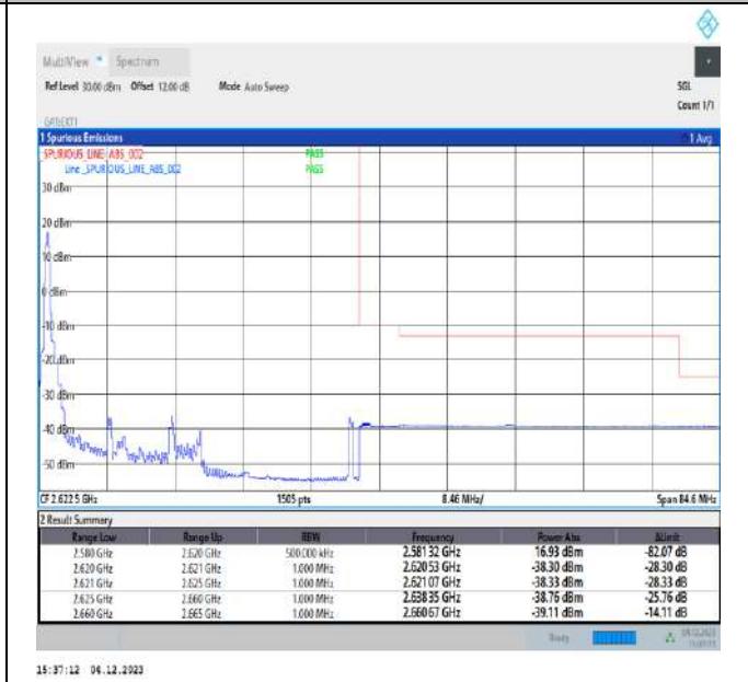
20MHz-20MHz_64QAM@64QAM-64QAM@64QAM_37952-38150_1RB#0@100RB#0-0RB#0@100RB#0
