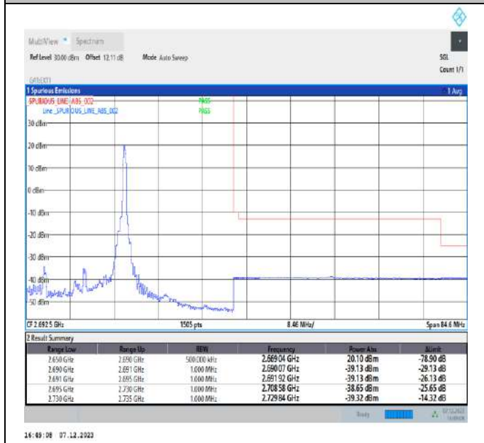
20MHz-20MHz_QPSK@QPSK-QPSK@QPSK_41292-41490_1RB#99@100RB#0-0RB#0@100RB#0
