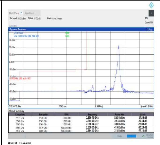
15MHz-15MHz_64QAM@64QAM-64QAM@64QAM_37825-37975_1RB#74@75RB#0-0RB#0@75RB#0
