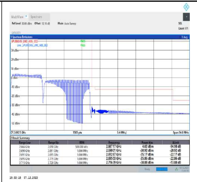
10MHz-15MHz_64QAM@64QAM-64QAM@64QAM_41395-41515_50RB#0@50RB#0-75RB#0@75RB#0
