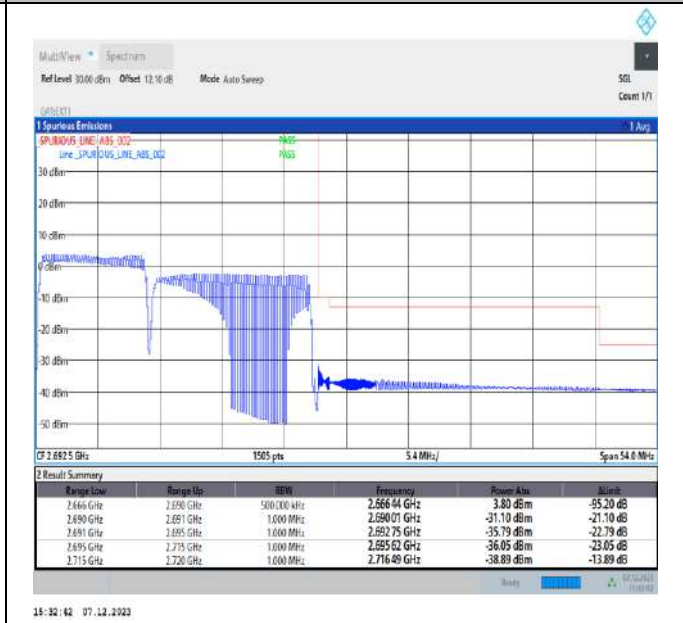
10MHz-15MHz_16QAM@16QAM-16QAM@16QAM_41395-41515_50RB#0@50RB#0-75RB#0@75RB#0
