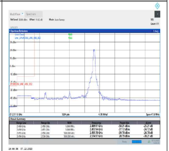
20MHz-20MHz_64QAM@64QAM-64QAM@64QAM_39750-39948_1RB#99@100RB#0-0RB#0@100RB#0
