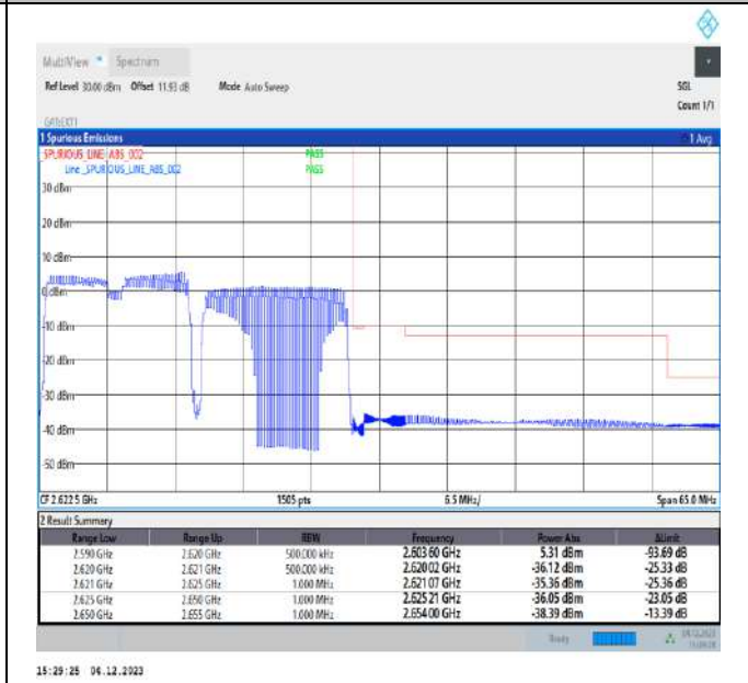
15MHz-15MHz_64QAM@64QAM-64QAM@64QAM_38025-38175_75RB#0@75RB#0-75RB#0@75RB#0
