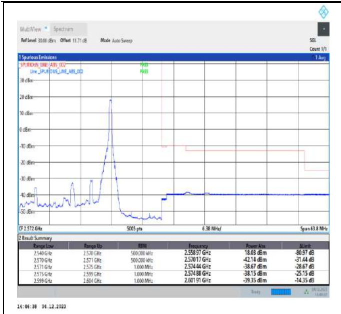
20MHz-10MHz_64QAM@64QAM-64QAM@64QAM_21251-21395_1RB#99@100RB#0-0RB#0@50RB#0
