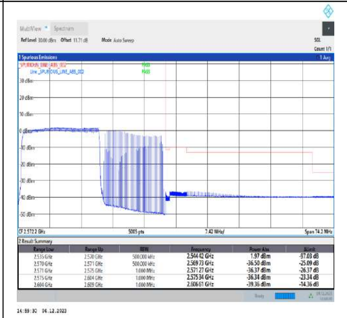
20MHz-15MHz_64QAM@64QAM-64QAM@64QAM_21201-21372_100RB#0@100RB#0-75RB#0@75RB#0
