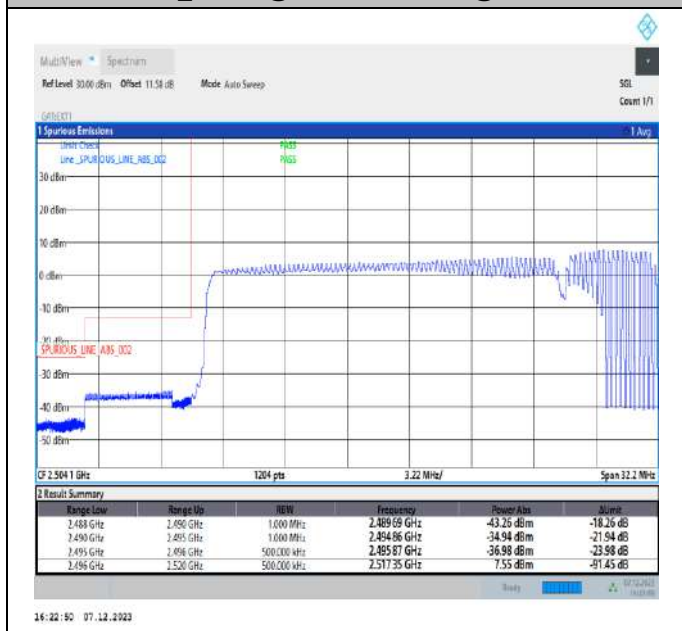
20MHz-5MHz_16QAM@16QAM-16QAM@16QAM_39750-39867_100RB#0@100RB#0-25RB#0@25RB#0
