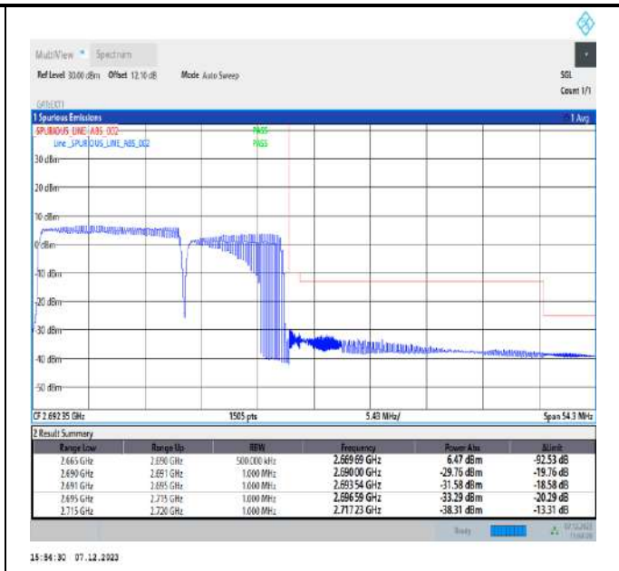
15MHz-10MHz_QPSK@QPSK-QPSK@QPSK_41417-41537_75RB#0@75RB#0-50RB#0@50RB#0
