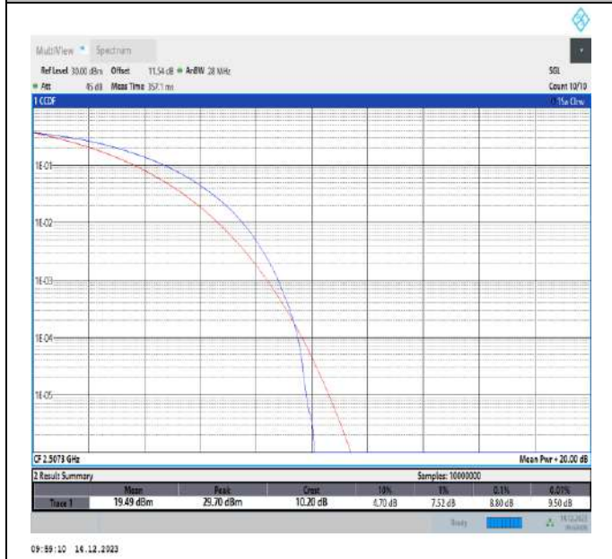
41-41-10MHz-15MHz-64QAM-64QAM-39703-39823-50RB#0-75RB#0-PASS
