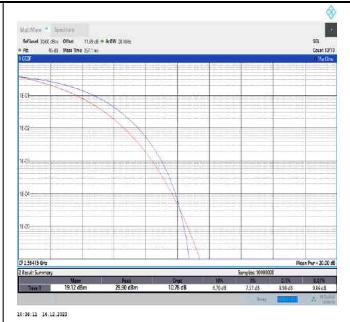
41-41-20MHz-15MHz-64QAM-64QAM-40546-40717-100RB#0-75RB#0-PASS
