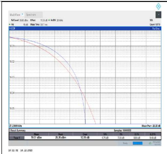
41-41-15MHz-10MHz-64QAM-64QAM-39725-39845-75RB#0-50RB#0-PASS
