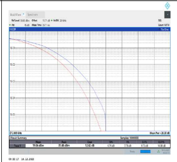
38-38-15MHz-15MHz-16QAM-16QAM-38025-38175-75RB#0-75RB#0-PASS
