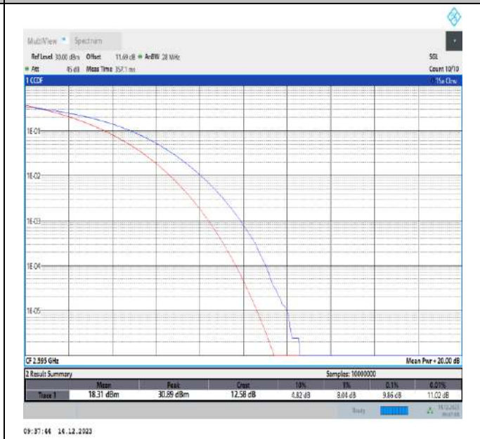
38-38-20MHz-20MHz-64QAM-64QAM-37901-38099-100RB#0-100RB#0-PASS
