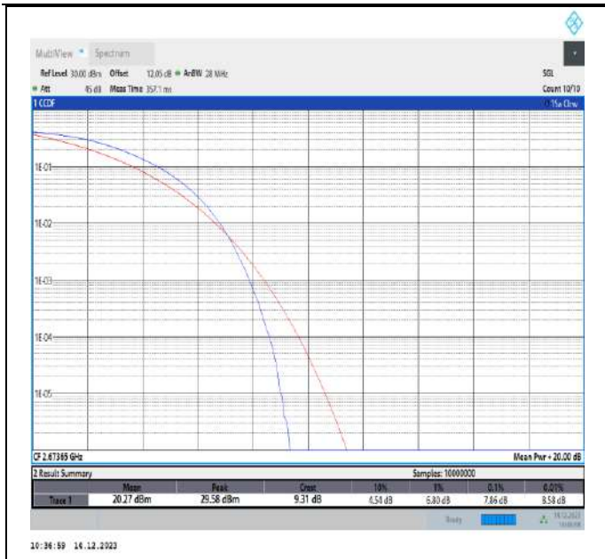
41-41-20MHz-15MHz-QPSK-QPSK-41341-41512-100RB#0-75RB#0-PASS
