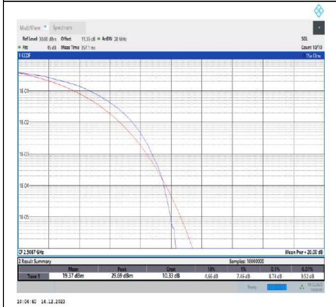
41-41-10MHz-20MHz-16QAM-16QAM-39705-39849-50RB#0-100RB#0-PASS
