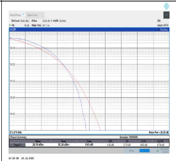
41-41-15MHz-15MHz-QPSK-QPSK-41365-41515-75RB#0-75RB#0-PASS
