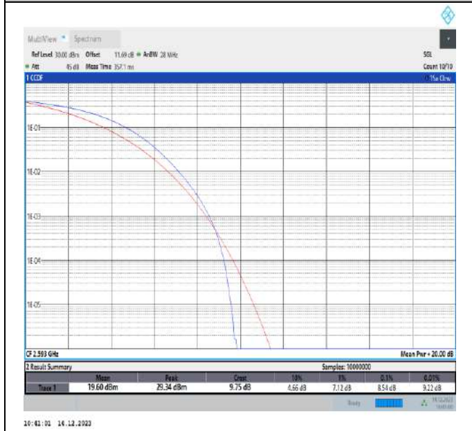
41-41-20MHz-20MHz-QPSK-QPSK-40521-40719-100RB#0-100RB#0-PASS
