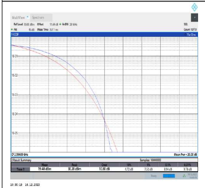
41-41-20MHz-5MHz-64QAM-64QAM-40595-40712-100RB#0-25RB#0-PASS
