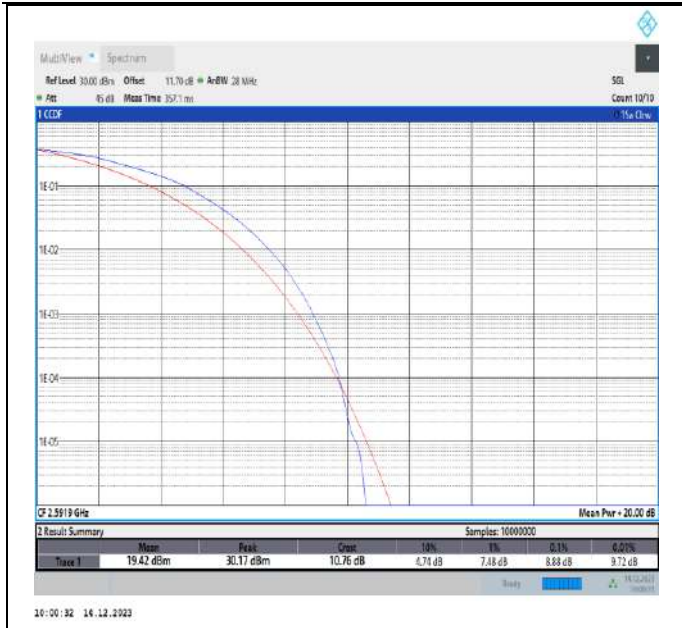
41-41-10MHz-15MHz-16QAM-16QAM-40549-40669-50RB#0-75RB#0-PASS
