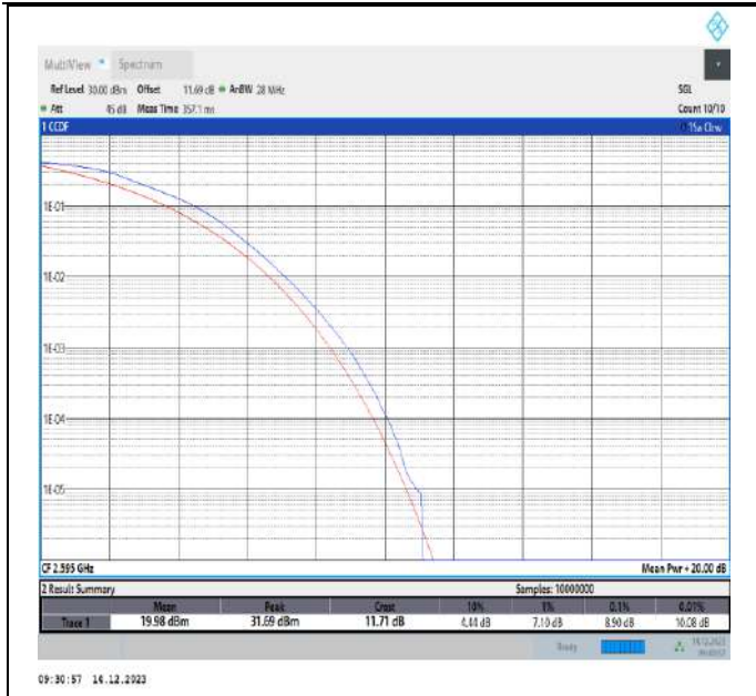
38-38-15MHz-15MHz-QPSK-QPSK-37925-38075-75RB#0-75RB#0-PASS
