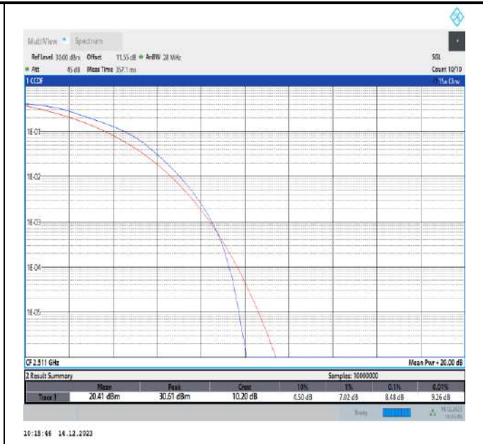
41-41-15MHz-15MHz-QPSK-QPSK-39725-39875-75RB#0-75RB#0-PASS
