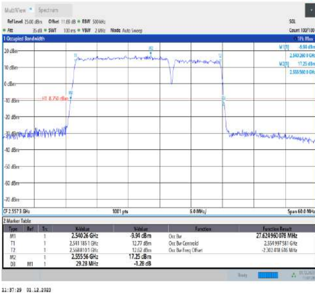
7-7-20MHz-10MHz-16QAM-16QAM-21251-21395-100RB#0-50RB#0-PASS
