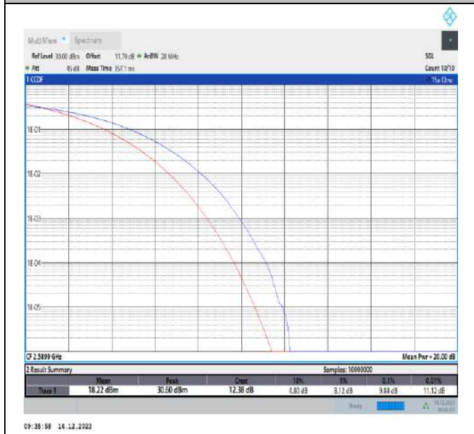
38-38-20MHz-20MHz-64QAM-64QAM-37850-38048-100RB#0-100RB#0-PASS
