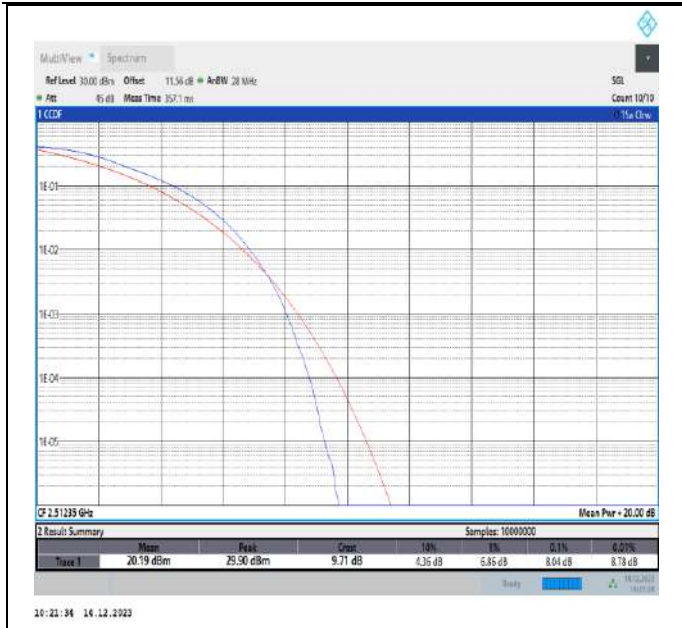
41-41-15MHz-20MHz-QPSK-QPSK-39728-39899-75RB#0-100RB#0-PASS
