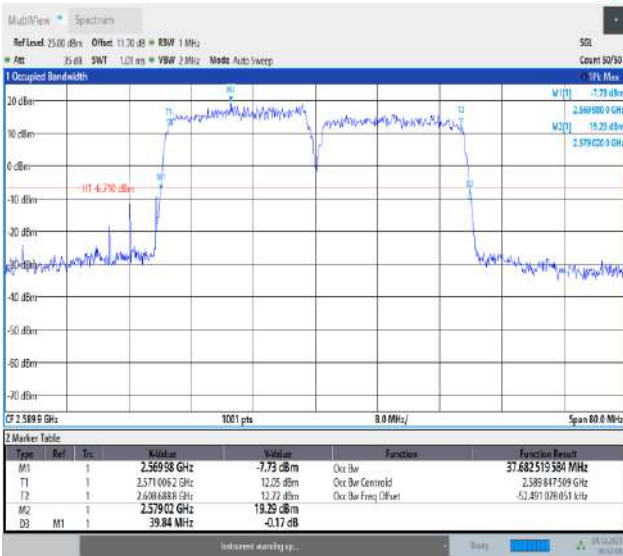
38-38-20MHz-20MHz-QPSK-QPSK-37850-38048-100RB#0-100RB#0-PASS
