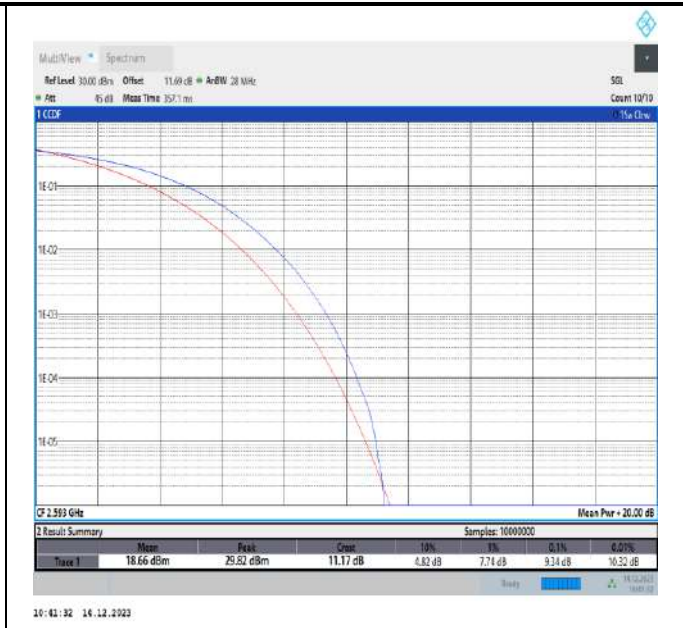
41-41-20MHz-20MHz-16QAM-16QAM-40521-40719-100RB#0-100RB#0-PASS
