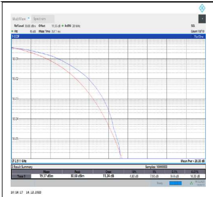
41-41-15MHz-15MHz-16QAM-16QAM-39725-39875-75RB#0-75RB#0-PASS
