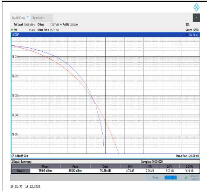
41-41-20MHz-5MHz-16QAM-16QAM-41440-41557-100RB#0-25RB#0-PASS
