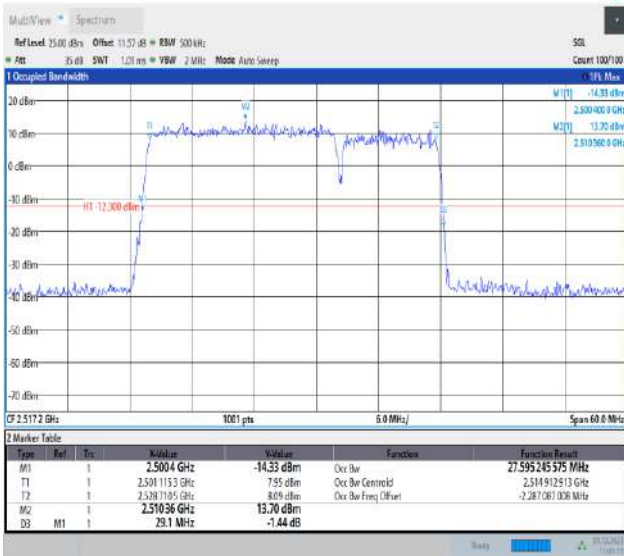
7-7-20MHz-10MHz-QPSK-QPSK-20850-20994-100RB#0-50RB#0-PASS
