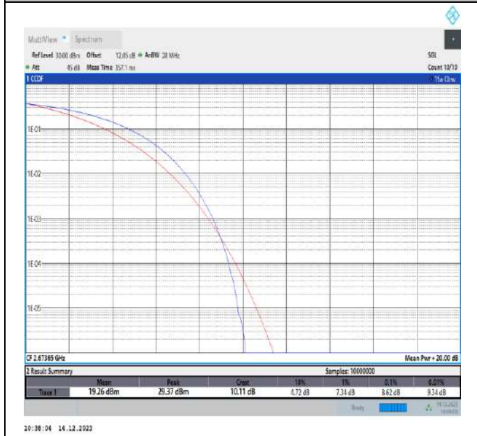
41-41-20MHz-15MHz-64QAM-64QAM-41341-41512-100RB#0-75RB#0-PASS
