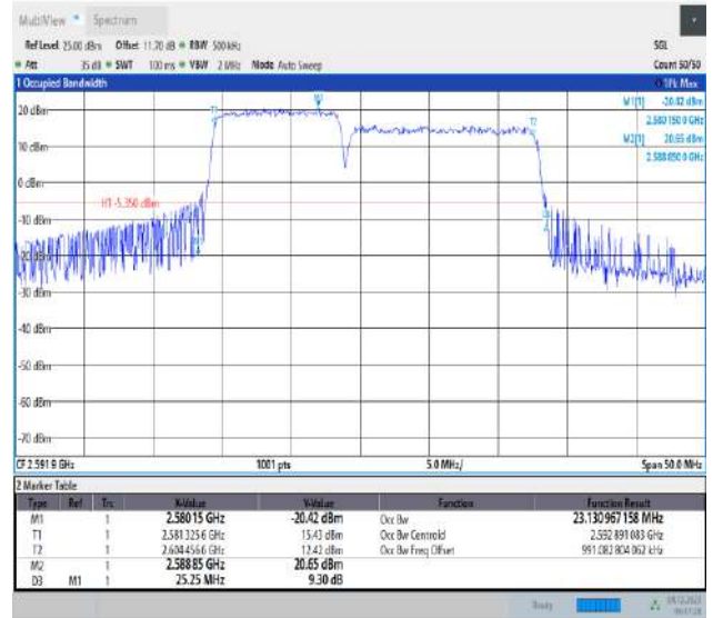
41-41-10MHz-15MHz-QPSK-QPSK-40549-40669-50RB#0-75RB#0-PASS
