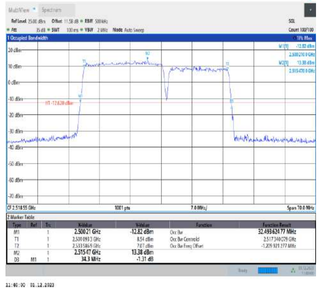
7-7-20MHz-15MHz-16QAM-16QAM-20850-21021-100RB#0-75RB#0-PASS
