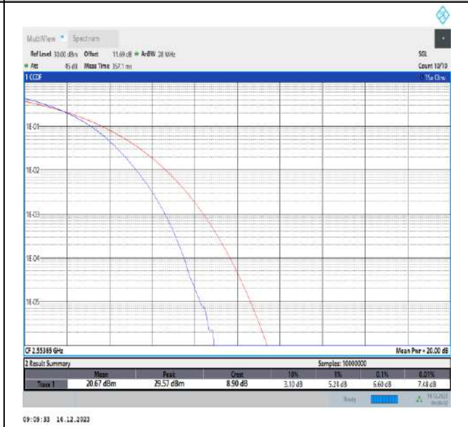
7-7-20MHz-15MHz-64QAM-64QAM-21201-21372-100RB#0-75RB#0-PASS
