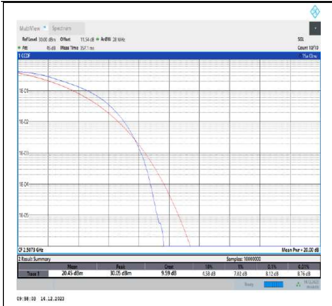
41-41-10MHz-15MHz-QPSK-QPSK-39703-39823-50RB#0-75RB#0-PASS
