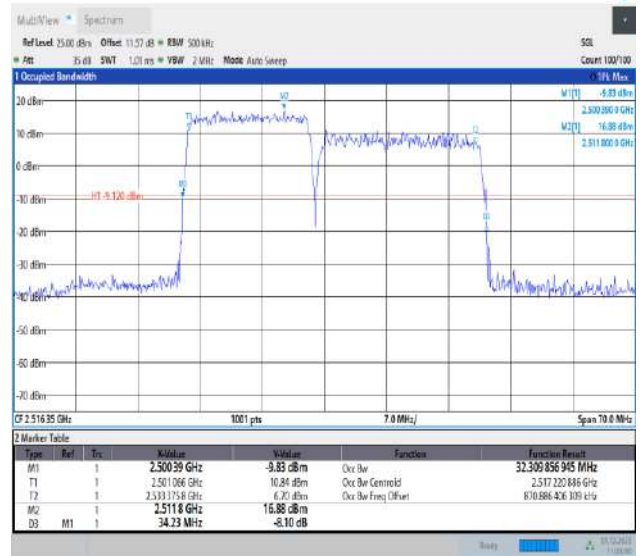
7-7-15MHz-20MHz-QPSK-QPSK-20828-20999-75RB#0-100RB#0-PASS
