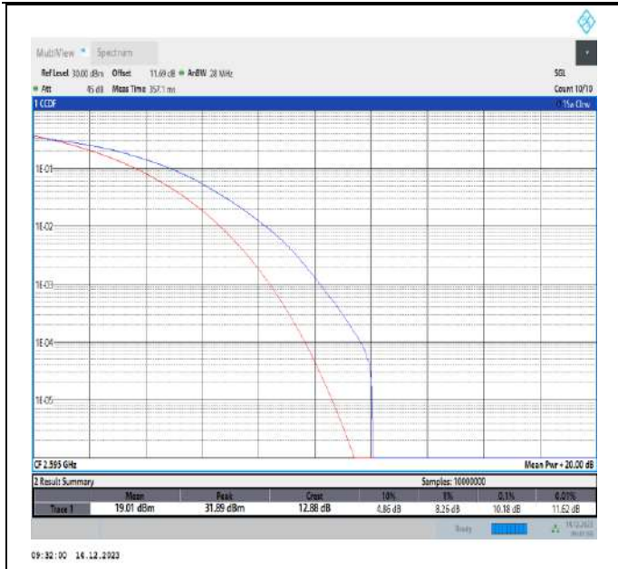
38-38-15MHz-15MHz-64QAM-64QAM-37925-38075-75RB#0-75RB#0-PASS
