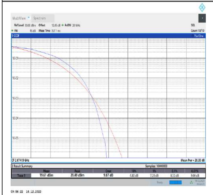
41-41-5MHz-20MHz-16QAM-16QAM-41373-41490-25RB#0-100RB#0-PASS
