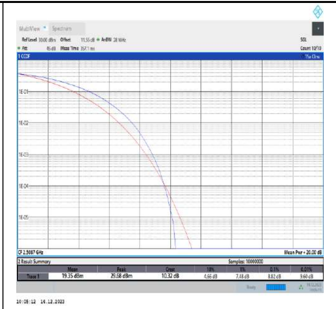
41-41-10MHz-20MHz-64QAM-64QAM-39705-39849-50RB#0-100RB#0-PASS
