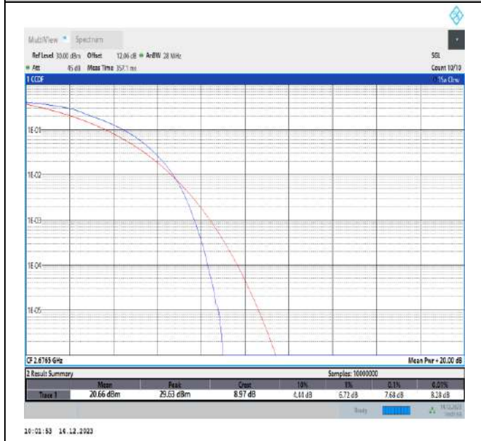
41-41-10MHz-15MHz-QPSK-QPSK-41395-41515-50RB#0-75RB#0-PASS
