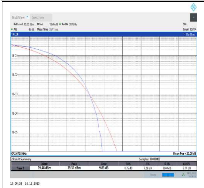
41-41-10MHz-20MHz-16QAM-16QAM-41346-41490-50RB#0-100RB#0-PASS
