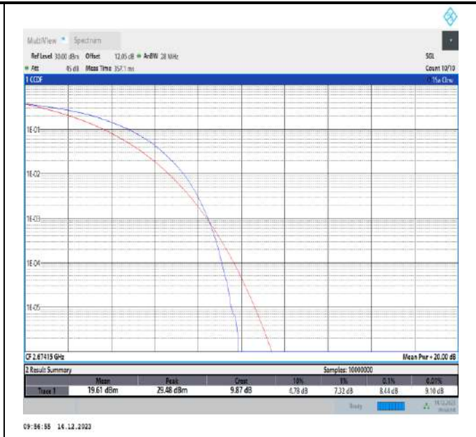
41-41-5MHz-20MHz-64QAM-64QAM-41373-41490-25RB#0-100RB#0-PASS
