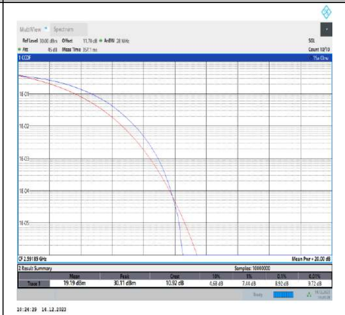
41-41-15MHz-20MHz-64QAM-64QAM-40523-40694-75RB#0-100RB#0-PASS
