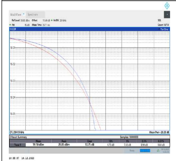
41-41-20MHz-15MHz-16QAM-16QAM-40546-40717-100RB#0-75RB#0-PASS
