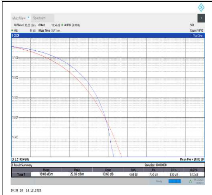
41-41-20MHz-15MHz-64QAM-64QAM-39750-39921-100RB#0-75RB#0-PASS
