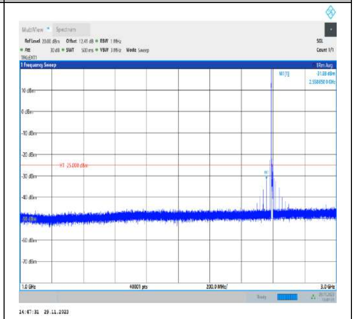
Band41_10MHz_QPSK_40620_1RB#0_1000~3000_1000~3000
