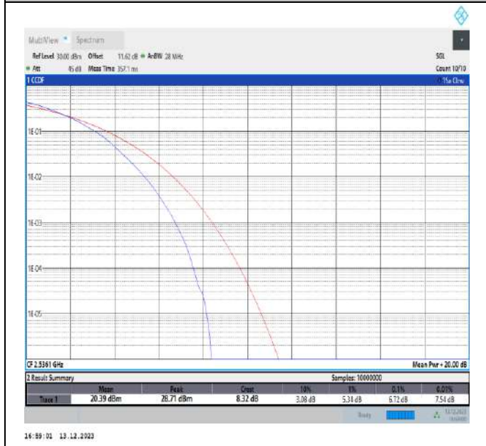
7-7-15MHz-10MHz-64QAM-64QAM-21051-21171-75RB#0-50RB#0-PASS
