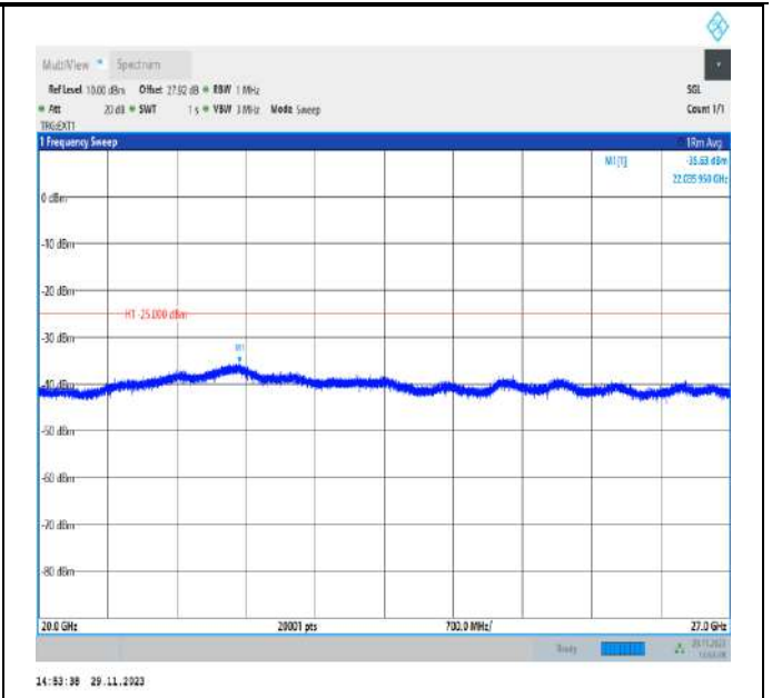
Band41_20MHz_QPSK_41490_1RB#0_20000~27000_2000~27000
