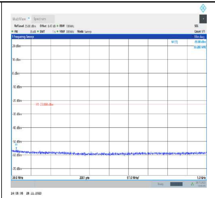
Band66_15MHz_QPSK_132322_1RB#0_30~1000_30~1000
