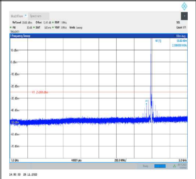
Band41_15MHz_QPSK_40620_1RB#0_1000~3000_1000~3000
