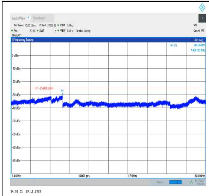
Band41_20MHz_QPSK_39750_1RB#0_3000~20000_3000~20000
