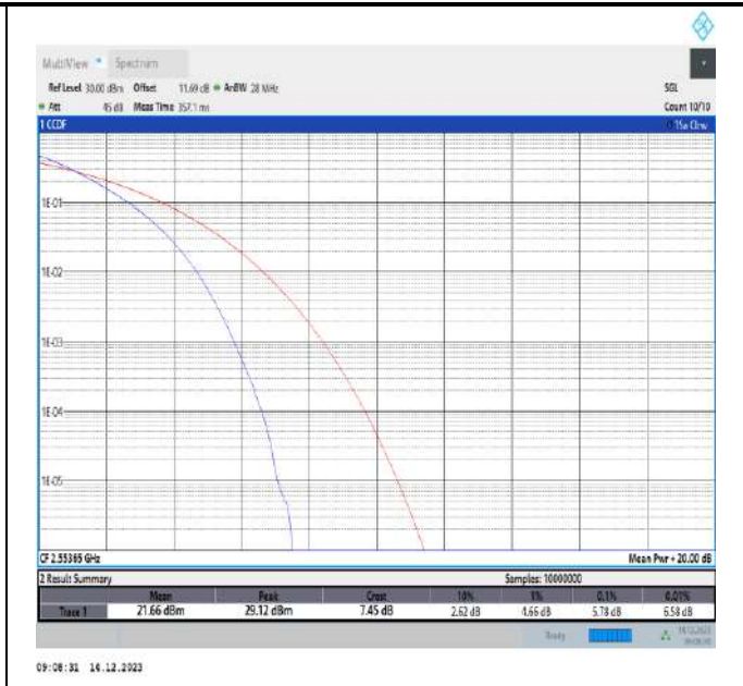
7-7-20MHz-15MHz-QPSK-QPSK-21201-21372-100RB#0-75RB#0-PASS
