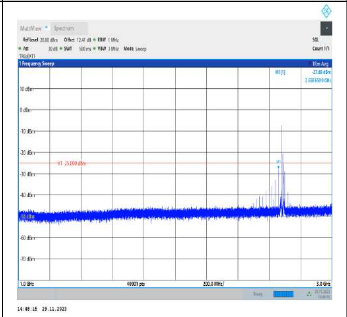
Band41_10MHz_QPSK_41540_1RB#0_1000~3000_1000~3000
