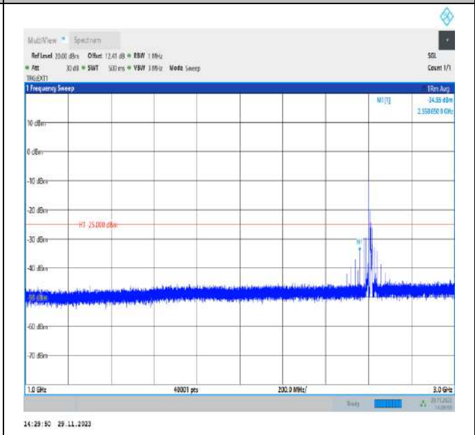
Band38_20MHz_QPSK_38150_1RB#0_1000~3000_1000~3000
