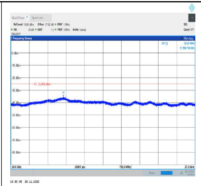
Band38_20MHz_QPSK_38150_1RB#0_20000~27000_2000~27000
