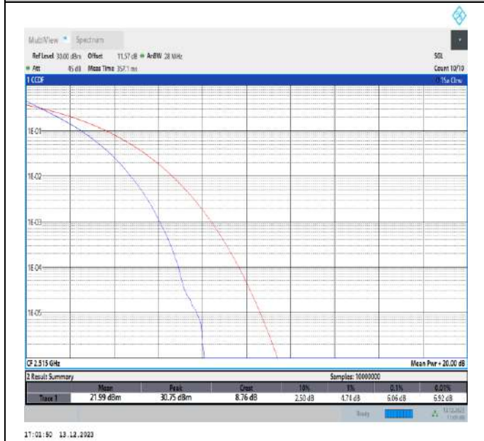
7-7-15MHz-15MHz-QPSK-QPSK-20825-20975-75RB#0-75RB#0-PASS
