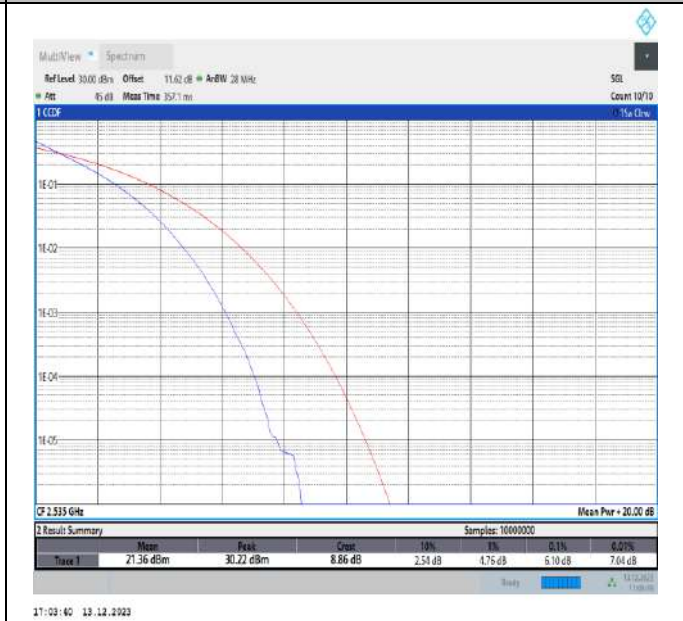
7-7-15MHz-15MHz-QPSK-QPSK-21025-21175-75RB#0-75RB#0-PASS
