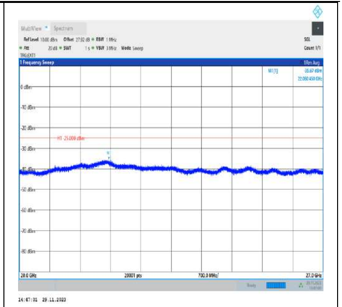
Band41_10MHz_QPSK_39700_1RB#0_20000~27000_20000~27000
