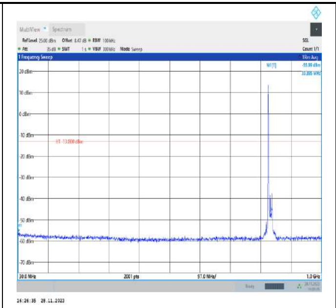
Band26_15MHz_QPSK_26915_1RB#0_30~1000_30~1000
