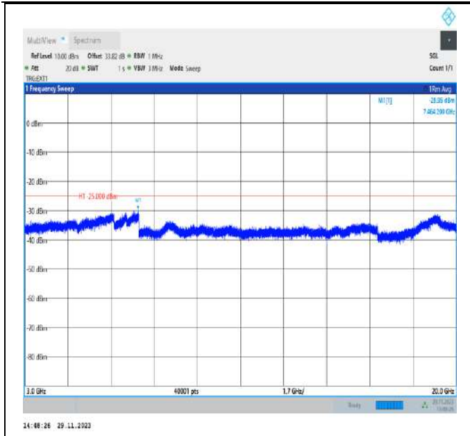
Band41_10MHz_QPSK_41540_1RB#0_3000~20000_3000~20000
