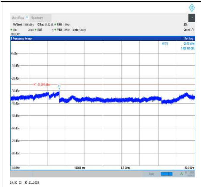
Band41_5MHz_QPSK_40620_1RB#0_3000~20000_3000~20000
