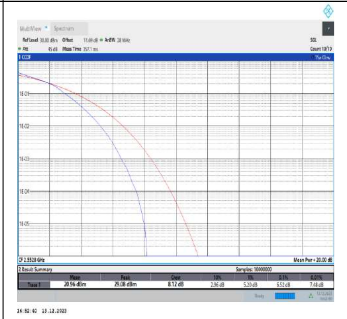
7-7-10MHz-20MHz-16QAM-16QAM-21206-21350-50RB#0-100RB#0-PASS
