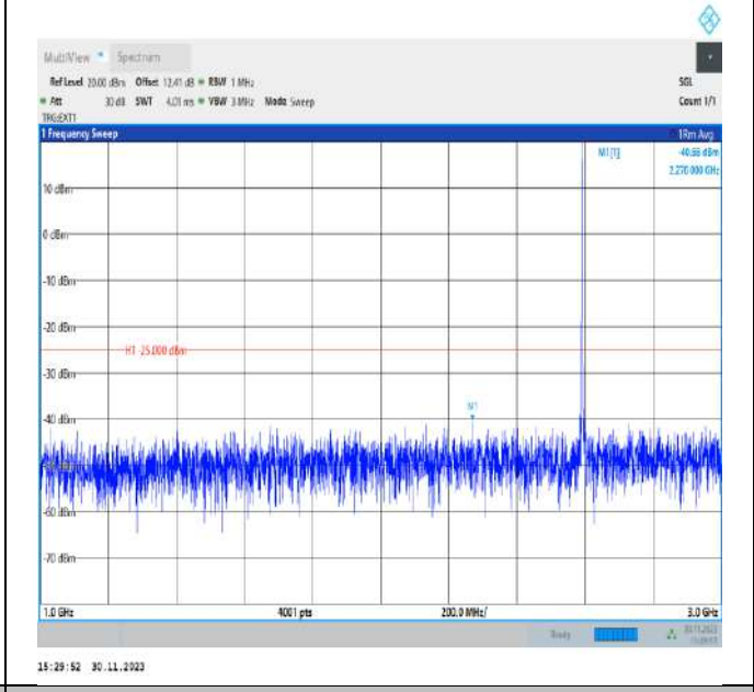
Band41_5MHz_QPSK_40620_1RB#0_1000~3000_1000~3000
