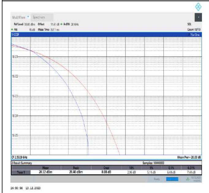
7-7-10MHz-20MHz-16QAM-16QAM-21006-21150-50RB#0-100RB#0-PASS
