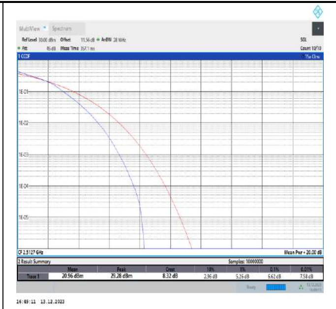
7-7-10MHz-20MHz-16QAM-16QAM-20805-20949-50RB#0-100RB#0-PASS
