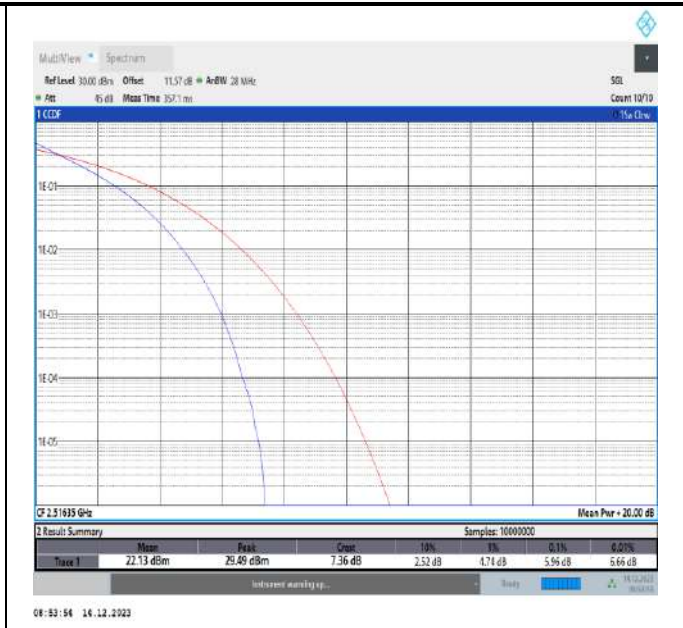
7-7-15MHz-20MHz-QPSK-QPSK-20828-20999-75RB#0-100RB#0-PASS
