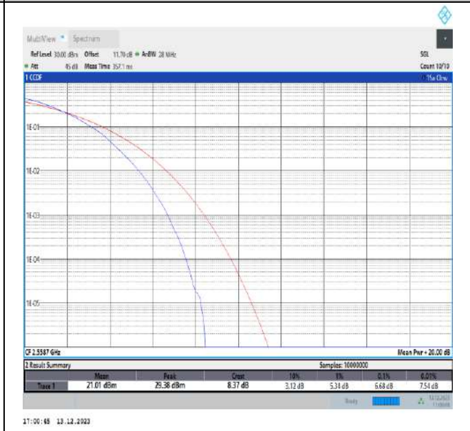
7-7-15MHz-10MHz-64QAM-64QAM-21277-21397-75RB#0-50RB#0-PASS
