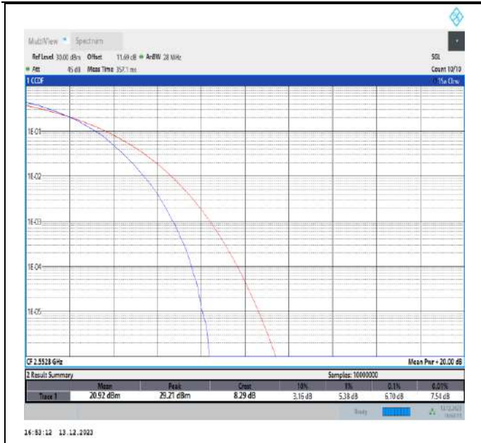
7-7-10MHz-20MHz-64QAM-64QAM-21206-21350-50RB#0-100RB#0-PASS
