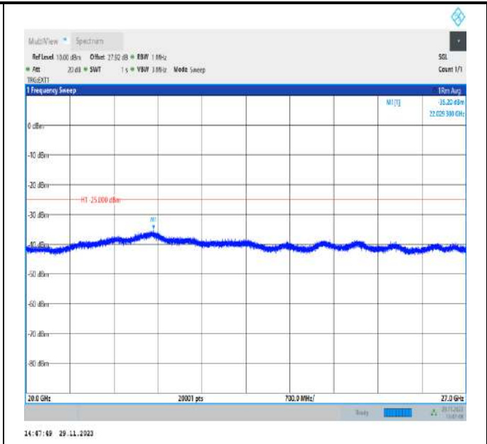
Band41_10MHz_QPSK_40620_1RB#0_20000~27000_20000~27000
