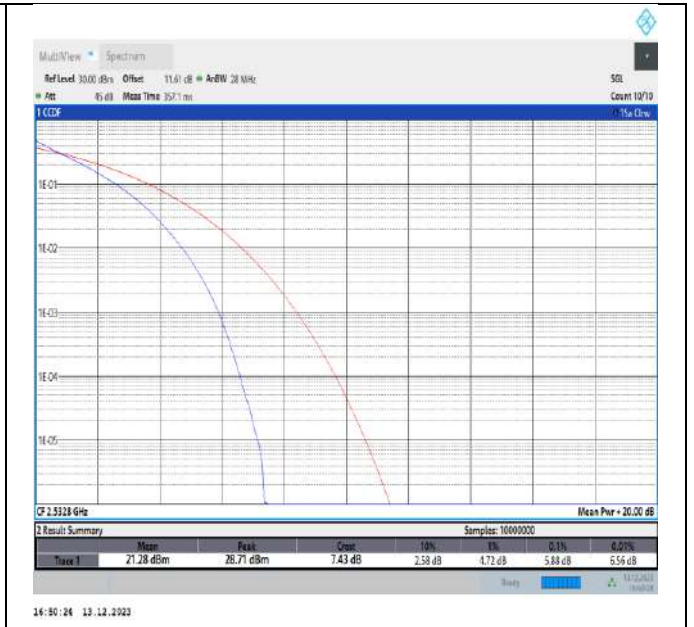
7-7-10MHz-20MHz-QPSK-QPSK-21006-21150-50RB#0-100RB#0-PASS
