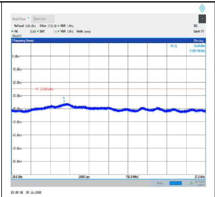
Band41_5MHz_QPSK_39675_1RB#0_20000~27000_20000~27000
