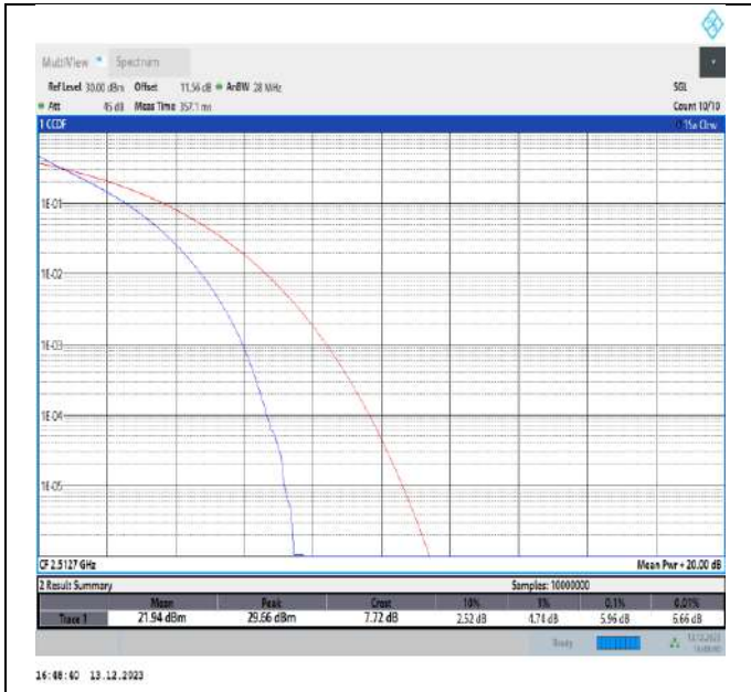
7-7-10MHz-20MHz-QPSK-QPSK-20805-20949-50RB#0-100RB#0-PASS
