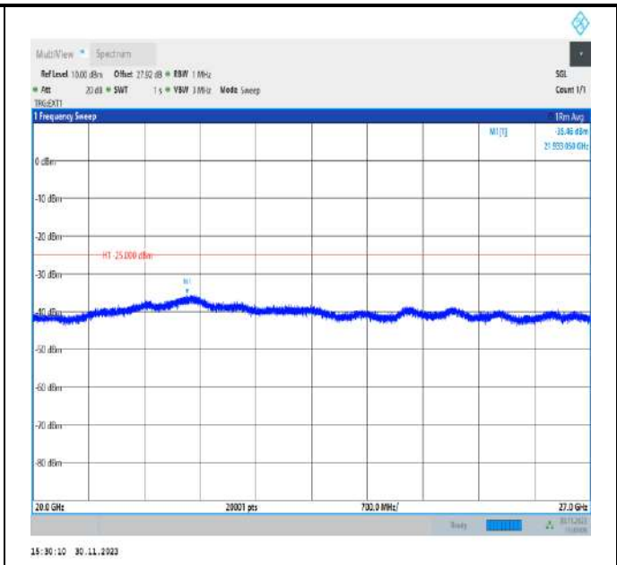
Band41_5MHz_QPSK_40620_1RB#0_20000~27000_20000~27000
