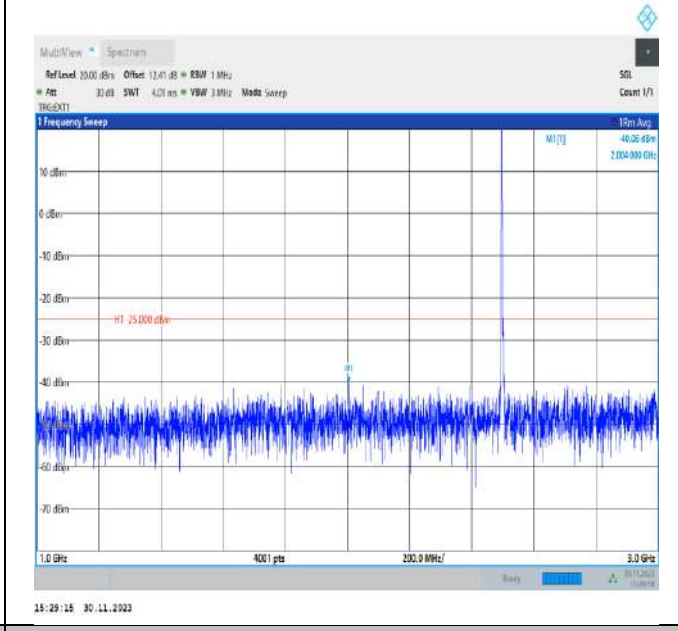
Band41_5MHz_QPSK_39675_1RB#0_1000~3000_1000~3000
