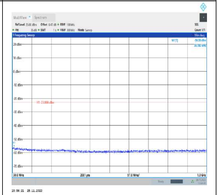
Band66_3MHz_QPSK_131987_1RB#0_30~1000_30~1000
