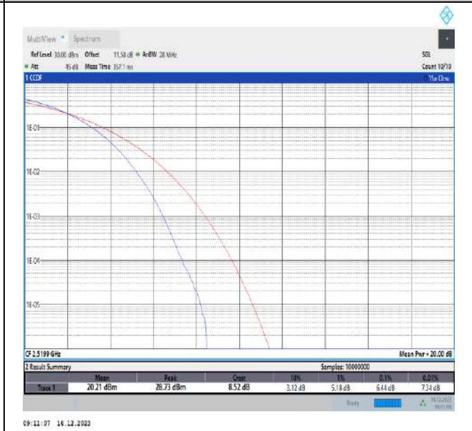
7-7-20MHz-20MHz-16QAM-16QAM-20850-21048-100RB#0-100RB#0-PASS
