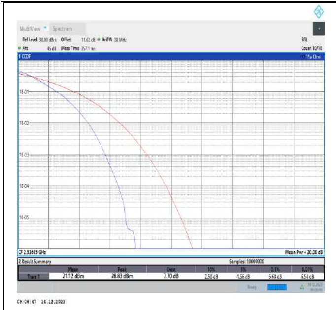
7-7-20MHz-15MHz-QPSK-QPSK-21026-21197-100RB#0-75RB#0-PASS
