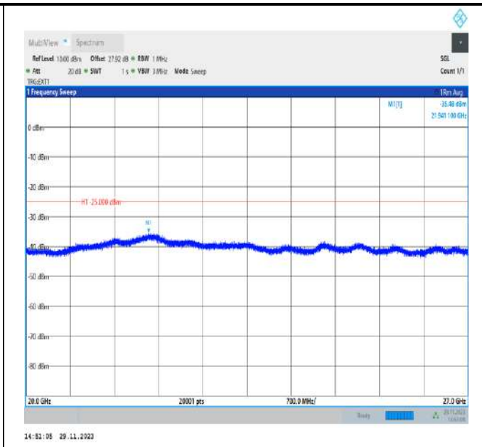
Band41_15MHz_QPSK_41515_1RB#0_20000~27000_2000~27000
