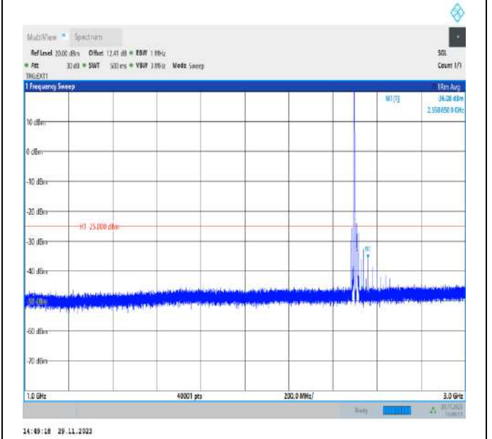
Band41_15MHz_QPSK_39725_1RB#0_1000~3000_1000~3000
