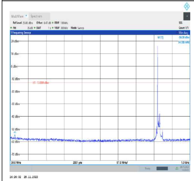
Band26_15MHz_QPSK_26865_1RB#0_30~1000_30~1000
