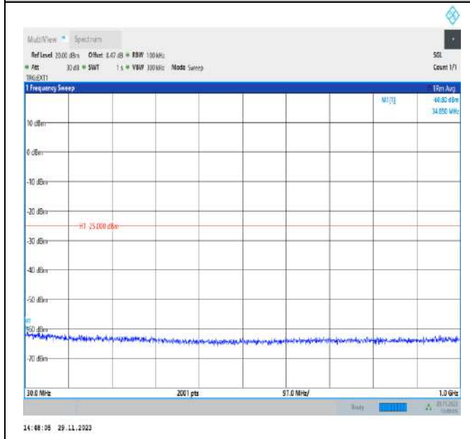
Band41_10MHz_QPSK_41540_1RB#0_30~1000_30~1000
