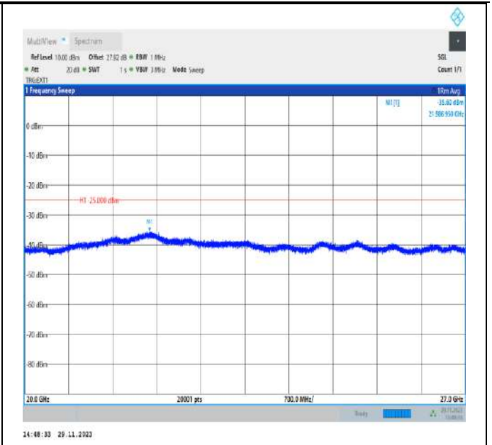
Band41_10MHz_QPSK_41540_1RB#0_20000~27000_2000~27000
