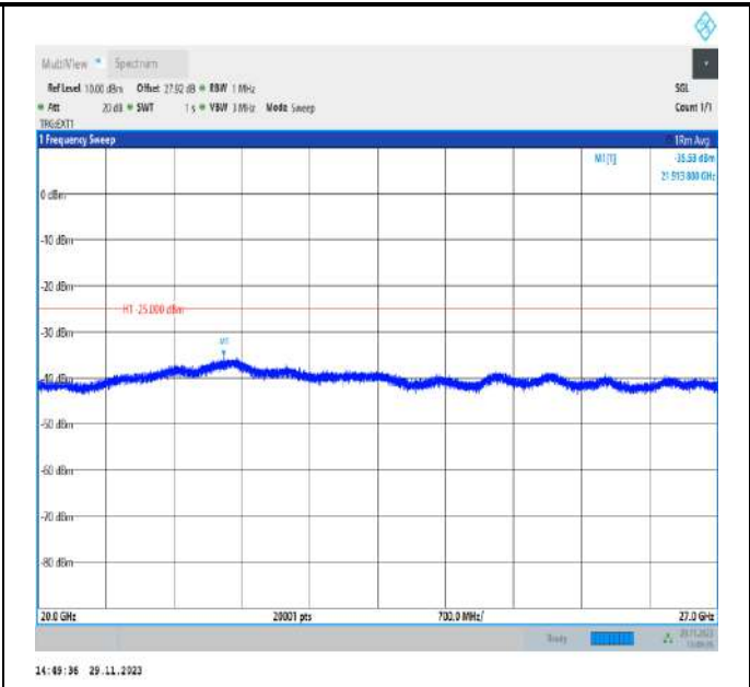
Band41_15MHz_QPSK_39725_1RB#0_20000~27000_20000~27000
