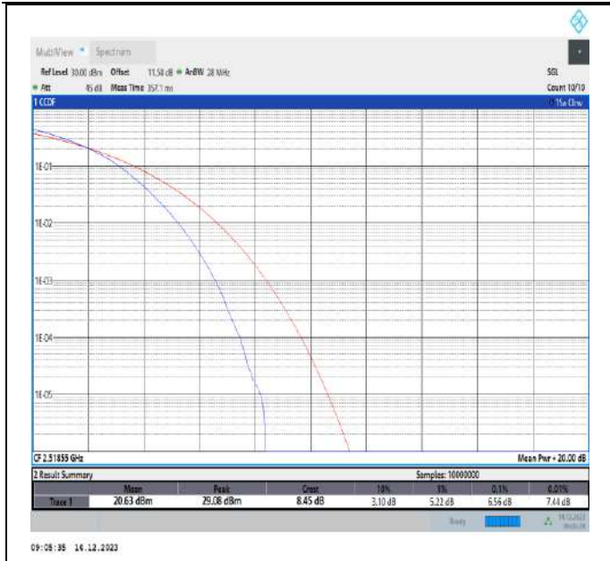
7-7-20MHz-15MHz-16QAM-16QAM-20850-21021-100RB#0-75RB#0-PASS
