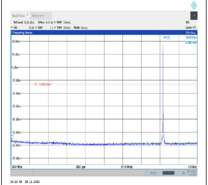
Band26_3MHz_QPSK_26775_1RB#0_30~1000_30~1000
