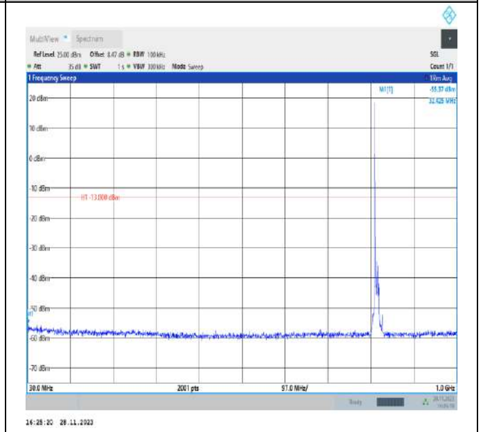
Band26_10MHz_QPSK_26740_1RB#0_30~1000_30~1000
