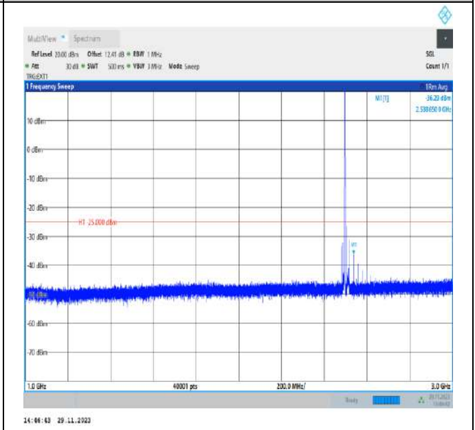
Band41_10MHz_QPSK_39700_1RB#0_1000~3000_1000~3000
