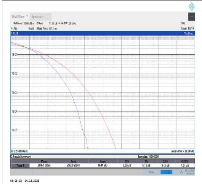
7-7-20MHz-15MHz-16QAM-16QAM-21201-21372-100RB#0-75RB#0-PASS
