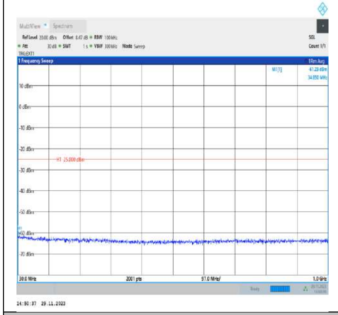
Band41_15MHz_QPSK_41515_1RB#0_30~1000_30~1000
