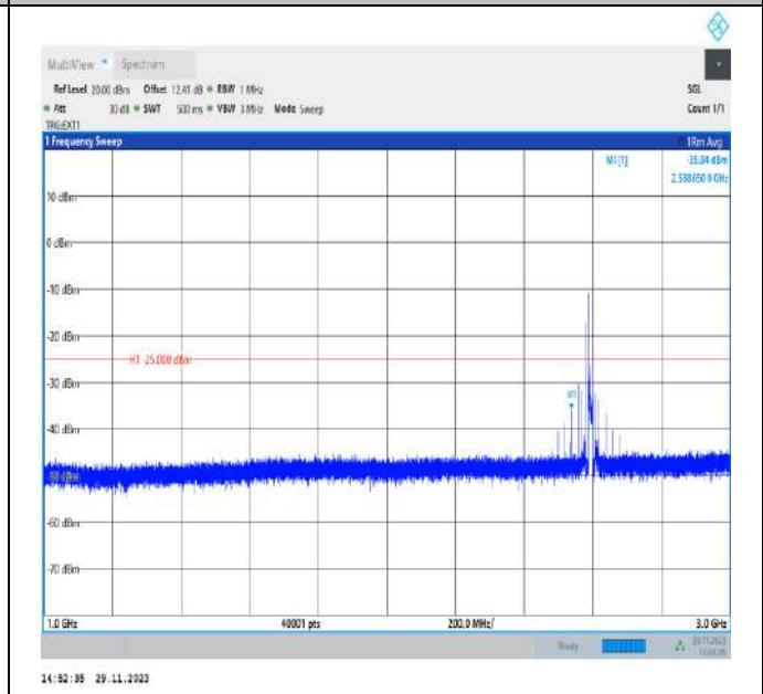
Band41_20MHz_QPSK_40620_1RB#0_1000~3000_1000~3000
