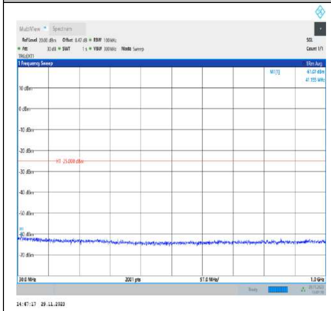
Band41_10MHz_QPSK_40620_1RB#0_30~1000_30~1000
