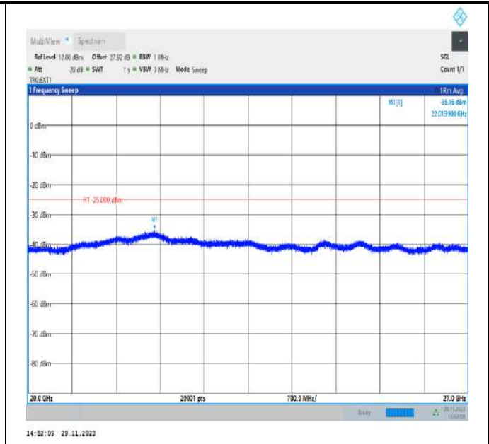
Band41_20MHz_QPSK_39750_1RB#0_20000~27000_20000~27000
