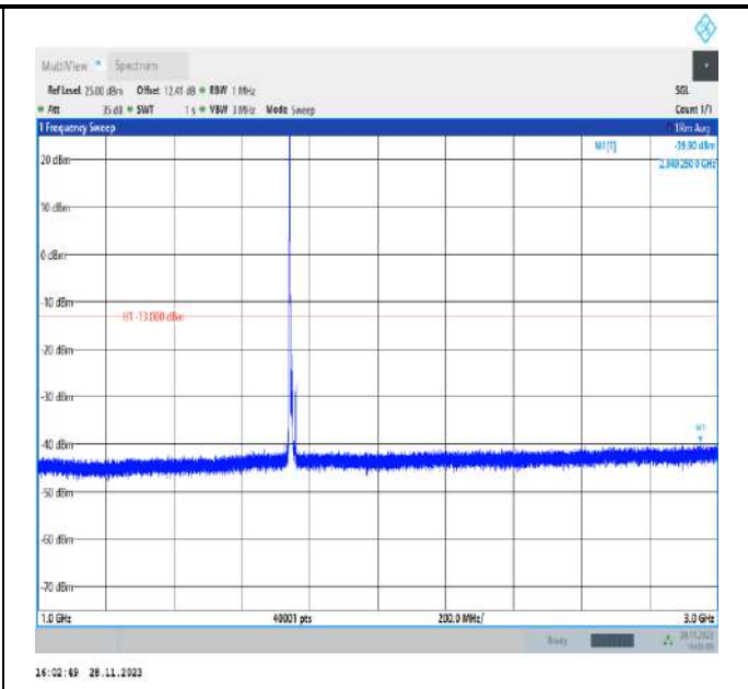
Band66_10MHz_QPSK_132322_1RB#0_1000~3000_1000~3000
