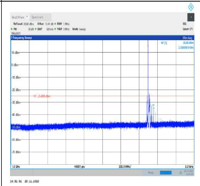
Band41_20MHz_QPSK_39750_1RB#0_1000~3000_1000~3000
