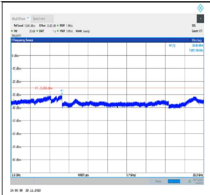
Band41_15MHz_QPSK_41515_1RB#0_3000~20000_3000~20000
