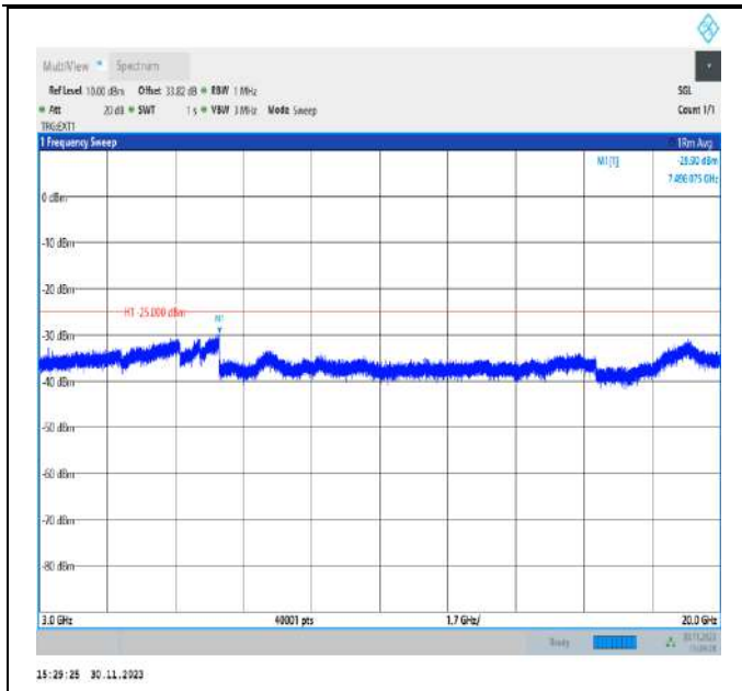
Band41_5MHz_QPSK_39675_1RB#0_3000~20000_3000~20000
