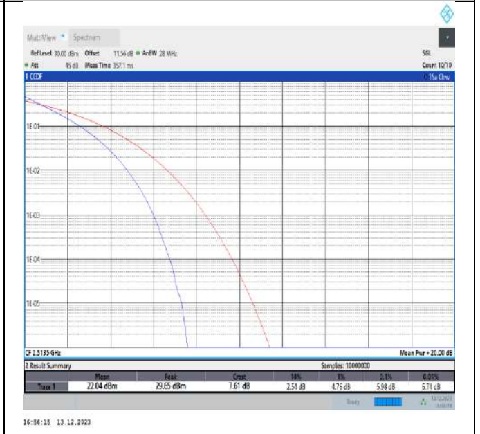
7-7-15MHz-10MHz-QPSK-QPSK-20825-20945-75RB#0-50RB#0-PASS
