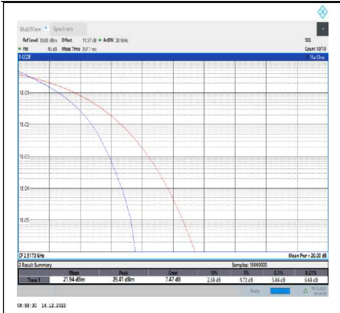
7-7-20MHz-10MHz-QPSK-QPSK-20850-20994-100RB#0-50RB#0-PASS
