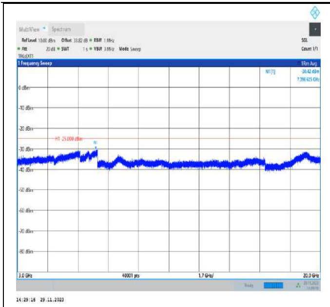
Band38_20MHz_QPSK_38000_1RB#0_3000~20000_3000~20000
