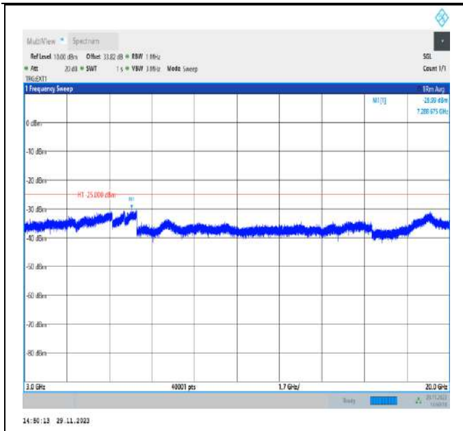
Band41_15MHz_QPSK_40620_1RB#0_3000~20000_3000~20000
