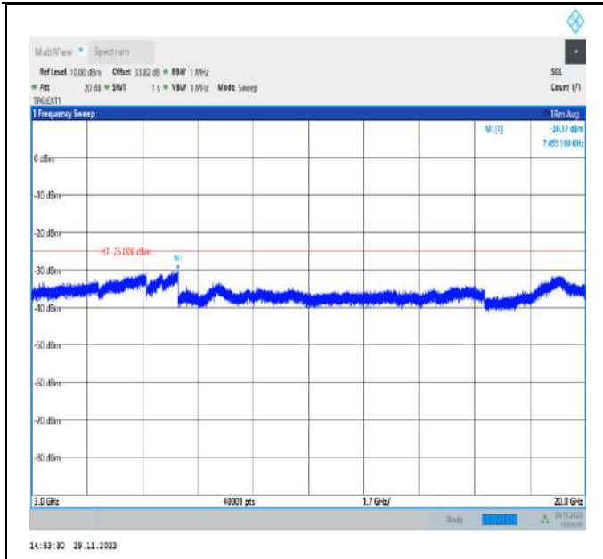
Band41_20MHz_QPSK_41490_1RB#0_3000~20000_3000~20000
