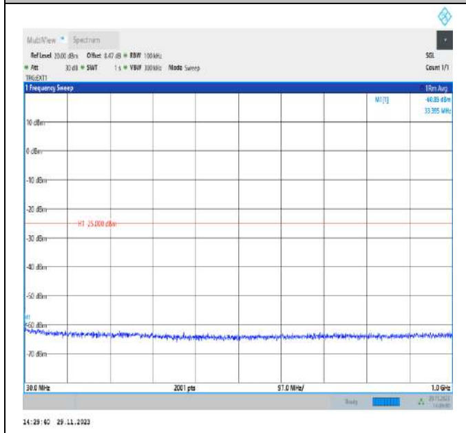
Band38_20MHz_QPSK_38150_1RB#0_30~1000_30~1000
