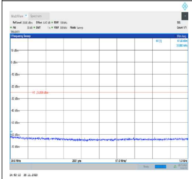
Band41_20MHz_QPSK_41490_1RB#0_30~1000_30~1000
