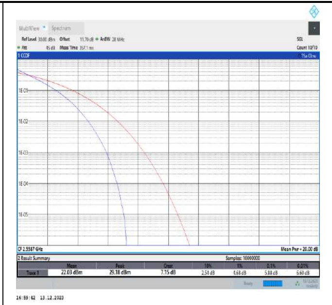
7-7-15MHz-10MHz-QPSK-QPSK-21277-21397-75RB#0-50RB#0-PASS
