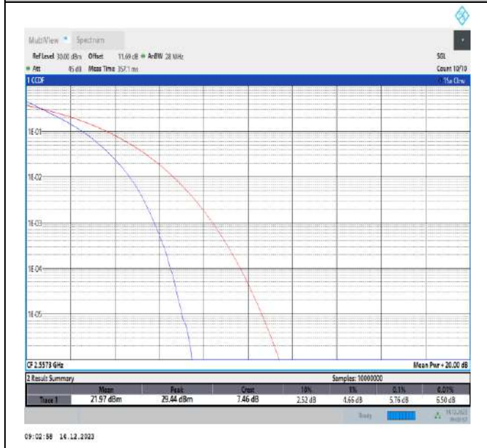
7-7-20MHz-10MHz-QPSK-QPSK-21251-21395-100RB#0-50RB#0-PASS
