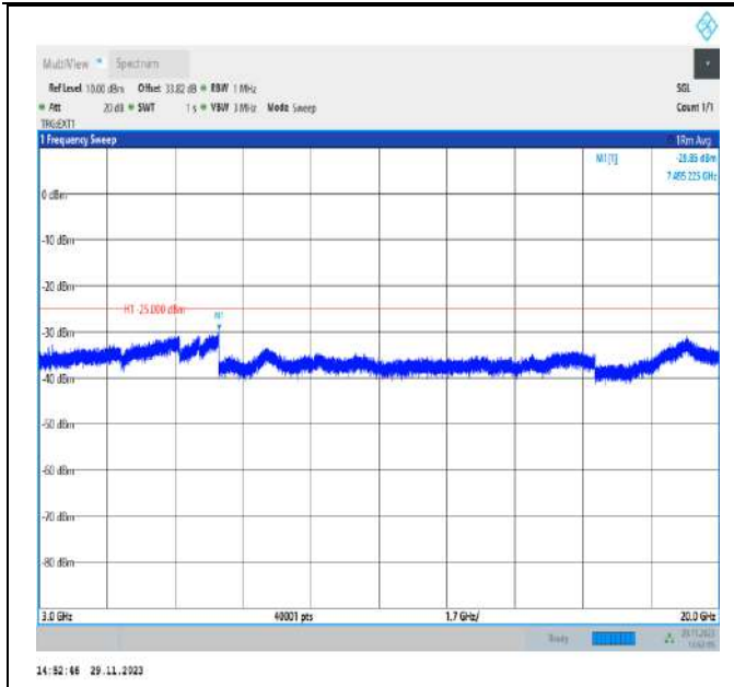
Band41_20MHz_QPSK_40620_1RB#0_3000~20000_3000~20000
