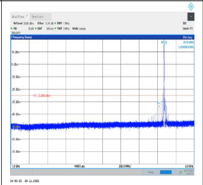
Band41_20MHz_QPSK_41490_1RB#0_1000~3000_1000~3000
