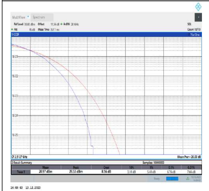
7-7-10MHz-20MHz-64QAM-64QAM-20805-20949-50RB#0-100RB#0-PASS
