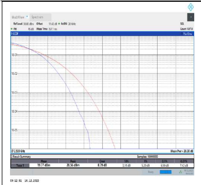
7-7-20MHz-20MHz-16QAM-16QAM-21001-21199-100RB#0-100RB#0-PASS
