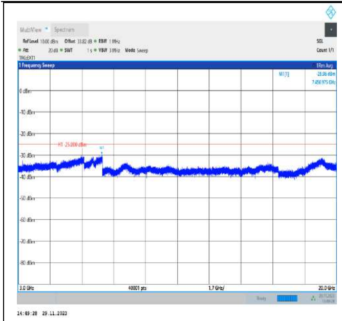
Band41_15MHz_QPSK_39725_1RB#0_3000~20000_3000~20000
