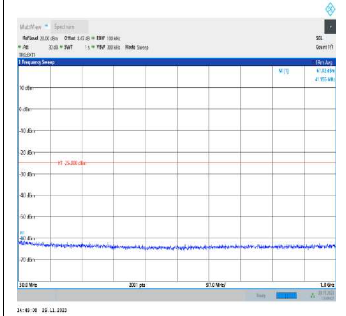
Band41_15MHz_QPSK_39725_1RB#0_30~1000_30~1000
