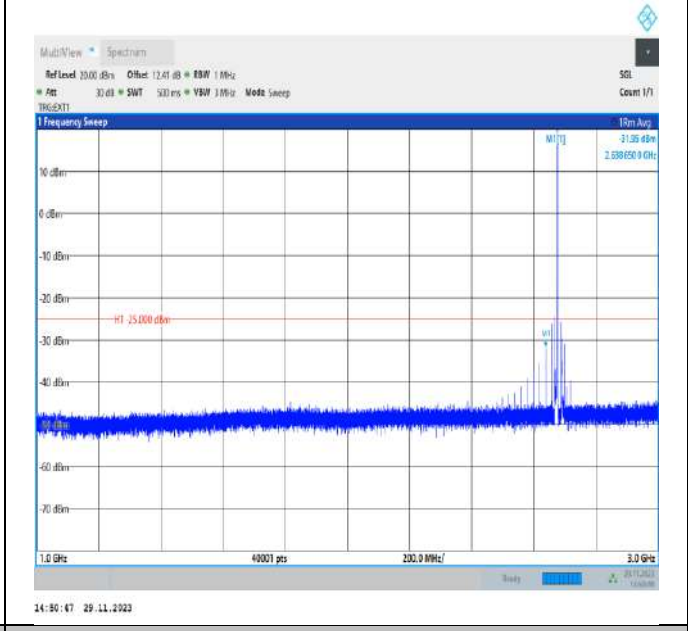
Band41_15MHz_QPSK_41515_1RB#0_1000~3000_1000~3000
