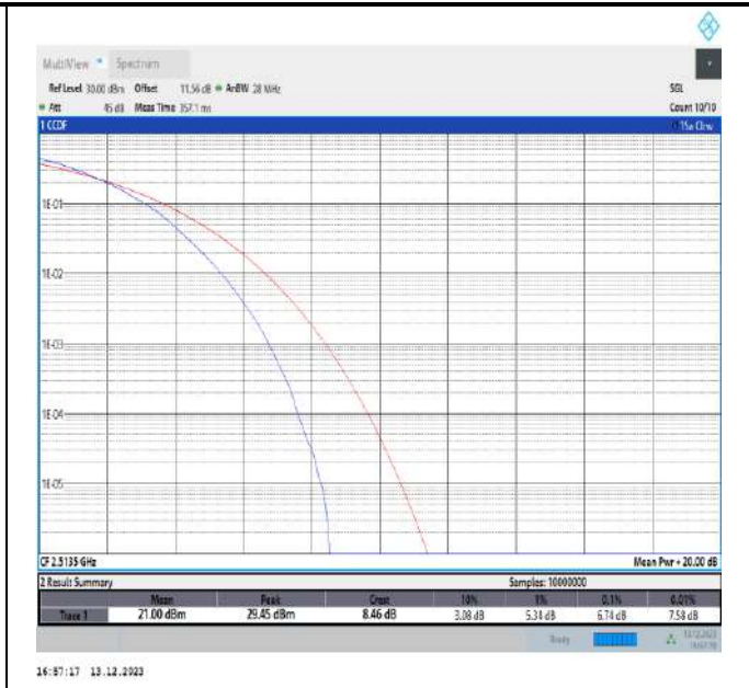
7-7-15MHz-10MHz-64QAM-64QAM-20825-20945-75RB#0-50RB#0-PASS
