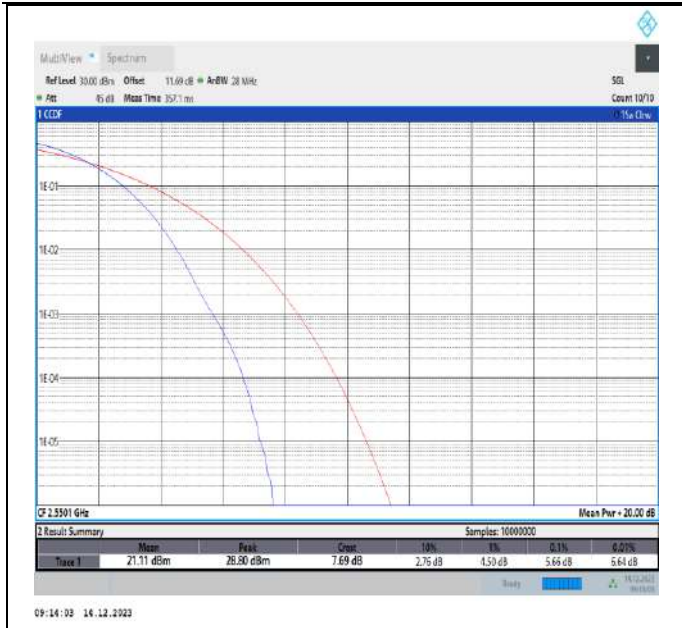
7-7-20MHz-20MHz-QPSK-QPSK-21152-21350-100RB#0-100RB#0-PASS
