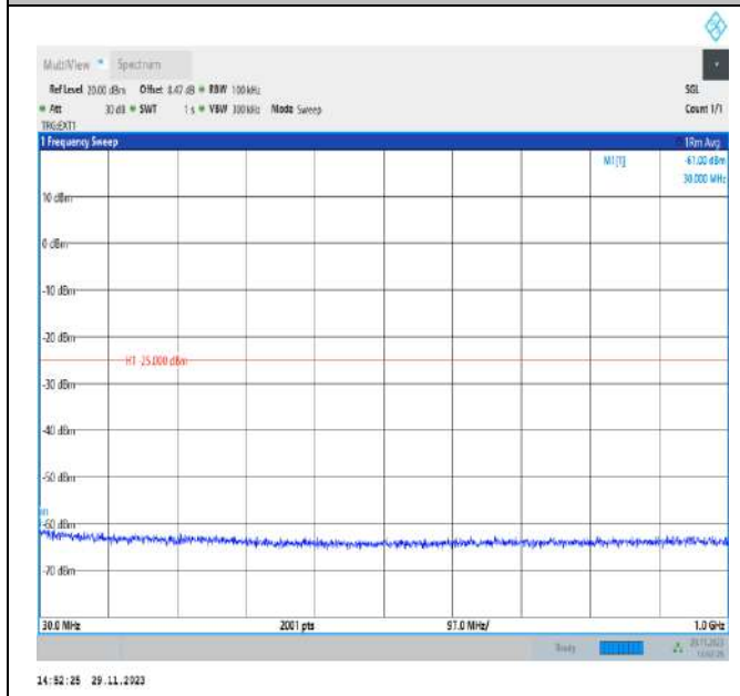
Band41_20MHz_QPSK_40620_1RB#0_30~1000_30~1000
