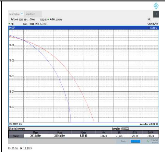
7-7-20MHz-15MHz-16QAM-16QAM-21026-21197-100RB#0-75RB#0-PASS
