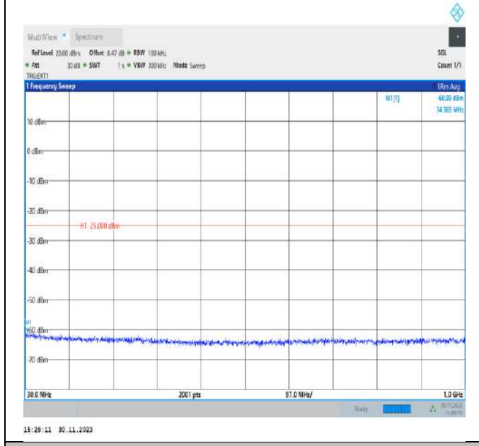
Band41_5MHz_QPSK_39675_1RB#0_30~1000_30~1000
