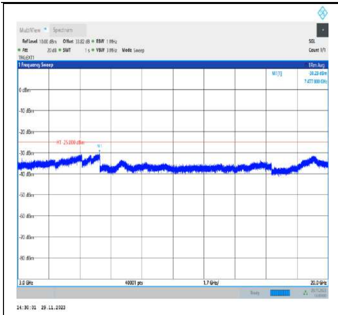
Band38_20MHz_QPSK_38150_1RB#0_3000~20000_3000~20000
