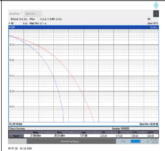
7-7-15MHz-20MHz-QPSK-QPSK-21179-21350-75RB#0-100RB#0-PASS
