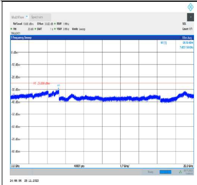
Band41_10MHz_QPSK_39700_1RB#0_3000~20000_3000~20000
