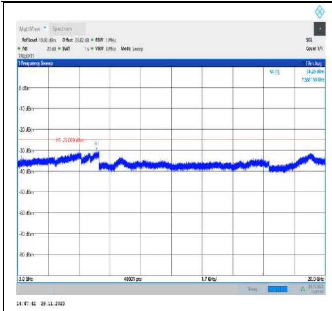
Band41_10MHz_QPSK_40620_1RB#0_3000~20000_3000~20000
