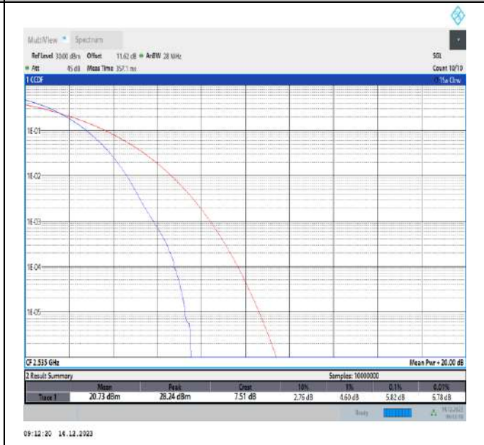
7-7-20MHz-20MHz-QPSK-QPSK-21001-21199-100RB#0-100RB#0-PASS
