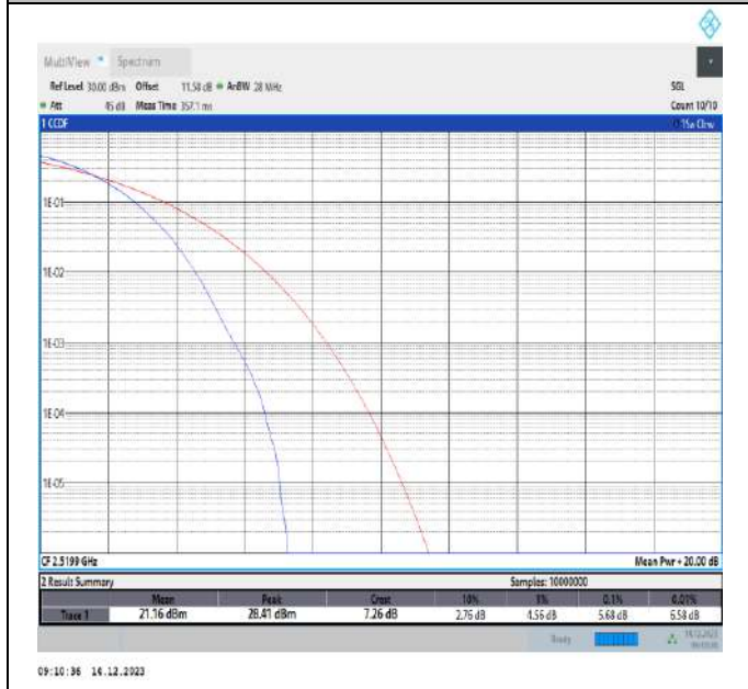
7-7-20MHz-20MHz-QPSK-QPSK-20850-21048-100RB#0-100RB#0-PASS
