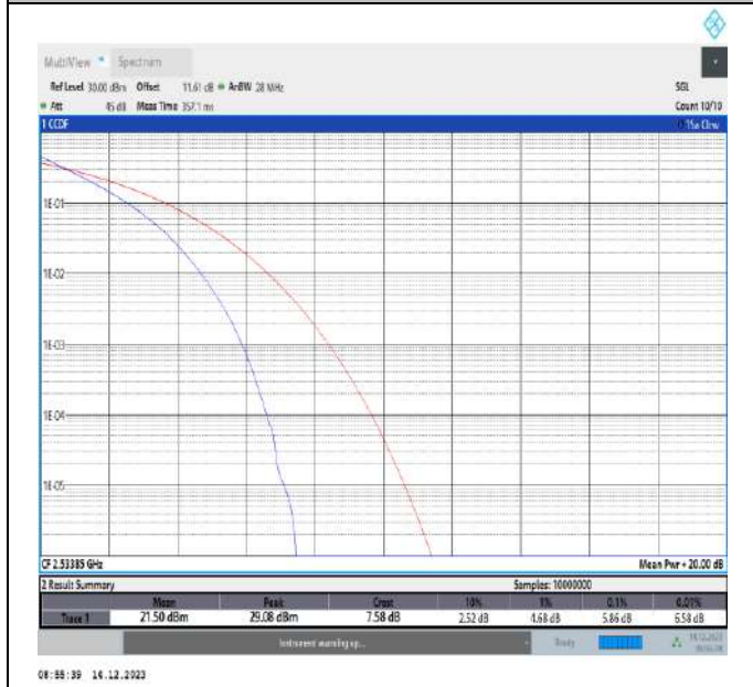
7-7-15MHz-20MHz-QPSK-QPSK-21003-21174-75RB#0-100RB#0-PASS
