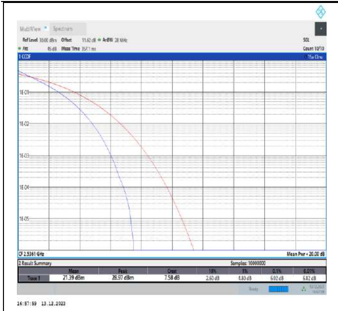
7-7-15MHz-10MHz-QPSK-QPSK-21051-21171-75RB#0-50RB#0-PASS
