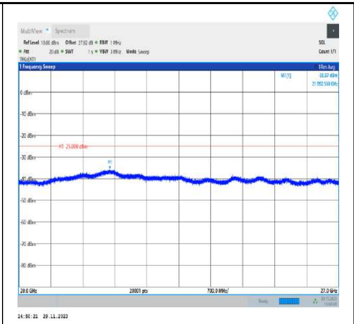
Band41_15MHz_QPSK_40620_1RB#0_20000~27000_20000~27000
