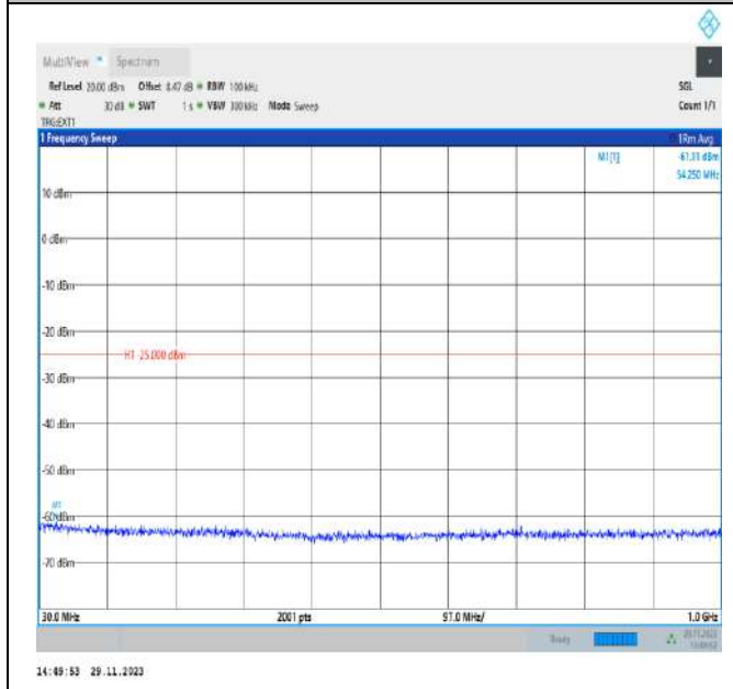
Band41_15MHz_QPSK_40620_1RB#0_30~1000_30~1000
