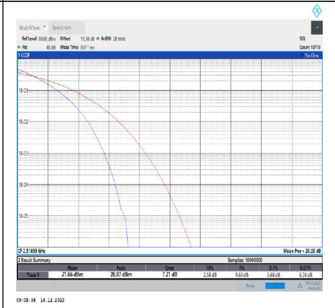
7-7-20MHz-15MHz-QPSK-QPSK-20850-21021-100RB#0-75RB#0-PASS
