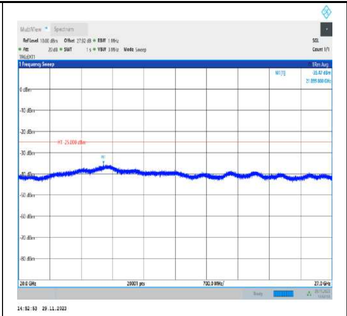
Band41_20MHz_QPSK_40620_1RB#0_20000~27000_20000~27000
