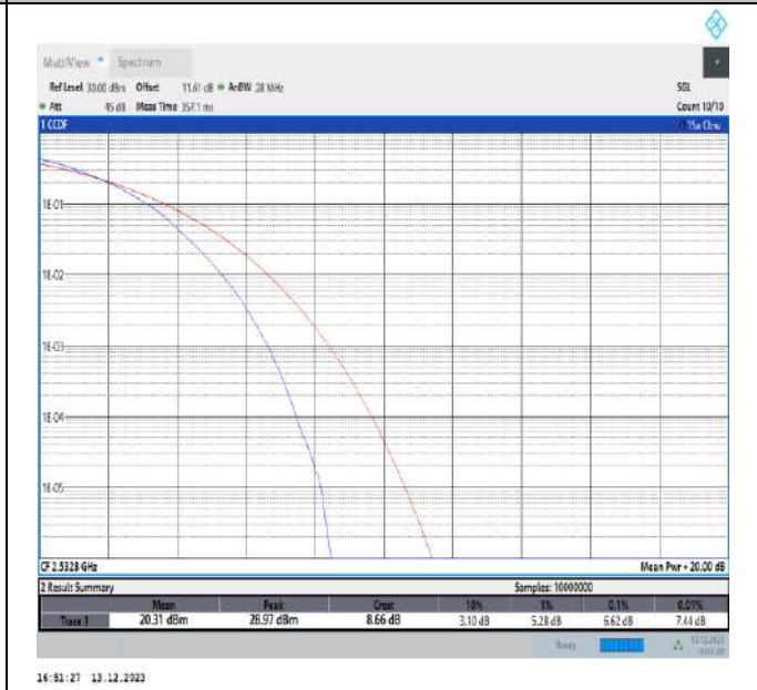
7-7-10MHz-20MHz-64QAM-64QAM-21006-21150-50RB#0-100RB#0-PASS
