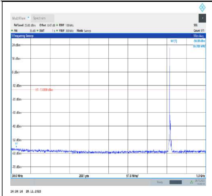
Band26_5MHz_QPSK_26765_1RB#0_30~1000_30~1000
