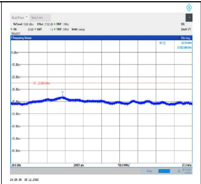
Band38_20MHz_QPSK_38000_1RB#0_20000~27000_20000~27000
