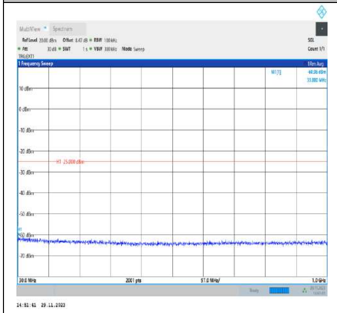
Band41_20MHz_QPSK_39750_1RB#0_30~1000_30~1000
