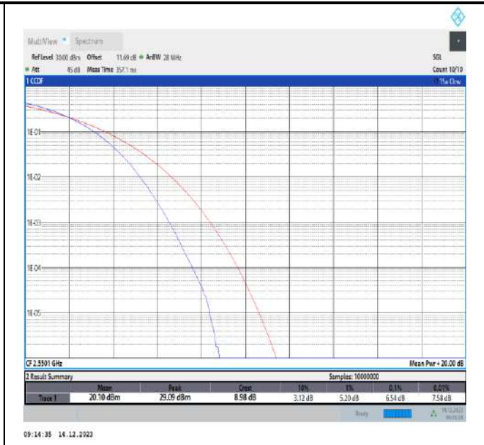
7-7-20MHz-20MHz-16QAM-16QAM-21152-21350-100RB#0-100RB#0-PASS
