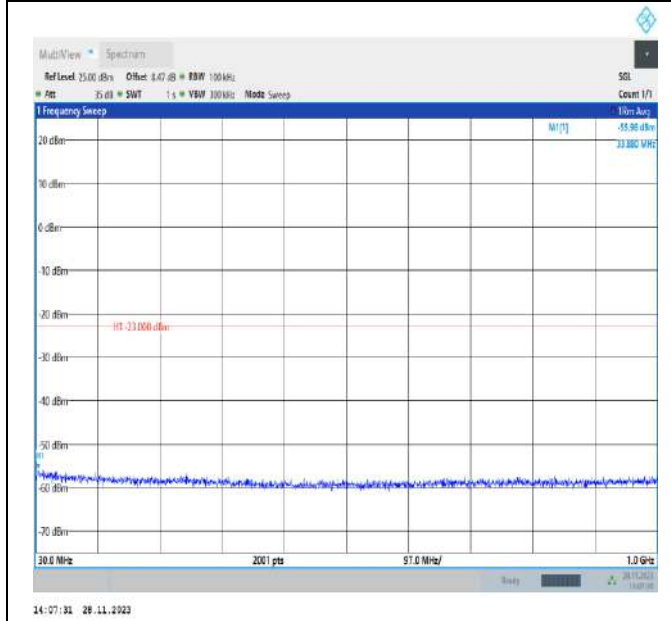
Band4_3MHz_QPSK_20175_1RB#0_30~1000_30~1000 0
