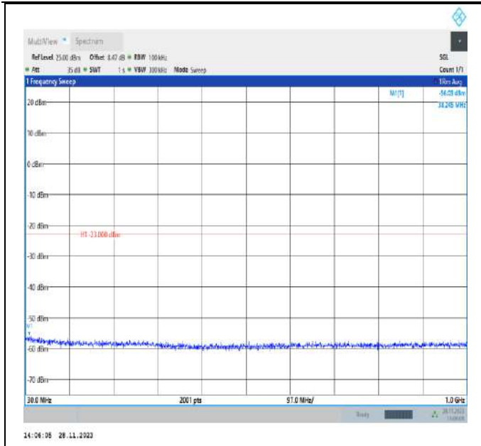
Band4_1.4MHz_QPSK_20393_1RB#0_30~1000_30~1000
