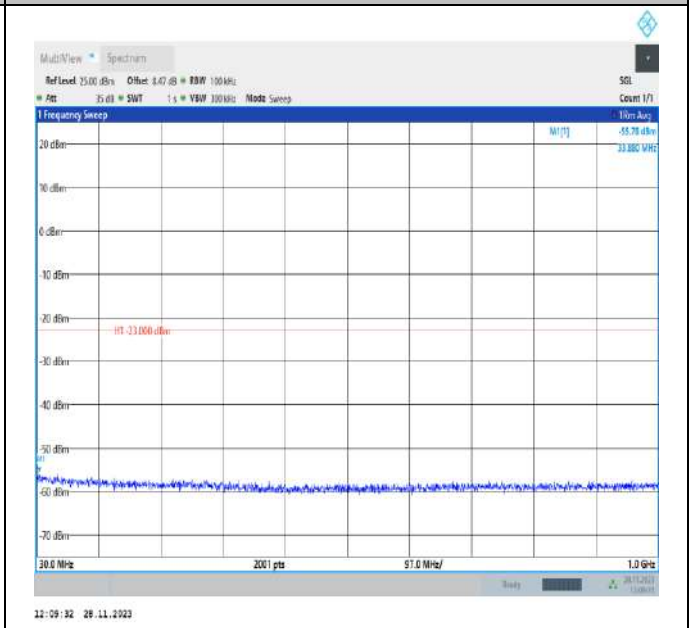
Band2_20MHz_QPSK_19100_1RB#0_30~1000_30~1000
