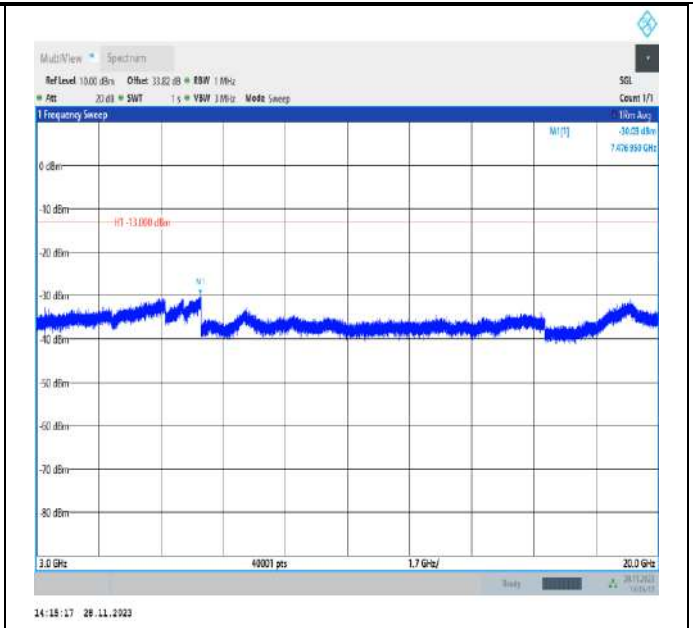
Band4_20MHz_QPSK_20050_1RB#0_3000~20000_3000~20000 0000
