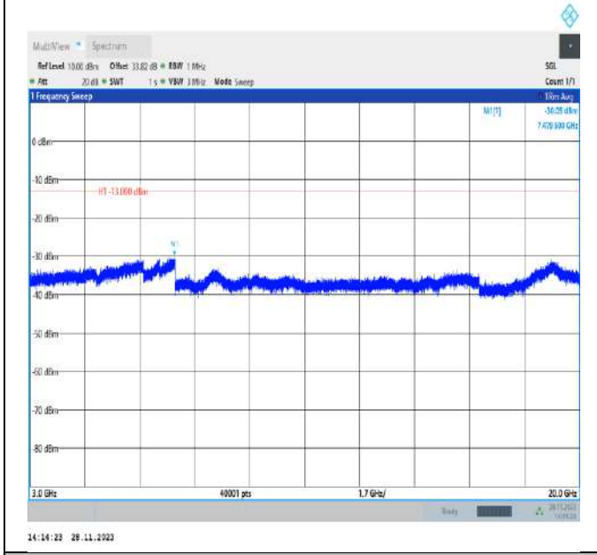
Band4_15MHz_QPSK_20325_1RB#0_3000~20000_3000~20000
