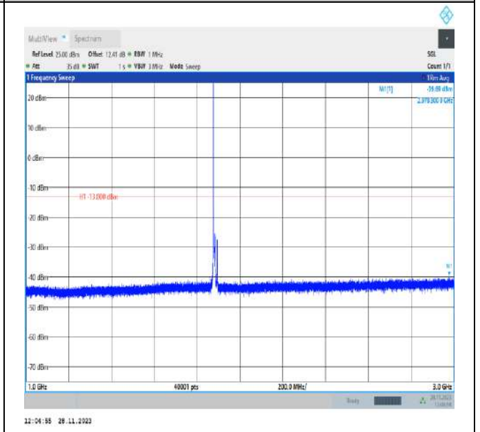
Band2_10MHz_QPSK_18900_1RB#0_1000~3000_1000~3000
