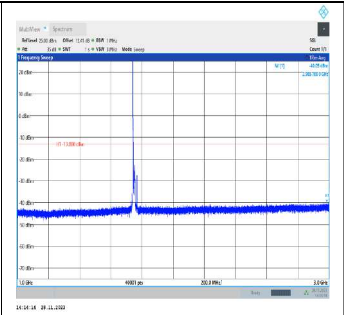
Band4_15MHz_QPSK_20325_1RB#0_1000~3000_1000~3000
