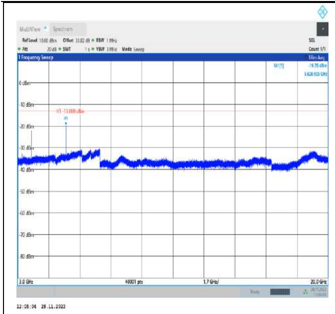
Band2_10MHz_QPSK_18900_1RB#0_3000~20000_3000~20000
