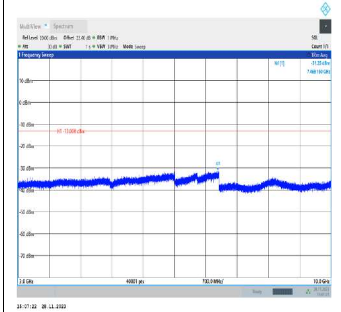
Band12_5MHz_QPSK_23155_1RB#0_3000~10000_3000~10000 0000
