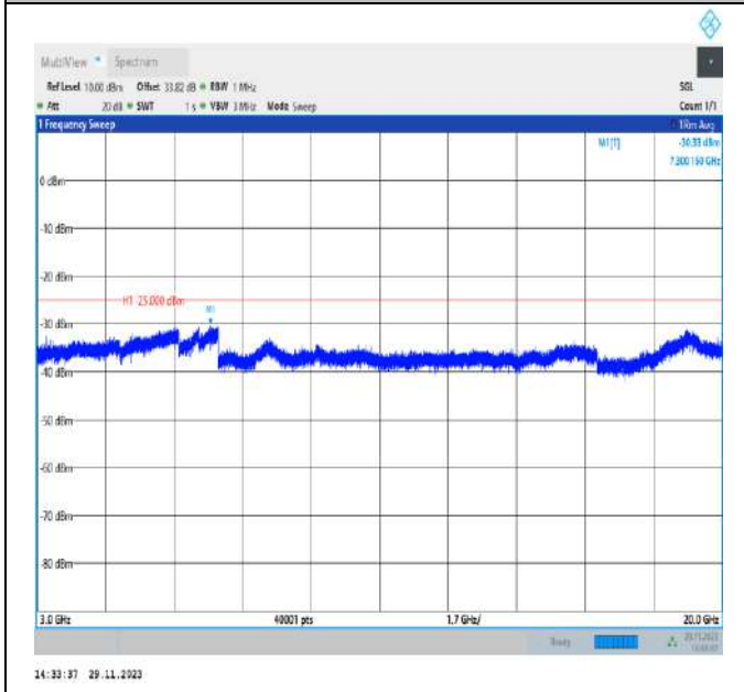
Band7_5MHz_QPSK_21425_1RB#0_3000~20000_3000~20 000
