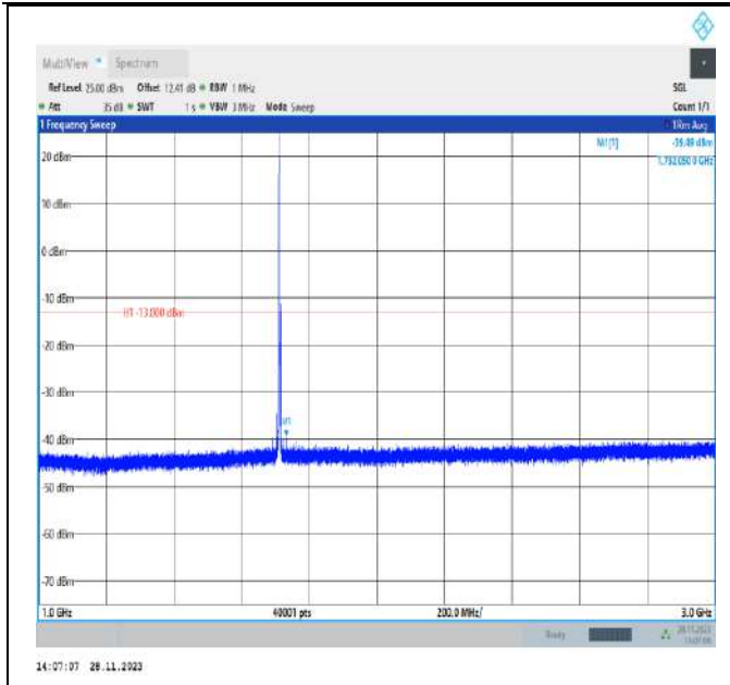
Band4_3MHz_QPSK_19965_1RB#0_1000~3000_1000~300 0
