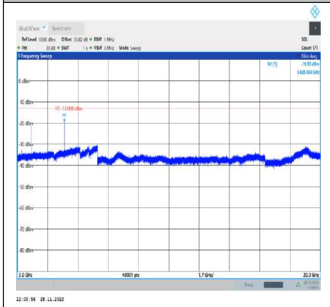
Band2_3MHz_QPSK_18900_1RB#0_3000~20000_3000~20 000
