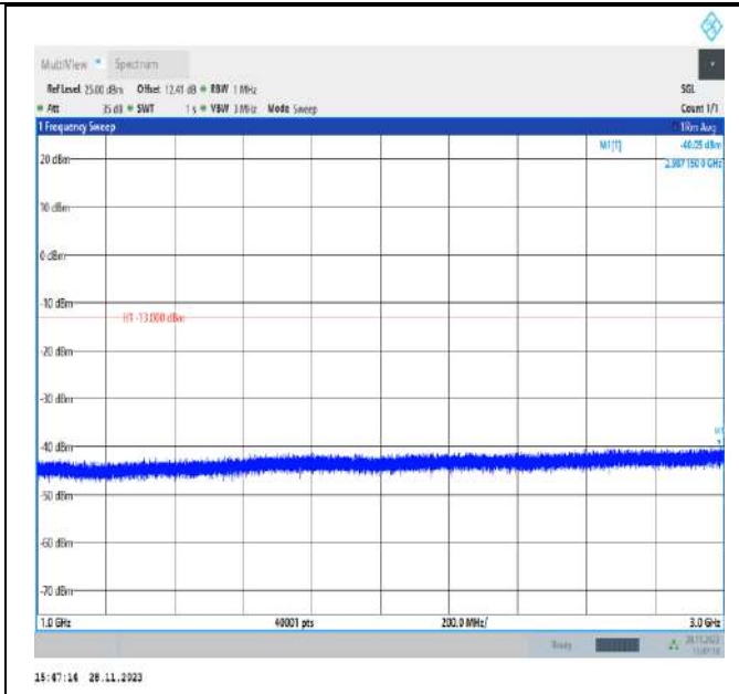
Band17_5MHz_QPSK_23790_1RB#0_1000~3000_1000~3000
