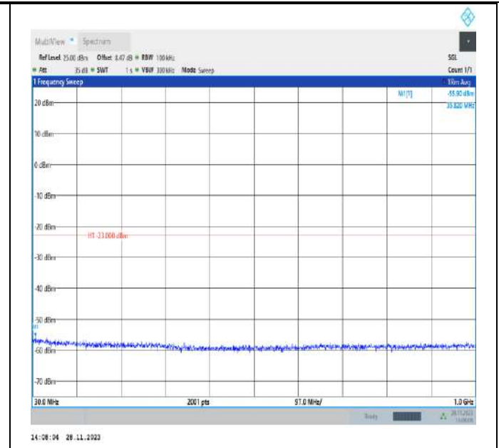
Band4_3MHz_QPSK_20385_1RB#0_30~1000_30~1000
