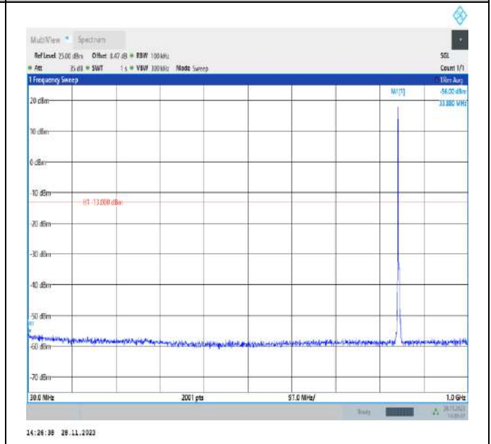
Band5_3MHz_QPSK_20635_1RB#0_30~1000_30~1000
