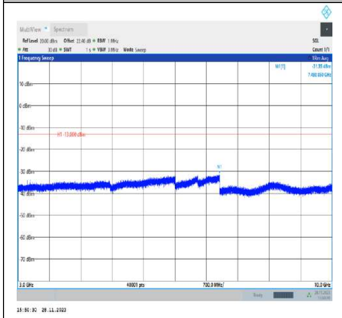
Band17_10MHz_QPSK_23790_1RB#0_3000~10000_3000~10000
