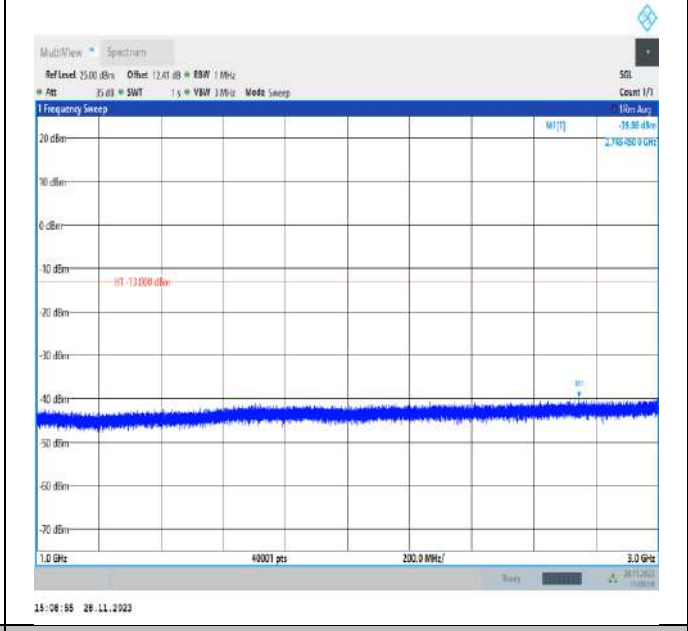
Band12_10MHz_QPSK_23095_1RB#0_1000~3000_1000~3000
