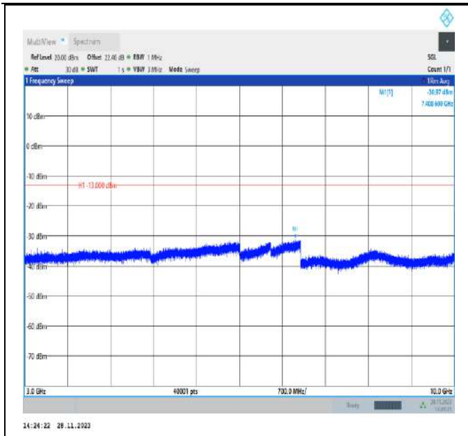
Band5_1.4MHz_QPSK_20643_1RB#0_3000~10000_3000~10000
