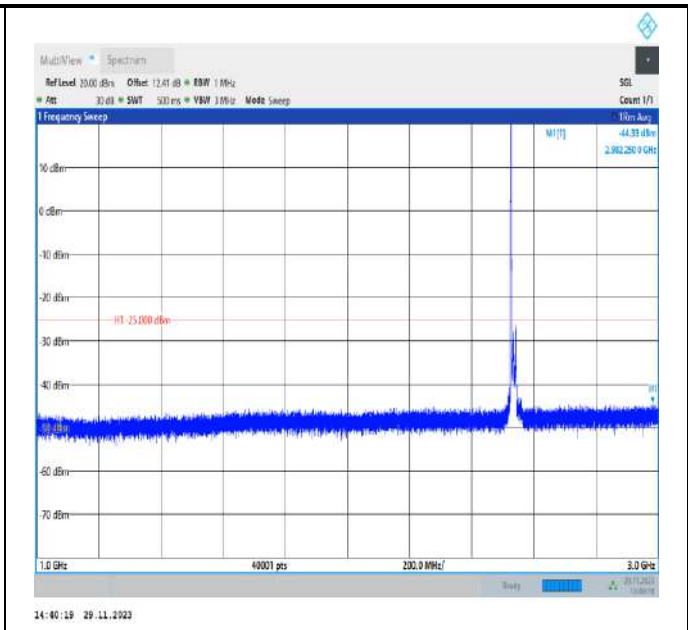
Band7_20MHz_QPSK_21100_1RB#0_1000~3000_1000~3000
