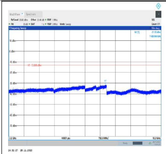
Band5_10MHz_QPSK_20525_1RB#0_3000~10000_3000~10000
