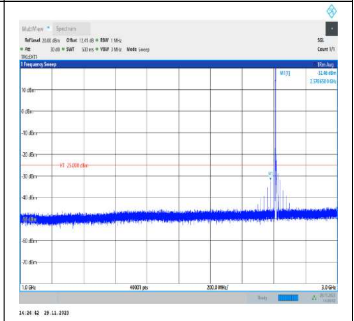
Band38_10MHz_QPSK_38200_1RB#0_1000~3000_1000~3000
