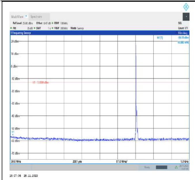
Band12_5MHz_QPSK_23155_1RB#0_30~1000_30~1000
