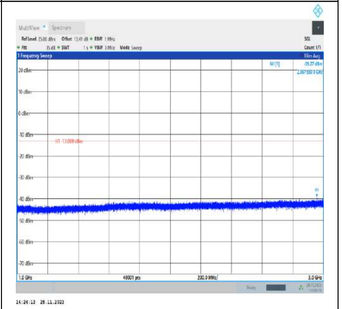
Band5_1.4MHz_QPSK_20643_1RB#0_1000~3000_1000~3000
