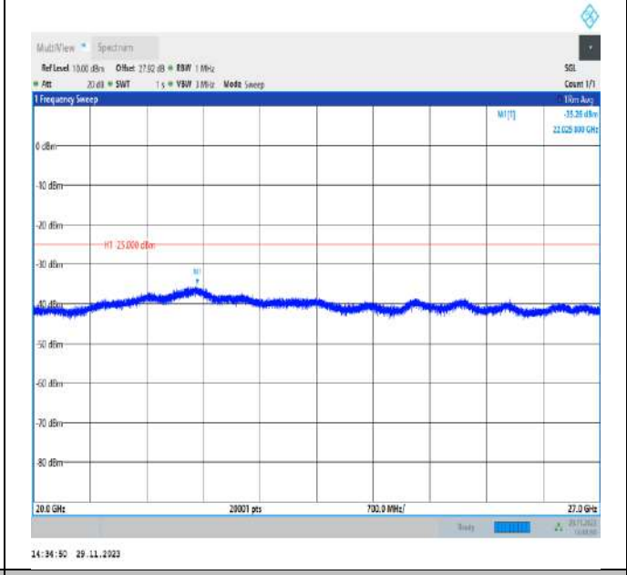
Band7_10MHz_QPSK_20800_1RB#0_20000~27000_20000~27000
