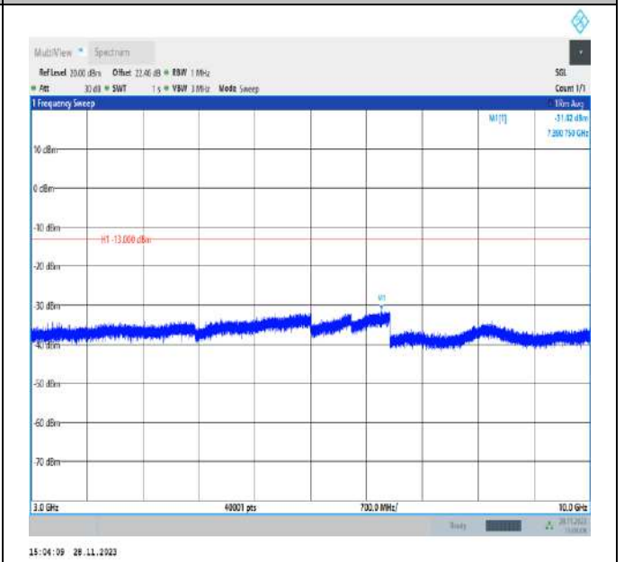
Band12_3MHz_QPSK_23025_1RB#0_3000~10000_3000~10000
