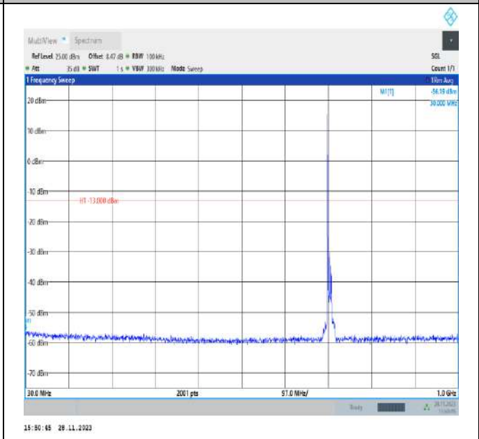
Band17_10MHz_QPSK_23800_1RB#0_30~1000_30~1000
