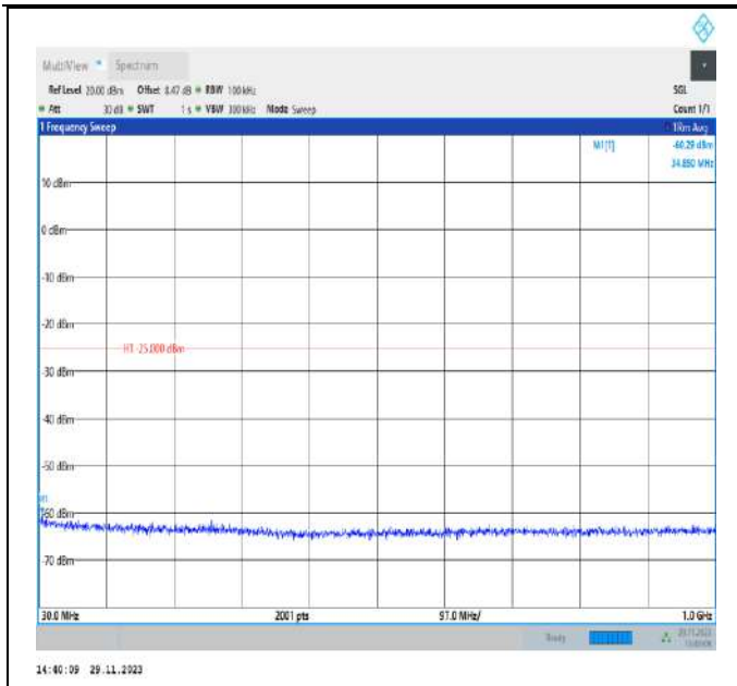
Band7_20MHz_QPSK_21100_1RB#0_30~1000_30~1000
