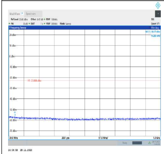
Band4_1.4MHz_QPSK_19957_1RB#0_30~1000_30~1000
