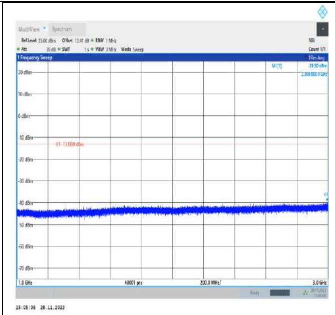
Band12_3MHz_QPSK_23165_1RB#0_1000~3000_1000~3000
