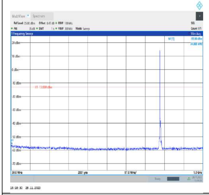
Band13_5MHz_QPSK_23255_1RB#0_30~1000_30~1000 00
