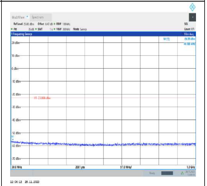
Band2_10MHz_QPSK_18650_1RB#0_30~1000_30~1000
