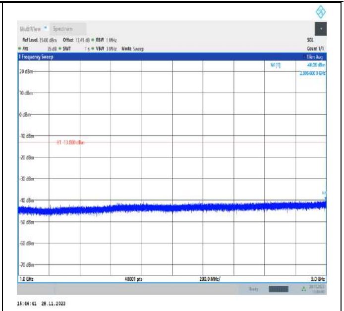
Band17_5MHz_QPSK_23755_1RB#0_1000~3000_1000~3000 00
