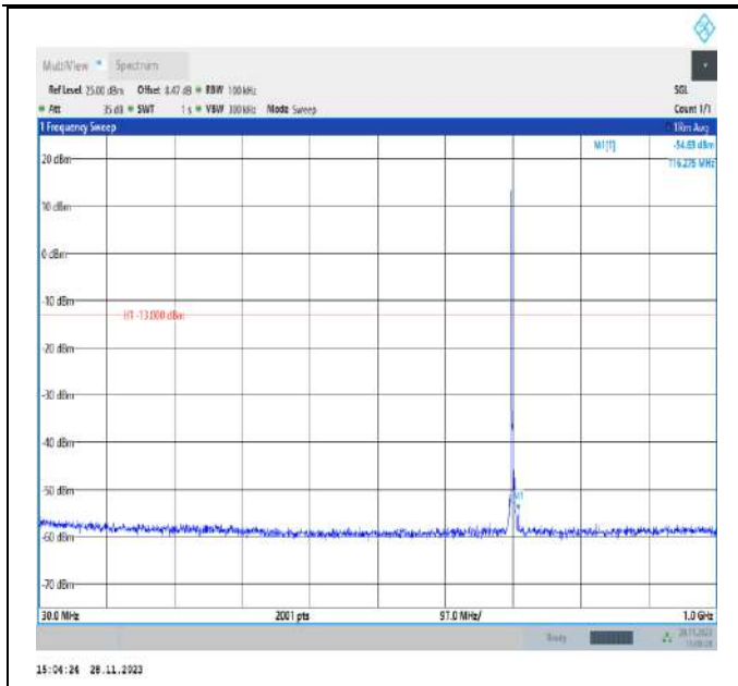
Band12_3MHz_QPSK_23095_1RB#0_30~1000_30~1000
