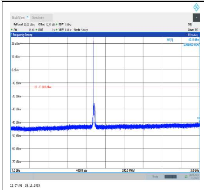
Band2_15MHz_QPSK_18900_1RB#0_1000~3000_1000~3000
