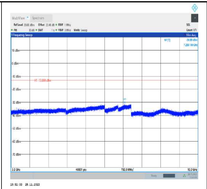
Band17_10MHz_QPSK_23800_1RB#0_3000~10000_3000~10000
