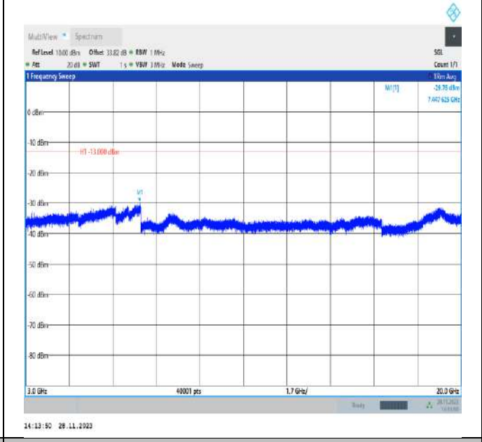
Band4_15MHz_QPSK_20175_1RB#0_3000~20000_3000~20000
