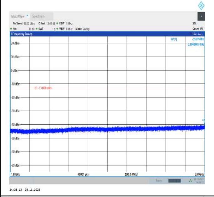
Band5_5MHz_QPSK_20425_1RB#0_1000~3000_1000~300 0
