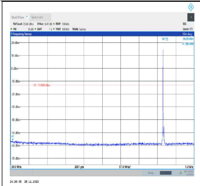
Band5_3MHz_QPSK_20525_1RB#0_30~1000_30~1000
