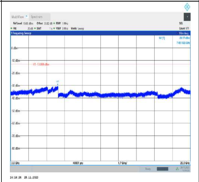
Band4_20MHz_QPSK_20300_1RB#0_3000~20000_3000~20000
