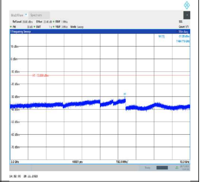
Band5_10MHz_QPSK_20600_1RB#0_3000~10000_3000~10000
