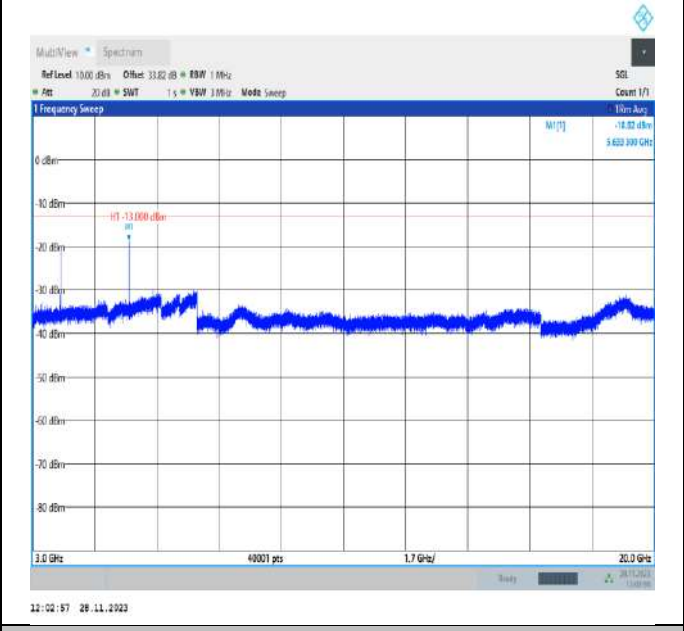
Band2_5MHz_QPSK_18900_1RB#0_3000~20000_3000~2000
