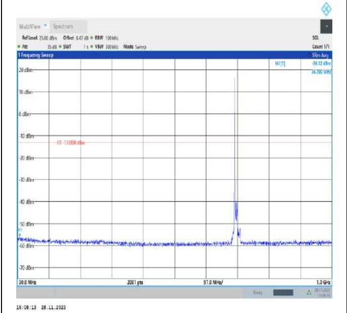
Band12_10MHz_QPSK_23060_1RB#0_30~1000_30~1000
