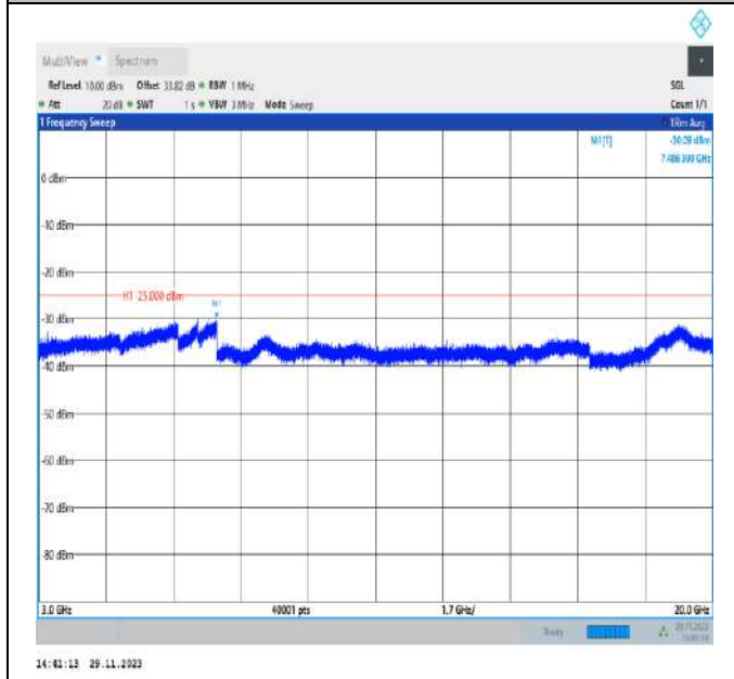
Band7_20MHz_QPSK_21350_1RB#0_3000~20000_3000~20000 0000
