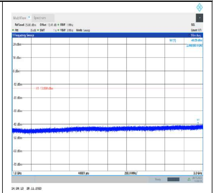
Band5_3MHz_QPSK_20525_1RB#0_1000~3000_1000~3000 0
