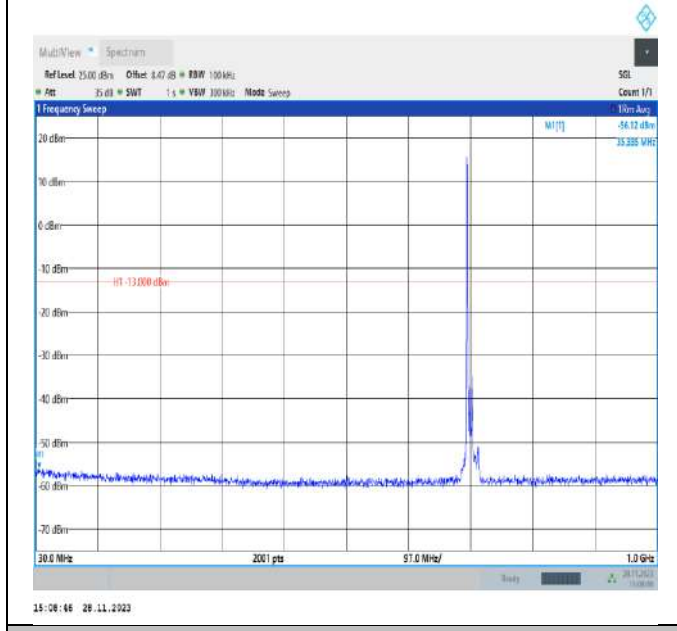
Band12_10MHz_QPSK_23095_1RB#0_30~1000_30~1000
