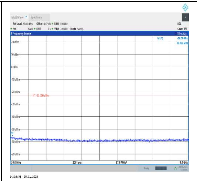
Band4_20MHz_QPSK_20300_1RB#0_30~1000_30~1000
