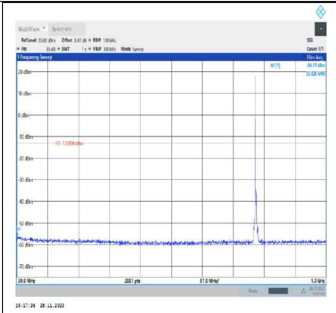
Band13_5MHz_QPSK_23205_1RB#0_30~1000_30~1000
