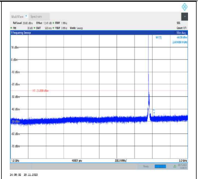
Band7_15MHz_QPSK_21375_1RB#0_1000~3000_1000~3000 00
