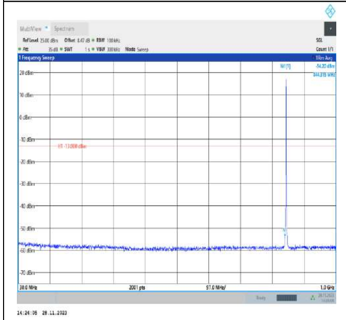
Band5_1.4MHz_QPSK_20643_1RB#0_30~1000_30~1000
