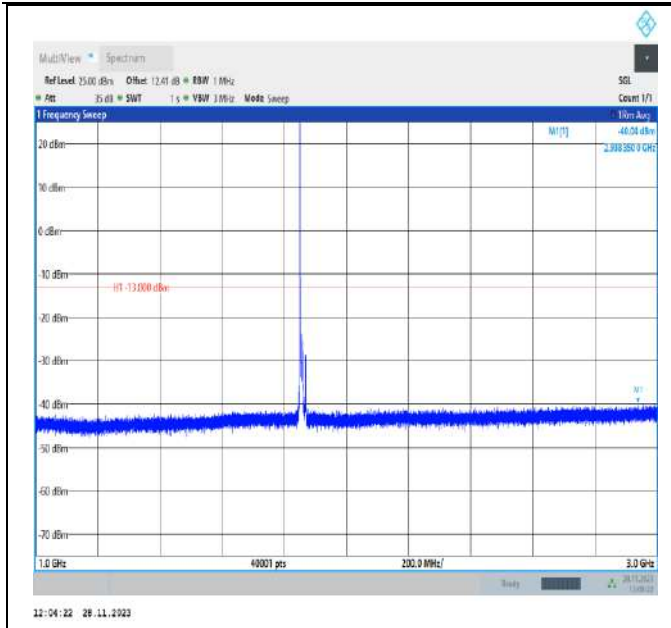
Band2_10MHz_QPSK_18650_1RB#0_1000~3000_1000~3000
