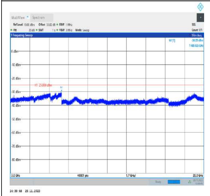
Band7_20MHz_QPSK_20850_1RB#0_3000~20000_3000~20000 0000
