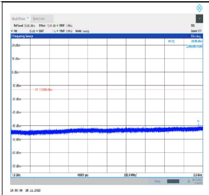
Band17_10MHz_QPSK_23800_1RB#0_1000~3000_1000~3000
