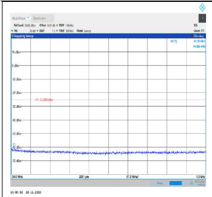
Band7_20MHz_QPSK_21350_1RB#0_30~1000_30~1000
