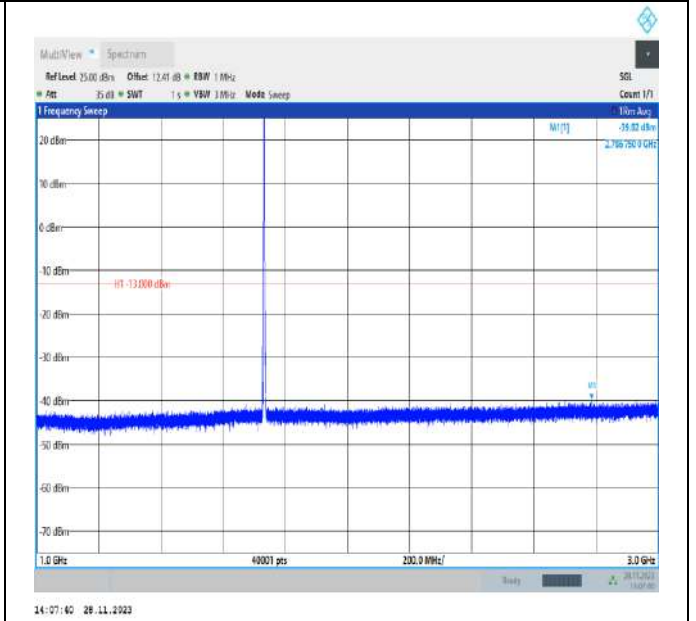
Band4_3MHz_QPSK_20175_1RB#0_1000~3000_1000~300 0
