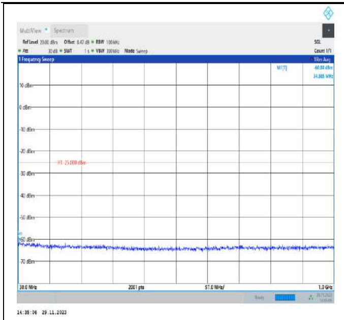
Band7_10MHz_QPSK_21100_1RB#0_30~1000_30~1000
