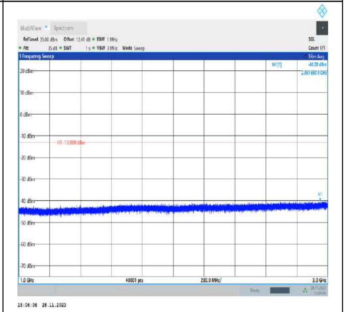
Band12_5MHz_QPSK_23035_1RB#0_1000~3000_1000~3000
