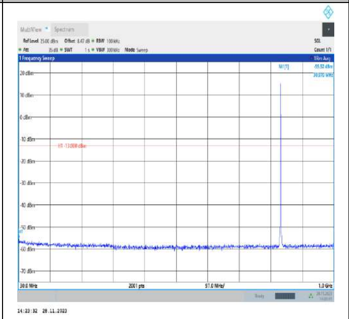
Band5_1.4MHz_QPSK_20525_1RB#0_30~1000_30~1000
