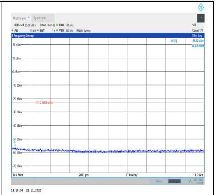
Band4_10MHz_QPSK_20000_1RB#0_30~1000_30~1000
