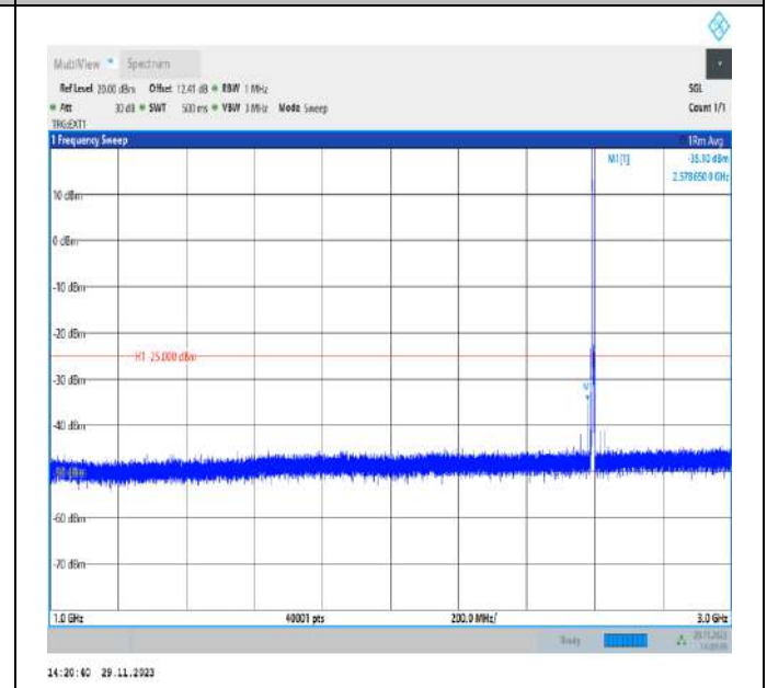
Band38_5MHz_QPSK_38000_1RB#0_1000~3000_1000~3000
