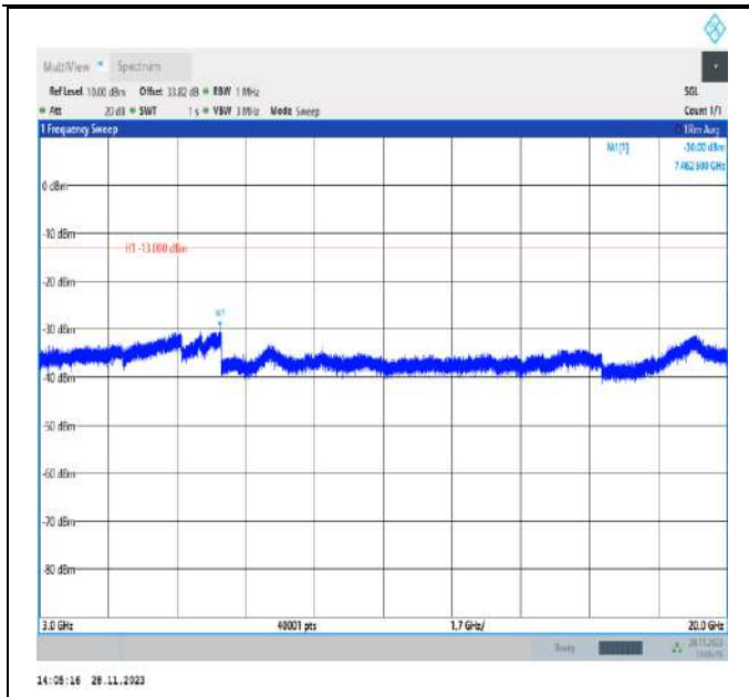
Band4_1.4MHz_QPSK_19957_1RB#0_3000~20000_3000~20000
