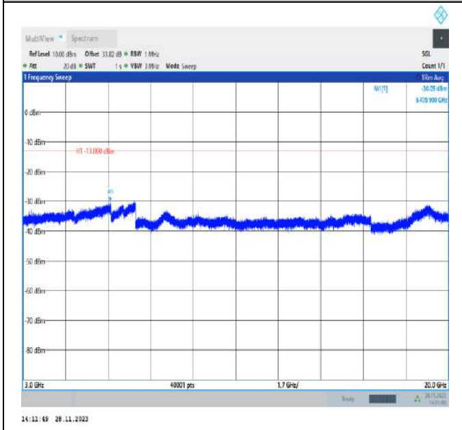
Band4_10MHz_QPSK_20175_1RB#0_3000~20000_3000~20000
