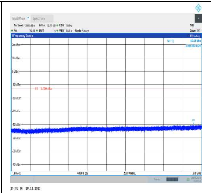
Band12_1.4MHz_QPSK_23017_1RB#0_1000~3000_1000~3000
