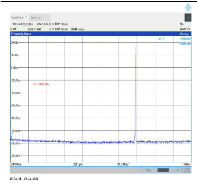
Band12_1.4MHz_QPSK_23017_1RB#0_30~1000_30~1000
