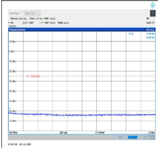
Band38_10MHz_QPSK_38200_1RB#0_30~1000_30~1000
