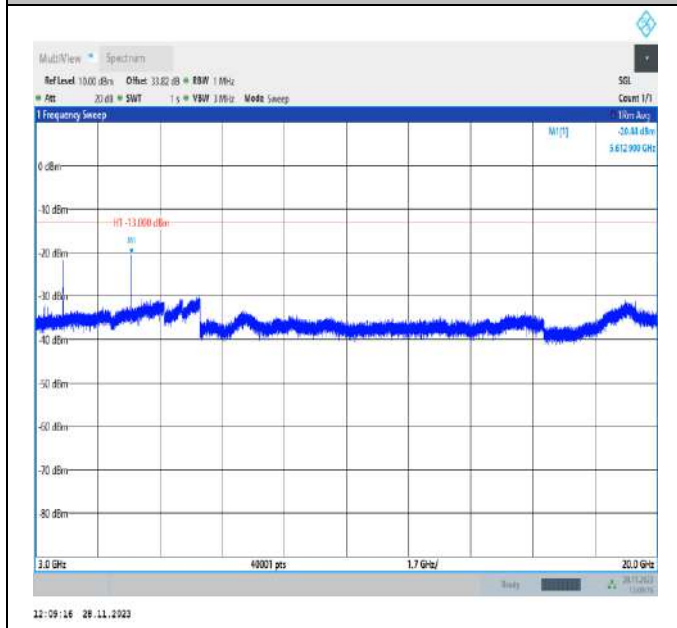
Band2_20MHz_QPSK_18900_1RB#0_3000~20000_3000~20000 0000
