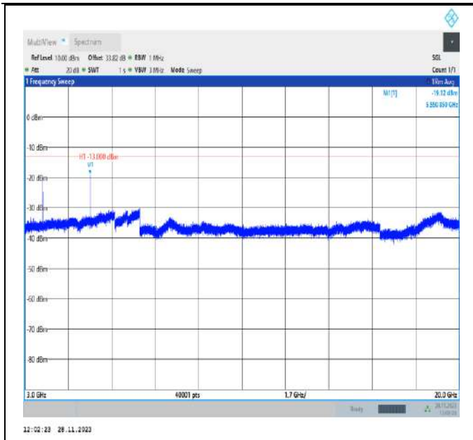
Band2_5MHz_QPSK_18625_1RB#0_3000~20000_3000~2000
