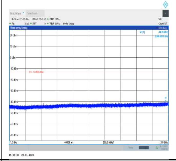
Band12_1.4MHz_QPSK_23173_1RB#0_1000~3000_1000~3000
