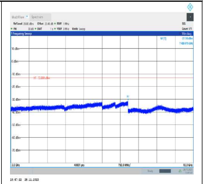
Band17_5MHz_QPSK_23790_1RB#0_3000~10000_3000~10000
