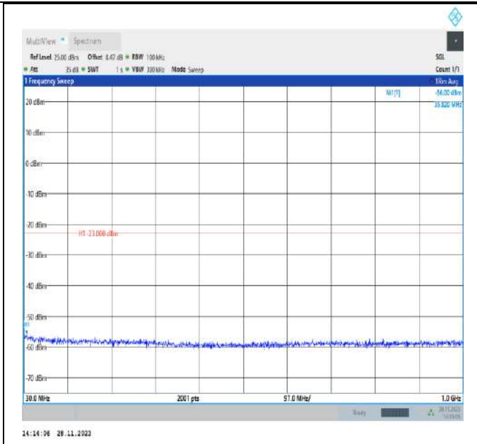
Band4_15MHz_QPSK_20325_1RB#0_30~1000_30~1000
