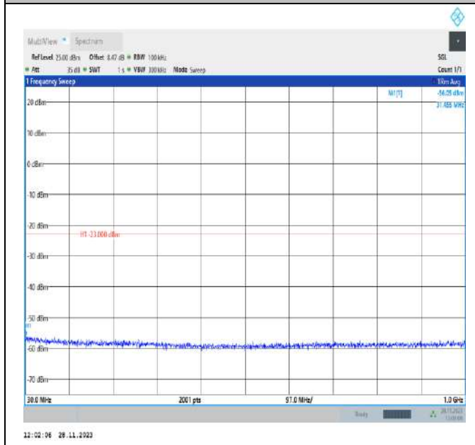
Band2_5MHz_QPSK_18625_1RB#0_30~1000_30~1000
