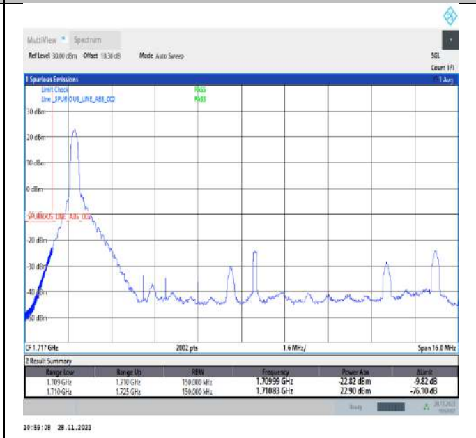
Band66_15MHz_QPSK_132047_1RB#0
