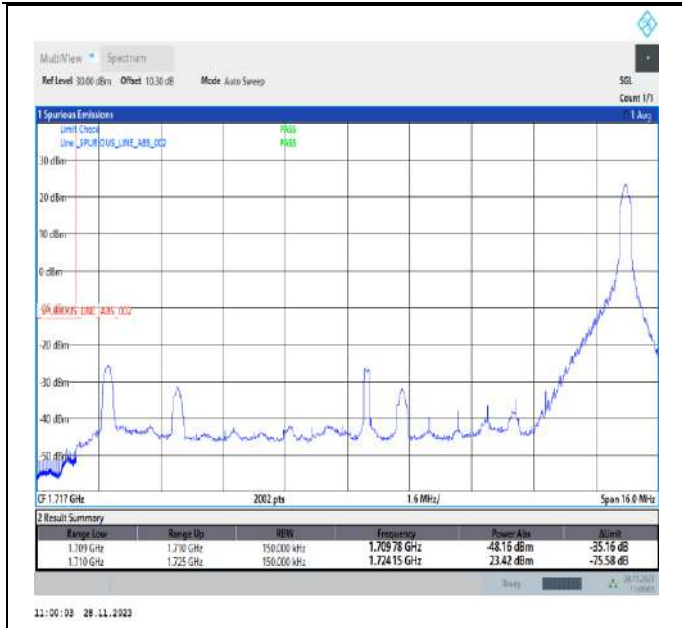
Band66_15MHz_QPSK_132047_1RB#74
