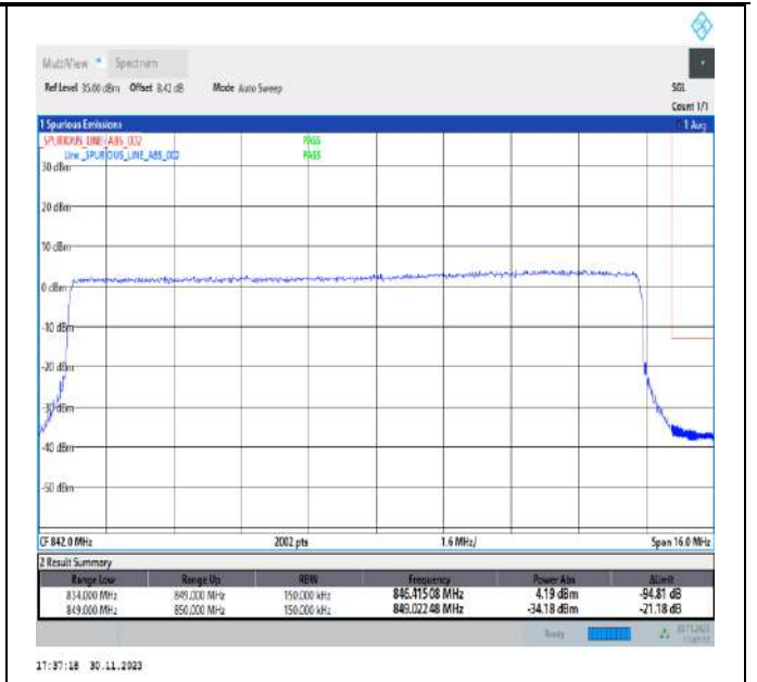
Band26_15MHz_16QAM_26965_75RB#0
