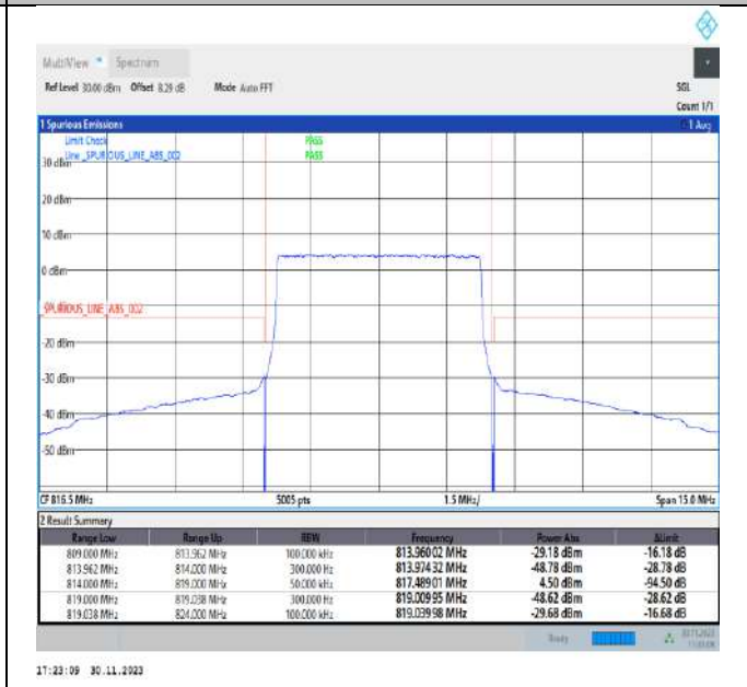
Band26_5MHz_16QAM_26715_25RB#0
