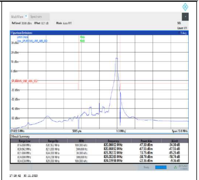
Band26_3MHz_64QAM_26775_1RB#14
