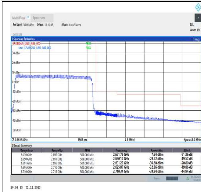
Band41_20MHz_16QAM_41490_100RB#0
