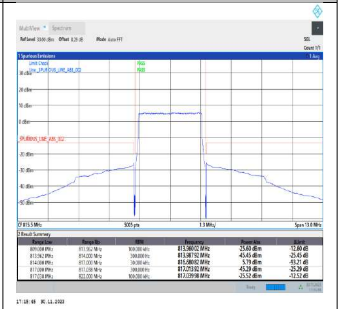
Band26_3MHz_QPSK_26705_15RB#0
