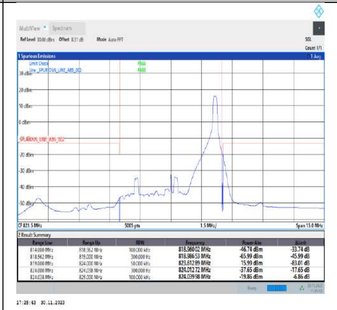
Band26_5MHz_64QAM_26765_1RB#24
