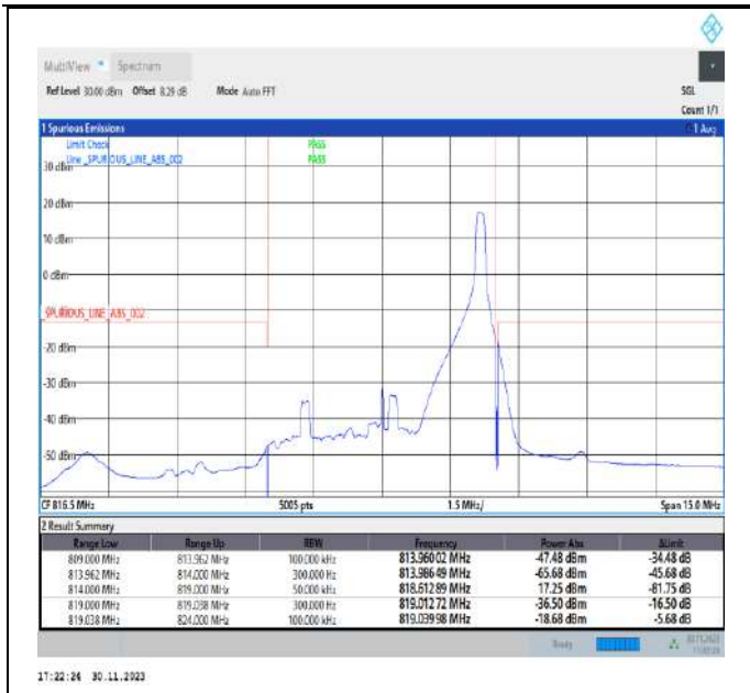
Band26_5MHz_64QAM_26715_1RB#24
