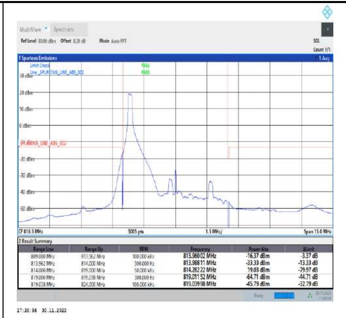
Band26_5MHz_16QAM_26715_1RB#0
