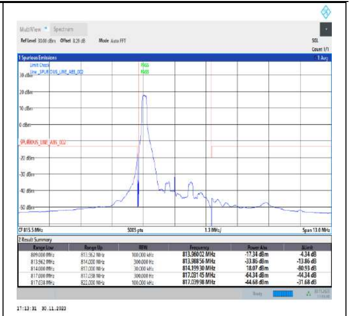
Band26_3MHz_QPSK_26705_1RB#0
