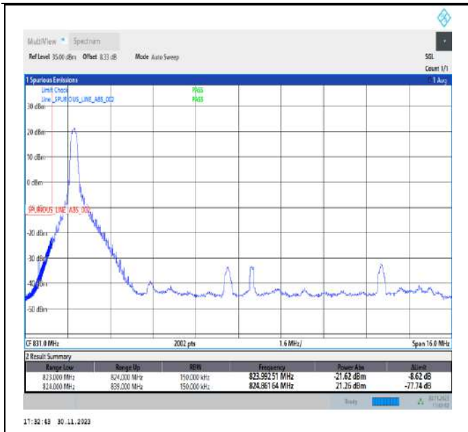
Band26_15MHz_16QAM_26865_1RB#0
