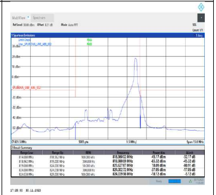
Band26_5MHz_QPSK_26765_1RB#24
