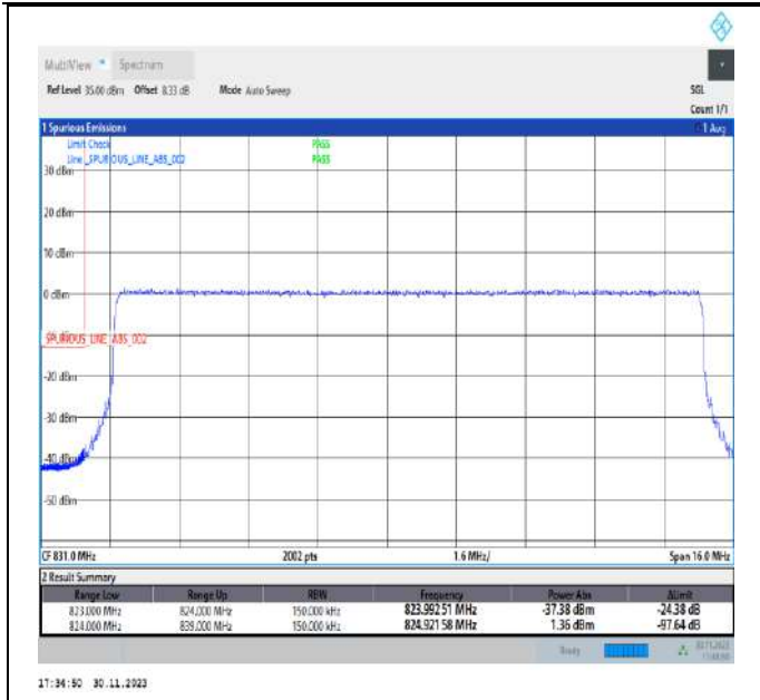
Band26_15MHz_64QAM_26865_75RB#0
