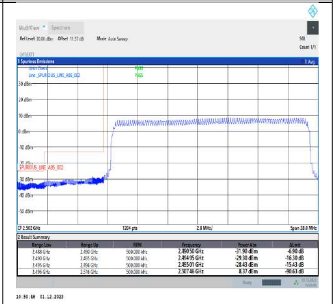
Band41_20MHz_QPSK_39750_100RB#0
