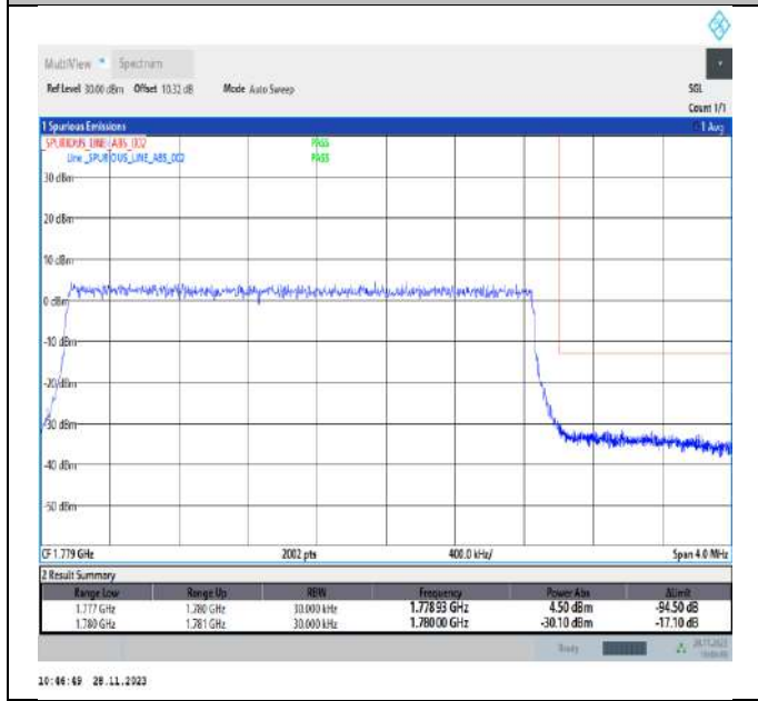
Band66_3MHz_64QAM_132657_15RB#0
