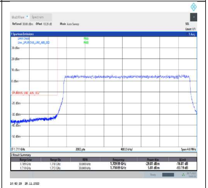
Band66_3MHz_QPSK_131987_15RB#0
