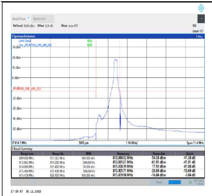
Band26_1.4MHz_QPSK_26697_1RB#5
