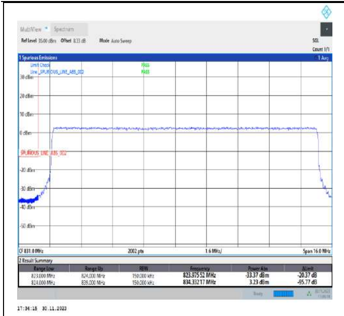
Band26_15MHz_QPSK_26865_75RB#0
