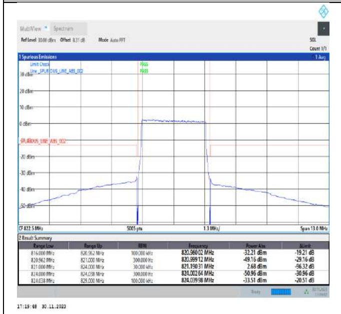
Band26_3MHz_64QAM_26775_15RB#0
