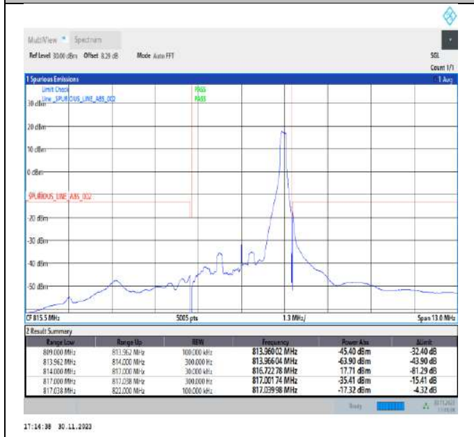
Band26_3MHz_QPSK_26705_1RB#14
