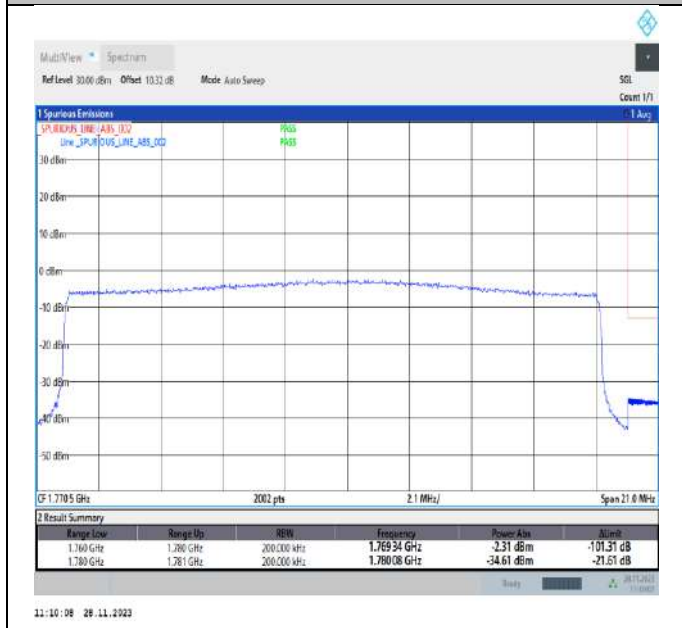
Band66_20MHz_64QAM_132572_100RB#0
