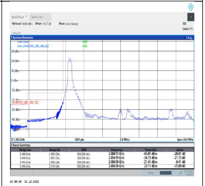
Band41_20MHz_16QAM_39750_1RB#0
