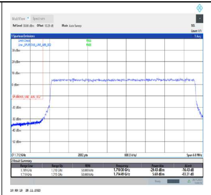
Band66_5MHz_QPSK_131997_25RB#0
