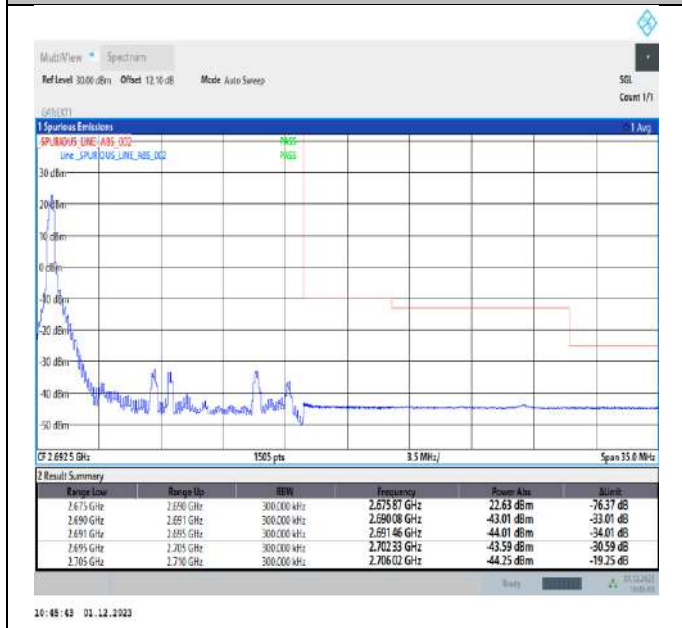
Band41_15MHz_64QAM_41515_1RB#0
