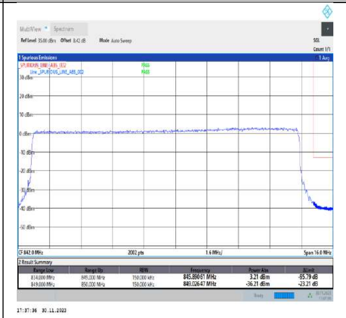
Band26_15MHz_64QAM_26965_75RB#0
