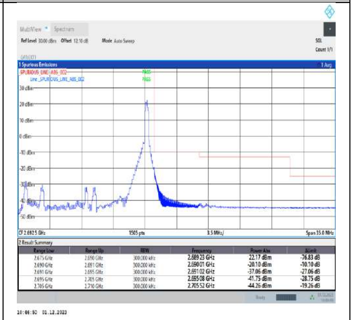
Band41_15MHz_64QAM_41515_1RB#74
