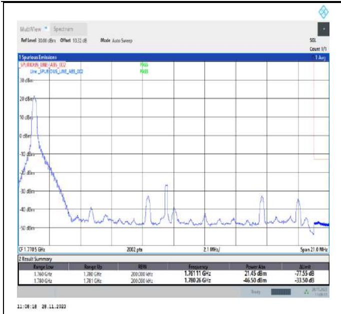
Band66_20MHz_64QAM_132572_1RB#0
