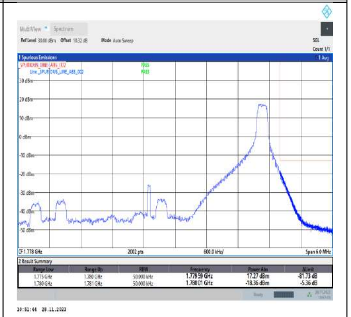
Band66_5MHz_64QAM_132647_1RB#24
