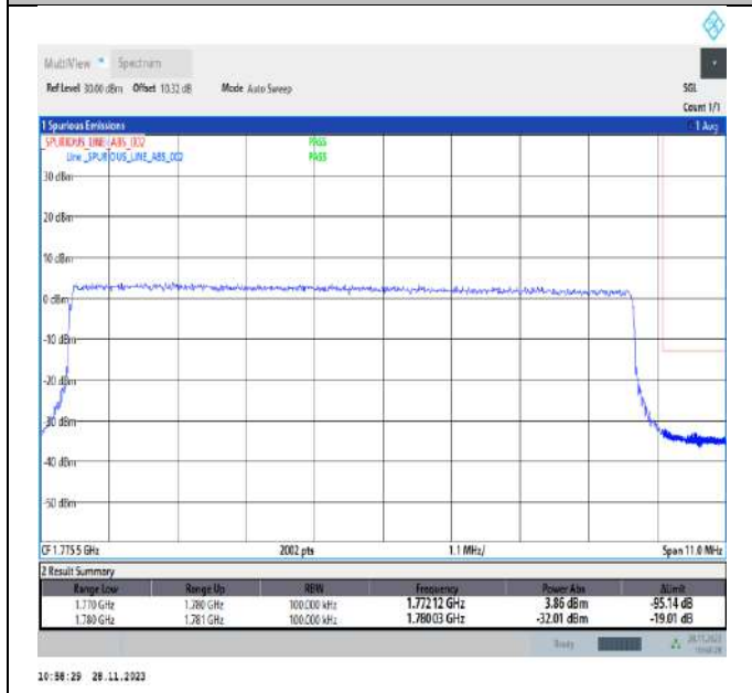
Band66_10MHz_64QAM_132622_50RB#0
