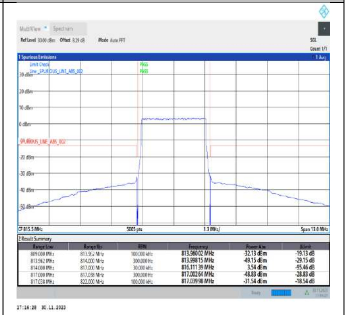
Band26_3MHz_64QAM_26705_15RB#0
