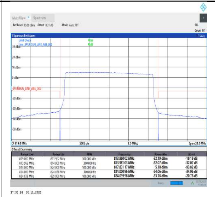
Band26_10MHz_QPSK_26740_50RB#0
