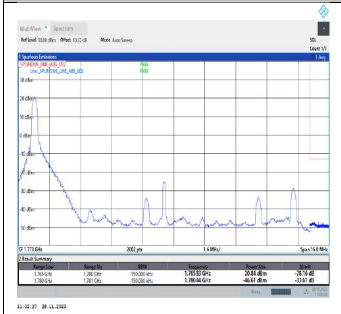
Band66_15MHz_64QAM_132597_1RB#0
