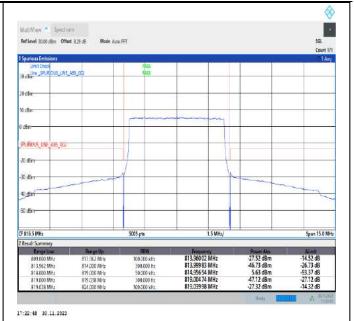
Band26_5MHz_QPSK_26715_25RB#0
