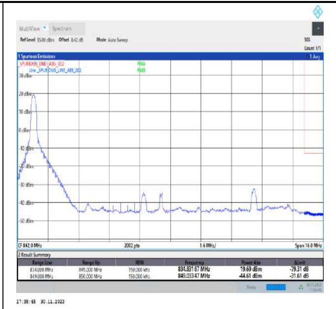
Band26_15MHz_64QAM_26965_1RB#0
