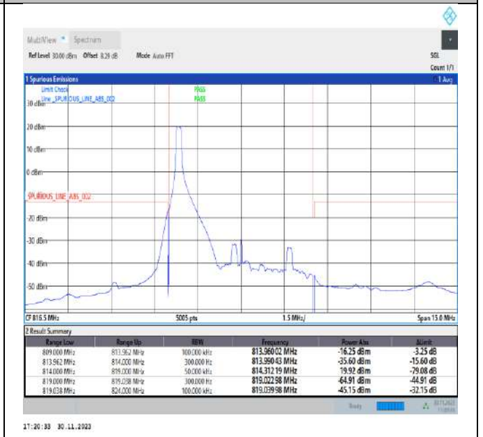
Band26_5MHz_QPSK_26715_1RB#0
