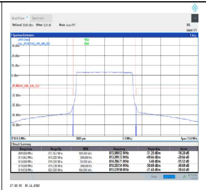
Band26_5MHz_64QAM_26715_25RB#0
