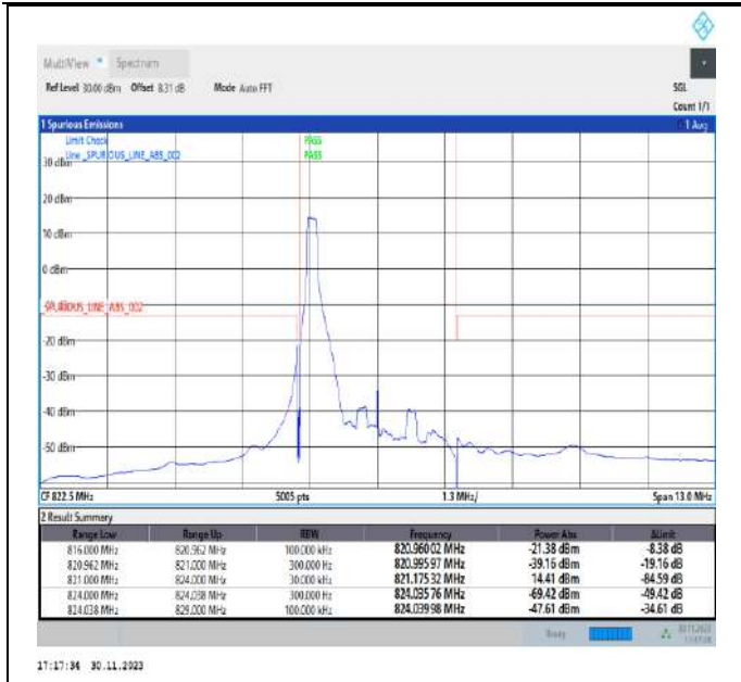
Band26_3MHz_64QAM_26775_1RB#0
