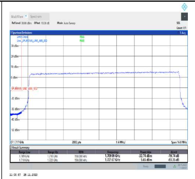
Band66_15MHz_QPSK_132047_75RB#0
