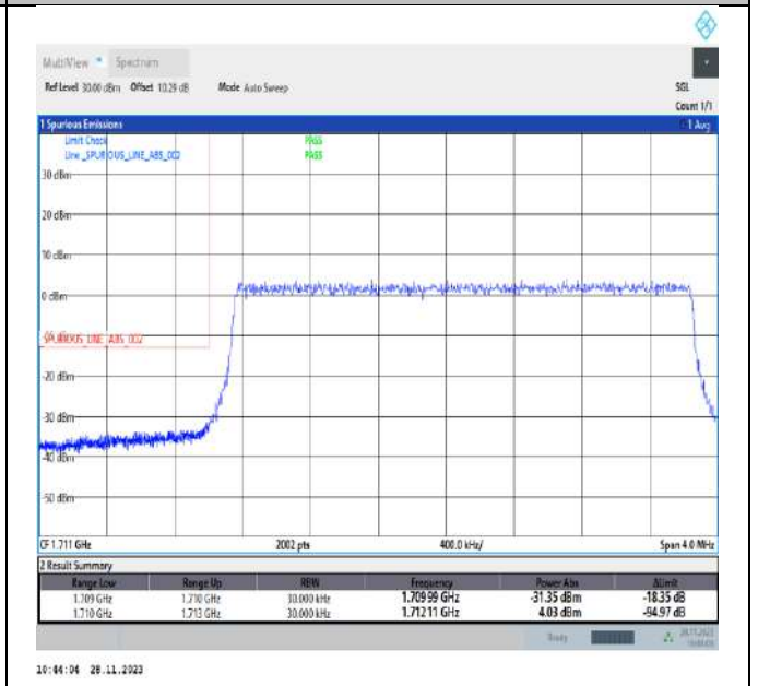
Band66_3MHz_64QAM_131987_15RB#0
