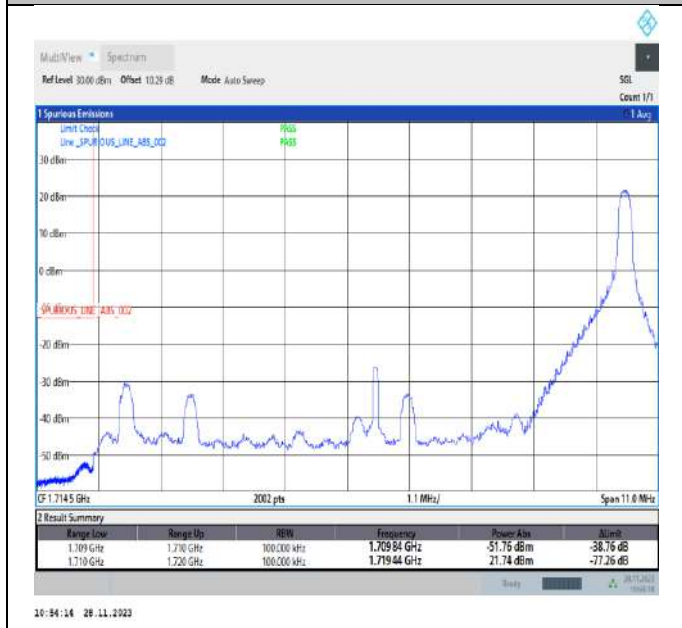
Band66_10MHz_QPSK_132022_1RB#49
