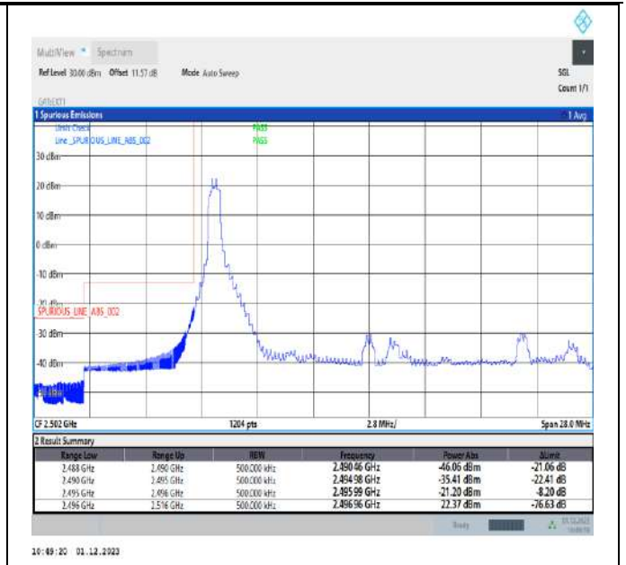
Band41_20MHz_64QAM_39750_1RB#0
