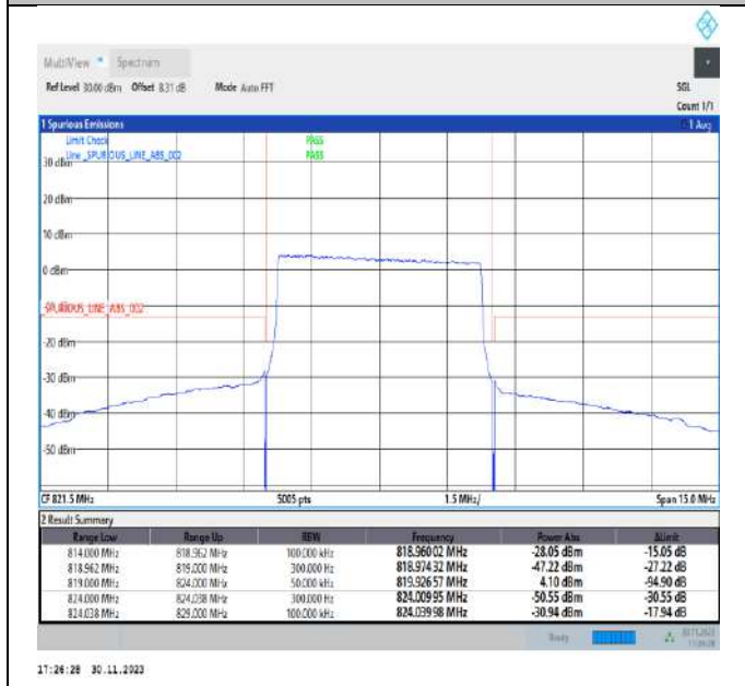
Band26_5MHz_16QAM_26765_25RB#0
