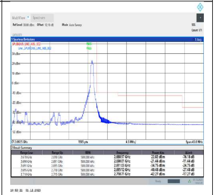
Band41_20MHz_16QAM_41490_1RB#99
