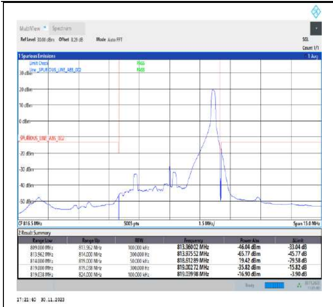
Band26_5MHz_QPSK_26715_1RB#24
