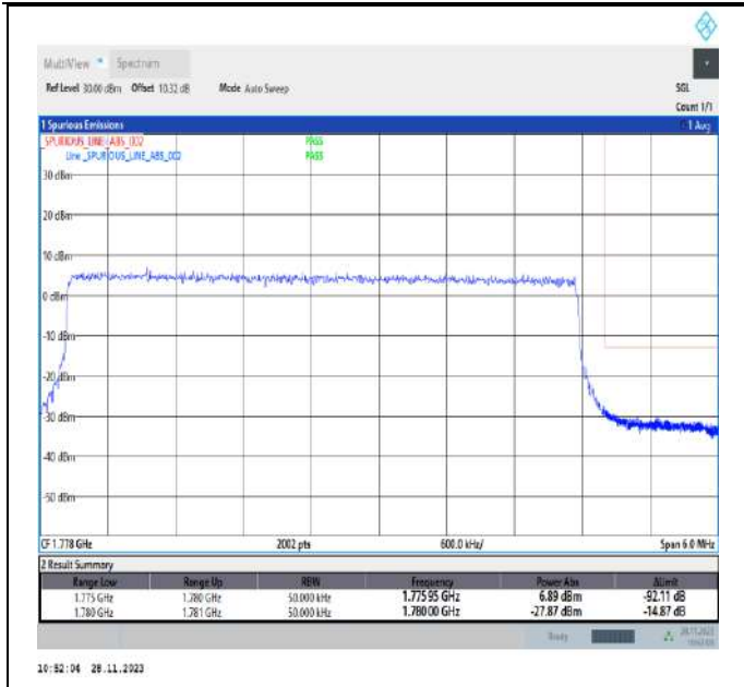
Band66_5MHz_QPSK_132647_25RB#0
