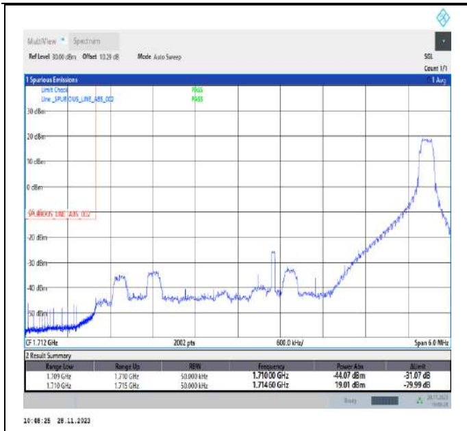
Band66_5MHz_QPSK_131997_1RB#24
