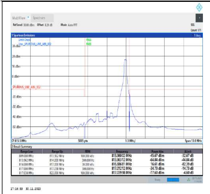
Band26_3MHz_16QAM_26705_1RB#14
