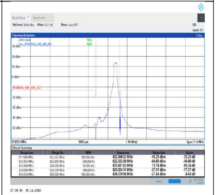
Band26_1.4MHz_64QAM_26783_1RB#5
