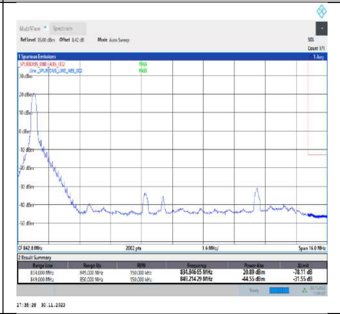
Band26_15MHz_16QAM_26965_1RB#0
