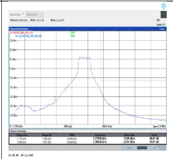
Band66_1.4MHz_64QAM_132665_1RB#5
