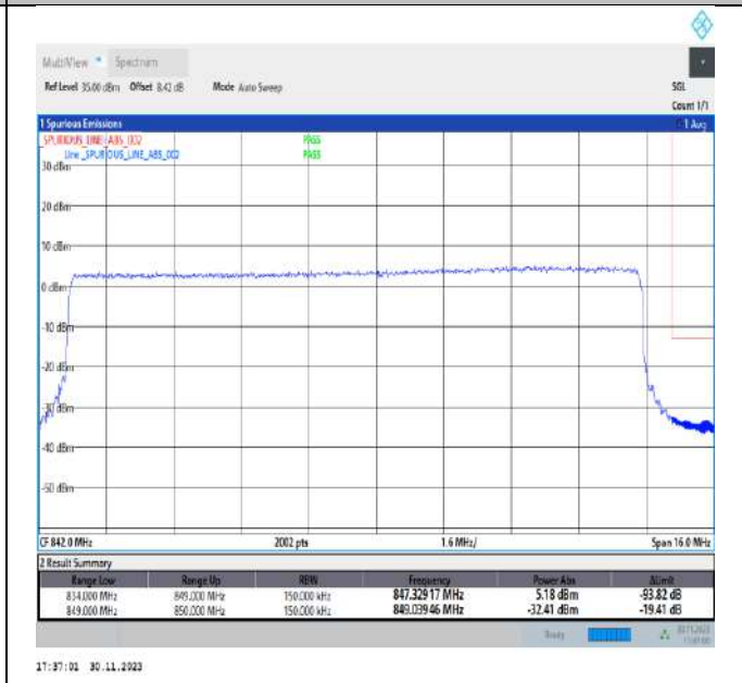
Band26_15MHz_QPSK_26965_75RB#0
