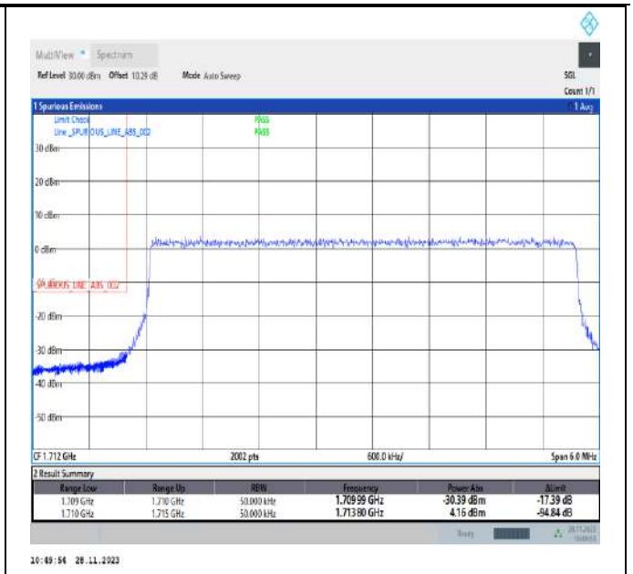
Band66_5MHz_64QAM_131997_25RB#0
