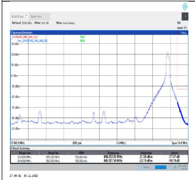
Band26_15MHz_64QAM_26965_1RB#74
