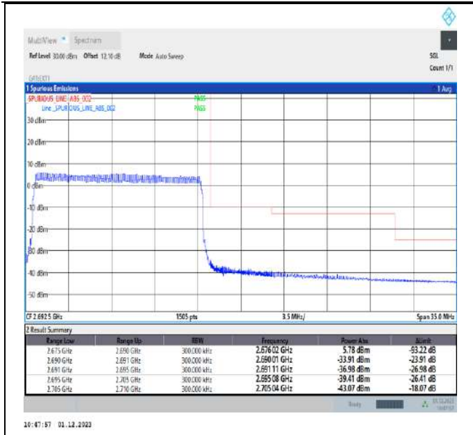
Band41_15MHz_64QAM_41515_75RB#0
