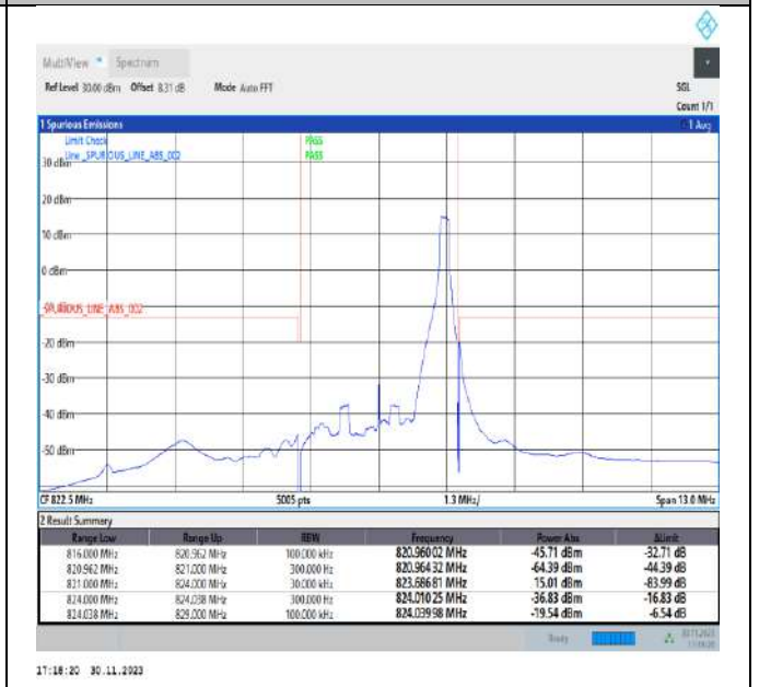
Band26_3MHz_16QAM_26775_1RB#14
