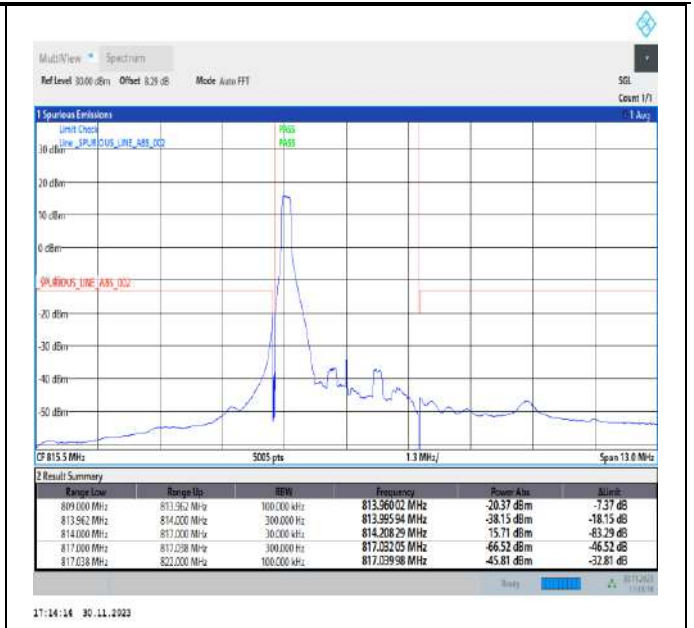
Band26_3MHz_64QAM_26705_1RB#0
