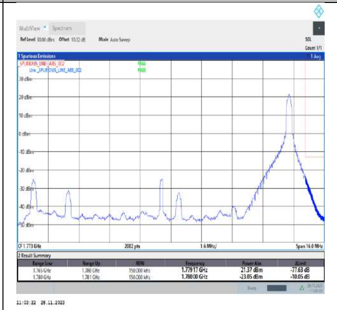
Band66_15MHz_64QAM_132597_1RB#74
