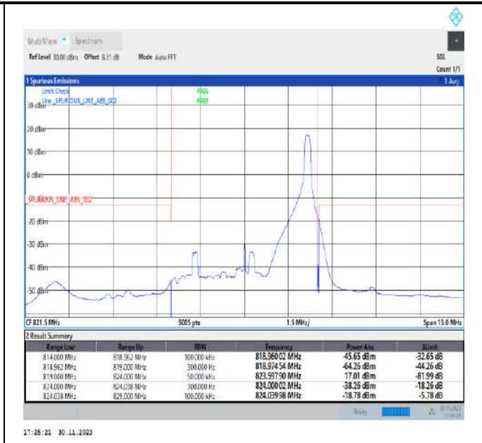
Band26_5MHz_16QAM_26765_1RB#24
