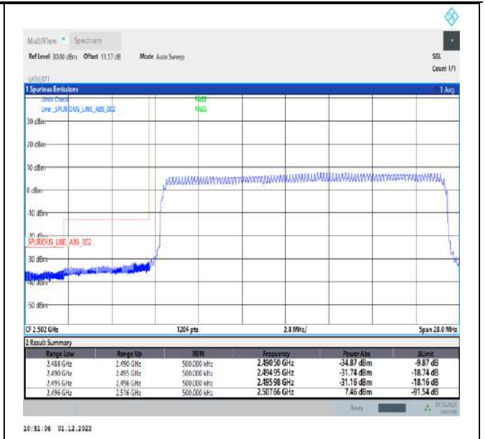
Band41_20MHz_16QAM_39750_100RB#0
