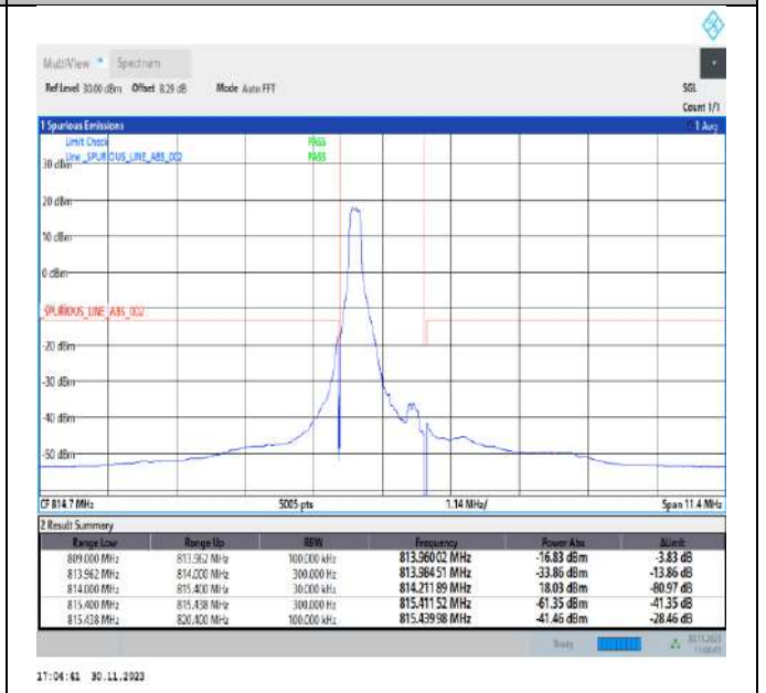
Band26_1.4MHz_QPSK_26697_1RB#0
