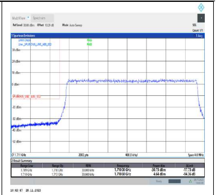
Band66_3MHz_16QAM_131987_15RB#0
