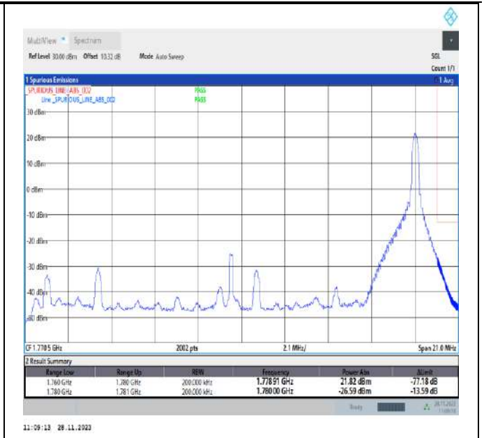
Band66_20MHz_64QAM_132572_1RB#99
