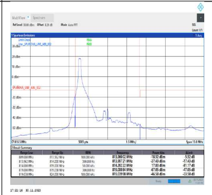
Band26_5MHz_64QAM_26715_1RB#0
