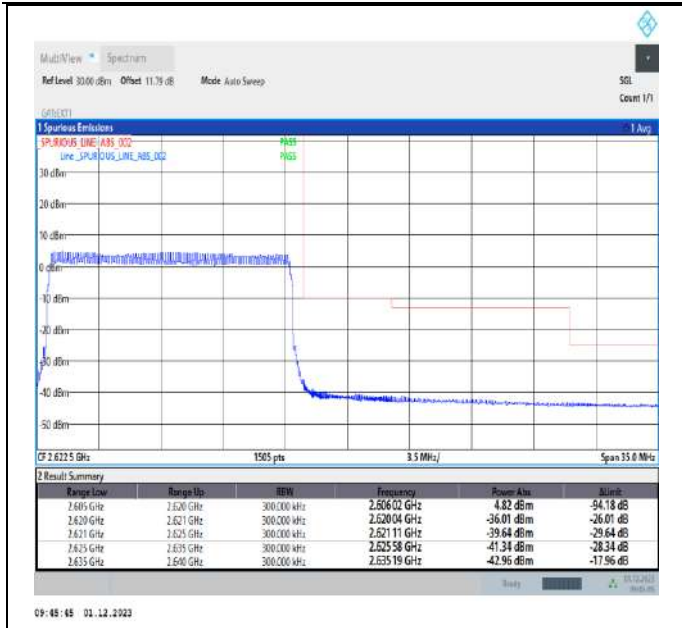
Band38_15MHz_64QAM_38175_75RB#0
