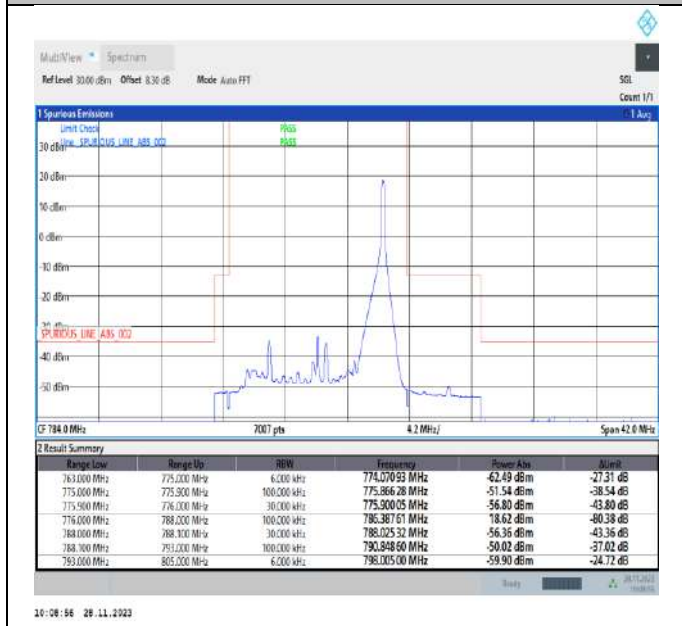
Band13_10MHz_16QAM_23230_1RB#49
