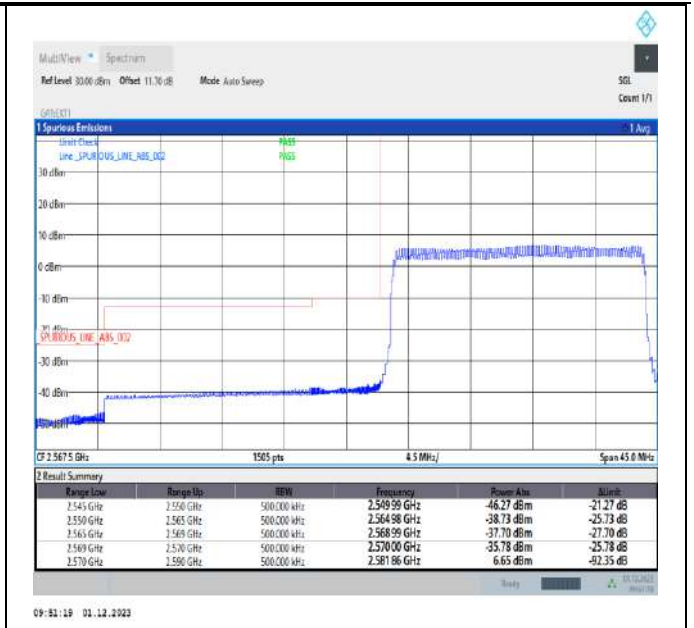
Band38_20MHz_16QAM_37850_100RB#0
