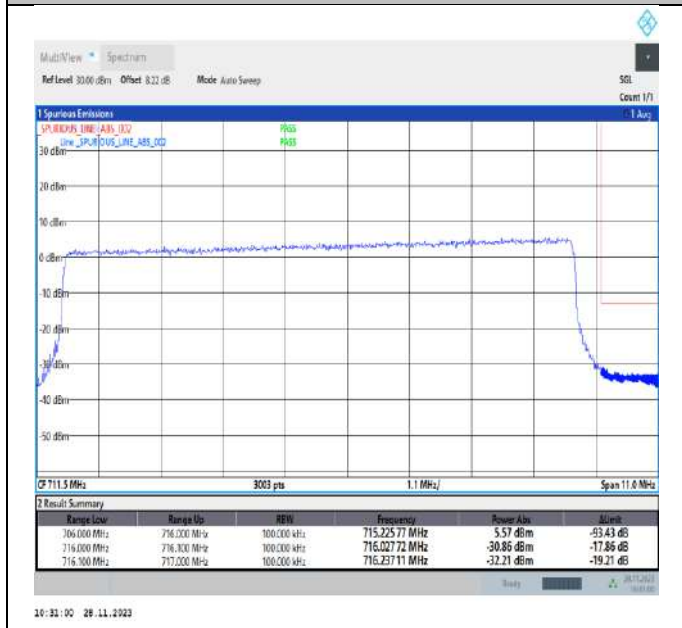
Band17_10MHz_QPSK_23800_50RB#0
