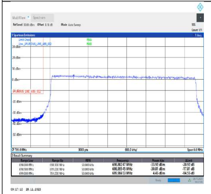
Band12_5MHz_QPSK_23035_25RB#0
