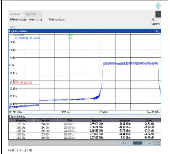
Band38_10MHz_64QAM_37800_50RB#0
