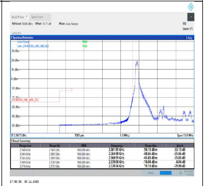
Band38_5MHz_64QAM_37775_1RB#0
