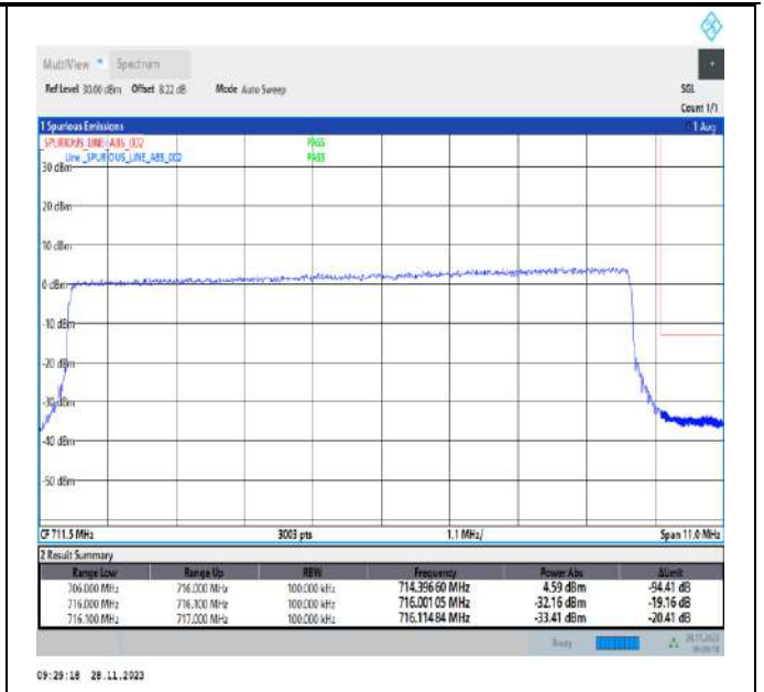
Band12_10MHz_16QAM_23130_50RB#0
