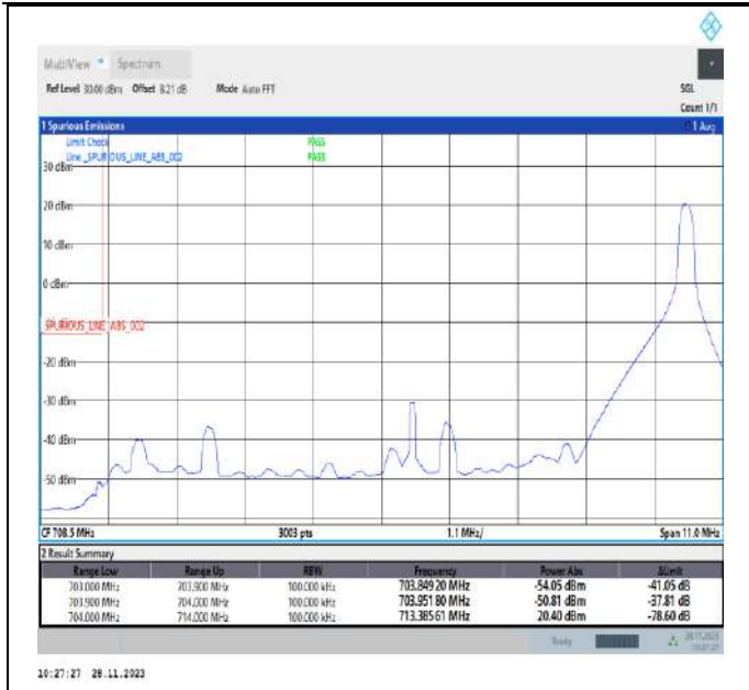
Band17_10MHz_16QAM_23780_1RB#49
