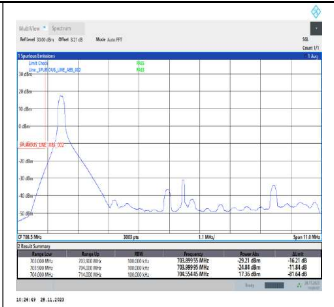
Band17_10MHz_64QAM_23780_1RB#0
