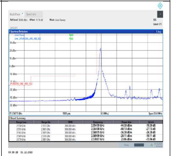
Band38_15MHz_QPSK_37825_1RB#0
