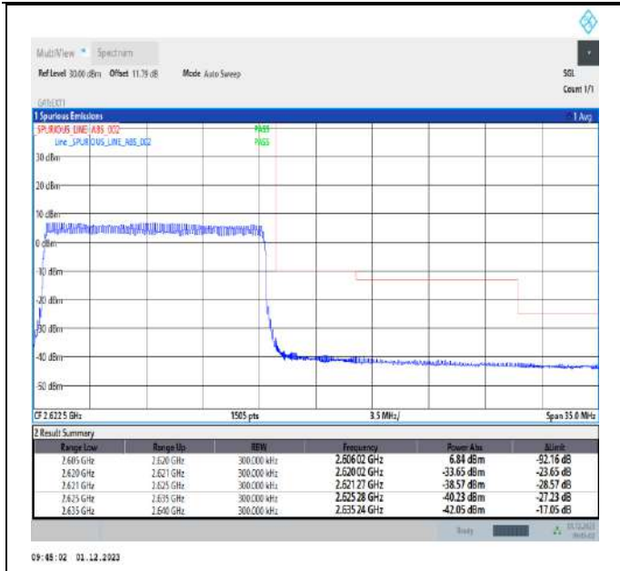
Band38_15MHz_QPSK_38175_75RB#0
