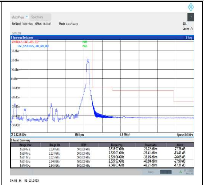
Band38_20MHz_64QAM_38150_1RB#99
