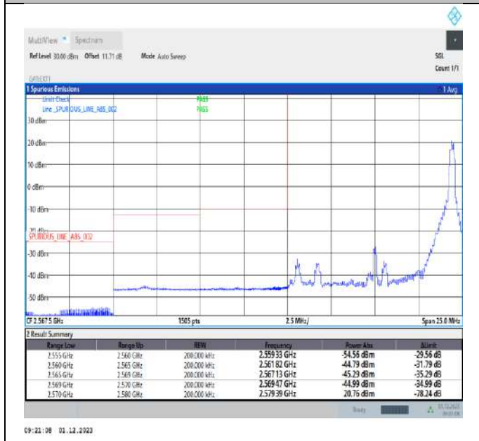
Band38_10MHz_64QAM_37800_1RB#49
