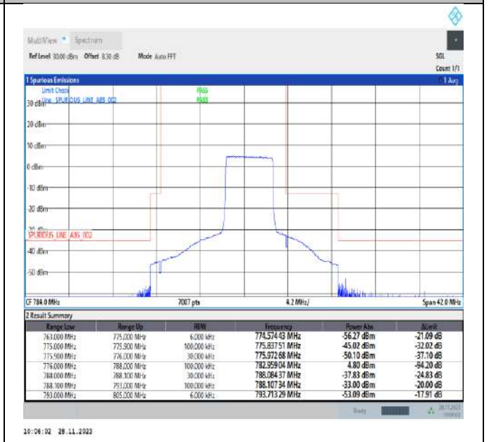
Band13_5MHz_16QAM_23255_25RB#0
