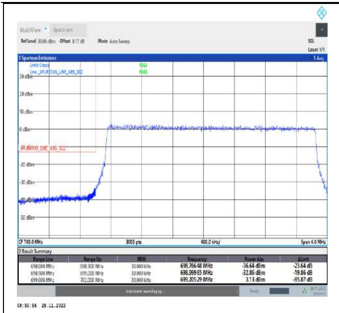
Band12_3MHz_64QAM_23025_15RB#0
