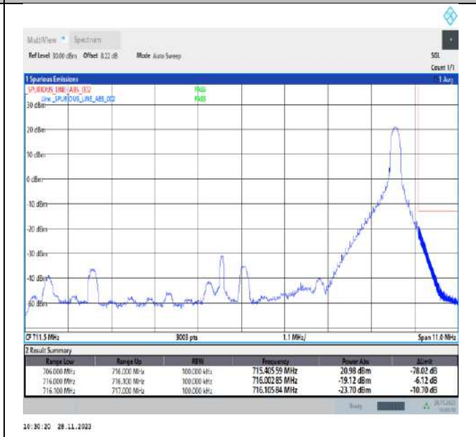
Band17_10MHz_16QAM_23800_1RB#49
