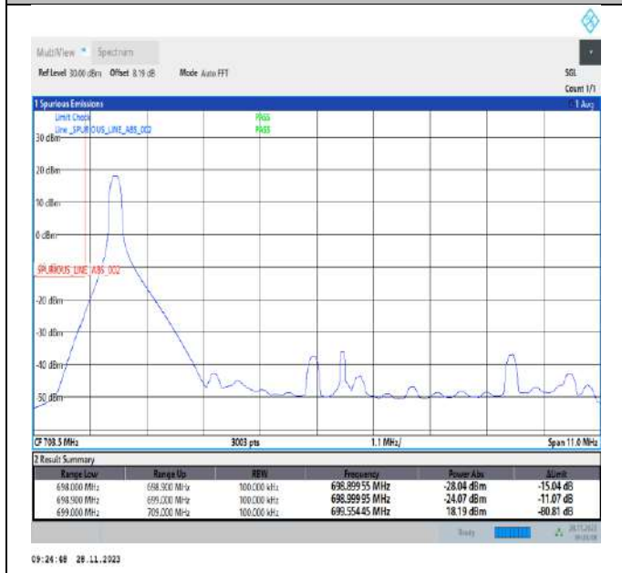
Band12_10MHz_64QAM_23060_1RB#0
