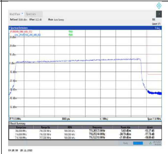
Band12_10MHz_QPSK_23130_50RB#0
