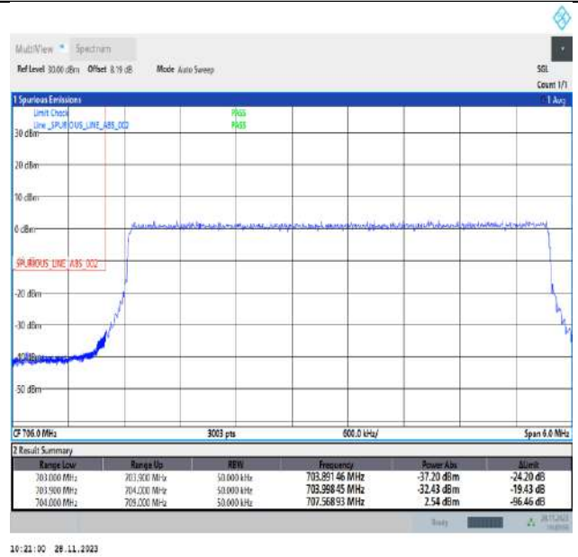
Band17_5MHz_16QAM_23755_25RB#0
