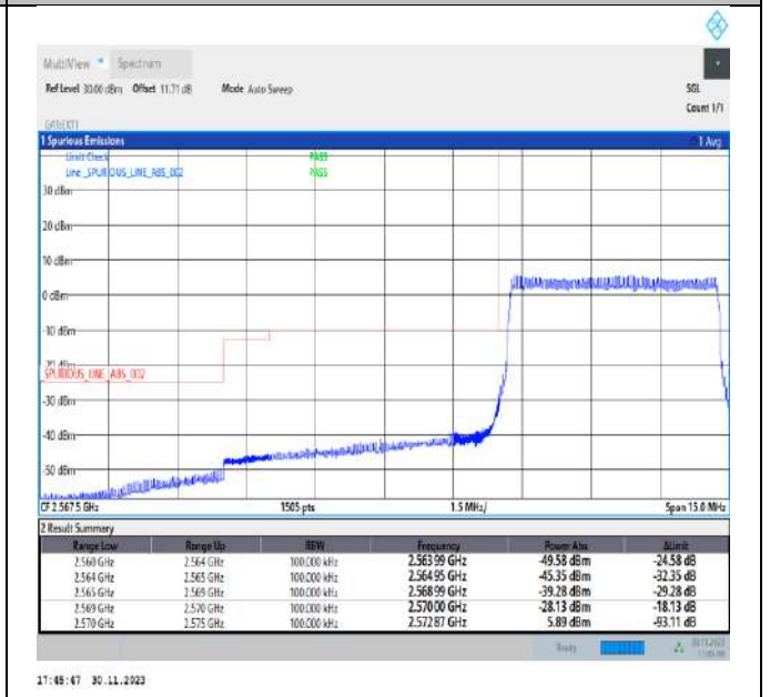
Band38_5MHz_16QAM_37775_25RB#0
