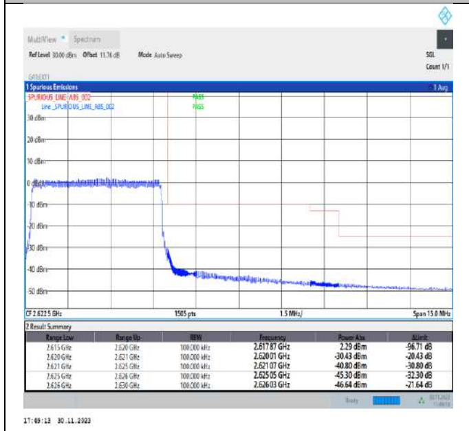
Band38_5MHz_16QAM_38225_25RB#0
