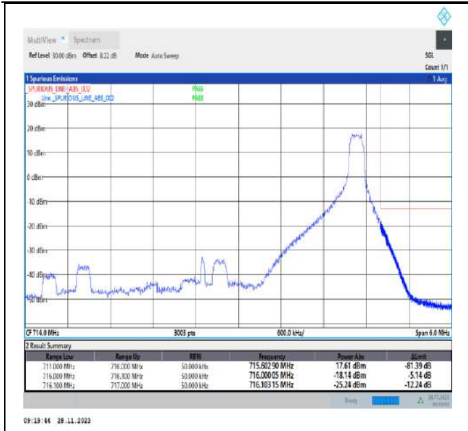
Band12_5MHz_64QAM_23155_1RB#24
