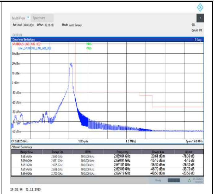
Band41_5MHz_16QAM_41565_1RB#24
