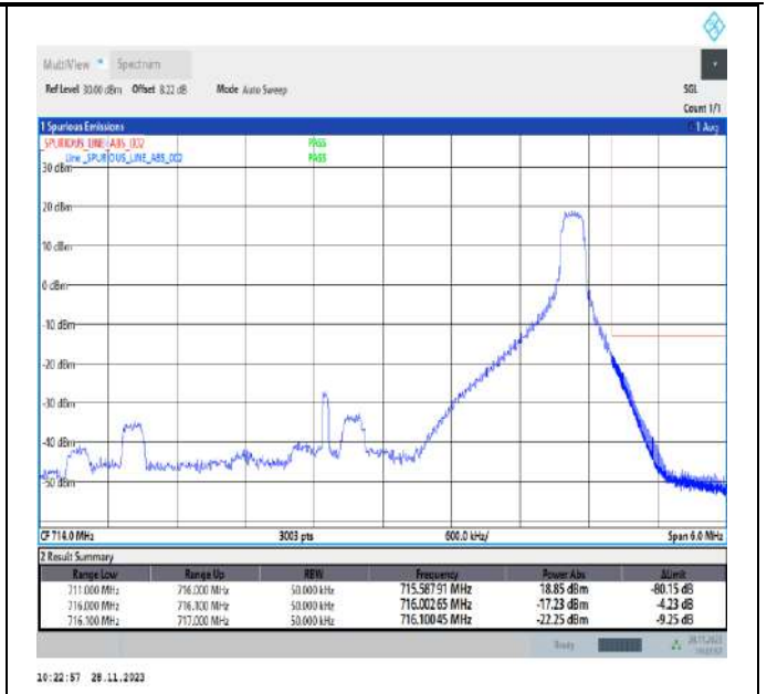
Band17_5MHz_16QAM_23825_1RB#24
