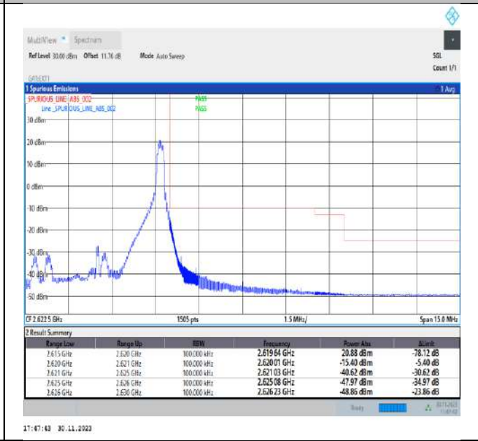
Band38_5MHz_QPSK_38225_1RB#24
