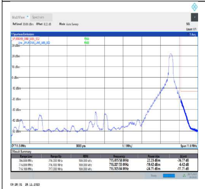
Band12_10MHz_QPSK_23130_1RB#49
