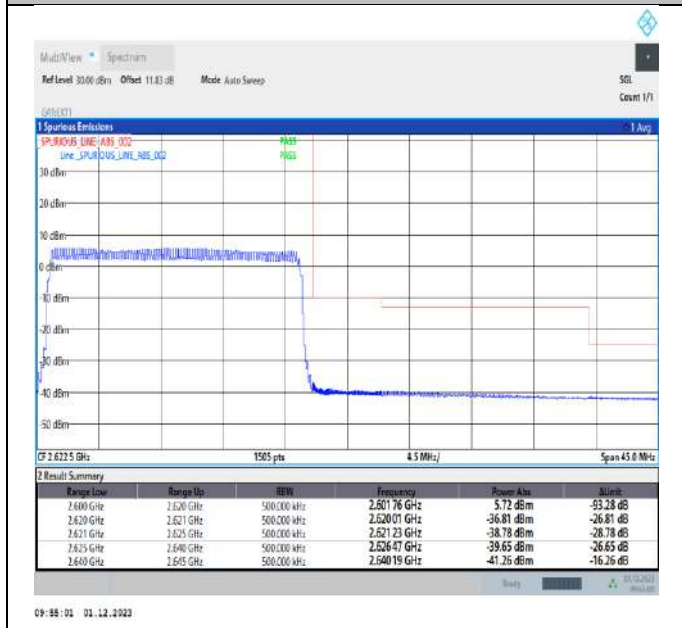
Band38_20MHz_64QAM_38150_100RB#0
