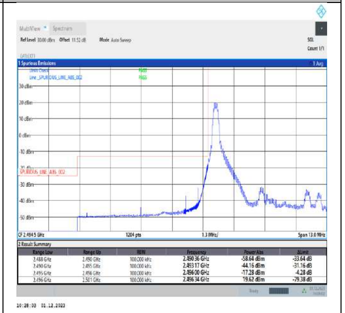
Band41_5MHz_64QAM_39675_1RB#0
