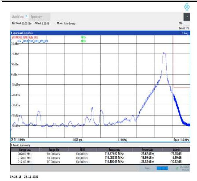
Band12_10MHz_16QAM_23130_1RB#49
