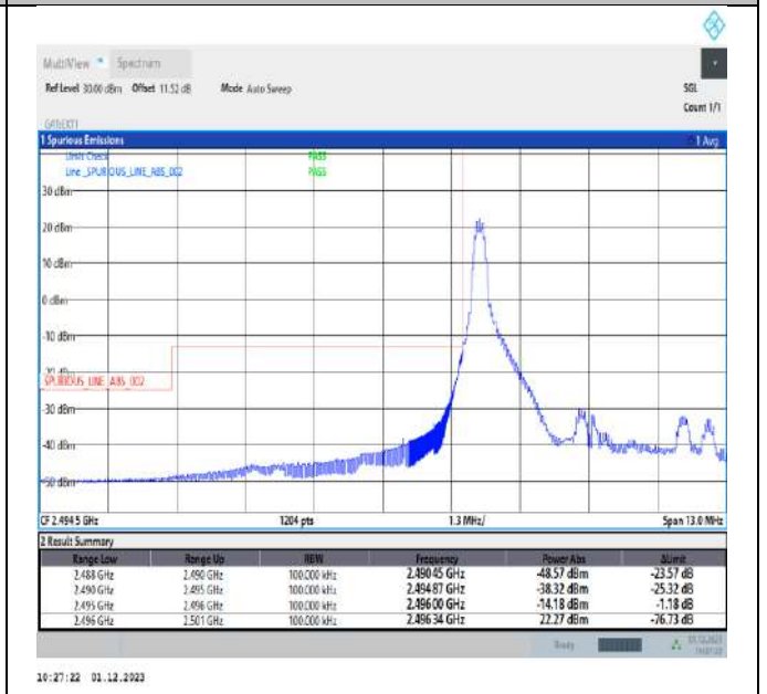
Band41_5MHz_QPSK_39675_1RB#0
