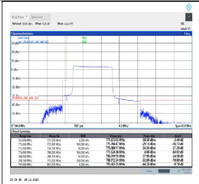
Band13_10MHz_QPSK_23230_50RB#0
