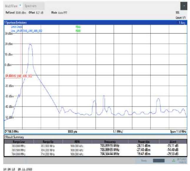
Band17_10MHz_QPSK_23780_1RB#0
