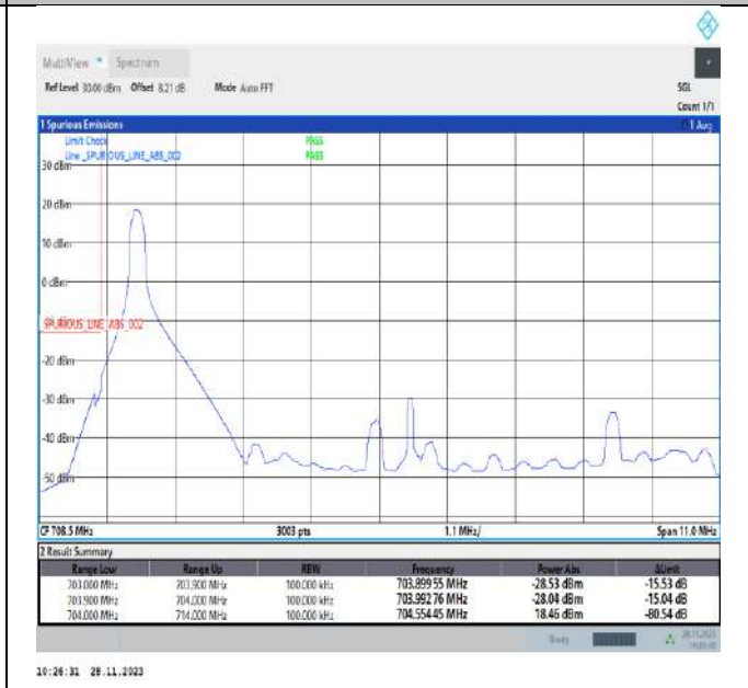
Band17_10MHz_16QAM_23780_1RB#0
