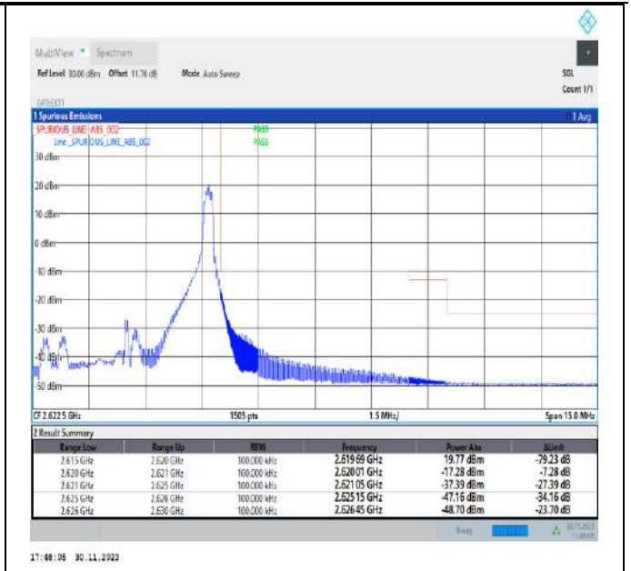
Band38_5MHz_16QAM_38225_1RB#24
