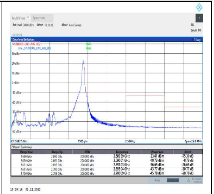
Band41_10MHz_QPSK_41540_1RB#49
