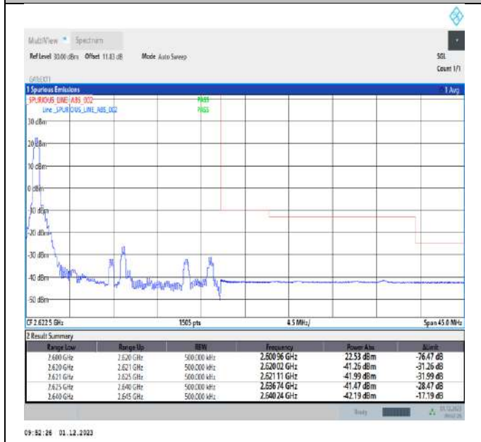
Band38_20MHz_16QAM_38150_1RB#0
