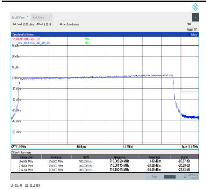
Band17_10MHz_64QAM_23800_50RB#0
