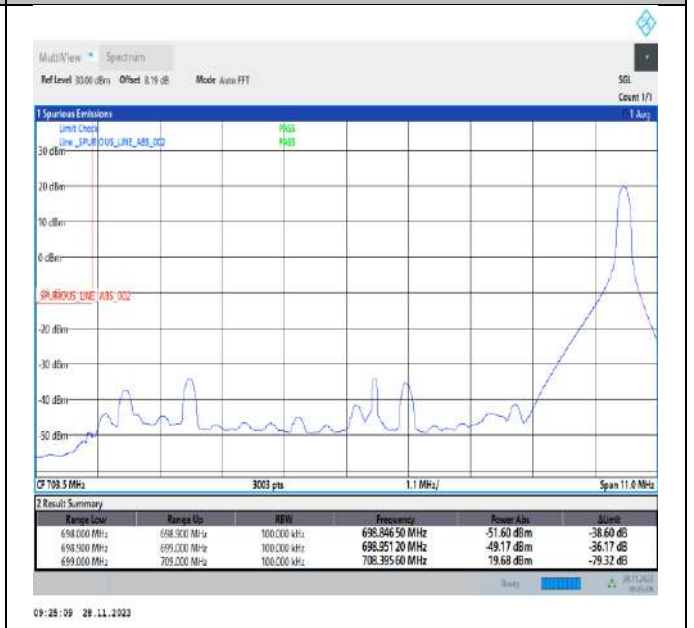
Band12_10MHz_QPSK_23060_1RB#49
