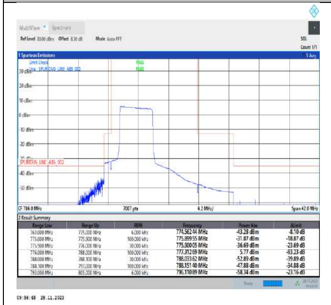
Band13_5MHz_64QAM_23205_25RB#0
