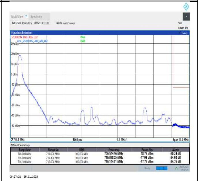
Band12_10MHz_16QAM_23130_1RB#0
