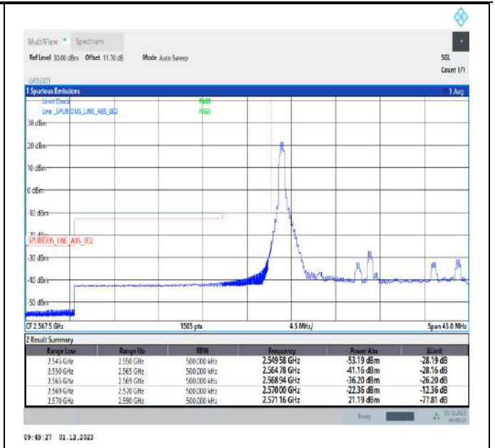
Band38_20MHz_64QAM_37850_1RB#0
