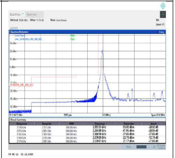
Band38_15MHz_64QAM_37825_1RB#0
