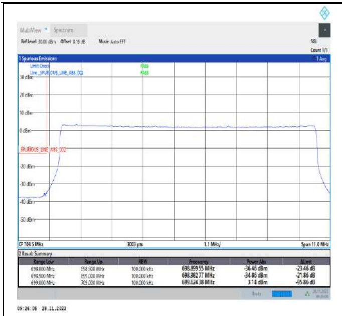
Band12_10MHz_QPSK_23060_50RB#0
