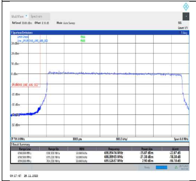
Band12_5MHz_64QAM_23035_25RB#0
