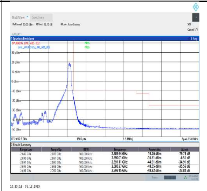
Band41_5MHz_64QAM_41565_1RB#24
