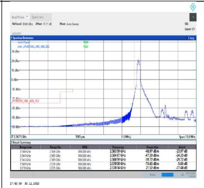
Band38_5MHz_QPSK_37775_1RB#0
