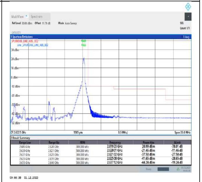
Band38_15MHz_64QAM_38175_1RB#74
