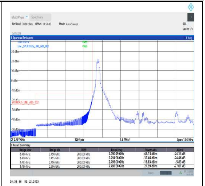
Band41_10MHz_64QAM_39700_1RB#0
