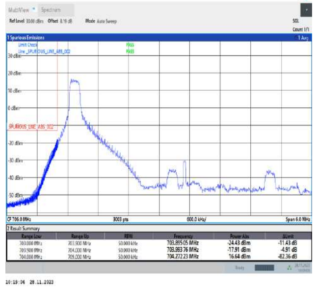
Band17_5MHz_16QAM_23755_1RB#0
