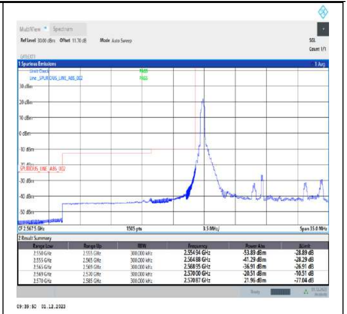
Band38_15MHz_16QAM_37825_1RB#0
