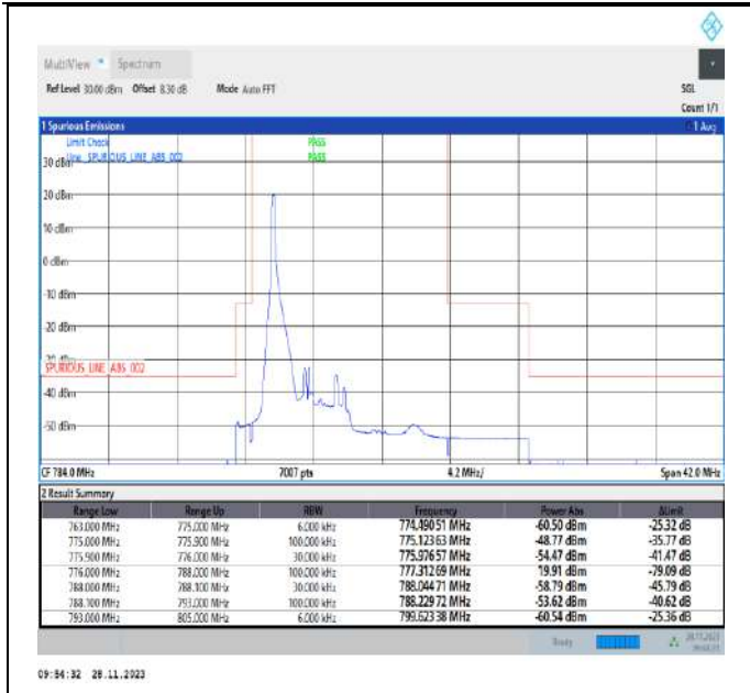
Band13_5MHz_64QAM_23205_1RB#0
