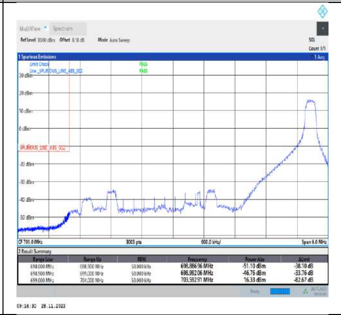
Band12_5MHz_16QAM_23035_1RB#24
