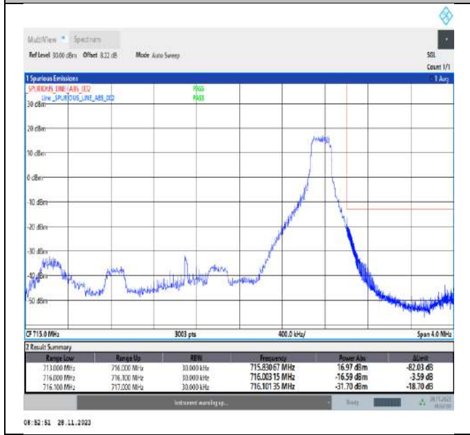
Band12_3MHz_64QAM_23165_1RB#14
