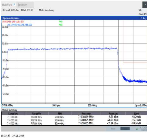
Band17_5MHz_QPSK_23825_25RB#0
