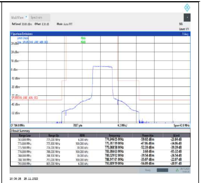
Band13_5MHz_64QAM_23255_25RB#0
