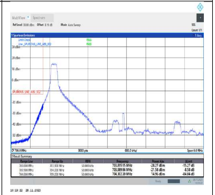
Band17_5MHz_64QAM_23755_1RB#0
