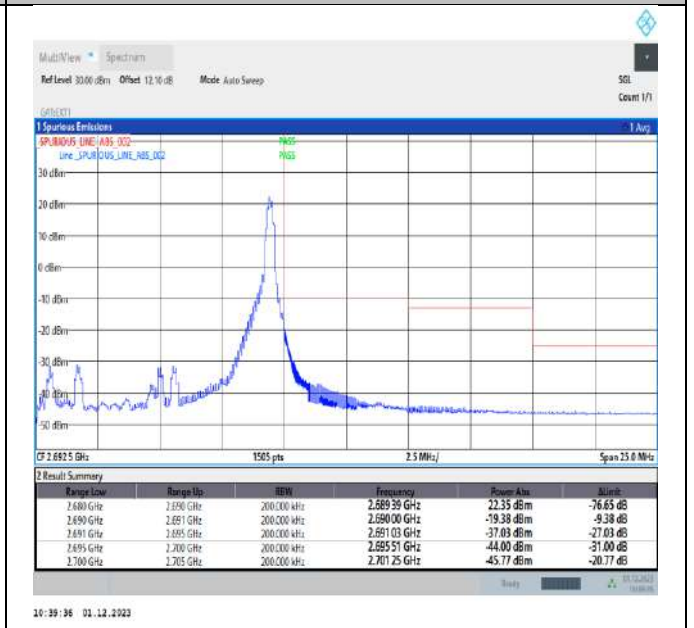
Band41_10MHz_16QAM_41540_1RB#49
