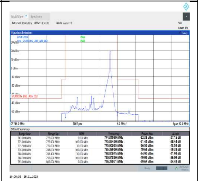
Band13_10MHz_QPSK_23230_1RB#49
