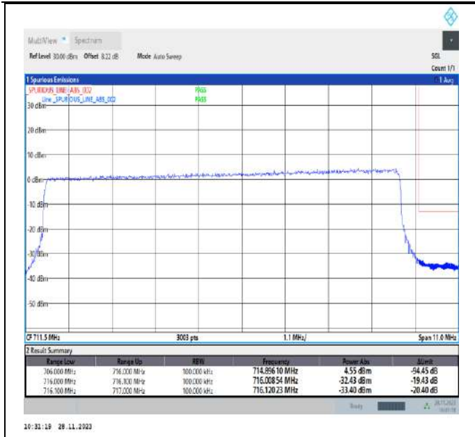
Band17_10MHz_16QAM_23800_50RB#0
