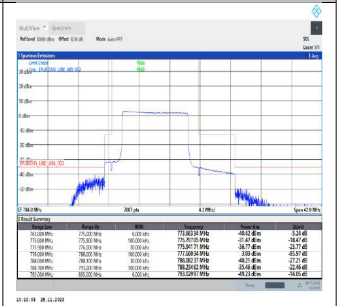
Band13_10MHz_16QAM_23230_50RB#0
