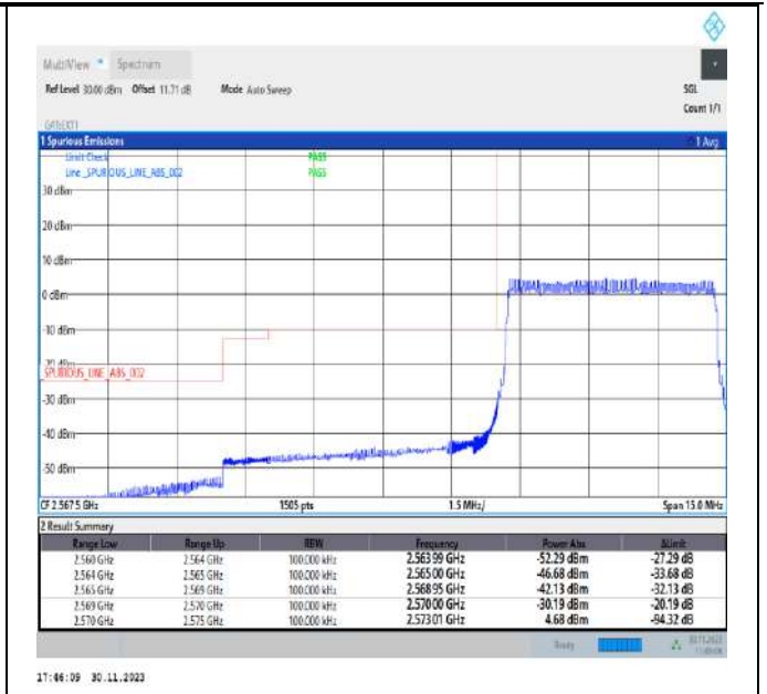
Band38_5MHz_64QAM_37775_25RB#0
