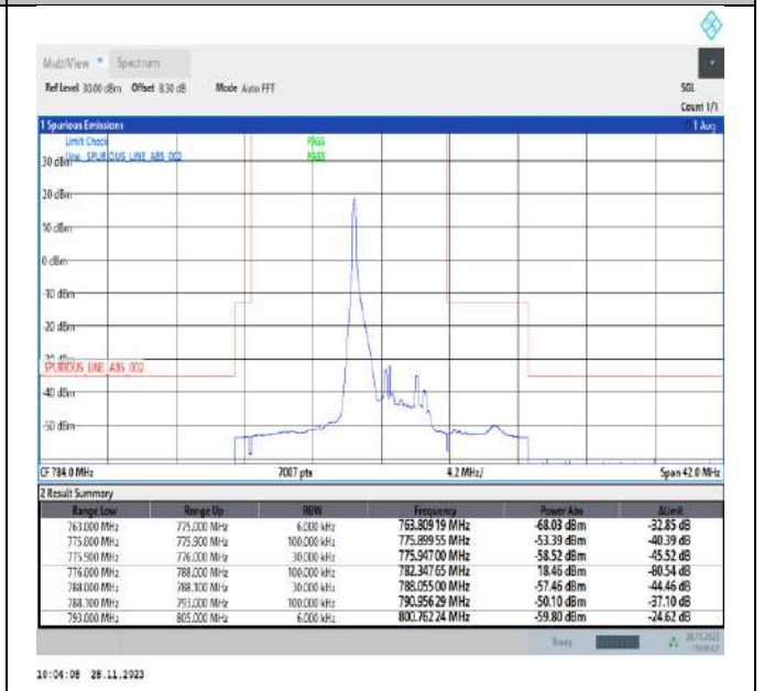
Band13_5MHz_64QAM_23255_1RB#0
