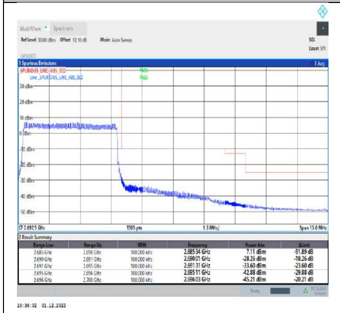
Band41_5MHz_16QAM_41565_25RB#0
