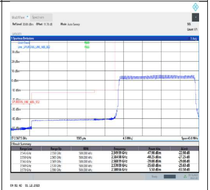
Band38_20MHz_64QAM_37850_100RB#0
