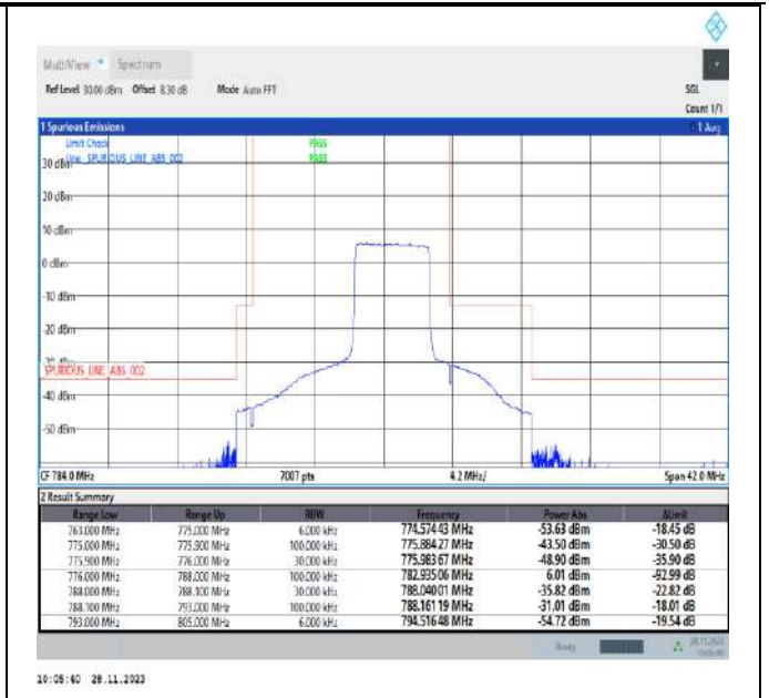
Band13_5MHz_QPSK_23255_25RB#0
