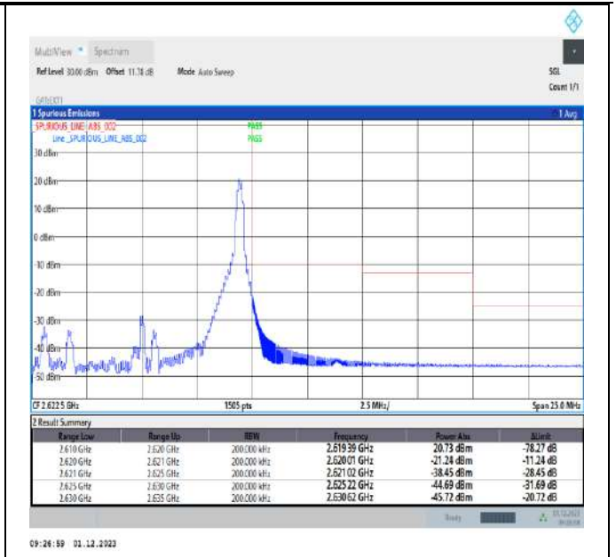
Band38_10MHz_64QAM_38200_1RB#49
