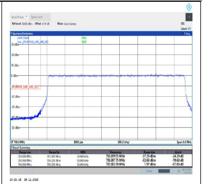
Band17_5MHz_64QAM_23755_25RB#0
