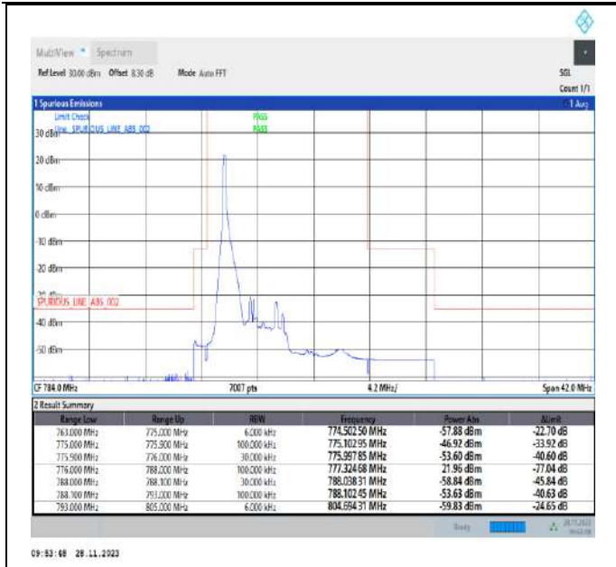
Band13_5MHz_QPSK_23205_1RB#0
