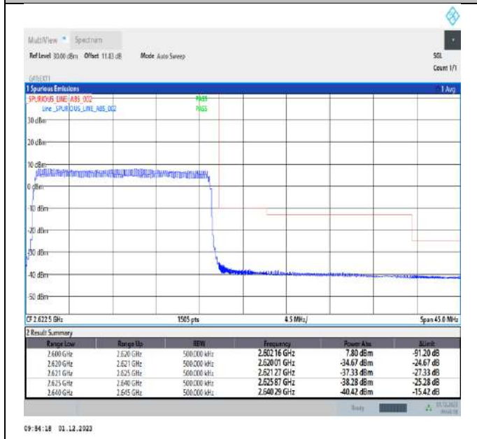
Band38_20MHz_QPSK_38150_100RB#0
