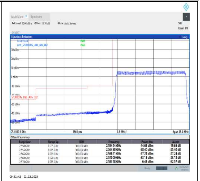
Band38_15MHz_QPSK_37825_75RB#0
