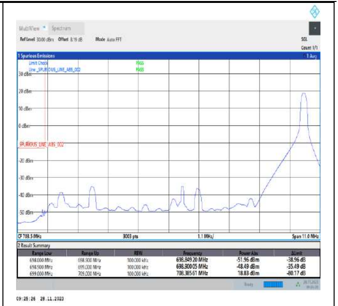
Band12_10MHz_16QAM_23060_1RB#49
