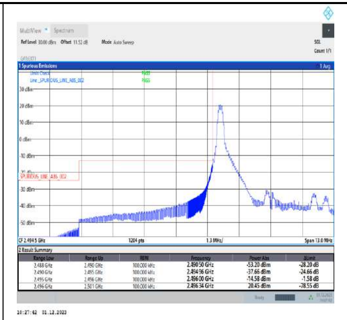
Band41_5MHz_16QAM_39675_1RB#0
