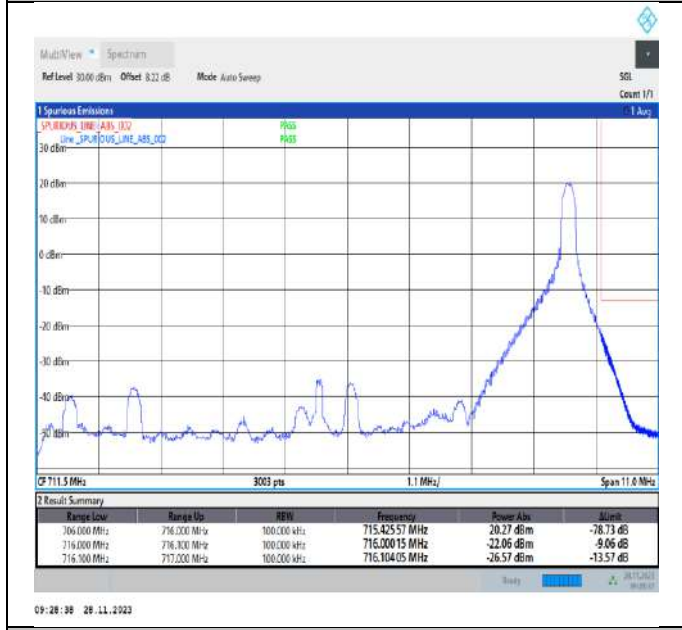
Band12_10MHz_64QAM_23130_1RB#49
