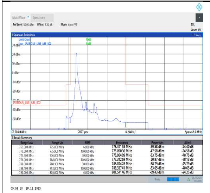
Band13_5MHz_16QAM_23205_1RB#0
