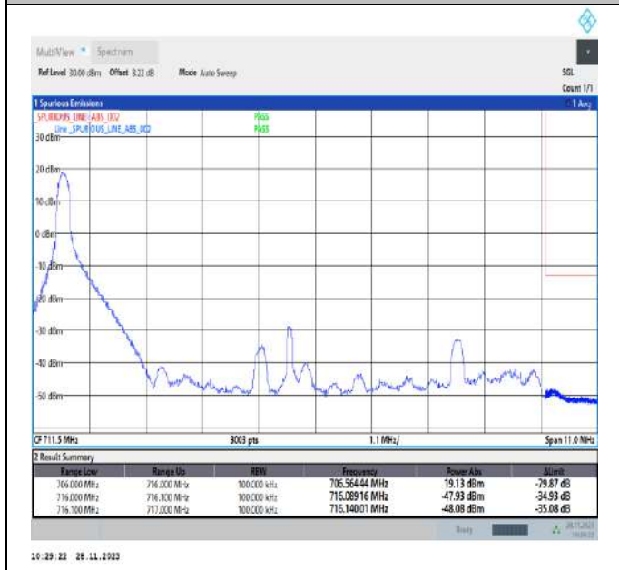
Band17_10MHz_16QAM_23800_1RB#0
