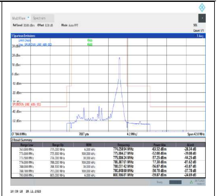
Band13_10MHz_64QAM_23230_1RB#49
