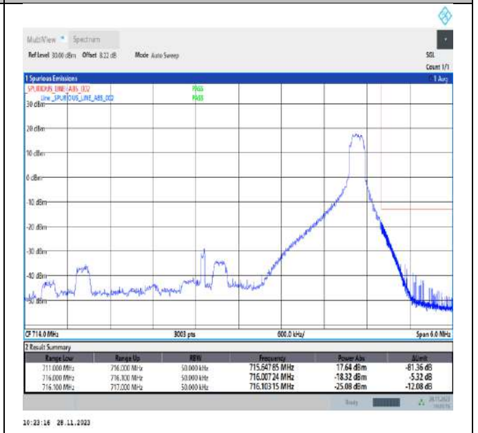
Band17_5MHz_64QAM_23825_1RB#24
