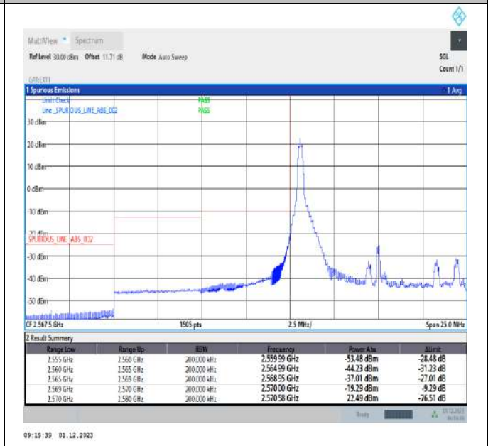
Band38_10MHz_16QAM_37800_1RB#0
