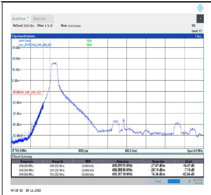
Band12_5MHz_64QAM_23035_1RB#0
