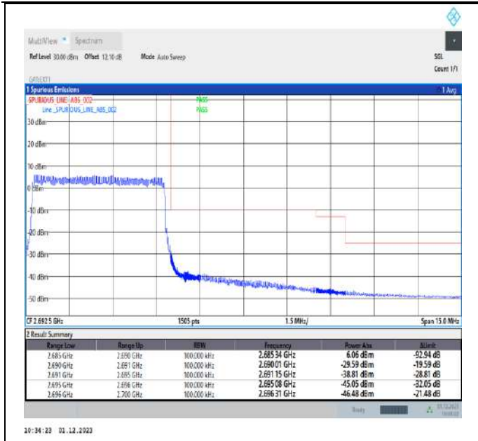
Band41_5MHz_64QAM_41565_25RB#0
