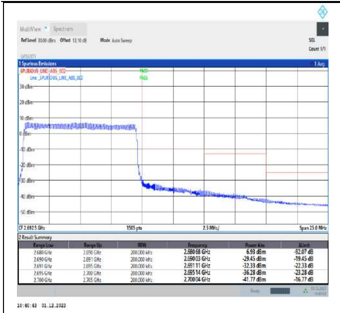
Band41_10MHz_16QAM_41540_50RB#0
