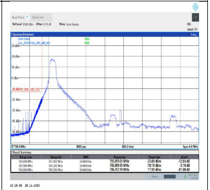
Band17_5MHz_QPSK_23755_1RB#0
