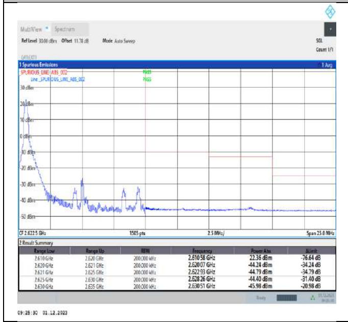
Band38_10MHz_16QAM_38200_1RB#0
