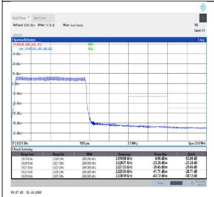
Band38_10MHz_QPSK_38200_50RB#0
