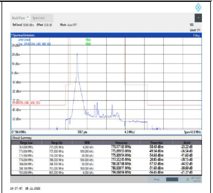
Band13_10MHz_16QAM_23230_1RB#0
