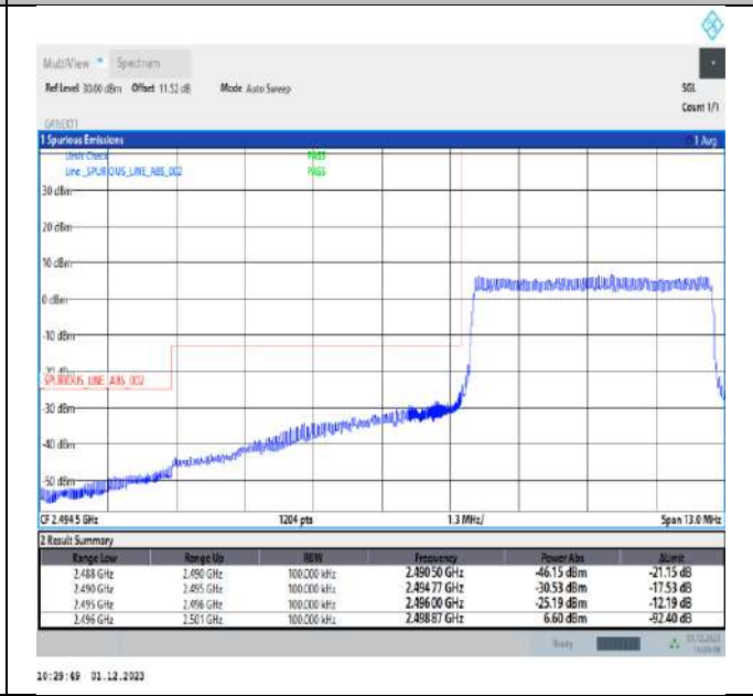
Band41_5MHz_16QAM_39675_25RB#0
