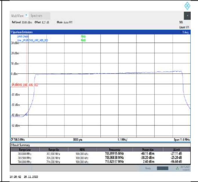
Band17_10MHz_64QAM_23780_50RB#0
