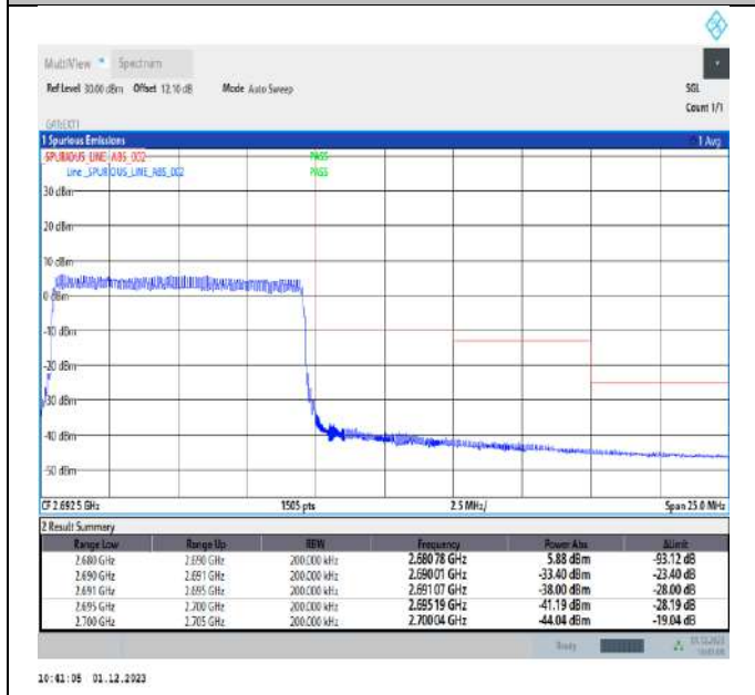
Band41_10MHz_64QAM_41540_50RB#0
