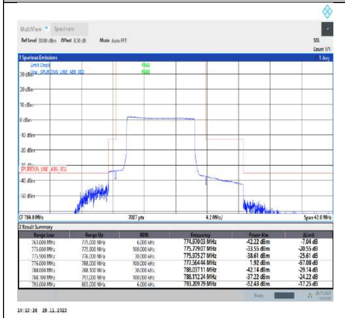
Band13_10MHz_64QAM_23230_50RB#0
