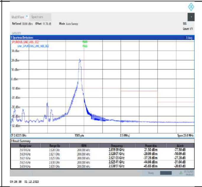
Band38_10MHz_16QAM_38200_1RB#49
