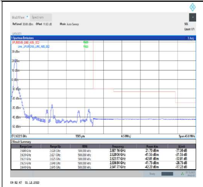
Band38_20MHz_64QAM_38150_1RB#0
