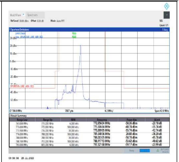
Band13_5MHz_QPSK_23205_1RB#24
