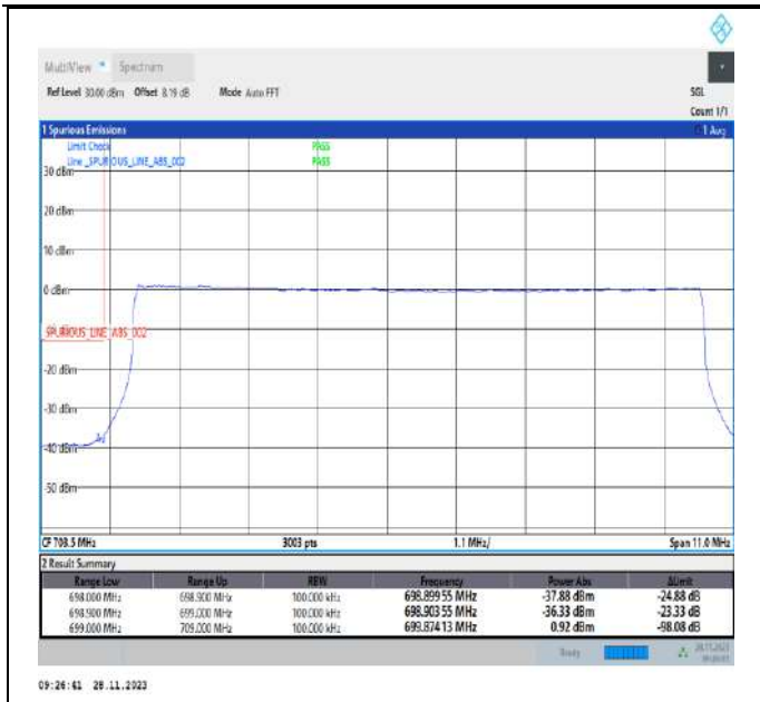
Band12_10MHz_64QAM_23060_50RB#0
