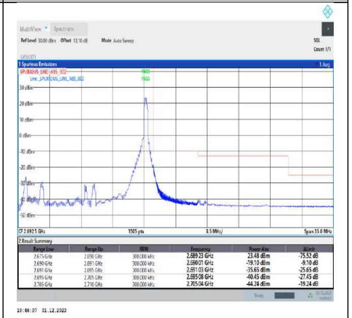
Band41_15MHz_QPSK_41515_1RB#74
