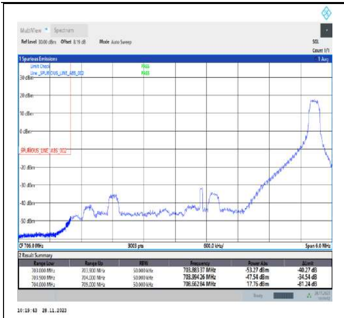
Band17_5MHz_QPSK_23755_1RB#24
