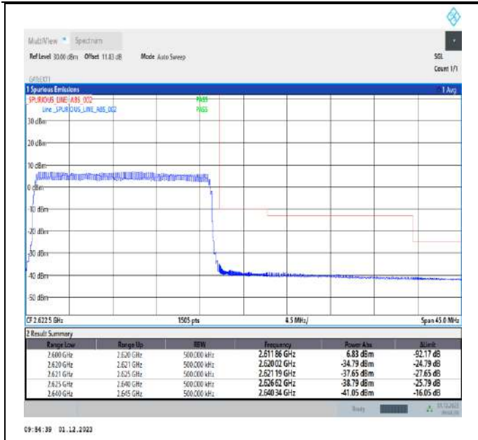
Band38_20MHz_16QAM_38150_100RB#0
