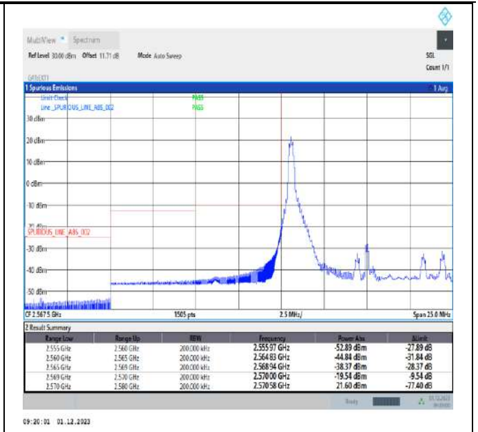
Band38_10MHz_64QAM_37800_1RB#0
