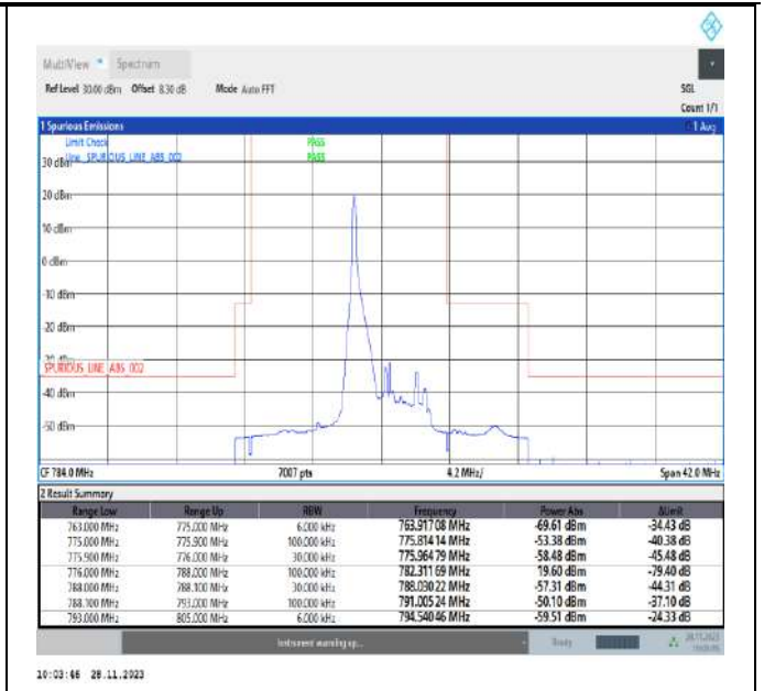
Band13_5MHz_16QAM_23255_1RB#0
