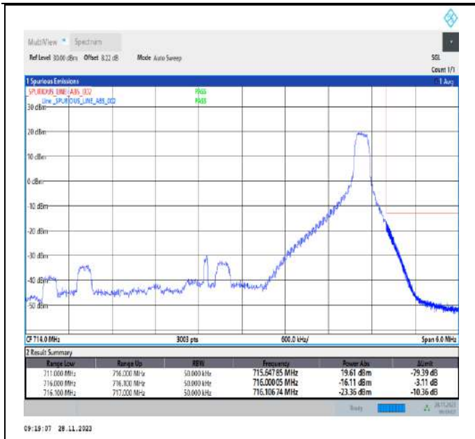
Band12_5MHz_QPSK_23155_1RB#24
