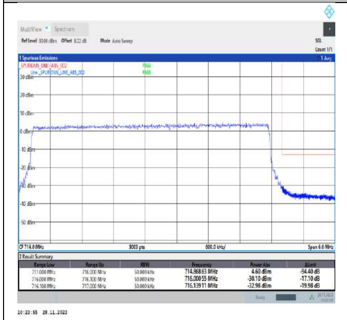
Band17_5MHz_16QAM_23825_25RB#0
