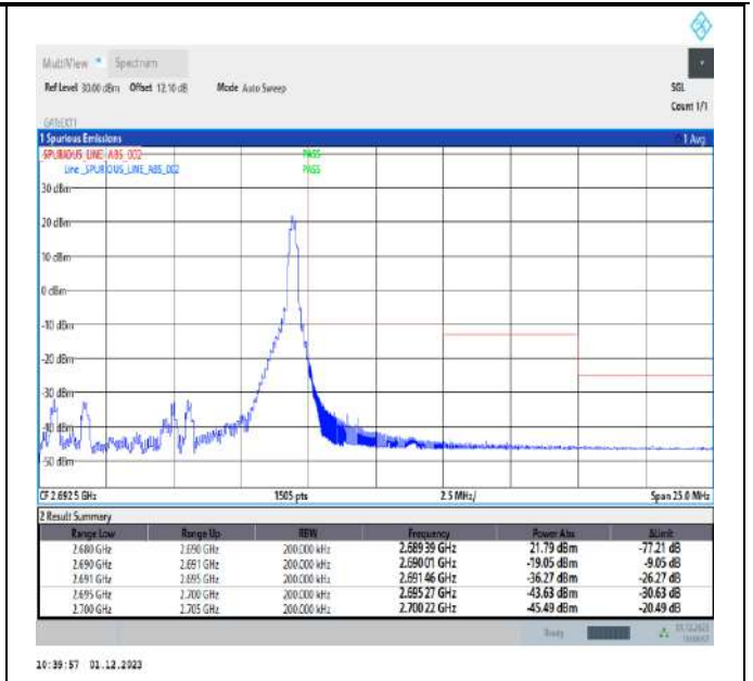
Band41_10MHz_64QAM_41540_1RB#49
