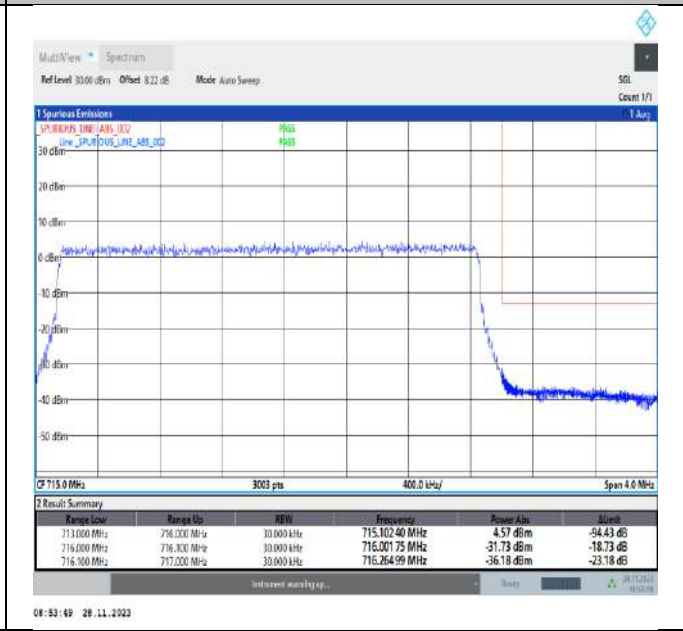
Band12_3MHz_64QAM_23165_15RB#0
