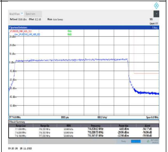
Band12_5MHz_16QAM_23155_25RB#0
