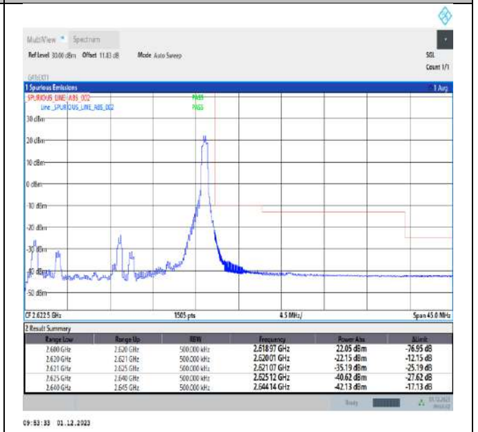
Band38_20MHz_16QAM_38150_1RB#99
