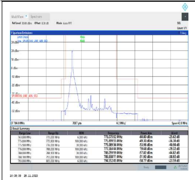
Band13_10MHz_64QAM_23230_1RB#0
