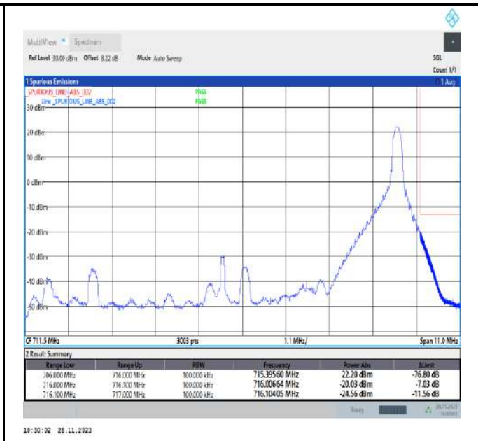
Band17_10MHz_QPSK_23800_1RB#49
