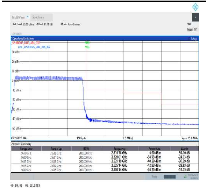
Band38_10MHz_64QAM_38200_50RB#0
