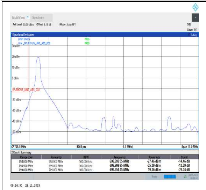
Band12_10MHz_16QAM_23060_1RB#0
