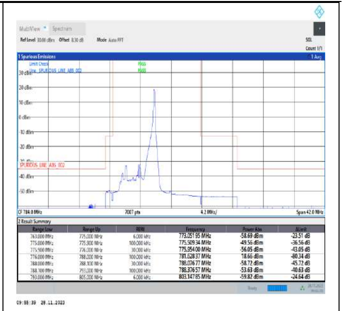
Band13_5MHz_64QAM_23205_1RB#24
