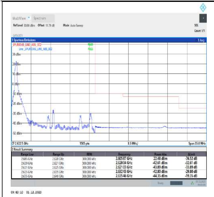
Band38_15MHz_16QAM_38175_1RB#0
