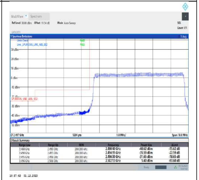
Band41_10MHz_64QAM_39700_50RB#0
