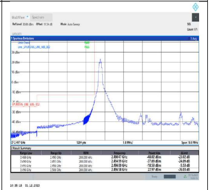
Band41_10MHz_16QAM_39700_1RB#0
