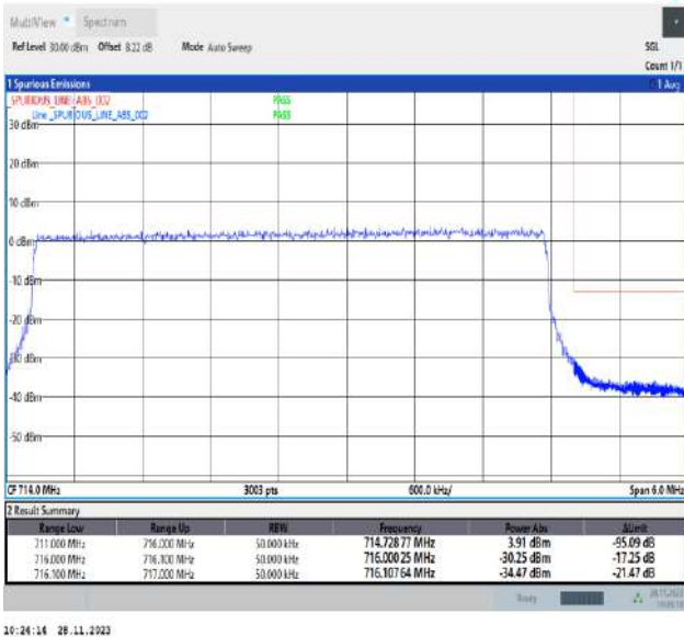
Band17_5MHz_64QAM_23825_25RB#0
