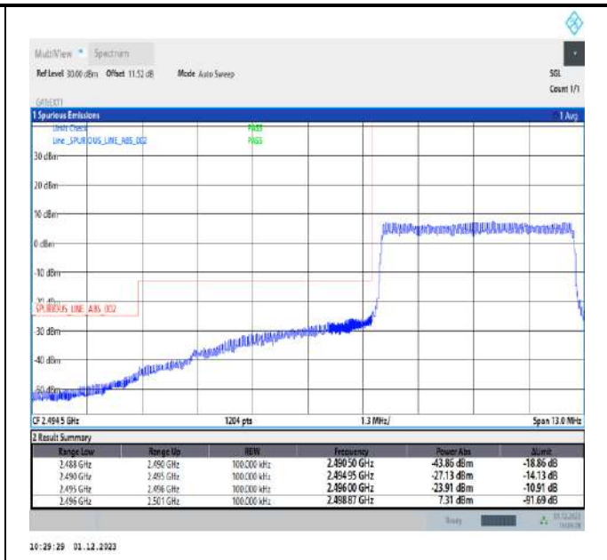
Band41_5MHz_QPSK_39675_25RB#0
