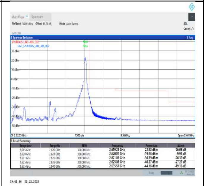
Band38_15MHz_QPSK_38175_1RB#74
