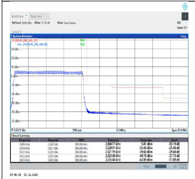
Band38_15MHz_16QAM_38175_75RB#0
