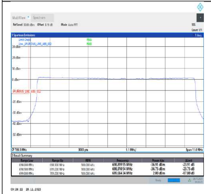
Band12_10MHz_16QAM_23060_50RB#0
