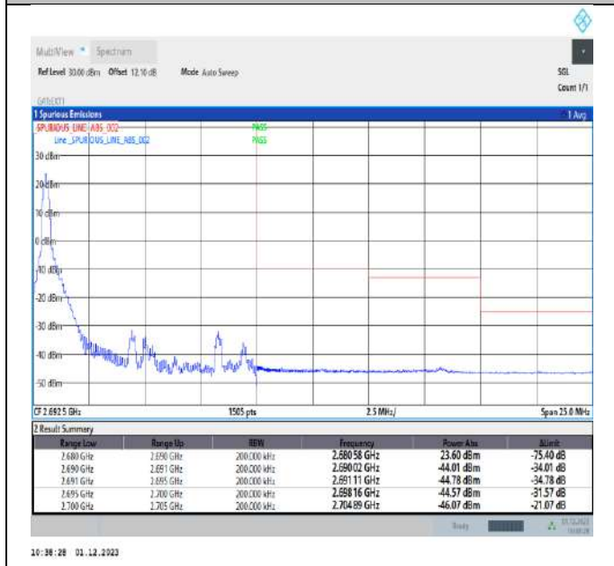
Band41_10MHz_16QAM_41540_1RB#0
