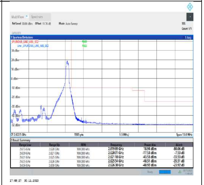
Band38_5MHz_64QAM_38225_1RB#24
