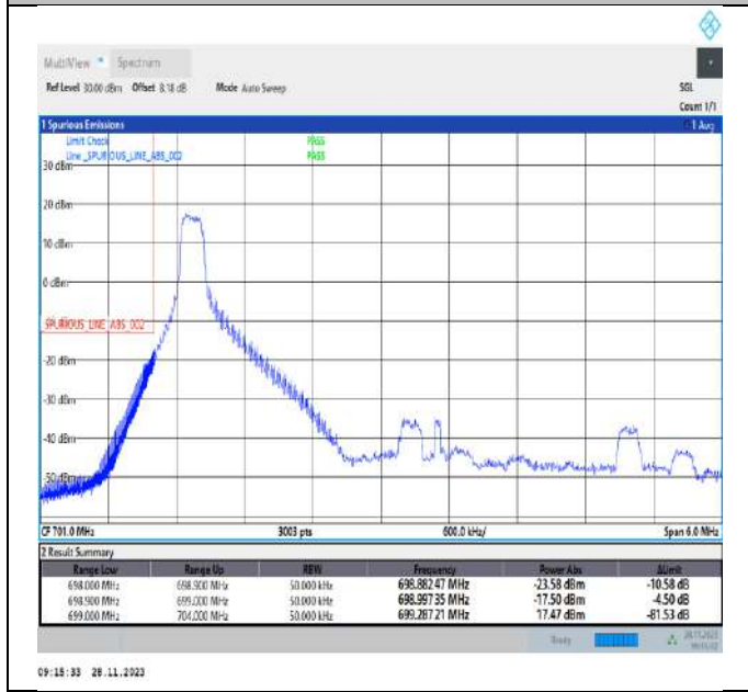
Band12_5MHz_16QAM_23035_1RB#0
