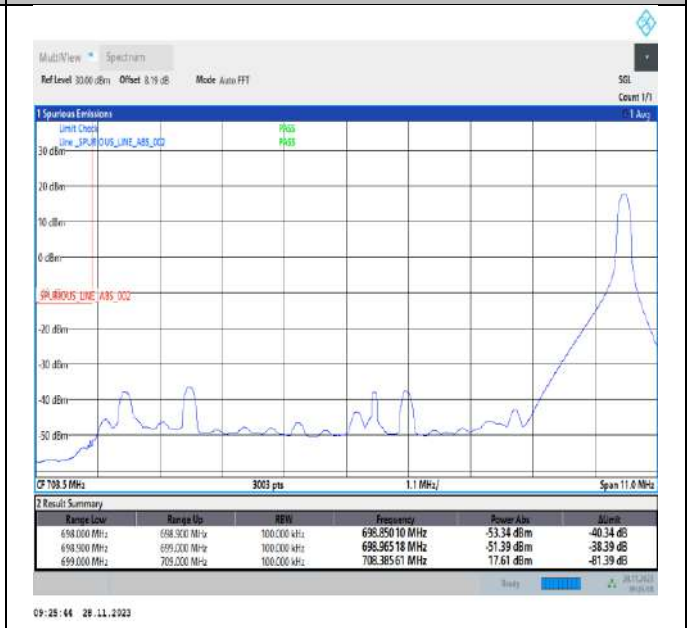
Band12_10MHz_64QAM_23060_1RB#49
