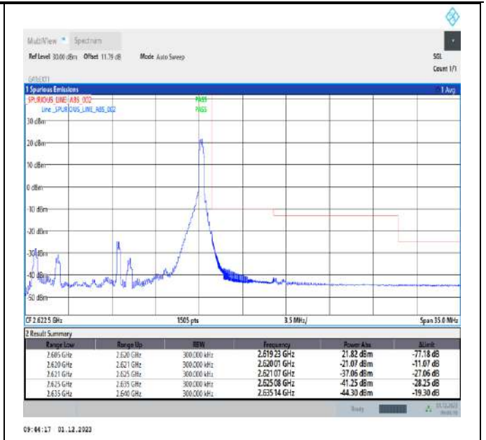
Band38_15MHz_16QAM_38175_1RB#74
