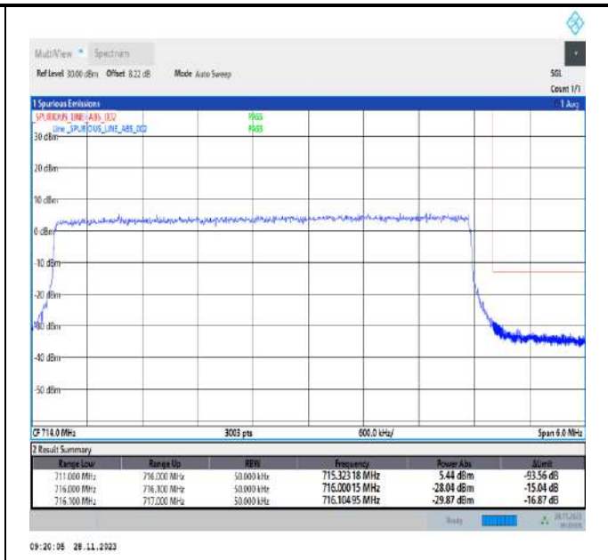
Band12_5MHz_QPSK_23155_25RB#0
