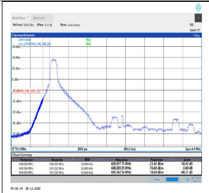
Band12_5MHz_QPSK_23035_1RB#0
