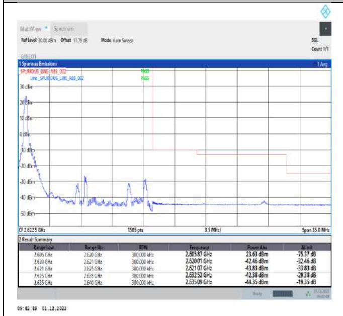
Band38_15MHz_QPSK_38175_1RB#0
