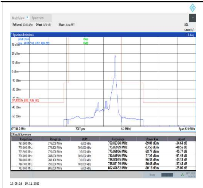
Band13_5MHz_64QAM_23255_1RB#24
