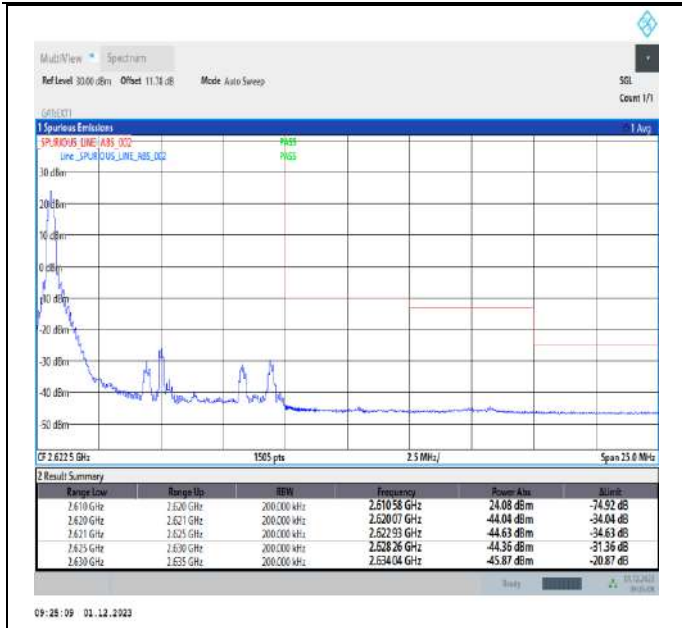
Band38_10MHz_QPSK_38200_1RB#0
