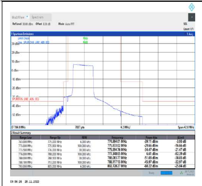
Band13_5MHz_16QAM_23205_25RB#0
