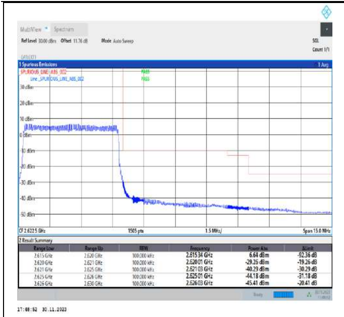
Band38_5MHz_QPSK_38225_25RB#0
