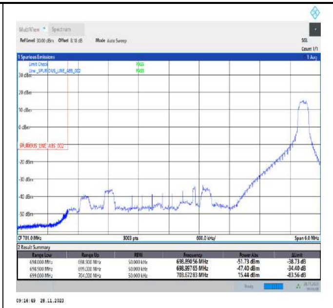
Band12_5MHz_64QAM_23035_1RB#24
