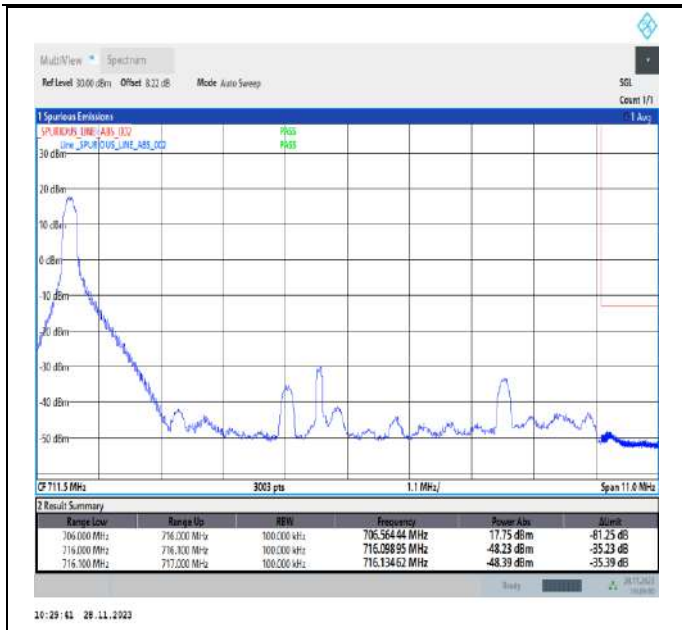
Band17_10MHz_64QAM_23800_1RB#0
