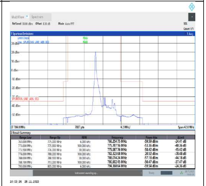
Band13_5MHz_QPSK_23255_1RB#0
