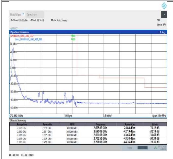
Band41_15MHz_QPSK_41515_1RB#0
