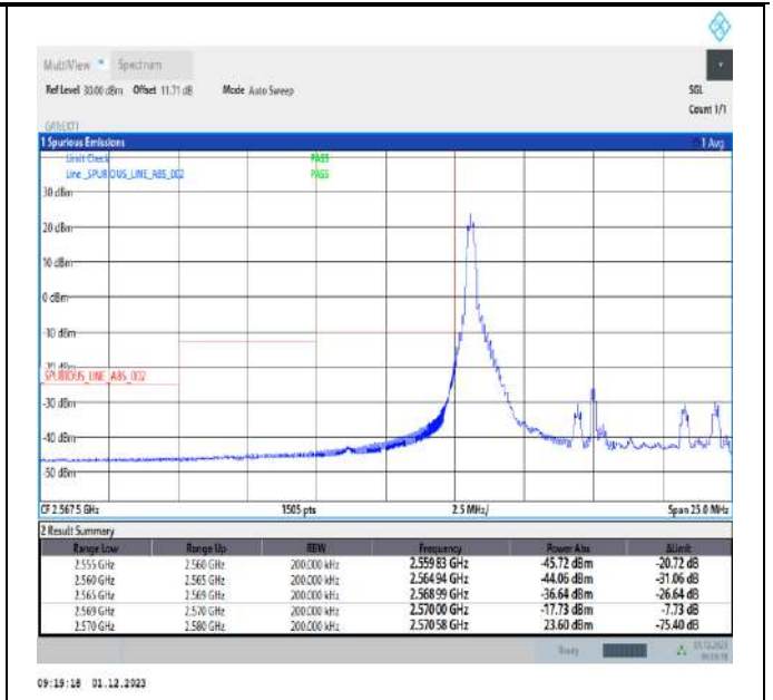
Band38_10MHz_QPSK_37800_1RB#0
