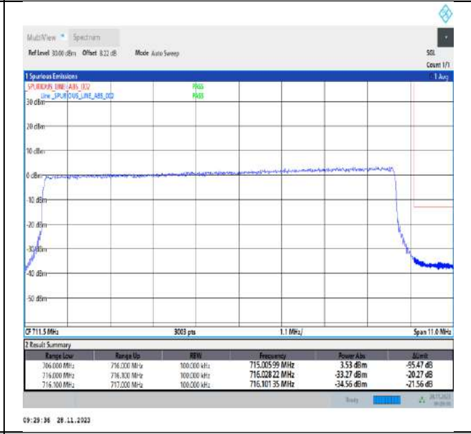
Band12_10MHz_64QAM_23130_50RB#0
