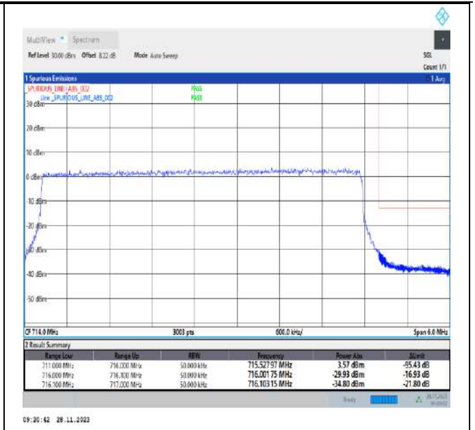
Band12_5MHz_64QAM_23155_25RB#0
