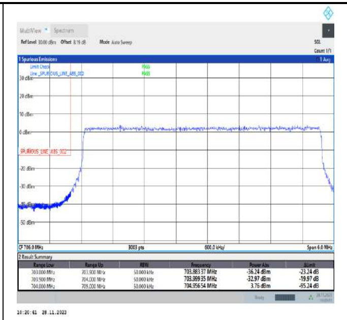
Band17_5MHz_QPSK_23755_25RB#0
