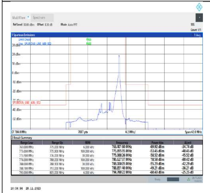
Band13_5MHz_16QAM_23255_1RB#24
