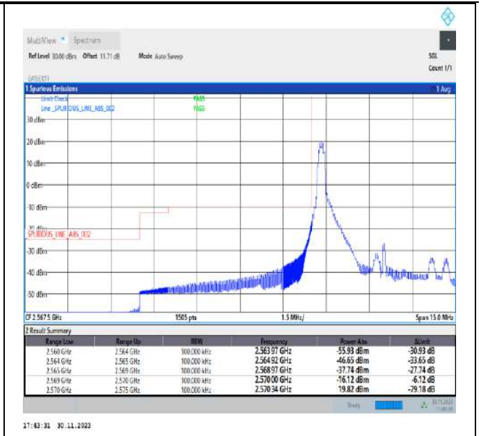
Band38_5MHz_16QAM_37775_1RB#0
