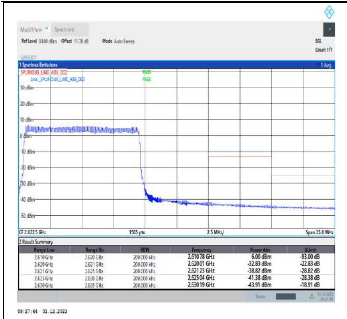
Band38_10MHz_16QAM_38200_50RB#0
