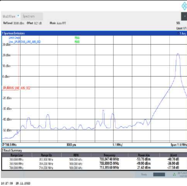
Band17_10MHz_QPSK_23780_1RB#49
