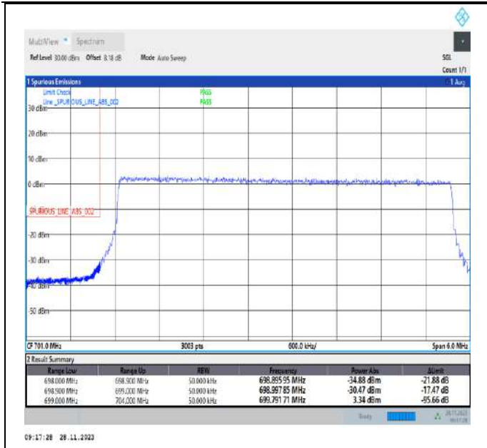
Band12_5MHz_16QAM_23035_25RB#0
