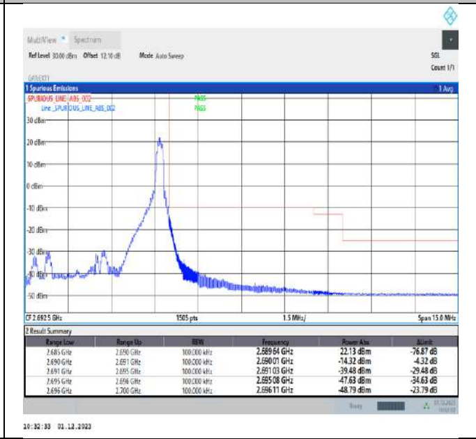
Band41_5MHz_QPSK_41565_1RB#24
