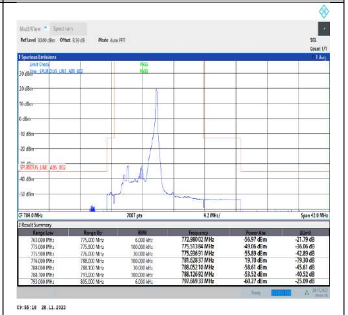
Band13_5MHz_16QAM_23205_1RB#24
