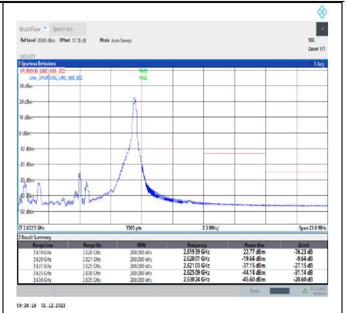
Band38_10MHz_QPSK_38200_1RB#49
