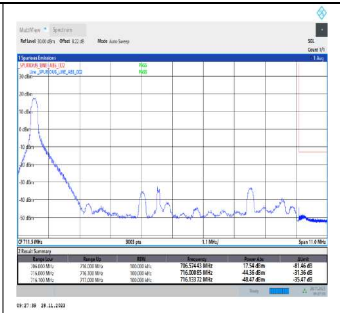
Band12_10MHz_64QAM_23130_1RB#0
