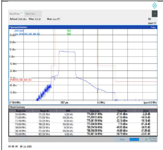
Band13_5MHz_QPSK_23205_25RB#0
