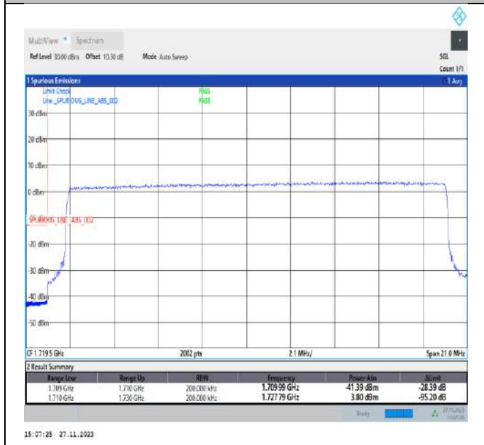
Band4_20MHz_16QAM_20050_100RB#0
