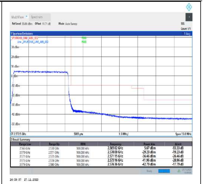
Band7_5MHz_64QAM_21425_25RB#0
