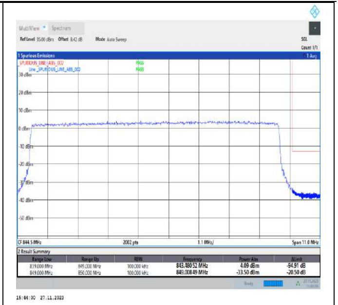
Band5_10MHz_16QAM_20600_50RB#0
