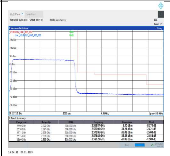
Band7_20MHz_64QAM_21350_100RB#0
