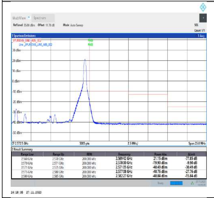
Band7_10MHz_64QAM_21400_1RB#49
