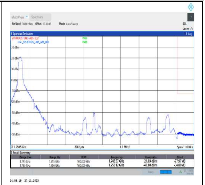
Band4_10MHz_QPSK_20350_1RB#0
