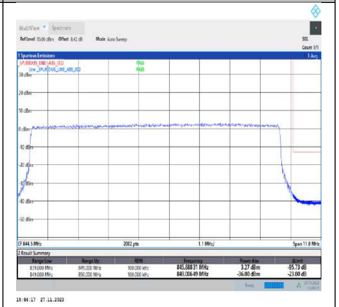
Band5_10MHz_64QAM_20600_50RB#0
