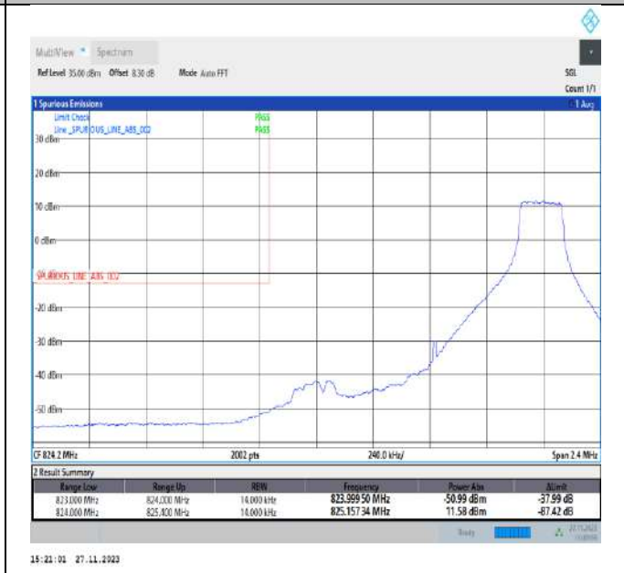
Band5_1.4MHz_16QAM_20407_1RB#5
