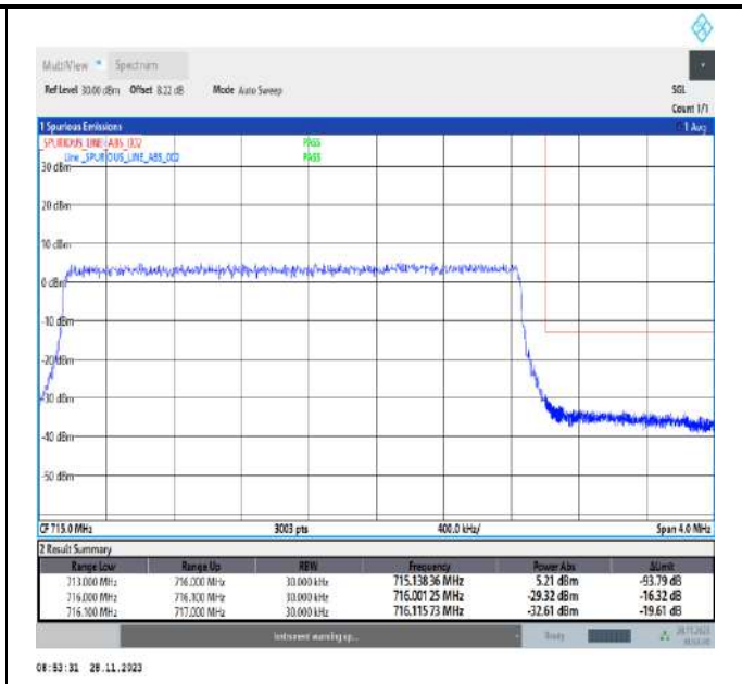
Band12_3MHz_16QAM_23165_15RB#0
