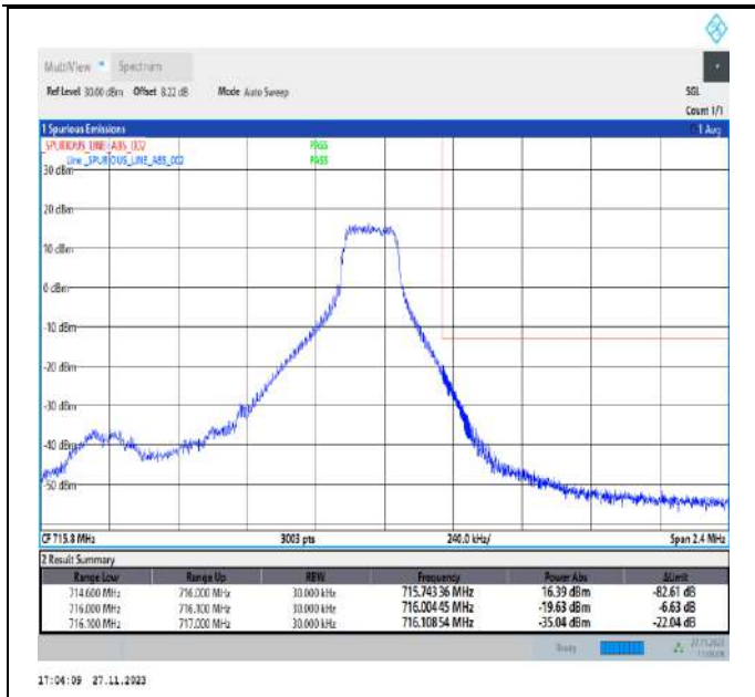
Band12_1.4MHz_64QAM_23173_1RB#5
