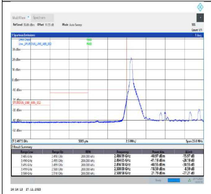
Band7_10MHz_64QAM_20800_1RB#0
