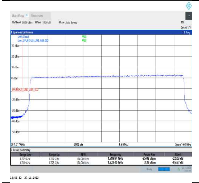
Band4_15MHz_64QAM_20025_75RB#0
