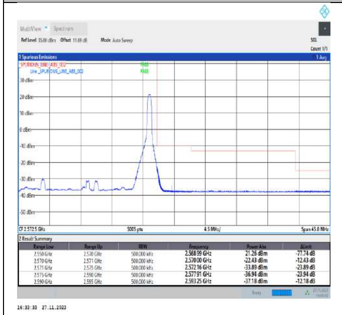
Band7_20MHz_64QAM_21350_1RB#99
