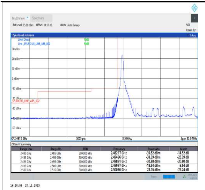
Band7_15MHz_QPSK_20825_1RB#0
