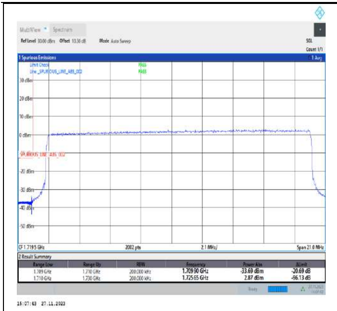
Band4_20MHz_64QAM_20050_100RB#0
