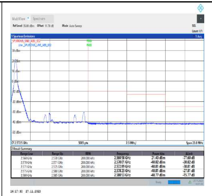
Band7_10MHz_64QAM_21400_1RB#0
