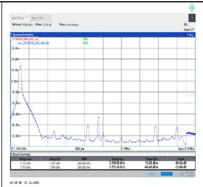
Band4_20MHz_64QAM_20300_1RB#0
