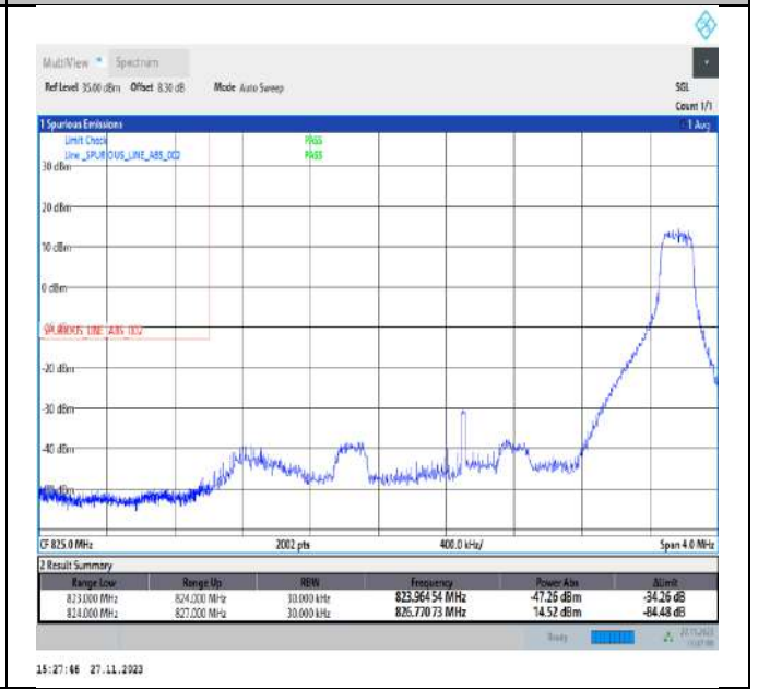
Band5_3MHz_64QAM_20415_1RB#14
