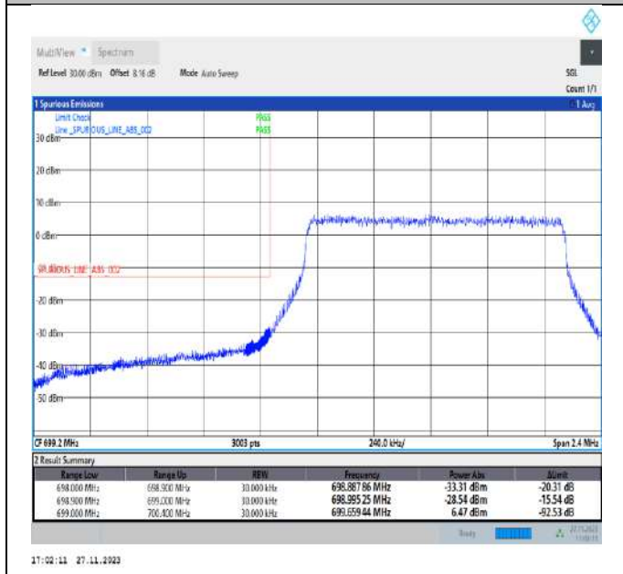
Band12_1.4MHz_64QAM_23017_6RB#0
