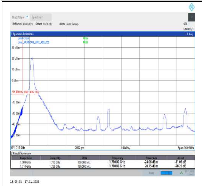
Band4_15MHz_64QAM_20025_1RB#0
