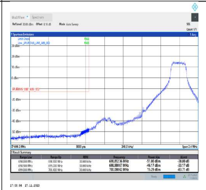
Band12_1.4MHz_16QAM_23017_1RB#5
