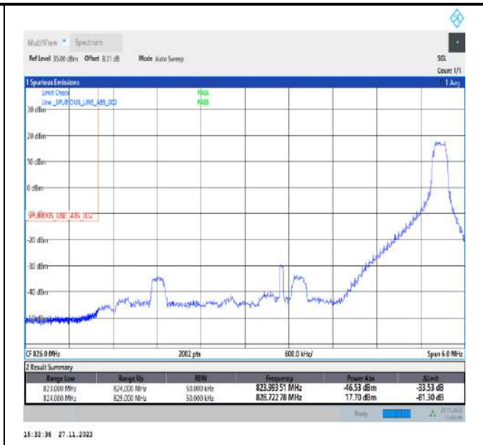
Band5_5MHz_QPSK_20425_1RB#24
