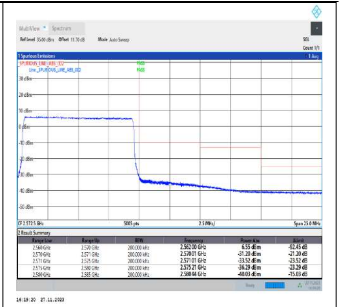
Band7_10MHz_16QAM_21400_50RB#0
