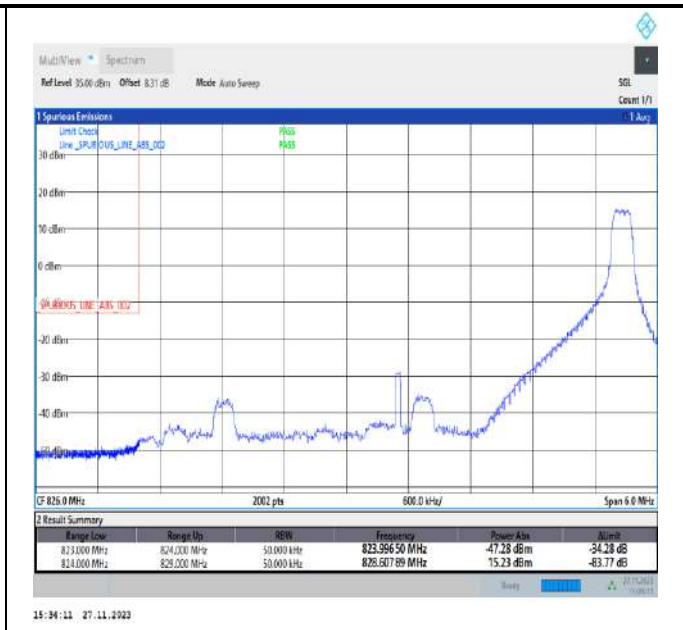
Band5_5MHz_64QAM_20425_1RB#24
