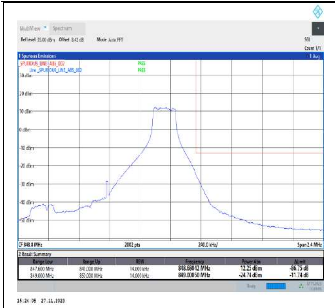
Band5_1.4MHz_64QAM_20643_1RB#5
