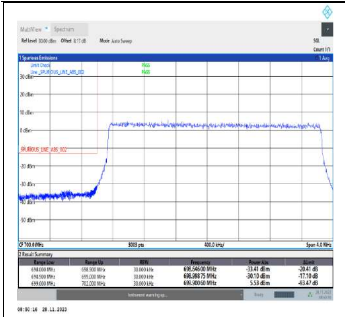
Band12_3MHz_QPSK_23025_15RB#0
