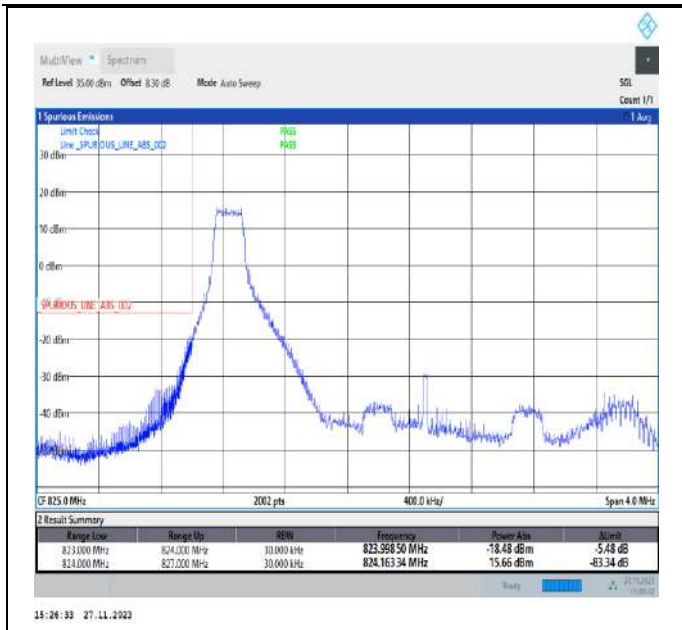
Band5_3MHz_16QAM_20415_1RB#0
