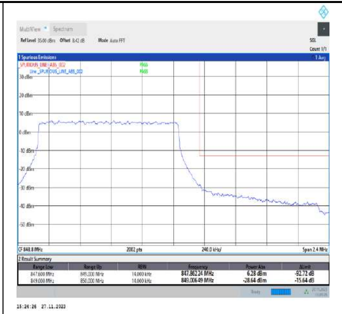
Band5_1.4MHz_QPSK_20643_6RB#0
