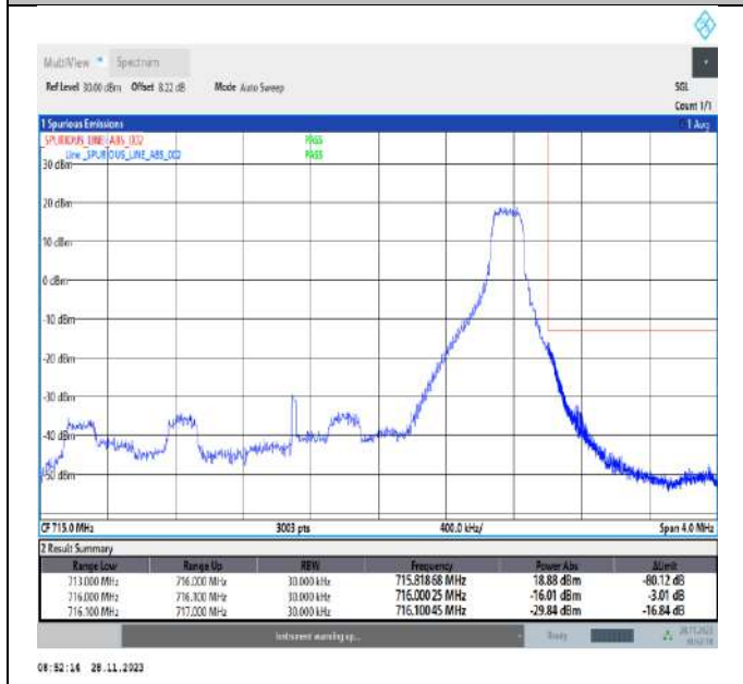
Band12_3MHz_QPSK_23165_1RB#14
