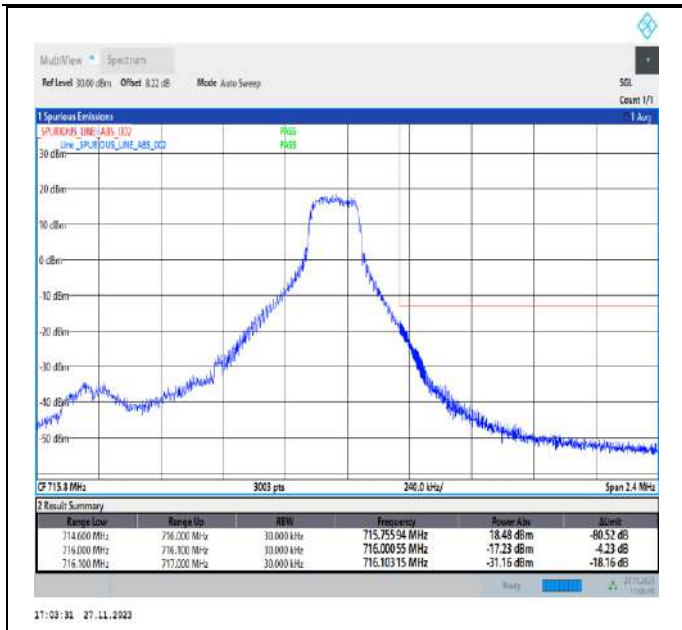
Band12_1.4MHz_QPSK_23173_1RB#5
