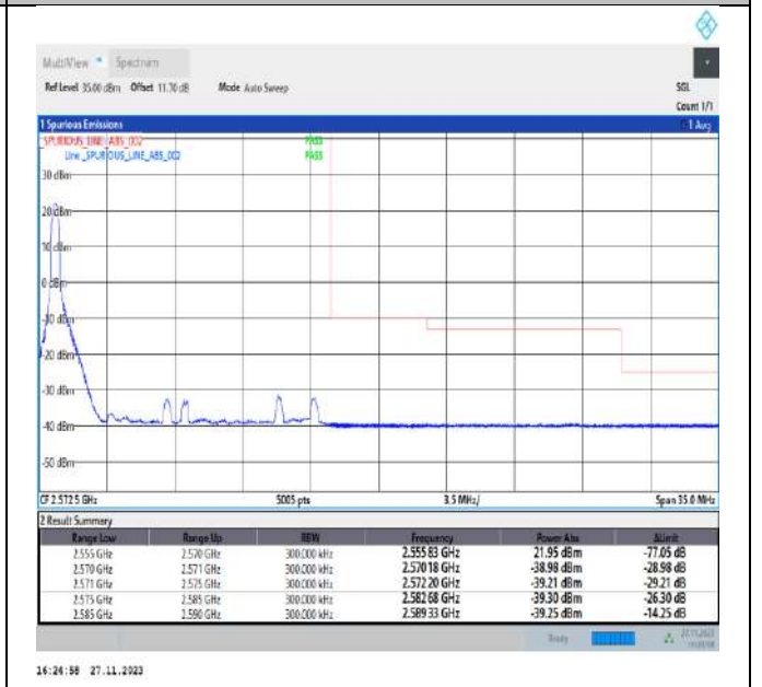
Band7_15MHz_64QAM_21375_1RB#0
