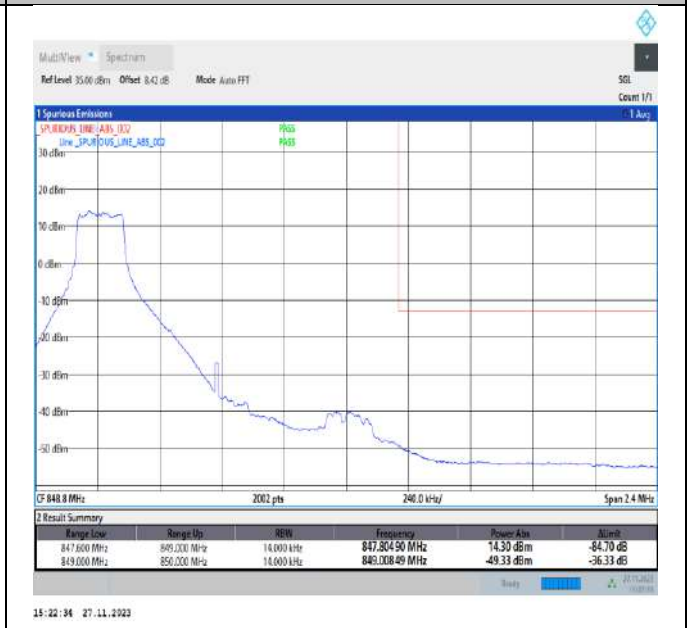
Band5_1.4MHz_QPSK_20643_1RB#0
