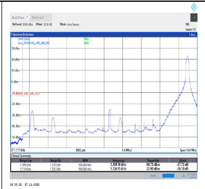
Band4_15MHz_QPSK_2025_1RB#74
