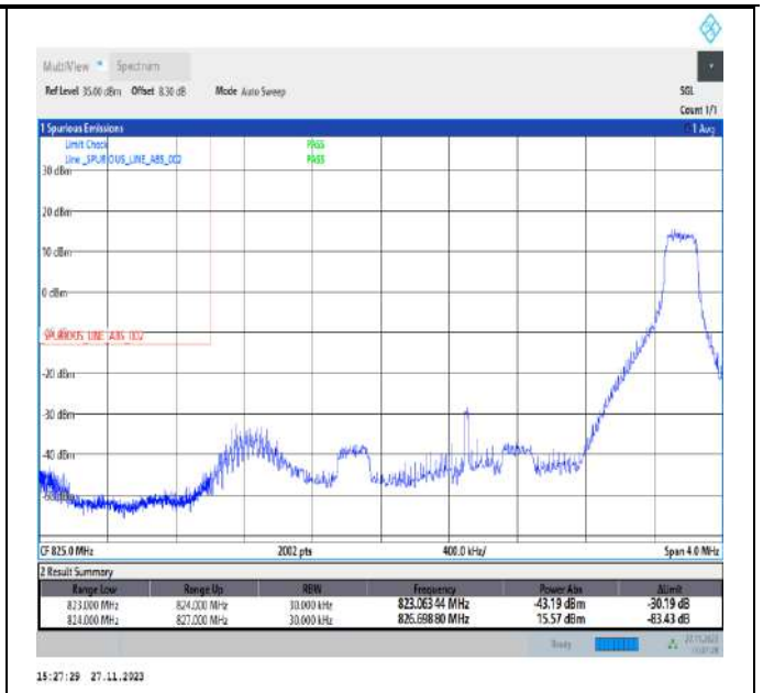
Band5_3MHz_16QAM_20415_1RB#14
