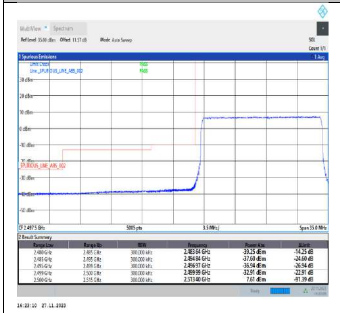
Band7_15MHz_QPSK_20825_75RB#0
