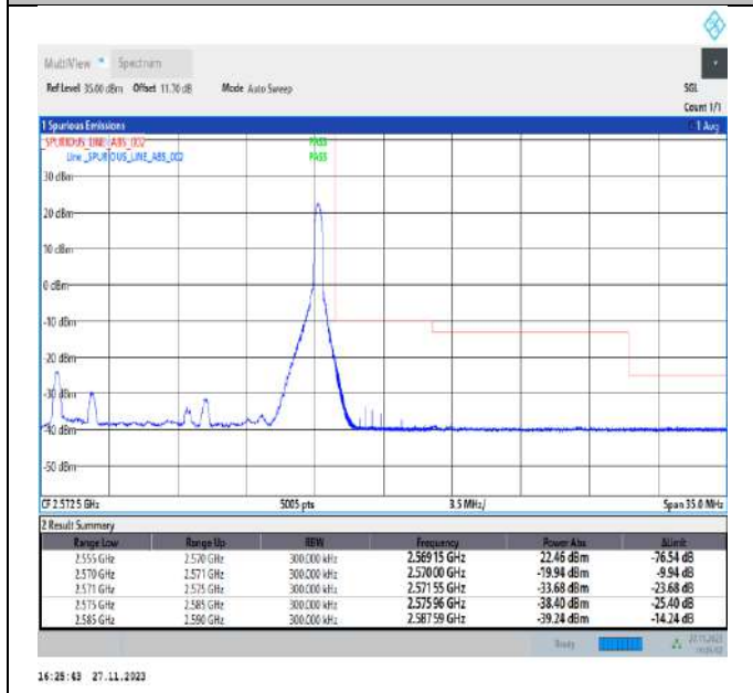
Band7_15MHz_16QAM_21375_1RB#74
