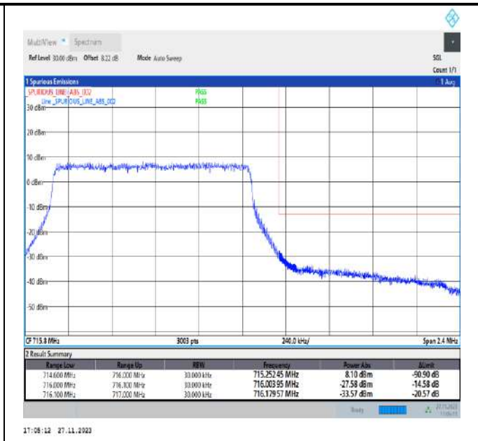
Band12_1.4MHz_64QAM_23173_6RB#0
