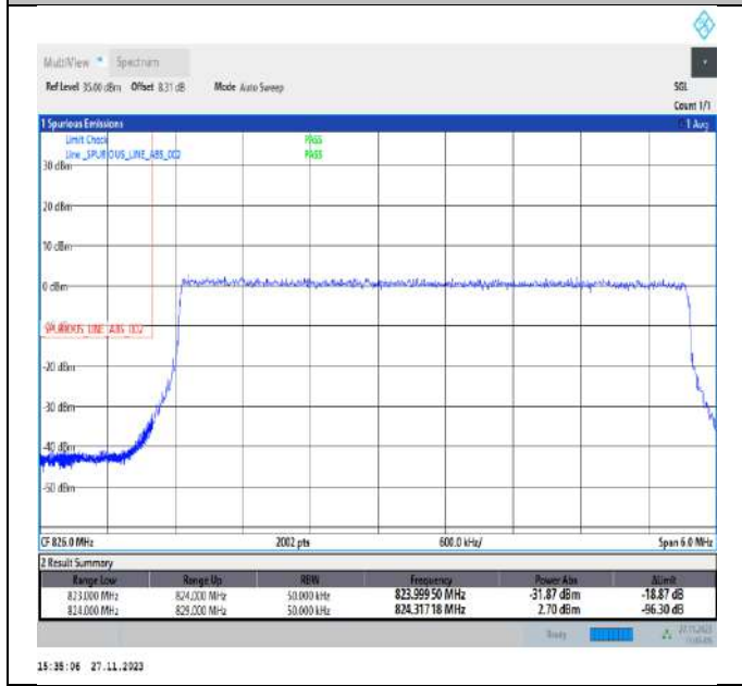
Band5_5MHz_64QAM_20425_25RB#0
