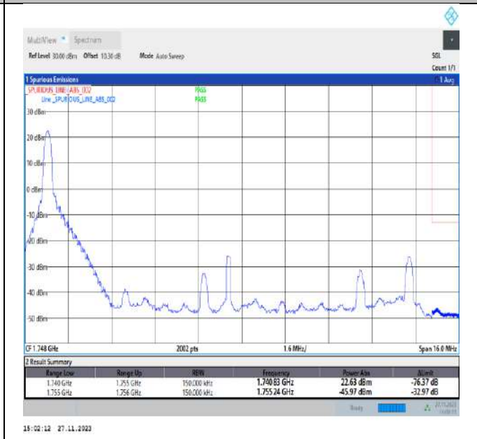
Band4_15MHz_QPSK_20325_1RB#0
