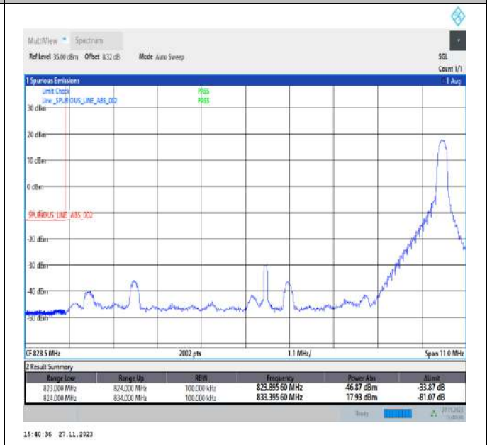
Band5_10MHz_64QAM_20450_1RB#49
