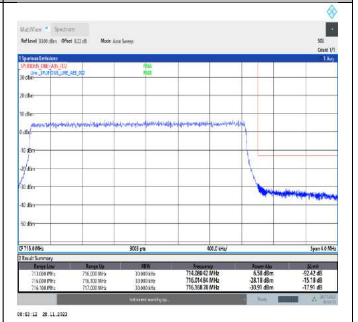
Band12_3MHz_QPSK_23165_15RB#0
