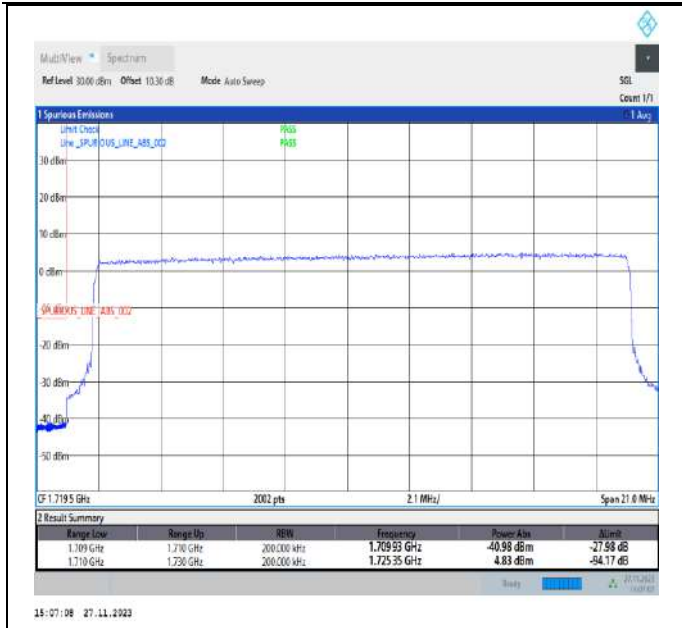
Band4_20MHz_QPSK_20050_100RB#0
