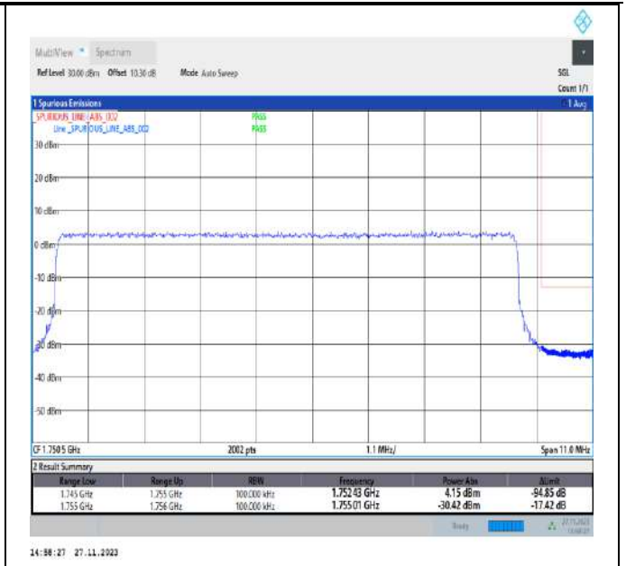
Band4_10MHz_16QAM_20350_50RB#0
