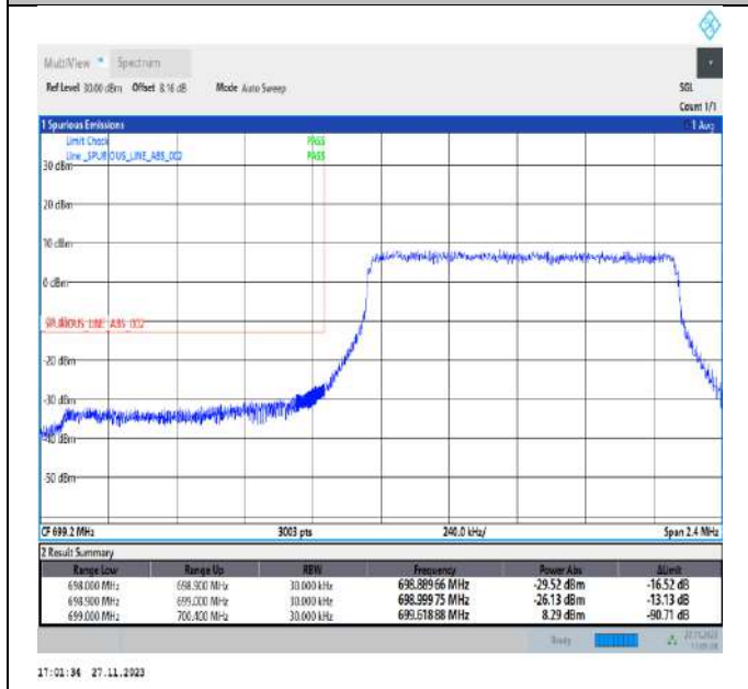
Band12_1.4MHz_QPSK_23017_6RB#0
