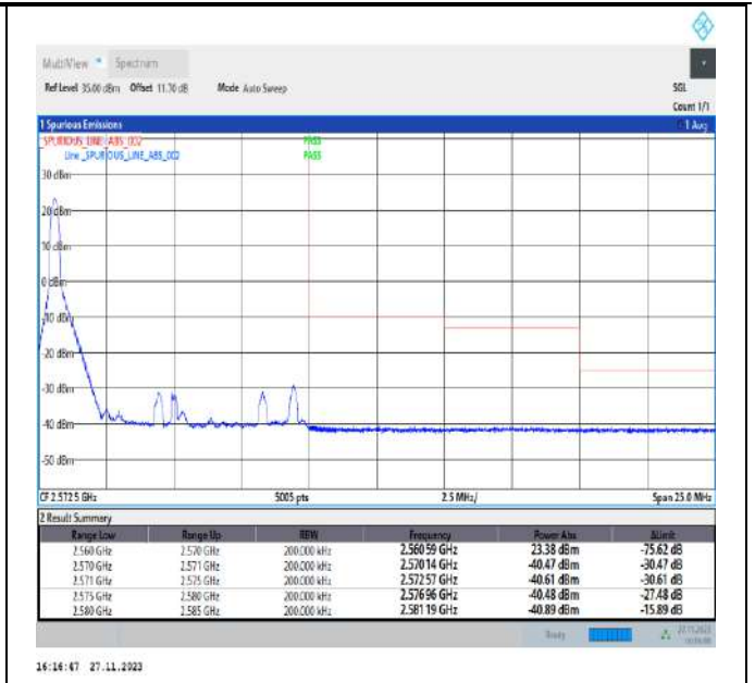
Band7_10MHz_QPSK_21400_1RB#0
