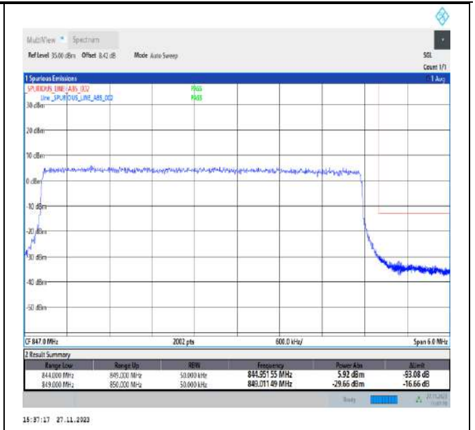
Band5_5MHz_QPSK_20625_25RB#0
