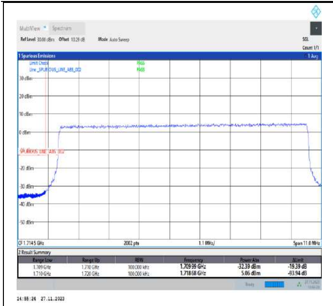
Band4_10MHz_QPSK_20000_50RB#0
