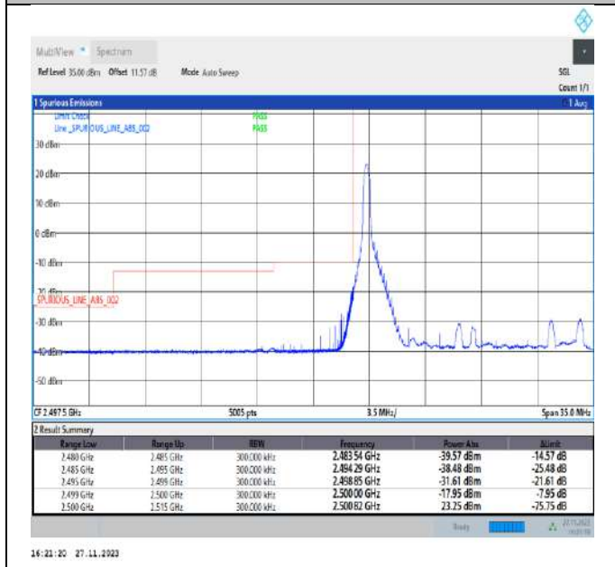
Band7_15MHz_16QAM_20825_1RB#0
