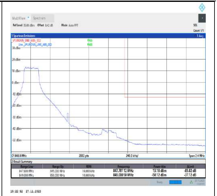
Band5_1.4MHz_16QAM_20643_1RB#0
