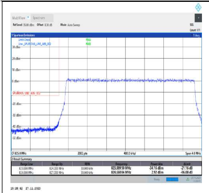
Band5_3MHz_64QAM_20415_15RB#0
