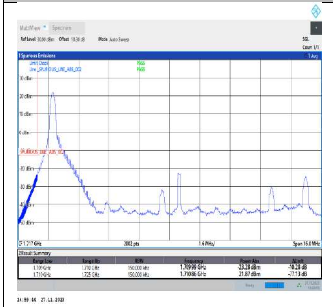
Band4_15MHz_16QAM_20025_1RB#0
