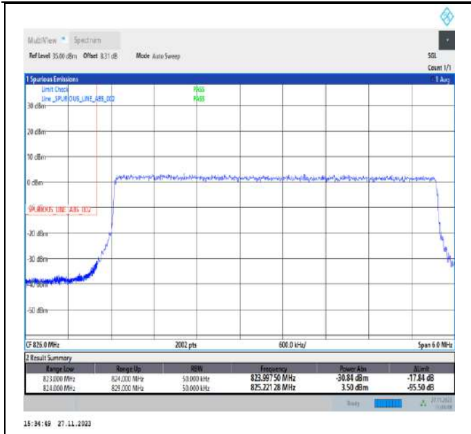
Band5_5MHz_16QAM_20425_25RB#0
