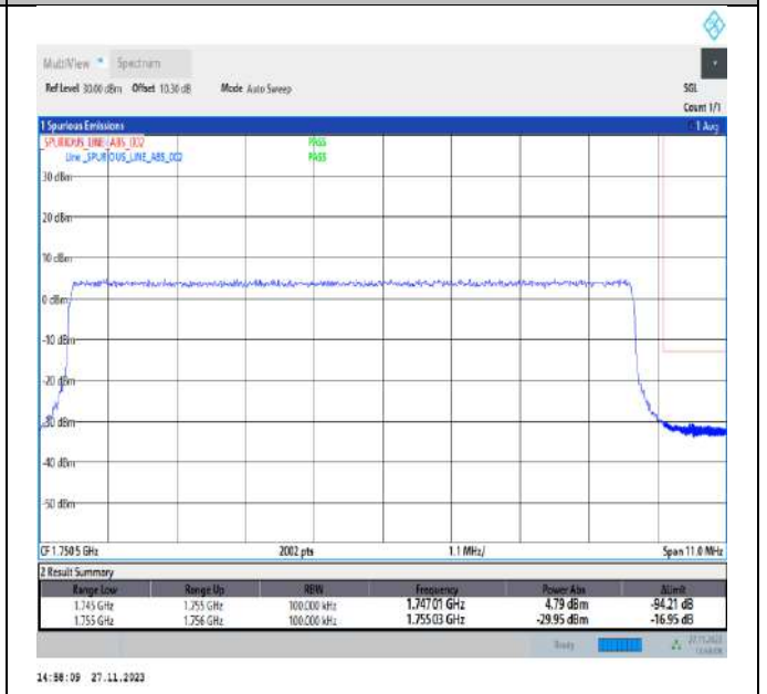
Band4_10MHz_QPSK_20350_50RB#0
