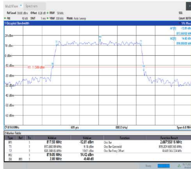
26(814-824)-3MHz-16QAM-26740-15RB#0-PASS
