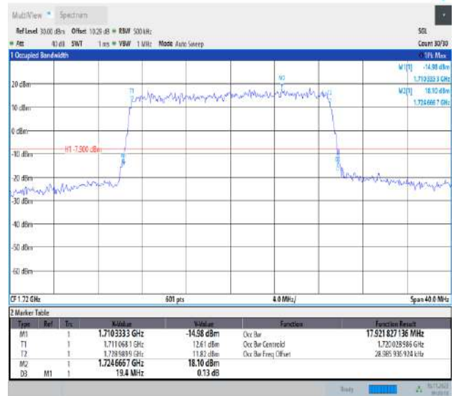
Band66-20MHz-QPSK-132072-100RB#0-PASS
