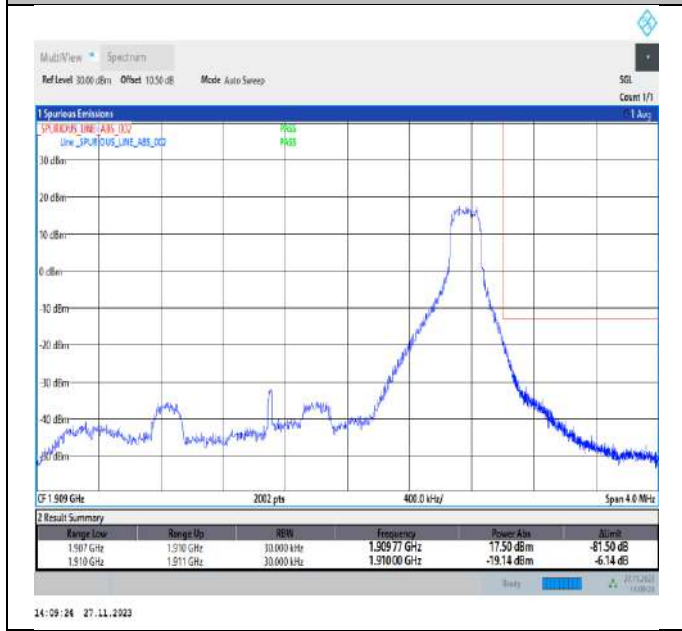
Band2_3MHz_QPSK_19185_1RB#14
