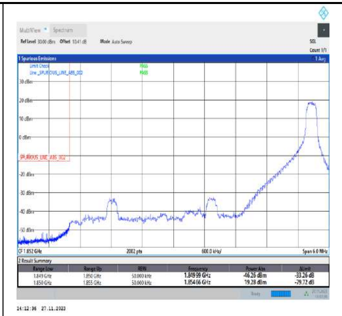
Band2_5MHz_QPSK_18625_1RB#24
