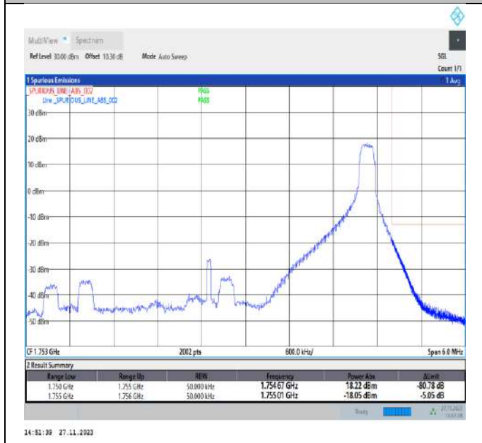
Band4_5MHz_16QAM_20375_1RB#24
