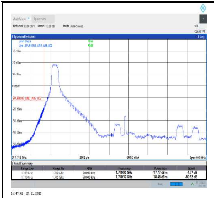
Band4_5MHz_QPSK_19975_1RB#0
