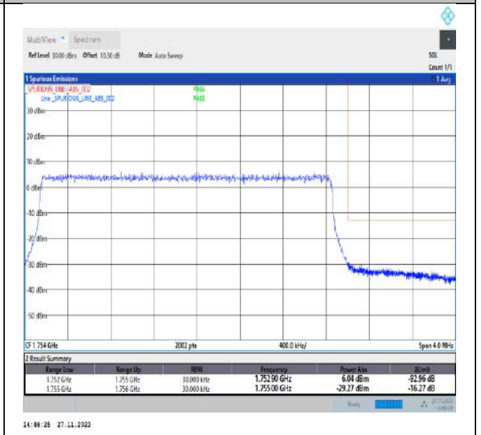
Band4_3MHz_QPSK_20385_15RB#0
