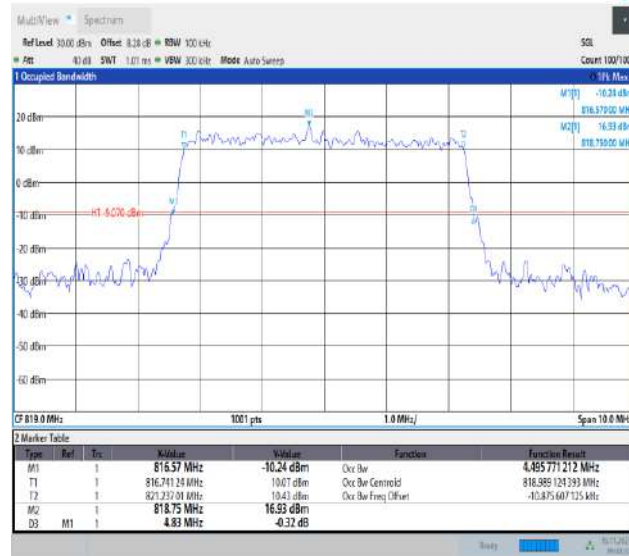
26(814-824)-5MHz-64QAM-26740-25RB#0-PASS
