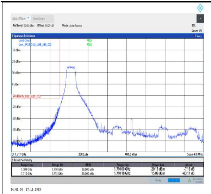
Band4_3MHz_16QAM_19965_1RB#0
