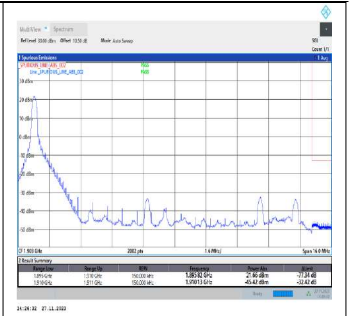
Band2_15MHz_16QAM_19125_1RB#0
