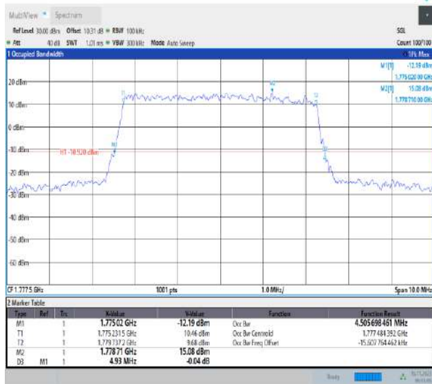
Band66-5MHz-64QAM-132647-25RB#0-PASS
