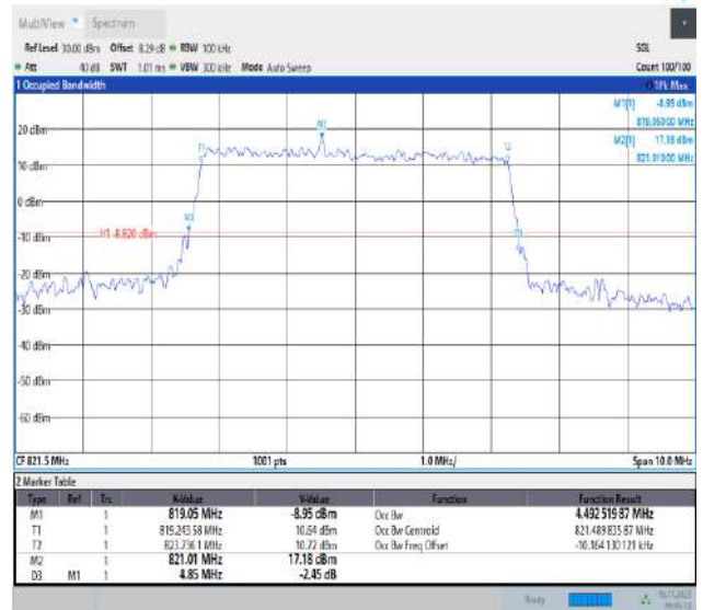
26(814-824)-5MHz-16QAM-26765-25RB#0-PASS
