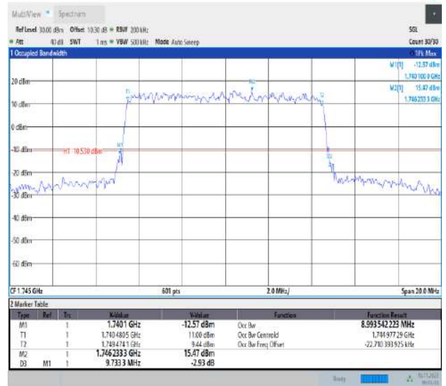
Band66-10MHz-16QAM-132322-50RB#0-PASS
