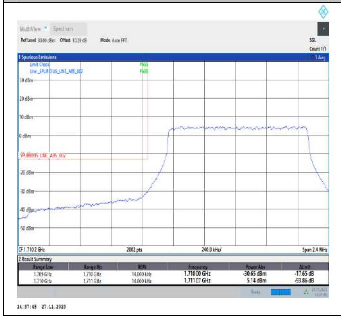
Band4_1.4MHz_QPSK_19957_6RB#0
