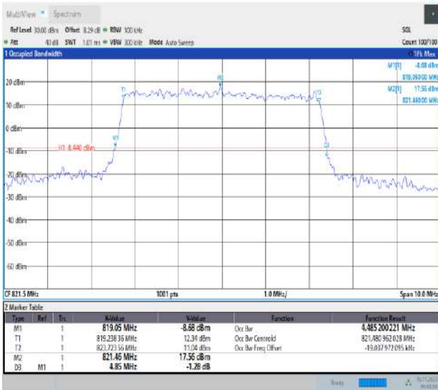
26(814-824)-5MHz-QPSK-26765-25RB#0-PASS
