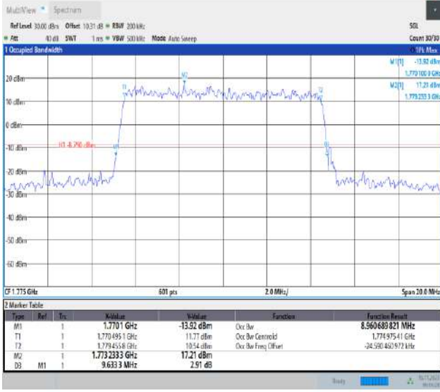
Band66-10MHz-16QAM-132622-50RB#0-PASS
