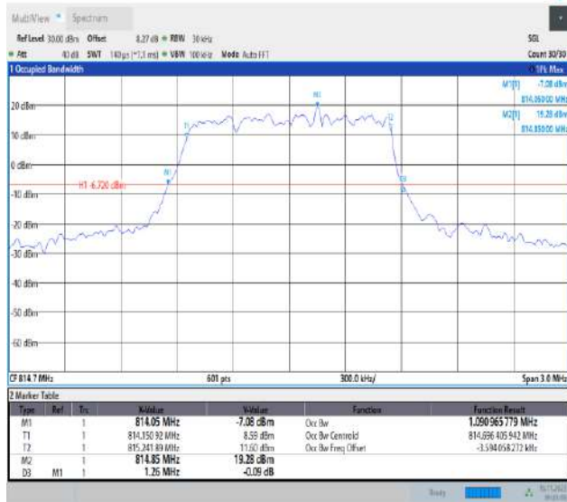
26(814-824)-1.4MHz-QPSK-26697-6RB#0-PASS
