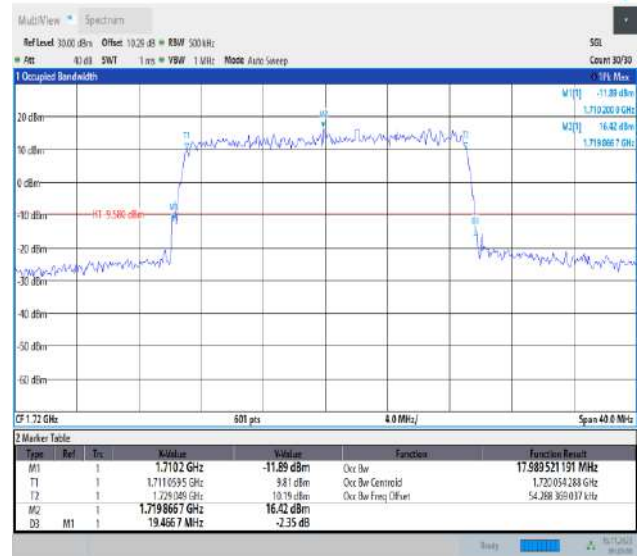
Band66-20MHz-64QAM-132072-100RB#0-PASS
