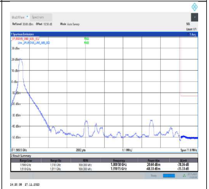
Band2_10MHz_16QAM_19150_1RB#0
