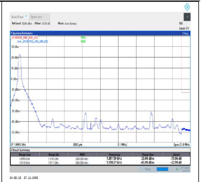
Band2_20MHz_QPSK_19100_1RB#0
