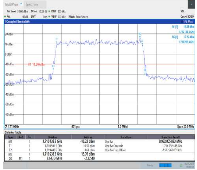
Band66-10MHz-64QAM-132022-50RB#0-PASS
