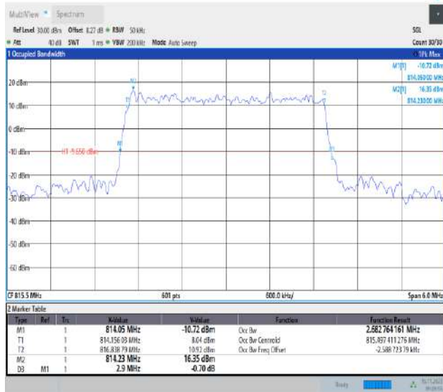
26(814-824)-3MHz-16QAM-26705-15RB#0-PASS
