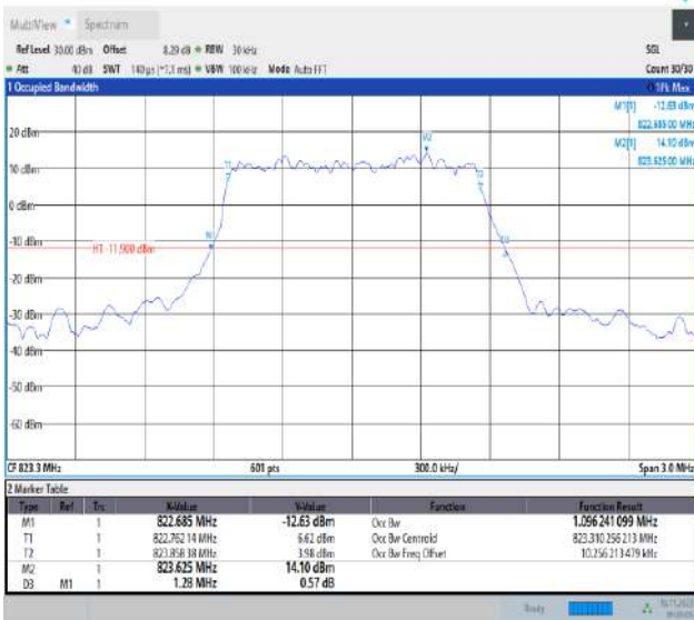
26(814-824)-1.4MHz-64QAM-26783-6RB#0-PASS
