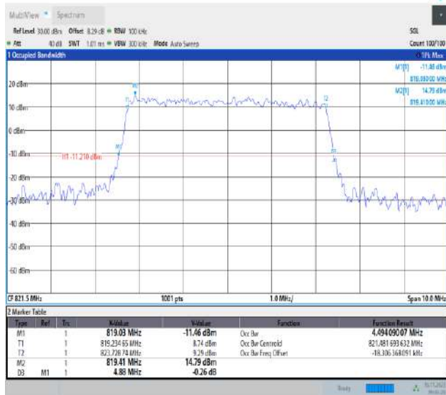
26(814-824)-5MHz-64QAM-26765-25RB#0-PASS
