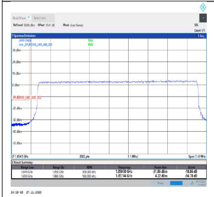
Band2_10MHz_16QAM_18650_50RB#0
