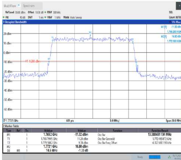
Band66-15MHz-QPSK-132597-75RB#0-PASS
