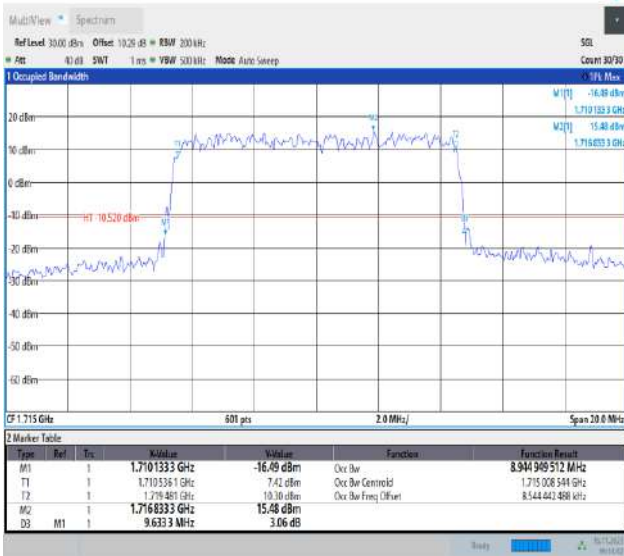
Band66-10MHz-16QAM-132022-50RB#0-PASS
