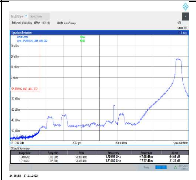
Band4_5MHz_16QAM_19975_1RB#24
