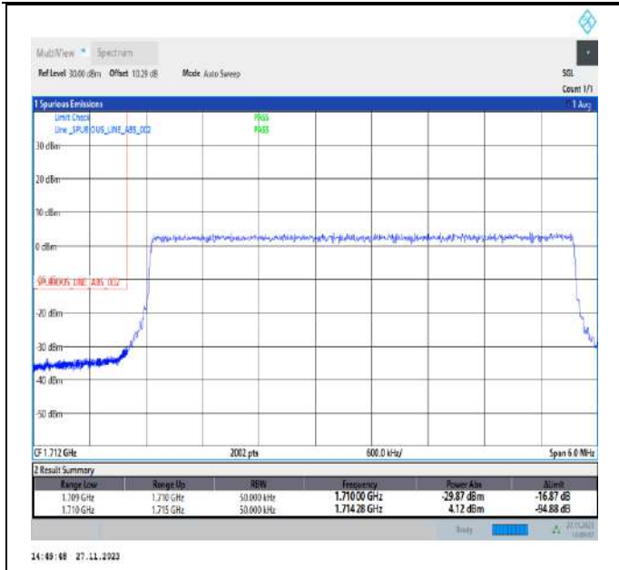
Band4_5MHz_16QAM_19975_25RB#0
