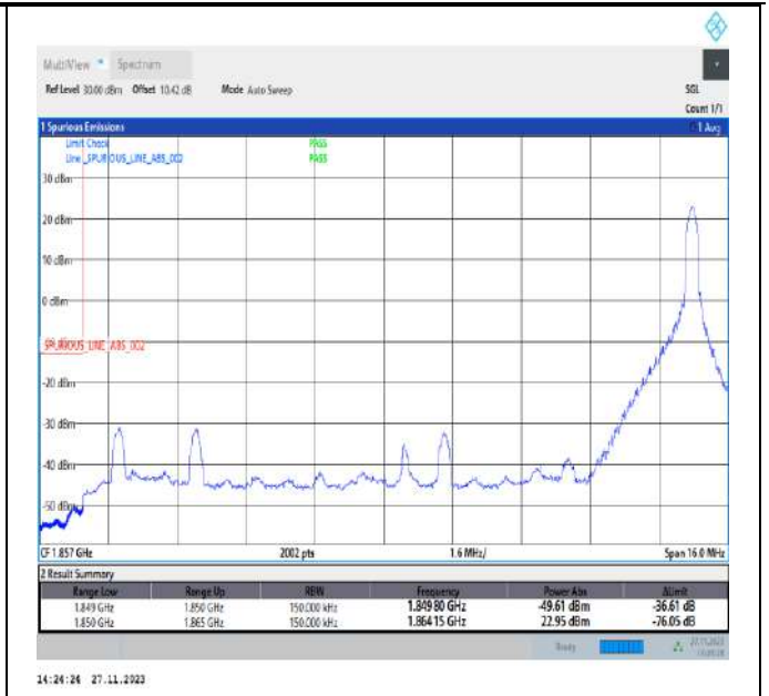
Band2_15MHz_QPSK_18675_1RB#74
