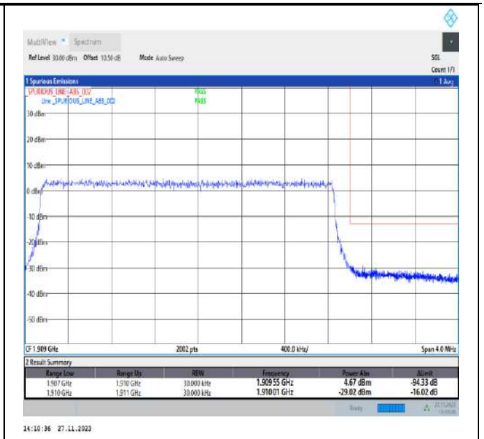
Band2_3MHz_16QAM_19185_15RB#0
