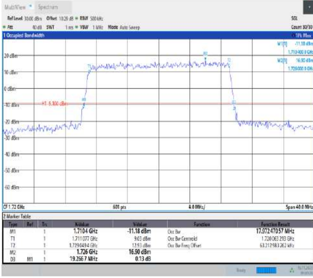
Band66-20MHz-16QAM-132072-100RB#0-PASS
