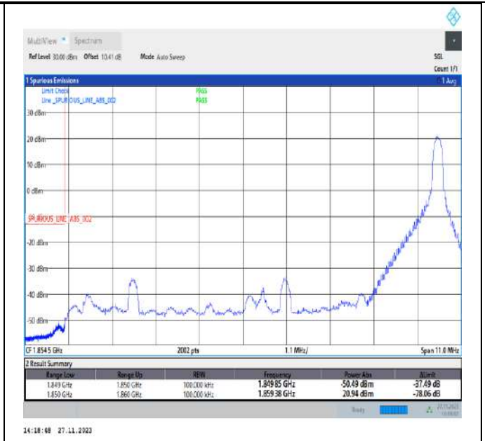
Band2_10MHz_16QAM_18650_1RB#49
