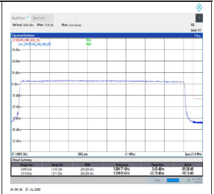
Band2_20MHz_16QAM_19100_100RB#0
