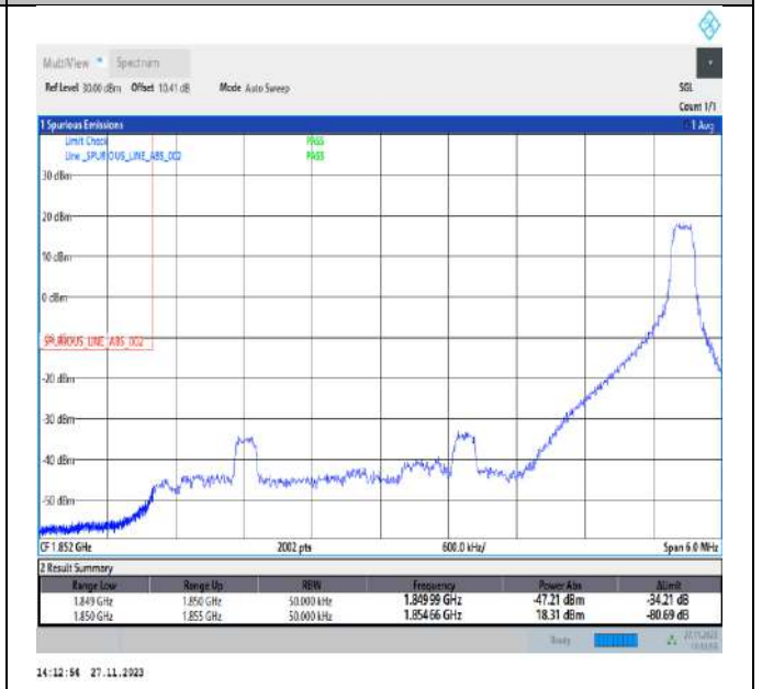
Band2_5MHz_16QAM_18625_1RB#24
