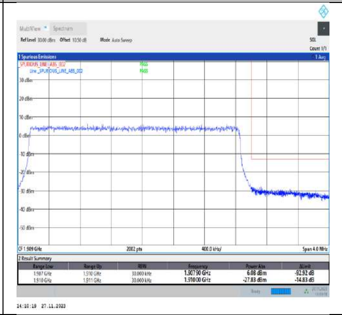
Band2_3MHz_QPSK_19185_15RB#0
