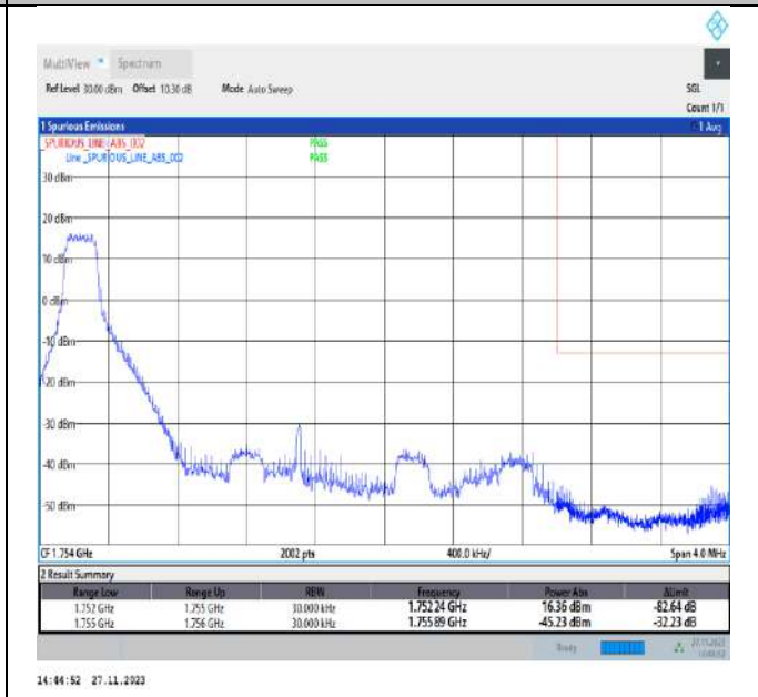
Band4_3MHz_16QAM_20385_1RB#0
