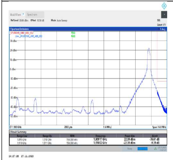
Band2_15MHz_16QAM_19125_1RB#74
