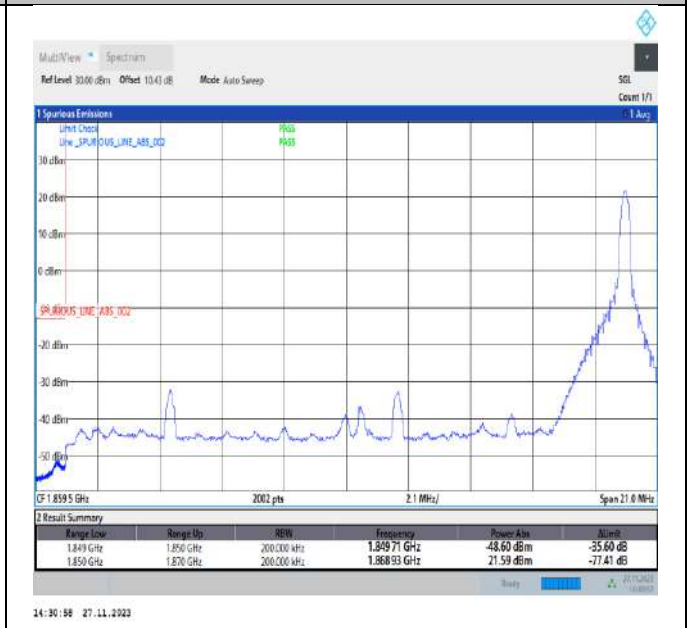
Band2_20MHz_64QAM_18700_1RB#99
