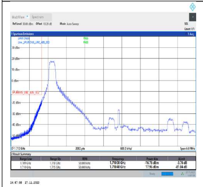
Band4_5MHz_16QAM_19975_1RB#0
