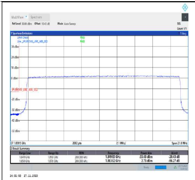
Band2_20MHz_64QAM_18700_100RB#0
