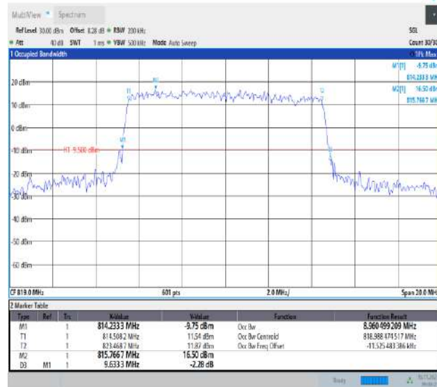
26(814-824)-10MHz-QPSK-26740-50RB#0-PASS
