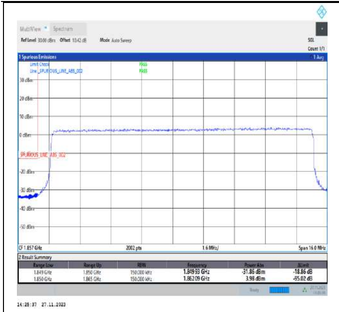
Band2_15MHz_16QAM_18675_75RB#0
