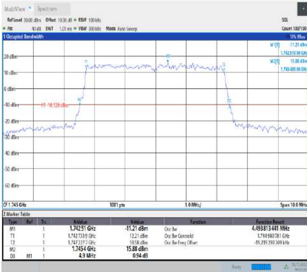
Band66-5MHz-16QAM-132322-25RB#0-PASS
