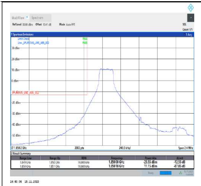
Band2_1.4MHz_64QAM_18607_1RB#0
