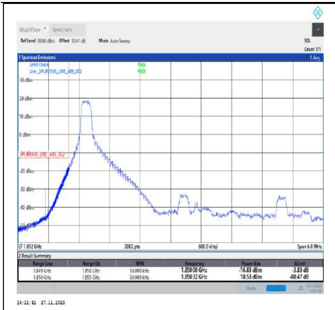
Band2_5MHz_QPSK_18625_1RB#0
