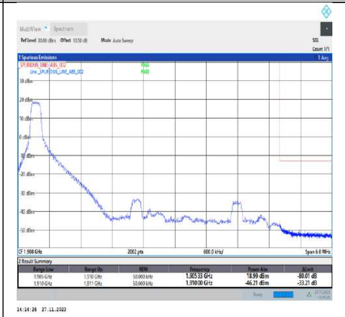
Band2_5MHz_QPSK_19175_1RB#0
