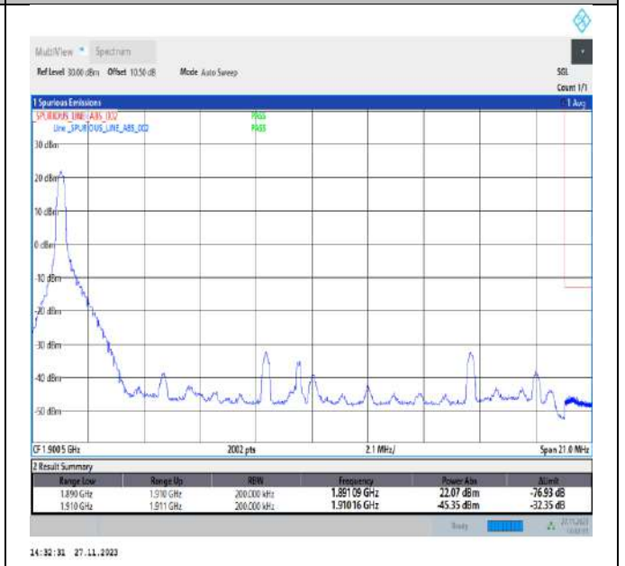
Band2_20MHz_16QAM_19100_1RB#0
