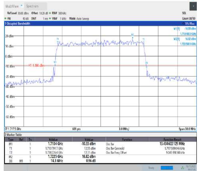
Band66-15MHz-16QAM-132047-75RB#0-PASS
