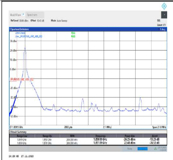
Band2_20MHz_16QAM_18700_1RB#0
