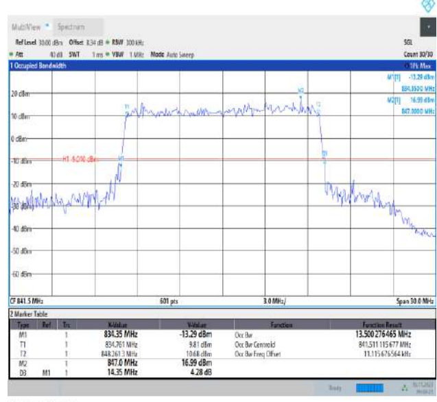
26(824-849)-15MHz-16QAM-26965-75RB#0-PASS
