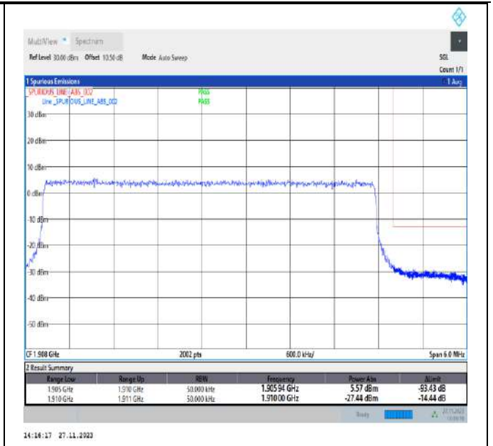
Band2_5MHz_QPSK_19175_25RB#0
