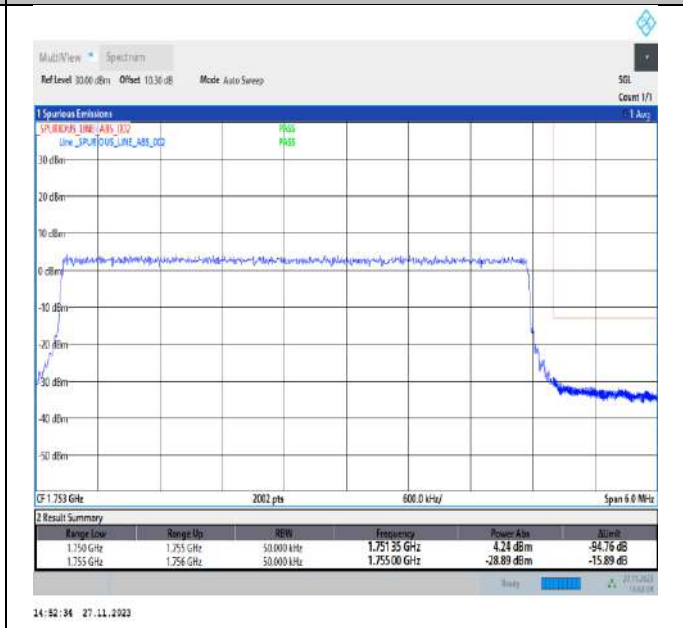
Band4_5MHz_16QAM_20375_25RB#0
