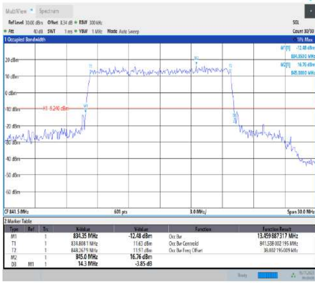
26(824-849)-15MHz-QPSK-26965-75RB#0-PASS
