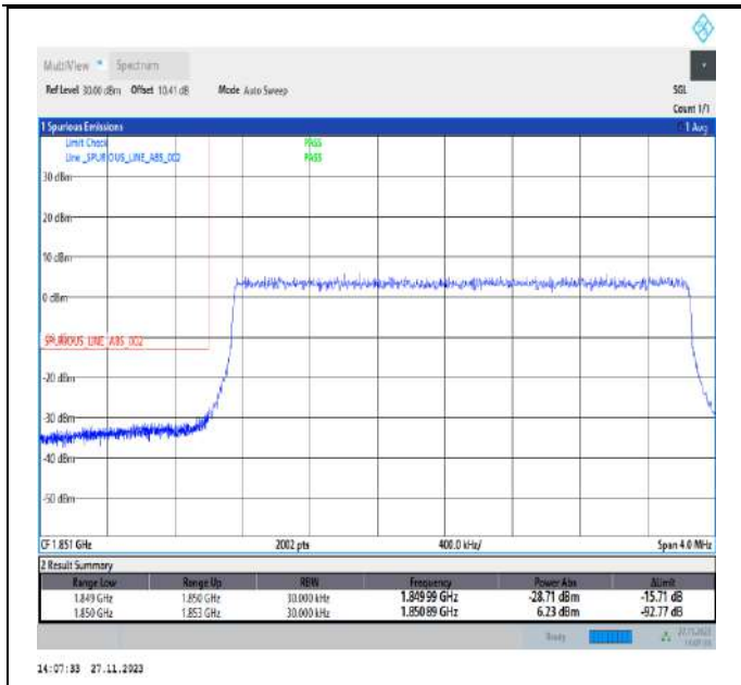
Band2_3MHz_QPSK_18615_15RB#0
