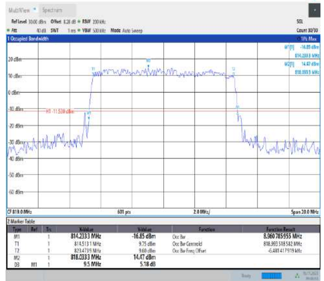
26(814-824)-10MHz-64QAM-26740-50RB#0-PASS
