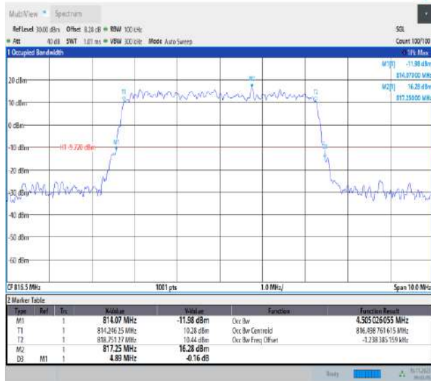
26(814-824)-5MHz-64QAM-26715-25RB#0-PASS
