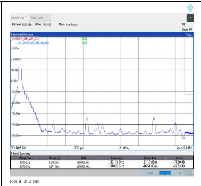
Band2_20MHz_64QAM_19100_1RB#0
