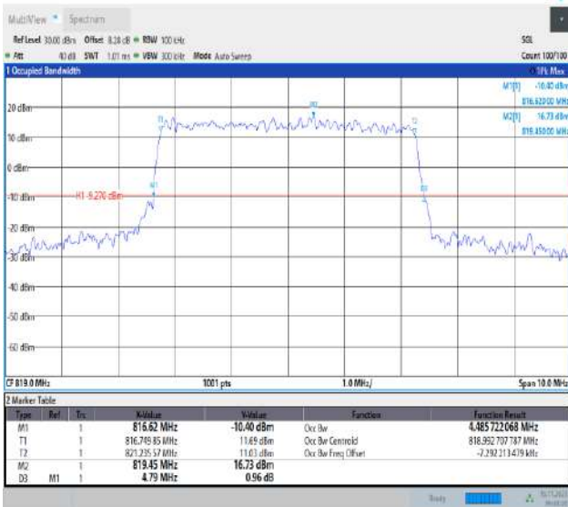
26(814-824)-5MHz-16QAM-26740-25RB#0-PASS
