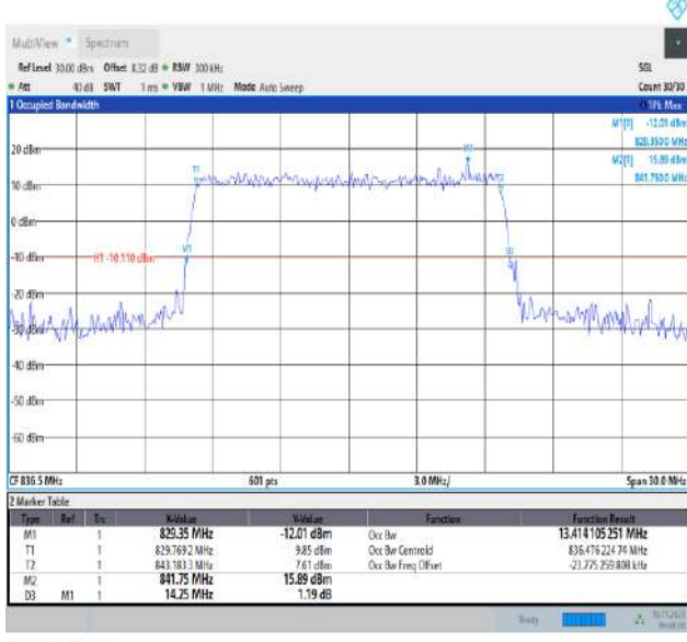
26(824-849)-15MHz-16QAM-26915-75RB#0-PASS
