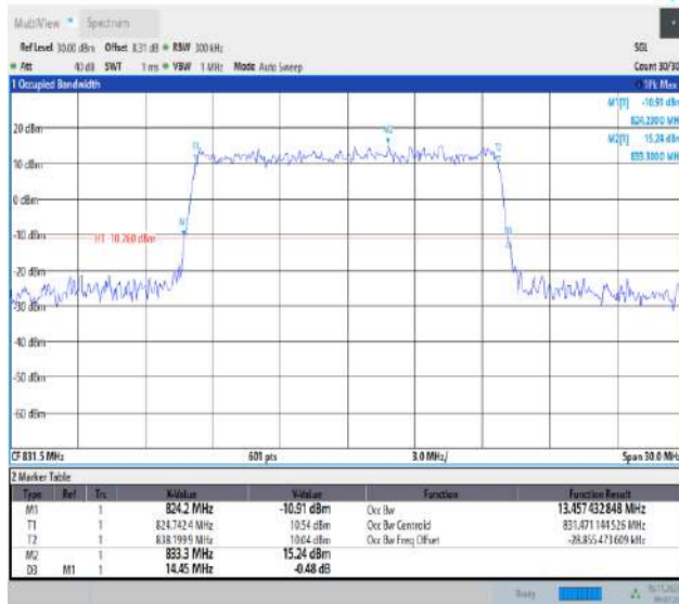
26(824-849)-15MHz-QPSK-26865-75RB#0-PASS
