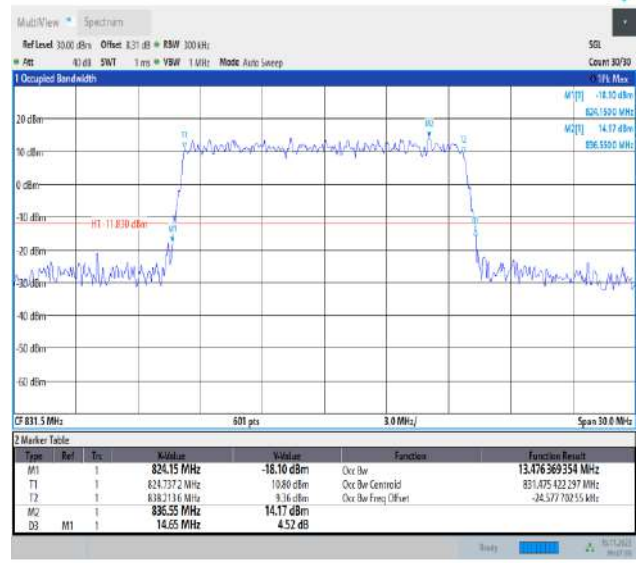
26(824-849)-15MHz-16QAM-26865-75RB#0-PASS
