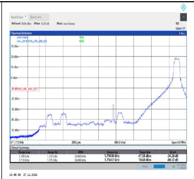
Band4_5MHz_QPSK_19975_1RB#24
