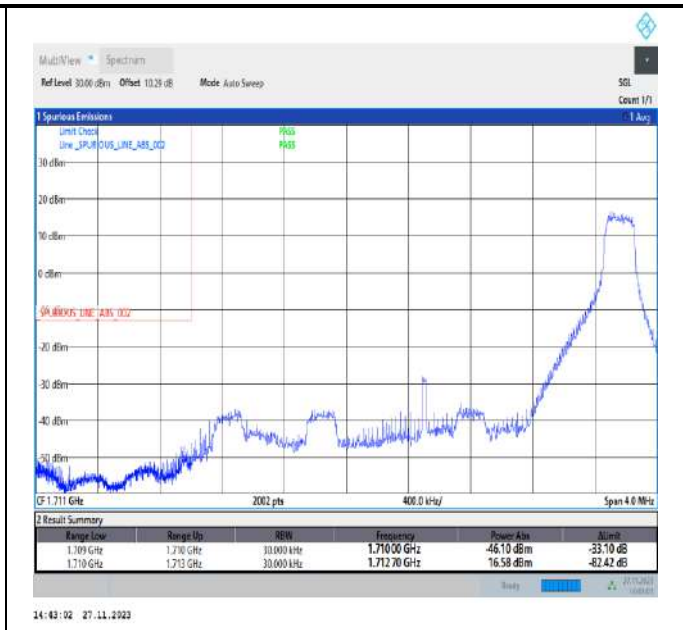
Band4_3MHz_16QAM_19965_1RB#14
