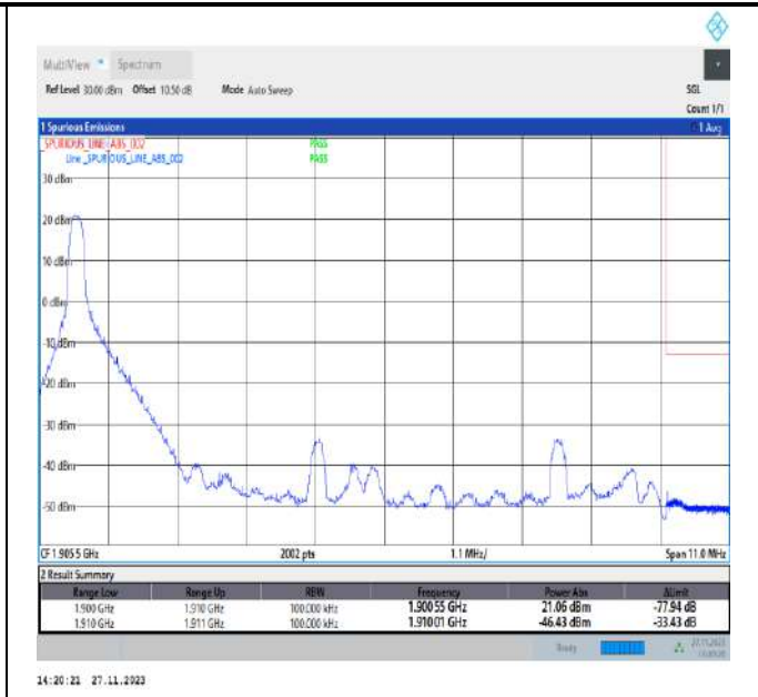
Band2_10MHz_QPSK_19150_1RB#0
