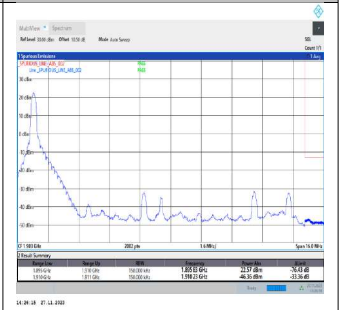
Band2_15MHz_QPSK_19125_1RB#0
