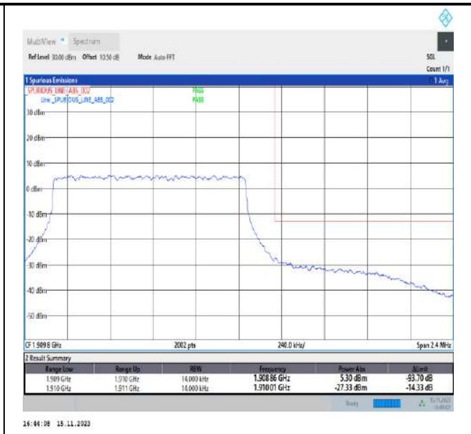
Band2_1.4MHz_QPSK_19193_6RB#0
