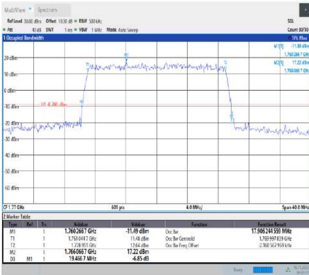
Band66-20MHz-16QAM-132572-100RB#0-PASS
