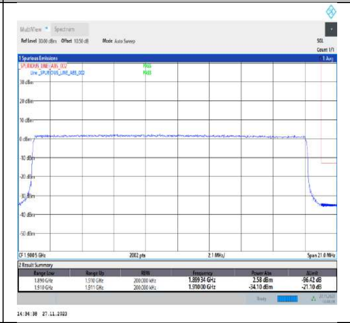
Band2_20MHz_64QAM_19100_100RB#0
