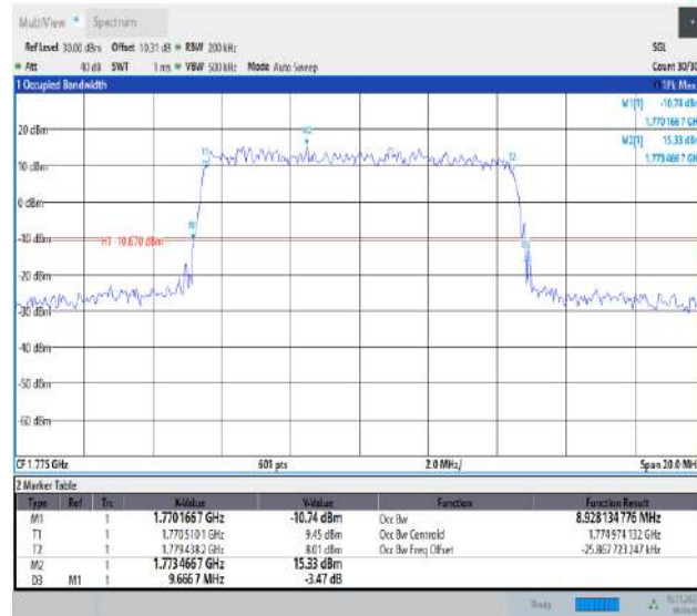
Band66-10MHz-64QAM-132622-50RB#0-PASS
