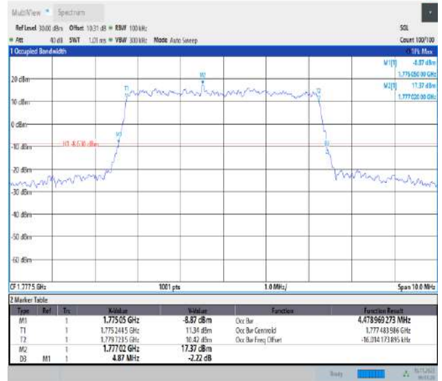
Band66-5MHz-16QAM-132647-25RB#0-PASS
