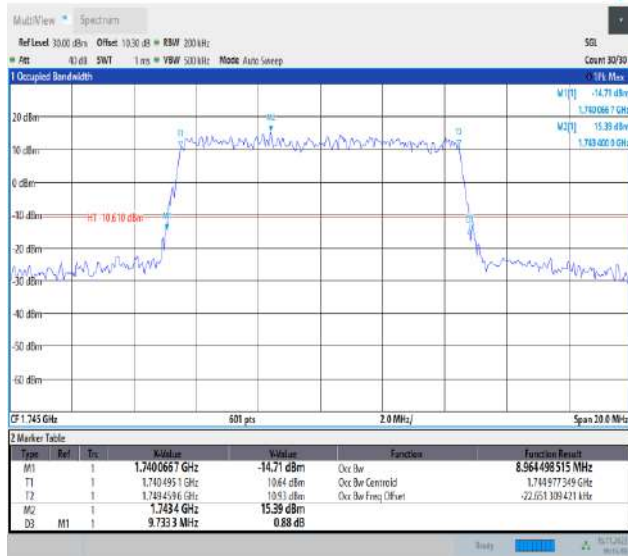
Band66-10MHz-64QAM-132322-50RB#0-PASS
