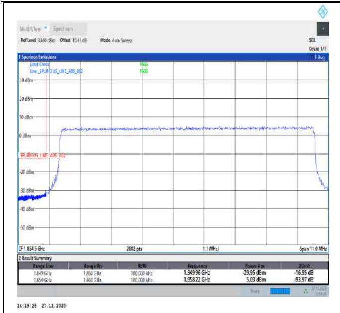
Band2_10MHz_QPSK_18650_50RB#0
