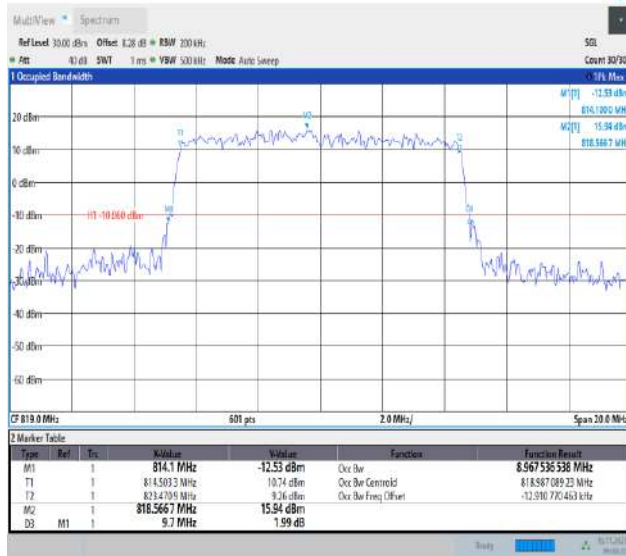
26(814-824)-10MHz-16QAM-26740-50RB#0-PASS
