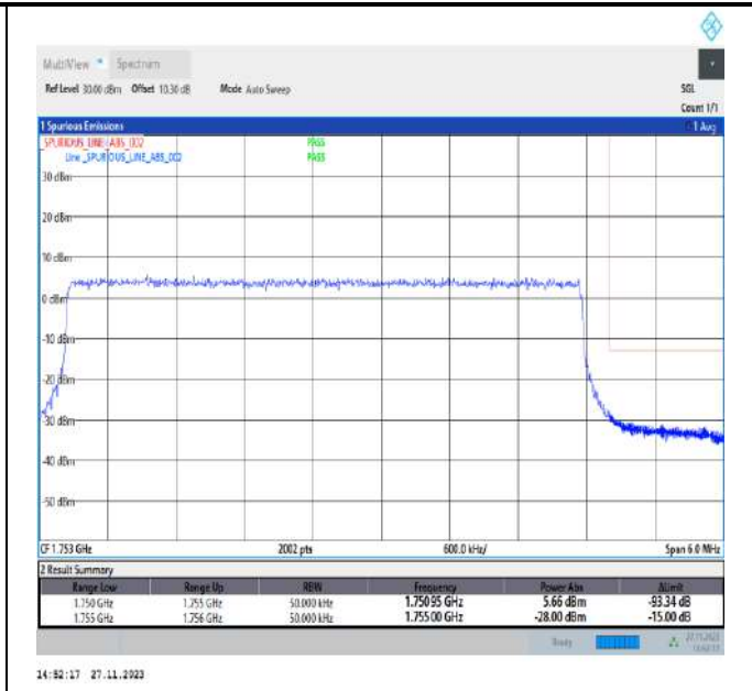
Band4_5MHz_QPSK_20375_25RB#0
