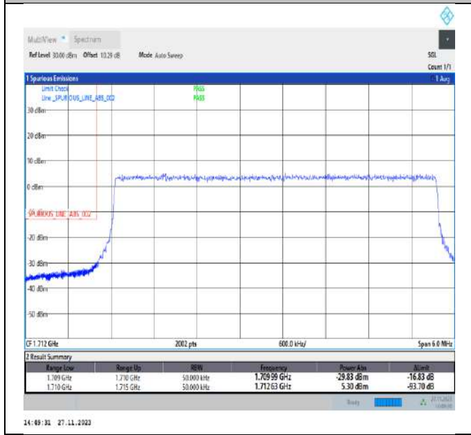
Band4_5MHz_QPSK_19975_25RB#0
