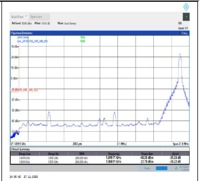
Band2_20MHz_16QAM_18700_1RB#99
