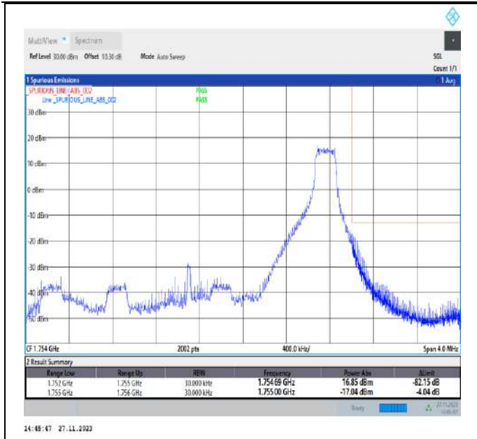
Band4_3MHz_16QAM_20385_1RB#14
