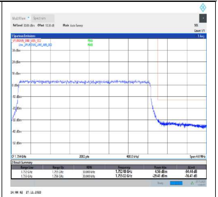
Band4_3MHz_16QAM_20385_15RB#0
