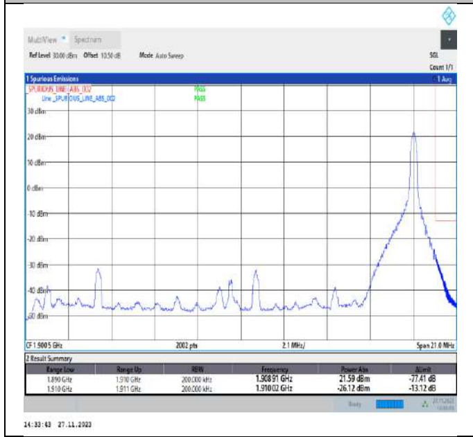
Band2_20MHz_64QAM_19100_1RB#99
