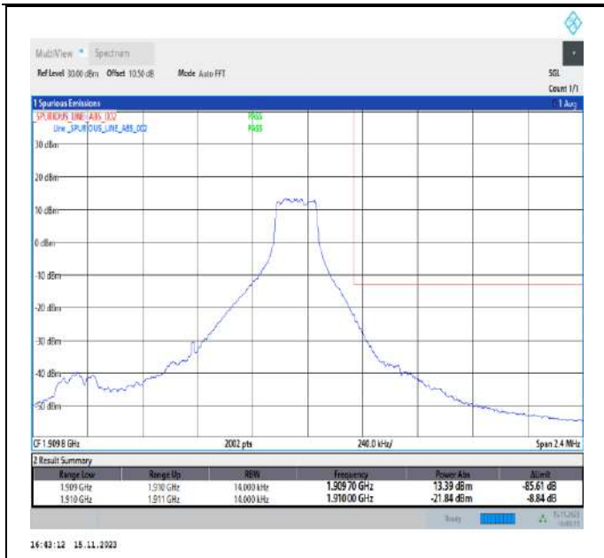
Band2_1.4MHz_QPSK_19193_1RB#5
