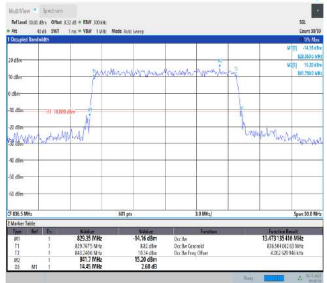
26(824-849)-15MHz-QPSK-26915-75RB#0-PASS
