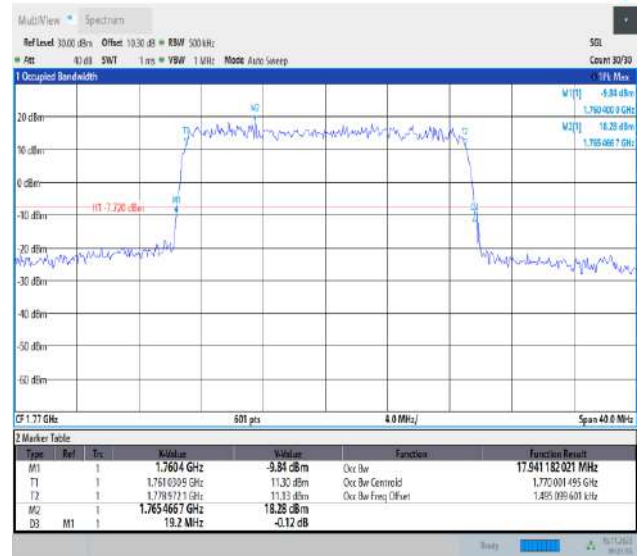
Band66-20MHz-QPSK-132572-100RB#0-PASS
