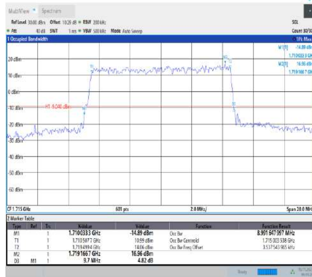
Band66-10MHz-QPSK-132022-50RB#0-PASS
