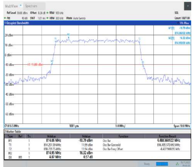
26(814-824)-5MHz-16QAM-26715-25RB#0-PASS
