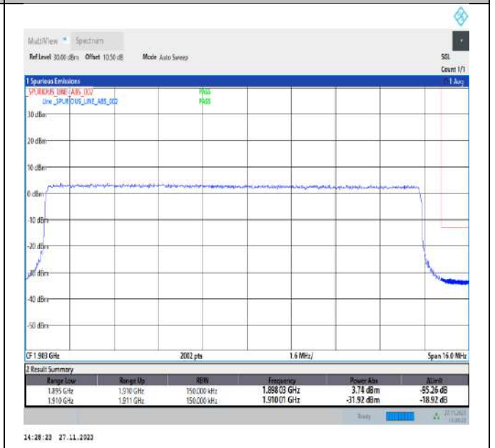
Band2_15MHz_16QAM_19125_75RB#0
