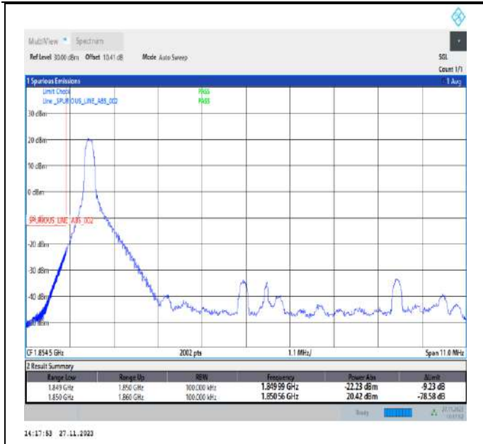
Band2_10MHz_16QAM_18650_1RB#0
