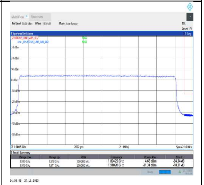
Band2_20MHz_QPSK_19100_100RB#0
