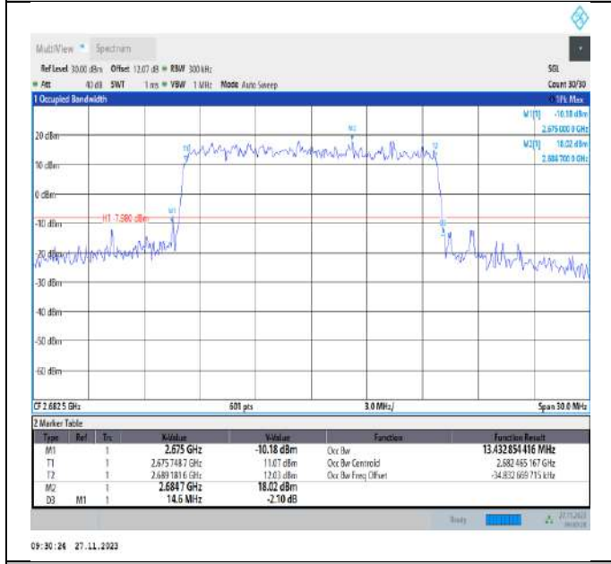
Band41-15MHz-QPSK-41515-75RB#0-PASS
