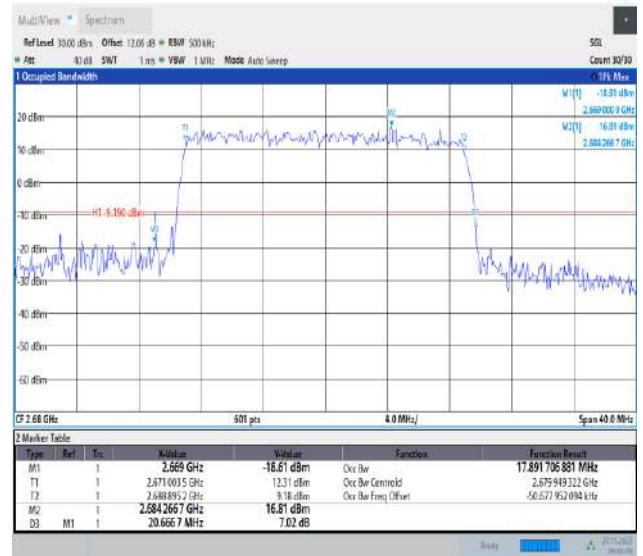
Band41-20MHz-64QAM-41490-100RB#0-PASS
