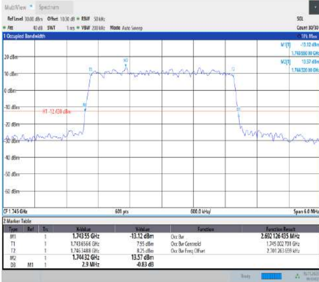
Band66-3MHz-64QAM-132322-15RB#0-PASS
