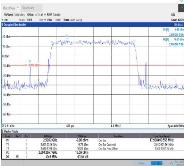
Band38-20MHz-16QAM-38150-100RB#0-PASS
