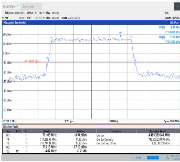
Band12-5MHz-QPSK-23155-25RB#0-PASS
