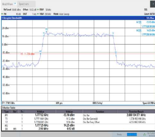
Band66-3MHz-16QAM-132657-15RB#0-PASS
