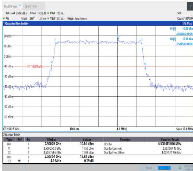
Band7-5MHz-QPSK-20775-25RB#0-PASS
