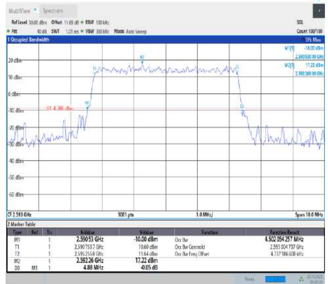
Band41-5MHz-QPSK-40620-25RB#0-PASS
