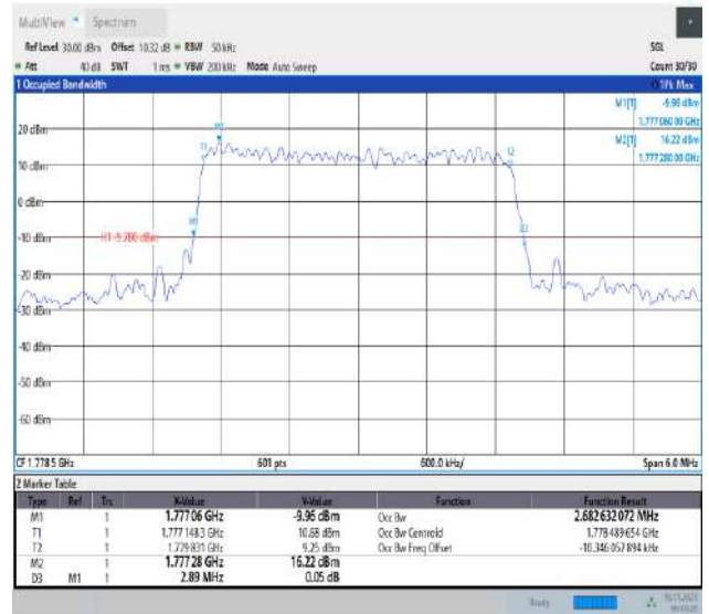
Band66-3MHz-QPSK-132657-15RB#0-PASS
