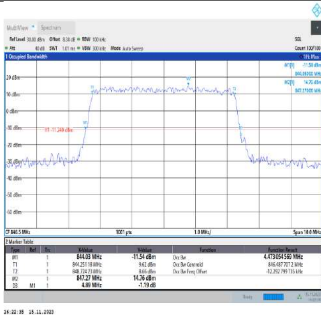
Band5-5MHz-64QAM-20625-25RB#0-PASS
