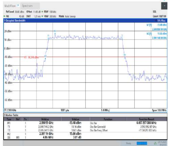
Band41-5MHz-64QAM-40620-25RB#0-PASS
