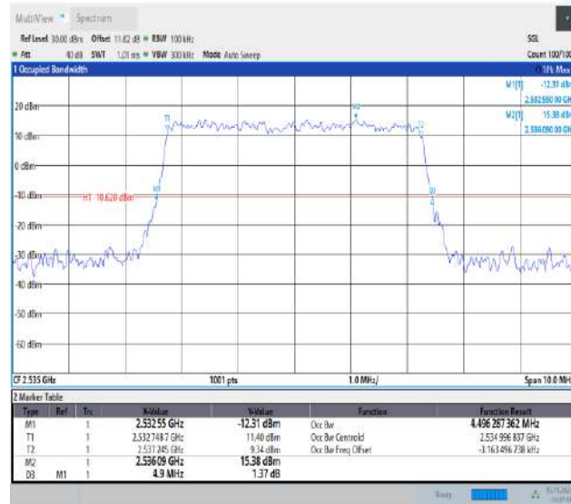
Band7-5MHz-QPSK-21100-25RB#0-PASS
