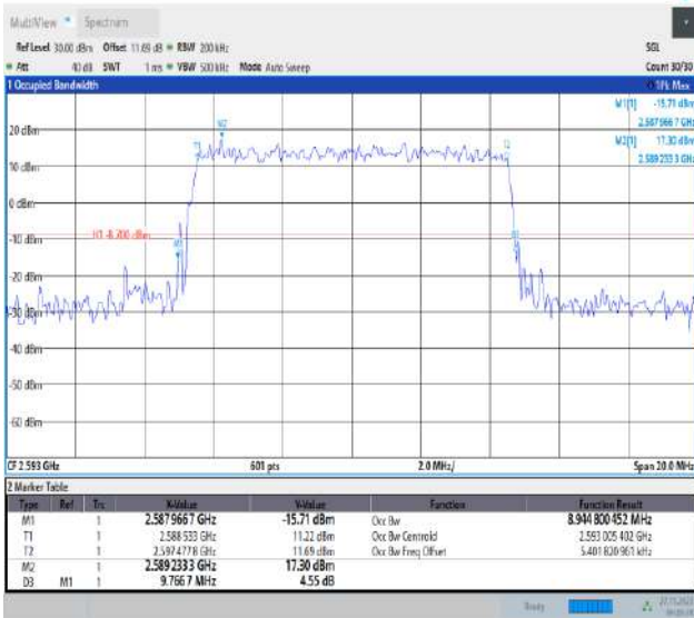
Band41-10MHz-QPSK-40620-50RB#0-PASS
