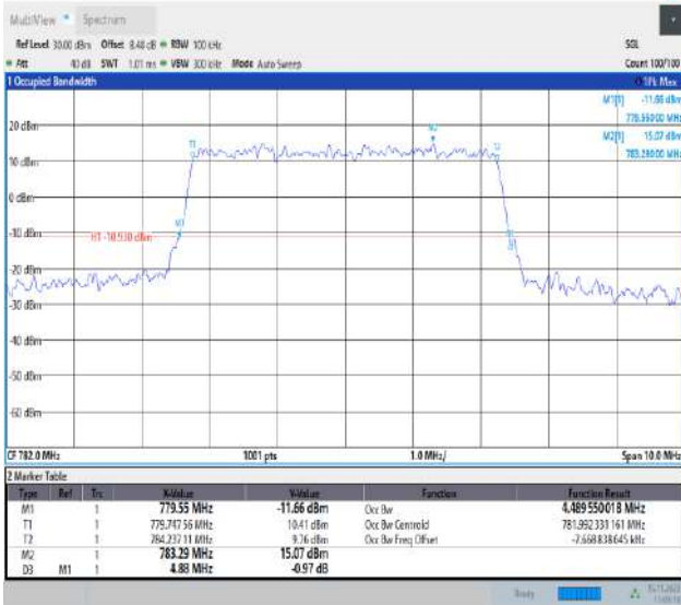
Band13-5MHz-16QAM-23230-25RB#0-PASS
