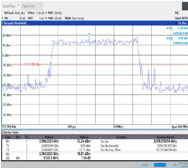
Band38-10MHz-QPSK-38000-50RB#0-PASS
