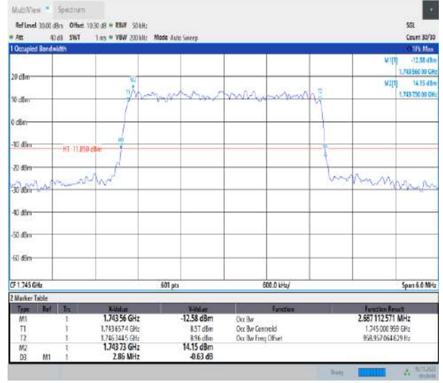
Band66-3MHz-16QAM-132322-15RB#0-PASS
