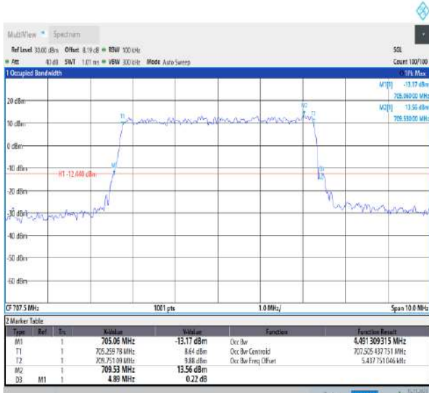
Band12-5MHz-QPSK-23155-25RB#0-PASS
