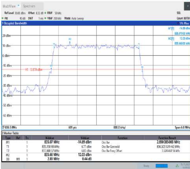
Band5-3MHz-64QAM-20525-15RB#0-PASS
