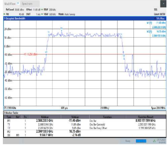
Band41-10MHz-16QAM-40620-50RB#0-PASS
