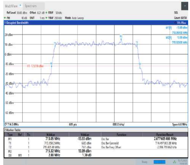
Band12-3MHz-64QAM-23165-15RB#0-PASS
