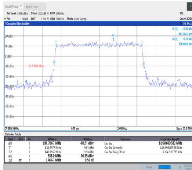
Band5-10MHz-16QAM-20525-50RB#0-PASS
