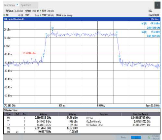
Band41-10MHz-QPSK-41540-50RB#0-PASS
