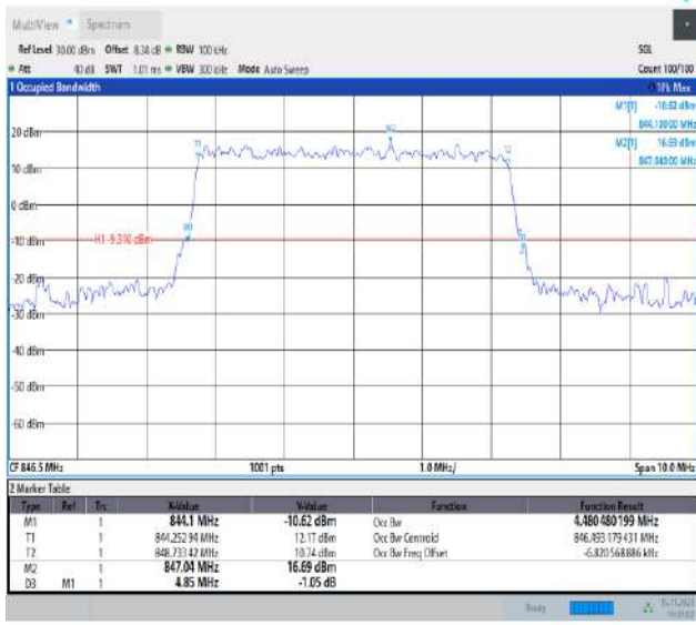
Band5-5MHz-QPSK-20625-25RB#0-PASS
