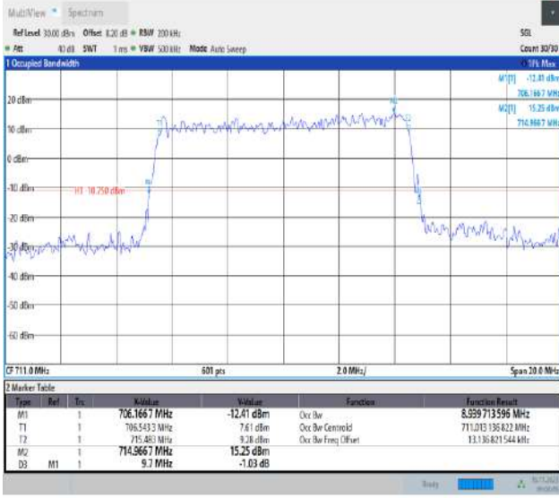
Band17-10MHz-16QAM-23800-50RB#0-PASS
