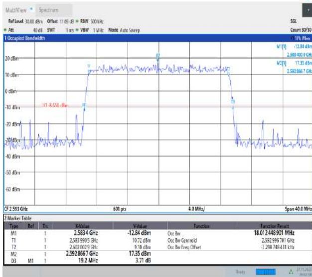
Band41-20MHz-64QAM-40620-100RB#0-PASS
