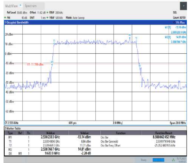
Band7-10MHz-16QAM-21100-50RB#0-PASS
