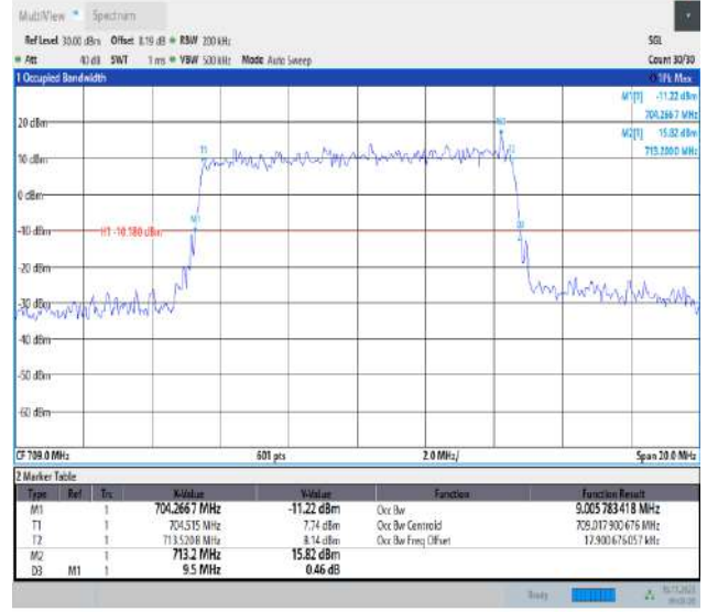
Band17-10MHz-64QAM-23780-50RB#0-PASS
