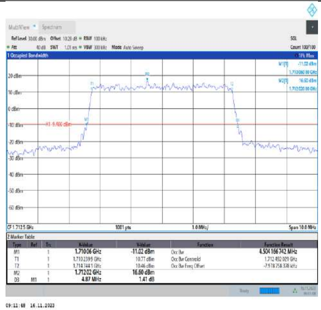
Band66-5MHz-16QAM-131997-25RB#0-PASS
