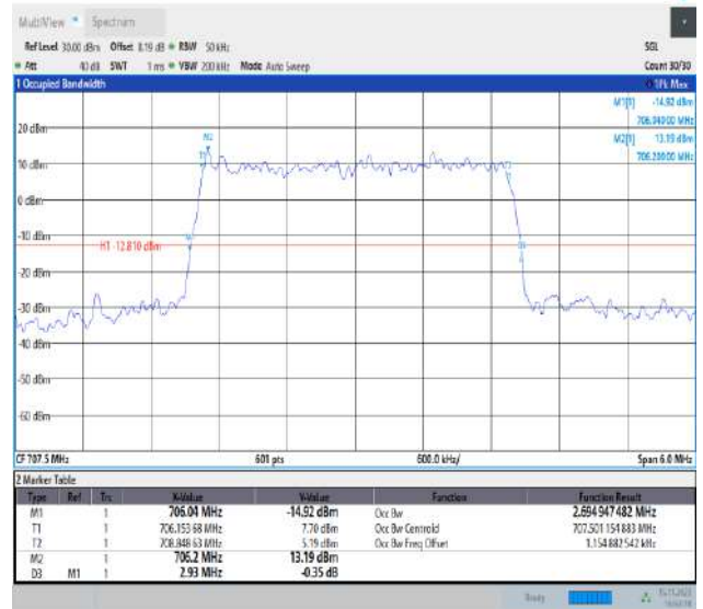
Band12-3MHz-16QAM-23095-15RB#0-PASS
