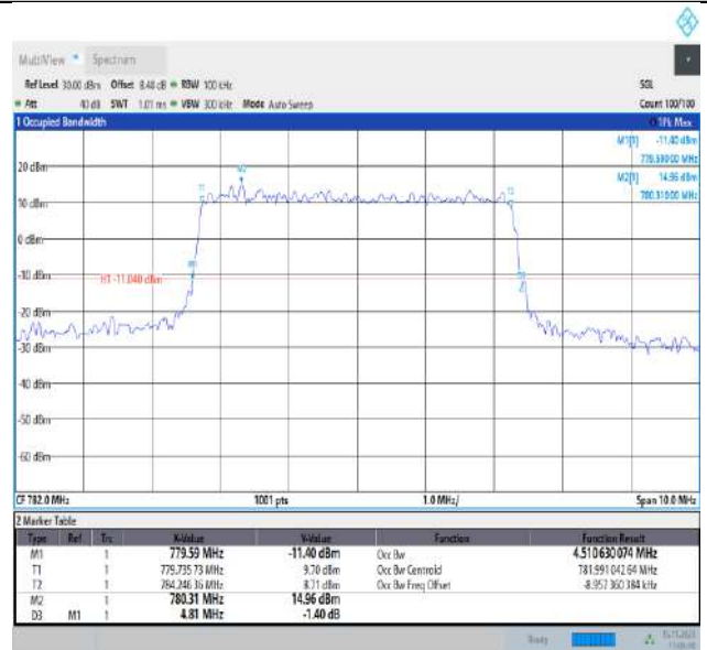
Band13-5MHz-16QAM-23255-25RB#0-PASS
