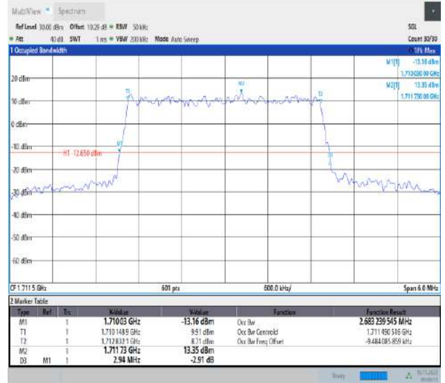
Band66-3MHz-64QAM-131987-15RB#0-PASS
