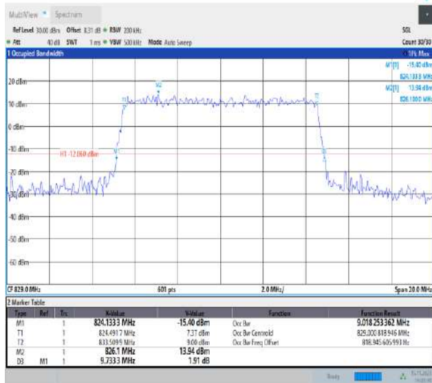
Band5-10MHz-16QAM-20450-50RB#0-PASS
