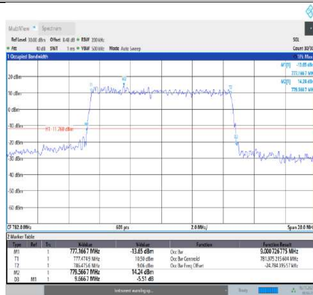
Band13-10MHz-QPSK-23230-50RB#0-PASS
