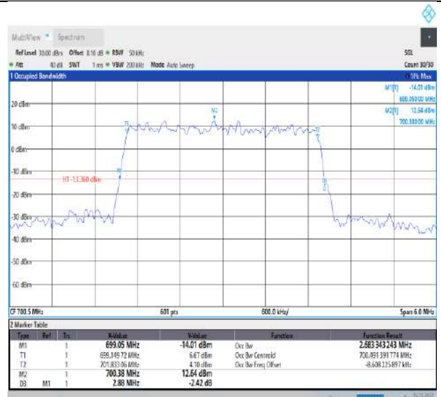
Band12-3MHz-16QAM-23095-15RB#0-PASS
