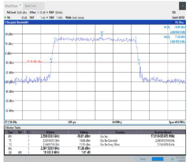
Band7-20MHz-QPSK-21350-100RB#0-PASS
