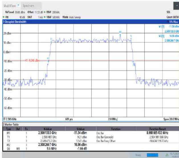
Band7-10MHz-16QAM-20800-50RB#0-PASS
