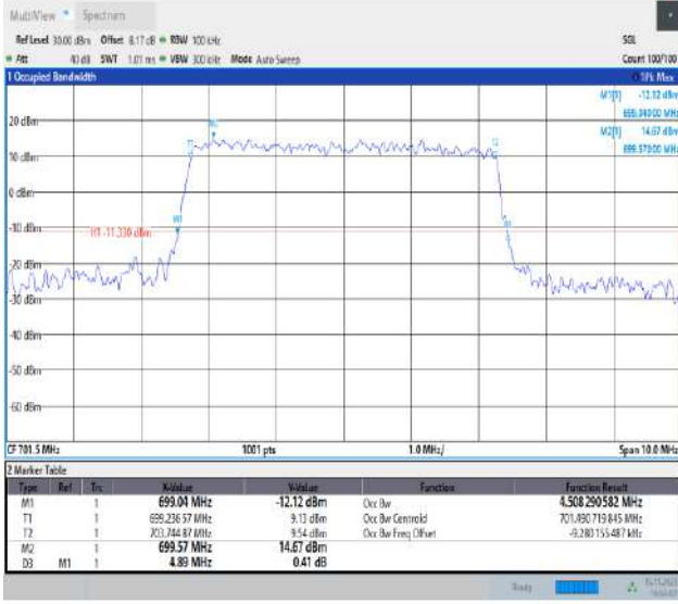
Band12-5MHz-QPSK-23035-25RB#0-PASS
