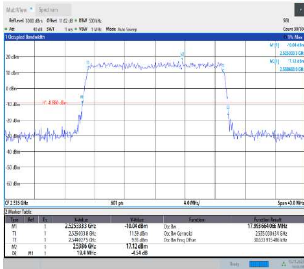
Band7-20MHz-QPSK-21100-100RB#0-PASS
