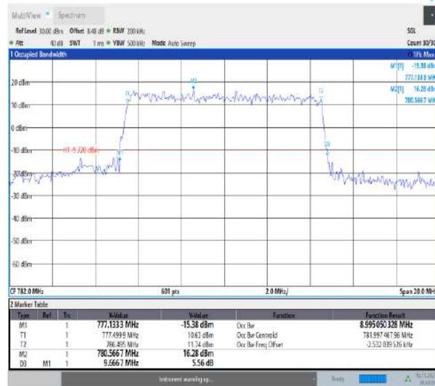
Band13-10MHz-QPSK-23230-50RB#0-PASS
