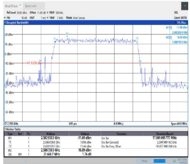
Band38-20MHz-16QAM-38000-100RB#0-PASS
