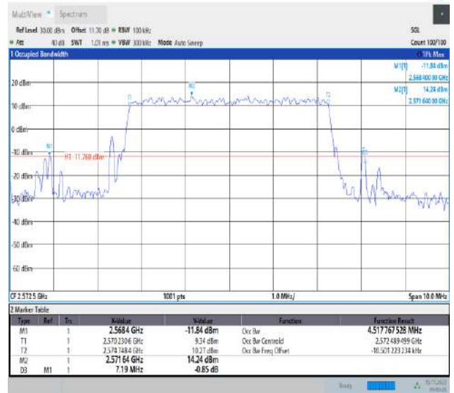
Band38-5MHz-16QAM-37775-25RB#0-PASS
