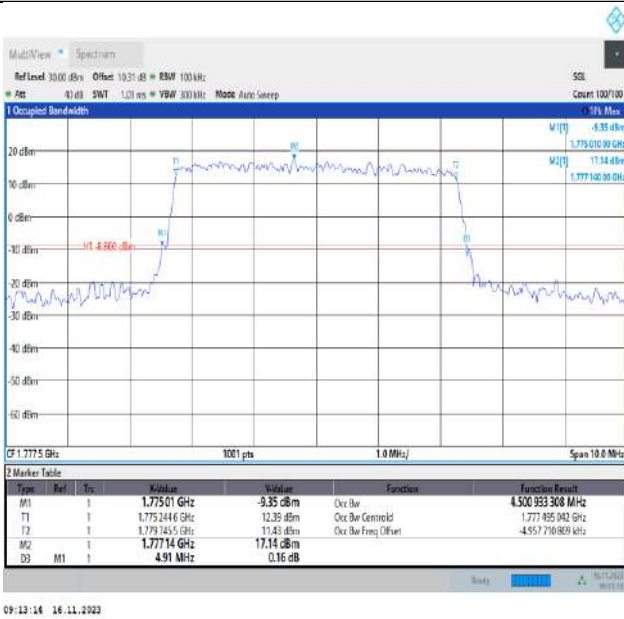
Band66-5MHz-QPSK-132647-25RB#0-PASS
