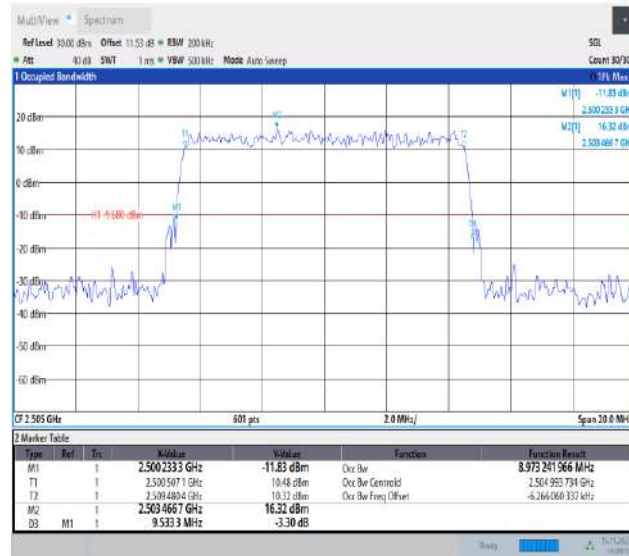
Band7-10MHz-QPSK-20800-50RB#0-PASS
