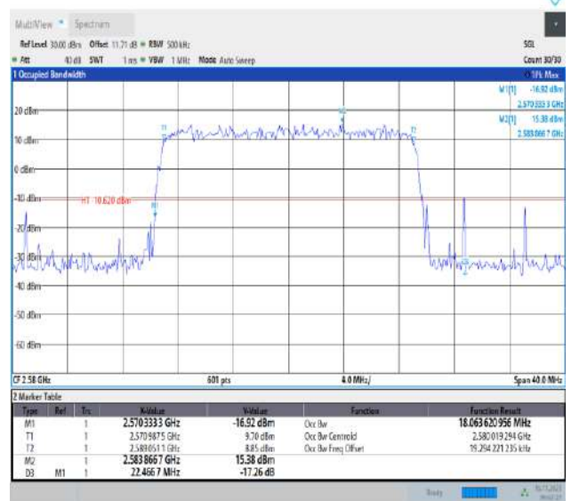
Band38-20MHz-64QAM-37850-100RB#0-PASS
