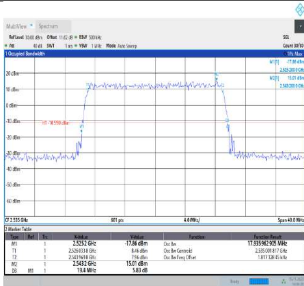
Band7-20MHz-16QAM-21350-100RB#0-PASS
