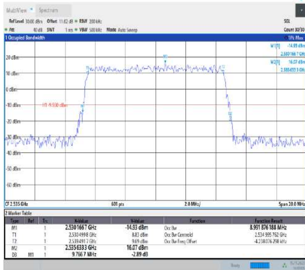
Band7-10MHz-QPSK-21100-50RB#0-PASS
