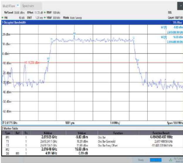
Band38-5MHz-QPSK-38225-25RB#0-PASS
