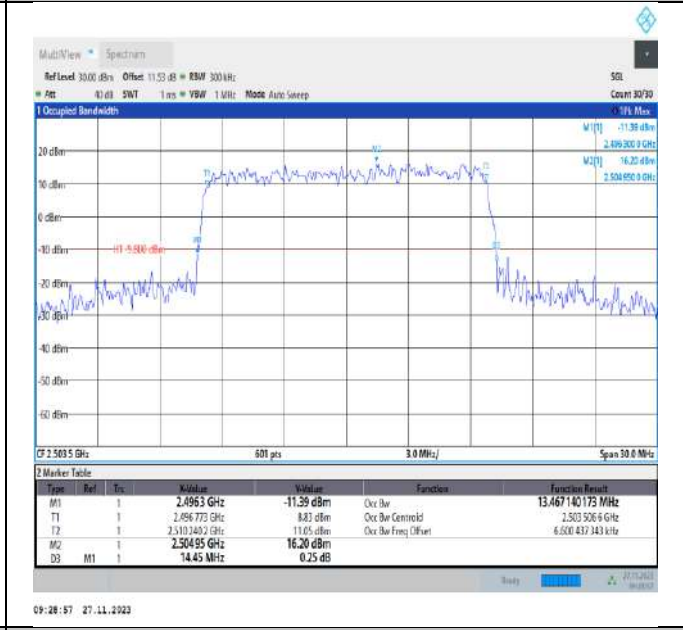
Band41-15MHz-16QAM-39725-75RB#0-PASS
