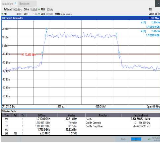
Band66-3MHz-16QAM-131987-15RB#0-PASS
