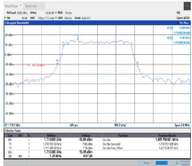
Band66-1.4MHz-16QAM-131979-6RB#0-PASS
