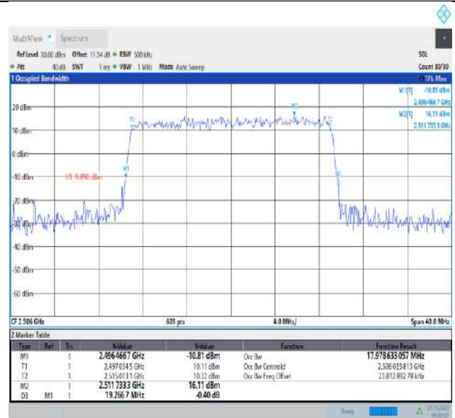
Band41-20MHz-16QAM-40620-100RB#0-PASS
