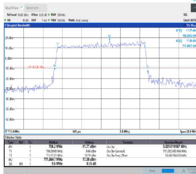
Band12-10MHz-QPSK-23130-50RB#0-PASS
