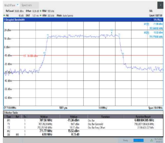
Band17-5MHz-QPSK-23790-25RB#0-PASS
