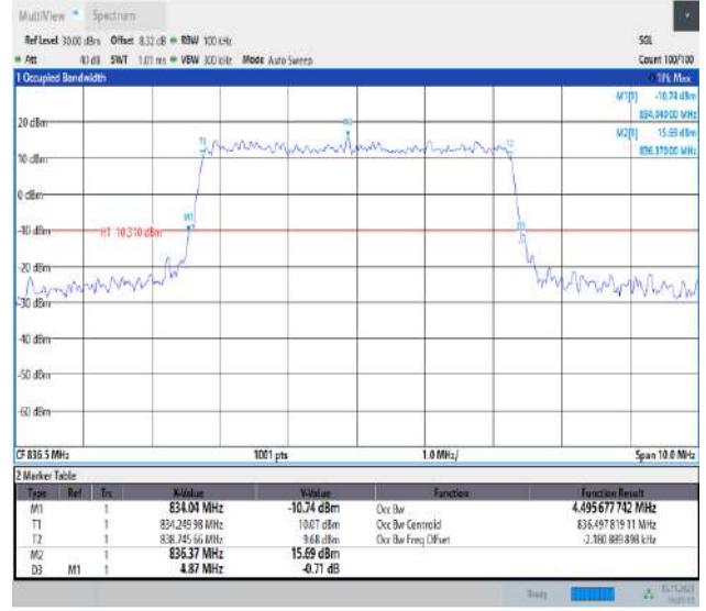
Band5-5MHz-QPSK-20525-25RB#0-PASS
