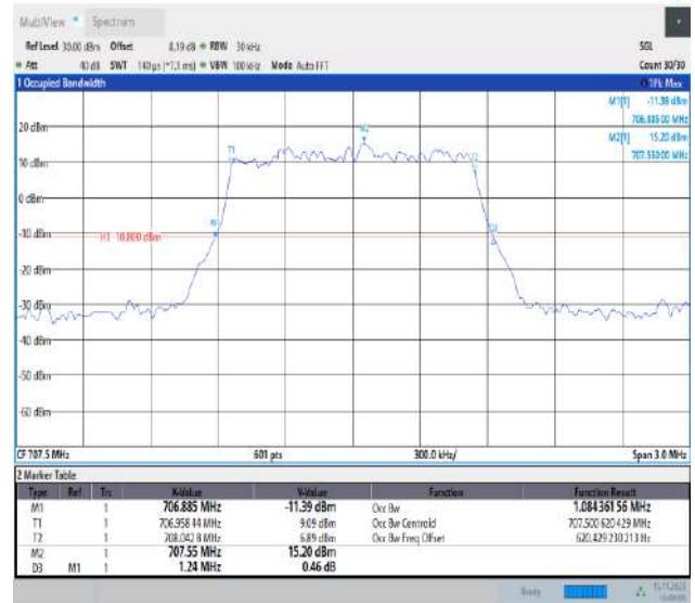
Band12-1.4MHz-QPSK-23095-6RB#0-PASS
