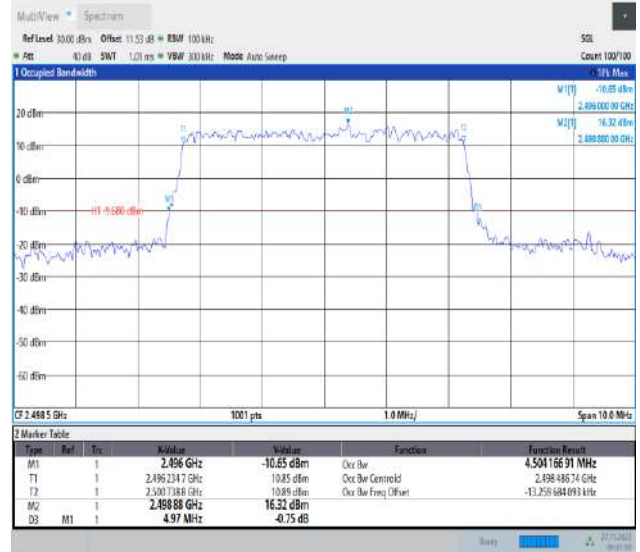
Band41-5MHz-16QAM-39675-25RB#0-PASS
