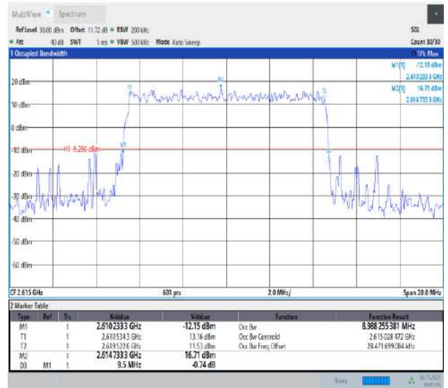
Band38-10MHz-QPSK-38200-50RB#0-PASS
