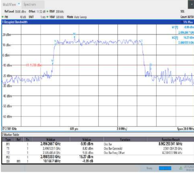
Band41-10MHz-16QAM-39700-50RB#0-PASS
