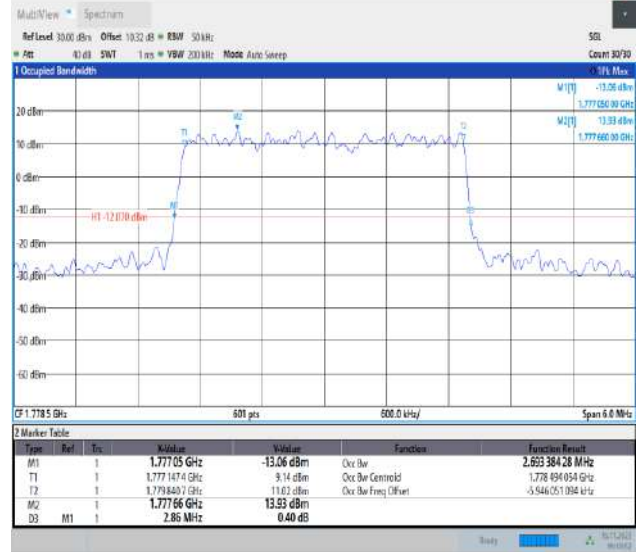
Band66-3MHz-64QAM-132657-15RB#0-PASS
