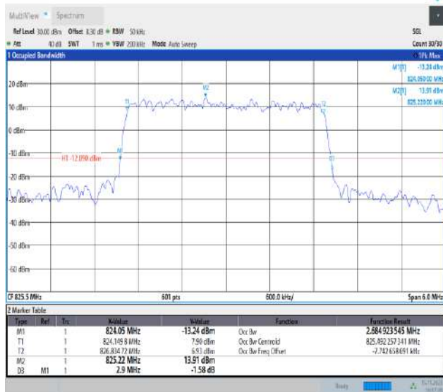
Band5-3MHz-16QAM-20415-15RB#0-PASS
