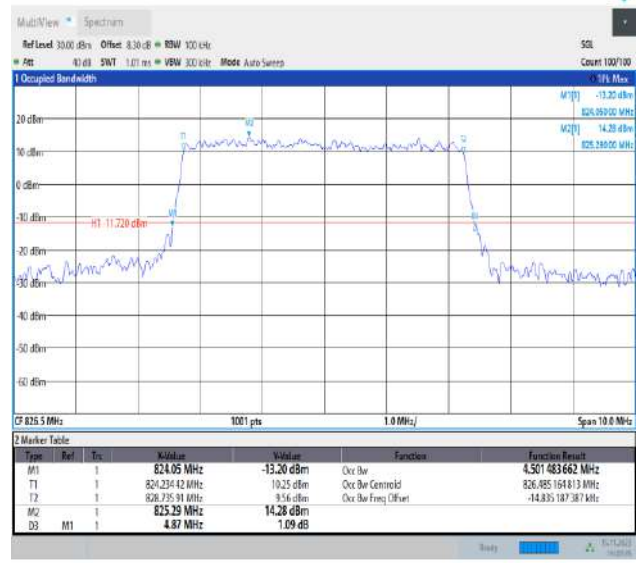
Band5-5MHz-16QAM-20425-25RB#0-PASS
