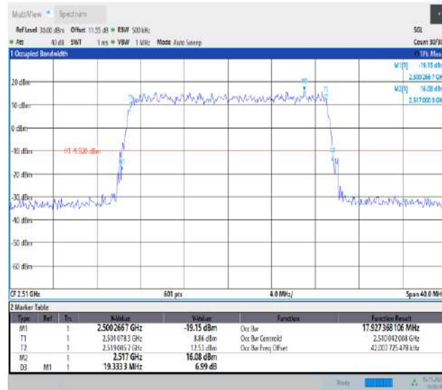
Band7-20MHz-64QAM-20850-100RB#0-PASS
