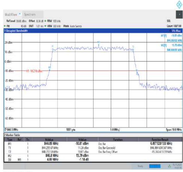
Band5-5MHz-16QAM-20625-25RB#0-PASS
