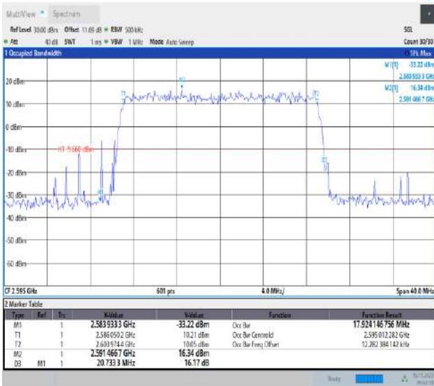
Band38-20MHz-64QAM-38000-100RB#0-PASS
