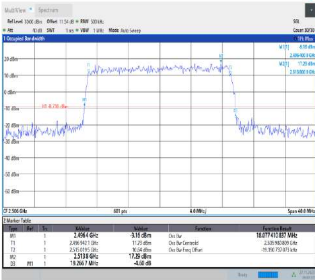
Band41-20MHz-16QAM-39750-100RB#0-PASS
