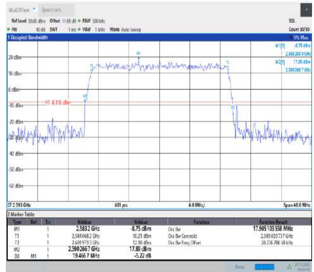
Band41-20MHz-16QAM-40620-100RB#0-PASS
