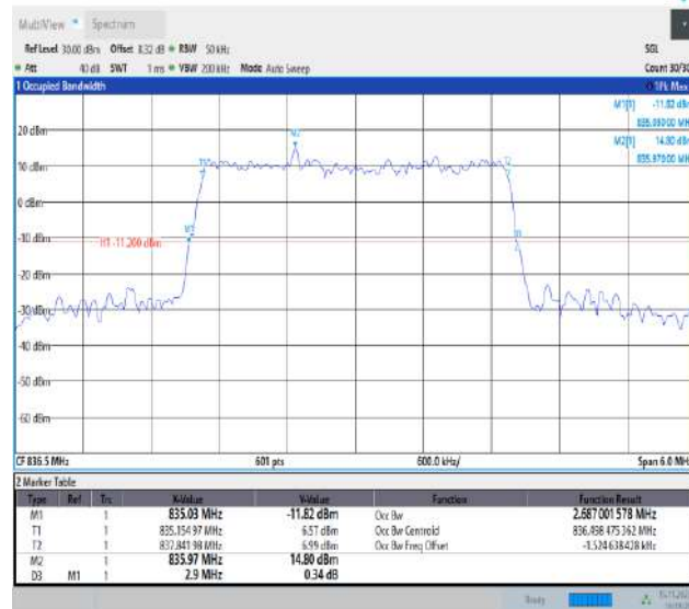
Band5-3MHz-16QAM-20525-15RB#0-PASS
