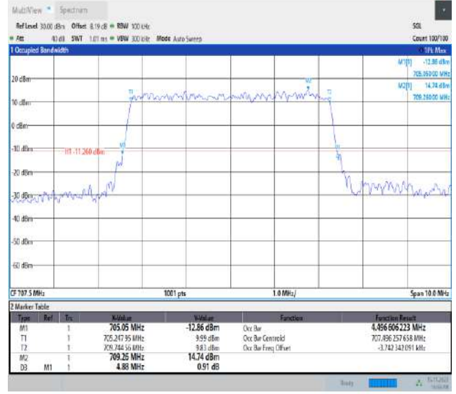
Band12-5MHz-QPSK-23095-25RB#0-PASS
