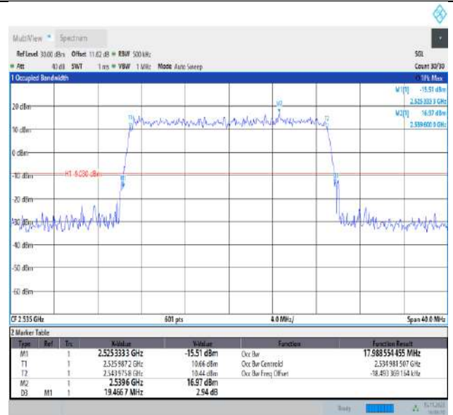
Band7-20MHz-QPSK-21350-100RB#0-PASS
