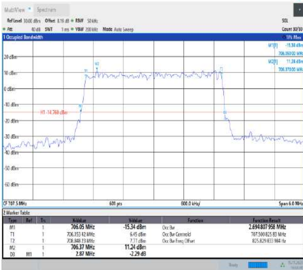
Band12-3MHz-64QAM-23095-15RB#0-PASS
