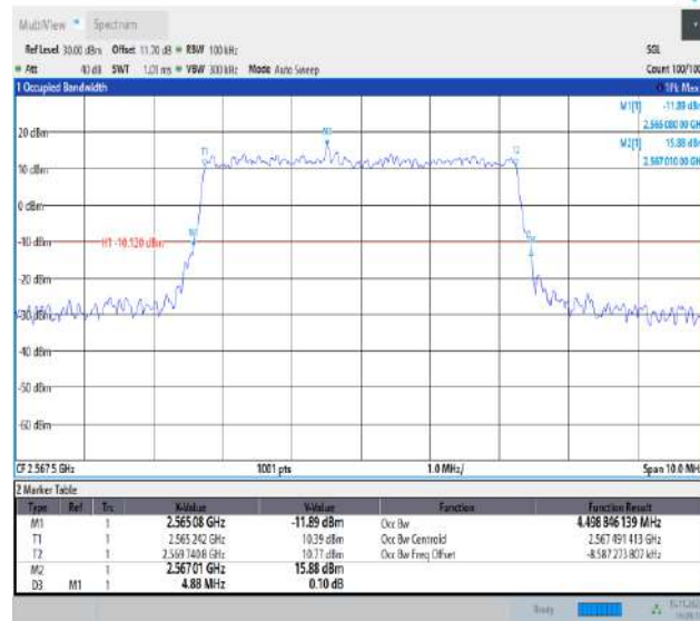
Band7-5MHz-16QAM-21425-25RB#0-PASS
