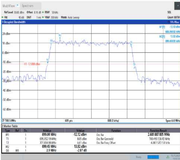
Band12-3MHz-16QAM-23025-15RB#0-PASS
