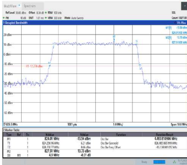
Band5-5MHz-64QAM-20425-25RB#0-PASS
