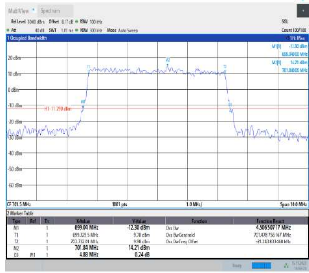
Band12-5MHz-16QAM-23035-25RB#0-PASS
