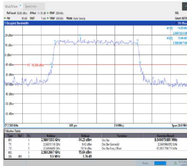
Band7-10MHz-QPSK-21400-50RB#0-PASS
