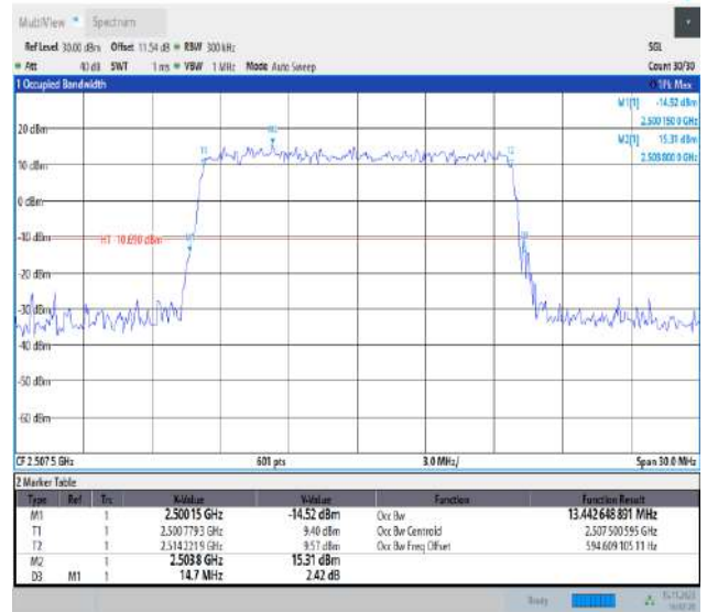
Band7-15MHz-16QAM-20825-75RB#0-PASS
