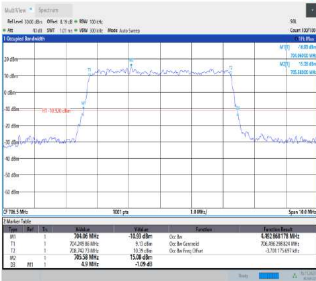
Band17-5MHz-QPSK-23755-25RB#0-PASS
