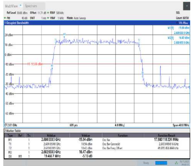
Band38-20MHz-64QAM-38150-100RB#0-PASS
