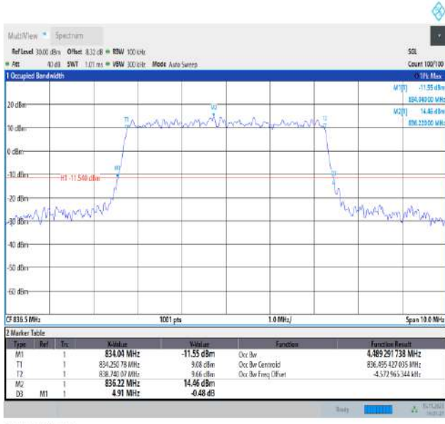
Band5-5MHz-16QAM-20525-25RB#0-PASS
