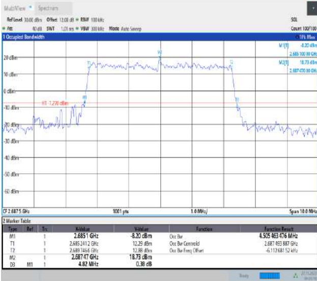
Band41-5MHz-QPSK-41565-25RB#0-PASS
