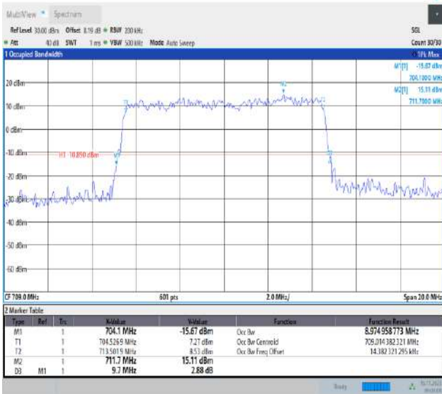
Band17-10MHz-16QAM-23780-50RB#0-PASS
