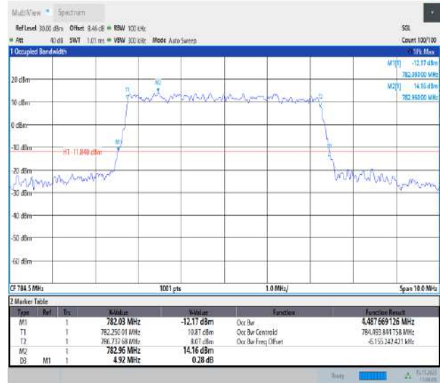
Band13-5MHz-16QAM-23255-25RB#0-PASS
