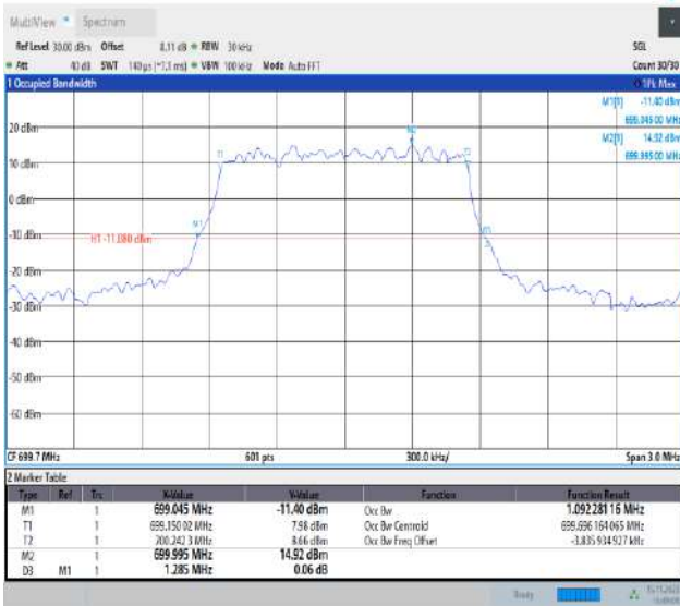
Band12-1.4MHz-QPSK-23017-6RB#0-PASS
