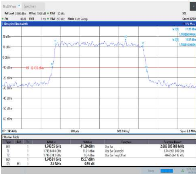
Band66-3MHz-QPSK-132322-15RB#0-PASS
