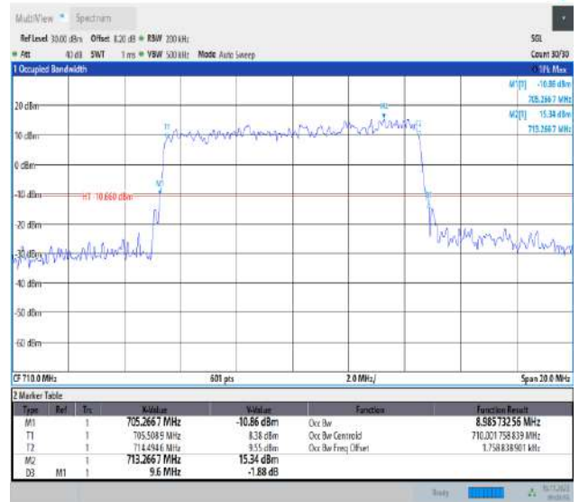
Band17-10MHz-16QAM-23790-50RB#0-PASS
