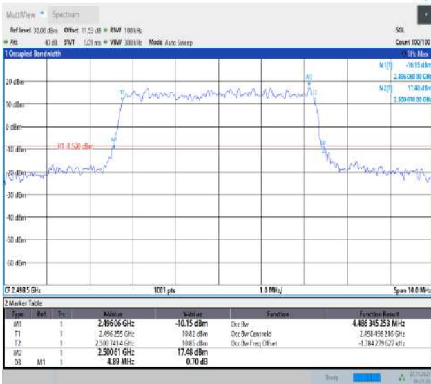
Band41-5MHz-QPSK-39675-25RB#0-PASS
