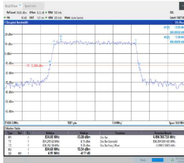
Band5-5MHz-64QAM-20525-25RB#0-PASS
