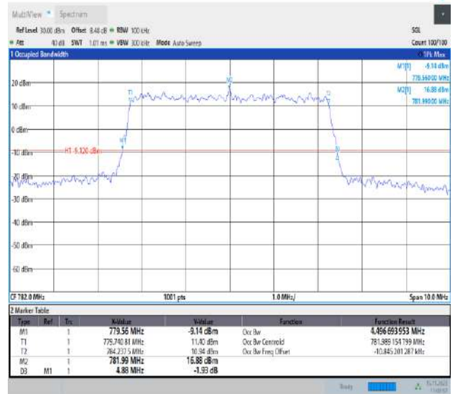
Band13-5MHz-QPSK-23230-25RB#0-PASS
