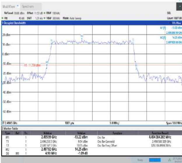
Band41-5MHz-64QAM-39675-25RB#0-PASS
