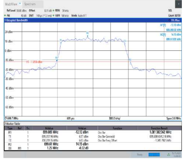
Band12-1.4MHz-16QAM-23017-6RB#0-PASS
