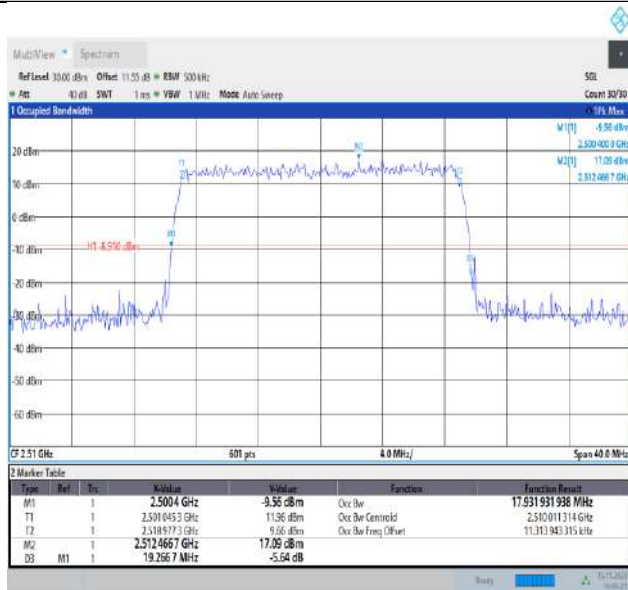
Band7-20MHz-QPSK-21100-100RB#0-PASS
