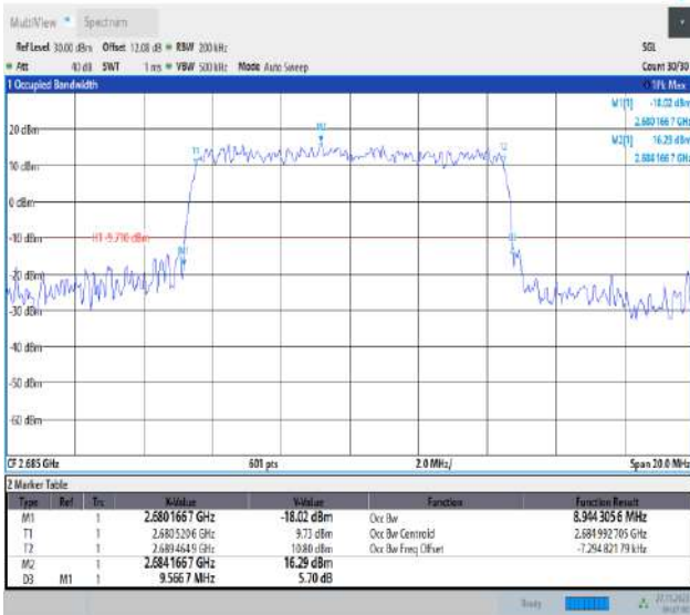
Band41-10MHz-16QAM-41540-50RB#0-PASS
