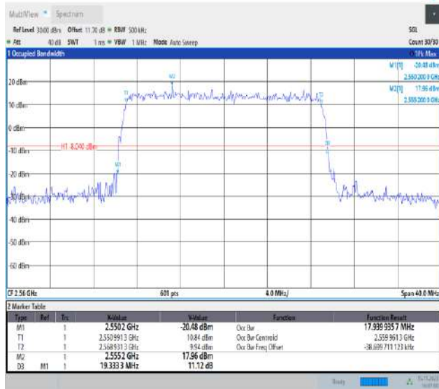
Band7-20MHz-16QAM-21350-100RB#0-PASS
