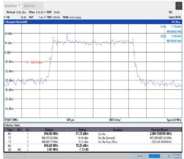
Band5-3MHz-64QAM-20635-15RB#0-PASS
