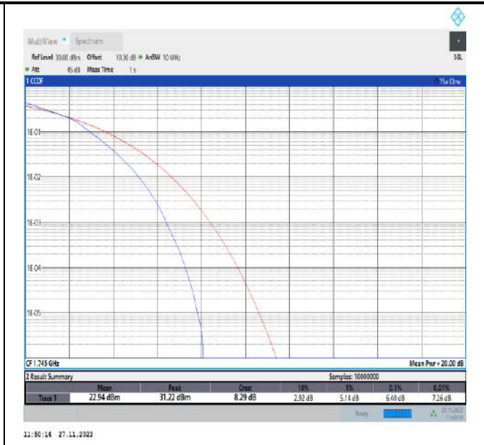
Band66-10MHz-16QAM-132322-50RB#0-PASS
