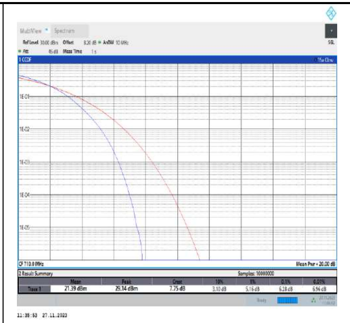
Band17-10MHz-16QAM-23790-50RB#0-PASS
