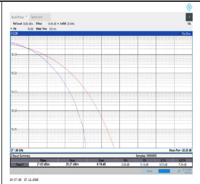
Band2-15MHz-64QAM-18900-75RB#0-PASS
