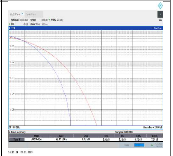
Band2-20MHz-64QAM-18900-100RB#0-PASS
