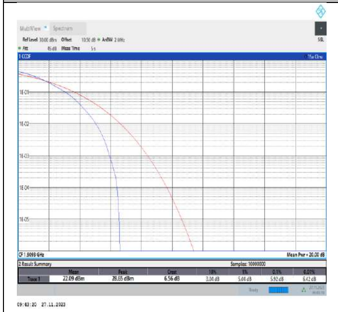
Band2-1.4MHz-64QAM-19193-1RB#0-PASS
