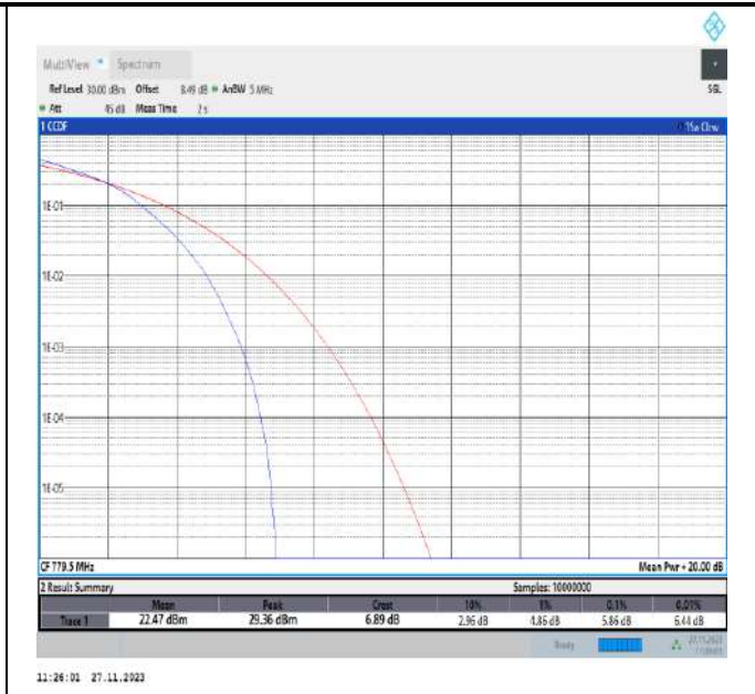
Band13-5MHz-16QAM-23205-25RB#0-PASS
