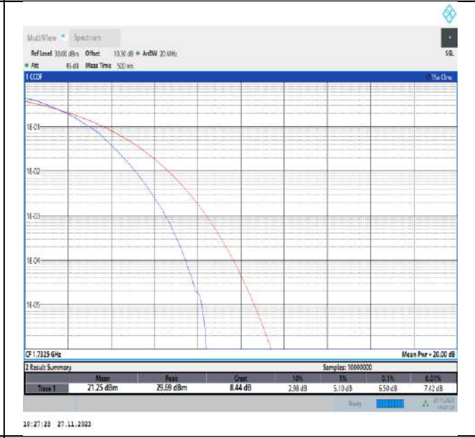
Band4-15MHz-64QAM-20175-75RB#0-PASS
