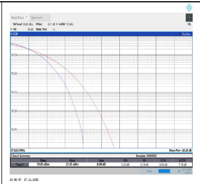
Band5-10MHz-64QAM-20450-50RB#0-PASS
