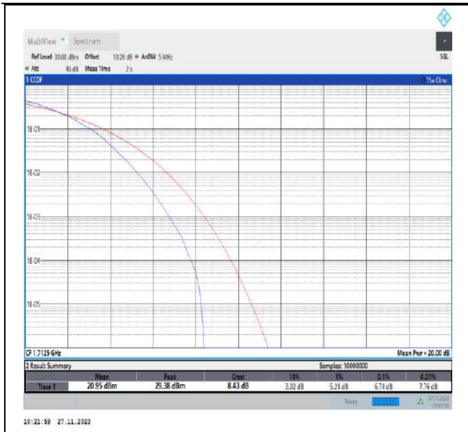
Band4-5MHz-64QAM-19975-25RB#0-PASS
