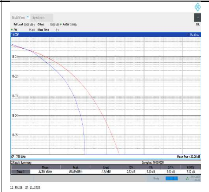
Band66-3MHz-16QAM-132322-15RB#0-PASS
