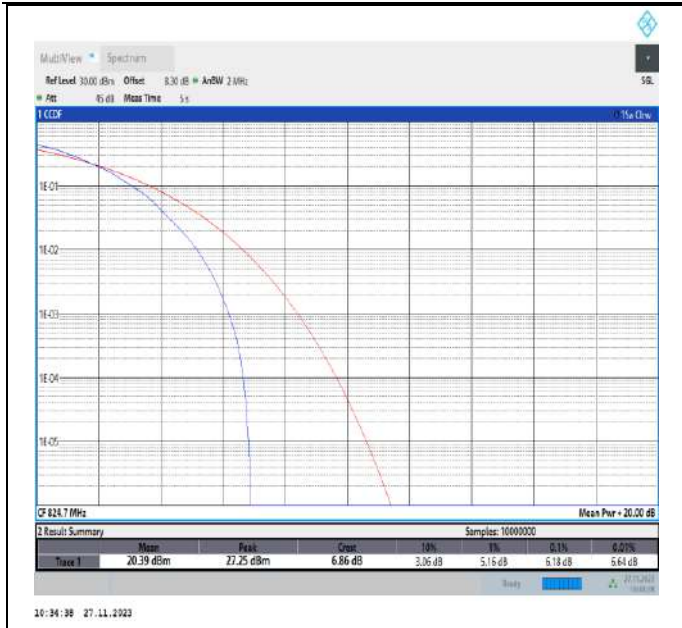
Band5-1.4MHz-64QAM-20407-6RB#0-PASS
