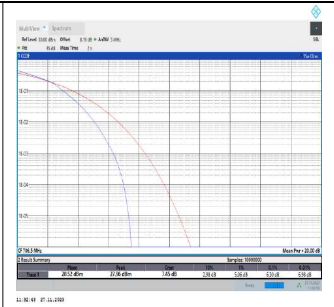
Band17-5MHz-16QAM-23755-25RB#0-PASS
