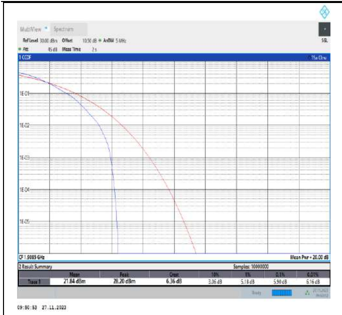
Band2-3MHz-64QAM-19185-1RB#0-PASS
