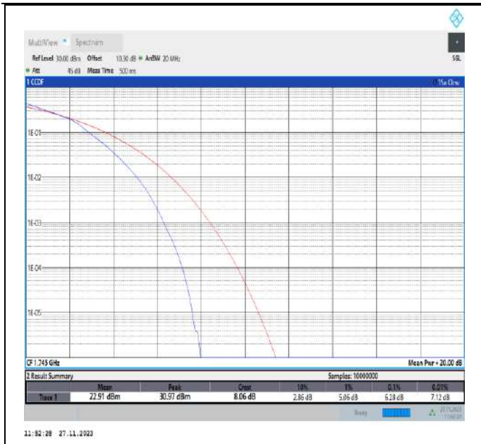
Band66-15MHz-16QAM-132322-75RB#0-PASS
