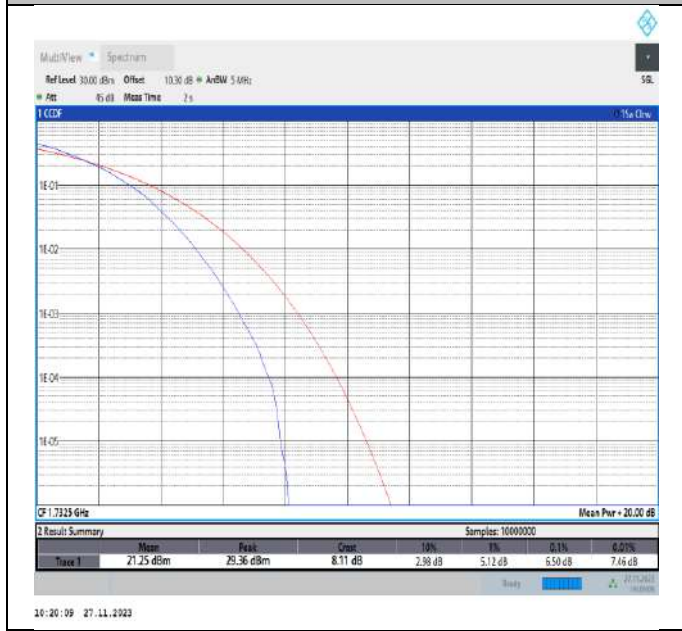
Band4-3MHz-64QAM-20175-15RB#0-PASS
