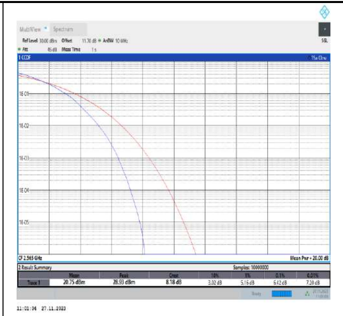
Band7-10MHz-64QAM-21400-50RB#0-PASS
