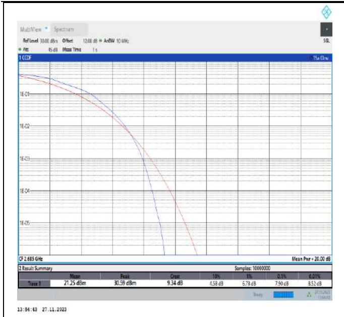
Band41-10MHz-16QAM-41540-50RB#0-PASS
