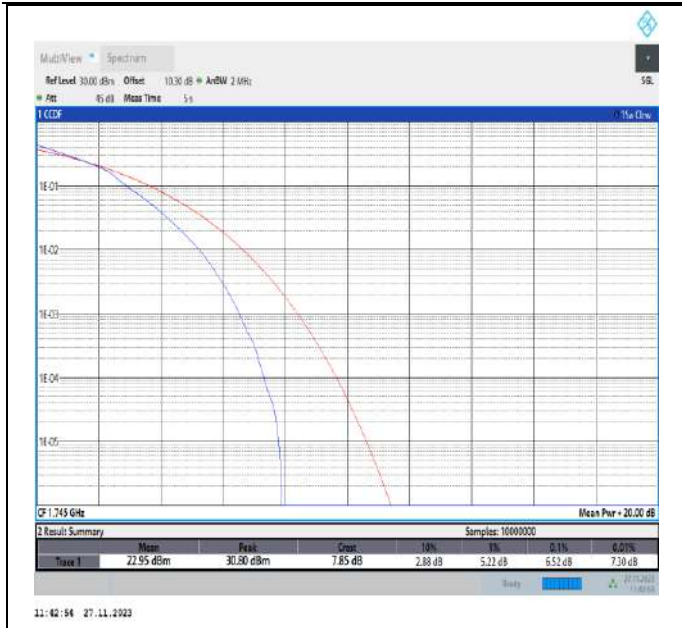
Band66-1.4MHz-16QAM-132322-6RB#0-PASS
