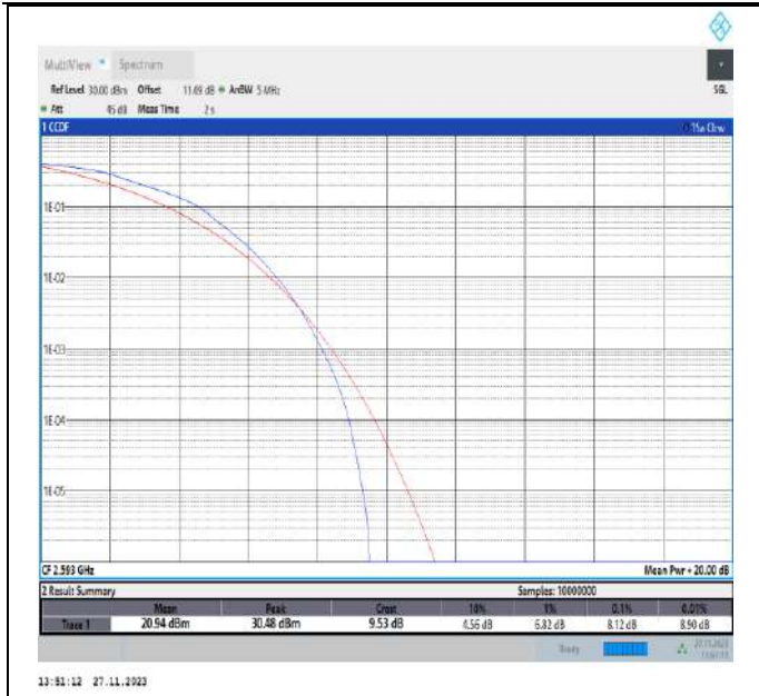
Band41-5MHz-16QAM-40620-25RB#0-PASS
