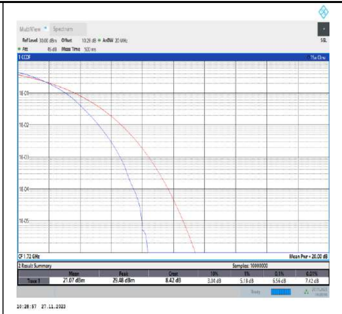
Band4-20MHz-64QAM-20050-100RB#0-PASS
