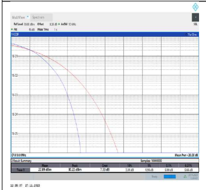
26(814-824)-10MHz-16QAM-26740-50RB#0-PASS
