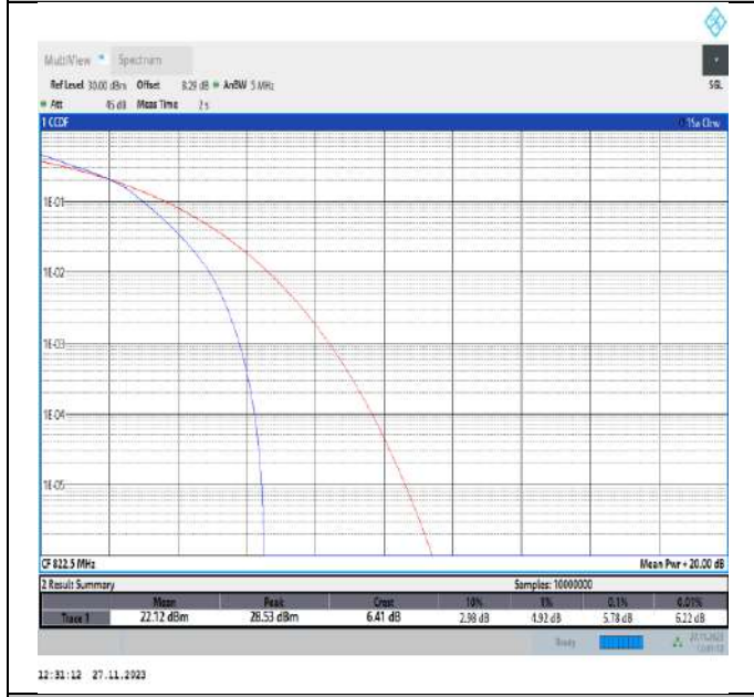
26(814-824)-3MHz-16QAM-26775-15RB#0-PASS
