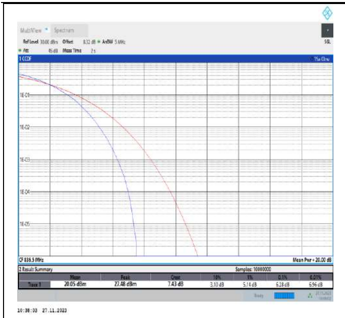
Band5-3MHz-64QAM-20525-15RB#0-PASS
