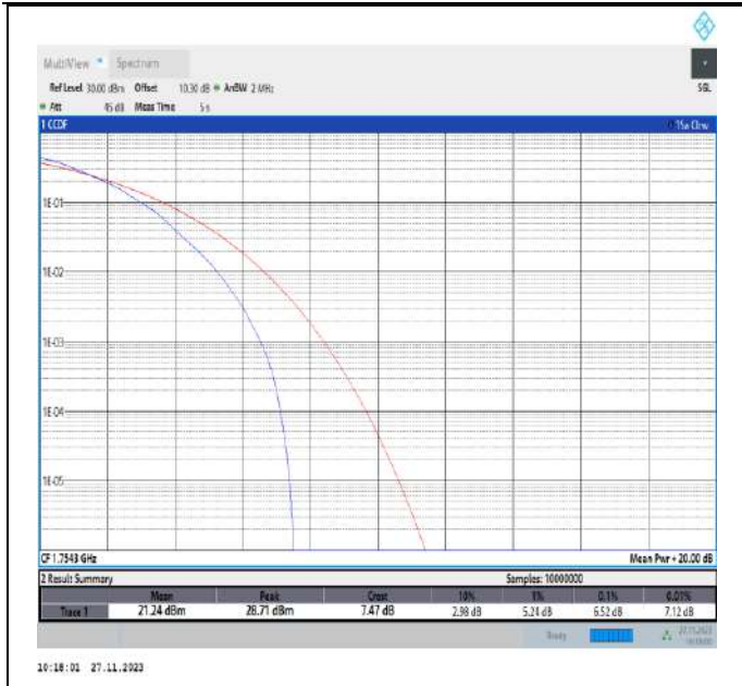
Band4-1.4MHz-64QAM-20393-6RB#0-PASS
