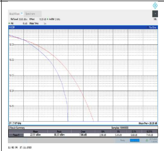
Band66-1.4MHz-16QAM-131979-6RB#0-PASS
