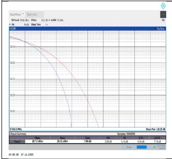
Band5-10MHz-64QAM-20525-50RB#0-PASS
