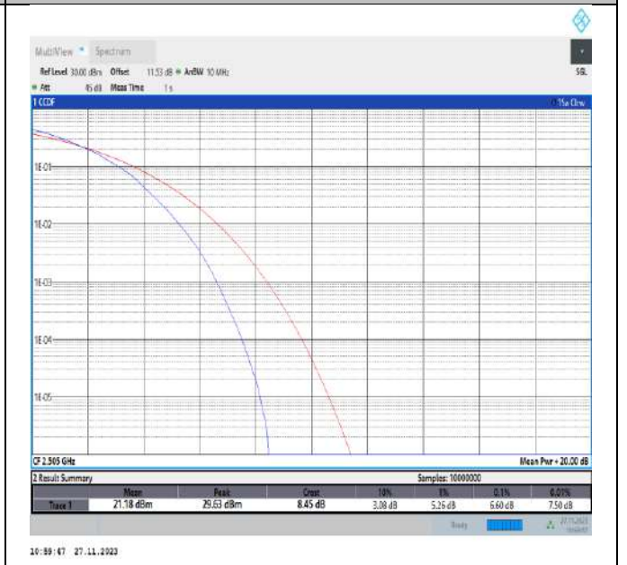
Band7-10MHz-64QAM-20800-50RB#0-PASS
