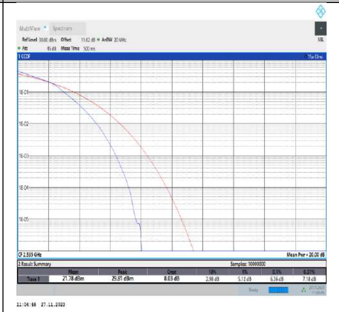
Band7-20MHz-16QAM-21100-100RB#0-PASS
