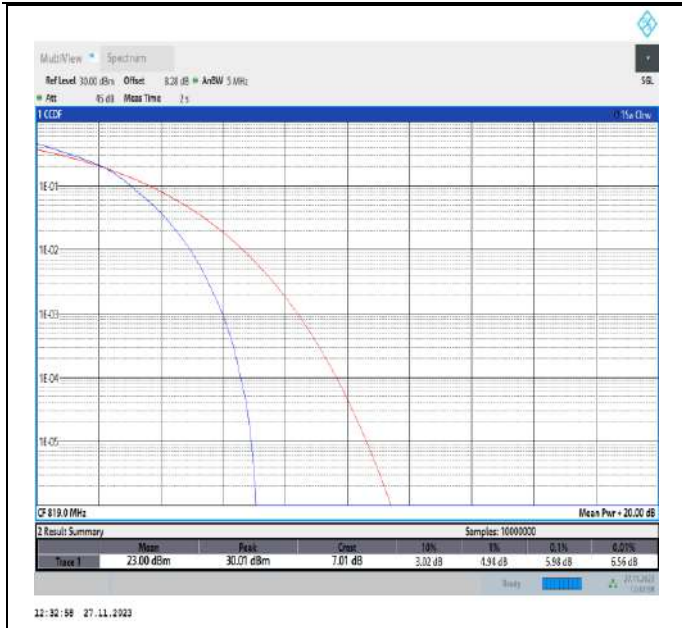
26(814-824)-5MHz-16QAM-26740-25RB#0-PASS
