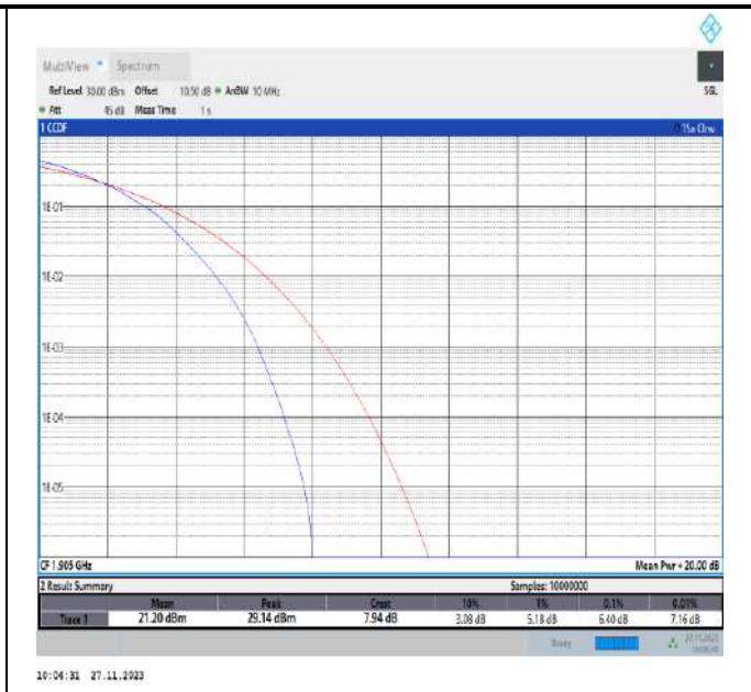
Band2-10MHz-64QAM-19150-50RB#0-PASS
