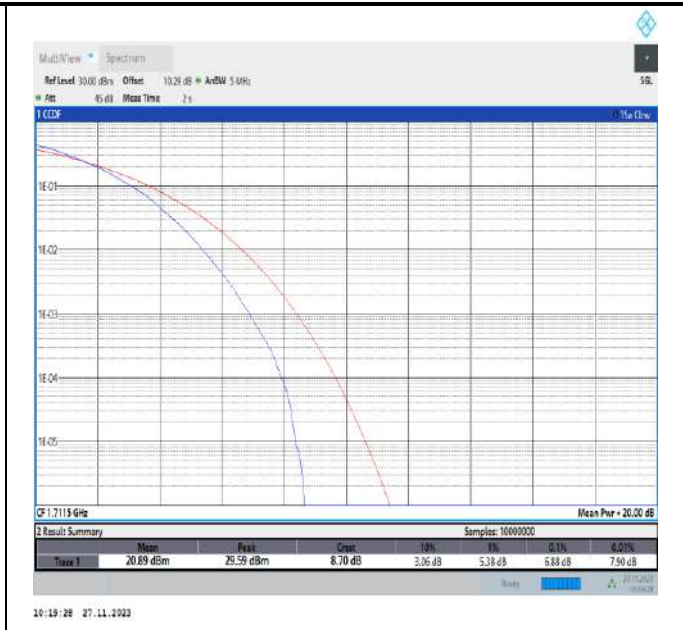
Band4-3MHz-64QAM-19965-15RB#0-PASS
