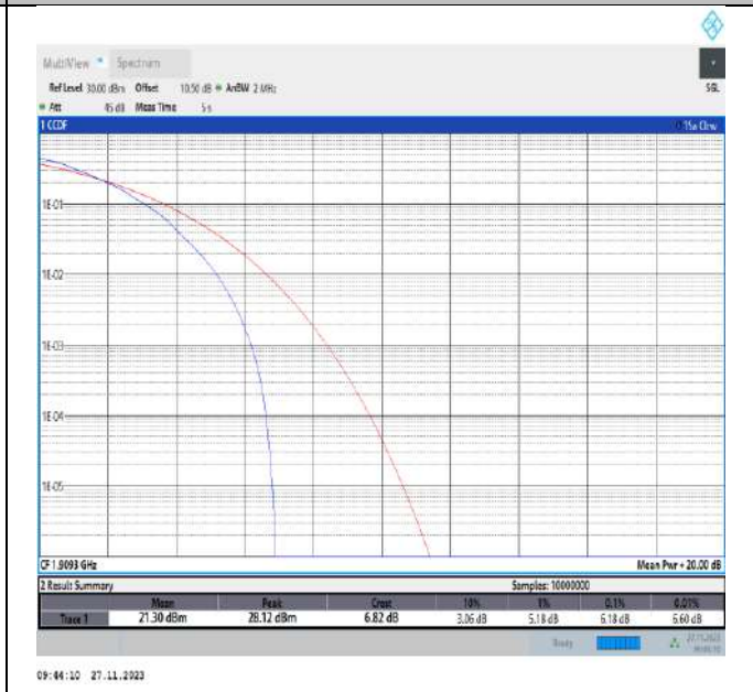
Band2-1.4MHz-64QAM-19193-6RB#0-PASS
