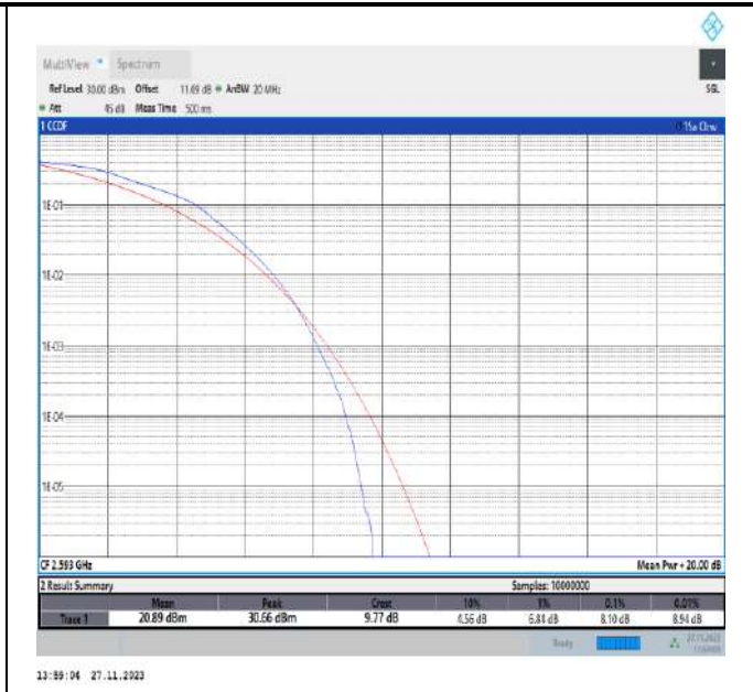
Band41-20MHz-16QAM-40620-100RB#0-PASS
