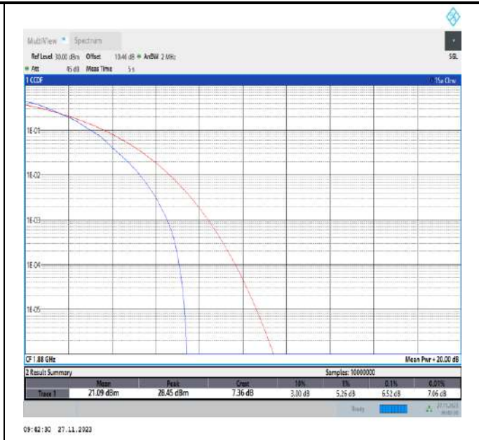
Band2-1.4MHz-64QAM-18900-6RB#0-PASS
