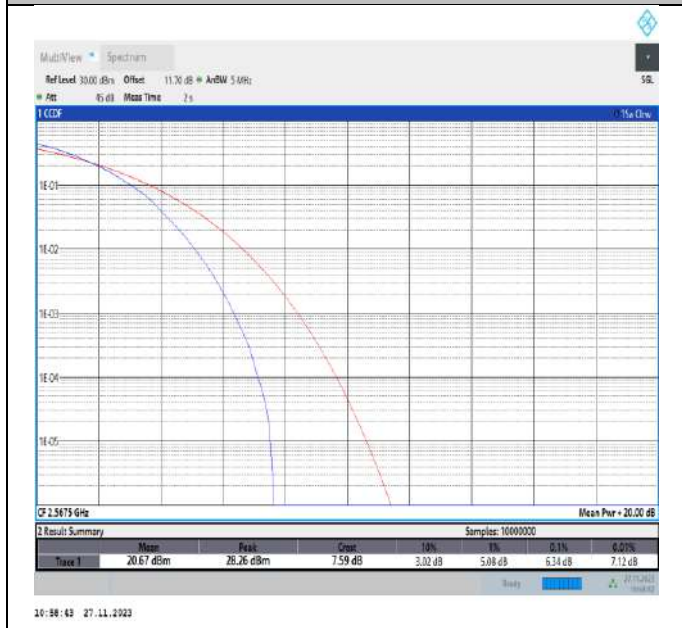
Band7-5MHz-64QAM-21425-25RB#0-PASS
