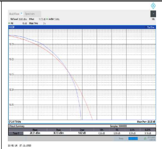
Band38-5MHz-16QAM-38225-25RB#0-PASS
