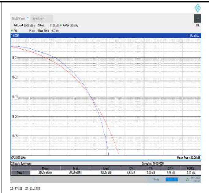
Band38-20MHz-16QAM-38000-100RB#0-PASS
