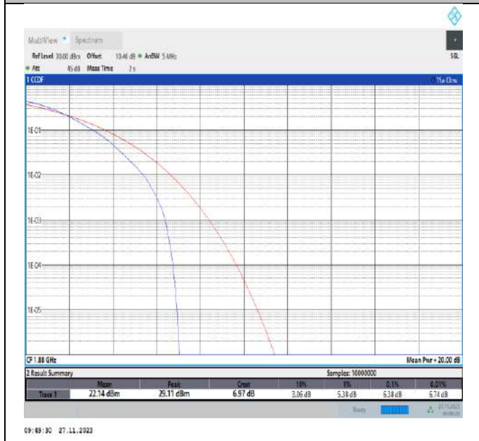
Band2-3MHz-64QAM-18900-1RB#0-PASS
