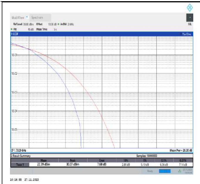
Band4-1.4MHz-16QAM-20175-6RB#0-PASS
