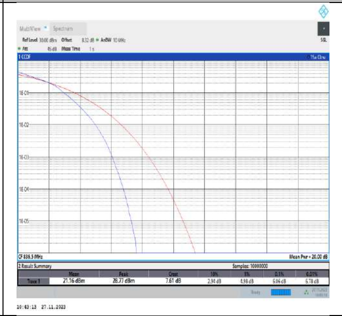
Band5-10MHz-16QAM-20525-50RB#0-PASS
