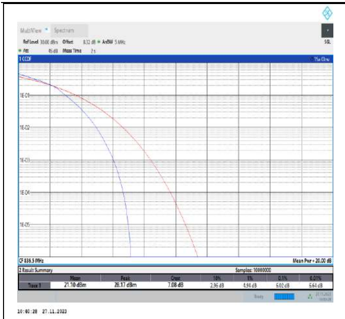
Band5-5MHz-16QAM-20525-25RB#0-PASS
