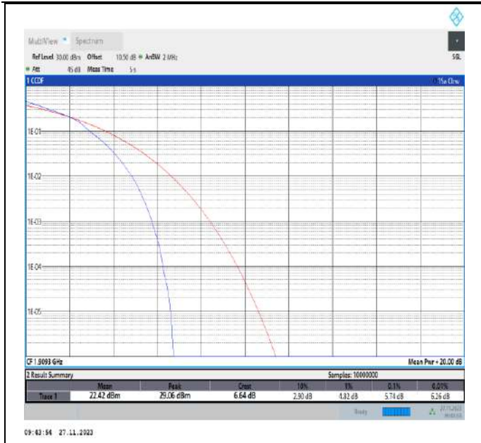
Band2-1.4MHz-16QAM-19193-6RB#0-PASS
