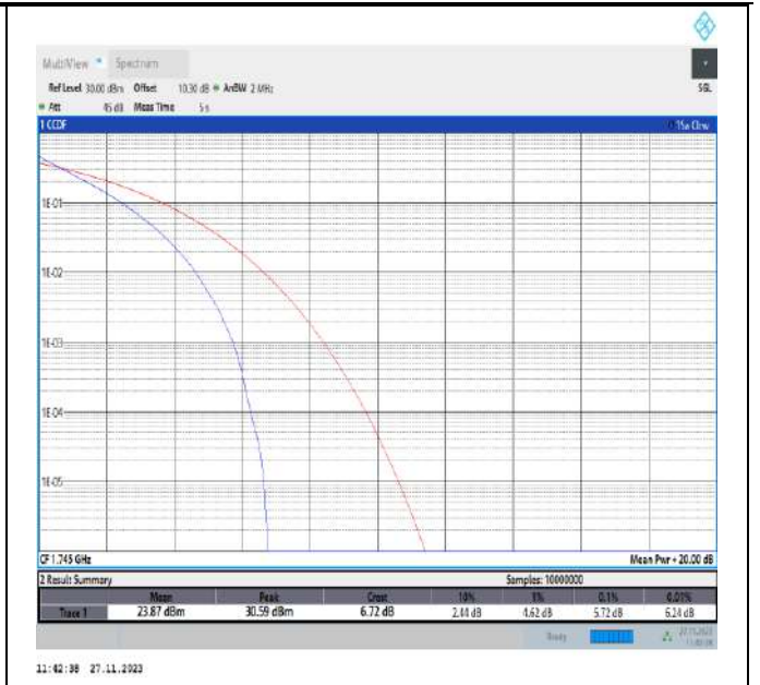
Band66-1.4MHz-QPSK-132322-6RB#0-PASS
