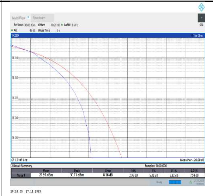
Band4-1.4MHz-16QAM-19957-6RB#0-PASS
