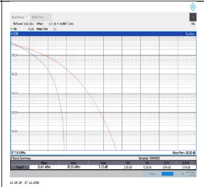
Band12-3MHz-QPSK-23165-15RB#0-PASS
