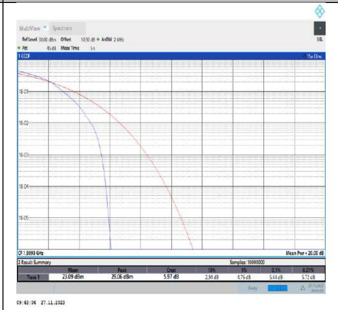
Band2-1.4MHz-16QAM-19193-1RB#0-PASS
