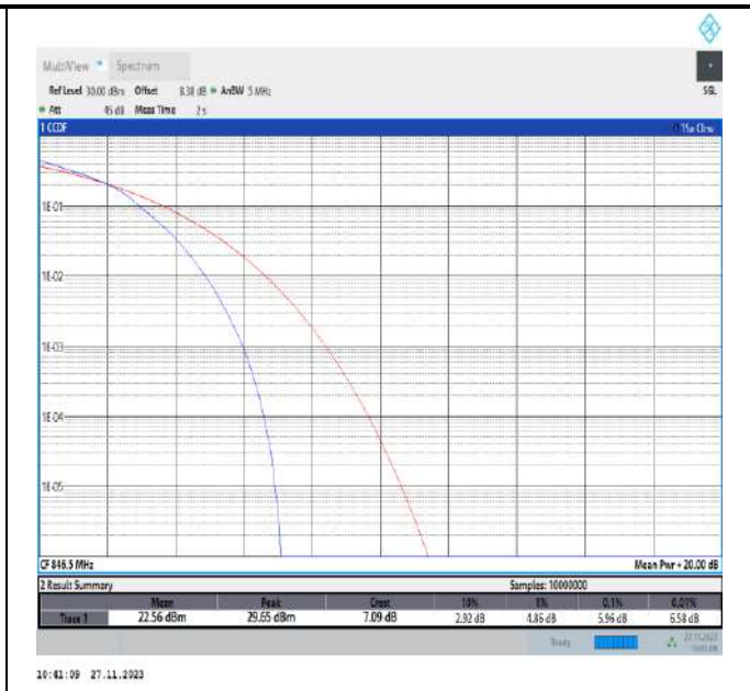
Band5-5MHz-16QAM-20625-25RB#0-PASS
