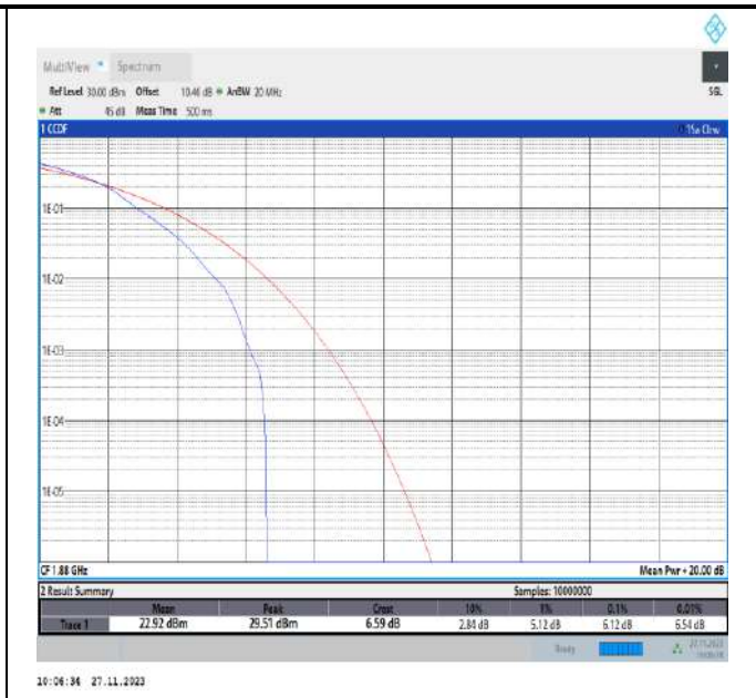
Band2-15MHz-16QAM-18900-1RB#0-PASS
