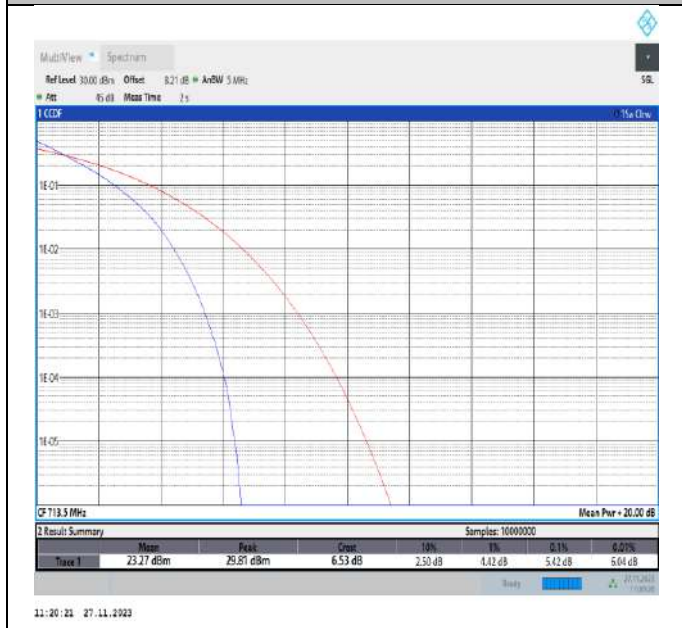
Band12-5MHz-QPSK-23155-25RB#0-PASS
