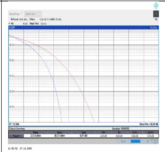
Band66-20MHz-QPSK-132072-100RB#0-PASS
