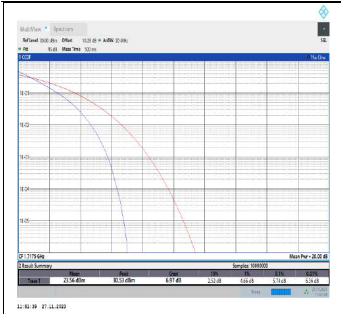
Band66-15MHz-QPSK-132047-75RB#0-PASS
