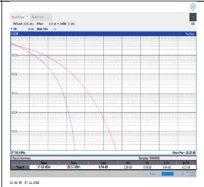
Band12-10MHz-QPSK-23060-50RB#0-PASS
