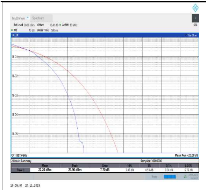
Band2-15MHz-16QAM-18675-75RB#0-PASS
