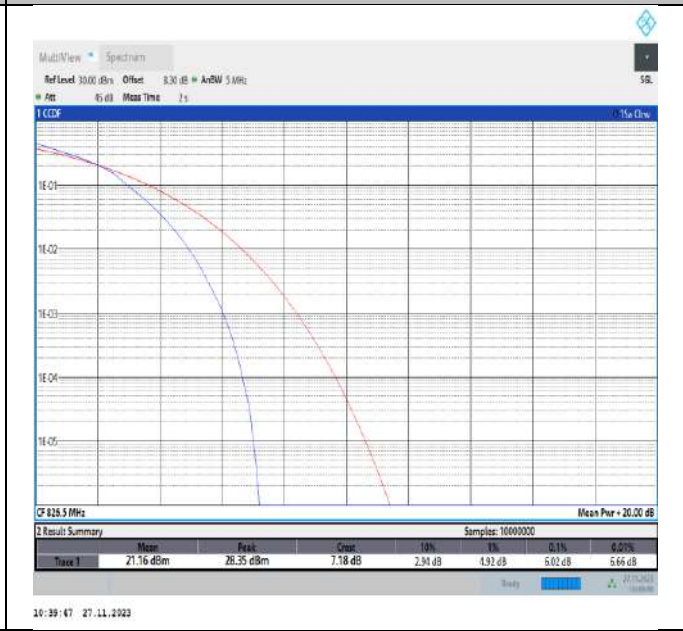
Band5-5MHz-16QAM-20425-25RB#0-PASS
