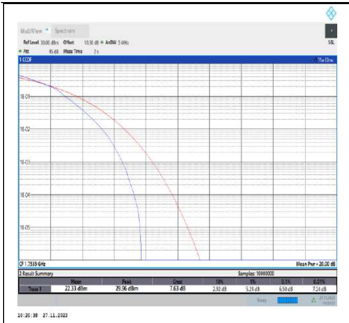
Band4-3MHz-16QAM-20385-15RB#0-PASS
