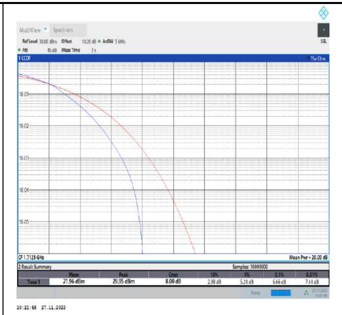
Band4-5MHz-16QAM-19975-25RB#0-PASS
