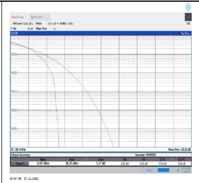
Band2-3MHz-16QAM-18615-1RB#0-PASS
