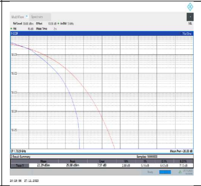
Band4-3MHz-16QAM-20175-15RB#0-PASS
