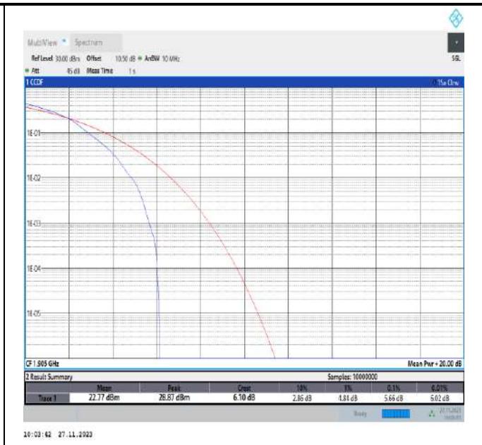
Band2-10MHz-16QAM-19150-1RB#0-PASS
