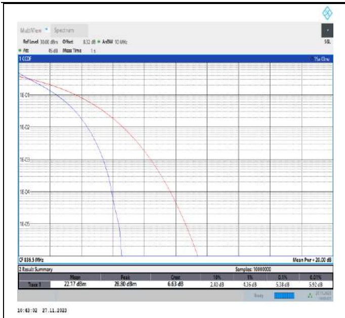
Band5-10MHz-QPSK-20525-50RB#0-PASS
