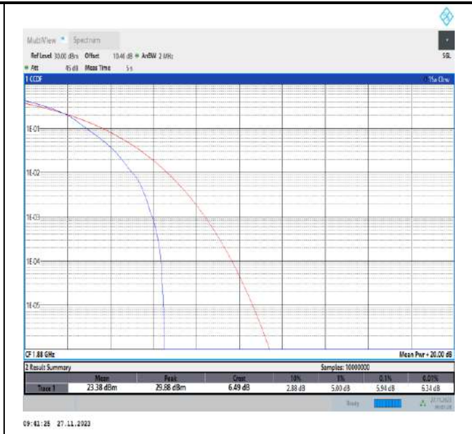
Band2-1.4MHz-16QAM-18900-1RB#0-PASS
