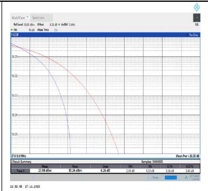
26(814-824)-5MHz-QPSK-26740-25RB#0-PASS
