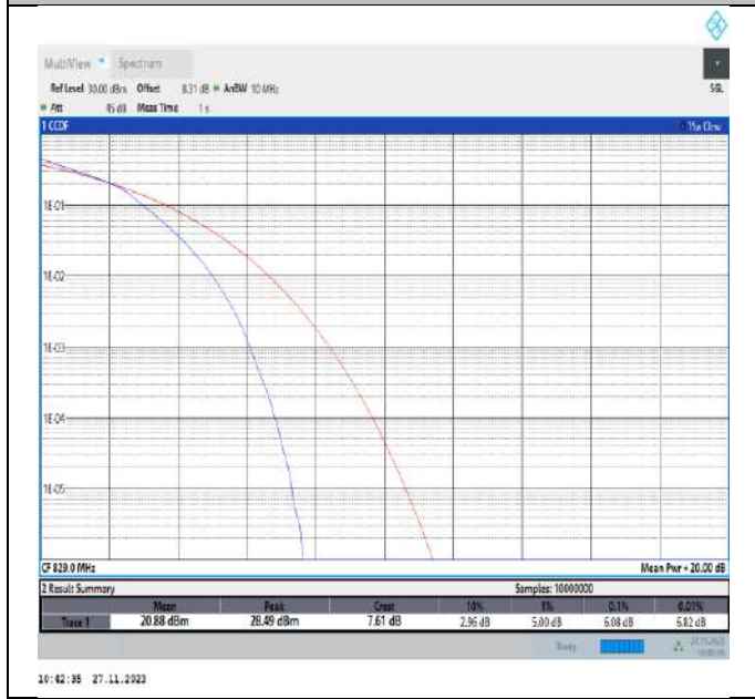
Band5-10MHz-16QAM-20450-50RB#0-PASS
