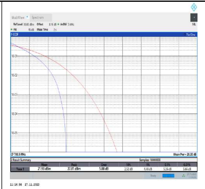
Band12-3MHz-QPSK-23025-15RB#0-PASS
