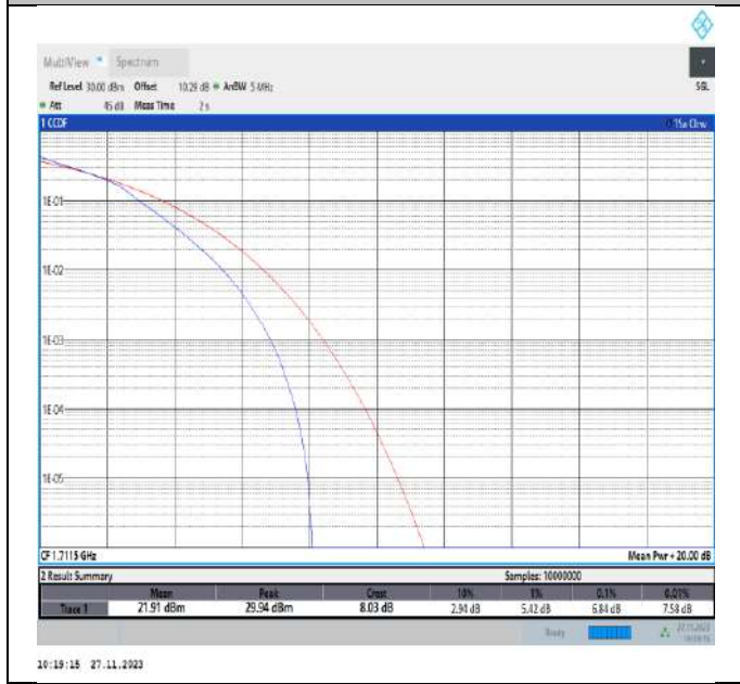
Band4-3MHz-16QAM-19965-15RB#0-PASS
