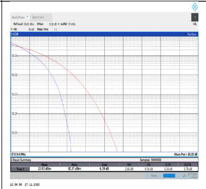
26(814-824)-10MHz-QPSK-26740-50RB#0-PASS
