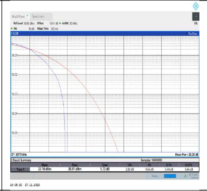
Band2-15MHz-16QAM-18675-1RB#0-PASS
