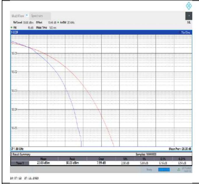
Band2-15MHz-16QAM-18900-75RB#0-PASS
