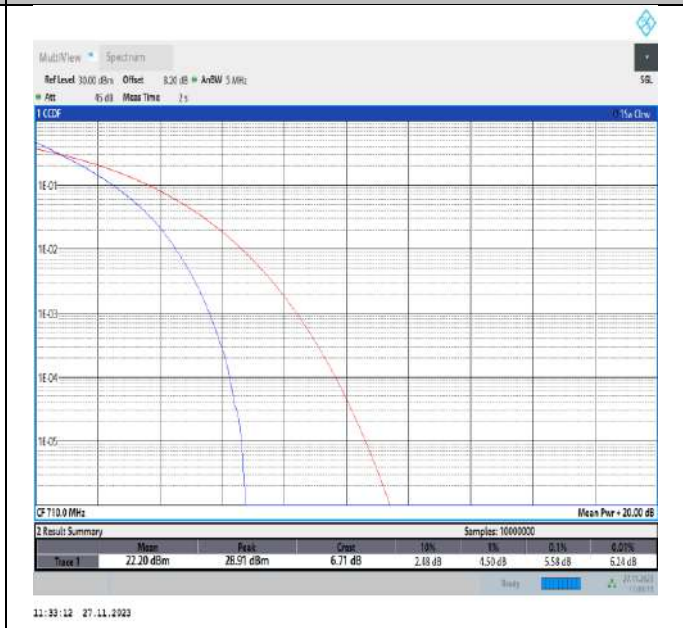
Band17-5MHz-QPSK-23790-25RB#0-PASS
