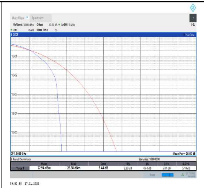
Band2-3MHz-16QAM-19185-1RB#0-PASS
