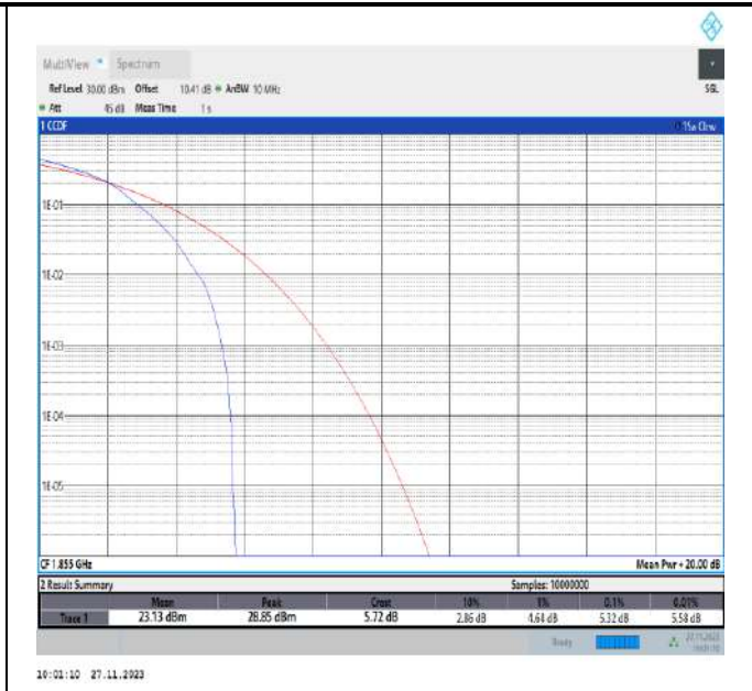
Band2-10MHz-16QAM-18650-1RB#0-PASS
