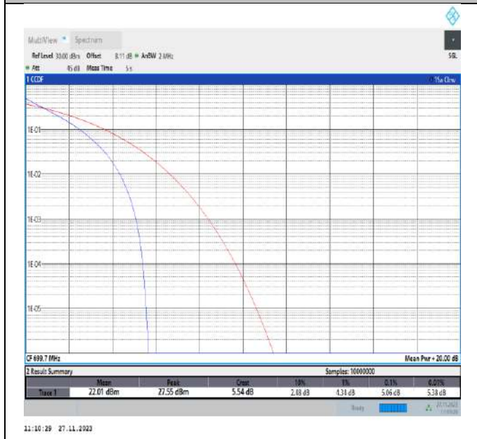
Band12-1.4MHz-QPSK-23017-6RB#0-PASS
