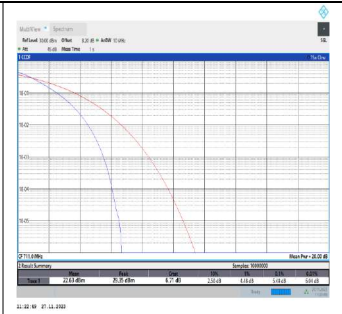
Band12-10MHz-QPSK-23130-50RB#0-PASS
