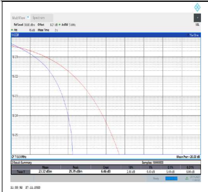
Band17-5MHz-QPSK-23825-25RB#0-PASS
