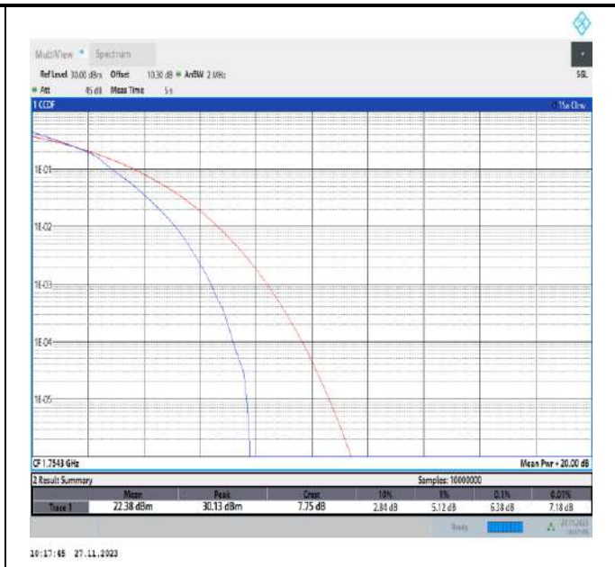
Band4-1.4MHz-16QAM-20393-6RB#0-PASS
