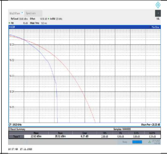
Band2-15MHz-16QAM-19125-1RB#0-PASS
