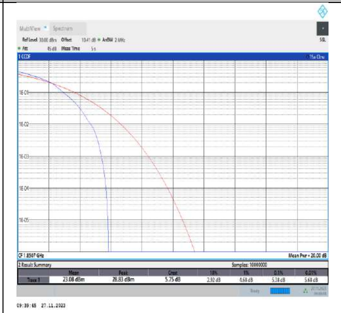
Band2-1.4MHz-16QAM-18607-1RB#0-PASS
