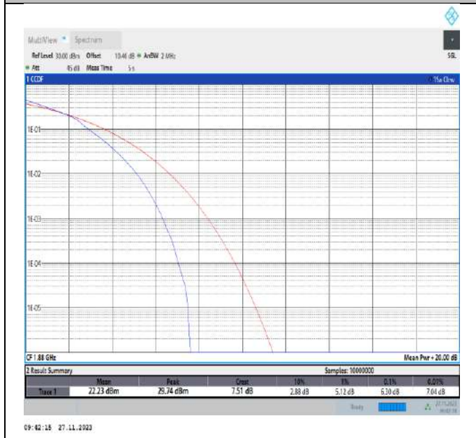
Band2-1.4MHz-16QAM-18900-6RB#0-PASS
