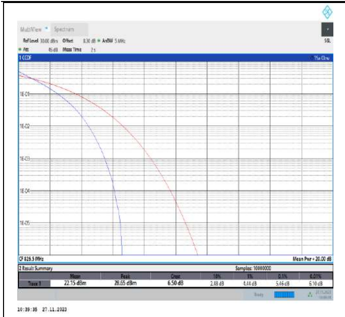
Band5-5MHz-QPSK-20425-25RB#0-PASS
