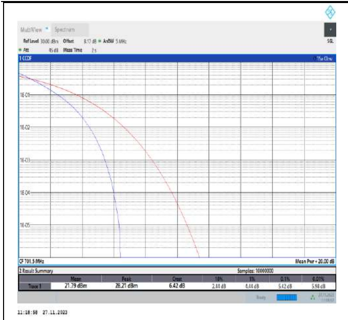
Band12-5MHz-QPSK-23035-25RB#0-PASS
