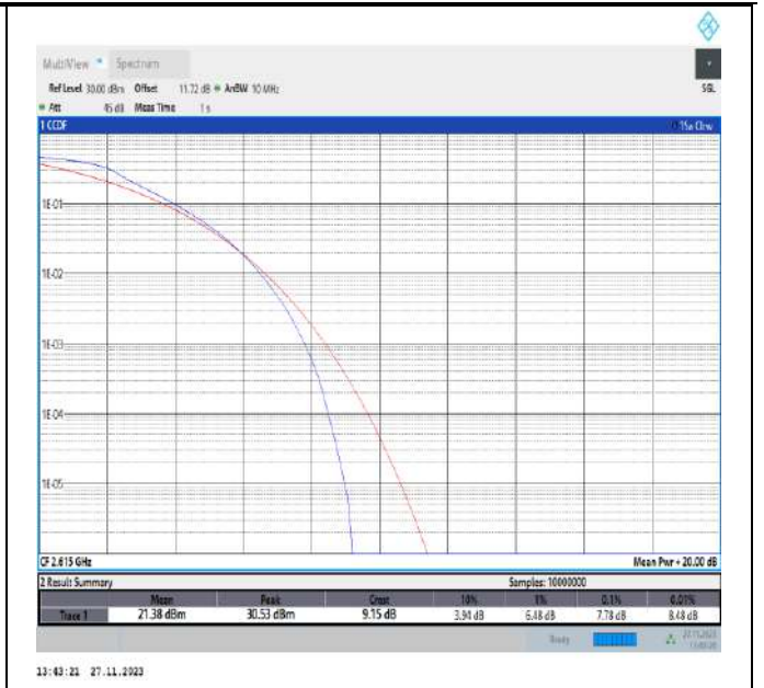
Band38-10MHz-QPSK-38200-50RB#0-PASS
