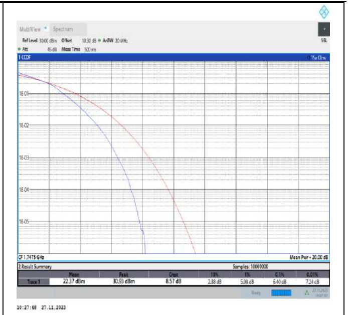
Band4-15MHz-16QAM-20325-75RB#0-PASS
