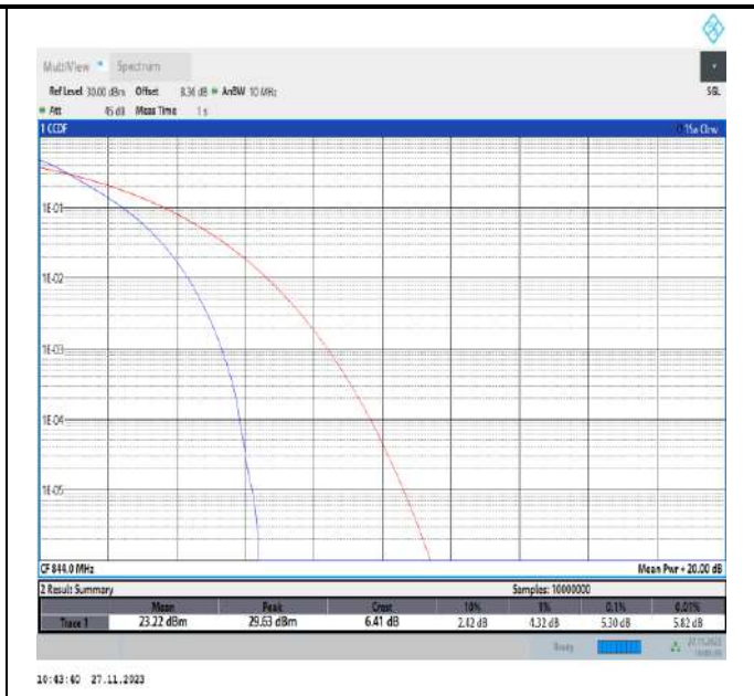
Band5-10MHz-QPSK-20600-50RB#0-PASS
