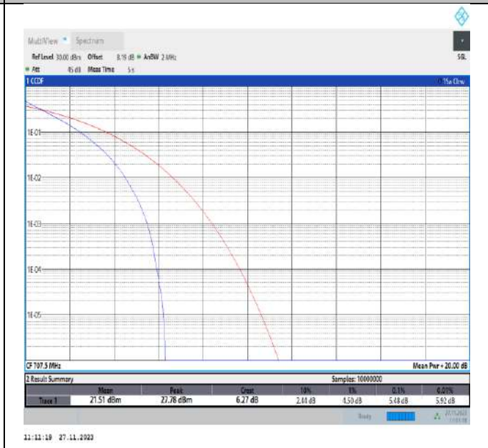
Band12-1.4MHz-QPSK-23095-6RB#0-PASS
