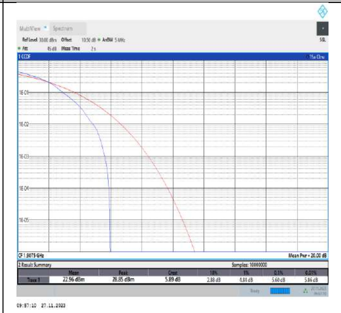
Band2-5MHz-16QAM-19175-1RB#0-PASS
