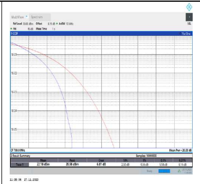
Band17-10MHz-QPSK-23780-50RB#0-PASS
