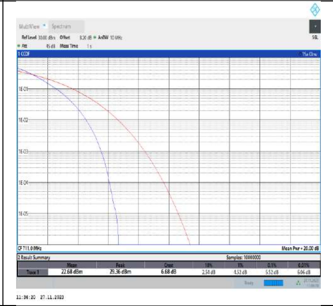
Band17-10MHz-QPSK-23800-50RB#0-PASS
