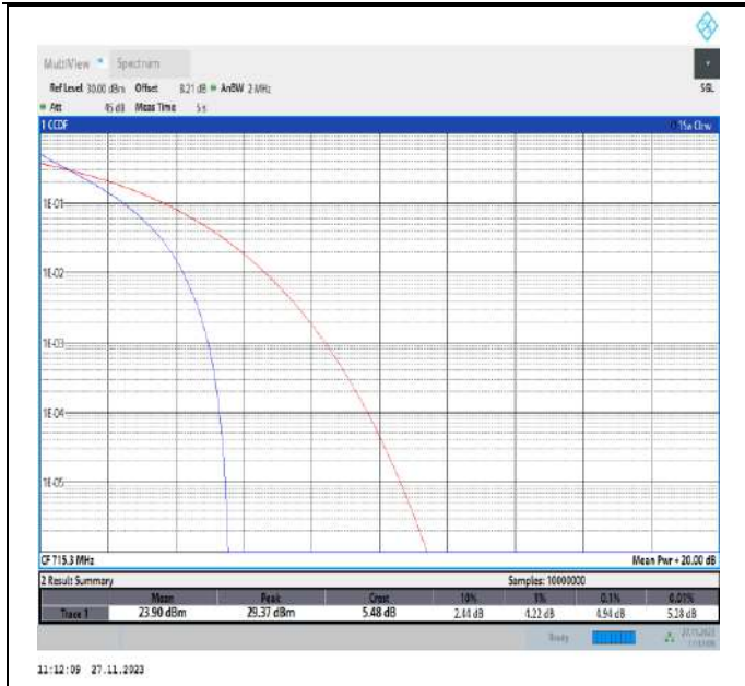
Band12-1.4MHz-QPSK-23173-6RB#0-PASS
