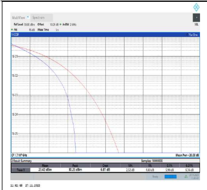
Band66-1.4MHz-QPSK-131979-6RB#0-PASS
