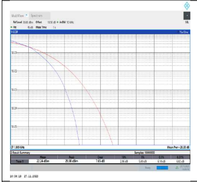
Band2-10MHz-16QAM-19150-50RB#0-PASS
