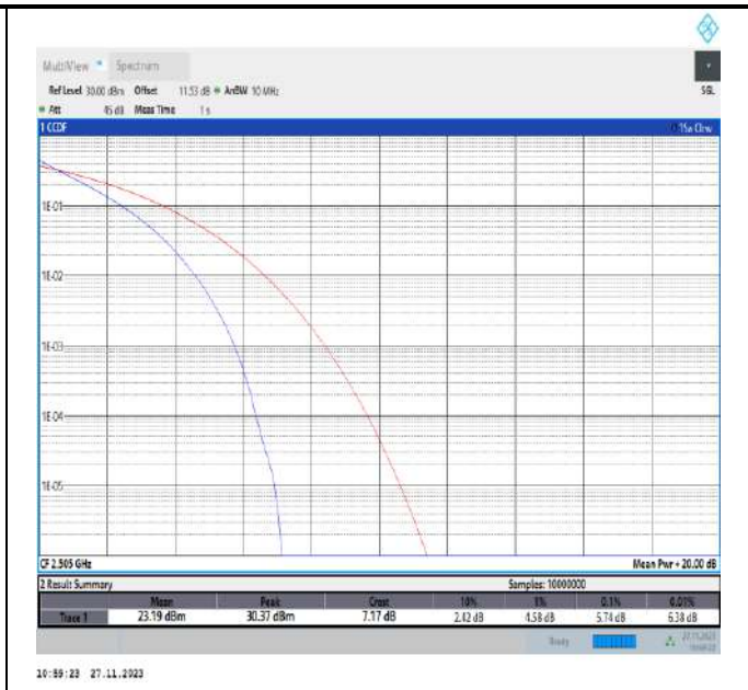
Band7-10MHz-QPSK-20800-50RB#0-PASS
