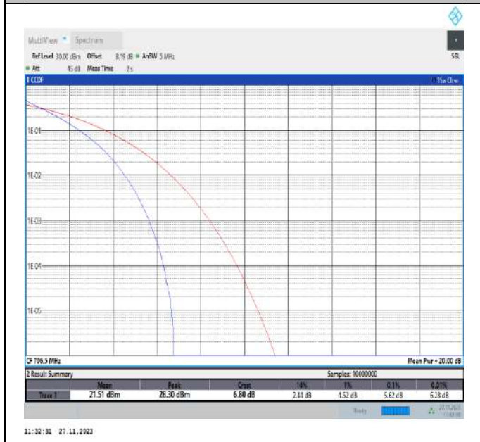
Band17-5MHz-QPSK-23755-25RB#0-PASS
