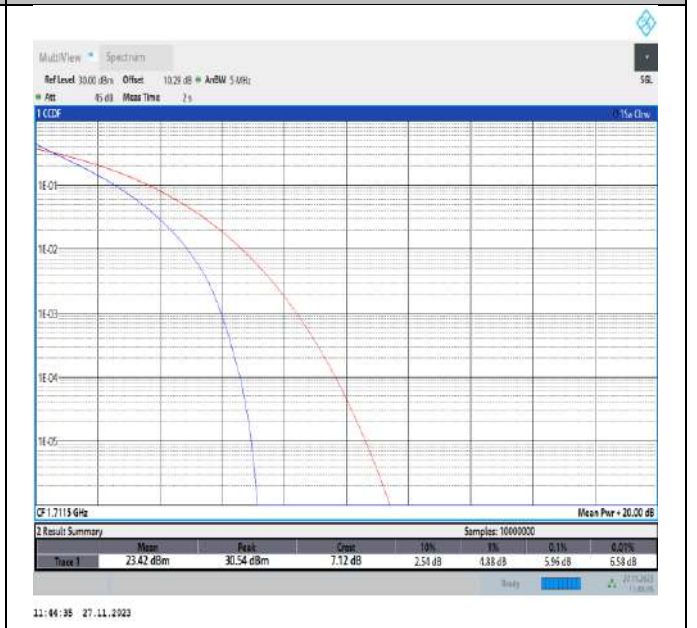
Band66-3MHz-QPSK-131987-15RB#0-PASS
