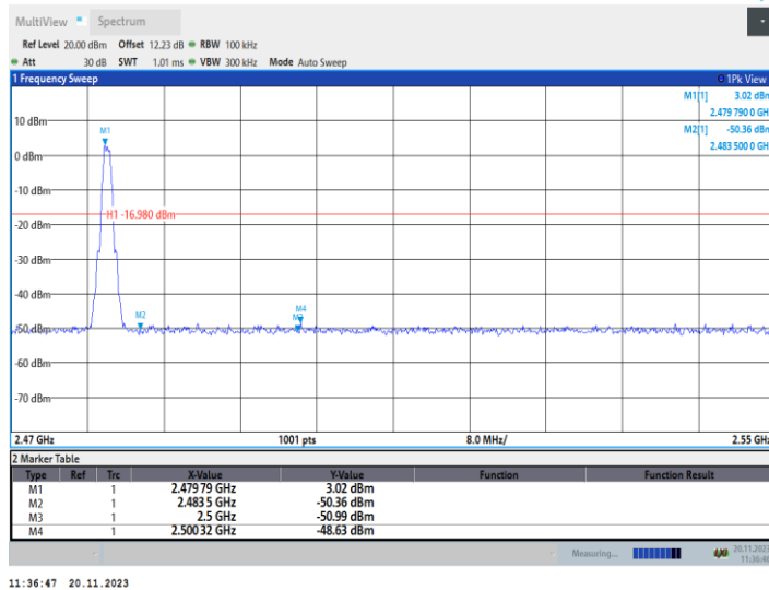
BLE_500K_Ant1_High_2480
