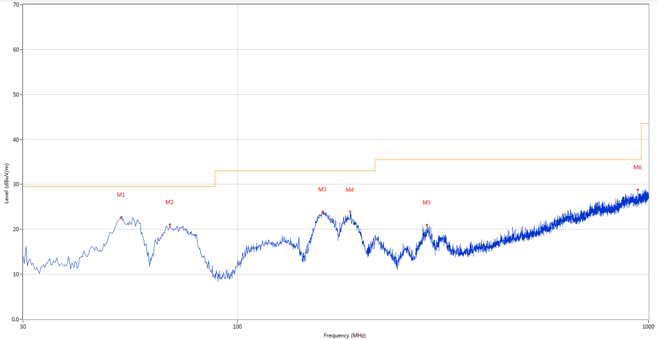
30 MHz to 1 GHz, Test Antenna Vertical, EUT X axis
