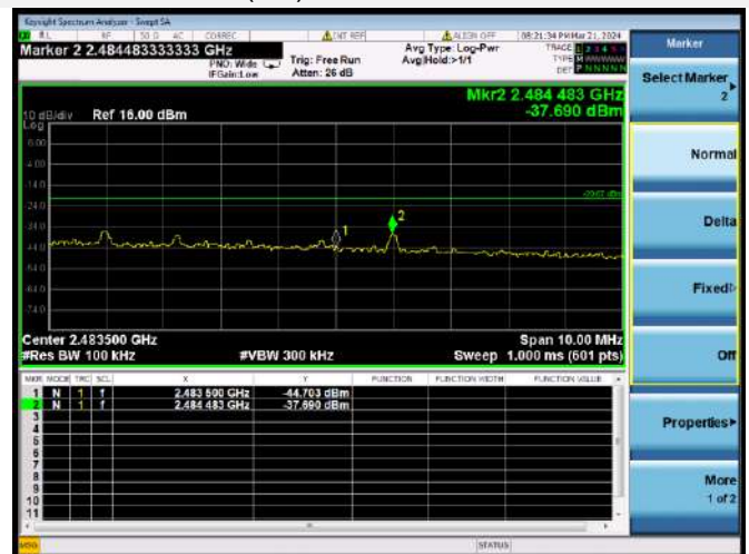
802.11ax-40 MHz(SU) CHANNEL 8, BAND EDGE
