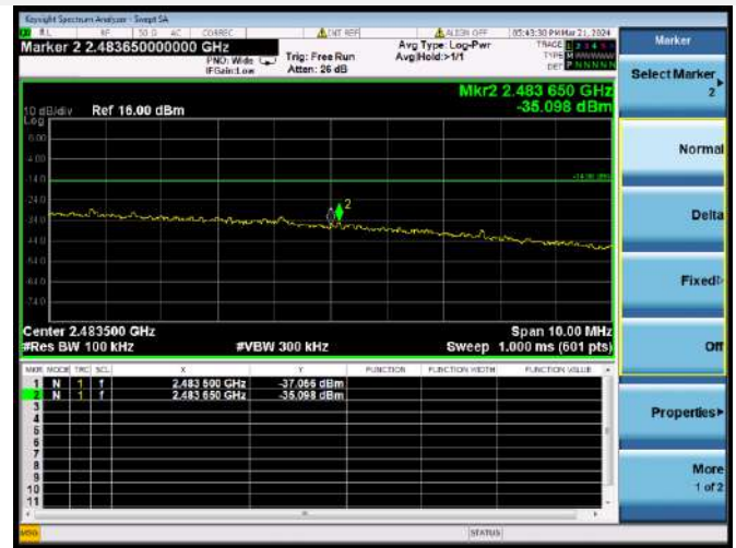
802.11ax-20 MHz(SU) CHANNEL 11, BAND EDGE
