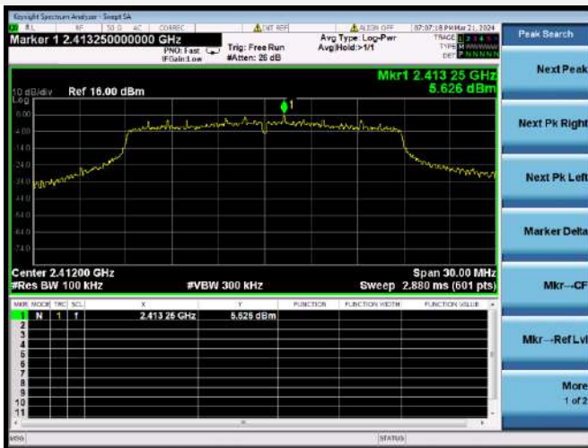
VHT-20 MHz CHANNEL 1, CARRIER LEVEL
