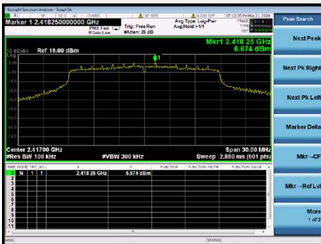
VHT-20 MHz CHANNEL 2, CARRIER LEVEL
