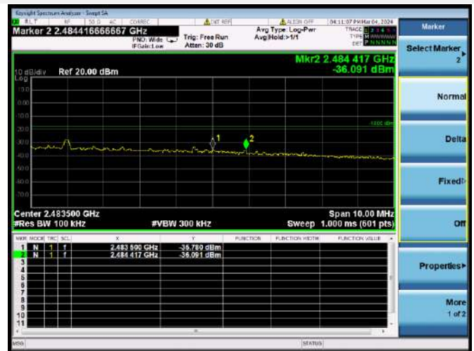
802.11ax-40 MHz(SU) CHANNEL 7, BAND EDGE
