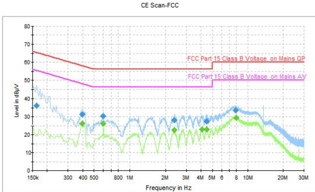
Figure A-5 Conducted Emission (Traffic)
