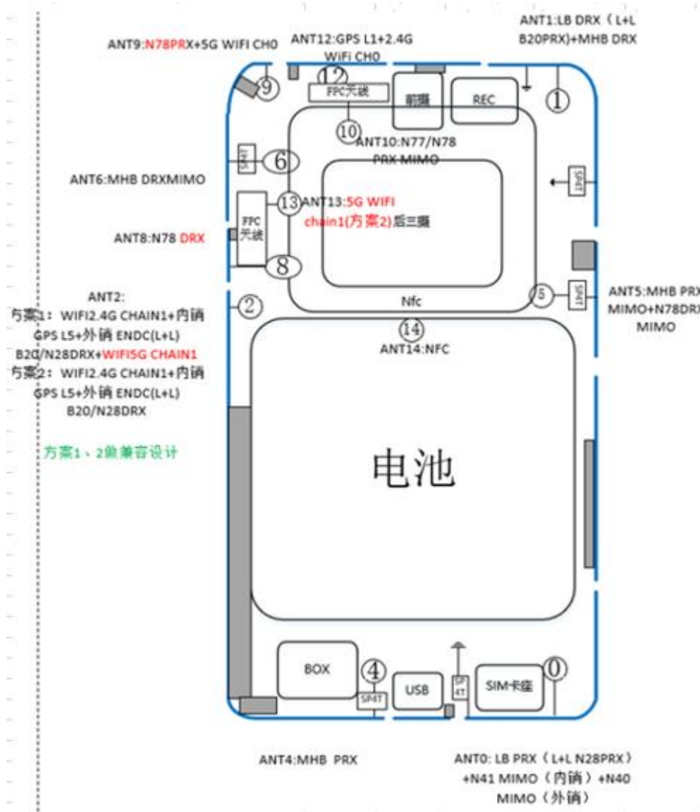
Fig 1 Antenna location & dimension
