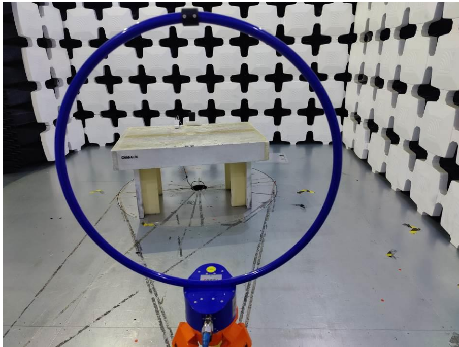
1. Radiated Emissions (Part 15C&Part 15E, 9kHz-30MHz)
