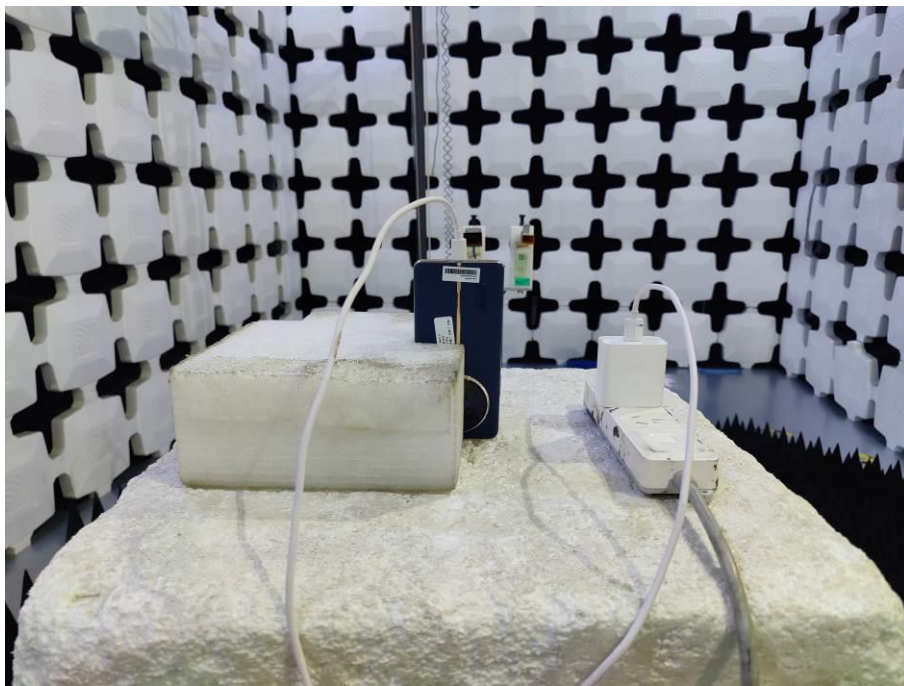
4. Radiated Emissions (Part 15C&Part 15E, 18GHz -26.5GHz)
