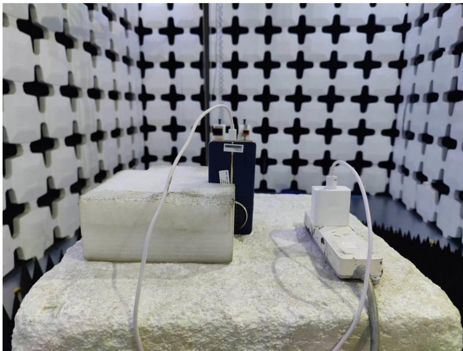
8. Radiated Emissions (Part 22/24/27/90, 26.5GHz-40GHz)
