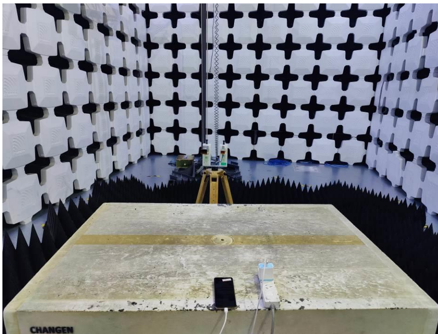
8. Radiated Emissions (Part 15B, Camera/Video Player/GSM receiver/WCDMA receiver/LTE receiver, 26.5GHz-40GHz)
