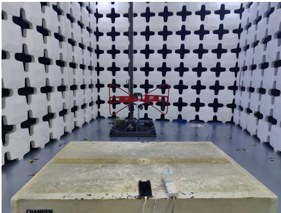
2. Radiated Emissions (Part 15C&Part 15E, 30MHz-1GHz)
