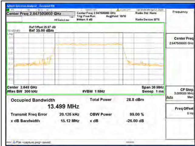
Band41(2535-2655) / 15MHz / QPSK / High CH
