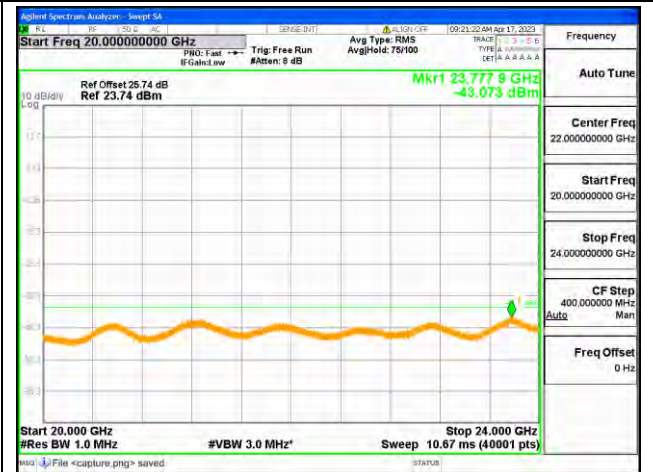
Band40-2-20G-24G / 5MHz / Mid CH / QPSK
