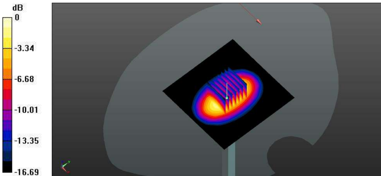
0 dB = 4.08 W/kg
