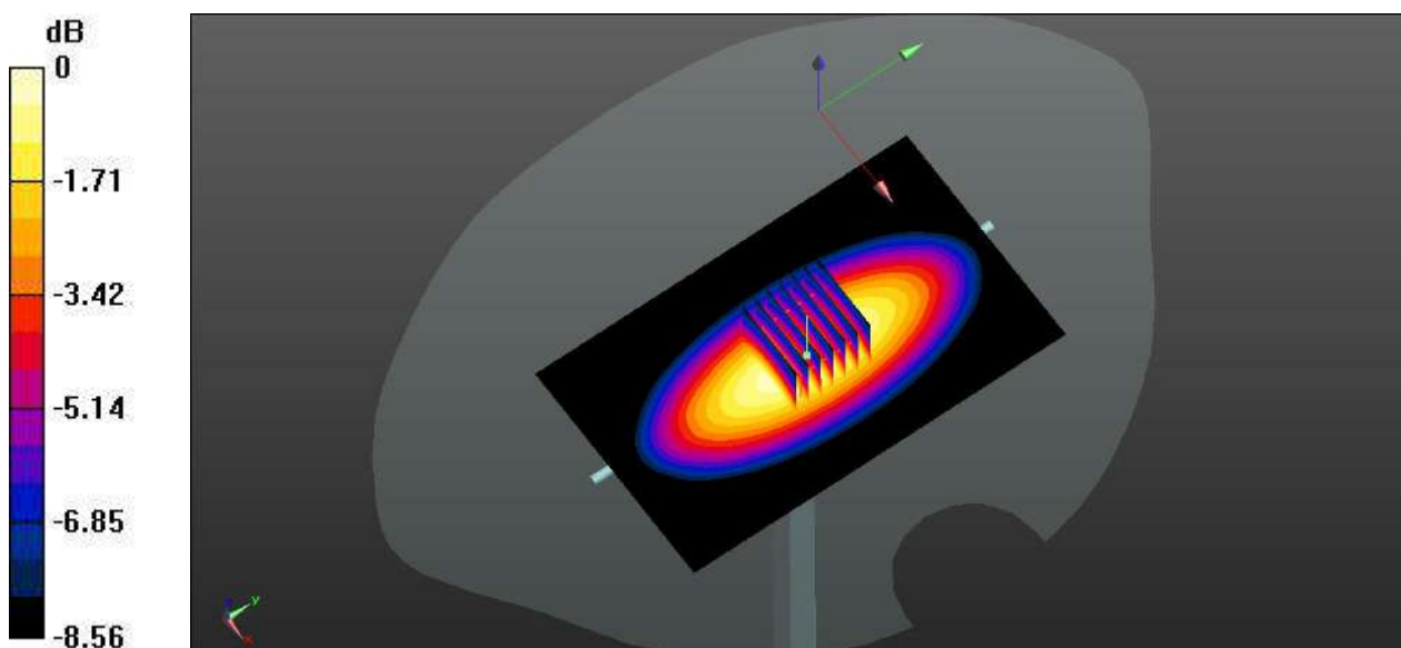
0 dB = 0.956 W/kg
