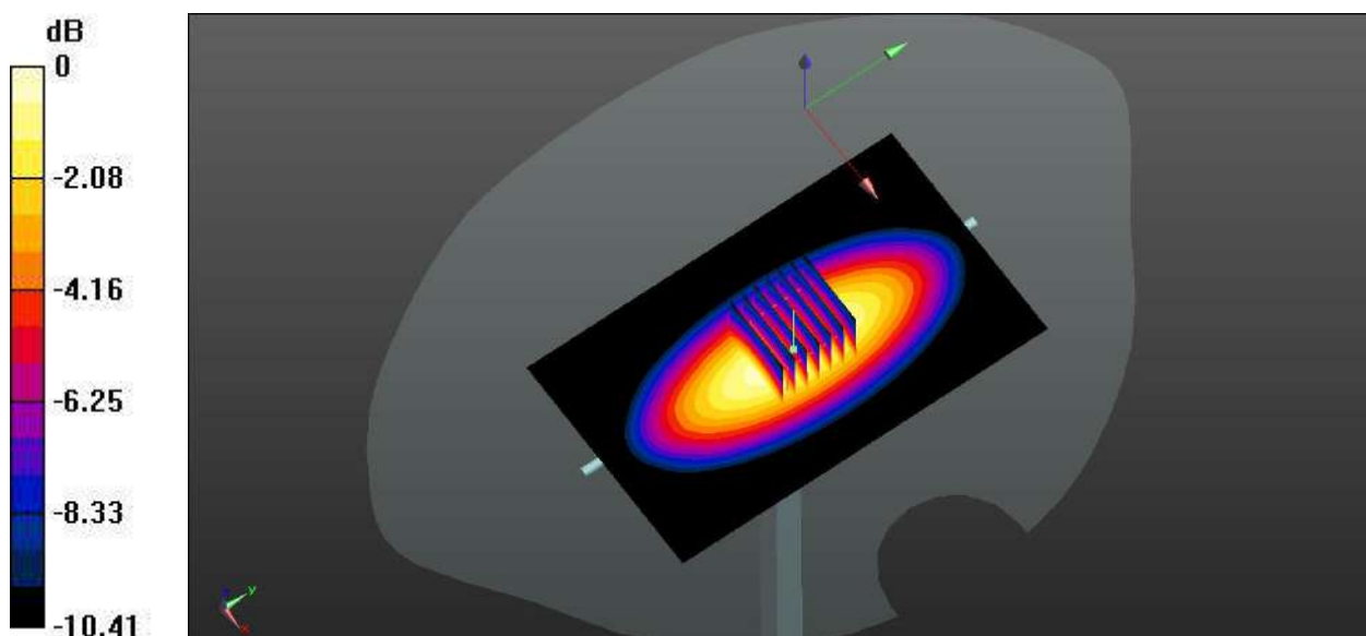
0 dB = 1.18 W/kg
