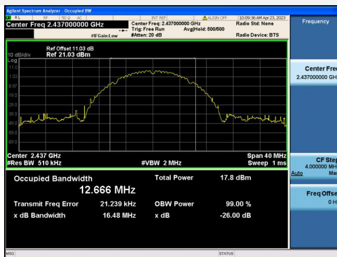
802.11b CHANNEL 6
