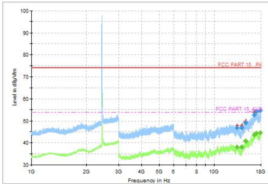
Fig.30 Radiated Spurious Emission (CH19, 1GHz ~18GHz), LE 2M
