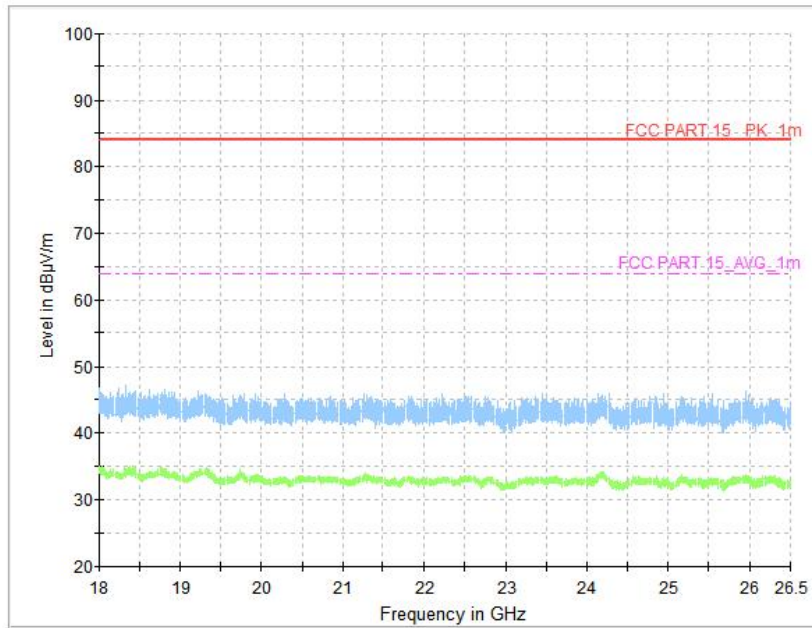
Fig.36 Radiated Spurious Emission (All Channels, 18GHz-26.5 GHz)
