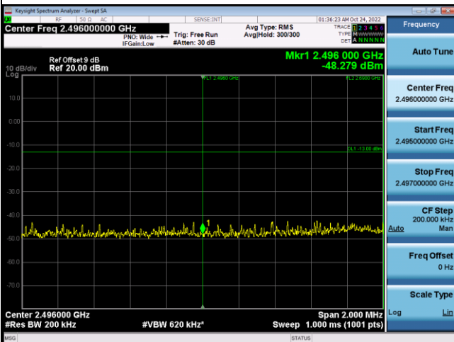
1RB#0+1RB#49_Low Range
