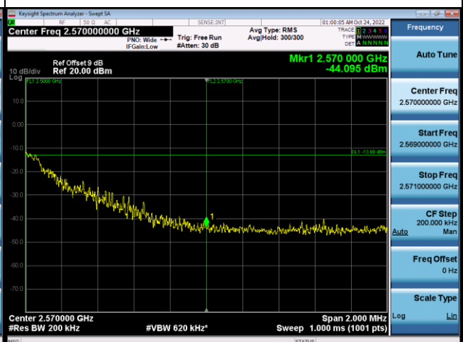
100RB#0+75RB#0_High Range
