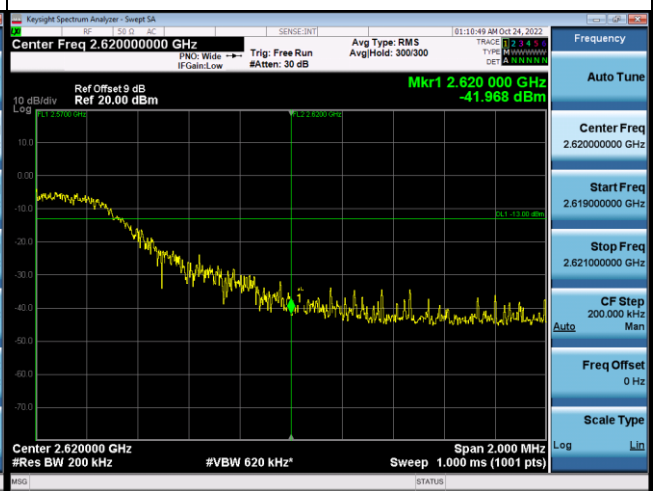
75RB#0+75RB#0_High Range
