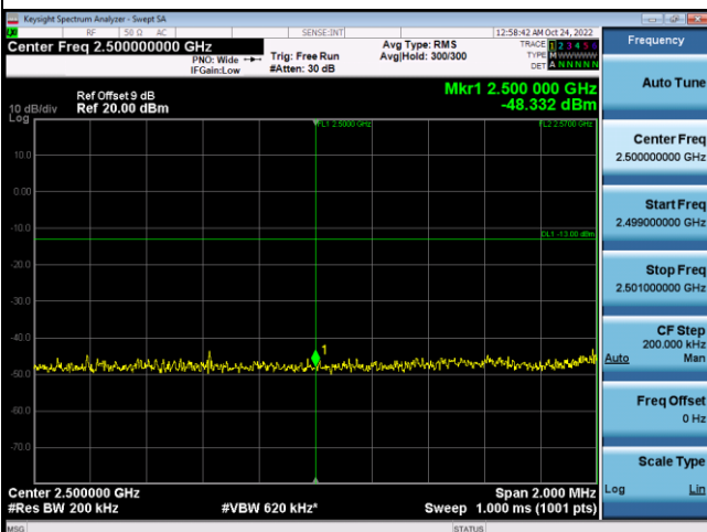
100RB#0+75RB#0_Low Range
