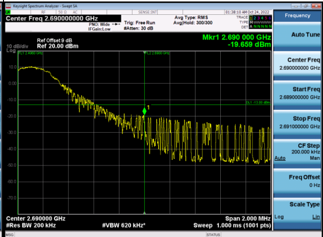
75RB#0+50RB#0_High Range
