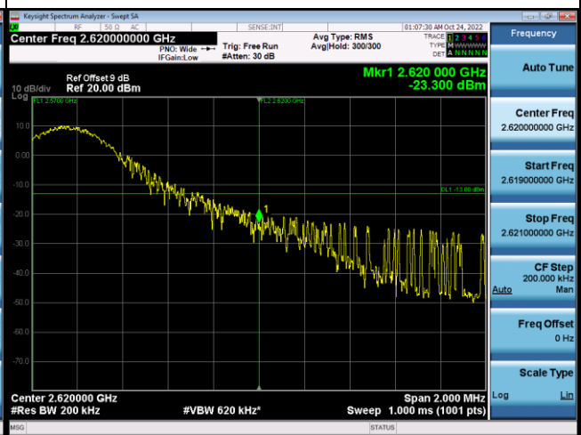
1RB#74+1RB#0_High Range
