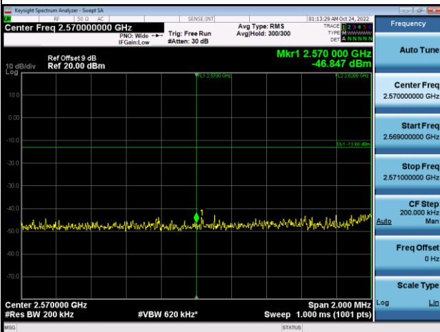
100RB#0+100RB#0_Low Range
