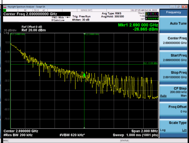
1RB#0+1RB#99_High Range
