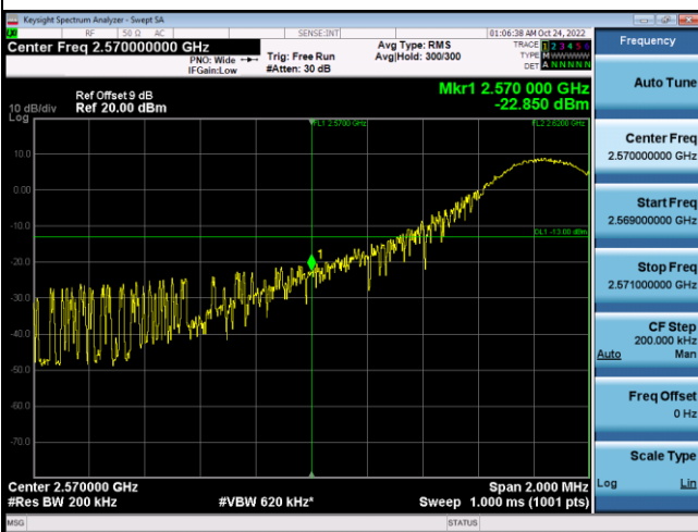
1RB#74+1RB#0_Low Range
