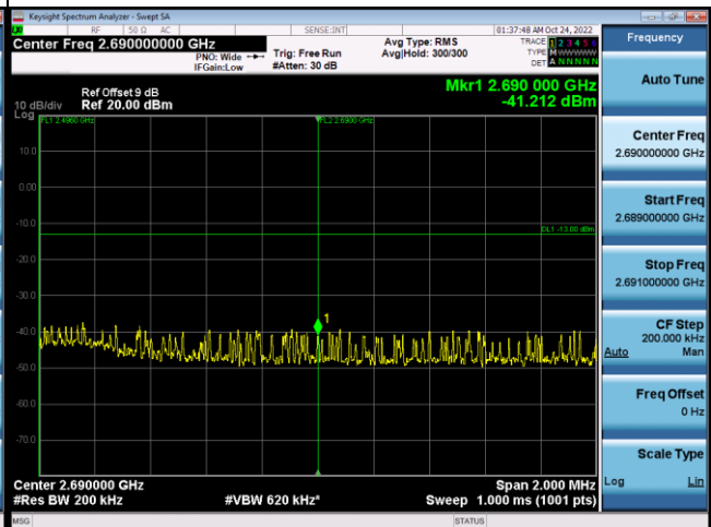
1RB#0+1RB#49_High Range
