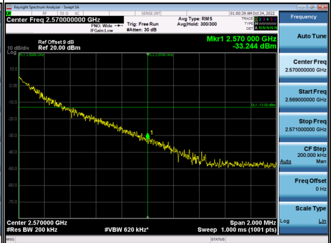
1RB#99+1RB#0_High Range
