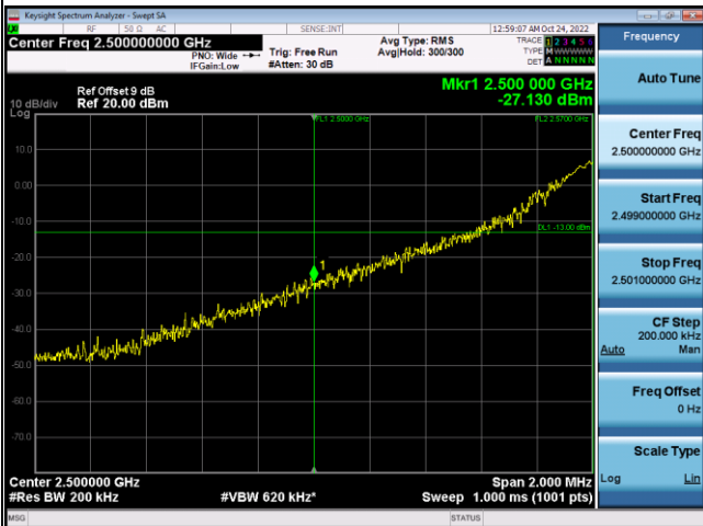
1RB#99+1RB#0_Low Range
