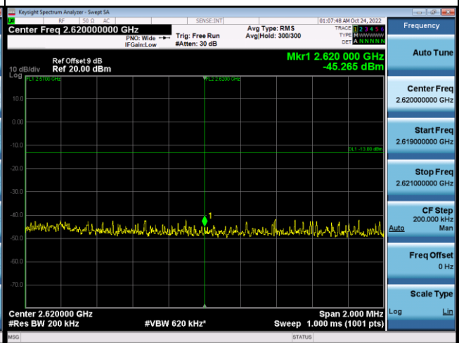
75RB#0+75RB#0_High Range
