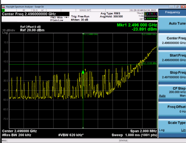
1RB#0+1RB#99_Low Range
