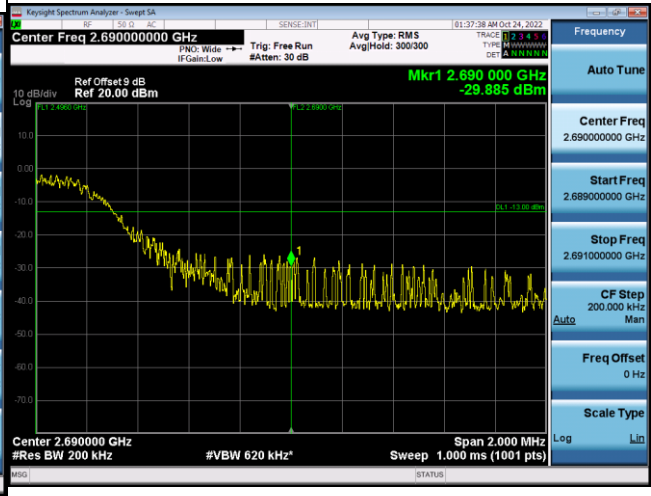
75RB#0+50RB#0_High Range
