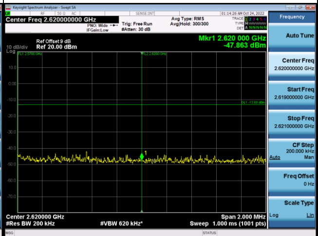
100RB#0+100RB#0_High Range
