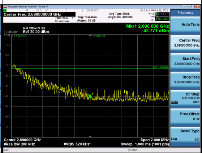
25RB#0+100RB#0_High Range
