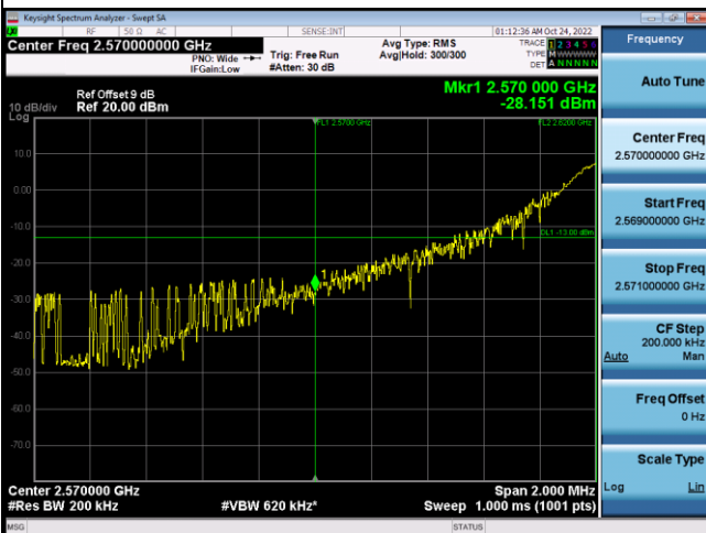
1RB#99+1RB#0_Low Range
