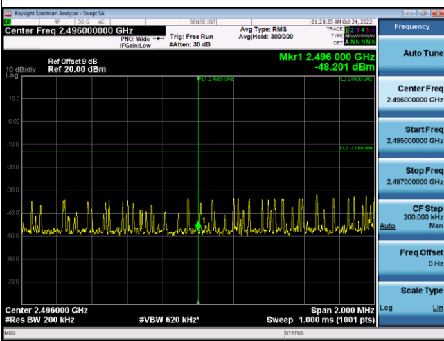
25RB#0+100RB#0_Low Range
