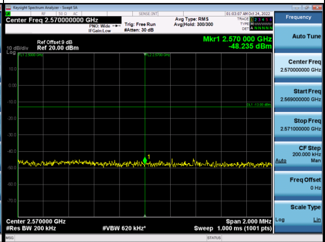
100RB#0+100RB#0_High Range
