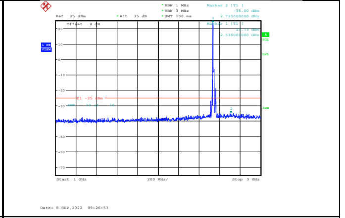
Band41-15MHz-16QAM-40115-1RB#0-Range2:1000~3000MHz
