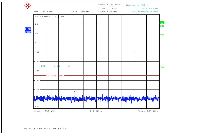
Band13-5MHz-64QAM-23255-1RB#0-Range4:793~805MHz
