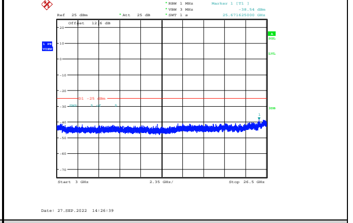
Band41-10MHz-64QAM-40090-1RB#0-Range3:3000~26500MHz
