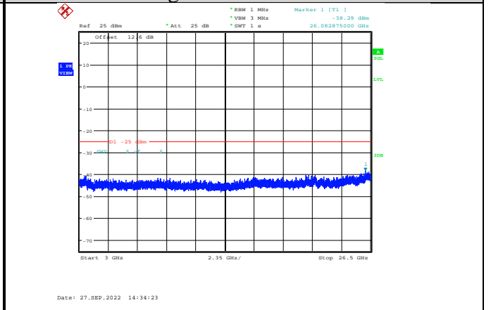
Band38-15MHz-16QAM-37825-1RB#0-Range3:3000~26500MHz
