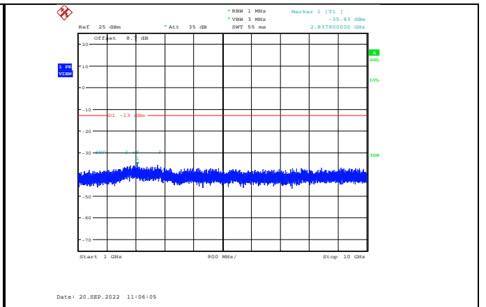
Band12-5MHz-64QAM-23095-1RB#0- Range2:1000~10000MHz
