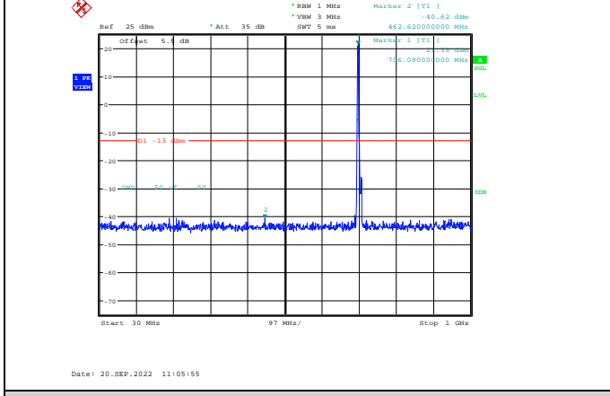
Band12-5MHz-64QAM-23095-1RB#0- Range1:30~1000MHz
