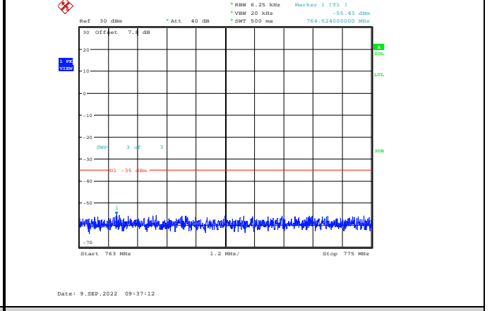
Band13-5MHz-64QAM-23255-1RB#0-Range3:763~775MHz
