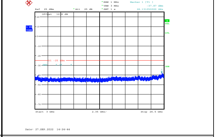
Band41-5MHz-16QAM-41215-1RB#0-Range3:3000~26500MHz
