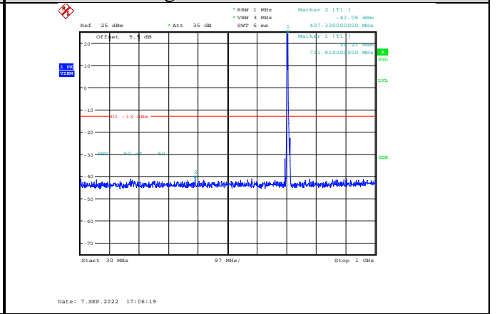
Band17-5MHz-QPSK-23825-1RB#0- Range1:30~1000MHz
