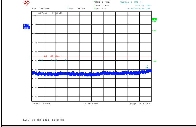
Band41-5MHz-64QAM-41215-1RB#0-Range3:3000~26500MHz
