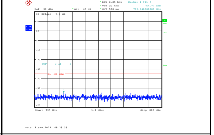
Band13-5MHz-16QAM-23205-1RB#0-Range4:793~805MHz
