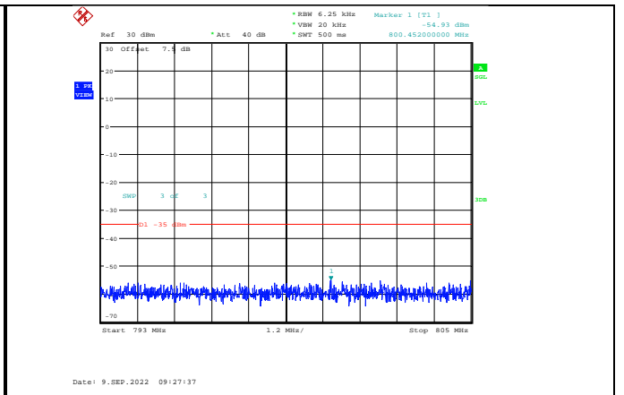
Band13-5MHz-16QAM-23255-1RB#0-Range4:793~805MHz
