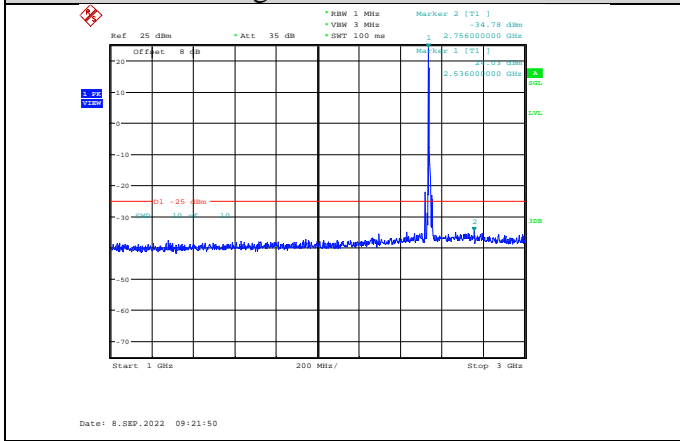
Band41-10MHz-16QAM-40090-1RB#0- Range2:1000~3000MHz
