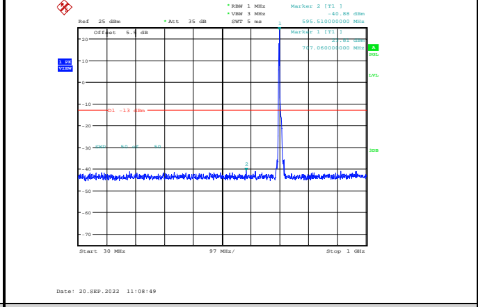
Band12-10MHz-64QAM-23130-1RB#0- Range1:30~1000MHz
