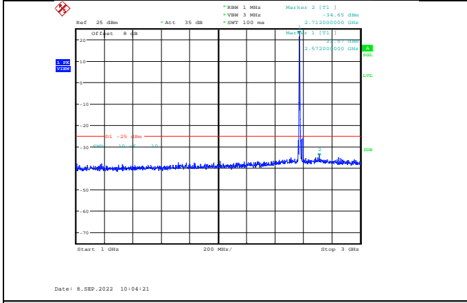
Band38-10MHz-16QAM-37800-1RB#0-Range2:1000~3000MHz
