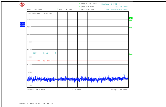
Band13-5MHz-64QAM-23230-1RB#0-Range3:763~775MHz
