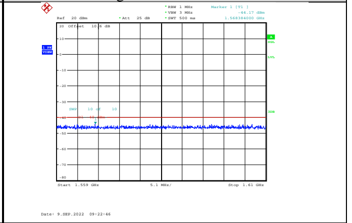
Band13-5MHz-QPSK-23205-1RB#0-Range5:1559~1610MHz
