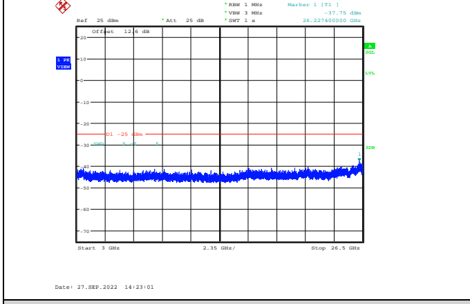
Band41-5MHz-64QAM-40065-1RB#0-Range3:3000~26500MHz
