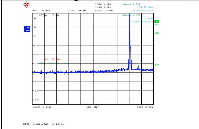
Band38-15MHz-QPSK-38175-1RB#0-Range2:1000~3000MHz
