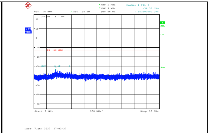
Band12-10MHz-16QAM-23095-1RB#0- Range2:1000~10000MHz
