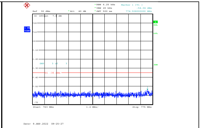
Band13-5MHz-16QAM-23230-1RB#0- Range3:763~775MHz
