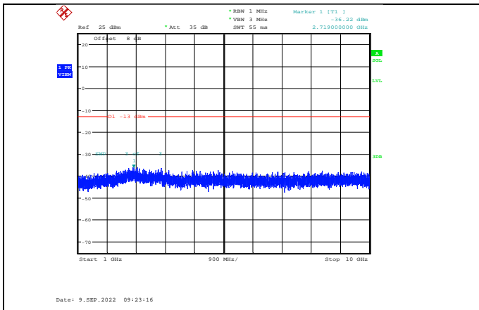
Band13-5MHz-16QAM-23205-1RB#0- Range2:1000~10000MHz
