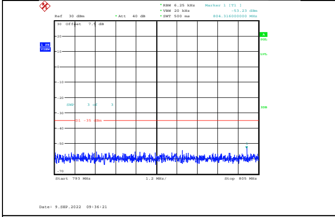
Band13-5MHz-64QAM-23230-1RB#0-Range4:793~805MHz
