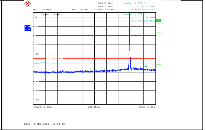
Band38-10MHz-QPSK-37800-1RB#0-Range2:1000~3000MHz
