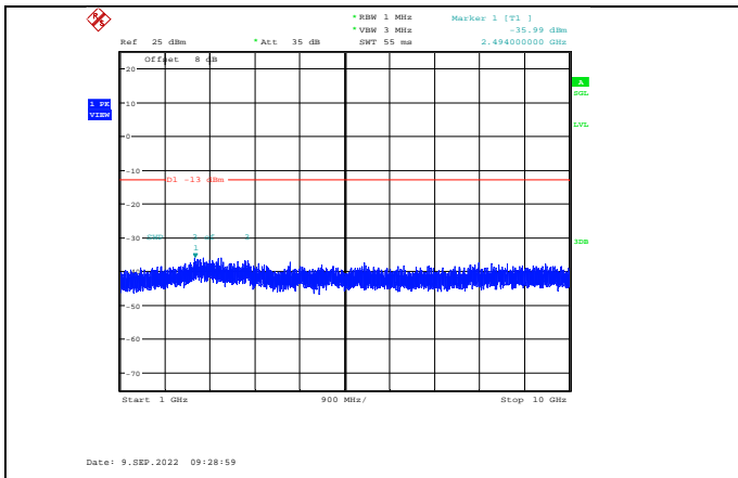
Band13-10MHz-QPSK-23230-1RB#0-Range2:1000~10000MHz
