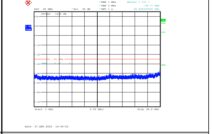
Band38-10MHz-16QAM-38000-1RB#0-Range3:3000~26500MHz
