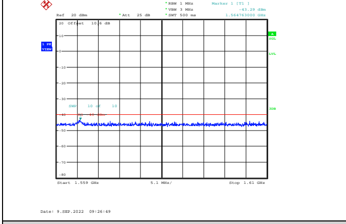
Band13-5MHz-QPSK-23255-1RB#0-Range5:1559~1610MHz
