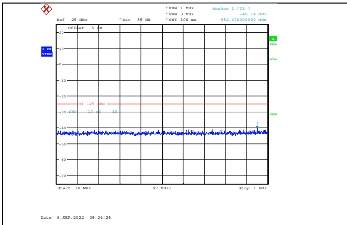
Band41-10MHz-16QAM-41190-1RB#0-Range1:30~1000MHz
