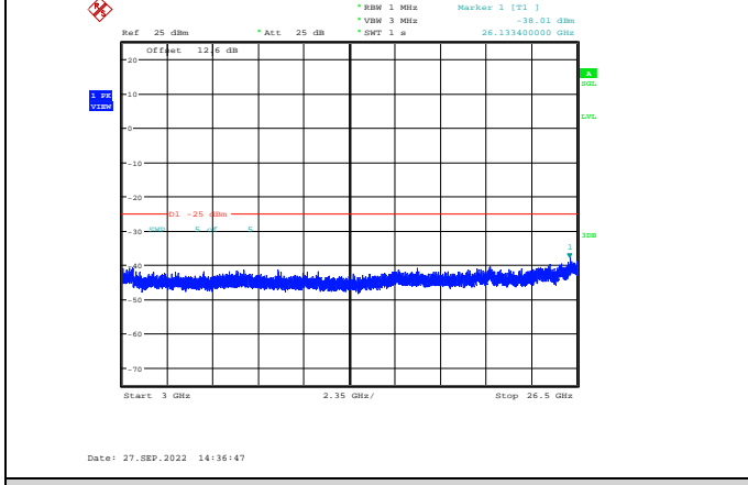
Band38-15MHz-64QAM-38175-1RB#0-Range3:3000~26500MHz
