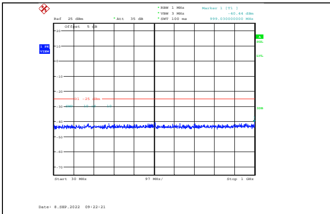
Band41-10MHz-QPSK-40640-1RB#0-Range1:30~1000MHz
