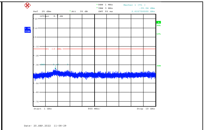
Band12-10MHz-64QAM-23095-1RB#0- Range2:1000~10000MHz
