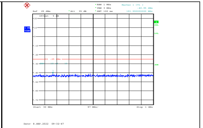
Band41-20MHz-16QAM-40640-1RB#0-Range1:30~1000MHz
