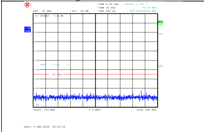
Band13-5MHz-QPSK-23205-1RB#0-Range4:793~805MHz
