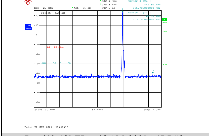
Band12-10MHz-64QAM-23095-1RB#0- Range1:30~1000MHz
