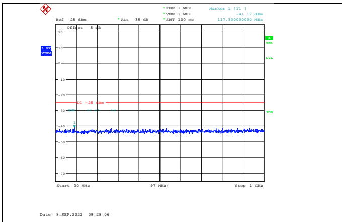
Band41-15MHz-16QAM-40640-1RB#0-Range1:30~1000MHz
