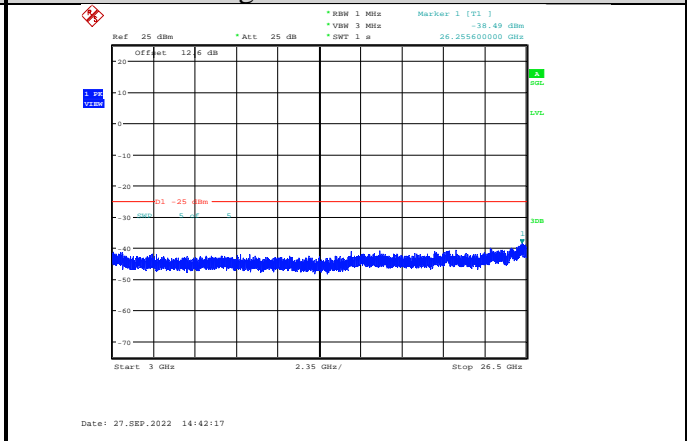
Band38-5MHz-QPSK-38000-1RB#0-Range3:3000~26500MHz
