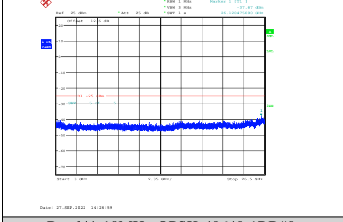
Band41-10MHz-QPSK-40640-1RB#0-Range3:3000~26500MHz
