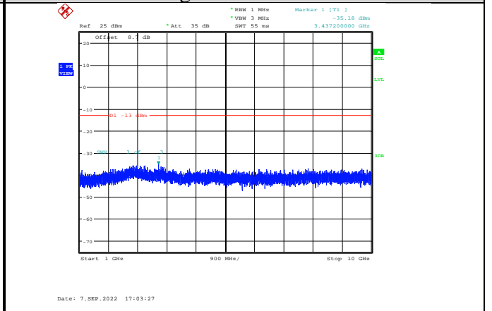
Band12-10MHz-16QAM-23130-1RB#0- Range2:1000~10000MHz
