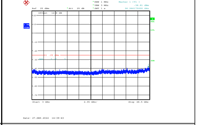
Band38-10MHz-QPSK-38200-1RB#0-Range3:3000~26500MHz
