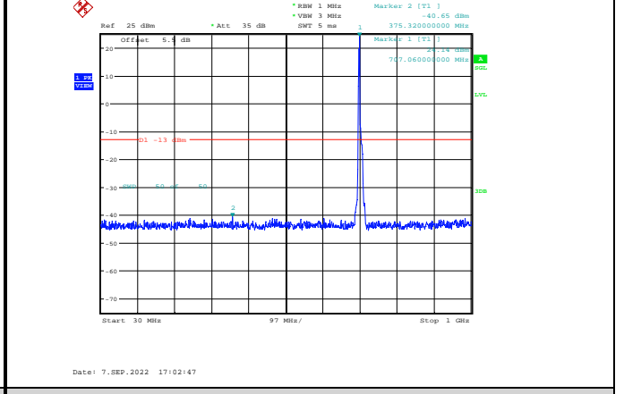
Band12-10MHz-QPSK-23130-1RB#0-Range1:30~1000MHz
