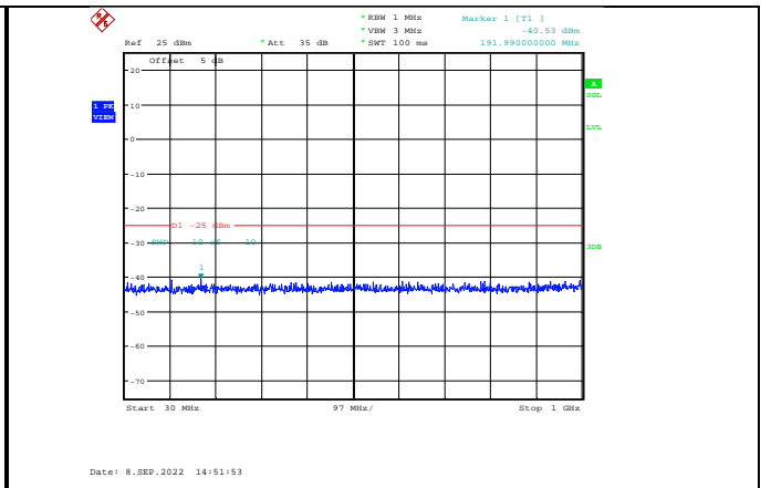
Band38-10MHz-64QAM-37800-1RB#0- Range1:30~1000MHz
