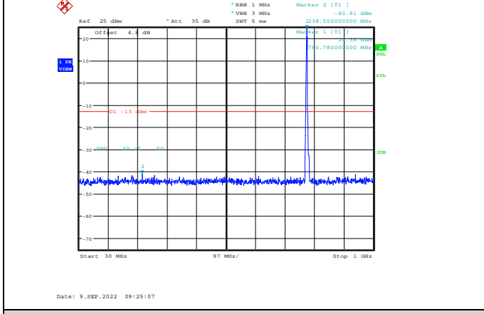
Band13-5MHz-16QAM-23230-1RB#0- Range1:30~1000MHz
