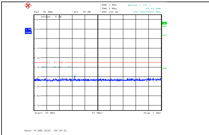
Band41-5MHz-16QAM-40640-1RB#0-Range1:30~1000MHz
