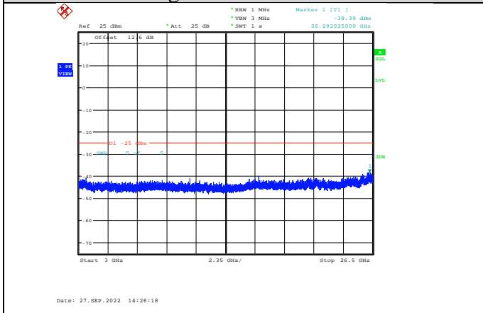
Band41-10MHz-16QAM-40090-1RB#0- Range3:3000~26500MHz
