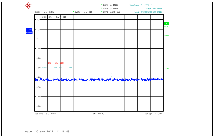
Band41-5MHz-64QAM-40640-1RB#0-Range1:30~1000MHz
