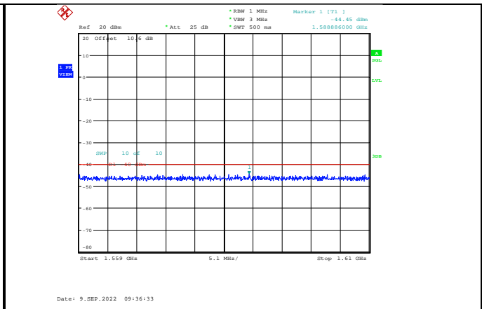
Band13-5MHz-64QAM-23230-1RB#0-Range5:1559~1610MHz
