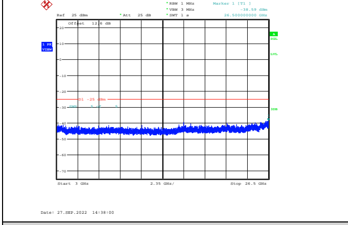
Band38-10MHz-16QAM-37800-1RB#0-Range3:3000~26500MHz
