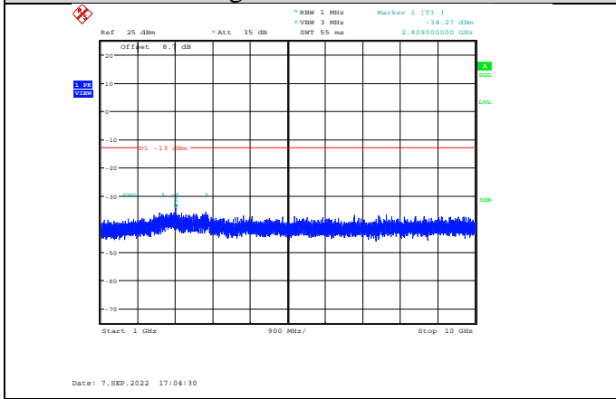
Band17-5MHz-QPSK-23755-1RB#0- Range2:1000~10000MHz
