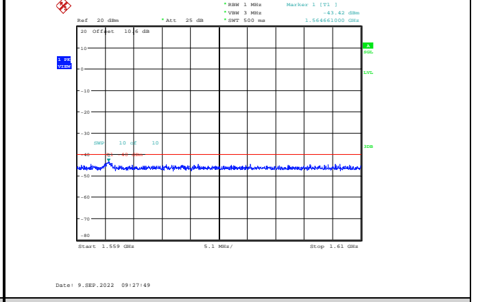
Band13-5MHz-16QAM-23255-1RB#0-Range5:1559~1610MHz
