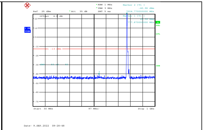
Band13-10MHz-QPSK-23230-1RB#0-Range1:30~1000MHz
