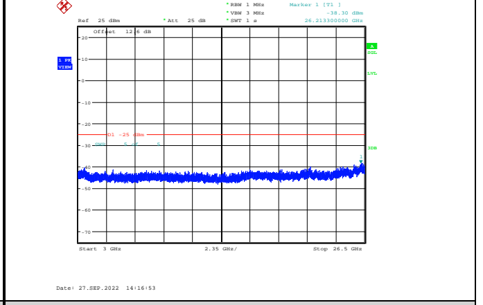
Band41-20MHz-QPSK-41140-1RB#0-Range3:3000~26500MHz
