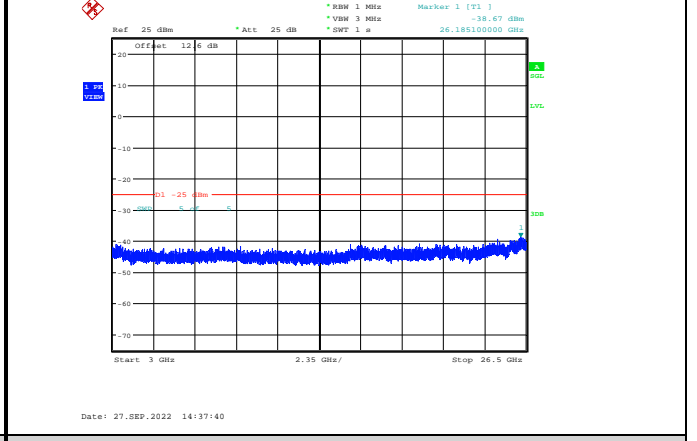
Band38-10MHz-QPSK-37800-1RB#0-Range3:3000~26500MHz
