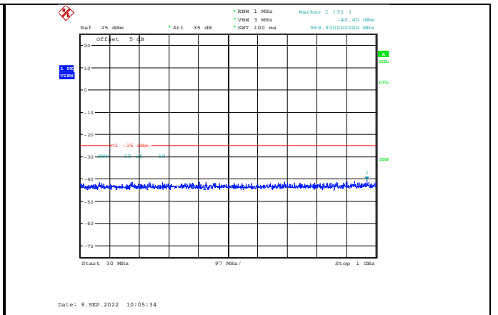
Band38-10MHz-16QAM-38000-1RB#0-Range1:30~1000MHz
