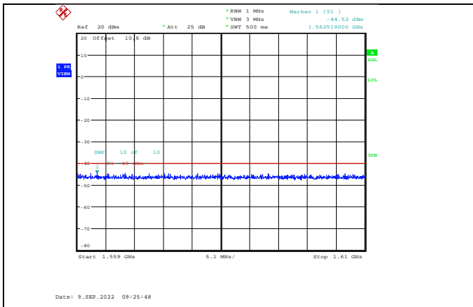
Band13-5MHz-16QAM-23230-1RB#0-Range5:1559~1610MHz
