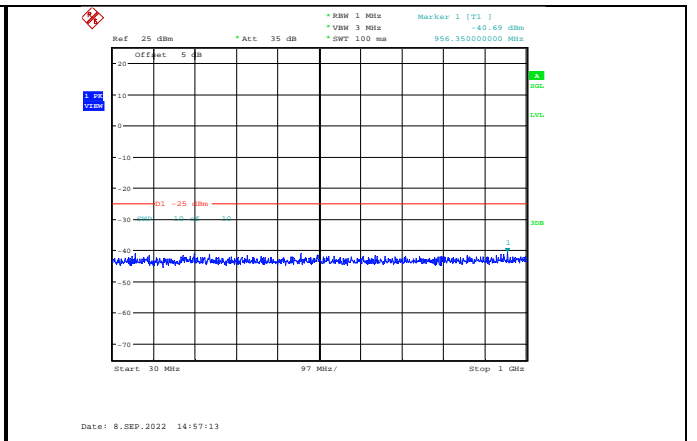
Band38-20MHz-64QAM-37850-1RB#0-Range1:30~1000MHz
