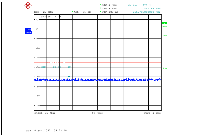
Band41-15MHz-QPSK-41165-1RB#0-Range1:30~1000MHz
