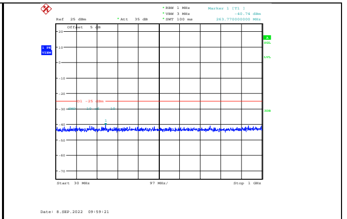
Band38-5MHz-16QAM-37775-1RB#0- Range1:30~1000MHz
