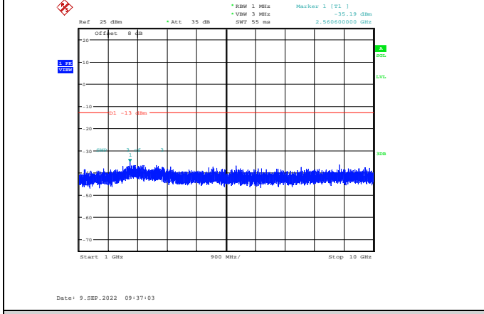
Band13-5MHz-64QAM-23255-1RB#0-Range2:1000~10000MHz
