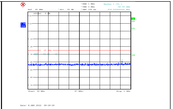
Band41-15MHz-16QAM-41165-1RB#0-Range1:30~1000MHz
