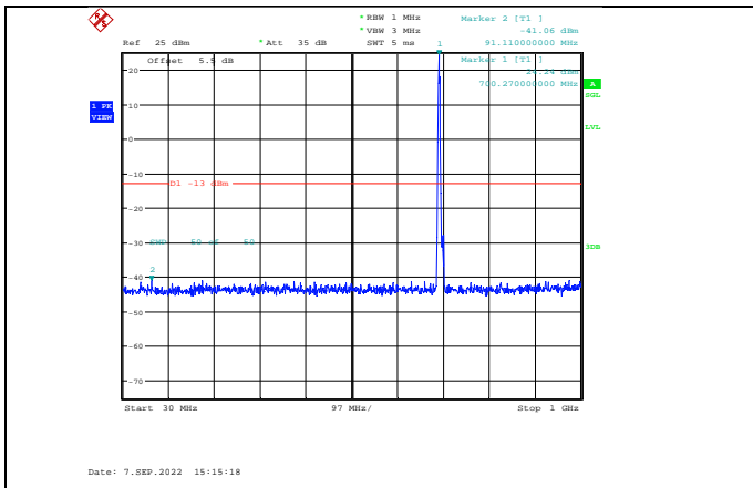
Band12-5MHz-16QAM-23035-1RB#0-Range1:30~1000MHz
