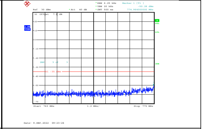
Band13-5MHz-16QAM-23205-1RB#0-Range3:763~775MHz
