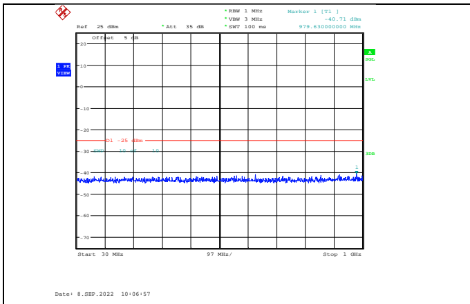
Band38-10MHz-16QAM-38200-1RB#0- Range1:30~1000MHz
