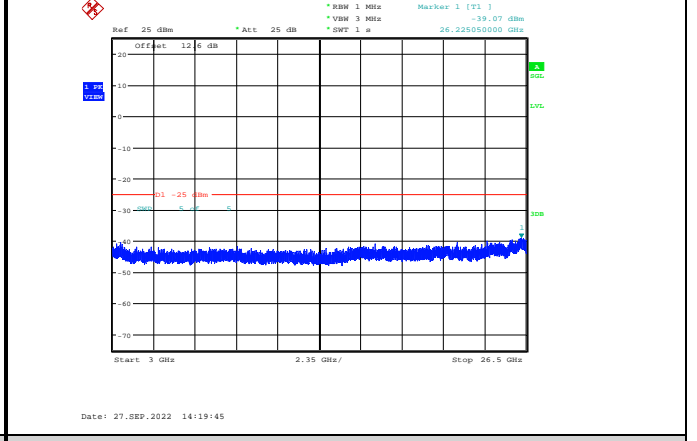
Band41-15MHz-QPSK-40640-1RB#0-Range3:3000~26500MHz
