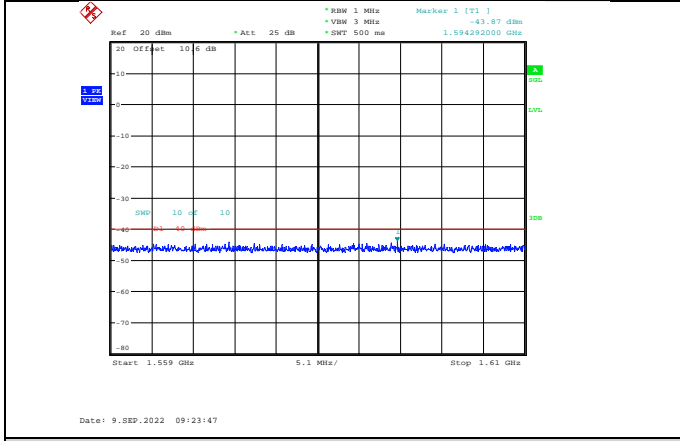
Band13-5MHz-16QAM-23205-1RB#0- Range5:1559~1610MHz
