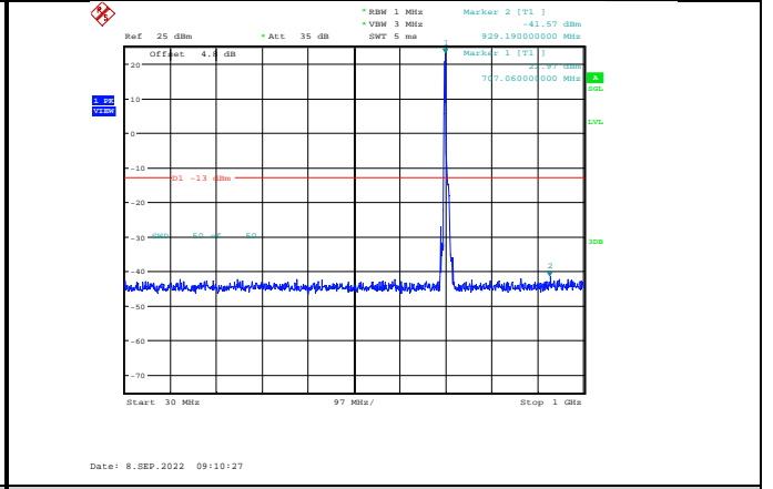
Band17-10MHz-QPSK-23800-1RB#0-Range1:30~1000MHz
