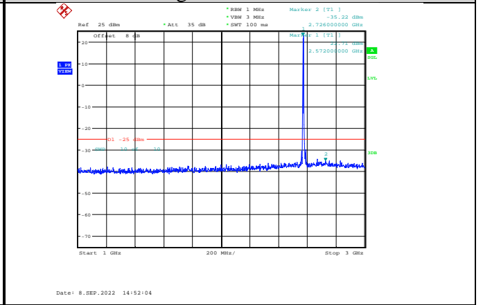
Band38-10MHz-64QAM-37800-1RB#0- Range2:1000~3000MHz
