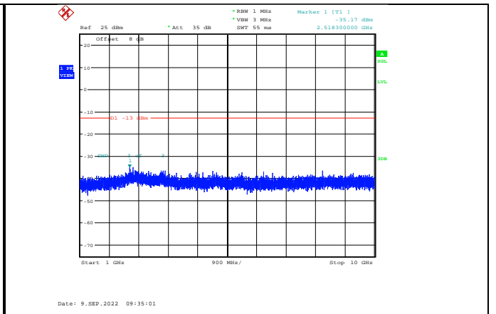
Band13-5MHz-64QAM-23205-1RB#0-Range2:1000~10000MHz
