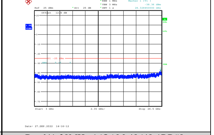
Band41-20MHz-16QAM-40640-1RB#0-Range3:3000~26500MHz
