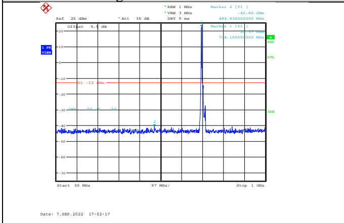
Band12-10MHz-16QAM-23095-1RB#0- Range1:30~1000MHz
