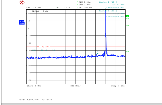
Band38-20MHz-16QAM-38150-1RB#0-Range2:1000~3000MHz
