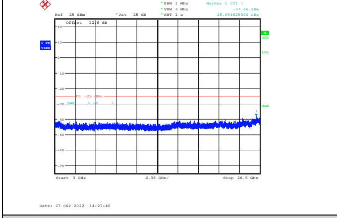
Band41-10MHz-64QAM-40640-1RB#0- Range3:3000~26500MHz
