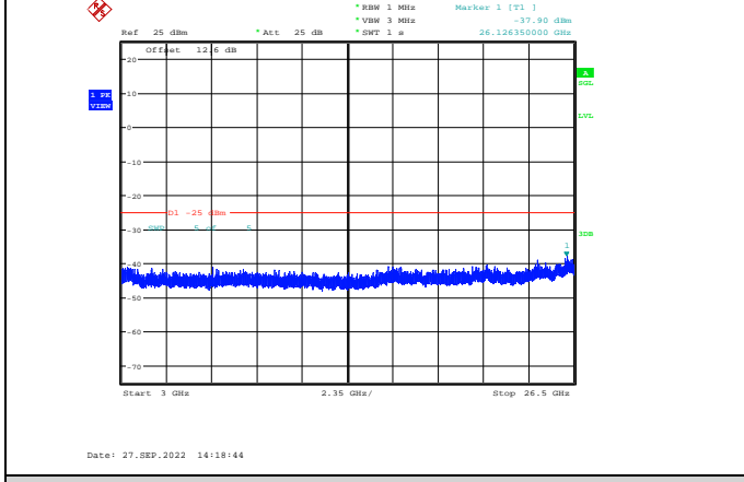
Band41-15MHz-QPSK-40115-1RB#0-Range3:3000~26500MHz
