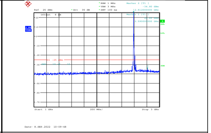
Band38-15MHz-QPSK-38000-1RB#0-Range2:1000~3000MHz
