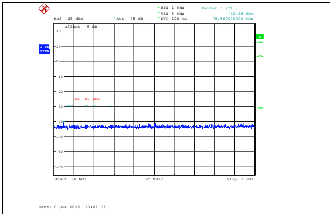
Band38-5MHz-QPSK-38225-1RB#0- Range1:30~1000MHz
