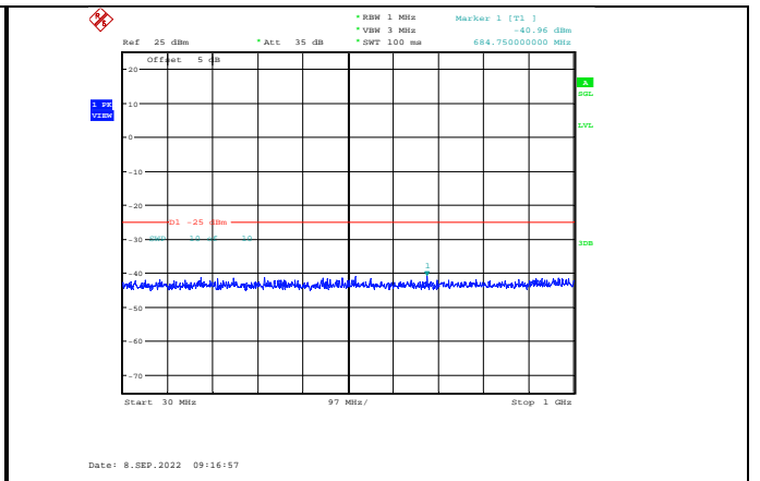
Band41-5MHz-16QAM-40065-1RB#0- Range1:30~1000MHz
