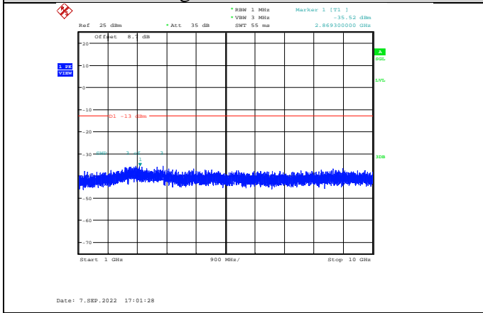
Band12-10MHz-16QAM-23060-1RB#0- Range2:1000~10000MHz
