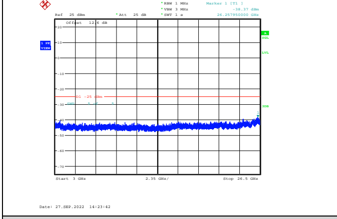
Band41-5MHz-16QAM-40640-1RB#0-Range3:3000~26500MHz
