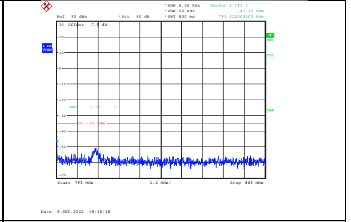
Band13-10MHz-16QAM-23230-1RB#0-Range4:793~805MHz
