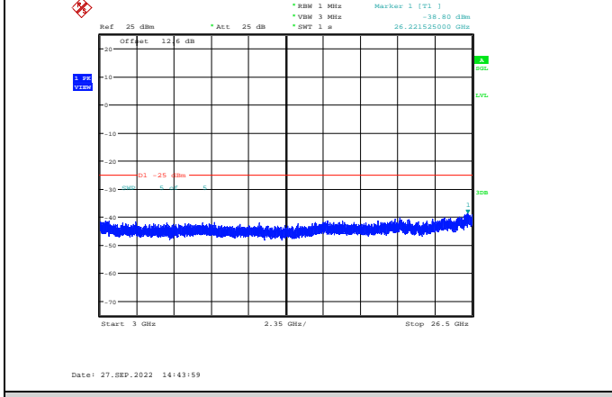
Band38-5MHz-64QAM-38225-1RB#0-Range3:3000~26500MHz
