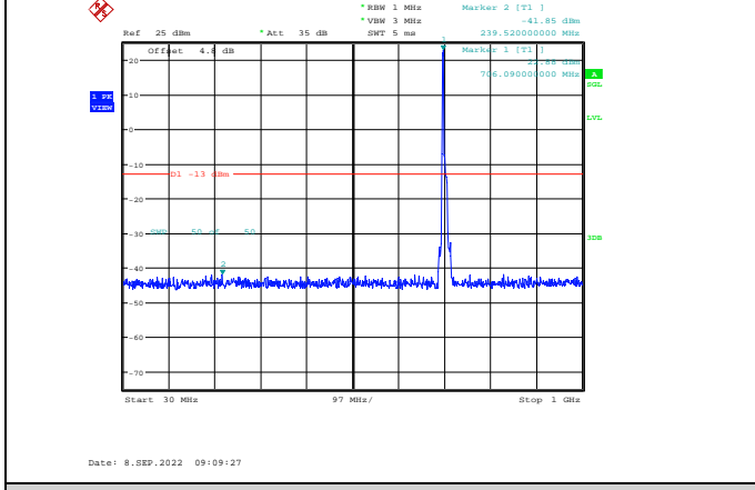
Band17-10MHz-QPSK-23790-1RB#0-Range1:30~1000MHz
