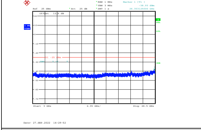
Band38-20MHz-16QAM-37850-1RB#0-Range3:3000~26500MHz
