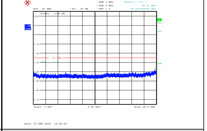
Band41-10MHz-64QAM-41190-1RB#0- Range3:3000~26500MHz
