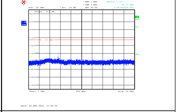
Band12-5MHz-64QAM-23155-1RB#0- Range2:1000~10000MHz
