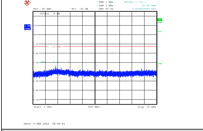
Band13-5MHz-64QAM-23230-1RB#0-Range2:1000~10000MHz
