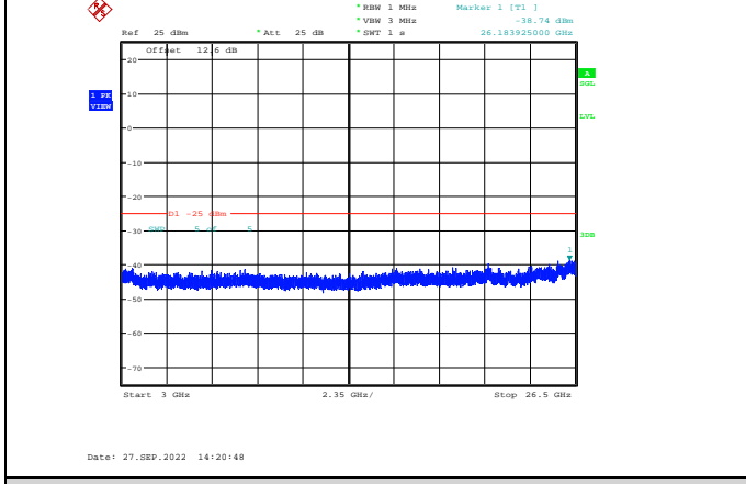
Band41-15MHz-QPSK-41165-1RB#0-Range3:3000~26500MHz
