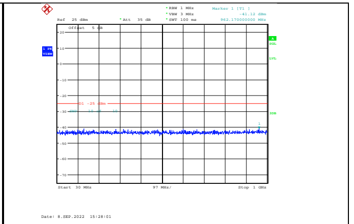
Band41-15MHz-64QAM-40640-1RB#0- Range1:30~1000MHz
