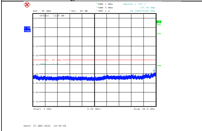
Band38-15MHz-QPSK-38175-1RB#0-Range3:3000~26500MHz
