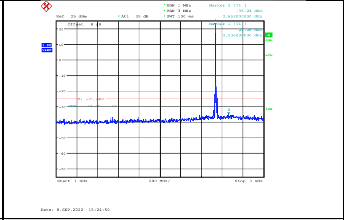
Band41-10MHz-64QAM-40090-1RB#0-Range2:1000~3000MHz
