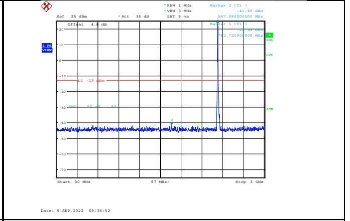
Band13-5MHz-64QAM-23255-1RB#0-Range1:30~1000MHz
