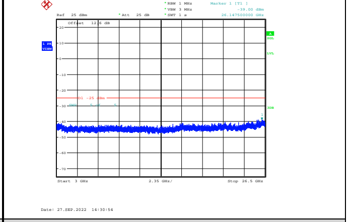
Band38-20MHz-16QAM-38000-1RB#0-Range3:3000~26500MHz
