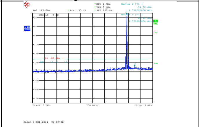
Band38-5MHz-16QAM-37775-1RB#0- Range2:1000~3000MHz
