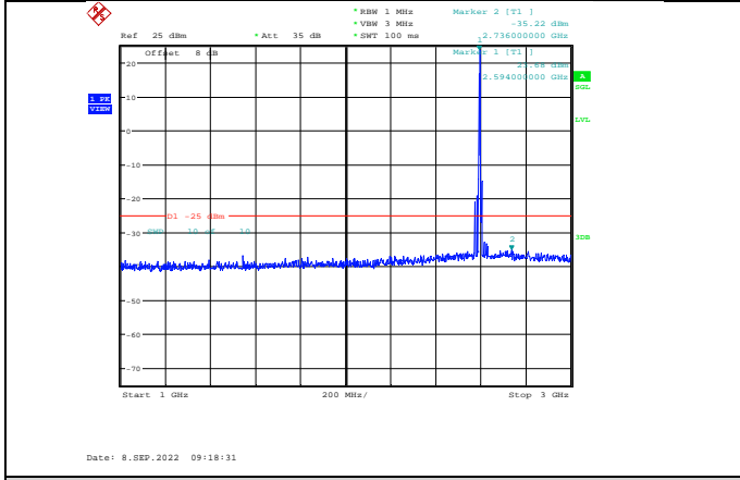
Band41-5MHz-16QAM-40640-1RB#0-Range2:1000~3000MHz
