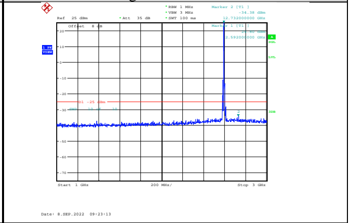
Band41-10MHz-16QAM-40640-1RB#0- Range2:1000~3000MHz
