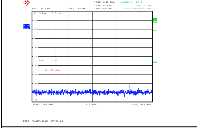
Band13-5MHz-64QAM-23205-1RB#0-Range4:793~805MHz
