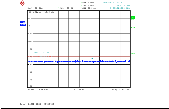
Band13-10MHz-QPSK-23230-1RB#0-Range5:1559~1610MHz
