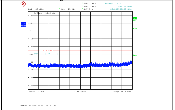
Band41-5MHz-16QAM-40065-1RB#0- Range3:3000~26500MHz
