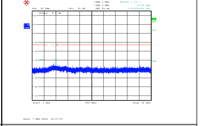
Band12-5MHz-16QAM-23155-1RB#0-Range2:1000~10000MHz
