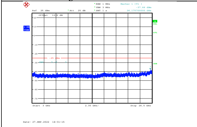
Band38-20MHz-64QAM-38000-1RB#0-Range3:3000~26500MHz
