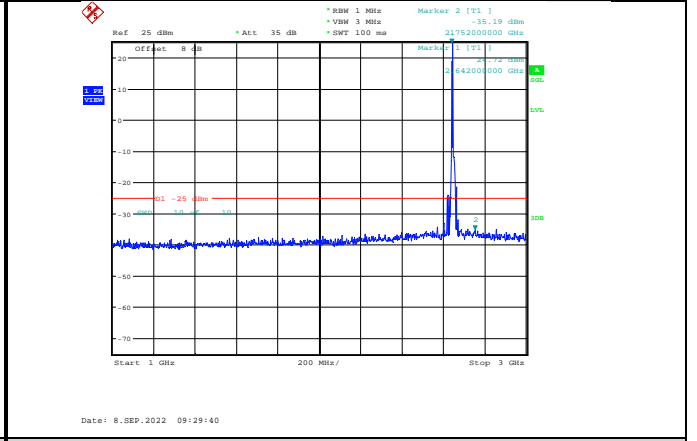
Band41-15MHz-16QAM-41165-1RB#0-Range2:1000~3000MHz
