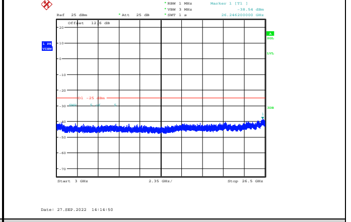
Band41-20MHz-QPSK-40140-1RB#0-Range3:3000~26500MHz
