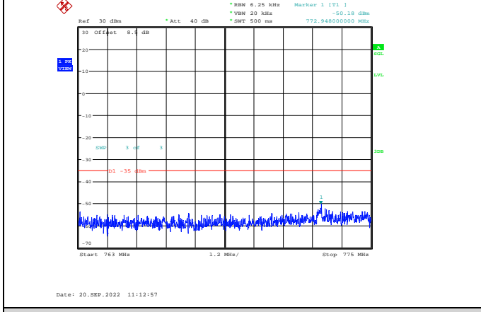
Band13-10MHz-64QAM-23230-1RB#0-Range3:763~775MHz
