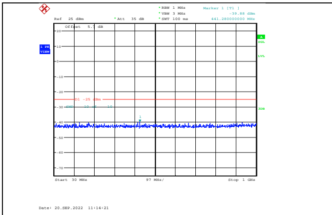
Band41-5MHz-64QAM-40065-1RB#0-Range1:30~1000MHz
