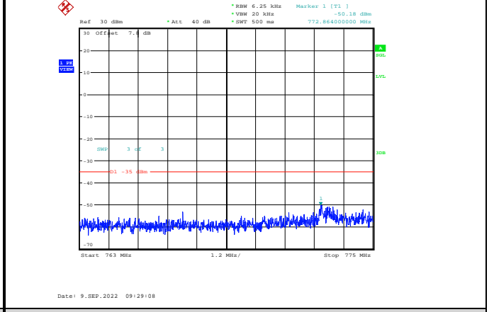
Band13-10MHz-QPSK-23230-1RB#0-Range3:763~775MHz
