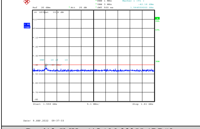
Band13-5MHz-64QAM-23255-1RB#0-Range5:1559~1610MHz
