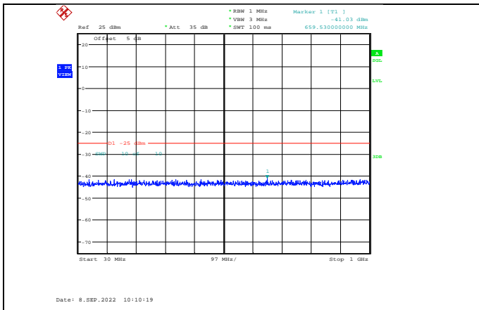
Band38-15MHz-16QAM-38000-1RB#0-Range1:30~1000MHz
