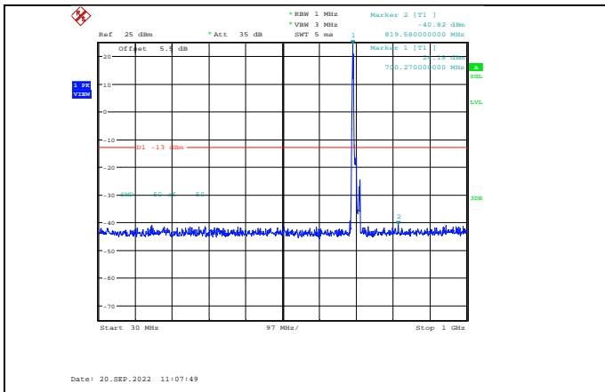
Band12-10MHz-64QAM-23060-1RB#0- Range1:30~1000MHz
