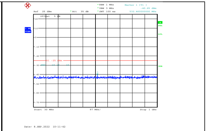
Band38-15MHz-16QAM-38175-1RB#0-Range1:30~1000MHz
