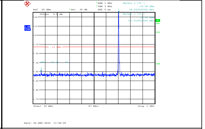
Band12-5MHz-64QAM-23155-1RB#0- Range1:30~1000MHz
