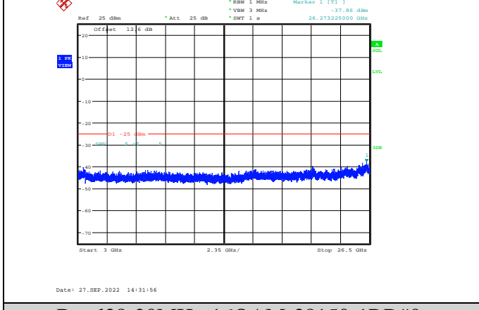
Band38-20MHz-16QAM-38150-1RB#0-Range3:3000~26500MHz
