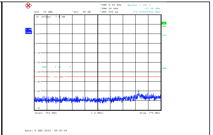
Band13-10MHz-16QAM-23230-1RB#0-Range3:763~775MHz
