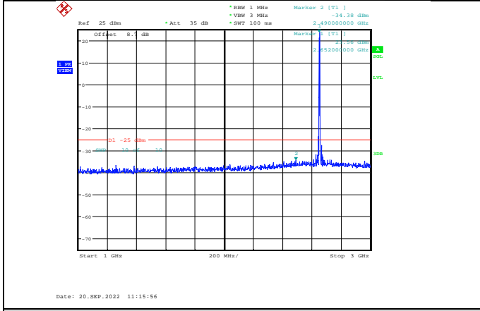
Band41-5MHz-64QAM-41215-1RB#0-Range2:1000~3000MHz
