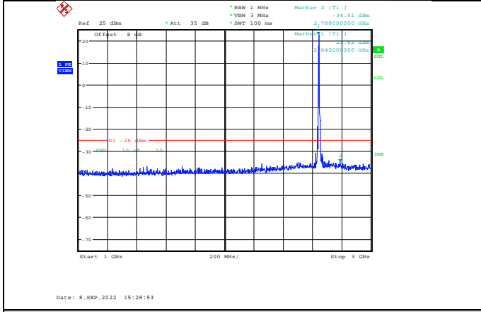
Band41-15MHz-64QAM-41165-1RB#0-Range2:1000~3000MHz
