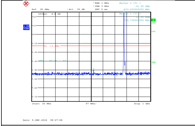
Band13-5MHz-16QAM-23255-1RB#0-Range1:30~1000MHz
