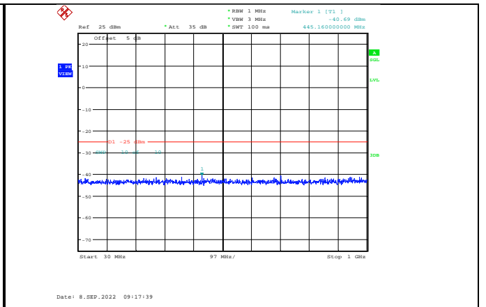
Band41-5MHz-QPSK-40640-1RB#0-Range1:30~1000MHz
