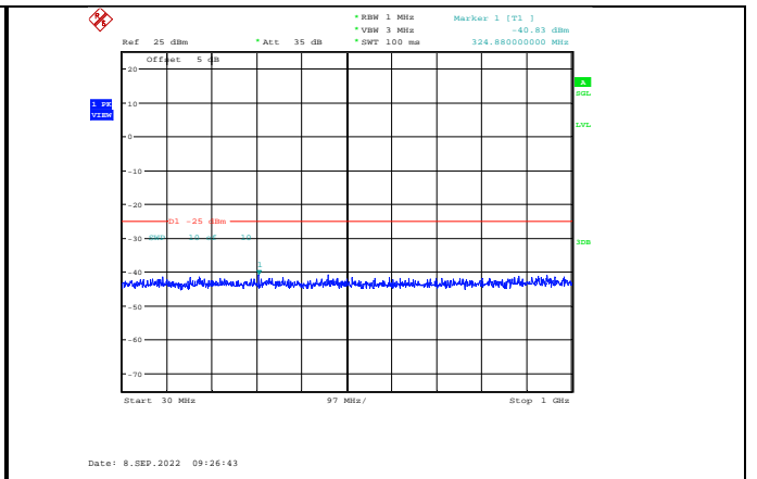
Band41-15MHz-16QAM-40115-1RB#0-Range1:30~1000MHz
