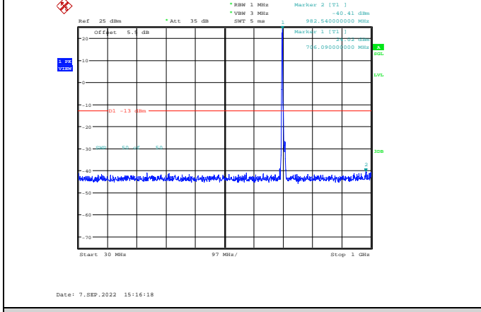
Band12-5MHz-16QAM-23095-1RB#0-Range1:30~1000MHz
