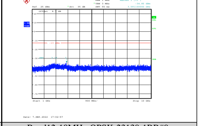
Band12-10MHz-QPSK-23130-1RB#0-Range2:1000~10000MHz
