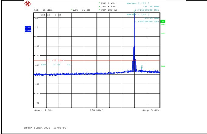
Band38-5MHz-16QAM-38000-1RB#0-Range2:1000~3000MHz
