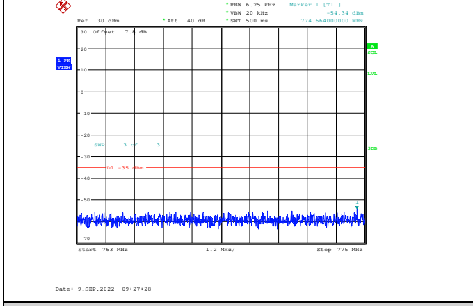
Band13-5MHz-16QAM-23255-1RB#0-Range3:763~775MHz
