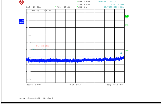
Band41-15MHz-16QAM-40640-1RB#0-Range3:3000~26500MHz
