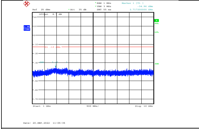
Band12-5MHz-64QAM-23035-1RB#0- Range2:1000~10000MHz
