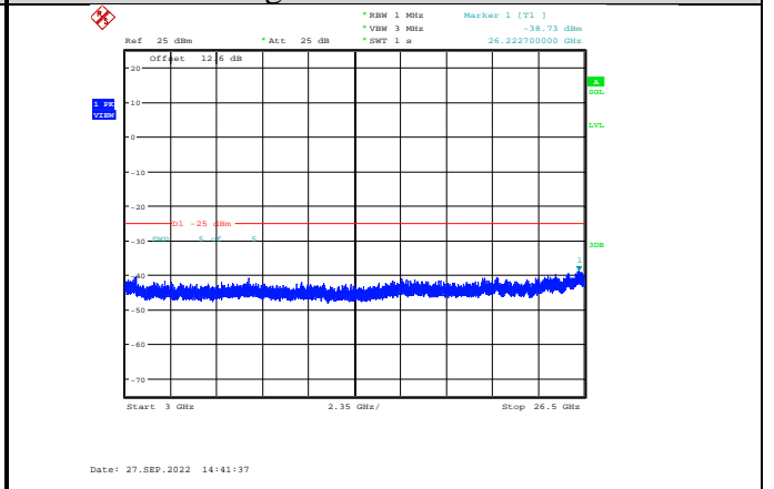
Band38-5MHz-16QAM-37775-1RB#0- Range3:3000~26500MHz
