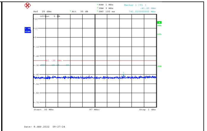
Band41-15MHz-QPSK-40640-1RB#0-Range1:30~1000MHz
