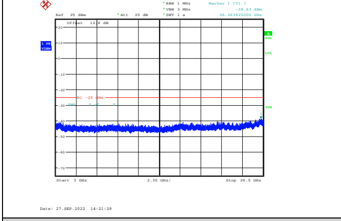
Band41-15MHz-64QAM-41165-1RB#0-Range3:3000~26500MHz
