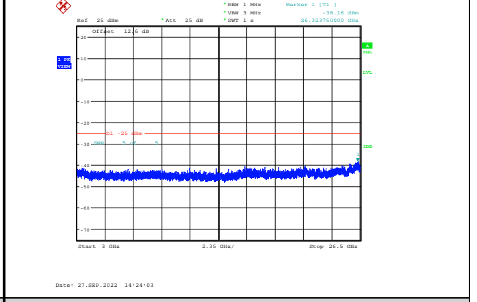
Band41-5MHz-64QAM-40640-1RB#0-Range3:3000~26500MHz
