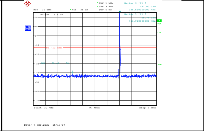
Band12-5MHz-16QAM-23155-1RB#0-Range1:30~1000MHz
