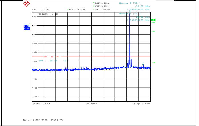
Band41-5MHz-16QAM-41215-1RB#0-Range2:1000~3000MHz
