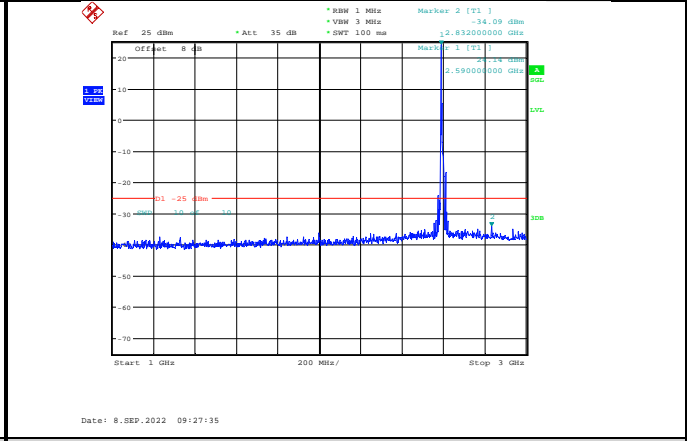
Band41-15MHz-QPSK-40640-1RB#0-Range2:1000~3000MHz
