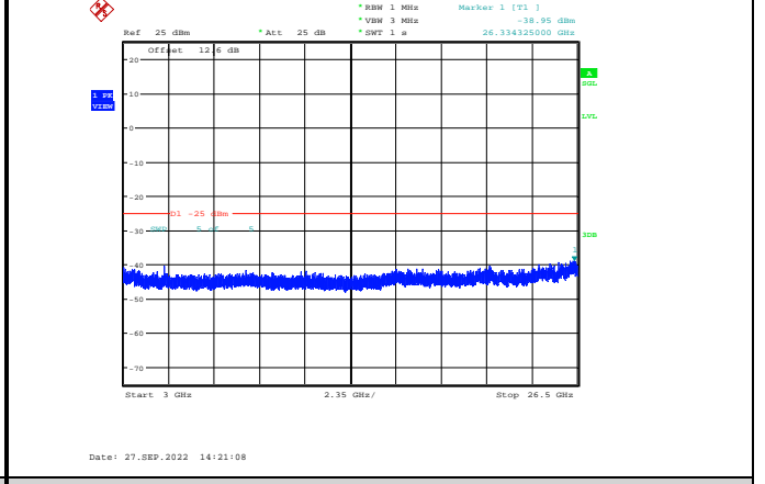
Band41-15MHz-16QAM-41165-1RB#0-Range3:3000~26500MHz
