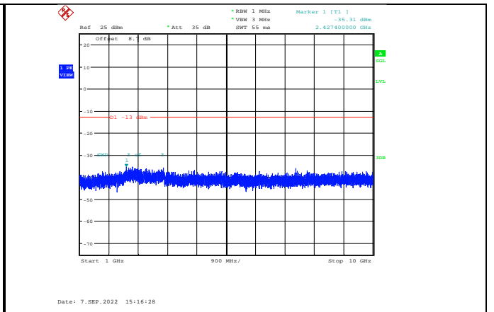
Band12-5MHz-16QAM-23095-1RB#0-Range2:1000~10000MHz
