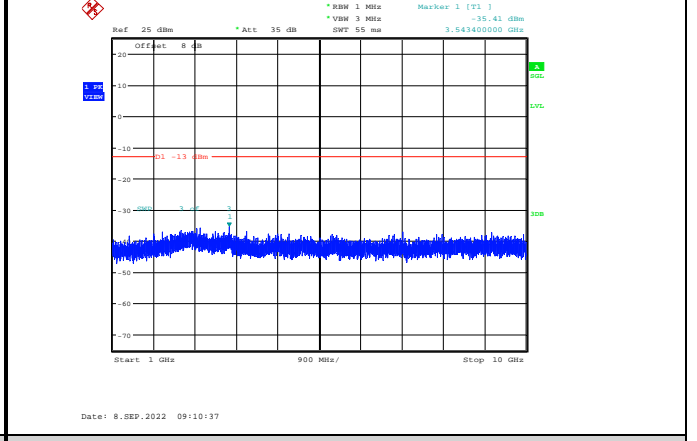
Band17-10MHz-QPSK-23800-1RB#0-Range2:1000~10000MHz
