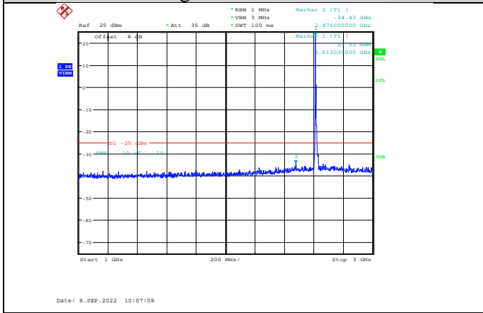
Band38-10MHz-16QAM-38200-1RB#0- Range2:1000~3000MHz
