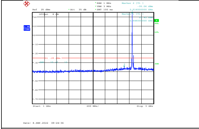
Band41-10MHz-16QAM-41190-1RB#0-Range2:1000~3000MHz
