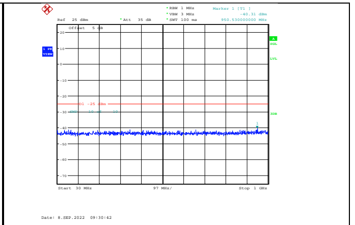
Band41-20MHz-QPSK-40140-1RB#0-Range1:30~1000MHz
