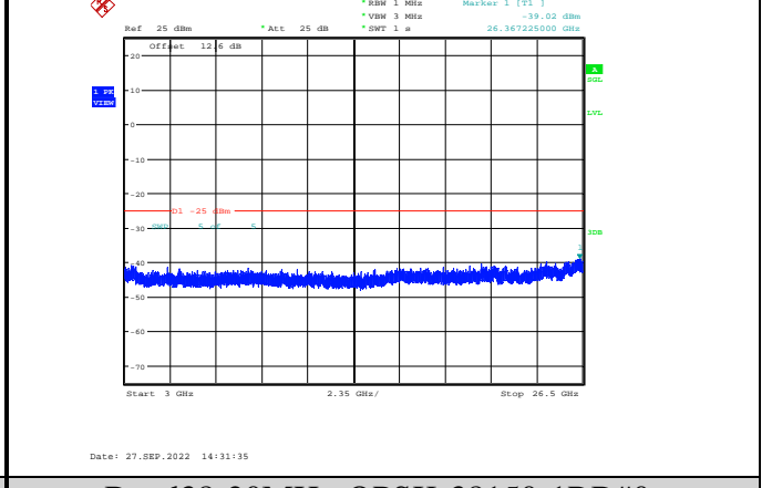
Band38-20MHz-QPSK-38150-1RB#0-Range3:3000~26500MHz
