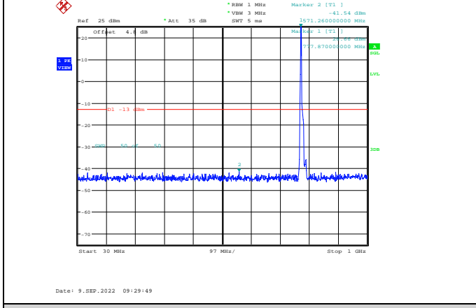
Band13-10MHz-16QAM-23230-1RB#0-Range1:30~1000MHz
