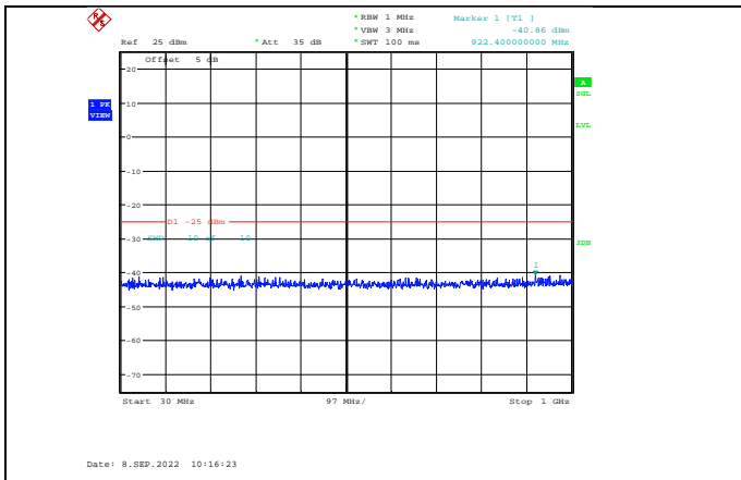
Band38-20MHz-16QAM-38150-1RB#0-Range1:30~1000MHz
