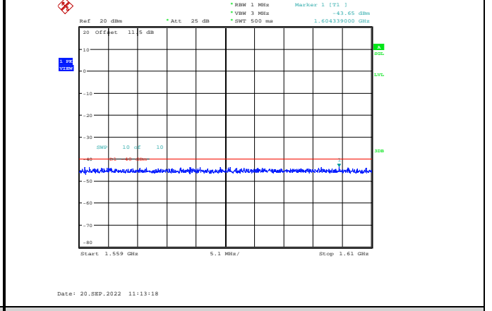
Band13-10MHz-64QAM-23230-1RB#0-Range5:1559~1610MHz
