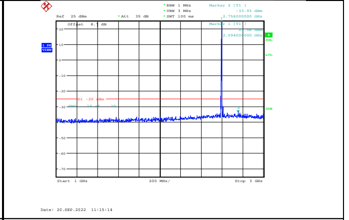
Band41-5MHz-64QAM-40640-1RB#0-Range2:1000~3000MHz
