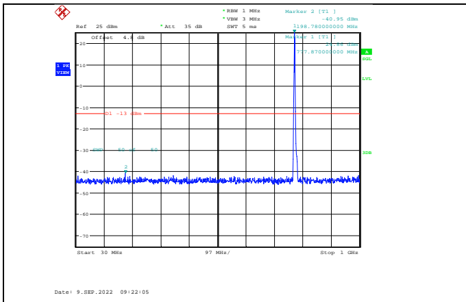
Band13-5MHz-QPSK-23205-1RB#0-Range1:30~1000MHz
