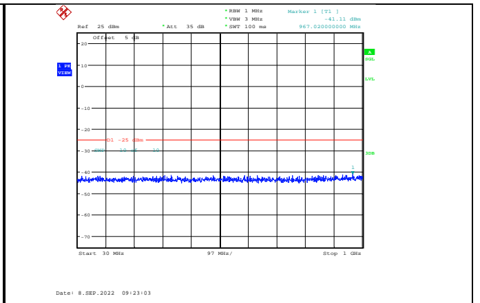
Band41-10MHz-16QAM-40640-1RB#0- Range1:30~1000MHz
