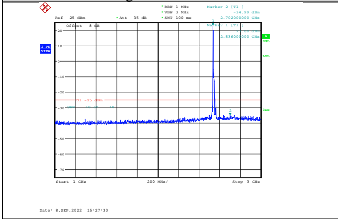
Band41-15MHz-64QAM-40115-1RB#0- Range2:1000~3000MHz
