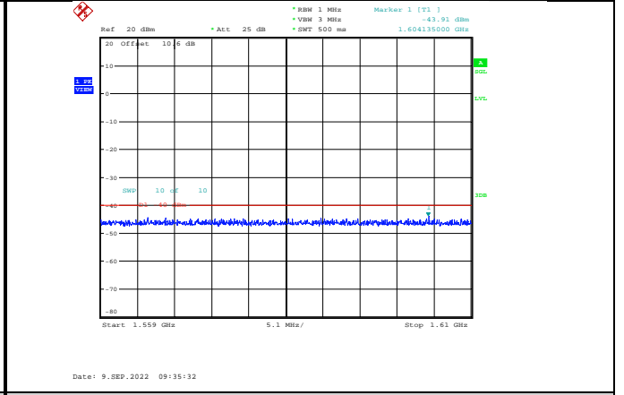
Band13-5MHz-64QAM-23205-1RB#0-Range5:1559~1610MHz
