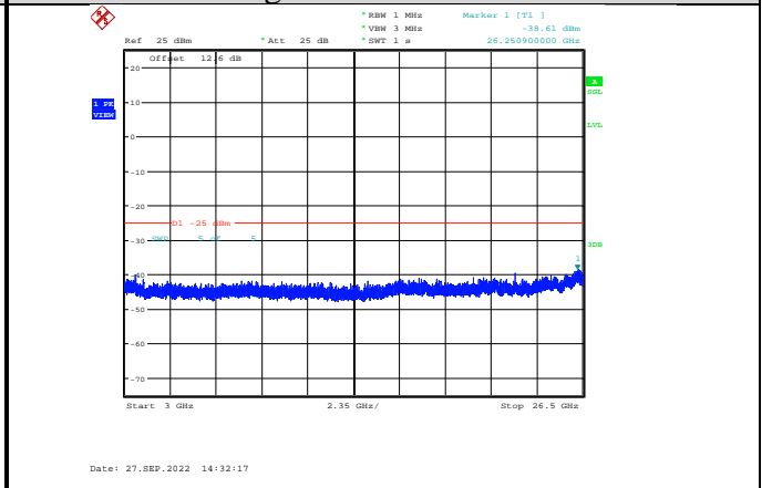
Band38-20MHz-64QAM-38150-1RB#0-Range3:3000~26500MHz
