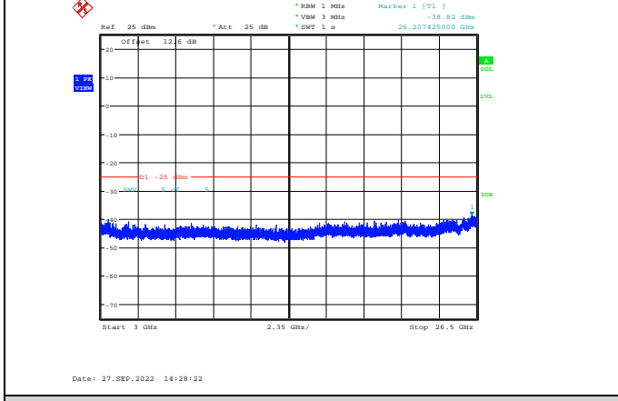
Band41-10MHz-16QAM-41190-1RB#0-Range3:3000~26500MHz
