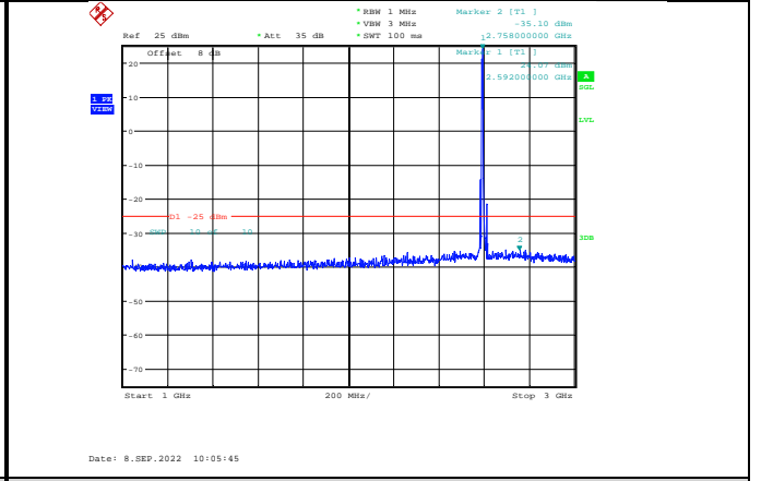
Band38-10MHz-16QAM-38000-1RB#0-Range2:1000~3000MHz
