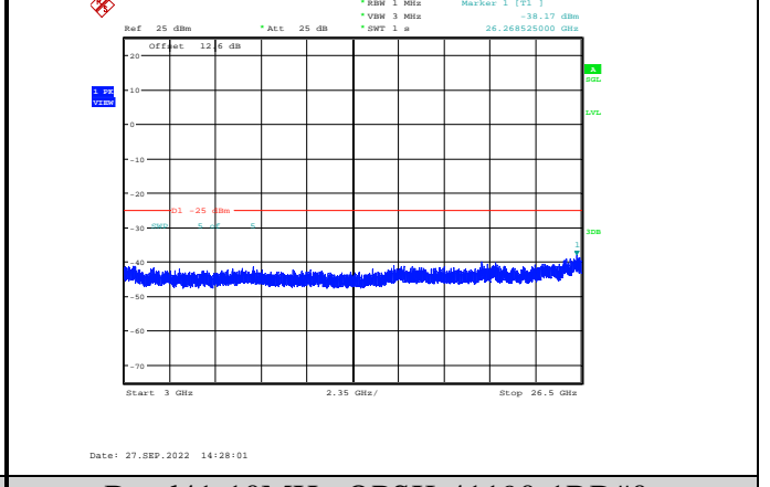
Band41-10MHz-QPSK-41190-1RB#0-Range3:3000~26500MHz
