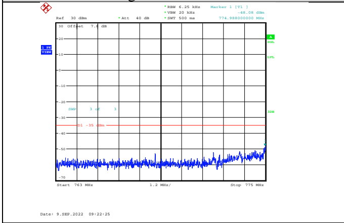
Band13-5MHz-QPSK-23205-1RB#0-Range3:763~775MHz
