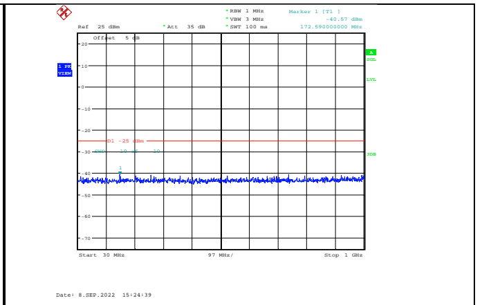
Band41-10MHz-64QAM-40090-1RB#0-Range1:30~1000MHz
