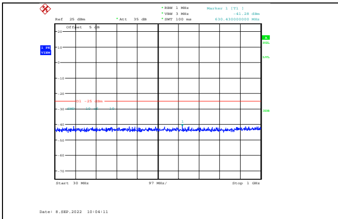
Band38-10MHz-16QAM-37800-1RB#0-Range1:30~1000MHz
