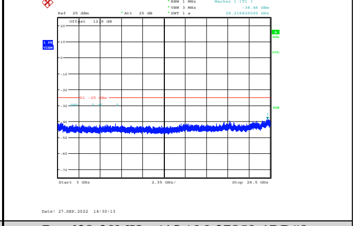
Band38-20MHz-64QAM-37850-1RB#0-Range3:3000~26500MHz
