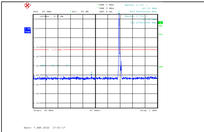
Band12-10MHz-16QAM-23060-1RB#0- Range1:30~1000MHz
