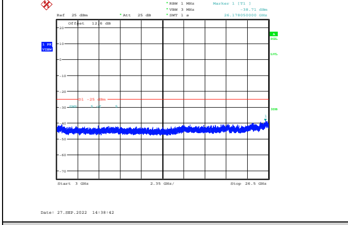
Band38-10MHz-QPSK-38000-1RB#0-Range3:3000~26500MHz
