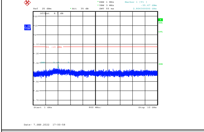
Band12-10MHz-QPSK-23060-1RB#0-Range2:1000~10000MHz
