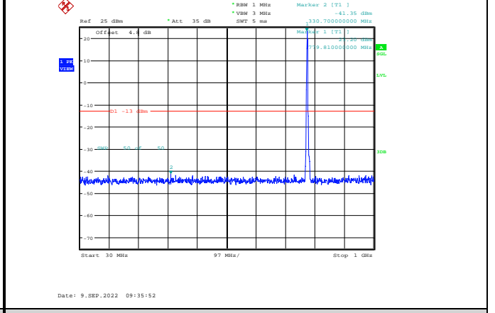
Band13-5MHz-64QAM-23230-1RB#0-Range1:30~1000MHz
