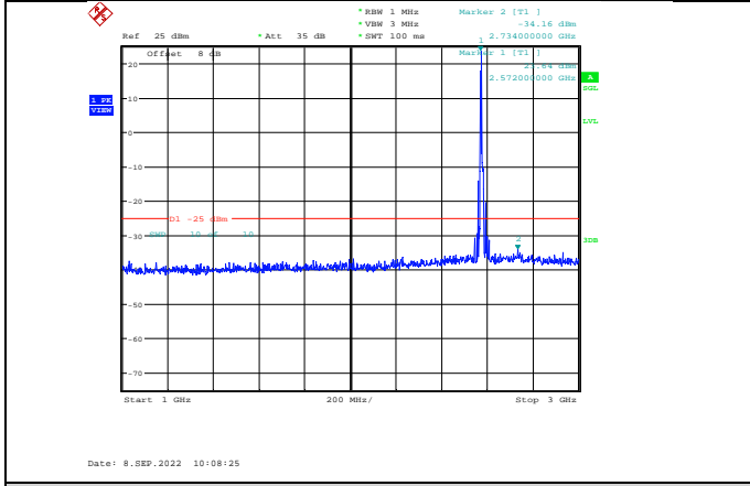
Band38-15MHz-QPSK-37825-1RB#0-Range2:1000~3000MHz
