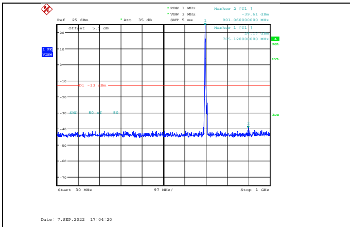
Band17-5MHz-QPSK-23755-1RB#0- Range1:30~1000MHz
