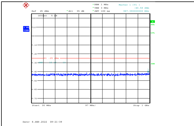
Band41-10MHz-16QAM-40090-1RB#0- Range1:30~1000MHz
