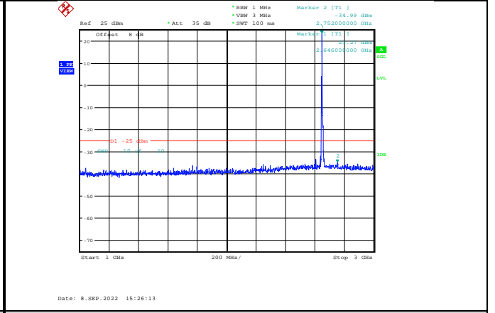
Band41-10MHz-64QAM-41190-1RB#0- Range2:1000~3000MHz
