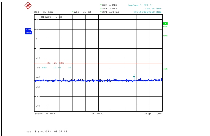
Band41-20MHz-QPSK-40640-1RB#0-Range1:30~1000MHz
