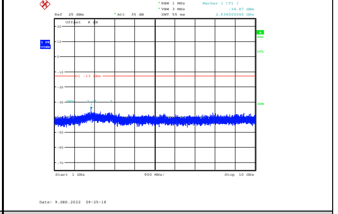
Band13-5MHz-16QAM-23230-1RB#0- Range2:1000~10000MHz
