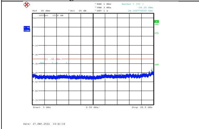
Band38-5MHz-QPSK-37775-1RB#0-Range3:3000~26500MHz
