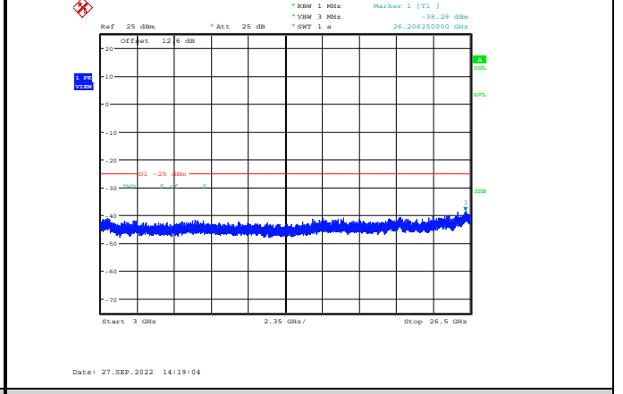
Band41-15MHz-16QAM-40115-1RB#0-Range3:3000~26500MHz
