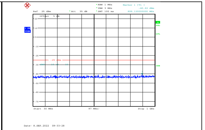
Band41-20MHz-QPSK-41140-1RB#0-Range1:30~1000MHz
