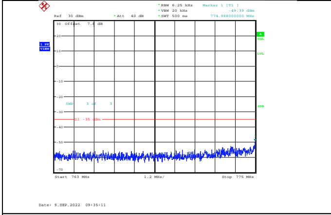
Band13-5MHz-64QAM-23205-1RB#0-Range3:763~775MHz
