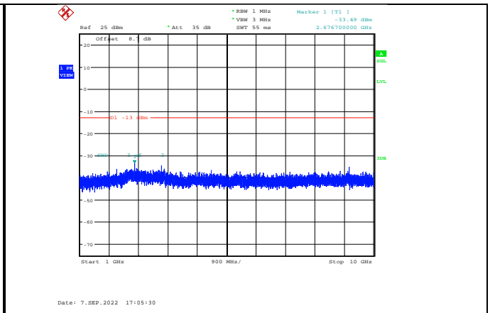
Band17-5MHz-QPSK-23790-1RB#0- Range2:1000~10000MHz
