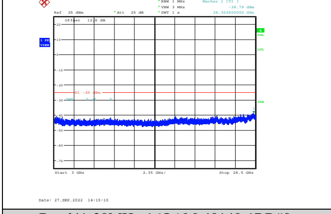
Band41-20MHz-16QAM-40140-1RB#0-Range3:3000~26500MHz
