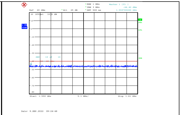
Band13-5MHz-QPSK-23230-1RB#0-Range5:1559~1610MHz
