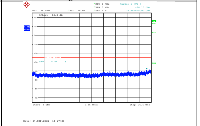
Band41-10MHz-16QAM-40640-1RB#0- Range3:3000~26500MHz
