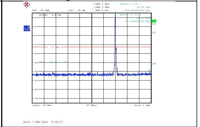
Band12-10MHz-16QAM-23130-1RB#0- Range1:30~1000MHz
