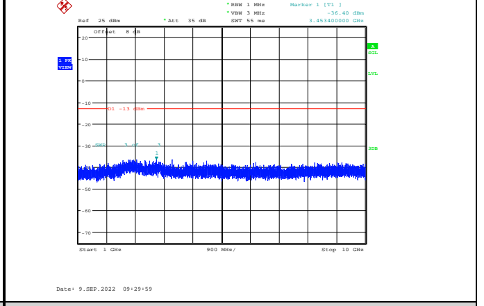
Band13-10MHz-16QAM-23230-1RB#0-Range2:1000~10000MHz
