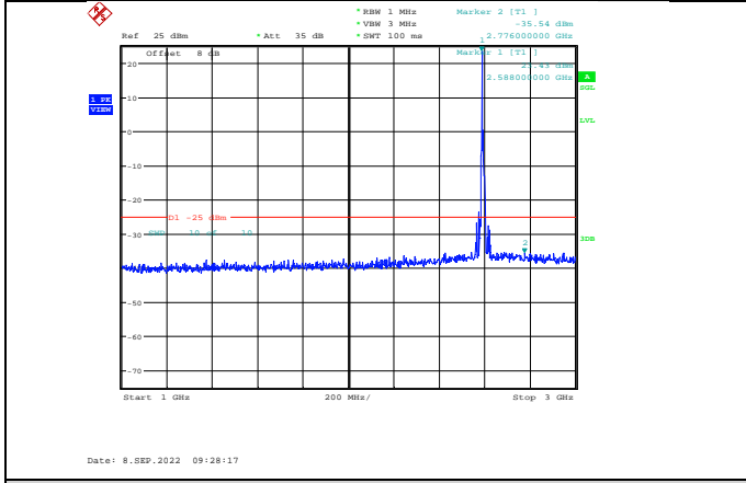
Band41-15MHz-16QAM-40640-1RB#0-Range2:1000~3000MHz
