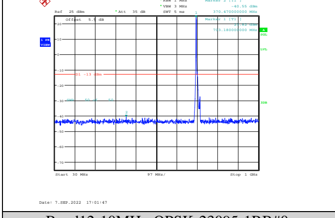
Band12-10MHz-QPSK-23095-1RB#0-Range1:30~1000MHz
