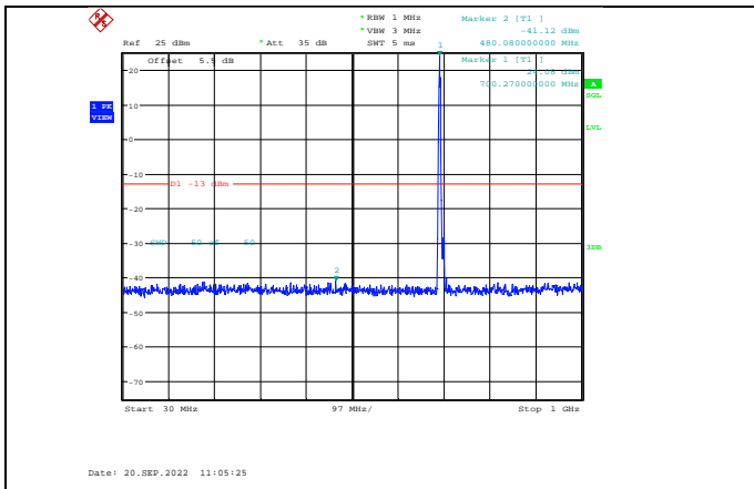
Band12-5MHz-64QAM-23035-1RB#0- Range1:30~1000MHz
