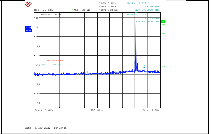
Band38-5MHz-16QAM-38225-1RB#0-Range2:1000~3000MHz
