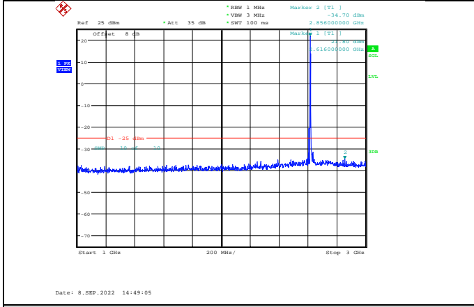
Band38-5MHz-64QAM-38225-1RB#0-Range2:1000~3000MHz
