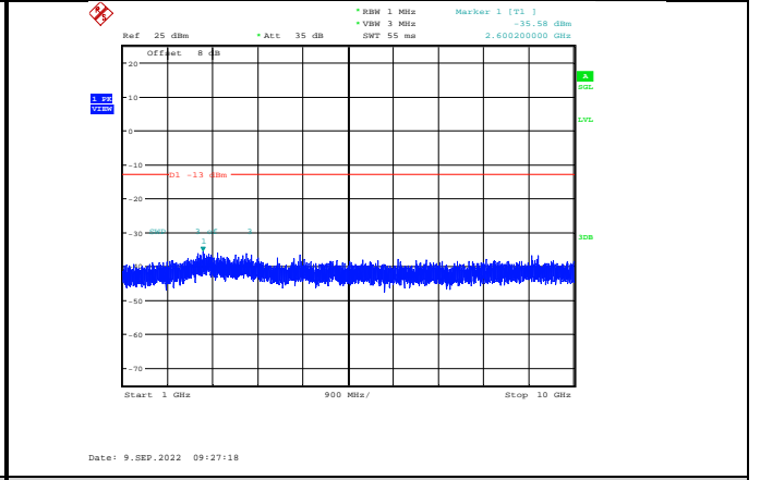
Band13-5MHz-16QAM-23255-1RB#0-Range2:1000~10000MHz
