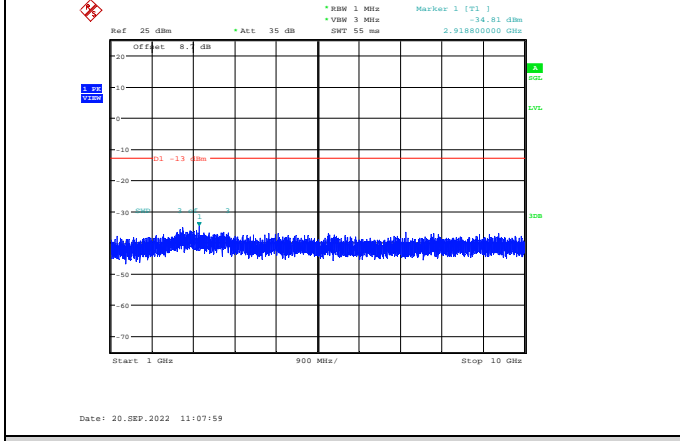
Band12-10MHz-64QAM-23060-1RB#0- Range2:1000~10000MHz
