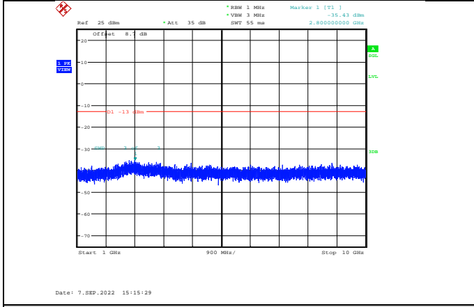
Band12-5MHz-16QAM-23035-1RB#0-Range2:1000~10000MHz
