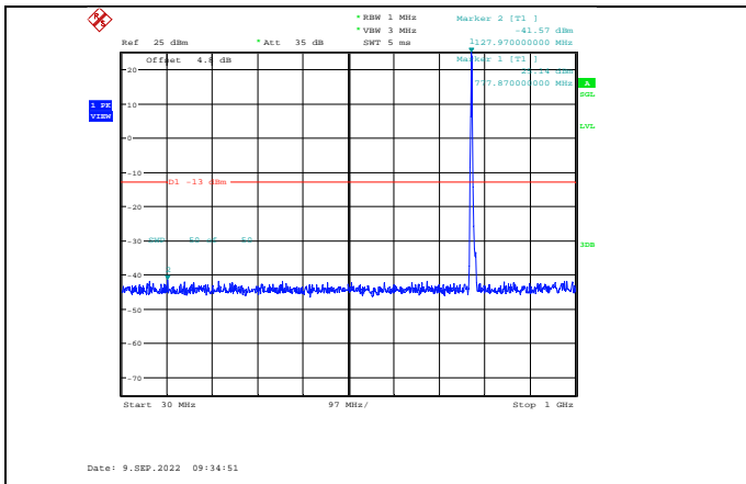
Band13-5MHz-64QAM-23205-1RB#0-Range1:30~1000MHz
