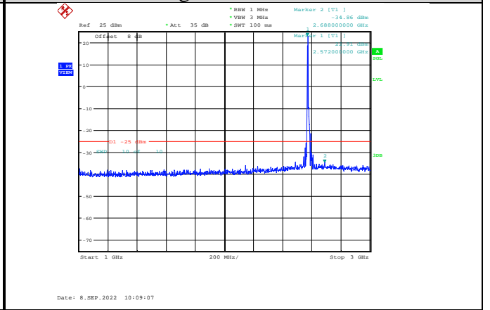
Band38-15MHz-16QAM-37825-1RB#0-Range2:1000~3000MHz
