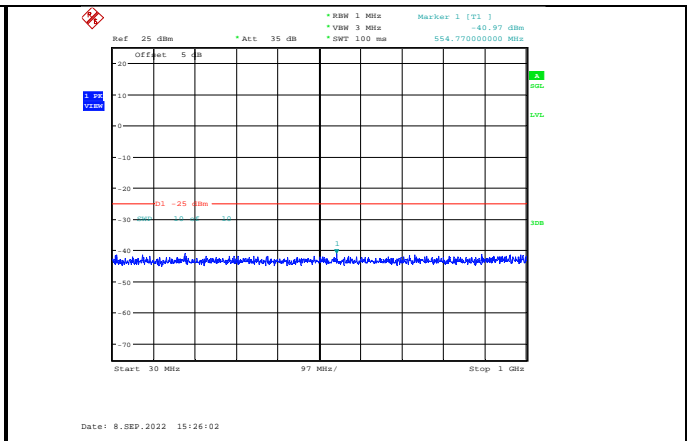
Band41-10MHz-64QAM-41190-1RB#0- Range1:30~1000MHz
