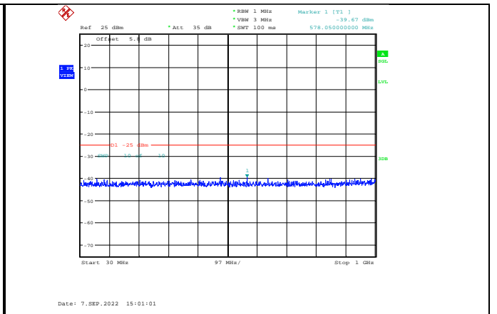
Band7-20MHz-QPSK-20850-1RB#0-Range1:30~1000MHz
