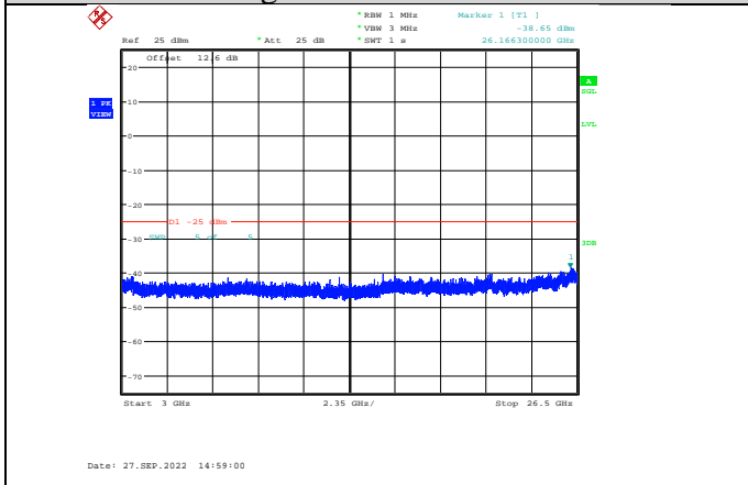
Band7-15MHz-QPSK-21375-1RB#0- Range3:3000~26500MHz
