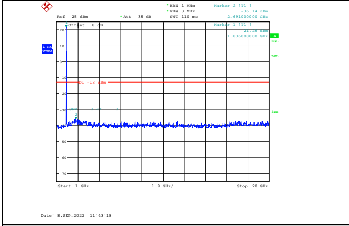
Band2-15MHz-64QAM-18675-1RB#0-Range2:1000~20000MHz
