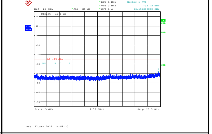
Band7-15MHz-16QAM-21375-1RB#0-Range3:3000~26500MHz
