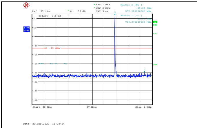
Band12-3MHz-64QAM-23025-1RB#0- Range1:30~1000MHz
