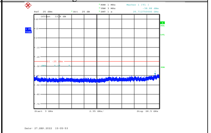
Band7-5MHz-64QAM-21100-1RB#0- Range3:3000~26500MHz
