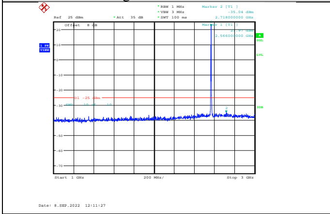
Band7-5MHz-64QAM-21425-1RB#0-Range2:1000~3000MHz
