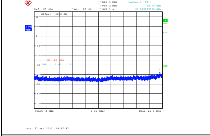
Band7-15MHz-64QAM-20825-1RB#0-Range3:3000~26500MHz
