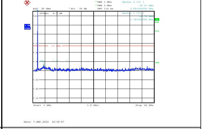
Band4-15MHz-16QAM-20325-1RB#0-Range2:1000~20000MHz
