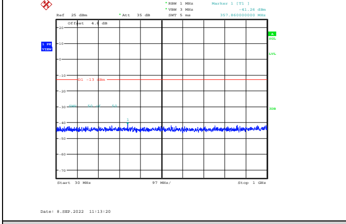
Band4-5MHz-64QAM-20175-1RB#0-Range1:30~1000MHz
