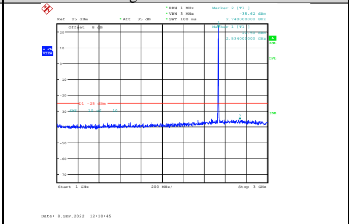
Band7-5MHz-64QAM-21100-1RB#0- Range2:1000~3000MHz
