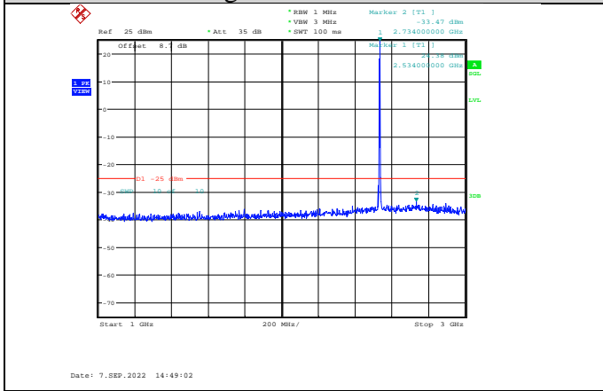
Band7-5MHz-16QAM-21100-1RB#0- Range2:1000~3000MHz
