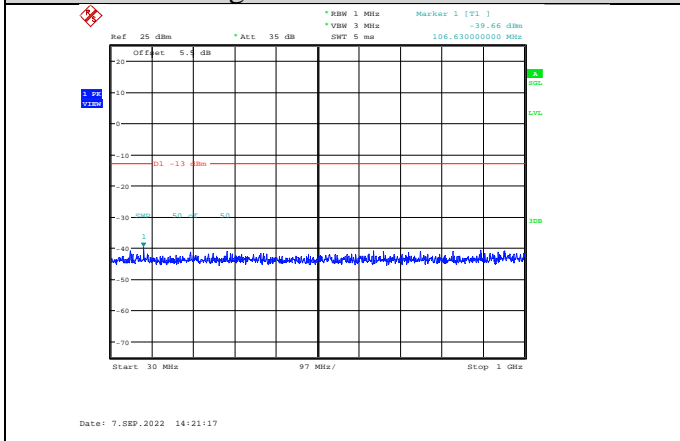
Band4-3MHz-16QAM-20175-1RB#0- Range1:30~1000MHz
