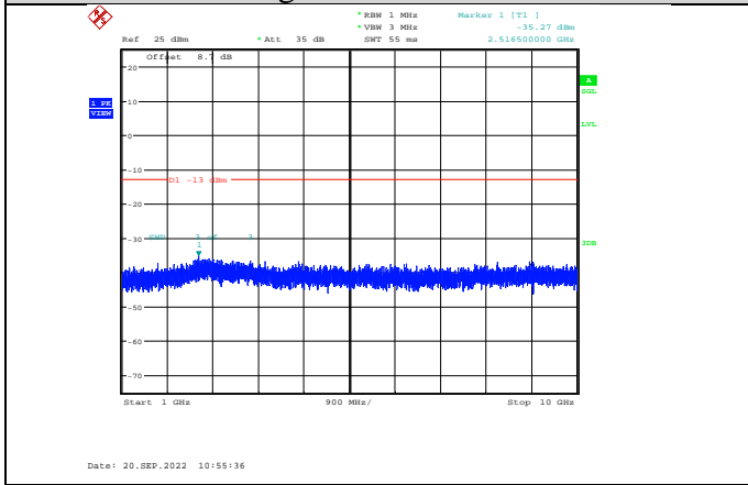
Band12-1.4MHz-64QAM-23017-1RB#0- Range2:1000~10000MHz
