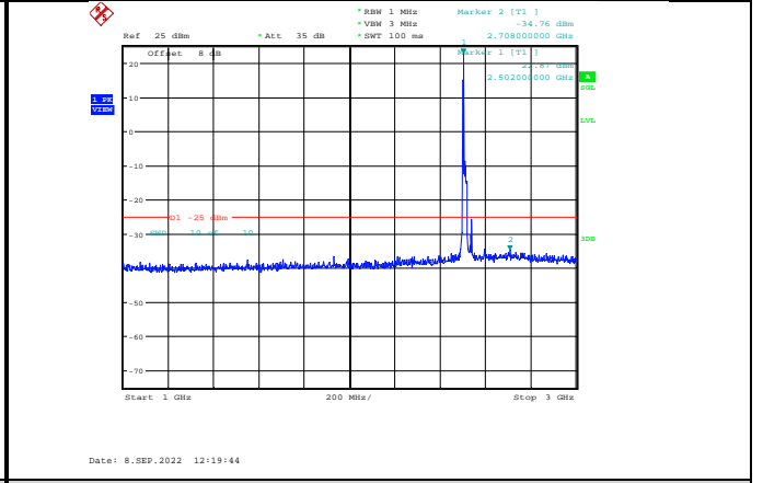
Band7-20MHz-64QAM-20850-1RB#0-Range2:1000~3000MHz
