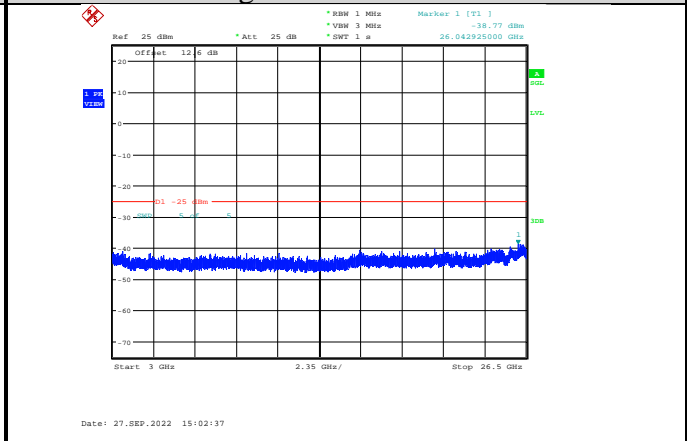
Band7-10MHz-QPSK-21400-1RB#0-Range3:3000~26500MHz
