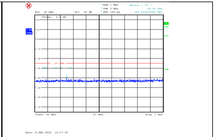
Band7-15MHz-64QAM-21100-1RB#0-Range1:30~1000MHz
