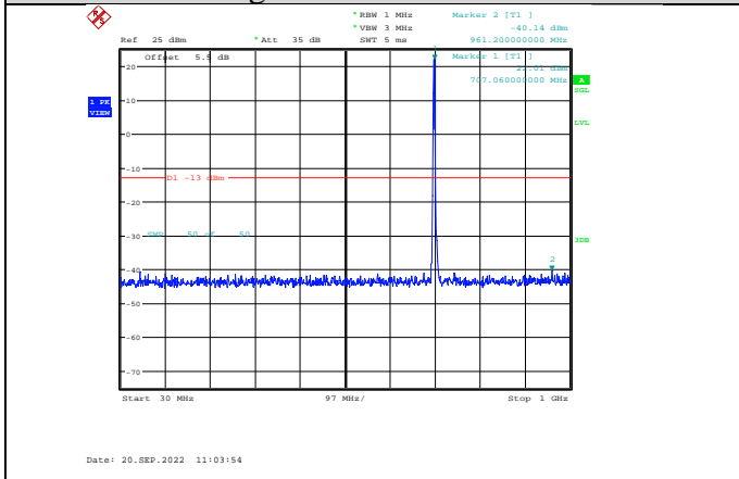
Band12-3MHz-64QAM-23095-1RB#0- Range1:30~1000MHz
