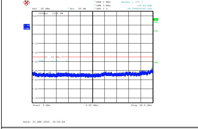
Band7-10MHz-16QAM-20800-1RB#0-Range3:3000~26500MHz
