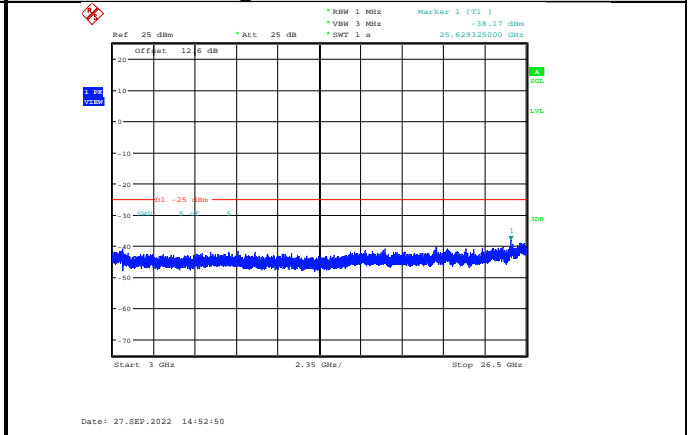
Band7-20MHz-16QAM-21100-1RB#0-Range3:3000~26500MHz
