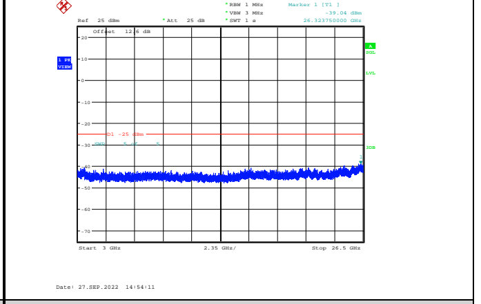
Band7-20MHz-64QAM-21350-1RB#0-Range3:3000~26500MHz
