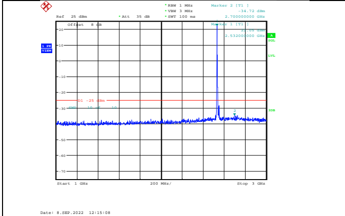
Band7-10MHz-64QAM-21100-1RB#0-Range2:1000~3000MHz
