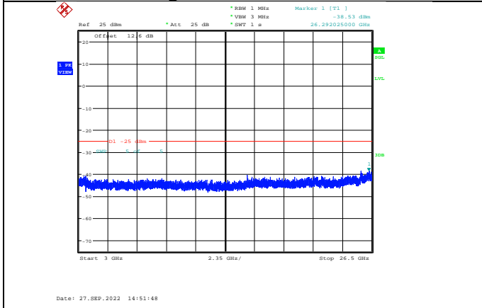
Band7-20MHz-16QAM-20850-1RB#0-Range3:3000~26500MHz
