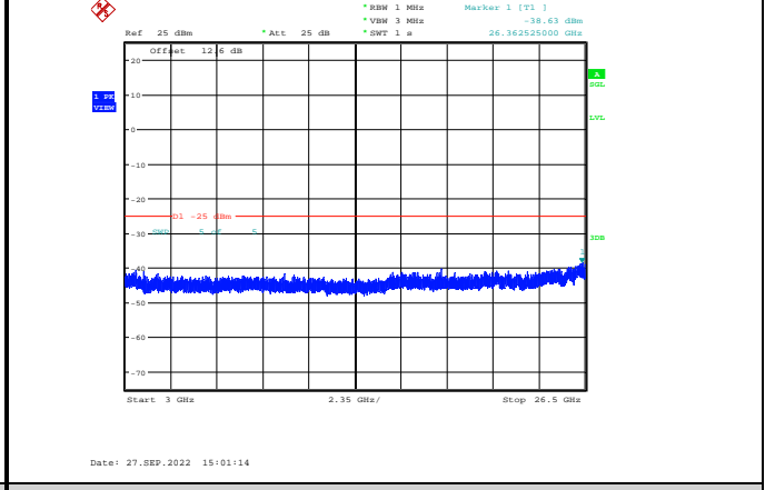
Band7-10MHz-64QAM-20800-1RB#0-Range3:3000~26500MHz
