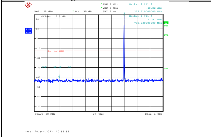
Band12-1.4MHz-64QAM-23095-1RB#0- Range1:30~1000MHz
