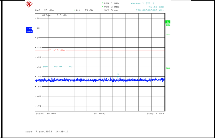
Band4-10MHz-16QAM-20350-1RB#0-Range1:30~1000MHz
