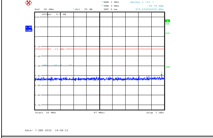
Band4-10MHz-16QAM-20175-1RB#0-Range1:30~1000MHz
