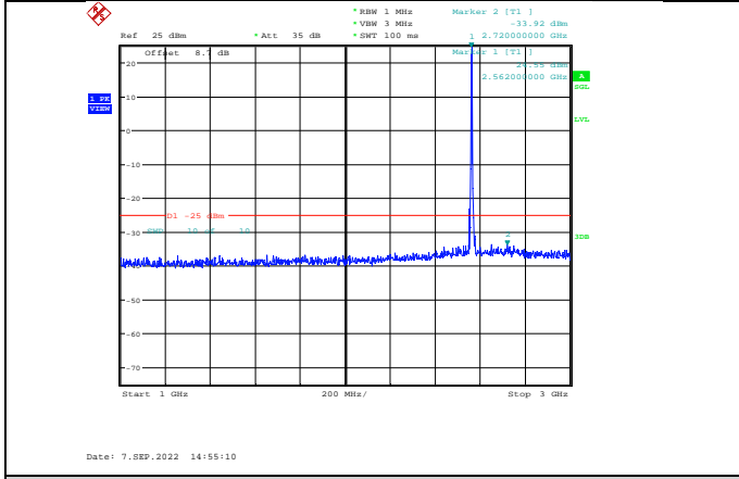
Band7-10MHz-16QAM-21400-1RB#0-Range2:1000~3000MHz
