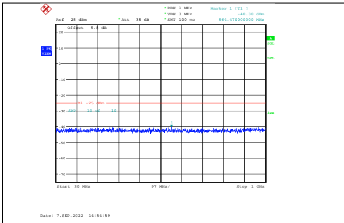
Band7-10MHz-16QAM-21400-1RB#0-Range1:30~1000MHz
