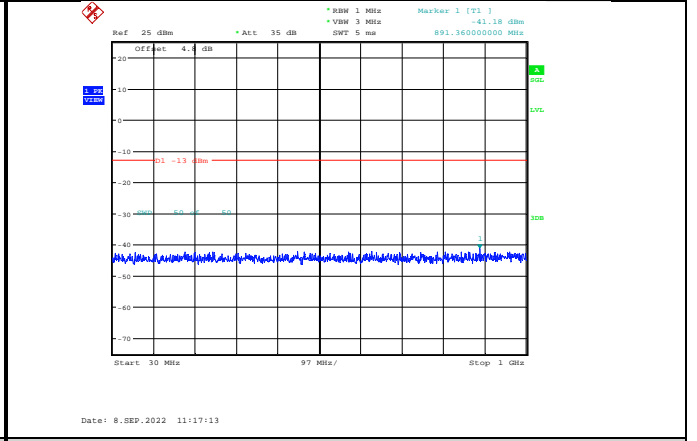
Band4-10MHz-64QAM-20350-1RB#0-Range1:30~1000MHz
