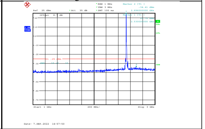
Band7-15MHz-QPSK-21100-1RB#0-Range2:1000~3000MHz
