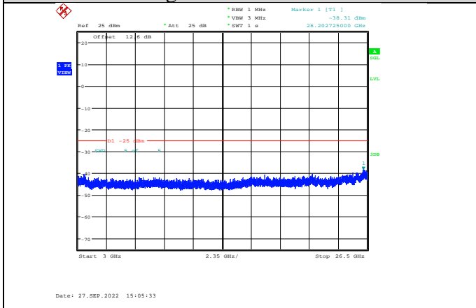
Band7-5MHz-16QAM-21100-1RB#0- Range3:3000~26500MHz
