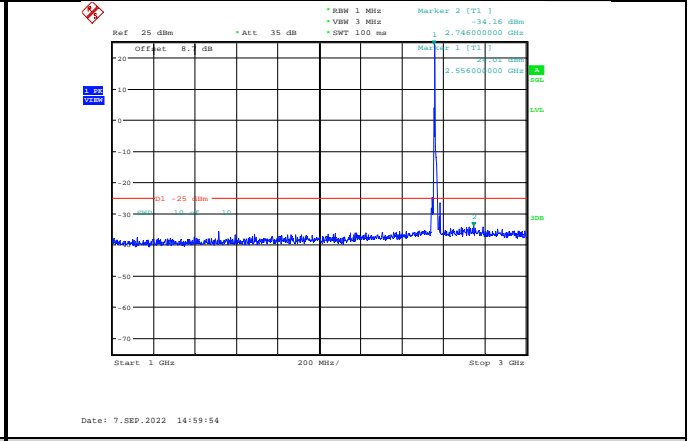
Band7-15MHz-16QAM-21375-1RB#0-Range2:1000~3000MHz
