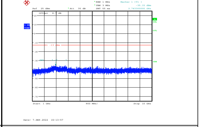
Band12-3MHz-16QAM-23165-1RB#0- Range2:1000~10000MHz
