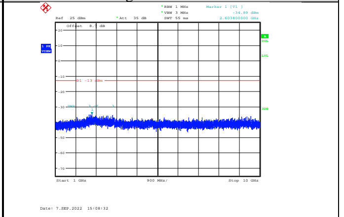
Band12-1.4MHz-16QAM-23173-1RB#0- Range2:1000~10000MHz
