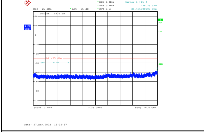
Band7-10MHz-16QAM-21400-1RB#0-Range3:3000~26500MHz
