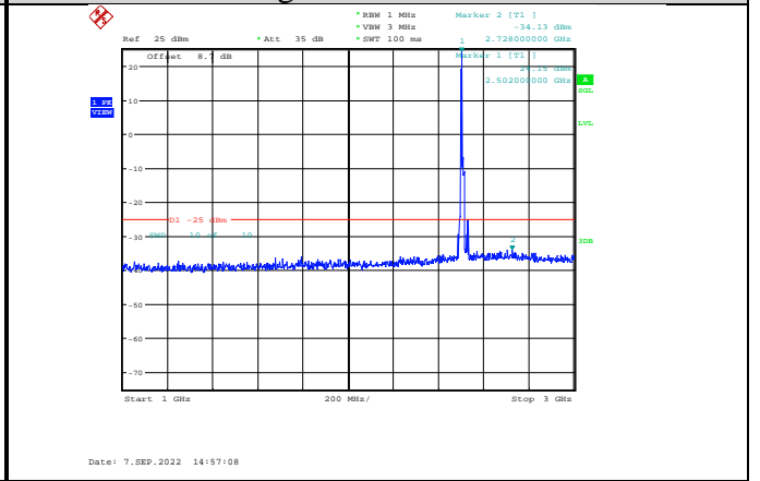
Band7-15MHz-16QAM-20825-1RB#0- Range2:1000~3000MHz
