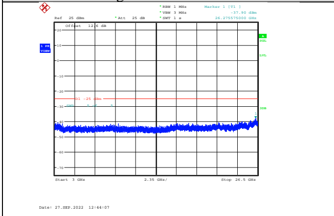
Band7-5MHz-QPSK-20775-1RB#0-Range3:3000~26500MHz
