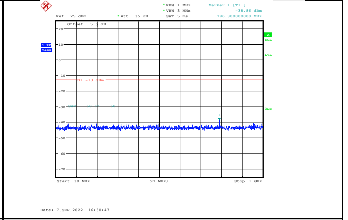
Band4-15MHz-16QAM-20325-1RB#0-Range1:30~1000MHz
