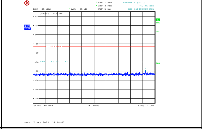
Band4-1.4MHz-16QAM-20393-1RB#0-Range1:30~1000MHz
