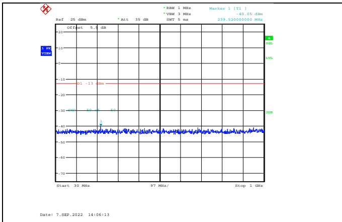
Band2-20MHz-16QAM-18700-1RB#0-Range1:30~1000MHz
