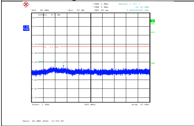
Band12-3MHz-64QAM-23025-1RB#0- Range2:1000~10000MHz
