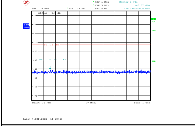
Band4-3MHz-QPSK-20175-1RB#0-Range1:30~1000MHz
