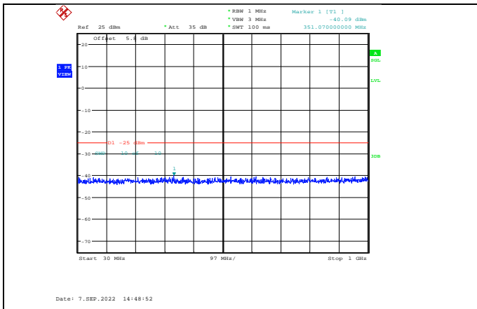
Band7-5MHz-16QAM-21100-1RB#0- Range1:30~1000MHz
