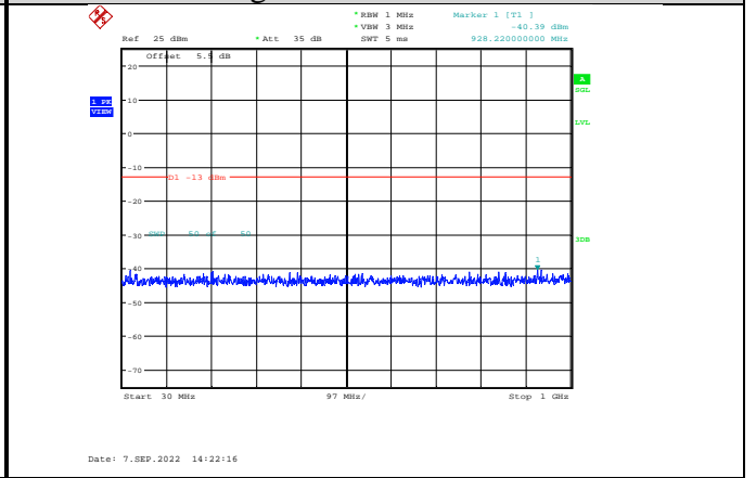
Band4-3MHz-16QAM-20385-1RB#0- Range1:30~1000MHz
