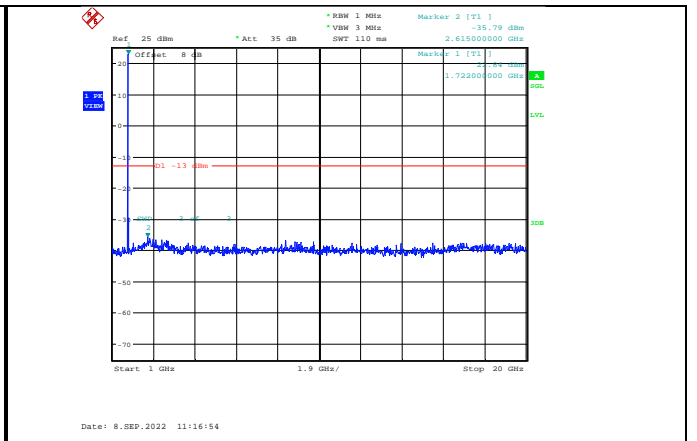
Band4-10MHz-64QAM-20175-1RB#0-Range2:1000~20000MHz
