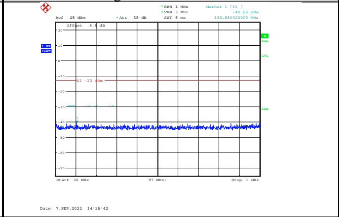
Band4-5MHz-16QAM-20375-1RB#0- Range1:30~1000MHz
