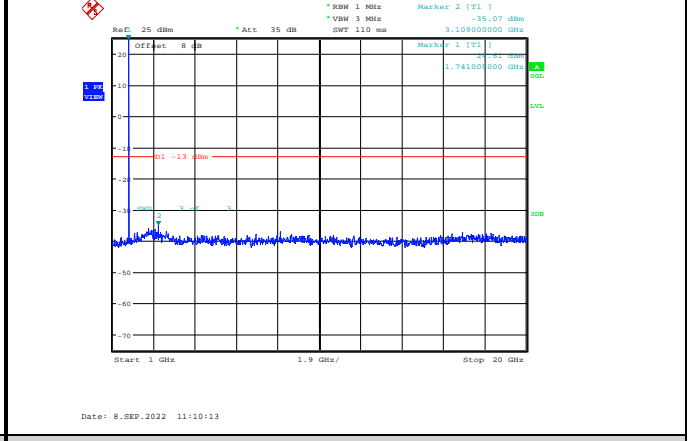
Band4-3MHz-64QAM-20385-1RB#0-Range2:1000~20000MHz
