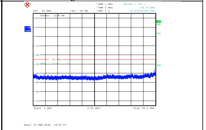
Band7-15MHz-16QAM-20825-1RB#0- Range3:3000~26500MHz
