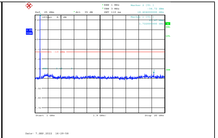
Band4-15MHz-16QAM-20175-1RB#0-Range2:1000~20000MHz
