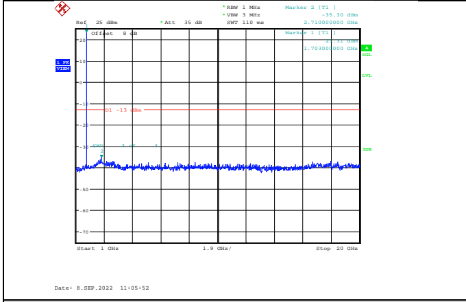
Band4-1.4MHz-64QAM-19957-1RB#0-Range2:1000~20000MHz
