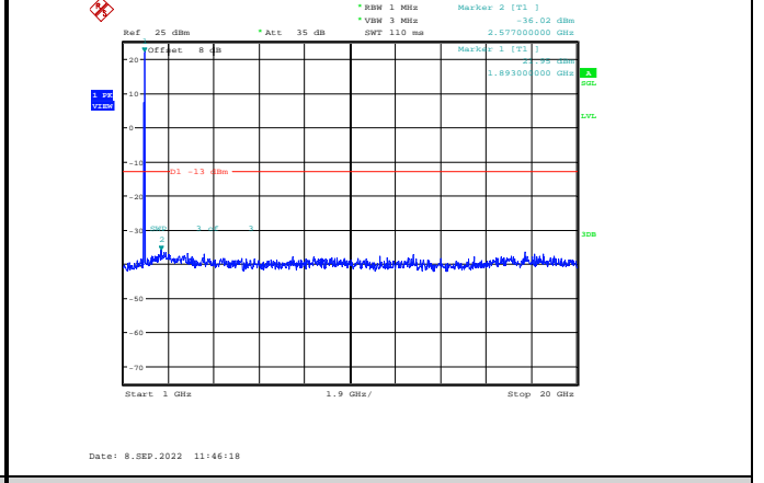
Band2-20MHz-64QAM-19100-1RB#0-Range2:1000~20000MHz
