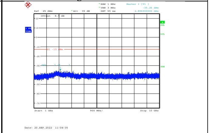
Band12-3MHz-64QAM-23165-1RB#0- Range2:1000~10000MHz
