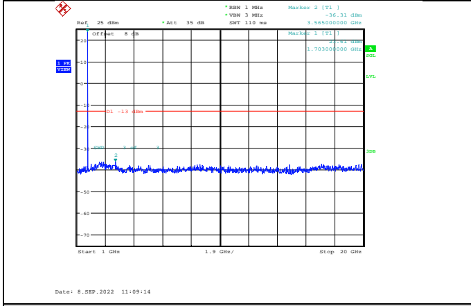
Band4-3MHz-64QAM-19965-1RB#0-Range2:1000~20000MHz
