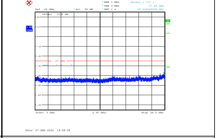
Band7-15MHz-64QAM-21100-1RB#0-Range3:3000~26500MHz
