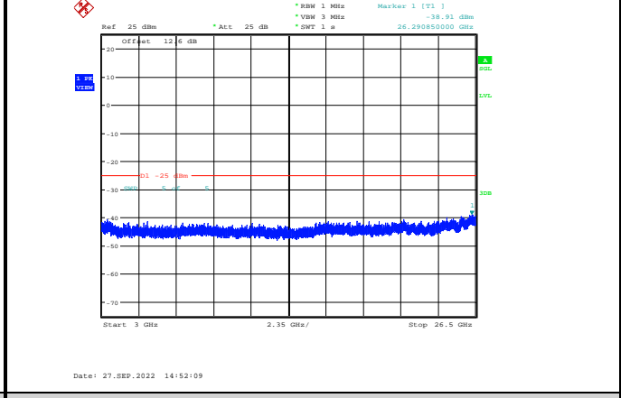
Band7-20MHz-64QAM-20850-1RB#0-Range3:3000~26500MHz
