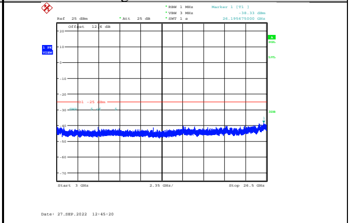
Band7-5MHz-QPSK-21100-1RB#0-Range3:3000~26500MHz
