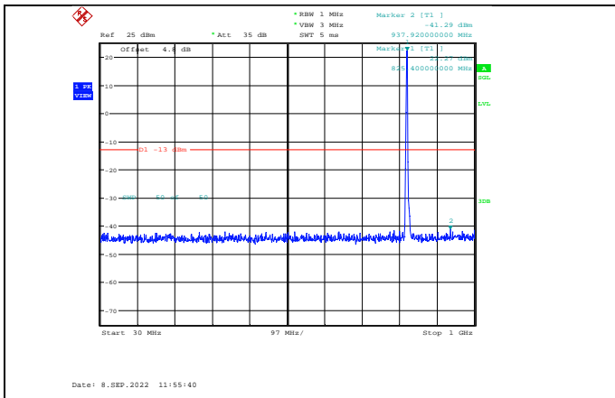
Band5-3MHz-64QAM-20415-1RB#0- Range1:30~1000MHz
