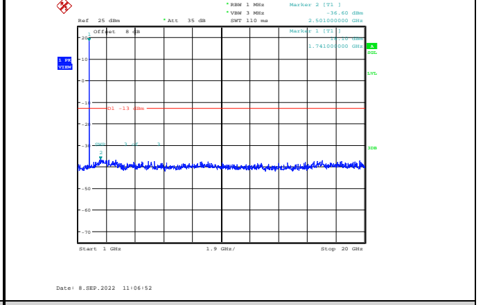
Band4-1.4MHz-64QAM-20393-1RB#0-Range2:1000~20000MHz
