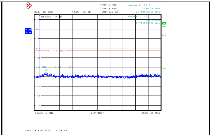
Band4-3MHz-64QAM-20175-1RB#0-Range2:1000~20000MHz
