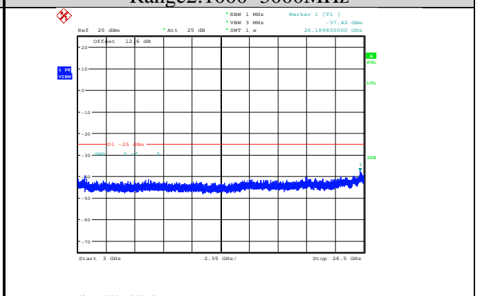
Band7-10MHz-64QAM-21400-1RB#0-Range3:3000~26500MHz
