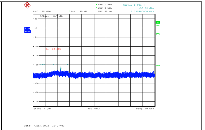
Band12-1.4MHz-QPSK-23095-1RB#0-Range2:1000~10000MHz
