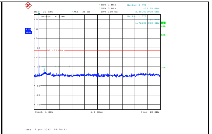
Band4-10MHz-16QAM-20175-1RB#0-Range2:1000~20000MHz
