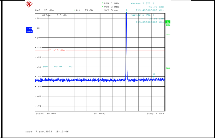
Band12-3MHz-16QAM-23165-1RB#0- Range1:30~1000MHz
