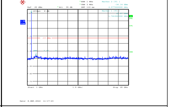
Band4-10MHz-64QAM-20350-1RB#0-Range2:1000~20000MHz
