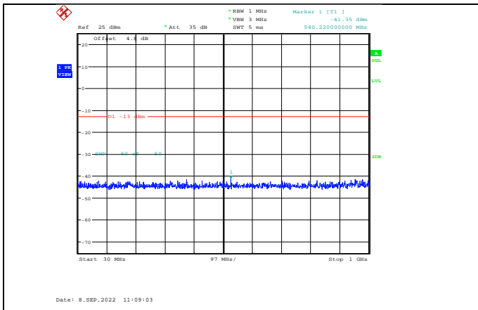
Band4-3MHz-64QAM-19965-1RB#0-Range1:30~1000MHz
