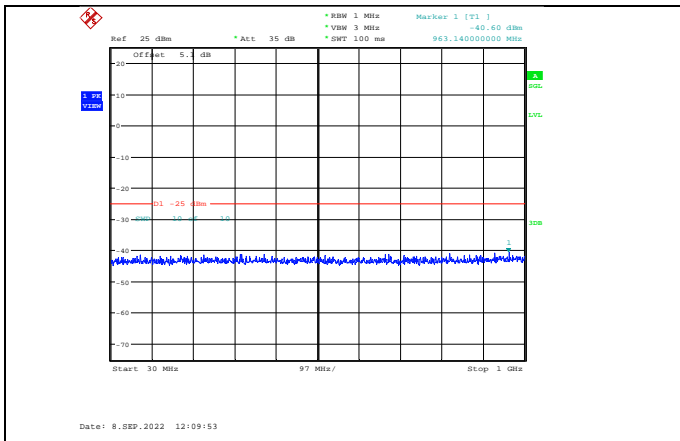
Band7-5MHz-64QAM-20775-1RB#0- Range1:30~1000MHz
