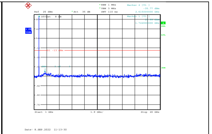
Band4-5MHz-64QAM-20175-1RB#0-Range2:1000~20000MHz
