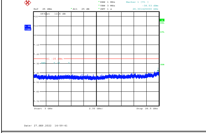
Band7-15MHz-64QAM-21375-1RB#0-Range3:3000~26500MHz
