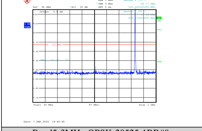
Band5-3MHz-QPSK-20525-1RB#0-Range1:30~1000MHz
