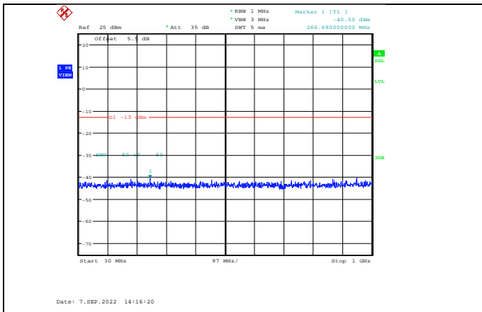
Band4-1.4MHz-QPSK-19957-1RB#0-Range1:30~1000MHz
