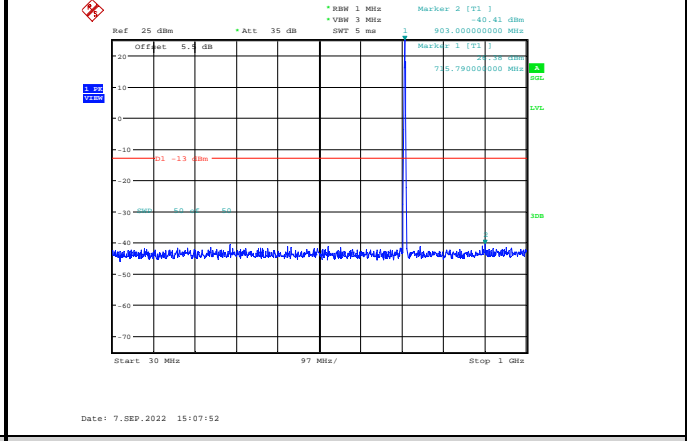
Band12-1.4MHz-QPSK-23173-1RB#0-Range1:30~1000MHz
