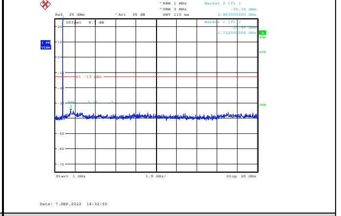
Band4-20MHz-16QAM-20300-1RB#0-Range2:1000~20000MHz
