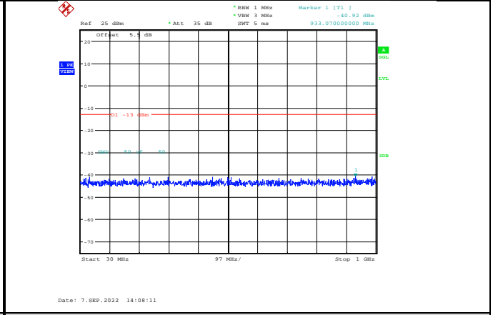
Band2-20MHz-16QAM-19100-1RB#0-Range1:30~1000MHz
