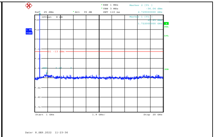
Band4-20MHz-64QAM-20175-1RB#0-Range2:1000~20000MHz
