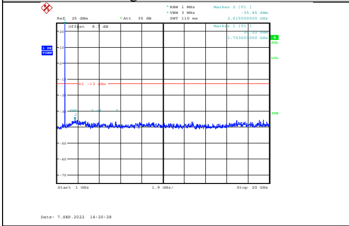
Band4-3MHz-16QAM-19965-1RB#0- Range2:1000~20000MHz
