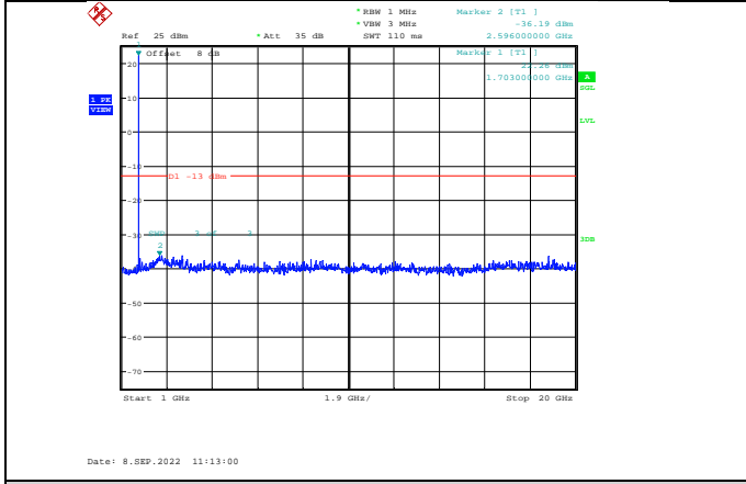
Band4-5MHz-64QAM-19975-1RB#0-Range2:1000~20000MHz
