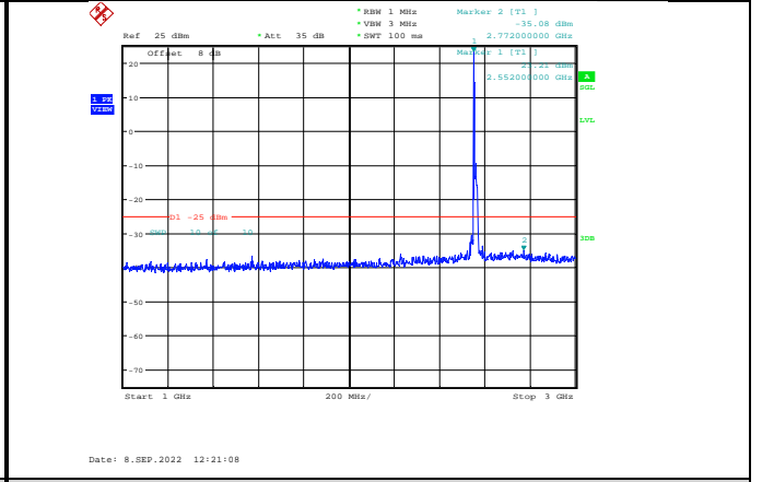
Band7-20MHz-64QAM-21350-1RB#0-Range2:1000~3000MHz
