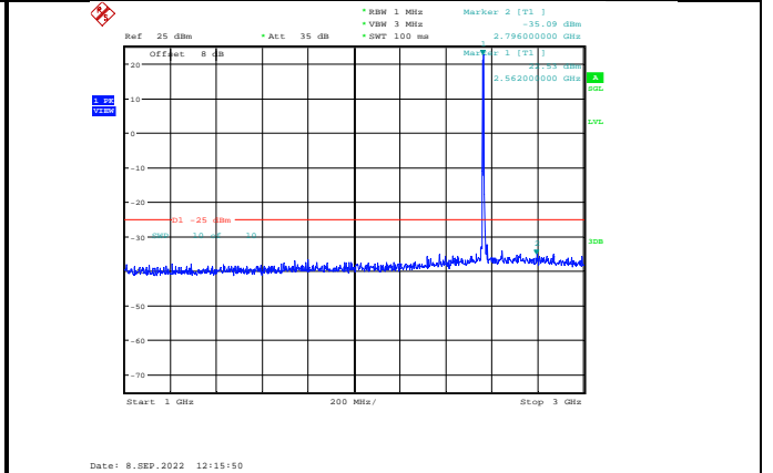
Band7-10MHz-64QAM-21400-1RB#0-Range2:1000~3000MHz
