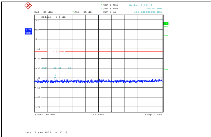
Band4-10MHz-16QAM-20000-1RB#0-Range1:30~1000MHz
