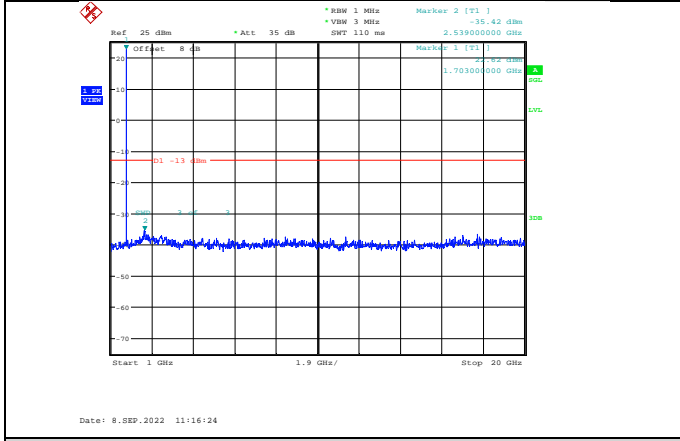
Band4-10MHz-64QAM-20000-1RB#0-Range2:1000~20000MHz
