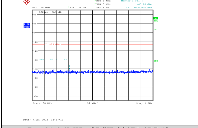
Band4-1.4MHz-QPSK-20175-1RB#0-Range1:30~1000MHz
