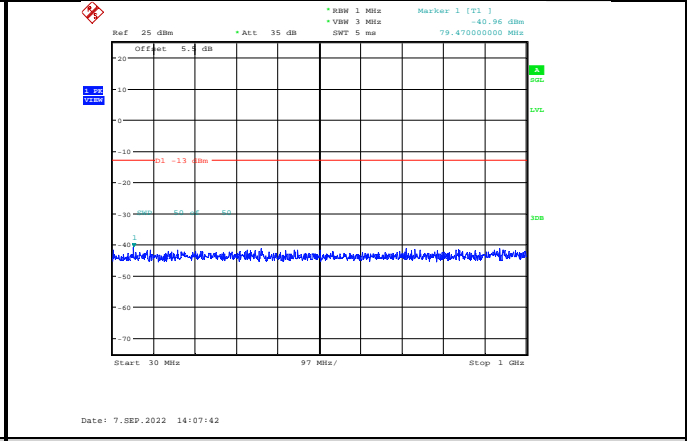
Band2-20MHz-QPSK-19100-1RB#0-Range1:30~1000MHz
