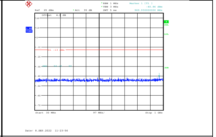
Band4-20MHz-64QAM-20300-1RB#0-Range1:30~1000MHz
