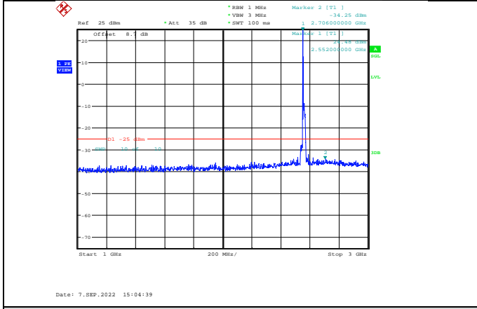
Band7-20MHz-16QAM-21350-1RB#0-Range2:1000~3000MHz
