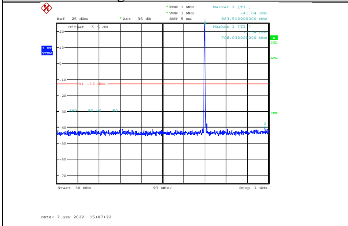
Band12-1.4MHz-16QAM-23095-1RB#0- Range1:30~1000MHz
