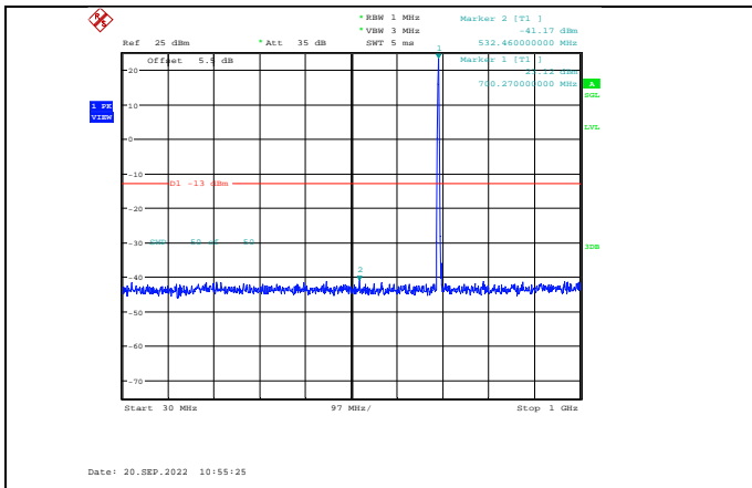
Band12-1.4MHz-64QAM-23017-1RB#0- Range1:30~1000MHz
