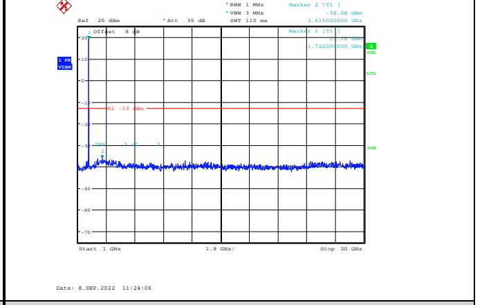
Band4-20MHz-64QAM-20300-1RB#0-Range2:1000~20000MHz
