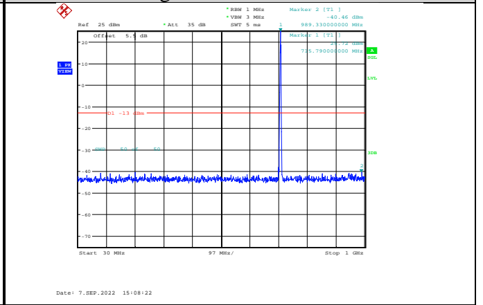
Band12-1.4MHz-16QAM-23173-1RB#0- Range1:30~1000MHz
