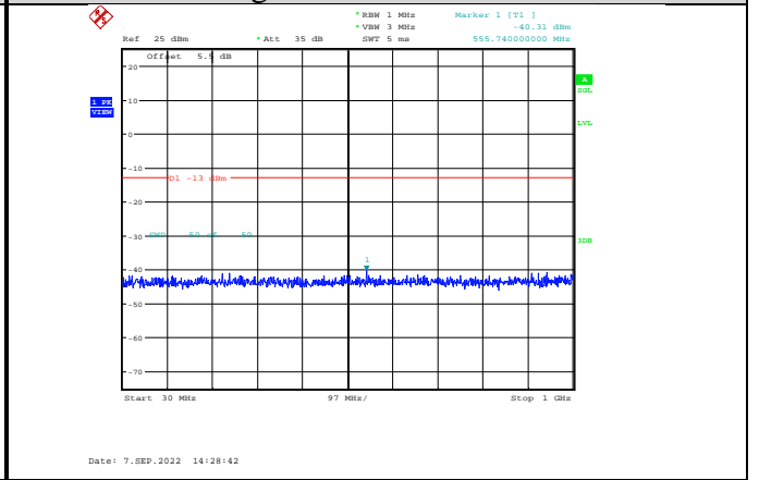
Band4-10MHz-QPSK-20350-1RB#0-Range1:30~1000MHz
