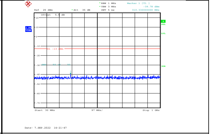
Band4-3MHz-QPSK-20385-1RB#0-Range1:30~1000MHz
