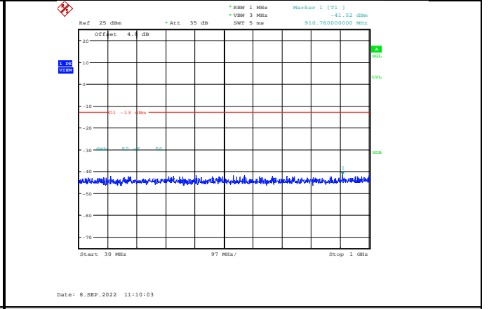
Band4-3MHz-64QAM-20385-1RB#0-Range1:30~1000MHz
