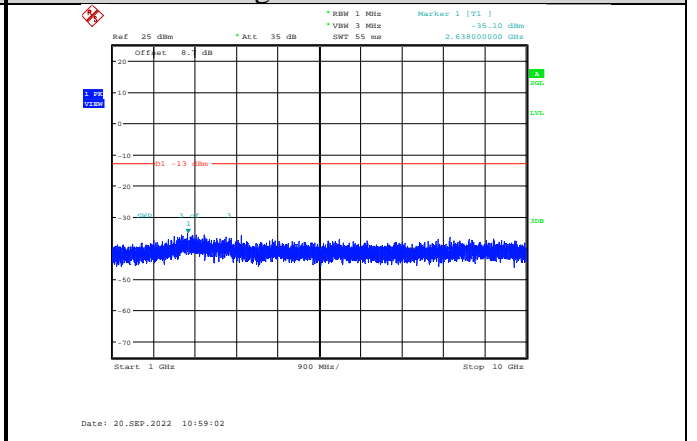
Band12-1.4MHz-64QAM-23173-1RB#0- Range2:1000~10000MHz
