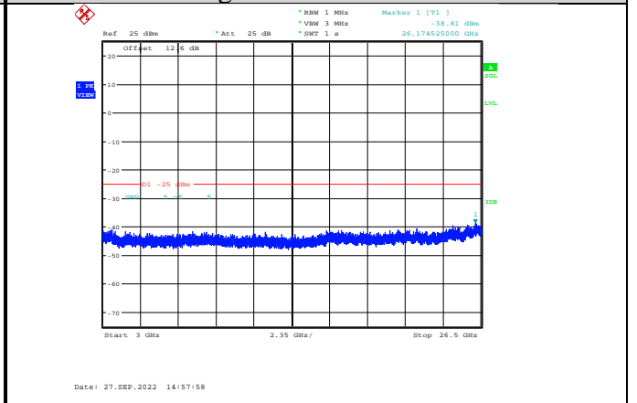
Band7-15MHz-QPSK-21100-1RB#0-Range3:3000~26500MHz
