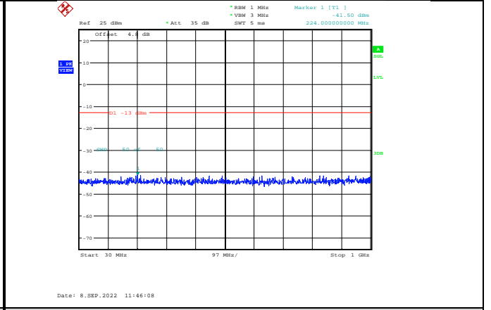
Band2-20MHz-64QAM-19100-1RB#0-Range1:30~1000MHz
