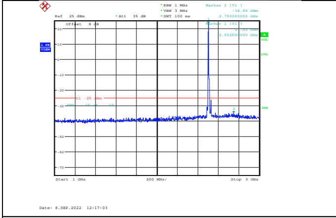
Band7-15MHz-64QAM-20825-1RB#0-Range2:1000~3000MHz
