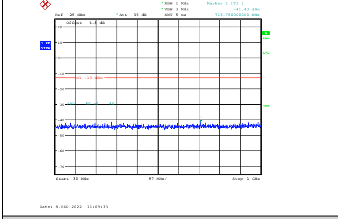
Band4-3MHz-64QAM-20175-1RB#0-Range1:30~1000MHz
