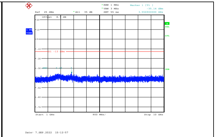
Band12-3MHz-16QAM-23095-1RB#0- Range2:1000~10000MHz
