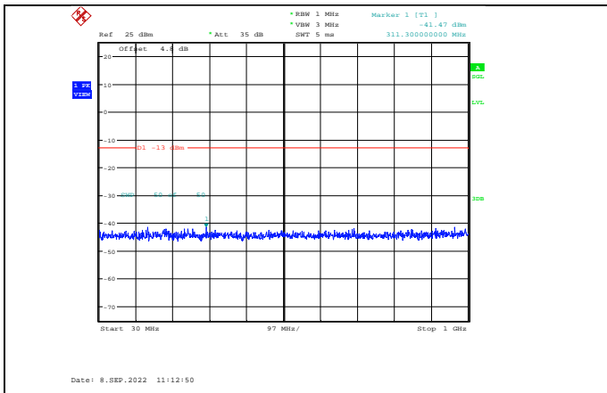
Band4-5MHz-64QAM-19975-1RB#0-Range1:30~1000MHz
