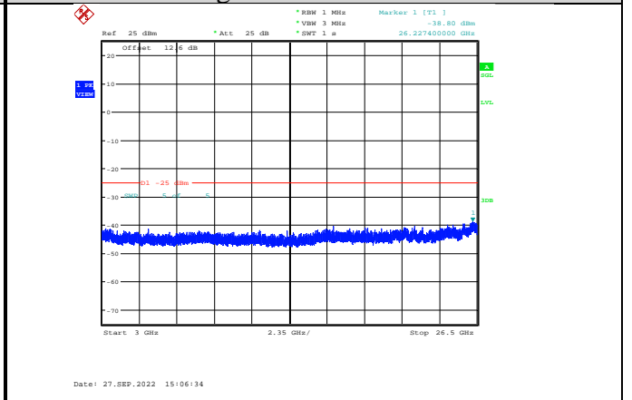
Band7-5MHz-16QAM-21425-1RB#0- Range3:3000~26500MHz
