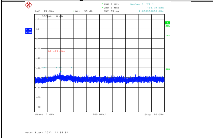
Band5-3MHz-64QAM-20415-1RB#0- Range2:1000~10000MHz
