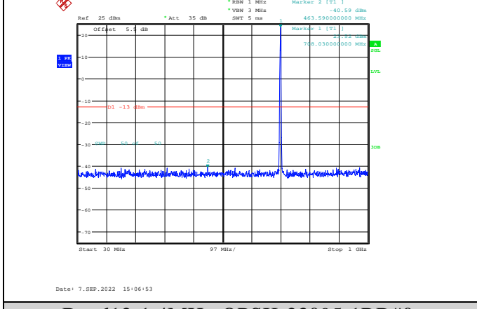
Band12-1.4MHz-QPSK-23095-1RB#0-Range1:30~1000MHz
