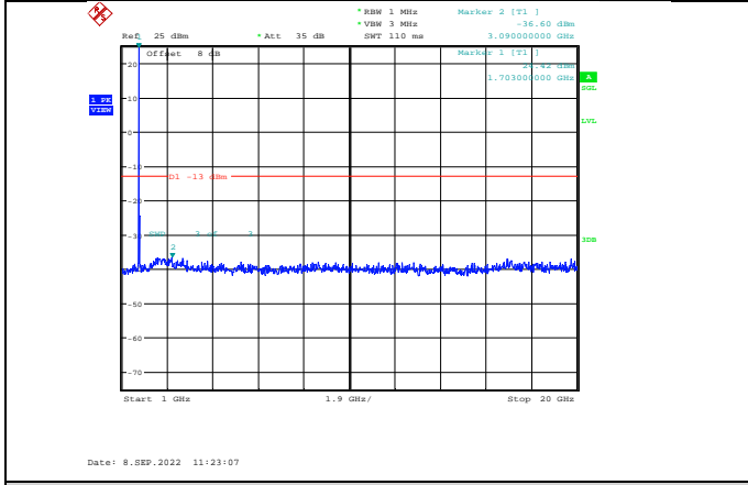
Band4-20MHz-64QAM-20050-1RB#0-Range2:1000~20000MHz
