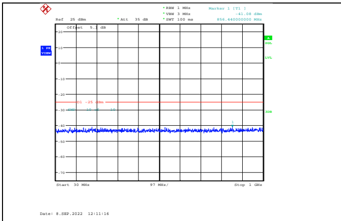
Band7-5MHz-64QAM-21425-1RB#0-Range1:30~1000MHz
