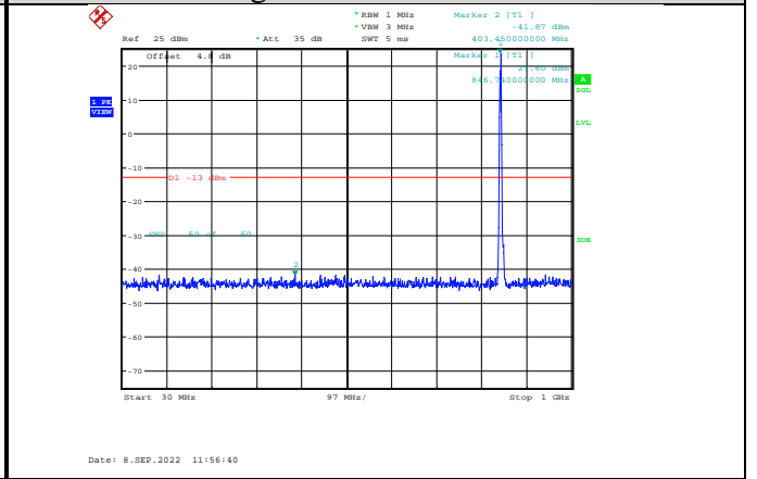
Band5-3MHz-64QAM-20635-1RB#0- Range1:30~1000MHz
