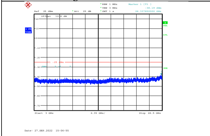
Band7-5MHz-64QAM-21425-1RB#0-Range3:3000~26500MHz
