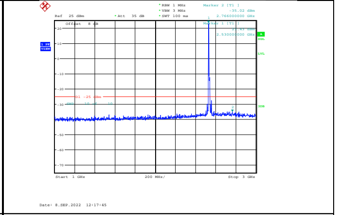
Band7-15MHz-64QAM-21100-1RB#0-Range2:1000~3000MHz
