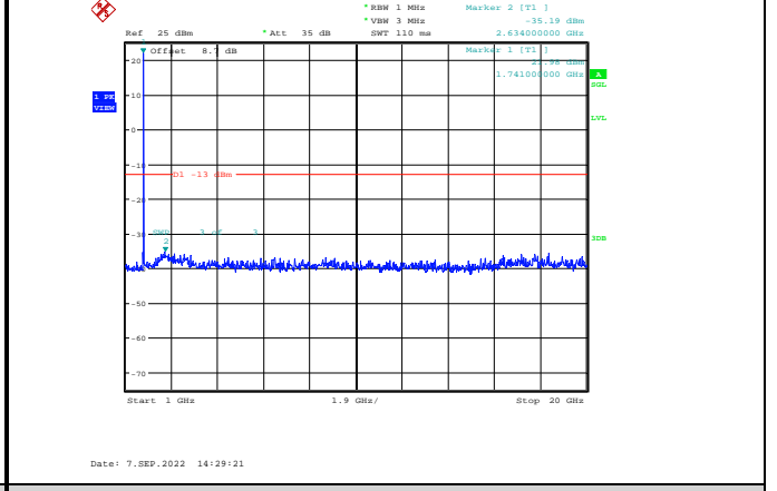
Band4-10MHz-16QAM-20350-1RB#0-Range2:1000~20000MHz
