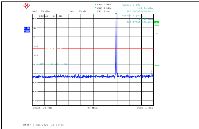
Band12-1.4MHz-16QAM-23017-1RB#0- Range1:30~1000MHz
