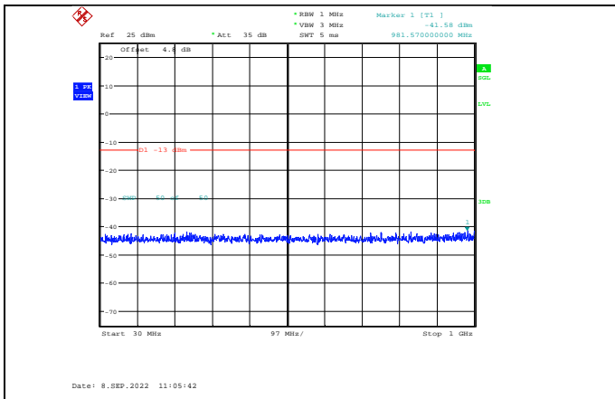
Band4-1.4MHz-64QAM-19957-1RB#0-Range1:30~1000MHz
