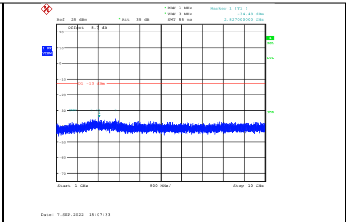
Band12-1.4MHz-16QAM-23095-1RB#0- Range2:1000~10000MHz
