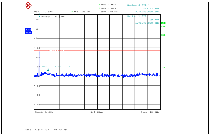
Band4-15MHz-QPSK-20175-1RB#0- Range2:1000~20000MHz
