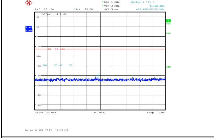
Band4-20MHz-64QAM-20175-1RB#0-Range1:30~1000MHz
