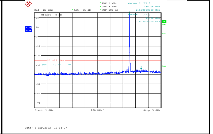
Band7-10MHz-64QAM-20800-1RB#0-Range2:1000~3000MHz
