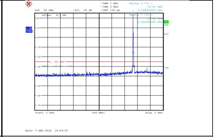
Band7-10MHz-16QAM-21100-1RB#0-Range2:1000~3000MHz
