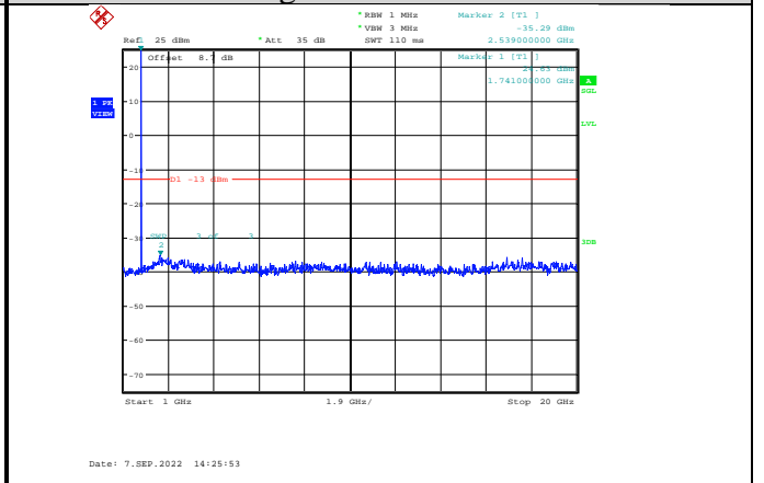
Band4-5MHz-16QAM-20375-1RB#0- Range2:1000~20000MHz
