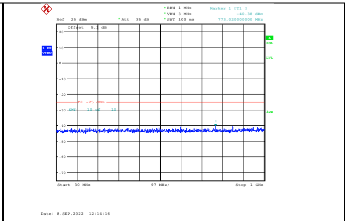
Band7-10MHz-64QAM-20800-1RB#0-Range1:30~1000MHz
