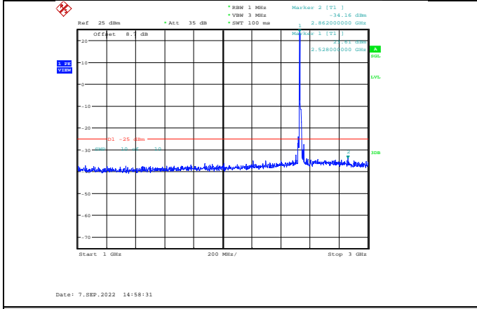
Band7-15MHz-16QAM-21100-1RB#0-Range2:1000~3000MHz
