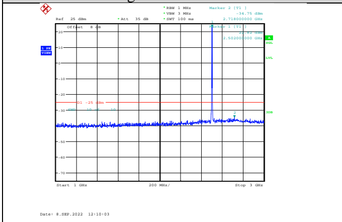
Band7-5MHz-64QAM-20775-1RB#0- Range2:1000~3000MHz
