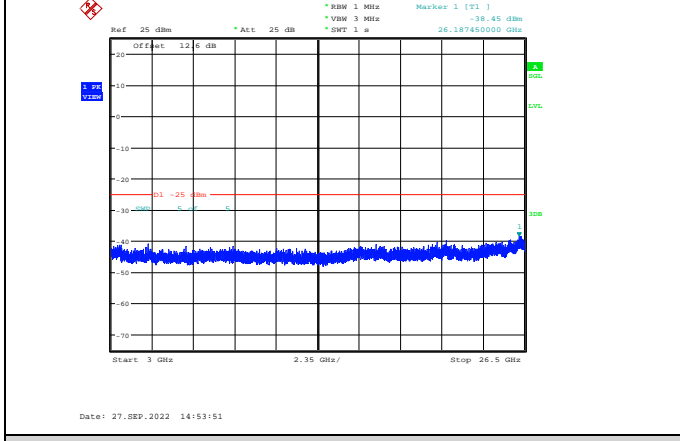
Band7-20MHz-16QAM-21350-1RB#0-Range3:3000~26500MHz
