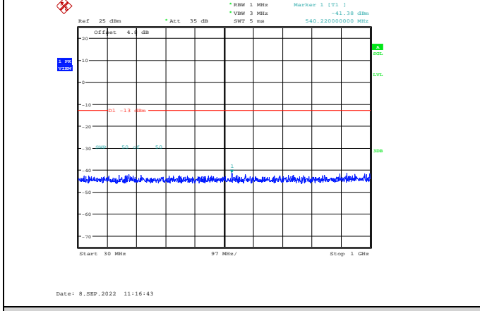
Band4-10MHz-64QAM-20175-1RB#0-Range1:30~1000MHz
