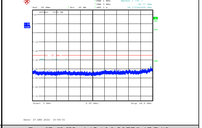
Band7-5MHz-16QAM-20775-1RB#0-Range3:3000~26500MHz
