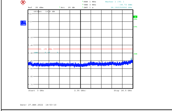
Band7-20MHz-64QAM-21100-1RB#0-Range3:3000~26500MHz
