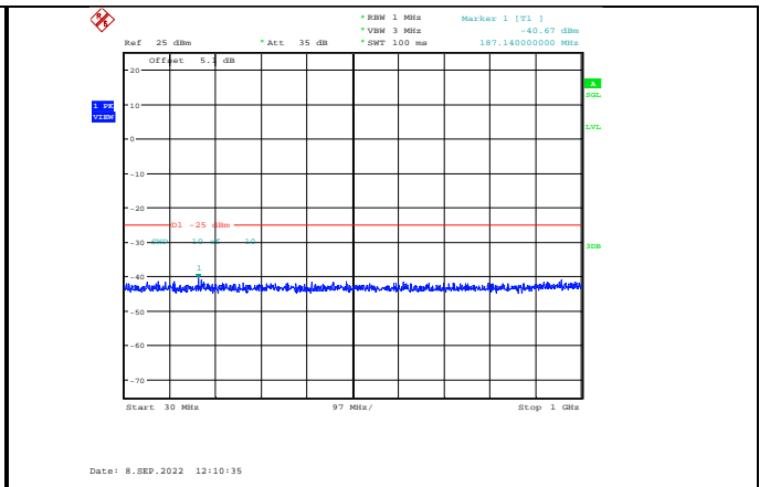
Band7-5MHz-64QAM-21100-1RB#0- Range1:30~1000MHz
