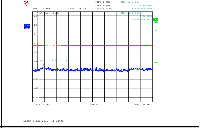
Band4-5MHz-64QAM-20375-1RB#0-Range2:1000~20000MHz
