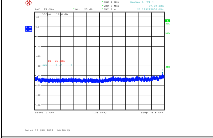
Band7-15MHz-16QAM-21100-1RB#0-Range3:3000~26500MHz
