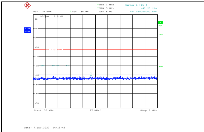
Band4-3MHz-QPSK-19965-1RB#0-Range1:30~1000MHz
