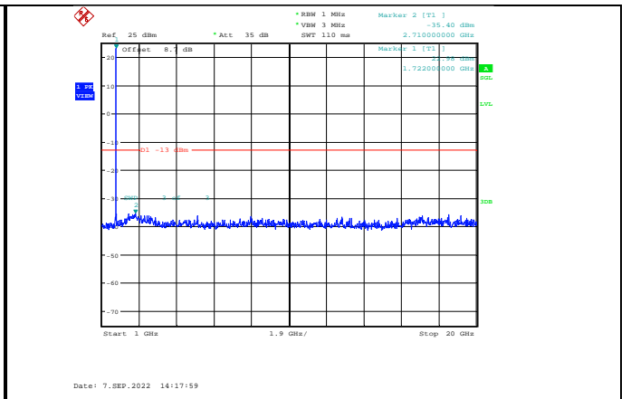
Band4-1.4MHz-16QAM-20175-1RB#0-Range2:1000~20000MHz
