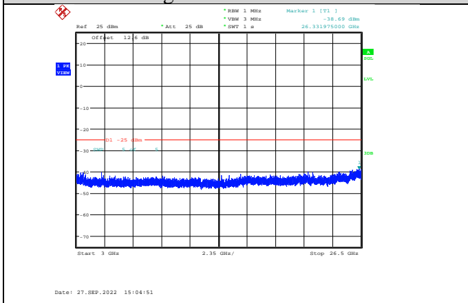
Band7-5MHz-64QAM-20775-1RB#0- Range3:3000~26500MHz
