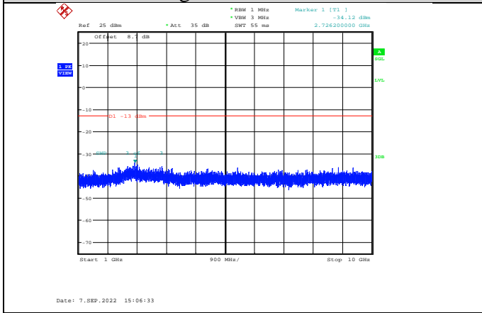
Band12-1.4MHz-16QAM-23017-1RB#0- Range2:1000~10000MHz
