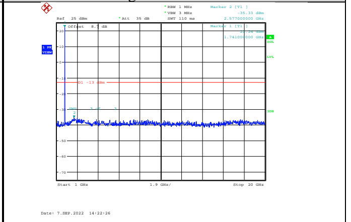
Band4-3MHz-16QAM-20385-1RB#0- Range2:1000~20000MHz
