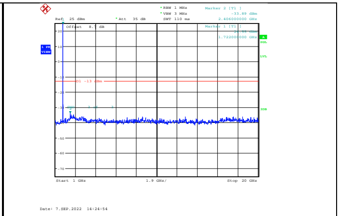
Band4-5MHz-16QAM-20175-1RB#0- Range2:1000~20000MHz
