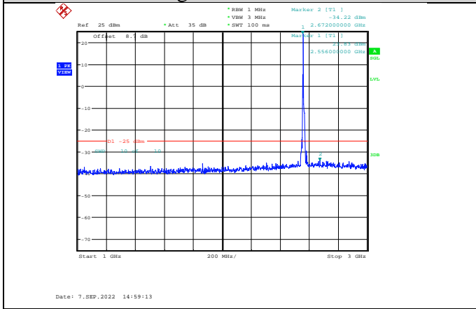
Band7-15MHz-QPSK-21375-1RB#0- Range2:1000~3000MHz
