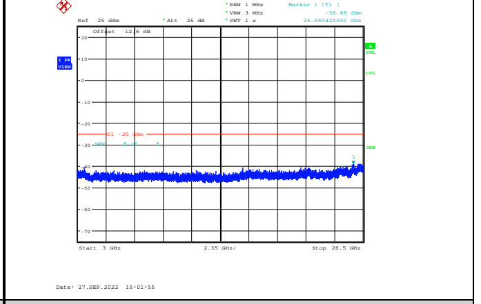
Band7-10MHz-16QAM-21100-1RB#0-Range3:3000~26500MHz
