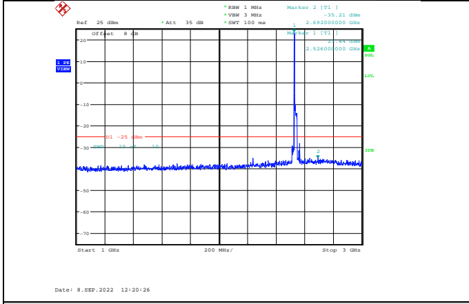
Band7-20MHz-64QAM-21100-1RB#0-Range2:1000~3000MHz
