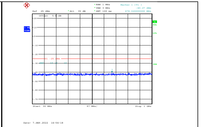
Band7-10MHz-QPSK-21400-1RB#0-Range1:30~1000MHz
