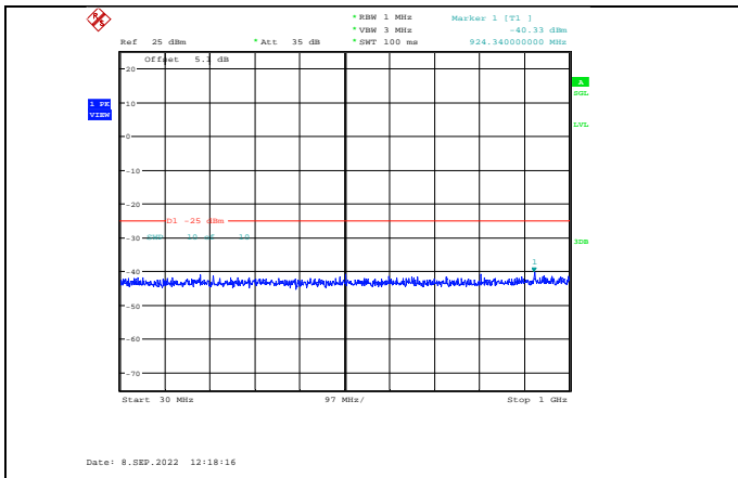
Band7-15MHz-64QAM-21375-1RB#0-Range1:30~1000MHz
