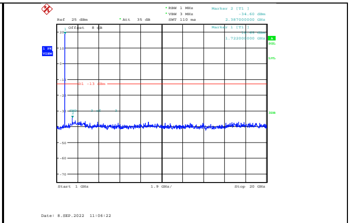
Band4-1.4MHz-64QAM-20175-1RB#0-Range2:1000~20000MHz
