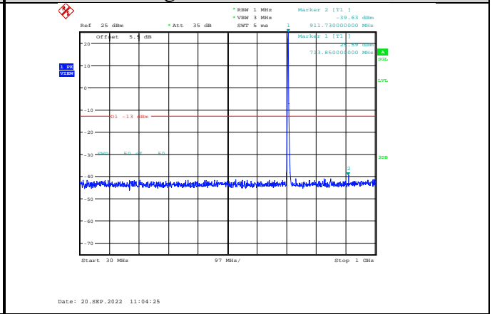
Band12-3MHz-64QAM-23165-1RB#0- Range1:30~1000MHz
