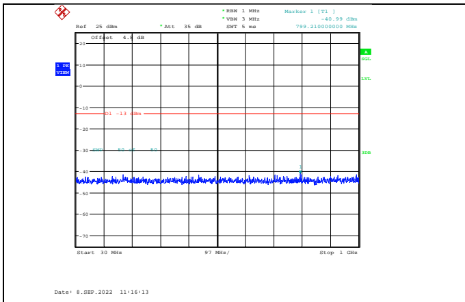
Band4-10MHz-64QAM-20000-1RB#0-Range1:30~1000MHz
