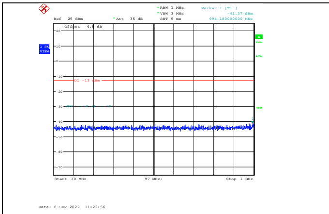
Band4-20MHz-64QAM-20050-1RB#0-Range1:30~1000MHz
