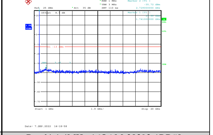
Band4-1.4MHz-16QAM-20393-1RB#0-Range2:1000~20000MHz
