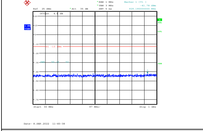
Band2-20MHz-64QAM-18900-1RB#0-Range1:30~1000MHz
