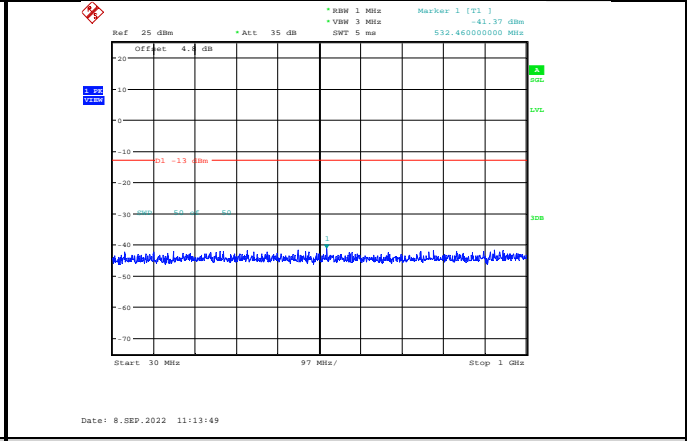
Band4-5MHz-64QAM-20375-1RB#0-Range1:30~1000MHz
