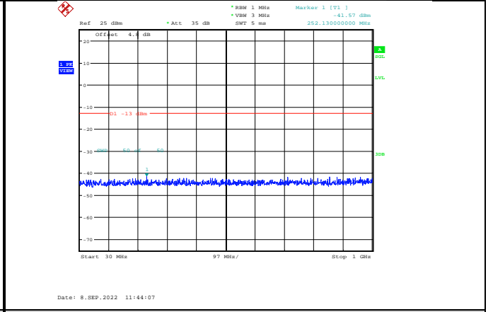
Band2-15MHz-64QAM-19125-1RB#0-Range1:30~1000MHz
