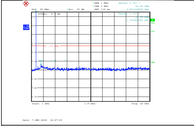
Band4-10MHz-16QAM-20000-1RB#0-Range2:1000~20000MHz
