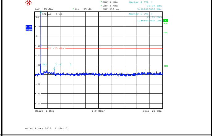
Band2-15MHz-64QAM-19125-1RB#0-Range2:1000~20000MHz
