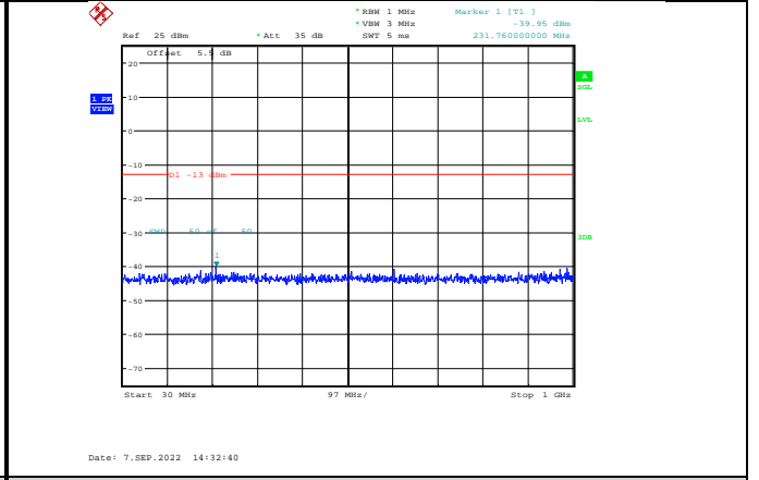
Band4-20MHz-16QAM-20300-1RB#0-Range1:30~1000MHz
