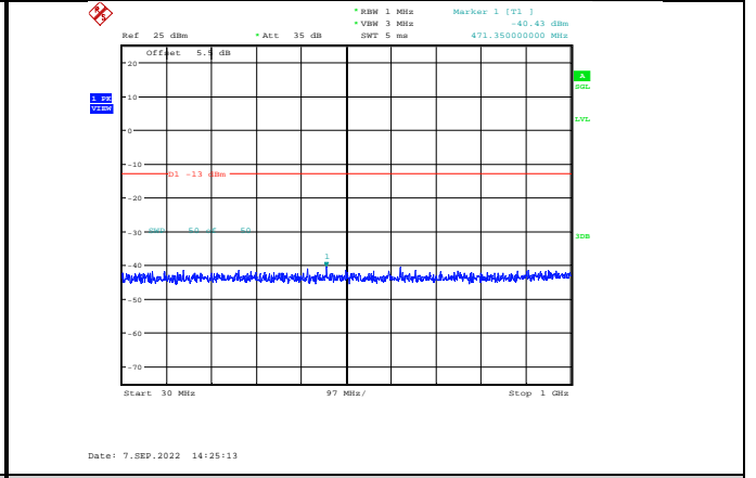
Band4-5MHz-QPSK-20375-1RB#0-Range1:30~1000MHz
