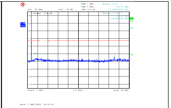
Band4-20MHz-16QAM-20175-1RB#0-Range2:1000~20000MHz
