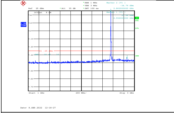
Band7-15MHz-64QAM-21375-1RB#0-Range2:1000~3000MHz
