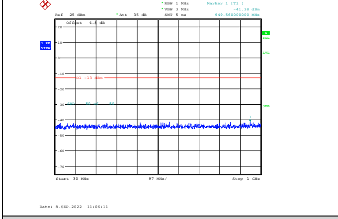
Band4-1.4MHz-64QAM-20175-1RB#0-Range1:30~1000MHz
