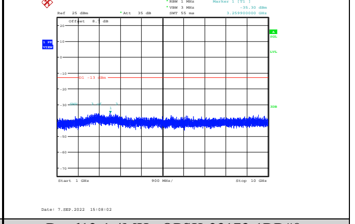
Band12-1.4MHz-QPSK-23173-1RB#0-Range2:1000~10000MHz
