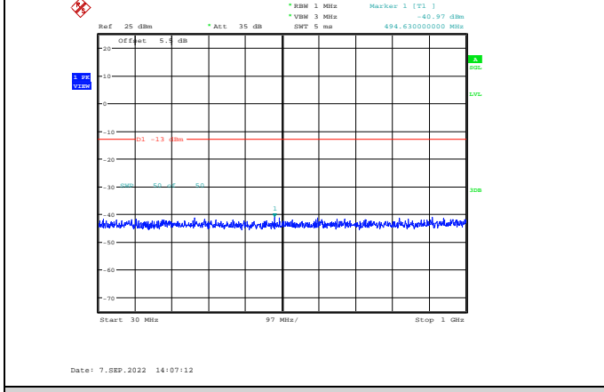
Band2-20MHz-16QAM-18900-1RB#0-Range1:30~1000MHz
