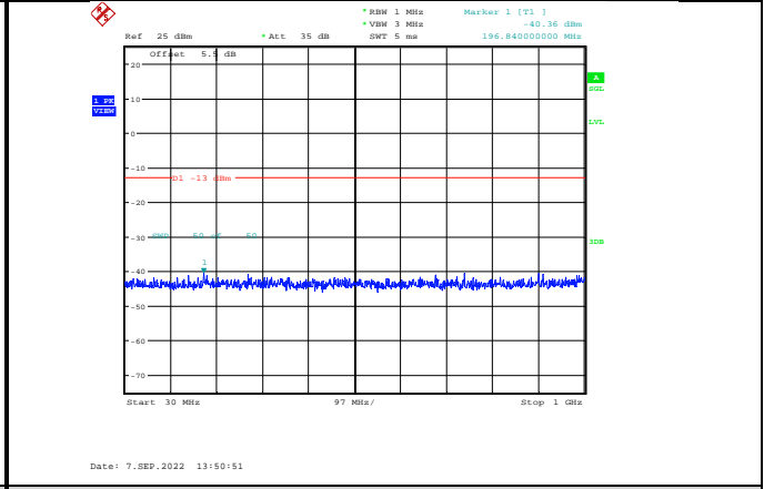
Band2-1.4MHz-16QAM-19193-1RB#0-Range1:30~1000MHz
