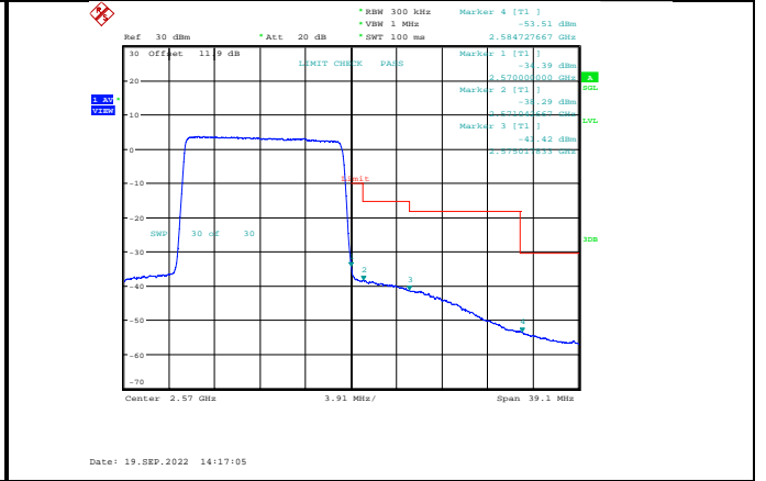
Band7-15MHz-64QAM-21375-75RB#0
