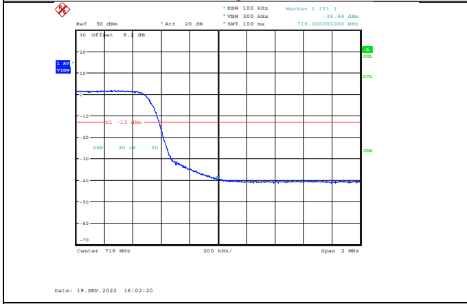
Band17-10MHz-16QAM-23800-50RB#0
