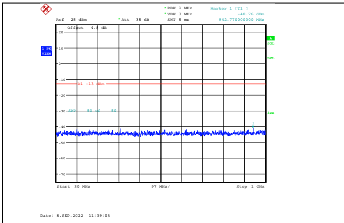
Band2-5MHz-64QAM-18625-1RB#0-Range1:30~1000MHz
