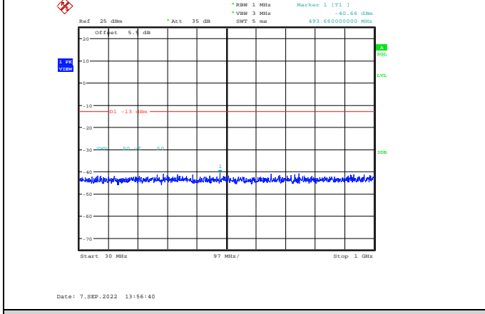
Band2-5MHz-16QAM-18900-1RB#0-Range1:30~1000MHz
