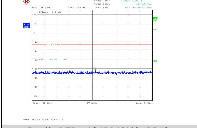
Band2-5MHz-64QAM-18900-1RB#0-Range1:30~1000MHz
