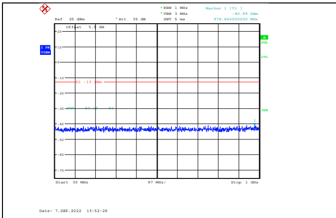
Band2-3MHz-16QAM-18615-1RB#0-Range1:30~1000MHz
