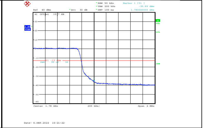
Band66-5MHz-64QAM-132647-25RB#0
