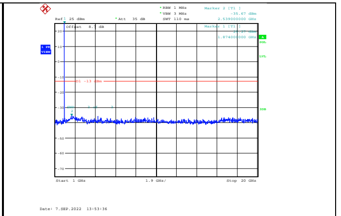
Band2-3MHz-16QAM-18900-1RB#0-Range2:1000~20000MHz
