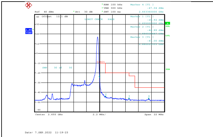
Band41-5MHz-16QAM-41215-1RB#24
