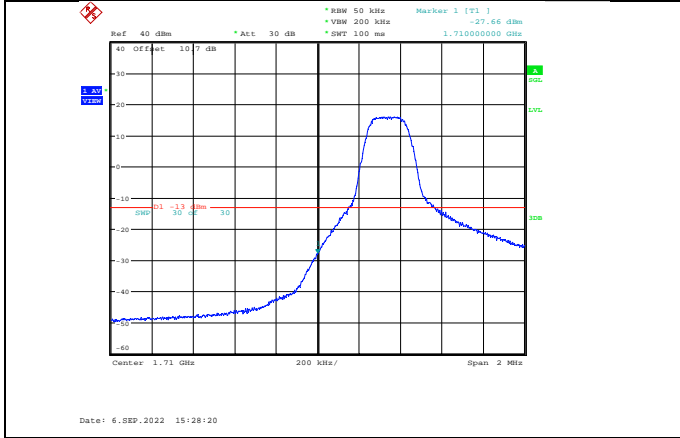
Band66-5MHz-64QAM-131997-1RB#0
