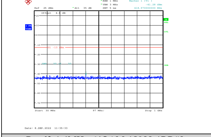
Band2-1.4MHz-64QAM-18900-1RB#0-Range1:30~1000MHz
