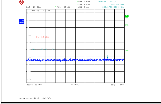
Band2-3MHz-64QAM-18900-1RB#0-Range1:30~1000MHz
