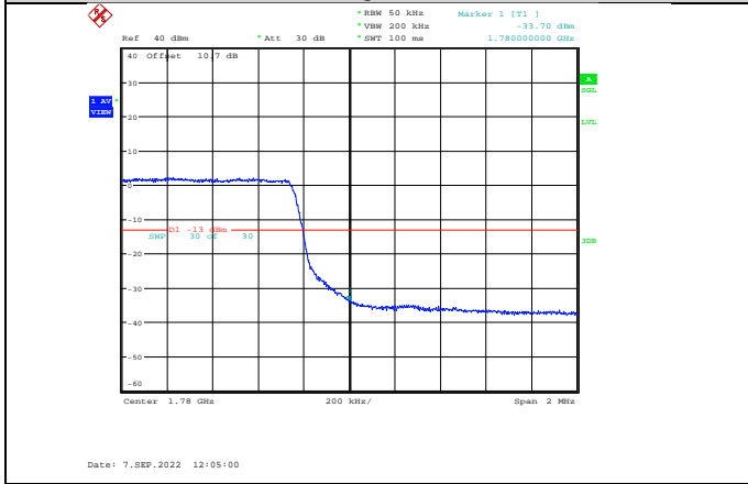
Band66-5MHz-16QAM-132647-25RB#0
