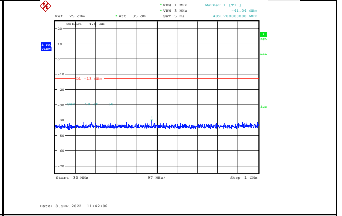
Band2-10MHz-64QAM-19150-1RB#0-Range1:30~1000MHz
