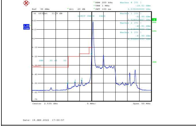
Band41-10MHz-64QAM-40090-1RB#0
