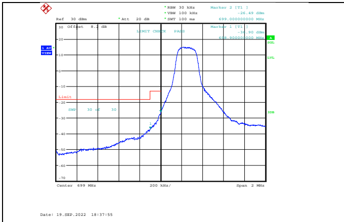
Band12-1.4MHz-QPSK-23017-1RB#0
