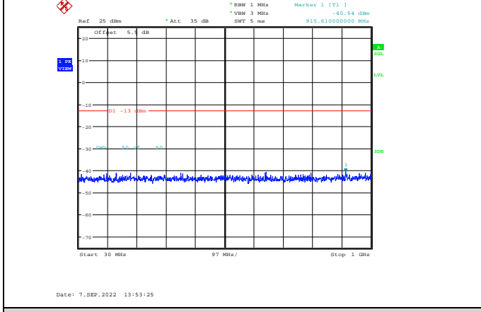
Band2-3MHz-16QAM-18900-1RB#0-Range1:30~1000MHz
