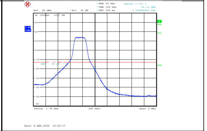
Band66-3MHz-64QAM-132657-1RB#14
