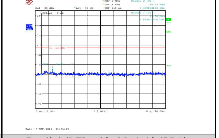
Band2-1.4MHz-64QAM-19193-1RB#0-Range2:1000~20000MHz
