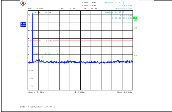
Band2-3MHz-64QAM-18615-1RB#0-Range2:1000~20000MHz
