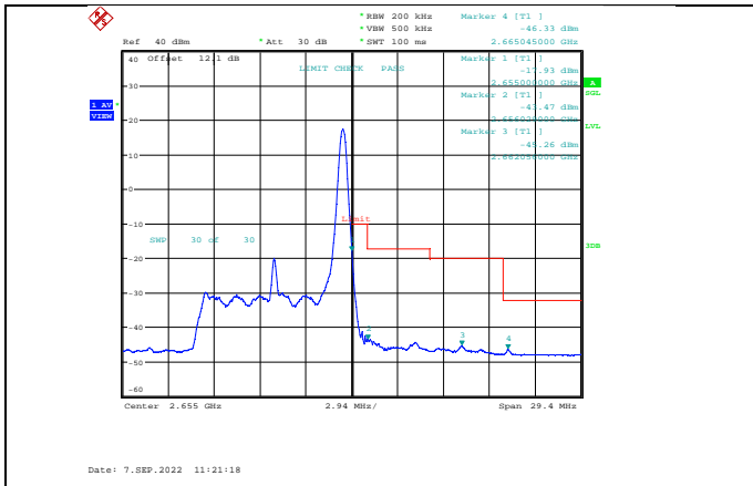
Band41-10MHz-16QAM-41190-1RB#49
