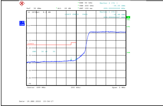
Band12-5MHz-QPSK-23035-25RB#0
