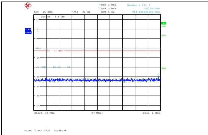
Band2-10MHz-QPSK-18650-1RB#0-Range1:30~1000MHz
