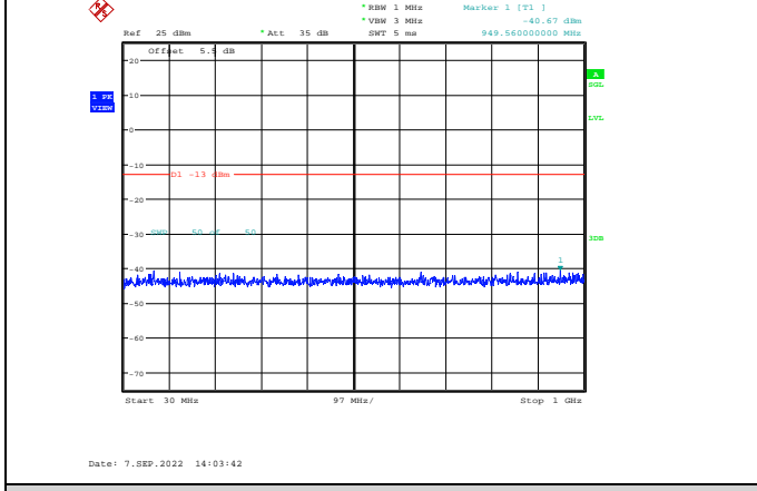
Band2-15MHz-16QAM-18900-1RB#0-Range1:30~1000MHz
