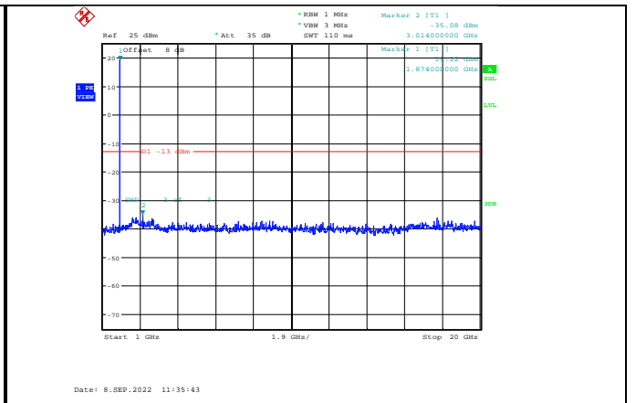
Band2-1.4MHz-64QAM-18900-1RB#0-Range2:1000~20000MHz
