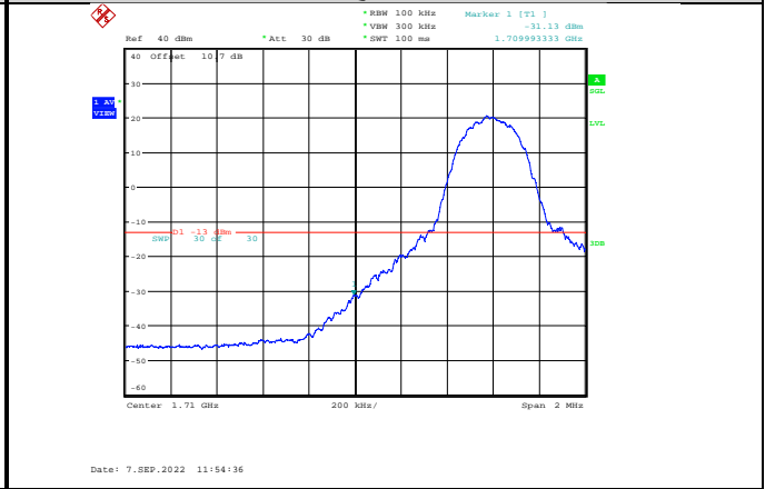
Band66-10MHz-16QAM-132022-1RB#0
