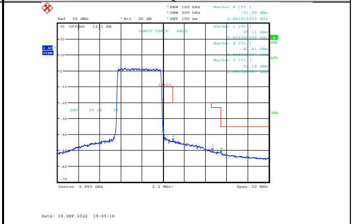
Band41-5MHz-64QAM-41215-25RB#0
