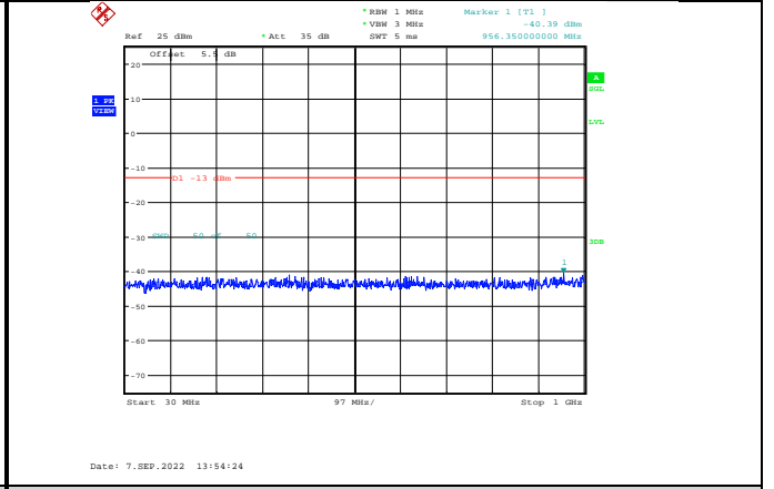
Band2-3MHz-16QAM-19185-1RB#0-Range1:30~1000MHz
