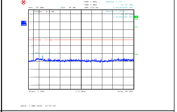
Band2-1.4MHz-16QAM-19193-1RB#0-Range2:1000~20000MHz
