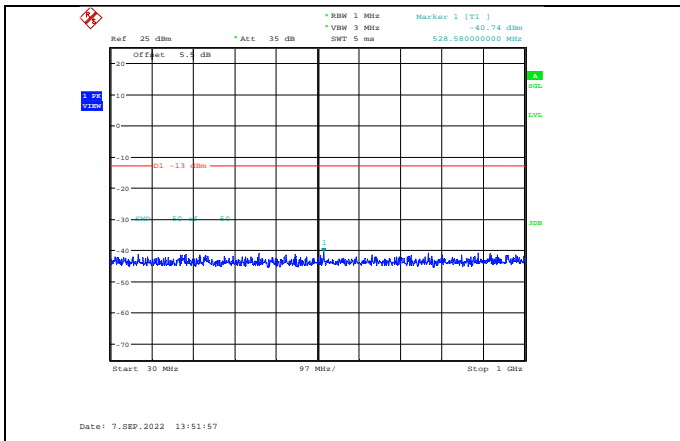
Band2-3MHz-QPSK-18615-1RB#0-Range1:30~1000MHz
