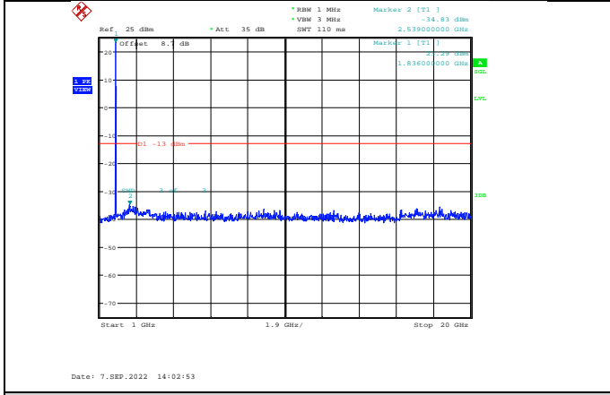
Band2-15MHz-16QAM-18675-1RB#0-Range2:1000~20000MHz
