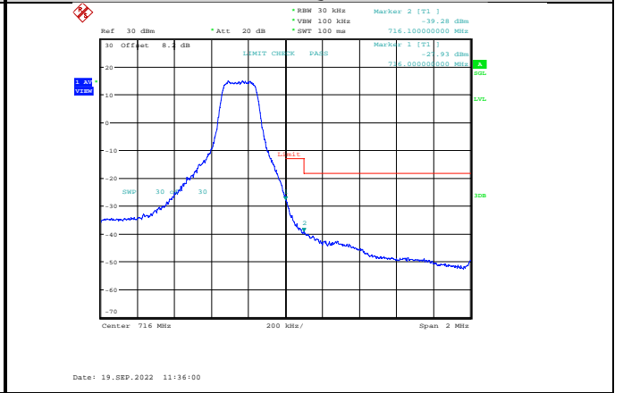
Band12-1.4MHz-64QAM-23173-1RB#5
