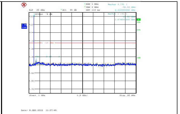
Band2-3MHz-64QAM-18900-1RB#0-Range2:1000~20000MHz
