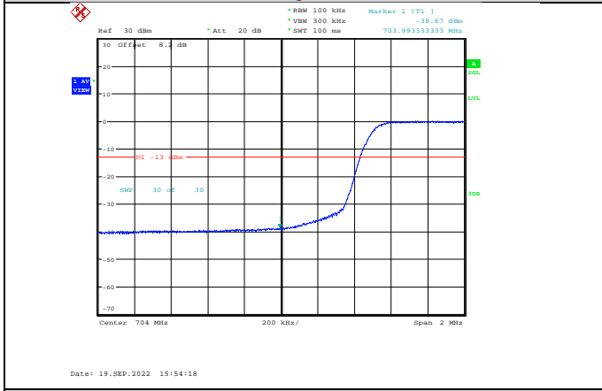
Band17-10MHz-QPSK-23780-50RB#0
