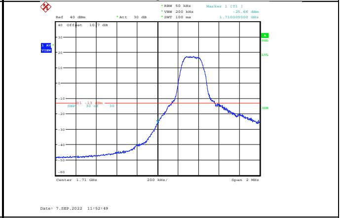
Band66-5MHz-16QAM-131997-1RB#0
