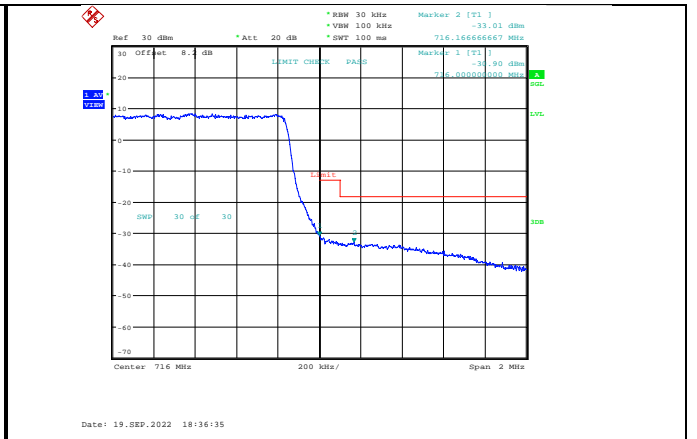
Band12-1.4MHz-QPSK-23173-6RB#0
