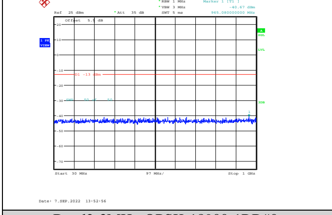
Band2-3MHz-QPSK-18900-1RB#0-Range1:30~1000MHz
