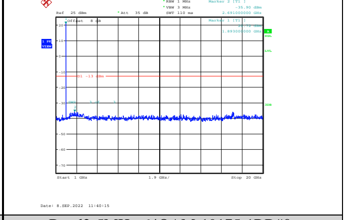
Band2-5MHz-64QAM-19175-1RB#0-Range2:1000~20000MHz
