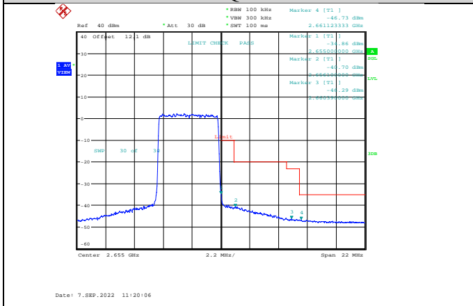
Band41-5MHz-16QAM-41215-25RB#0
