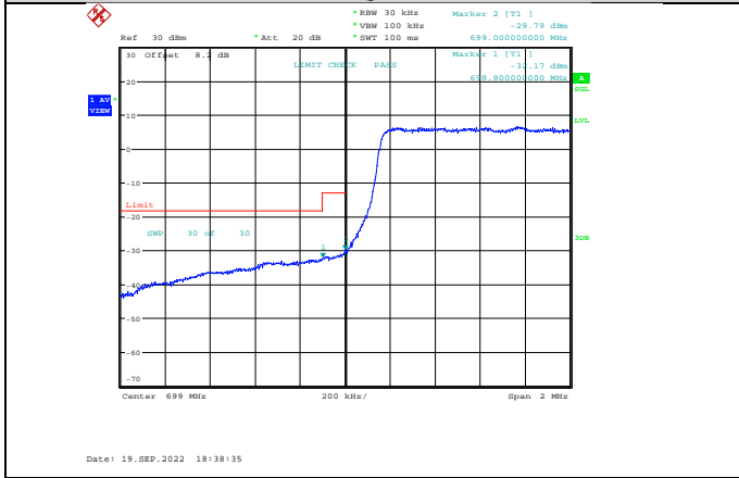
Band12-1.4MHz-QPSK-23017-6RB#0
