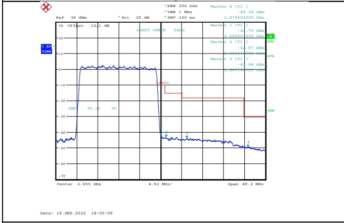
Band41-20MHz-16QAM-41140-100RB#0
