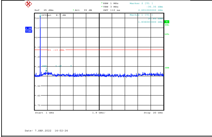
Band2-15MHz-QPSK-18675-1RB#0-Range2:1000~20000MHz
