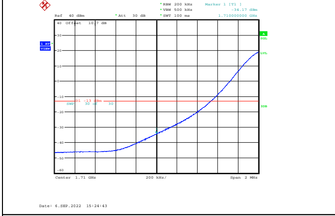
Band66-20MHz-64QAM-132072-1RB#0
