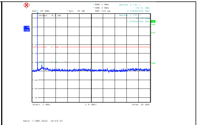
Band2-15MHz-QPSK-18900-1RB#0-Range2:1000~20000MHz
