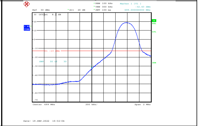
Band12-10MHz-16QAM-23060-1RB#0
