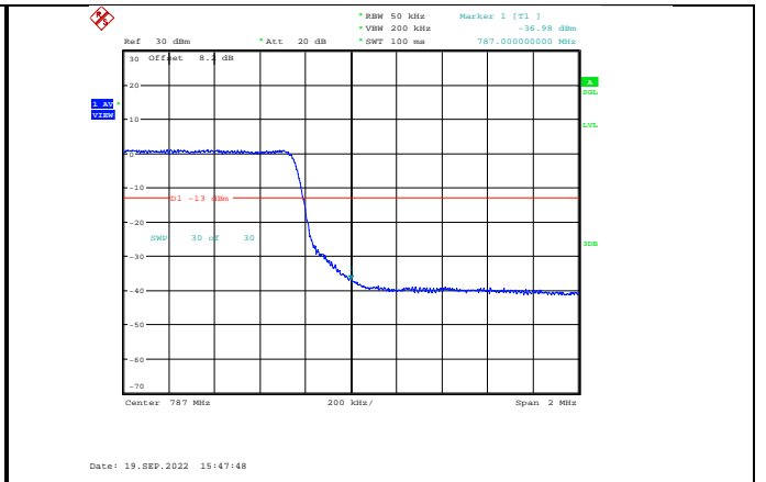
Band13-5MHz-QPSK-23255-25RB#0
