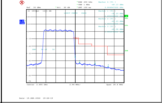
Band41-10MHz-64QAM-41190-50RB#0
