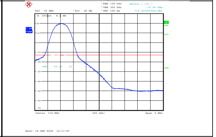
Band17-10MHz-64QAM-23800-1RB#49
