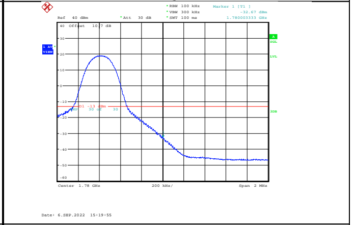
Band66-10MHz-64QAM-132622-1RB#49
