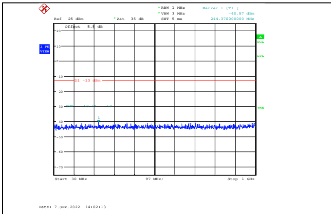
Band2-15MHz-QPSK-18675-1RB#0-Range1:30~1000MHz
