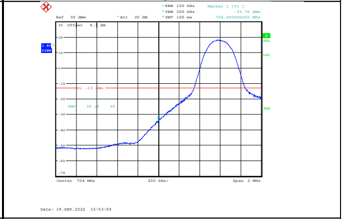
Band17-10MHz-16QAM-23780-1RB#0
