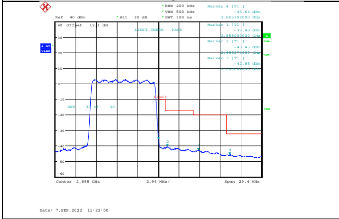
Band41-10MHz-16QAM-41190-50RB#0
