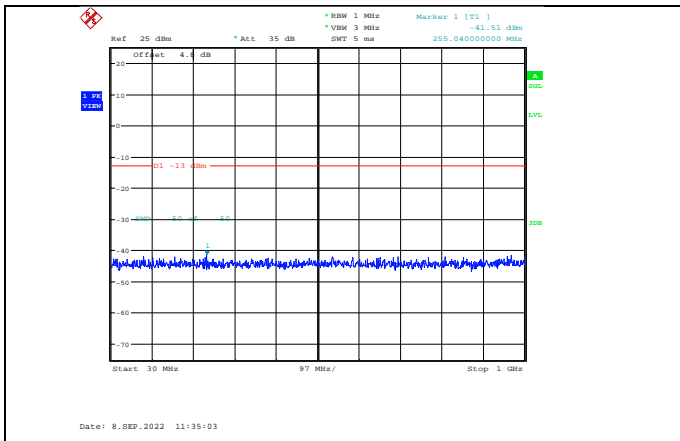
Band2-1.4MHz-64QAM-18607-1RB#0-Range1:30~1000MHz
