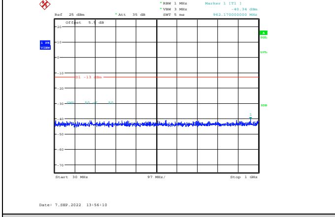
Band2-5MHz-QPSK-18900-1RB#0-Range1:30~1000MHz
