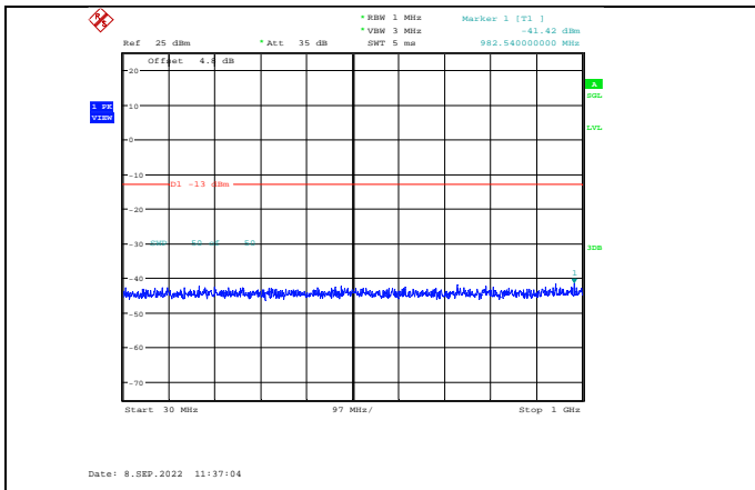
Band2-3MHz-64QAM-18615-1RB#0-Range1:30~1000MHz
