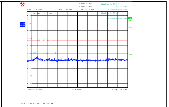
Band2-15MHz-16QAM-18900-1RB#0-Range2:1000~20000MHz
