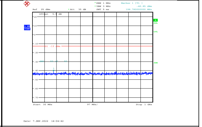
Band2-15MHz-16QAM-19125-1RB#0-Range1:30~1000MHz
