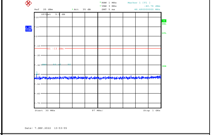
Band2-3MHz-QPSK-19185-1RB#0-Range1:30~1000MHz
