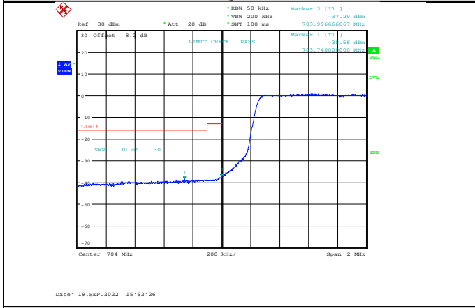
Band17-5MHz-QPSK-23755-25RB#0
