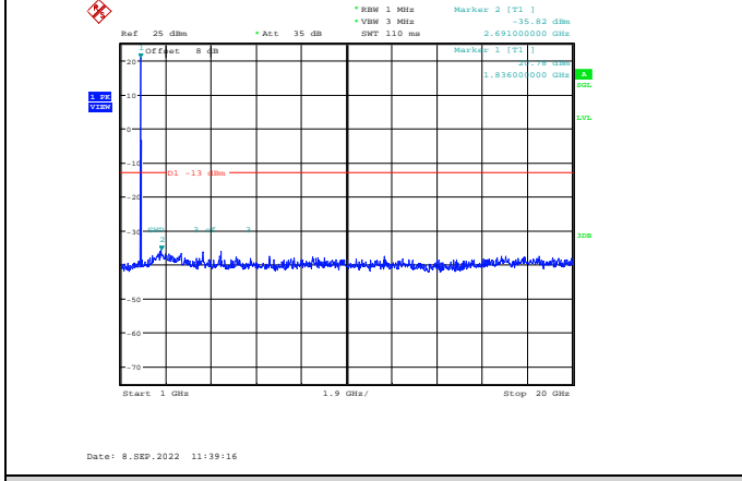
Band2-5MHz-64QAM-18625-1RB#0-Range2:1000~20000MHz
