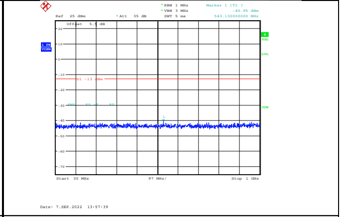
Band2-5MHz-16QAM-19175-1RB#0-Range1:30~1000MHz
