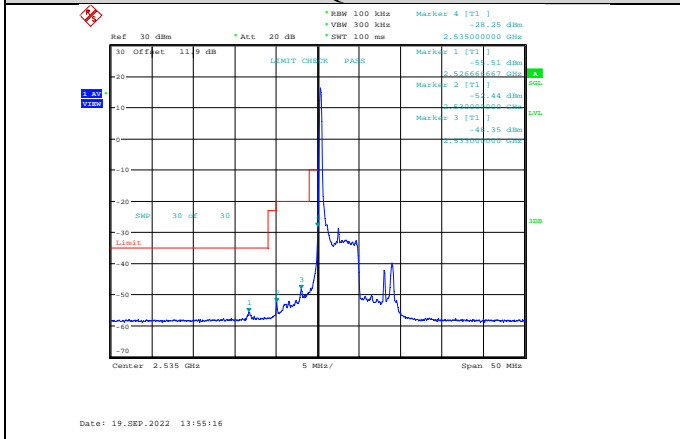
Band41-5MHz-64QAM-40065-1RB#0
