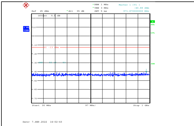
Band2-15MHz-16QAM-18675-1RB#0-Range1:30~1000MHz
