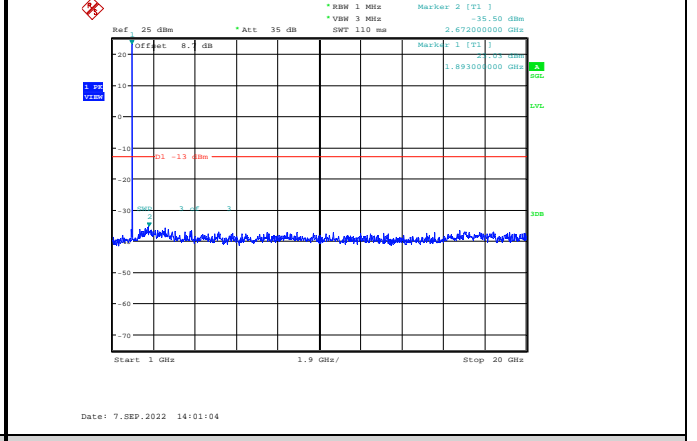
Band2-10MHz-16QAM-19150-1RB#0-Range2:1000~20000MHz
