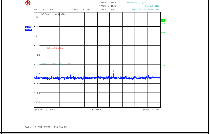
Band2-1.4MHz-64QAM-19193-1RB#0-Range1:30~1000MHz
