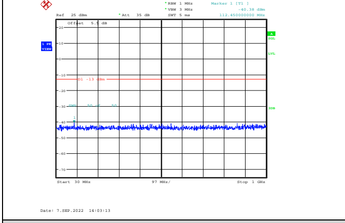
Band2-15MHz-QPSK-18900-1RB#0-Range1:30~1000MHz
