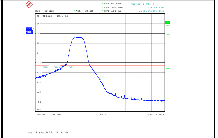
Band66-5MHz-64QAM-132647-1RB#24
