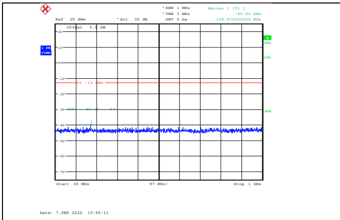
Band2-5MHz-QPSK-18625-1RB#0-Range1:30~1000MHz
