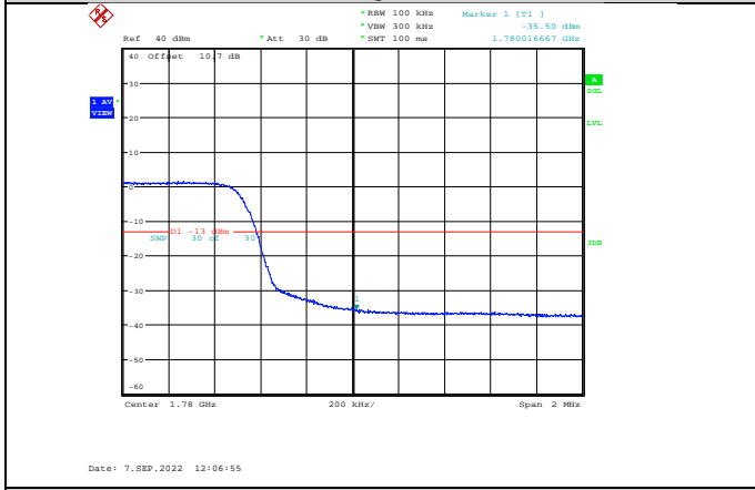
Band66-10MHz-16QAM-132622-50RB#0
