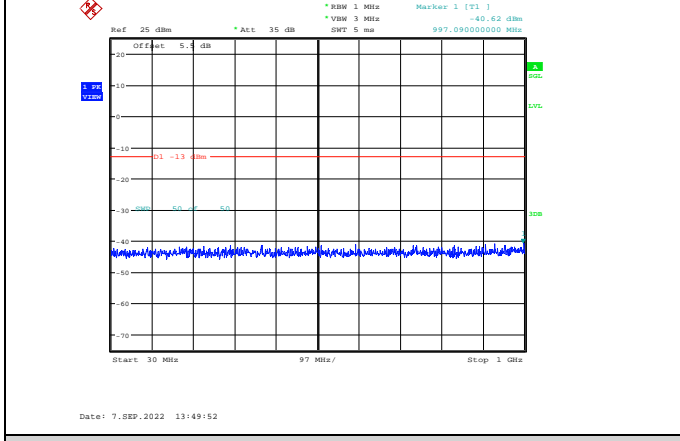
Band2-1.4MHz-16QAM-18900-1RB#0-Range1:30~1000MHz
