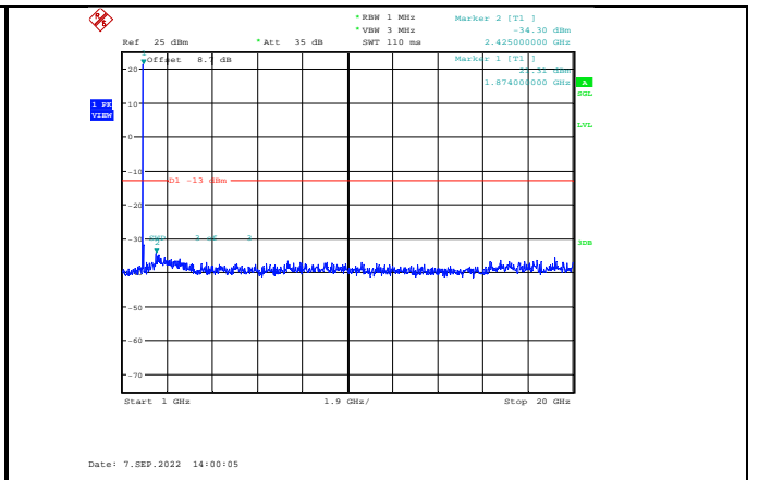
Band2-10MHz-16QAM-18900-1RB#0-Range2:1000~20000MHz
