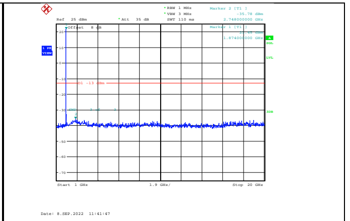
Band2-10MHz-64QAM-18900-1RB#0-Range2:1000~20000MHz
