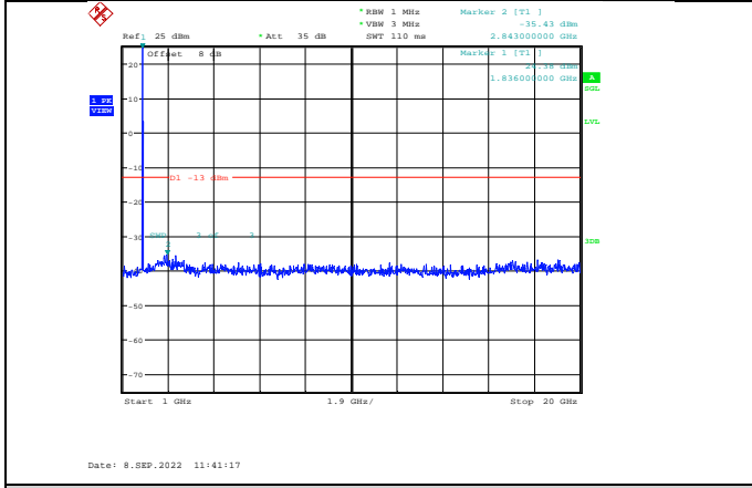
Band2-10MHz-64QAM-18650-1RB#0-Range2:1000~20000MHz
