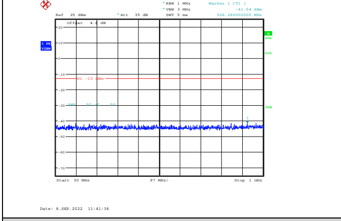
Band2-10MHz-64QAM-18900-1RB#0-Range1:30~1000MHz
