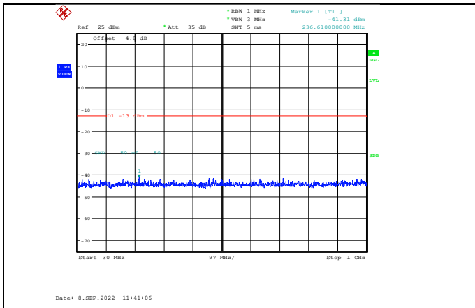
Band2-10MHz-64QAM-18650-1RB#0-Range1:30~1000MHz
