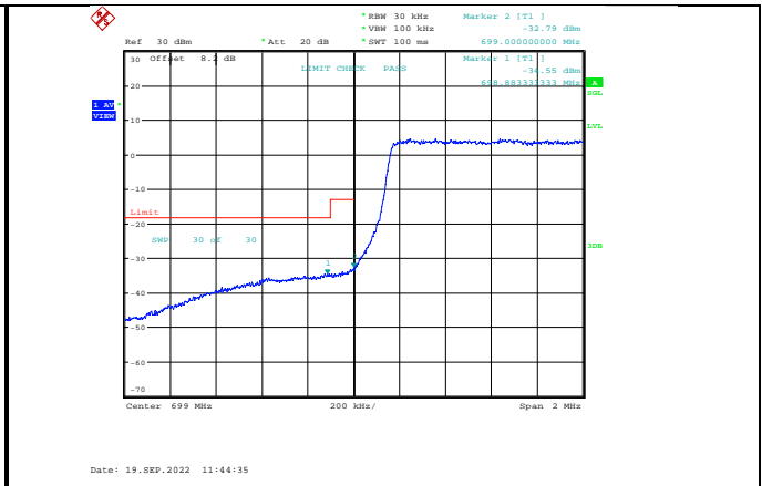
Band12-1.4MHz-64QAM-23017-6RB#0
