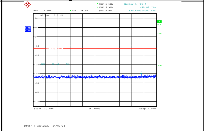
Band2-10MHz-QPSK-19150-1RB#0-Range1:30~1000MHz
