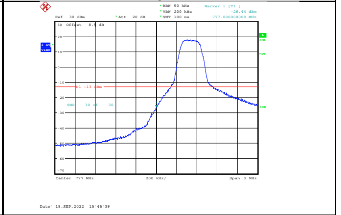
Band13-5MHz-16QAM-23205-1RB#0
