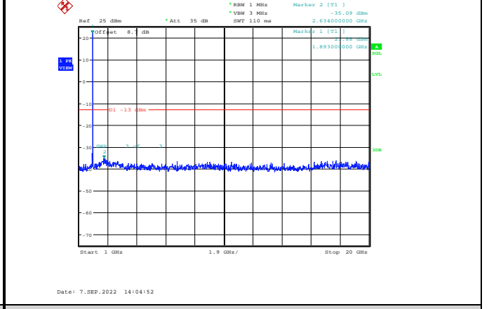
Band2-15MHz-16QAM-19125-1RB#0-Range2:1000~20000MHz
