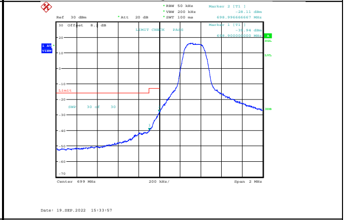
Band12-5MHz-16QAM-23035-1RB#0
