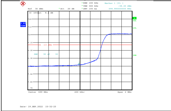
Band12-10MHz-QPSK-23060-50RB#0
