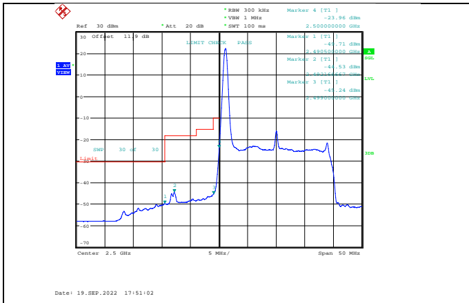
Band7-20MHz-QPSK-20850-1RB#0
