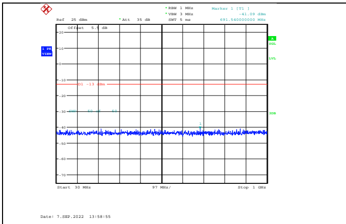
Band2-10MHz-16QAM-18650-1RB#0-Range1:30~1000MHz
