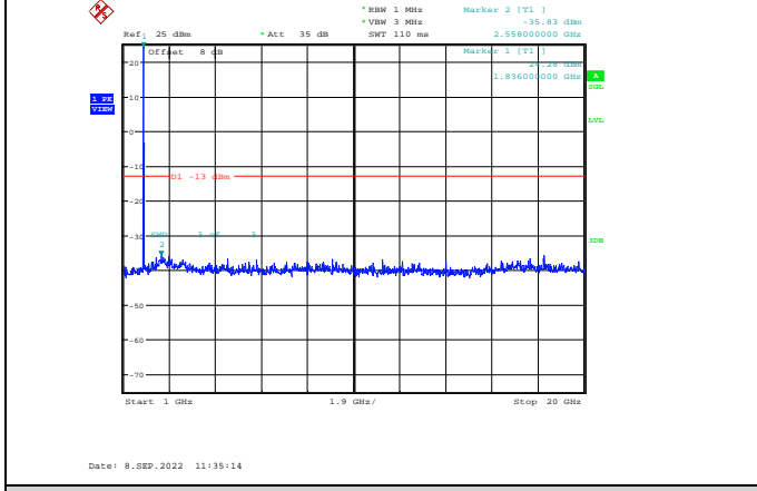
Band2-1.4MHz-64QAM-18607-1RB#0-Range2:1000~20000MHz
