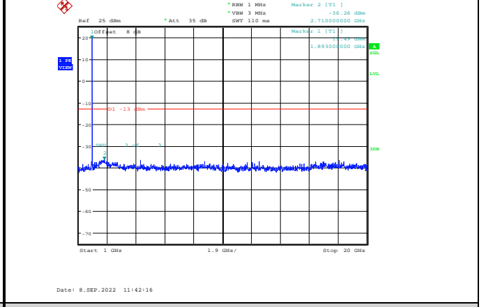
Band2-10MHz-64QAM-19150-1RB#0-Range2:1000~20000MHz
