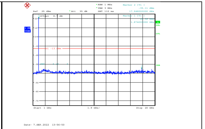
Band2-5MHz-16QAM-18900-1RB#0-Range2:1000~20000MHz
