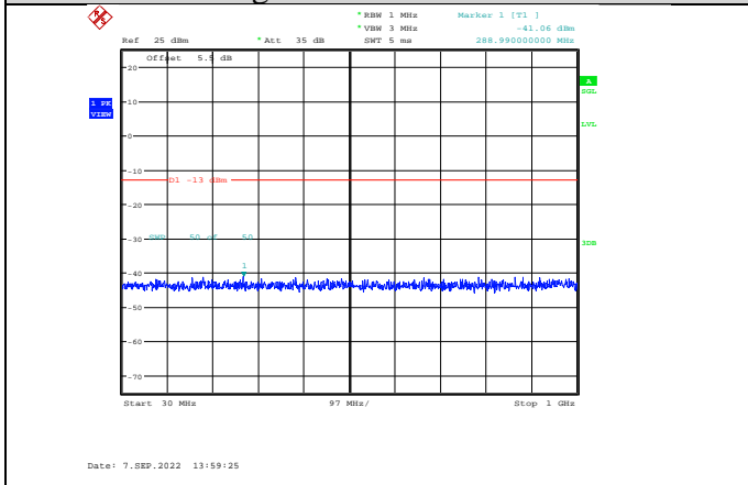
Band2-10MHz-QPSK-18900-1RB#0-Range1:30~1000MHz
