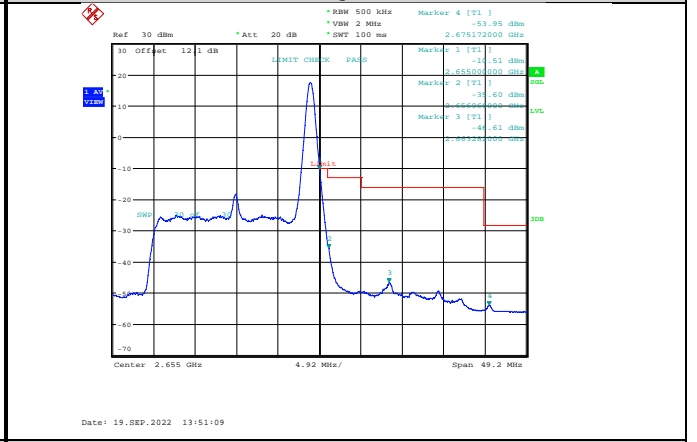
Band41-20MHz-64QAM-41140-1RB#99
