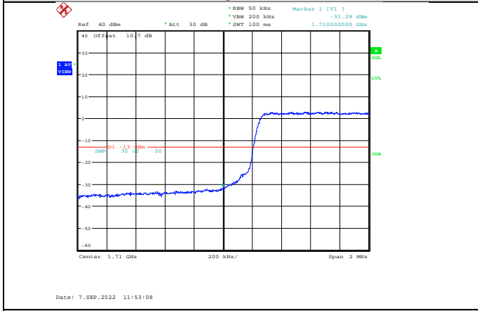
Band66-5MHz-QPSK-131997-25RB#0
