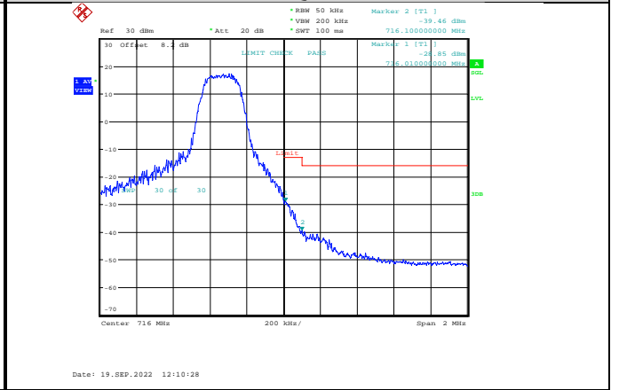
Band17-5MHz-64QAM-23825-1RB#24
