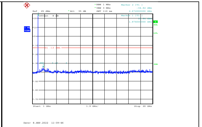
Band2-5MHz-64QAM-18900-1RB#0-Range2:1000~20000MHz
