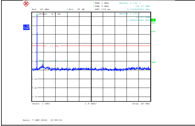
Band2-5MHz-16QAM-18625-1RB#0-Range2:1000~20000MHz
