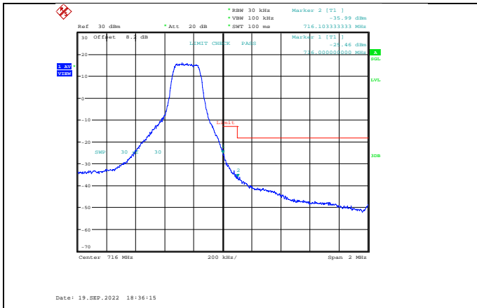
Band12-1.4MHz-16QAM-23173-1RB#5
