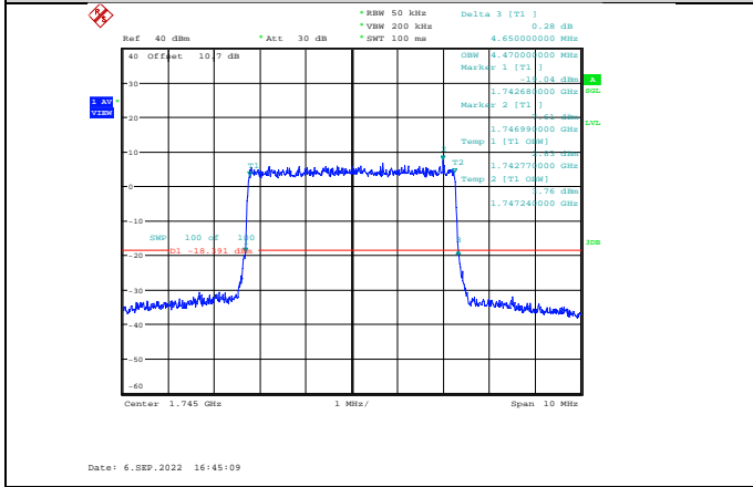
Band66-5MHz-64QAM-132322-25RB#0
