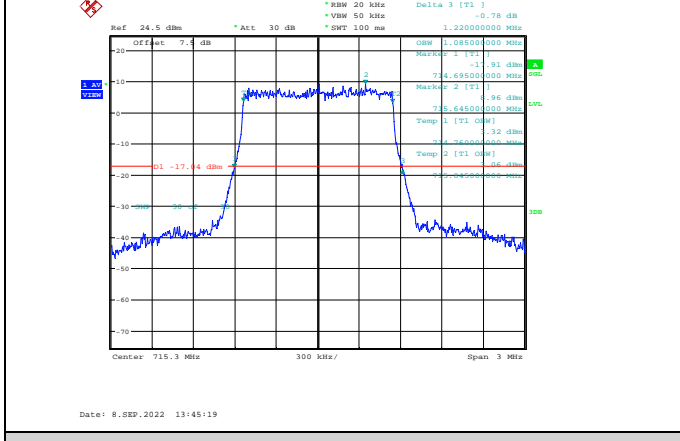
Band12-1.4MHz-64QAM-23173-6RB#0
