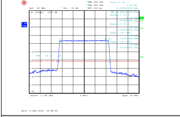
Band66-15MHz-64QAM-132322-75RB#0
