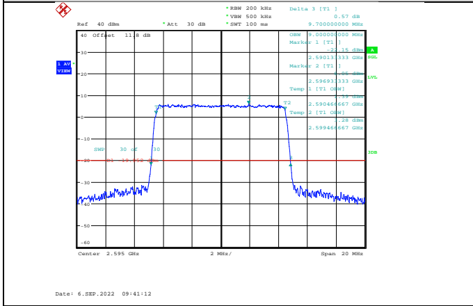
Band41-10MHz-16QAM-40640-50RB#0
