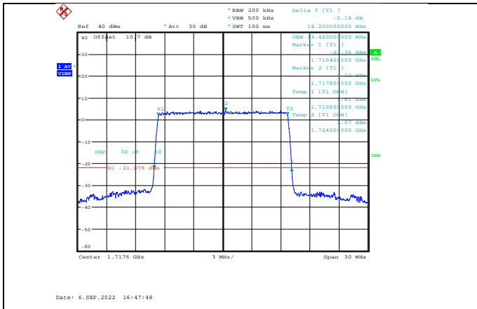
Band66-15MHz-64QAM-132047-75RB#0
