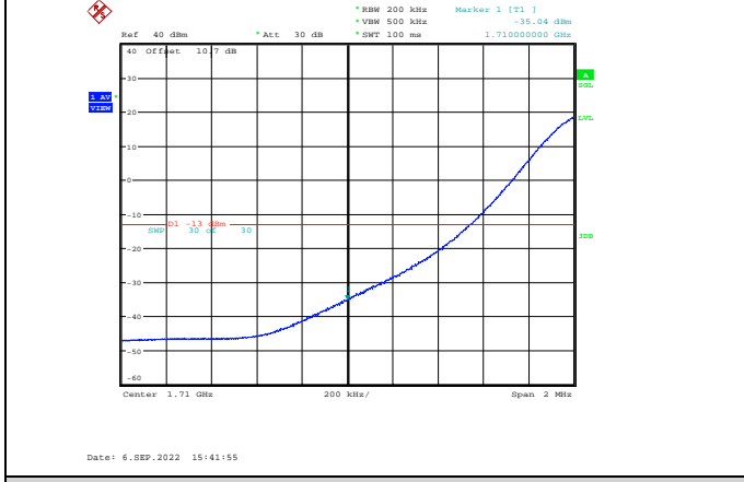
Band4-20MHz-64QAM-20050-1RB#0
