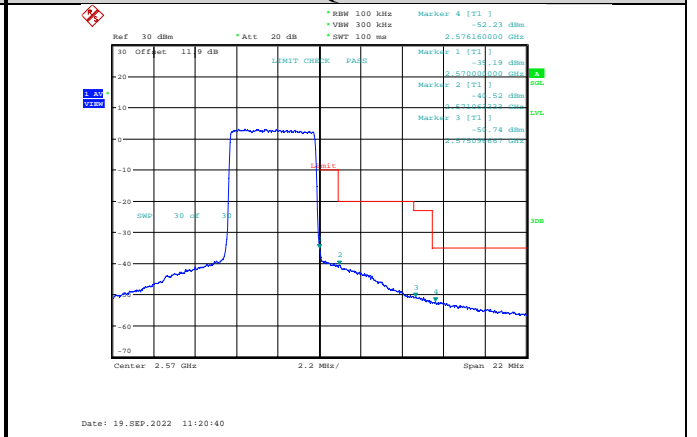
Band7-5MHz-64QAM-21425-25RB#0
