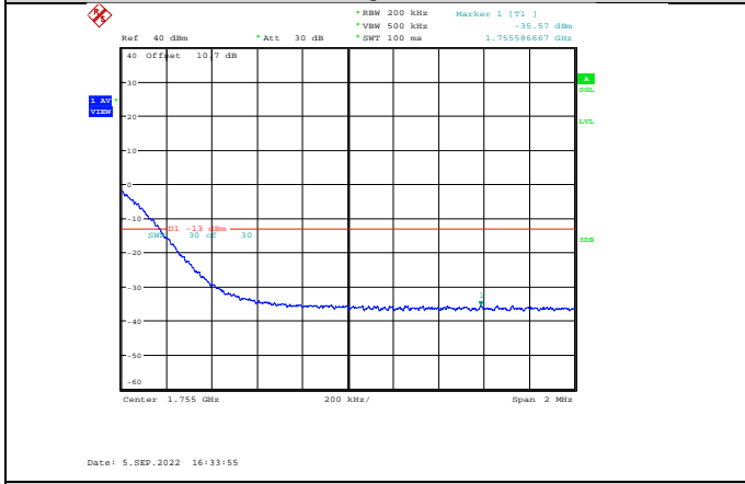
Band4-20MHz-16QAM-20300-100RB#0
