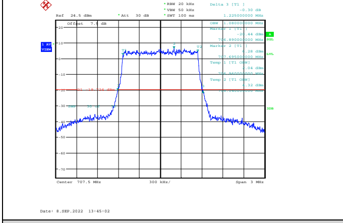
Band12-1.4MHz-64QAM-23095-6RB#0
