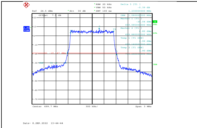
Band12-1.4MHz-64QAM-23017-6RB#0
