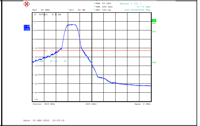
Band5-5MHz-64QAM-20625-1RB#24
