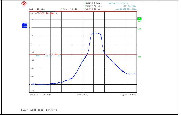
Band2-3MHz-16QAM-18615-1RB#0
