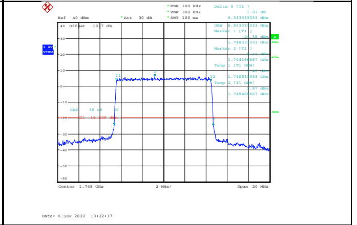
Band66-10MHz-QPSK-132322-50RB#0
