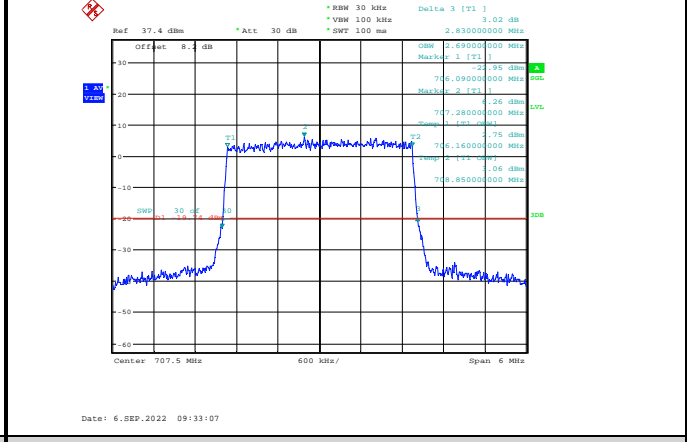
Band12-3MHz-QPSK-23095-15RB#0
