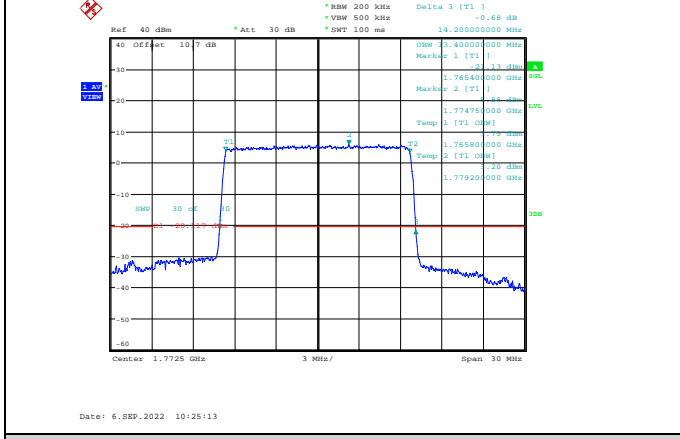
Band66-15MHz-QPSK-132597-75RB#0
