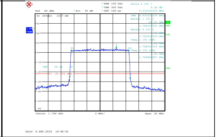
Band66-10MHz-64QAM-132322-50RB#0
