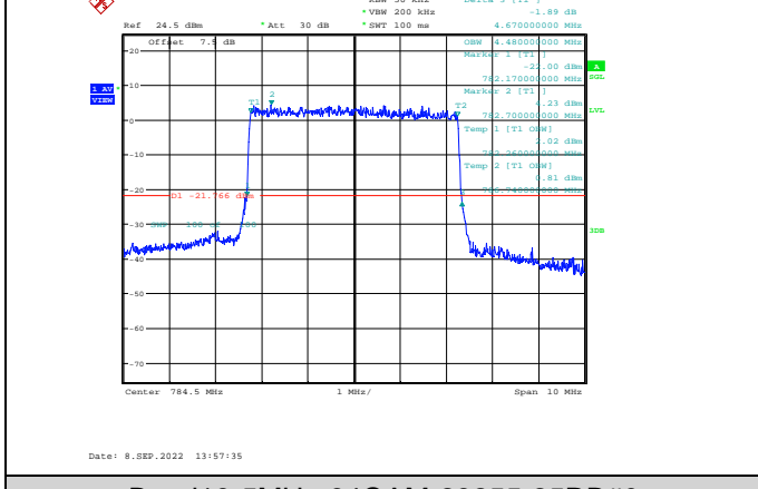
Band13-5MHz-64QAM-23255-25RB#0
