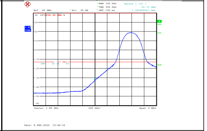
Band2-10MHz-16QAM-18650-1RB#0
