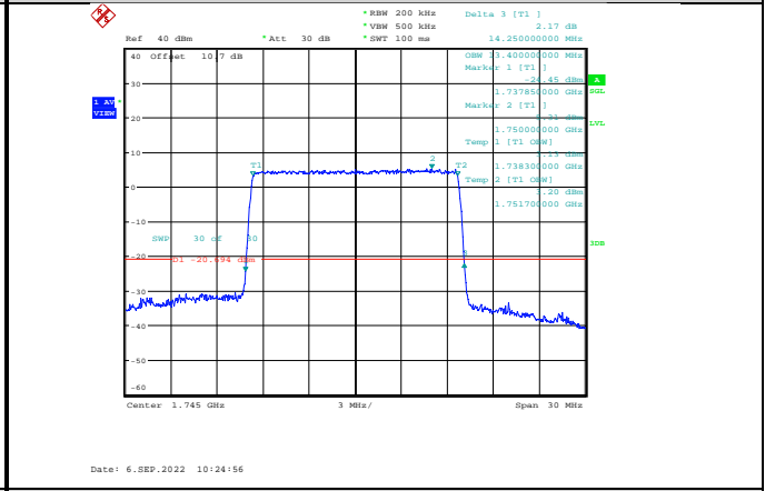
Band66-15MHz-16QAM-132322-75RB#0
