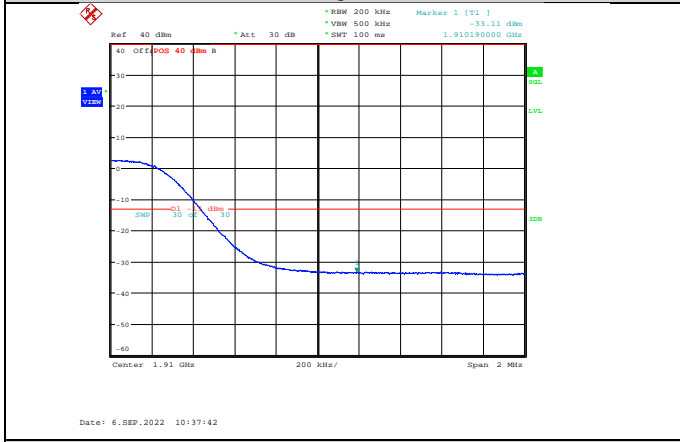
Band2-15MHz-16QAM-19125-75RB#0
