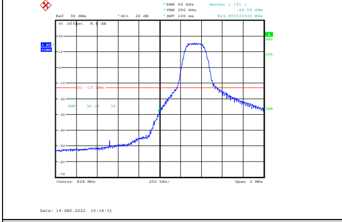
Band5-5MHz-64QAM-20425-1RB#0
