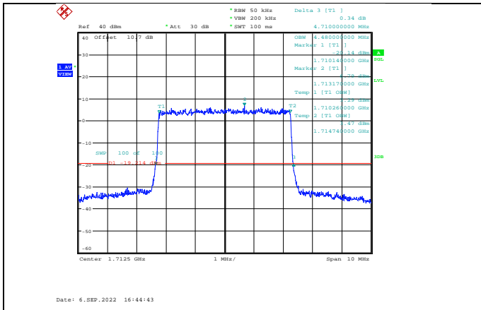
Band66-5MHz-64QAM-131997-25RB#0
