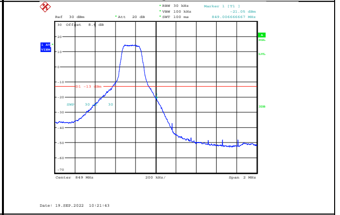
Band5-3MHz-64QAM-20635-1RB#14
