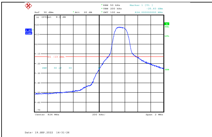
Band5-5MHz-QPSK-20425-1RB#0
