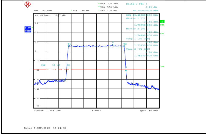
Band66-15MHz-QPSK-132322-75RB#0
