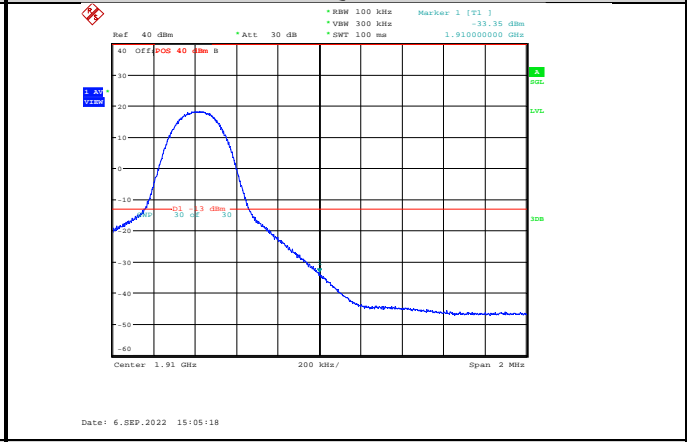
Band2-10MHz-64QAM-18650-50RB#0
