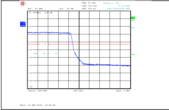
Band5-3MHz-16QAM-20635-15RB#0
