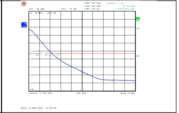
Band4-20MHz-64QAM-20300-1RB#99
