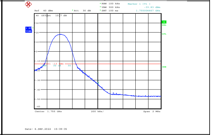
Band4-10MHz-64QAM-20350-1RB#49
