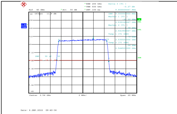
Band41-10MHz-16QAM-40090-50RB#0
