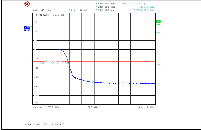
Band4-10MHz-16QAM-20350-50RB#0
