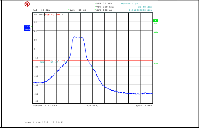
Band2-3MHz-64QAM-19185-1RB#14
