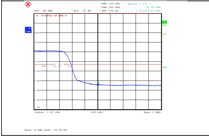
Band2-10MHz-16QAM-19150-50RB#0
