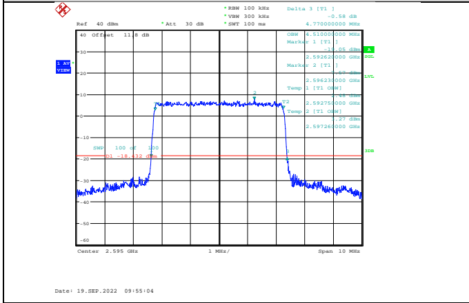
Band41-5MHz-64QAM-40640-25RB#0
