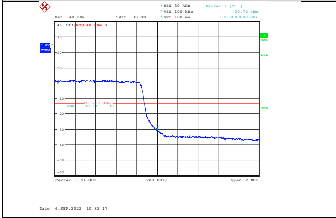
Band2-3MHz-16QAM-19185-15RB#0
