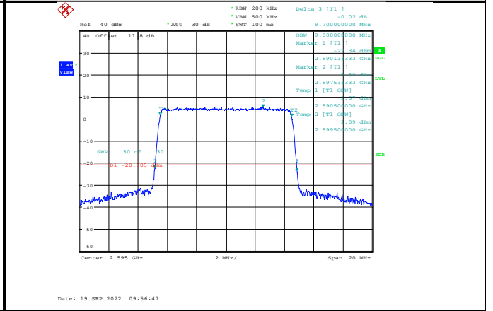
Band41-10MHz-64QAM-40640-50RB#0
