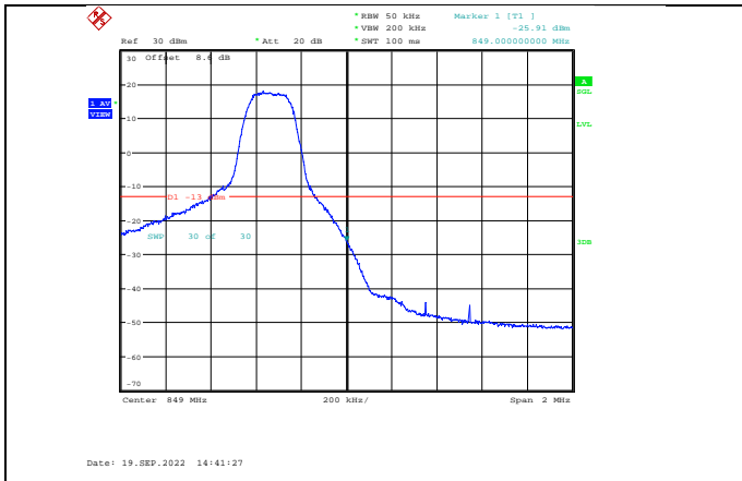
Band5-5MHz-16QAM-20625-1RB#24
