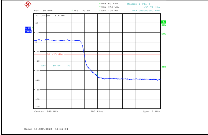
Band5-5MHz-16QAM-20625-25RB#0
