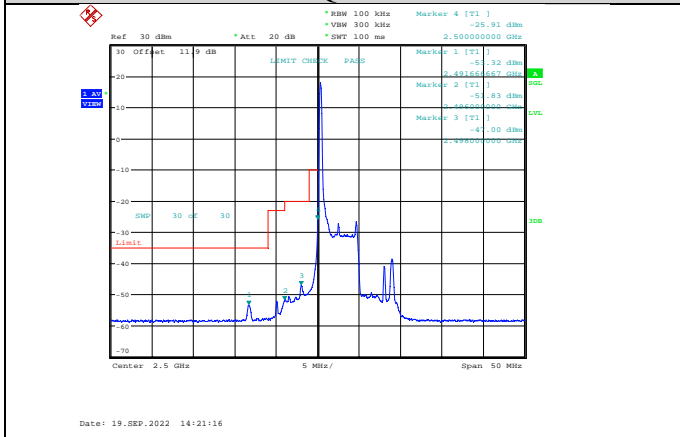
Band7-5MHz-64QAM-20775-1RB#0
