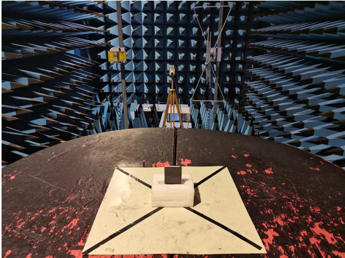
FCC Part15C Radiated Emission above 18-26.5GHz
