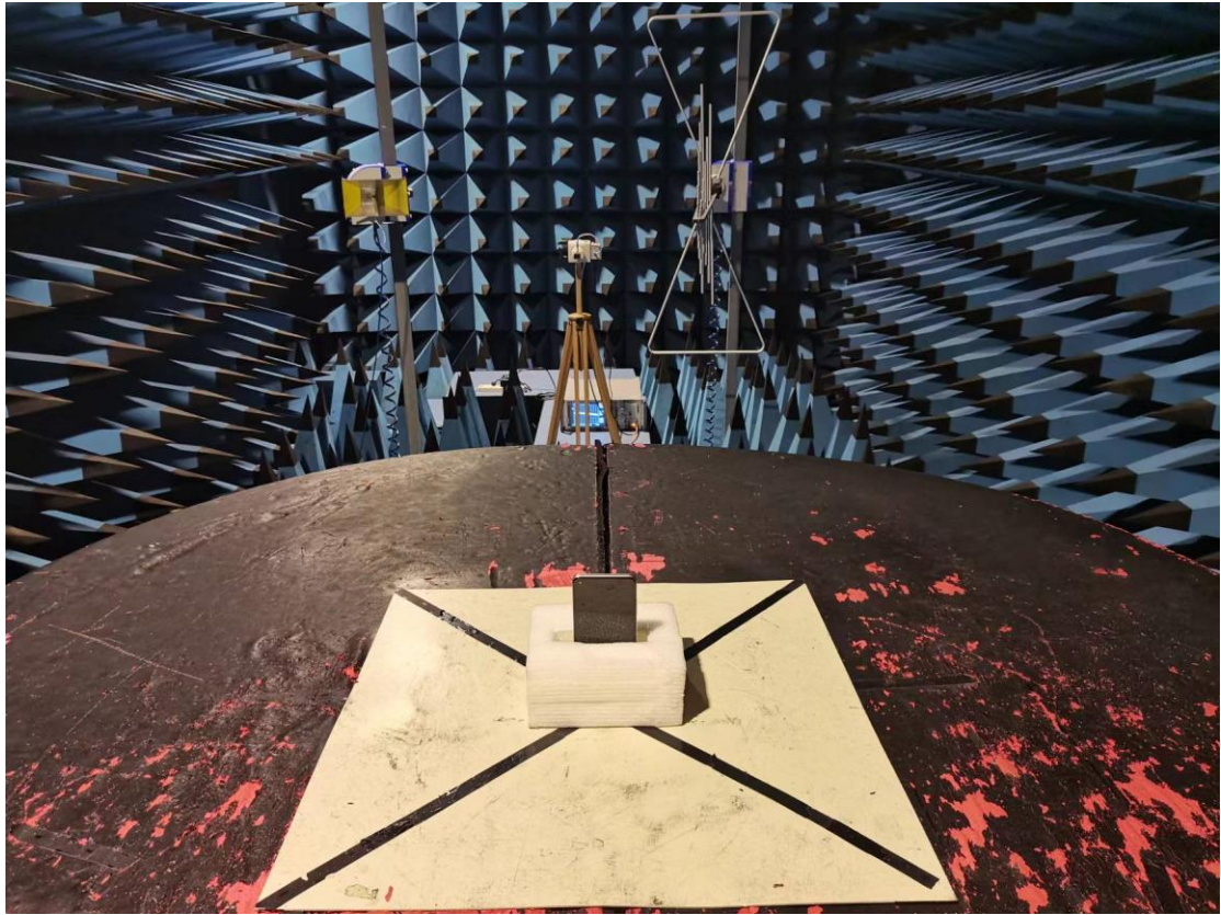
FCC Part15C Radiated Emission above 26.5-40GHz
