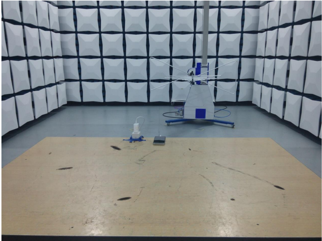
FCC Part15C Radiated Emission below 1GHz -Front
