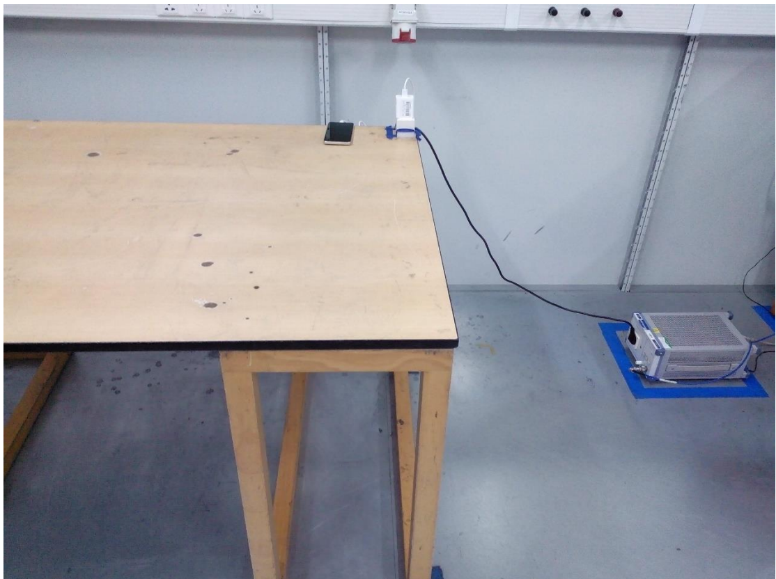
AC Conducted Emission Test Setup
