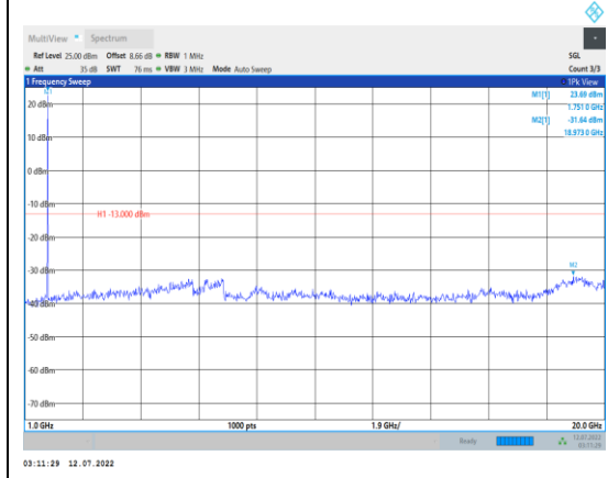
Band66-3MHz-QPSK-132322-1RB#0- Range2:1000~20000MHz
