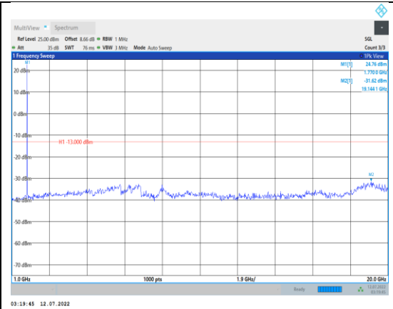
Band66-10MHz-16QAM-132622-1RB#0- Range2:1000~20000MHz
