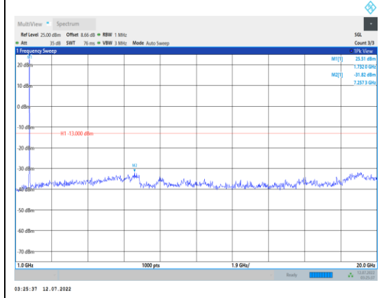
Band66-20MHz-16QAM-132322-1RB#0- Range2:1000~20000MHz
