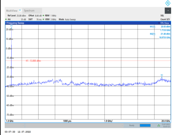
Band66-1.4MHz-16QAM-131979-1RB#0- Range2:1000~20000MHz
