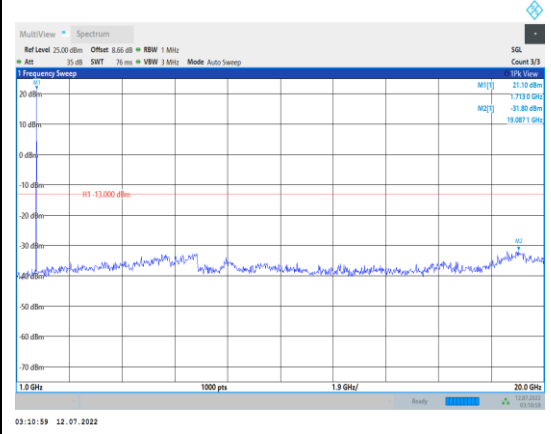
Band66-3MHz-16QAM-131987-1RB#0- Range2:1000~20000MHz
