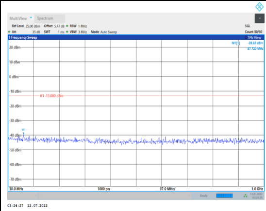
Band66-20MHz-16QAM-132072-1RB#0- Range1:30~1000MHz
