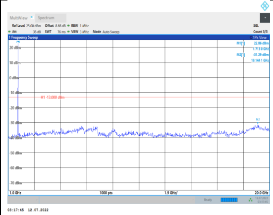
Band66-10MHz-16QAM-132022-1RB#0- Range2:1000~20000MHz
