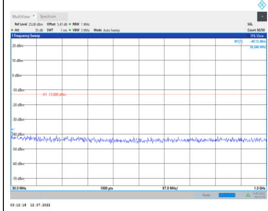
Band66-3MHz-QPSK-132657-1RB#0- Range1:30~1000MHz
