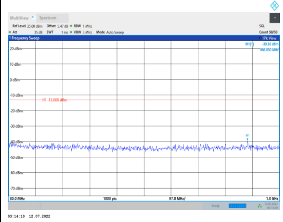
Band66-5MHz-16QAM-131997-1RB#0- Range1:30~1000MHz
