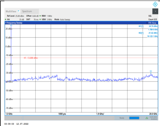
Band66-1.4MHz-QPSK-132665-1RB#0- Range2:1000~20000MHz
