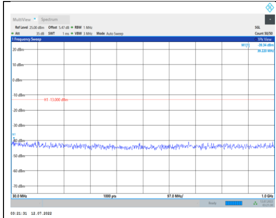
Band66-15MHz-QPSK-132322-1RB#0- Range1:30~1000MHz
