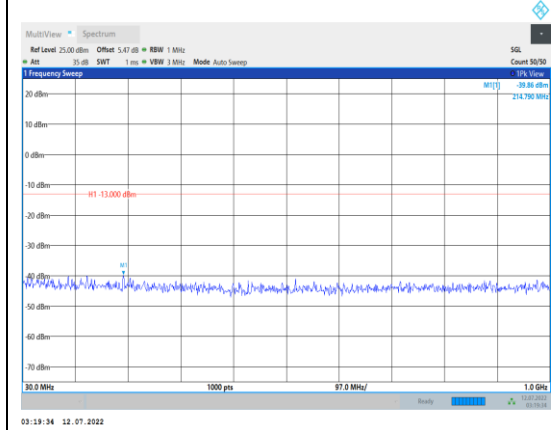
Band66-10MHz-16QAM-132622-1RB#0- Range1:30~1000MHz
