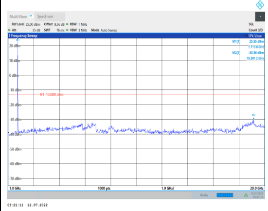
Band66-15MHz-16QAM-132047-1RB#0- Range2:1000~20000MHz
