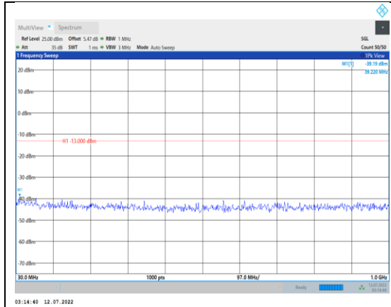
Band66-5MHz-QPSK-132322-1RB#0- Range1:30~1000MHz
