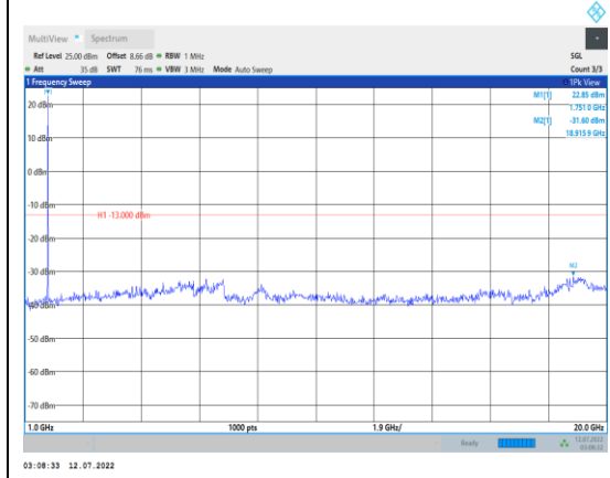
Band66-1.4MHz-16QAM-132322-1RB#0- Range2:1000~20000MHz
