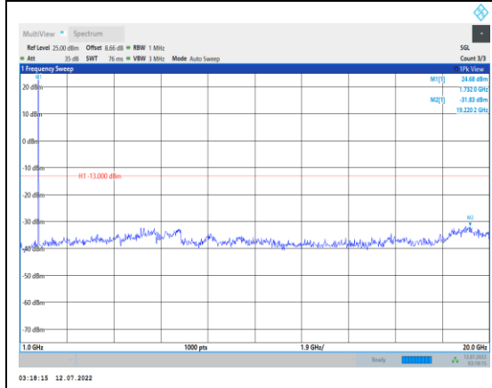
Band66-10MHz-QPSK-132322-1RB#0- Range2:1000~20000MHz
