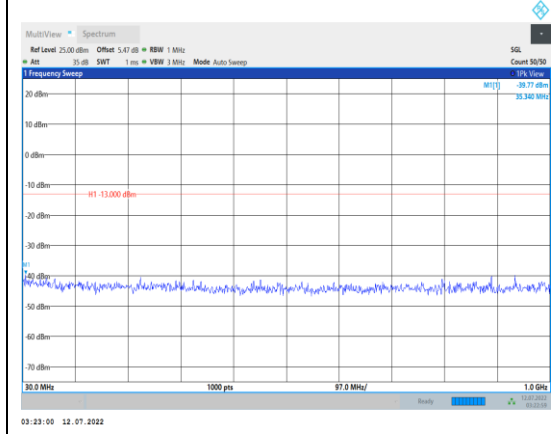
Band66-15MHz-16QAM-132597-1RB#0- Range1:30~1000MHz
