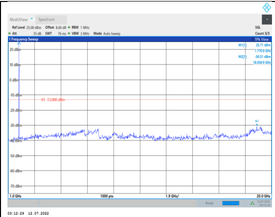
Band66-3MHz-QPSK-132657-1RB#0- Range2:1000~20000MHz
