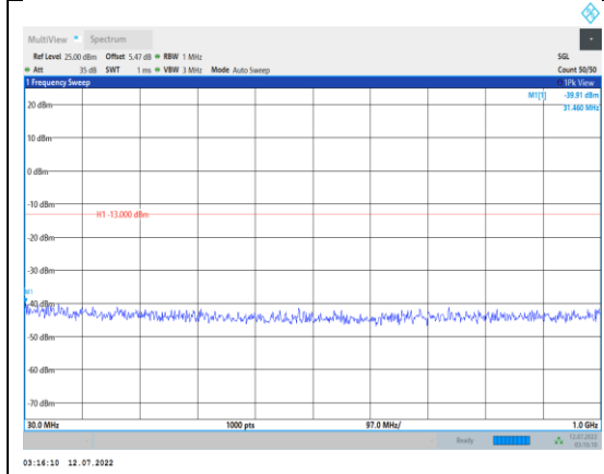
Band66-5MHz-16QAM-132647-1RB#0- Range1:30~1000MHz
