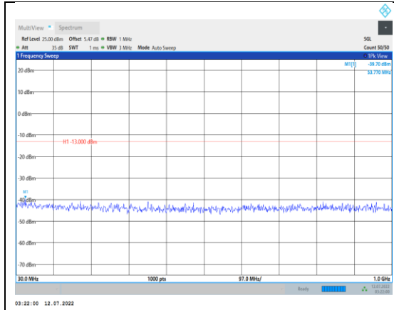
Band66-15MHz-16QAM-132322-1RB#0- Range1:30~1000MHz
