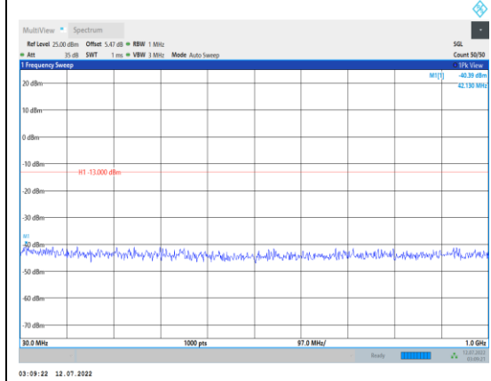
Band66-1.4MHz-16QAM-132665-1RB#0- Range1:30~1000MHz
