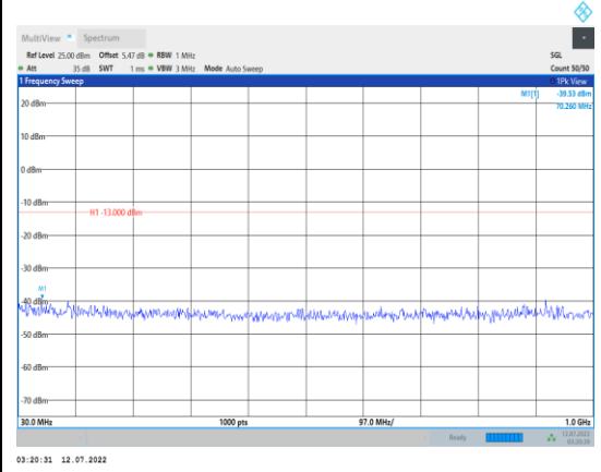
Band66-15MHz-QPSK-132047-1RB#0- Range1:30~1000MHz
