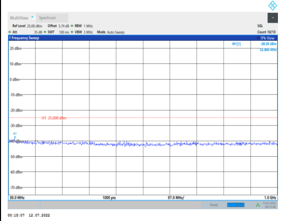
Band41-20MHz-16QAM-40620-1RB#0-Range1:30~1000MHz
