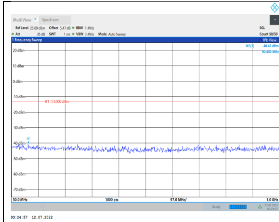
Band66-20MHz-QPSK-132322-1RB#0- Range1:30~1000MHz
