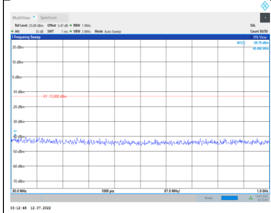
Band66-3MHz-16QAM-132657-1RB#0- Range1:30~1000MHz
