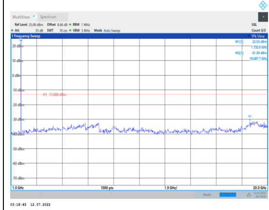
Band66-10MHz-16QAM-132322-1RB#0- Range2:1000~20000MHz
