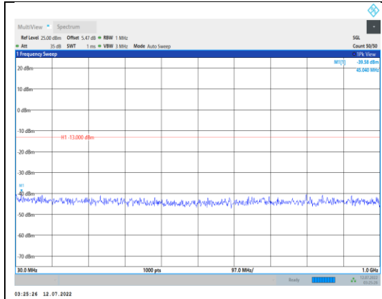
Band66-20MHz-16QAM-132322-1RB#0- Range1:30~1000MHz
