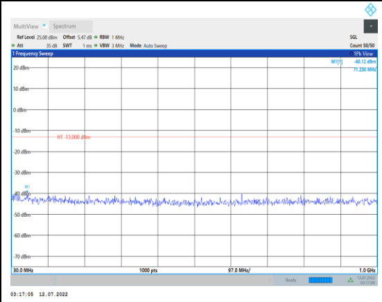
Band66-10MHz-QPSK-132022-1RB#0- Range1:30~1000MHz
