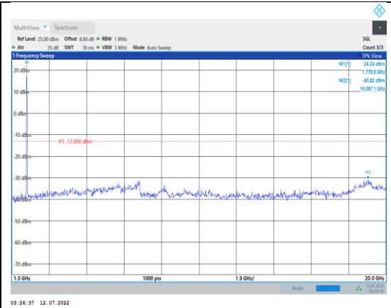
Band66-20MHz-16QAM-132572-1RB#0- Range2:1000~20000MHz
