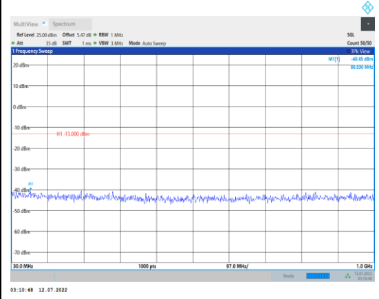
Band66-3MHz-16QAM-131987-1RB#0- Range1:30~1000MHz
