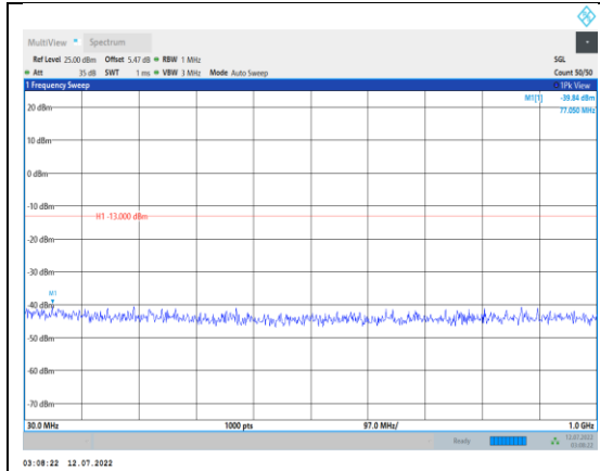
Band66-1.4MHz-16QAM-132322-1RB#0- Range1:30~1000MHz
