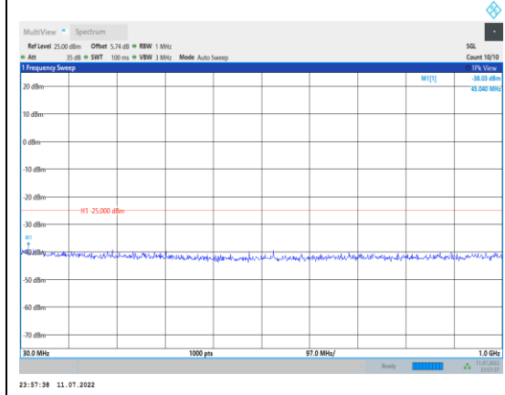
Band41-20MHz-16QAM-39750-1RB#0-Range1:30~1000MHz
