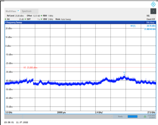
Band41-20MHz-16QAM-39750-1RB#0-Range3:3000~27000MHz
