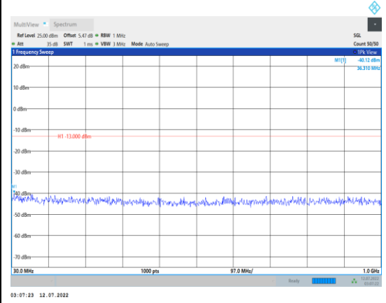
Band66-1.4MHz-16QAM-131979-1RB#0- Range1:30~1000MHz
