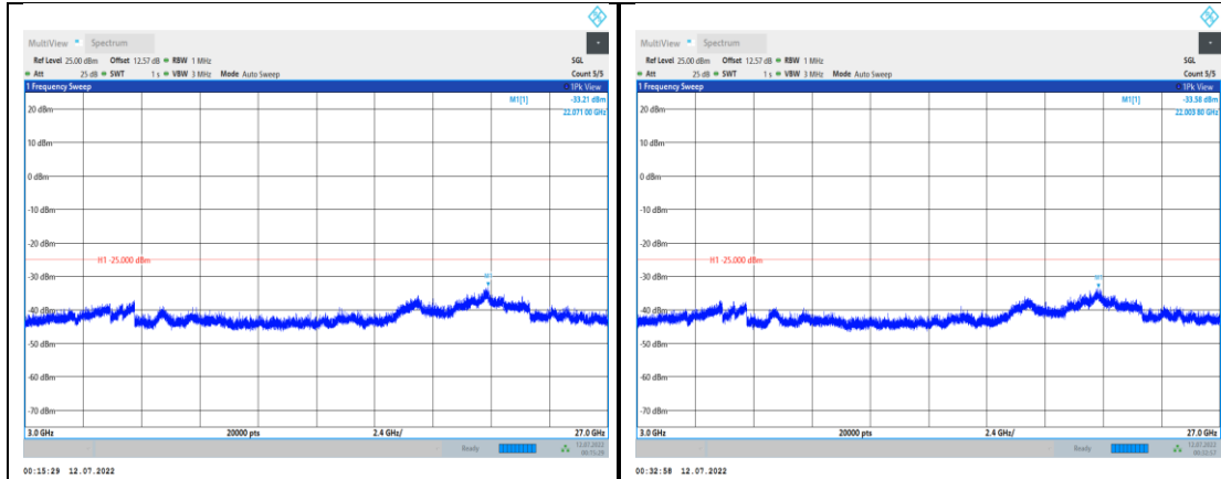
Band41-20MHz-16QAM-40620-1RB#0- Range3:3000~27000MHz
