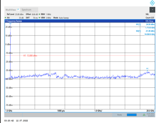
Band66-15MHz-QPSK-132047-1RB#0- Range2:1000~20000MHz
