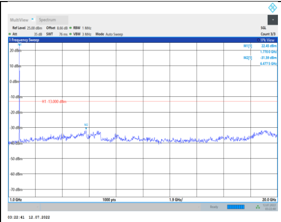
Band66-15MHz-QPSK-132597-1RB#0- Range2:1000~20000MHz
