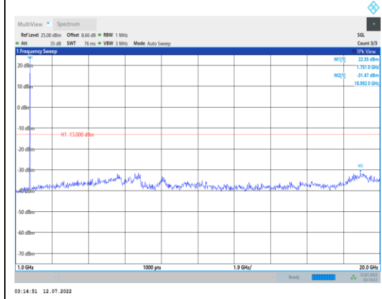
Band66-5MHz-QPSK-132322-1RB#0- Range2:1000~20000MHz
