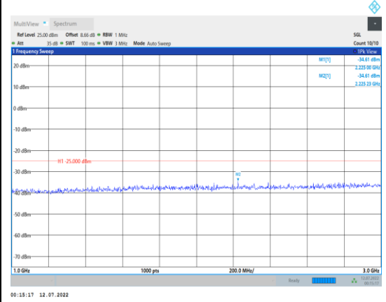
Band41-20MHz-16QAM-40620-1RB#0-Range2:1000~3000MHz
