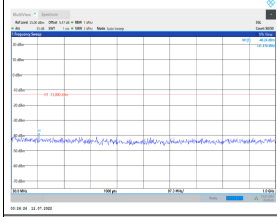
Band66-20MHz-16QAM-132572-1RB#0- Range1:30~1000MHz
