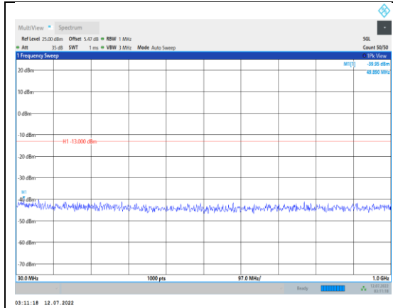
Band66-3MHz-QPSK-132322-1RB#0- Range1:30~1000MHz
