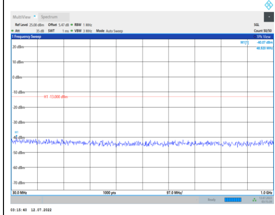
Band66-5MHz-QPSK-132647-1RB#0- Range1:30~1000MHz
