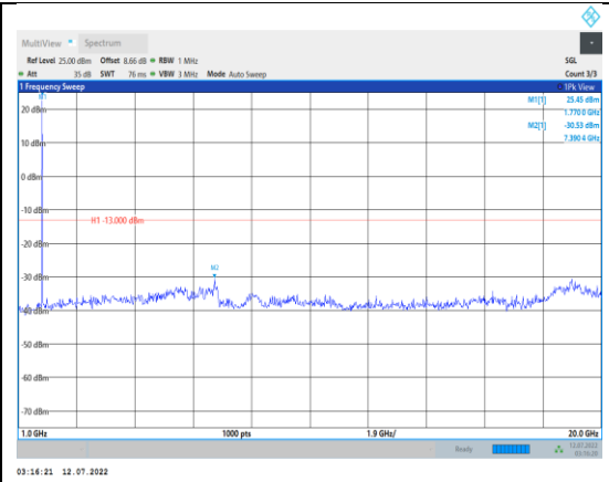
Band66-5MHz-16QAM-132647-1RB#0- Range2:1000~20000MHz
