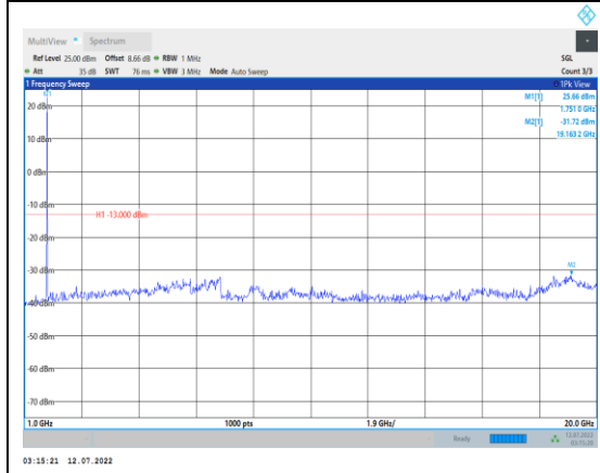
Band66-5MHz-16QAM-132322-1RB#0- Range2:1000~20000MHz
