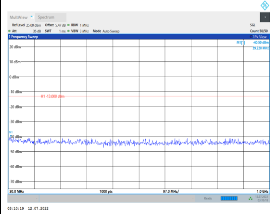
Band66-3MHz-QPSK-131987-1RB#0- Range1:30~1000MHz
