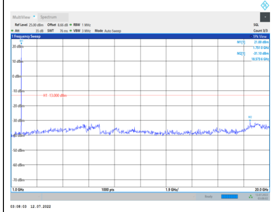
Band66-1.4MHz-QPSK-132322-1RB#0- Range2:1000~20000MHz
