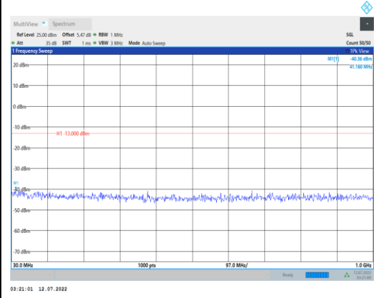
Band66-15MHz-16QAM-132047-1RB#0- Range1:30~1000MHz
