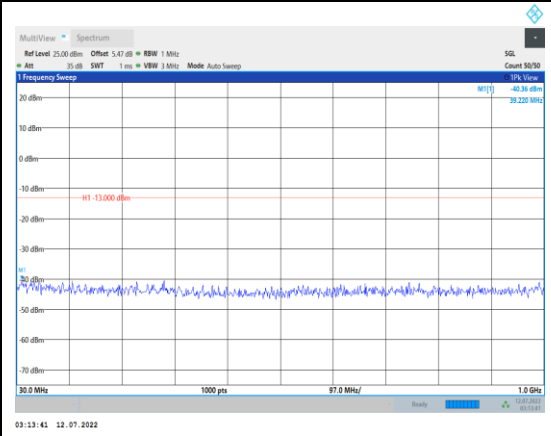
Band66-5MHz-QPSK-131997-1RB#0- Range1:30~1000MHz
