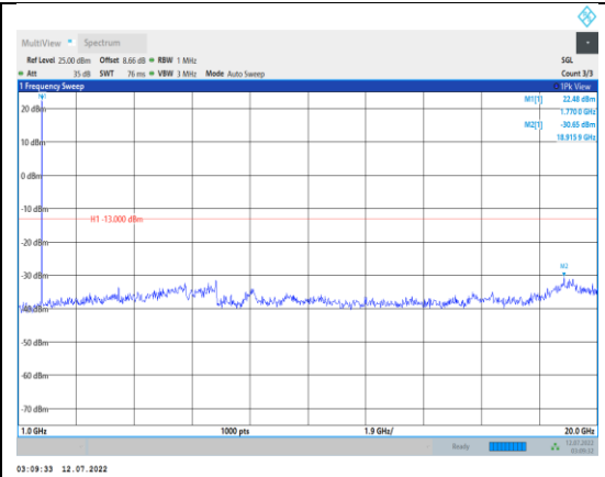
Band66-1.4MHz-16QAM-132665-1RB#0- Range2:1000~20000MHz
