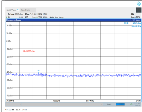
Band66-3MHz-16QAM-132322-1RB#0- Range1:30~1000MHz
