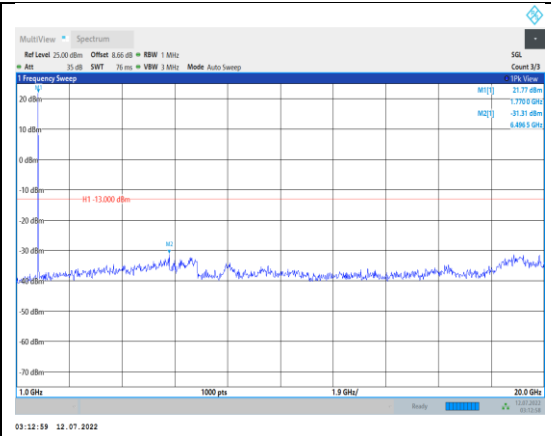
Band66-3MHz-16QAM-132657-1RB#0- Range2:1000~20000MHz
