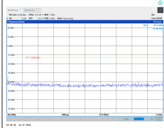
Band66-1.4MHz-QPSK-132665-1RB#0- Range1:30~1000MHz
