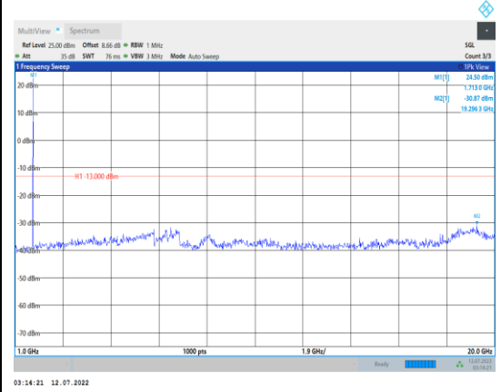
Band66-5MHz-16QAM-131997-1RB#0- Range2:1000~20000MHz
