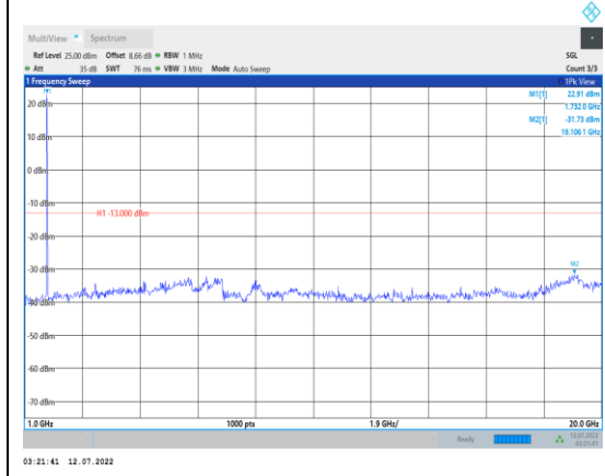
Band66-15MHz-QPSK-132322-1RB#0- Range2:1000~20000MHz
