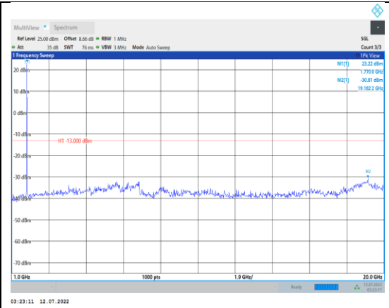
Band66-15MHz-16QAM-132597-1RB#0- Range2:1000~20000MHz
