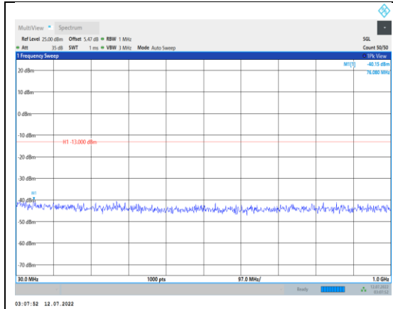
Band66-1.4MHz-QPSK-132322-1RB#0- Range1:30~1000MHz
