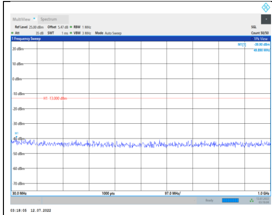
Band66-10MHz-QPSK-132322-1RB#0- Range1:30~1000MHz
