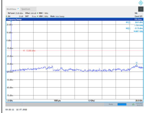
Band66-15MHz-16QAM-132322-1RB#0- Range2:1000~20000MHz
