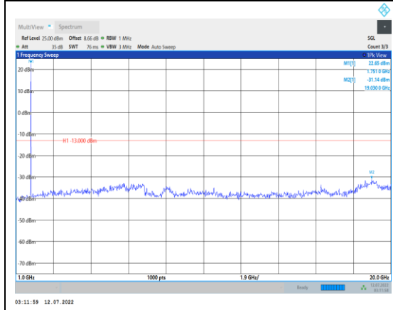
Band66-3MHz-16QAM-132322-1RB#0- Range2:1000~20000MHz
