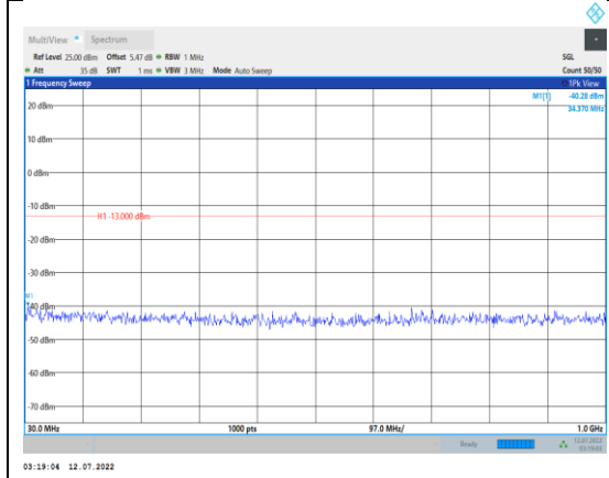
Band66-10MHz-QPSK-132622-1RB#0- Range1:30~1000MHz
