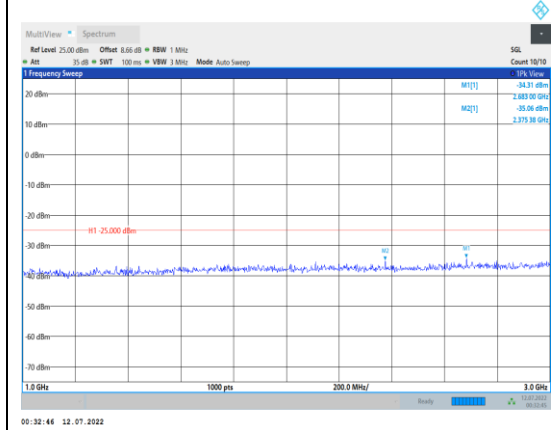
Band41-20MHz-16QAM-41490-1RB#0- Range2:1000~3000MHz
