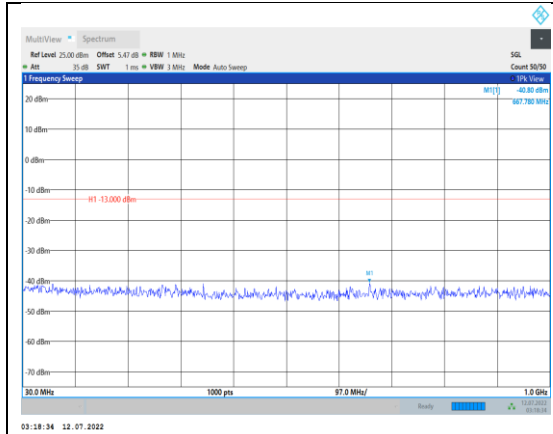
Band66-10MHz-16QAM-132322-1RB#0- Range1:30~1000MHz
