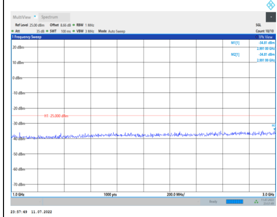
Band41-20MHz-16QAM-39750-1RB#0-Range2:1000~3000MHz
