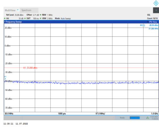
Band38-15MHz-QPSK-37825-1RB#0- Range1:30~1000MHz
