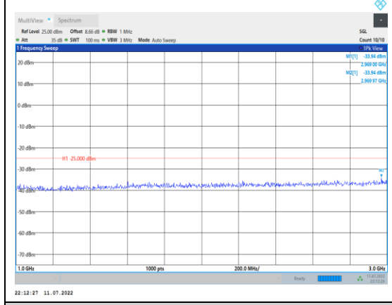
Band41-10MHz-16QAM-39700-1RB#0- Range2:1000~3000MHz
