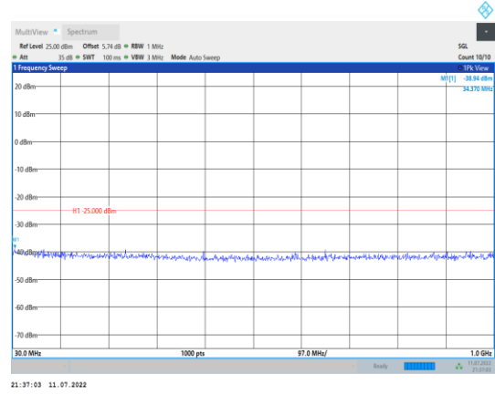
Band41-5MHz-16QAM-40620-1RB#0- Range1:30~1000MHz
