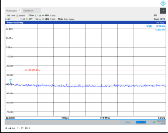
Band38-20MHz-16QAM-38000-1RB#0- Range1:30~1000MHz
