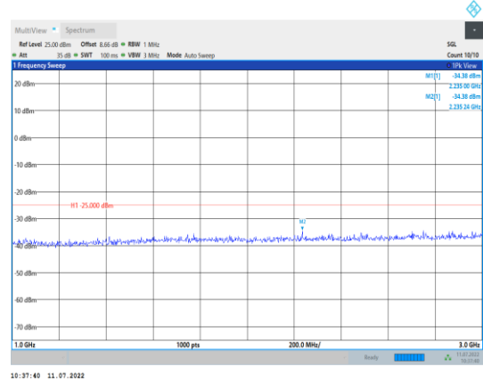
Band38-10MHz-QPSK-37800-1RB#0- Range2:1000~3000MHz
