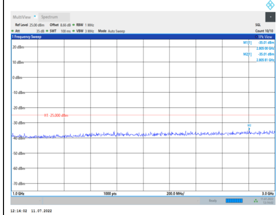
Band38-15MHz-16QAM-38175-1RB#0- Range2:1000~3000MHz
