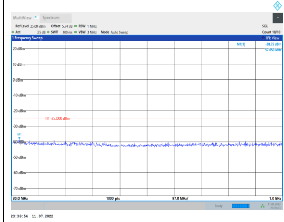
Band41-15MHz-16QAM-41515-1RB#0- Range1:30~1000MHz
