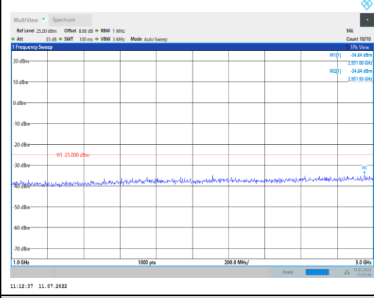
Band38-10MHz-QPSK-38200-1RB#0- Range2:1000~3000MHz
