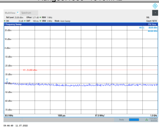
Band38-5MHz-QPSK-37775-1RB#0-Range1:30~1000MHz
