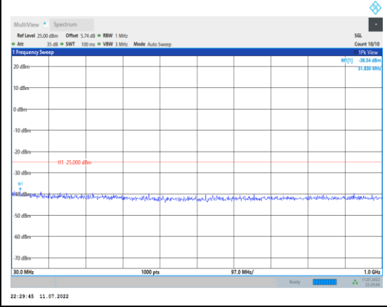
Band41-10MHz-16QAM-40620-1RB#0- Range1:30~1000MHz
