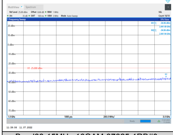
Band38-15MHz-16QAM-37825-1RB#0- Range2:1000~3000MHz
