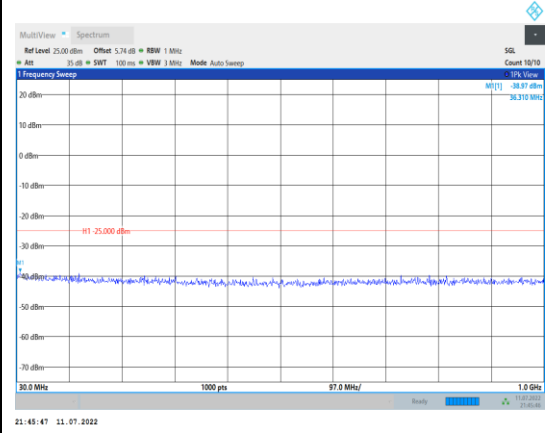
Band41-5MHz-QPSK-41565-1RB#0- Range1:30~1000MHz
