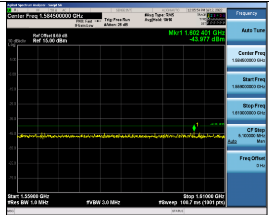
Band13-10MHz-16QAM-23230-1RB#0-Range3:1559~1610MHz
