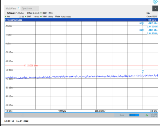
Band38-20MHz-16QAM-38000-1RB#0- Range2:1000~3000MHz
