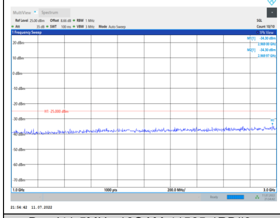
Band41-5MHz-16QAM-41565-1RB#0- Range2:1000~3000MHz
