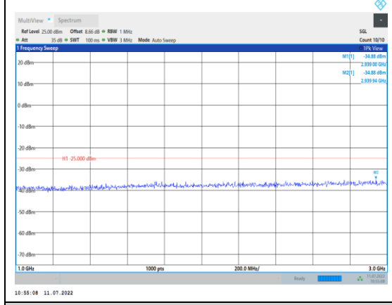
Band38-10MHz-QPSK-38000-1RB#0- Range2:1000~3000MHz
