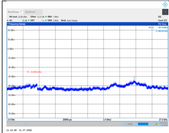
Band38-10MHz-QPSK-38200-1RB#0-Range3:3000~27000MHz
