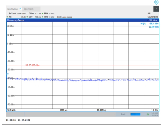
Band38-15MHz-16QAM-37825-1RB#0- Range1:30~1000MHz
