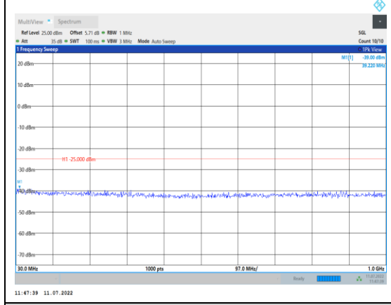
Band38-15MHz-QPSK-38000-1RB#0- Range1:30~1000MHz
