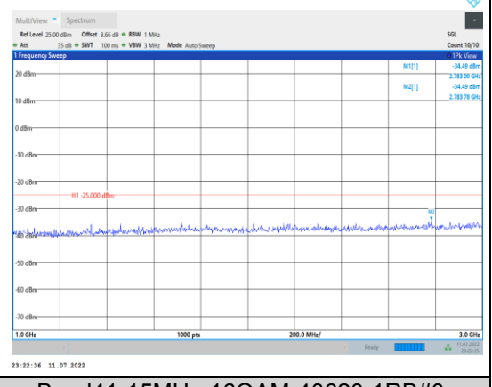
Band41-15MHz-16QAM-40620-1RB#0- Range2:1000~3000MHz
