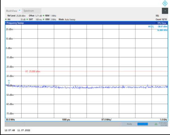
Band38-20MHz-QPSK-38150-1RB#0- Range1:30~1000MHz
