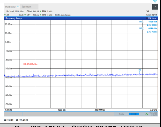
Band38-15MHz-QPSK-38175-1RB#0- Range2:1000~3000MHz
