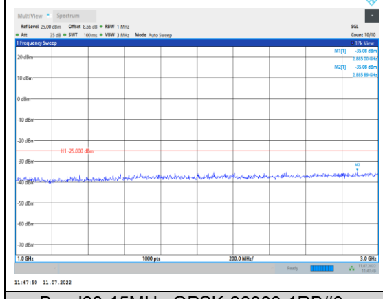
Band38-15MHz-QPSK-38000-1RB#0- Range2:1000~3000MHz
