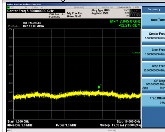
Band13-10MHz-16QAM-23230-1RB#0-Range2:1000~10000MHz
