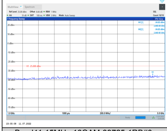
Band41-15MHz-16QAM-39725-1RB#0- Range2:1000~3000MHz
