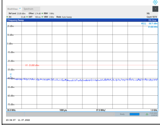
Band41-15MHz-16QAM-39725-1RB#0- Range1:30~1000MHz
