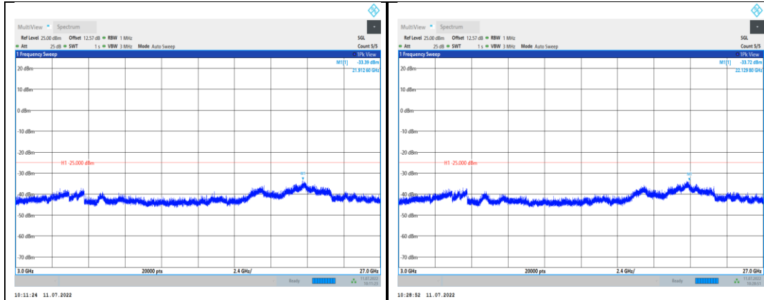
Band38-5MHz-16QAM-38000-1RB#0- Range3:3000~27000MHz
