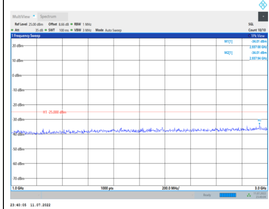
Band41-15MHz-16QAM-41515-1RB#0- Range2:1000~3000MHz
