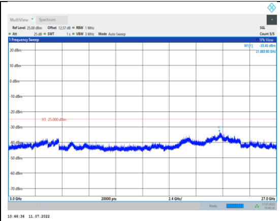
Band38-10MHz-16QAM-37800-1RB#0-Range3:3000~27000MHz
