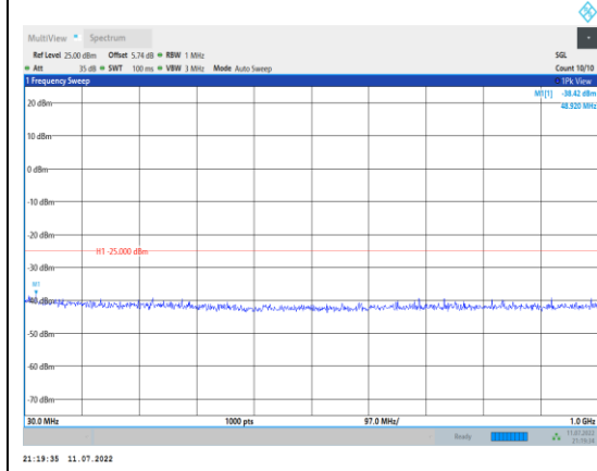
Band41-5MHz-16QAM-39675-1RB#0- Range1:30~1000MHz
