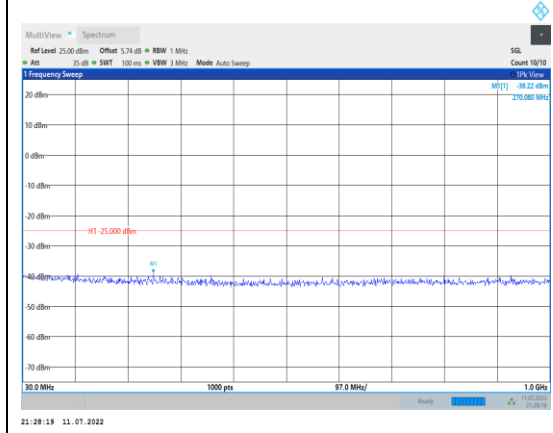
Band41-5MHz-QPSK-40620-1RB#0- Range1:30~1000MHz
