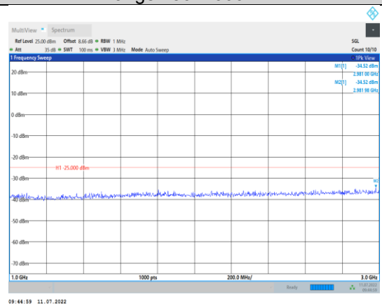
Band38-5MHz-QPSK-37775-1RB#0-Range2:1000~3000MHz
