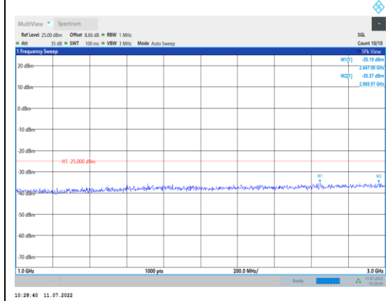
Band38-5MHz-16QAM-38225-1RB#0- Range2:1000~3000MHz
