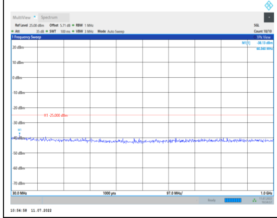
Band38-10MHz-QPSK-38000-1RB#0- Range1:30~1000MHz
