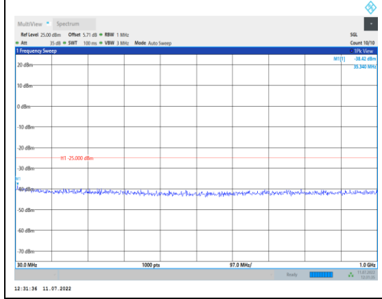
Band38-20MHz-16QAM-37850-1RB#0- Range1:30~1000MHz
