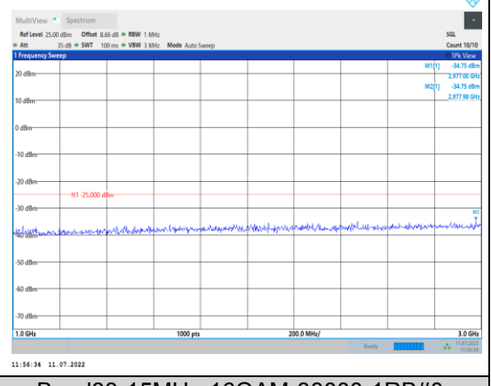
Band38-15MHz-16QAM-38000-1RB#0- Range2:1000~3000MHz
