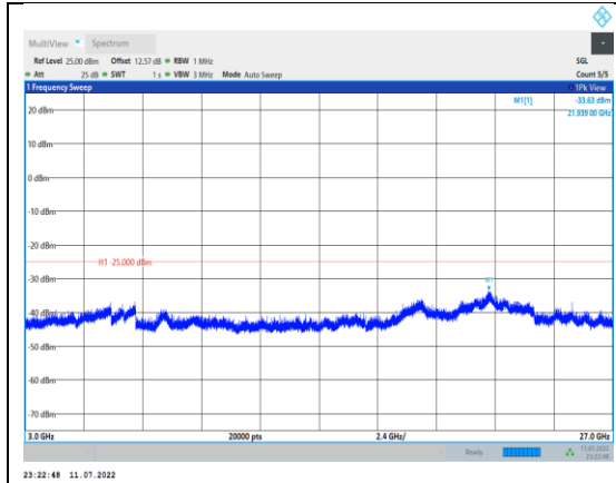
Band41-15MHz-16QAM-40620-1RB#0- Range3:3000~27000MHz
