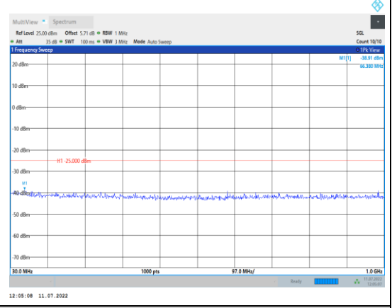
Band38-15MHz-QPSK-38175-1RB#0- Range1:30~1000MHz
