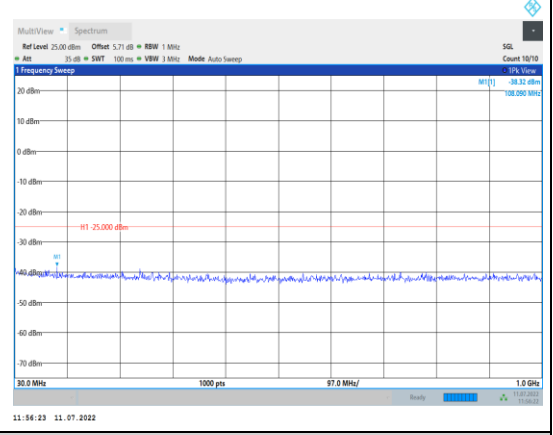
Band38-15MHz-16QAM-38000-1RB#0- Range1:30~1000MHz
