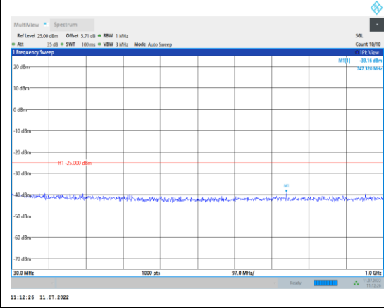
Band38-10MHz-QPSK-38200-1RB#0- Range1:30~1000MHz
