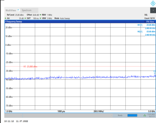
Band38-5MHz-16QAM-38000-1RB#0- Range2:1000~3000MHz
