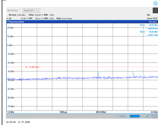
Band38-20MHz-16QAM-38150-1RB#0- Range2:1000~3000MHz
