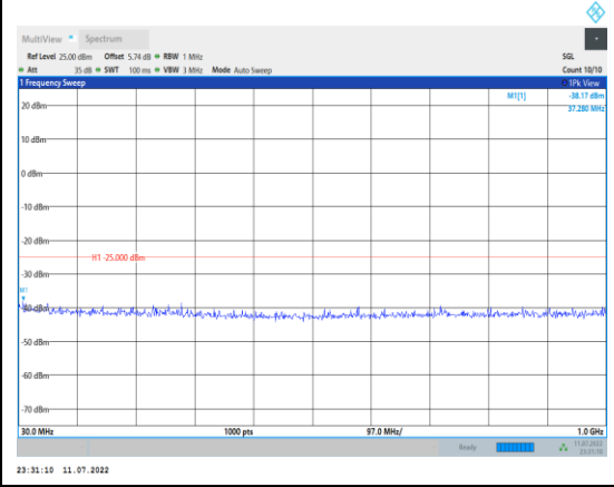
Band41-15MHz-QPSK-41515-1RB#0- Range1:30~1000MHz
