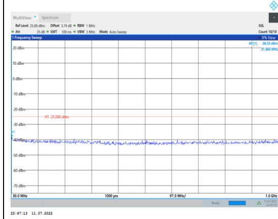
Band41-10MHz-16QAM-41540-1RB#0- Range1:30~1000MHz
