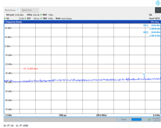
Band41-5MHz-16QAM-40620-1RB#0- Range2:1000~3000MHz
