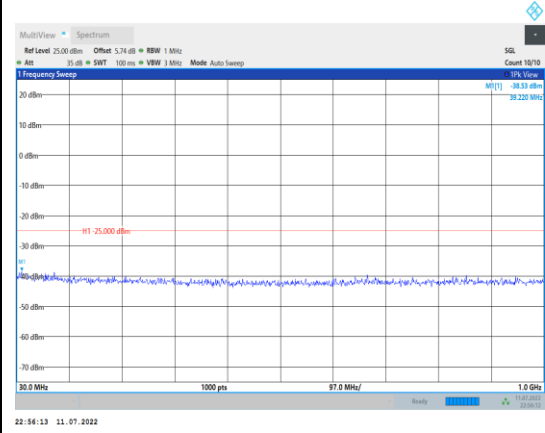
Band41-15MHz-QPSK-39725-1RB#0- Range1:30~1000MHz
