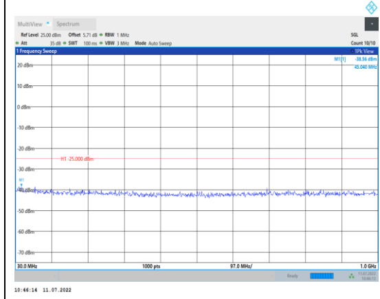
Band38-10MHz-16QAM-37800-1RB#0-Range1:30~1000MHz
