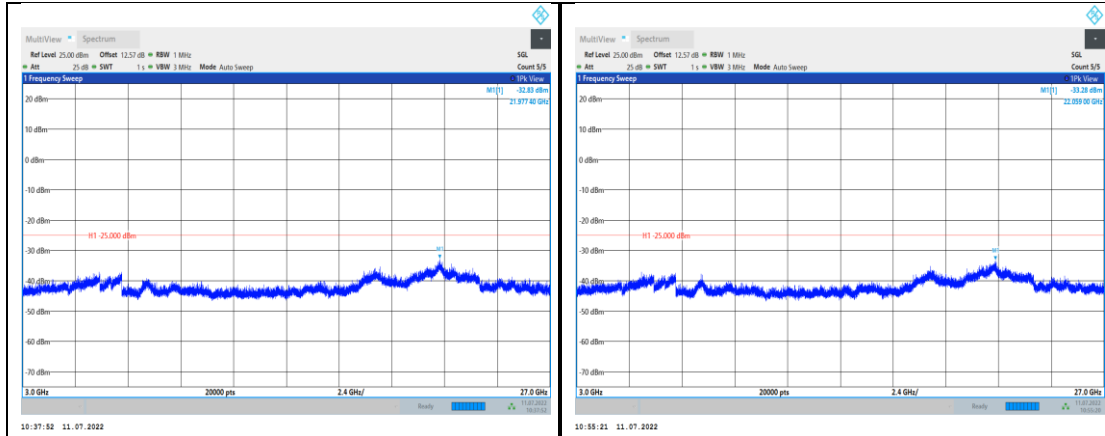
Band38-10MHz-QPSK-37800-1RB#0- Range3:3000~27000MHz
