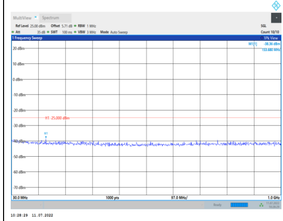
Band38-5MHz-16QAM-38225-1RB#0- Range1:30~1000MHz
