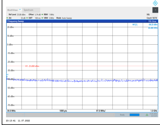
Band41-15MHz-QPSK-40620-1RB#0- Range1:30~1000MHz
