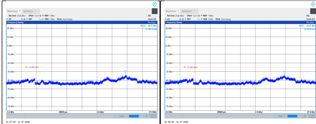
Band41-5MHz-16QAM-40620-1RB#0- Range3:3000~27000MHz
