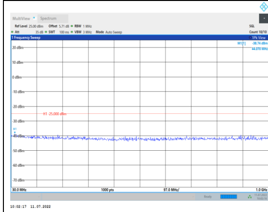
Band38-5MHz-QPSK-38000-1RB#0- Range1:30~1000MHz
