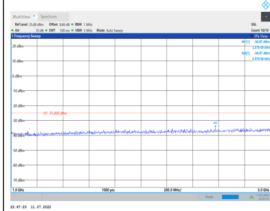
Band41-10MHz-16QAM-41540-1RB#0- Range2:1000~3000MHz
