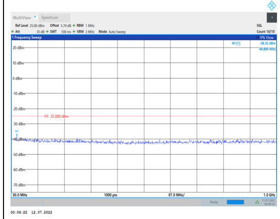
Band41-20MHz-QPSK-40620-1RB#0- Range1:30~1000MHz
