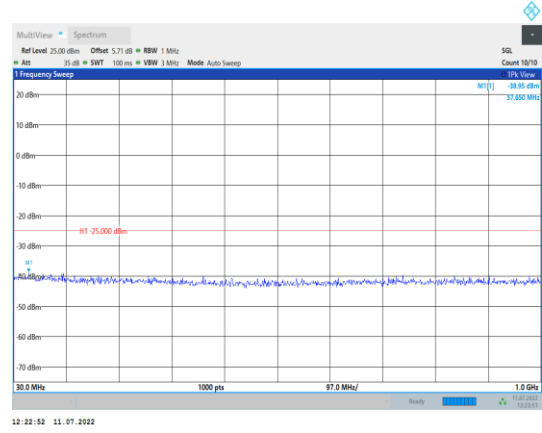
Band38-20MHz-QPSK-37850-1RB#0- Range1:30~1000MHz
