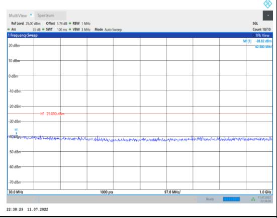
Band41-10MHz-QPSK-41540-1RB#0- Range1:30~1000MHz
