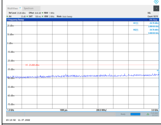
Band41-15MHz-QPSK-40620-1RB#0- Range2:1000~3000MHz
