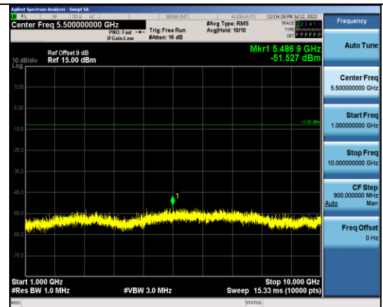
Band13-10MHz-QPSK-23230-1RB#0- Range2:1000~10000MHz
