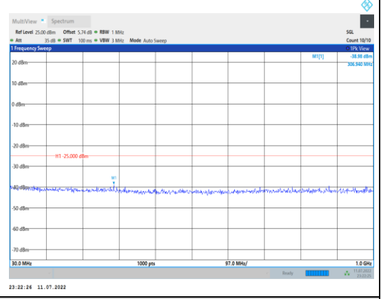
Band41-15MHz-16QAM-40620-1RB#0- Range1:30~1000MHz
