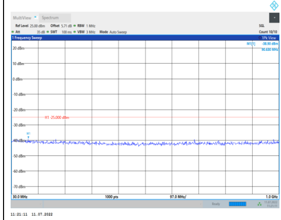
Band38-10MHz-16QAM-38200-1RB#0- Range1:30~1000MHz
