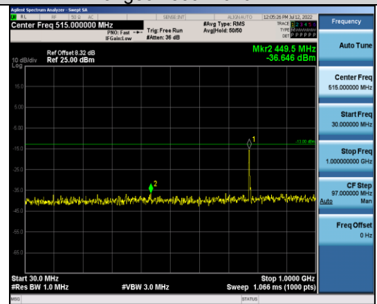
Band13-10MHz-16QAM-23230-1RB#0- Range1:30~1000MHz
