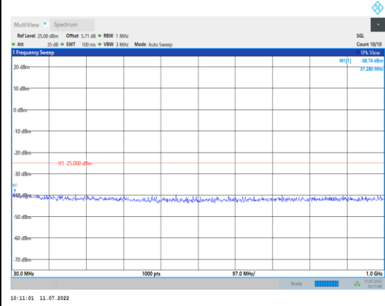
Band38-5MHz-16QAM-38000-1RB#0- Range1:30~1000MHz
