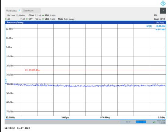
Band38-10MHz-16QAM-38000-1RB#0-Range1:30~1000MHz
