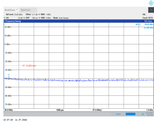
Band38-10MHz-QPSK-37800-1RB#0- Range1:30~1000MHz
