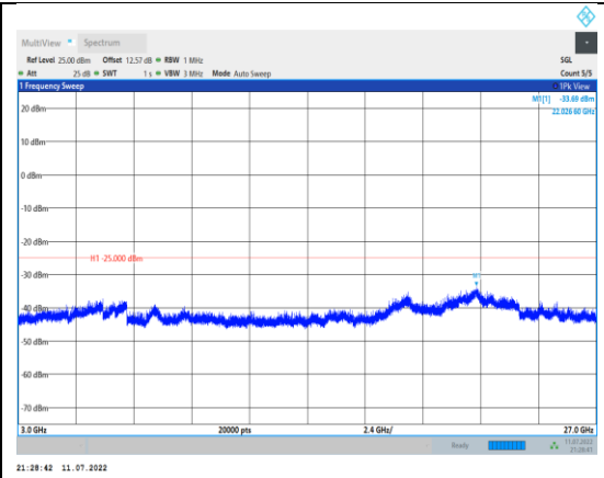
Band41-5MHz-QPSK-40620-1RB#0- Range3:3000~27000MHz
