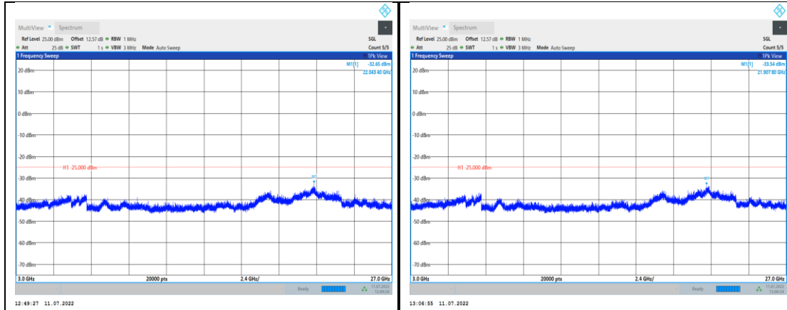
Band38-20MHz-16QAM-38000-1RB#0- Range3:3000~27000MHz
