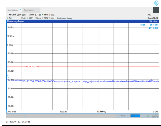
Band38-20MHz-QPSK-38000-1RB#0- Range1:30~1000MHz
