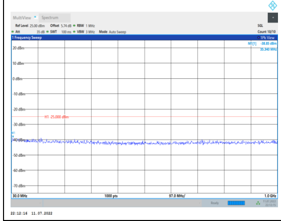
Band41-10MHz-16QAM-39700-1RB#0- Range1:30~1000MHz
