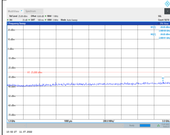
Band38-5MHz-QPSK-38000-1RB#0- Range2:1000~3000MHz
