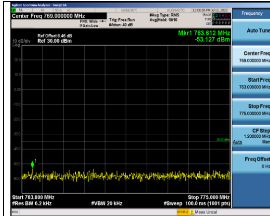
Band13-10MHz-16QAM-23230-1RB#0-Range4:763~775MHz
