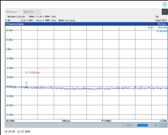
Band38-5MHz-QPSK-38225-1RB#0- Range1:30~1000MHz
