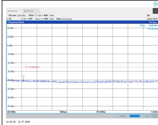
Band38-20MHz-16QAM-38150-1RB#0- Range1:30~1000MHz
