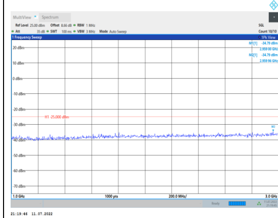
Band41-5MHz-16QAM-39675-1RB#0- Range2:1000~3000MHz
