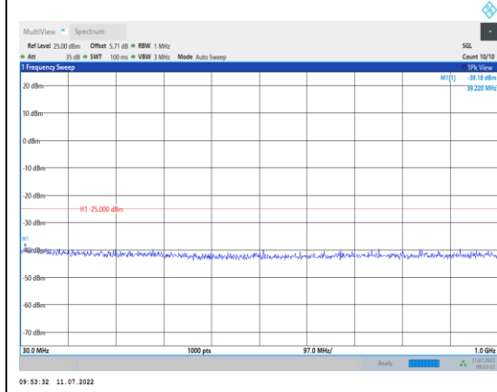
Band38-5MHz-16QAM-37775-1RB#0- Range1:30~1000MHz
