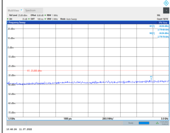
Band38-10MHz-16QAM-37800-1RB#0-Range2:1000~3000MHz
