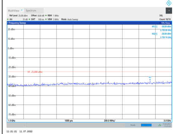
Band38-10MHz-16QAM-38200-1RB#0- Range2:1000~3000MHz
