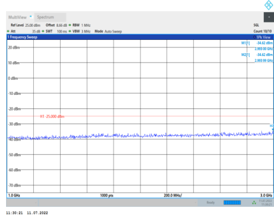
Band38-15MHz-QPSK-37825-1RB#0- Range2:1000~3000MHz
