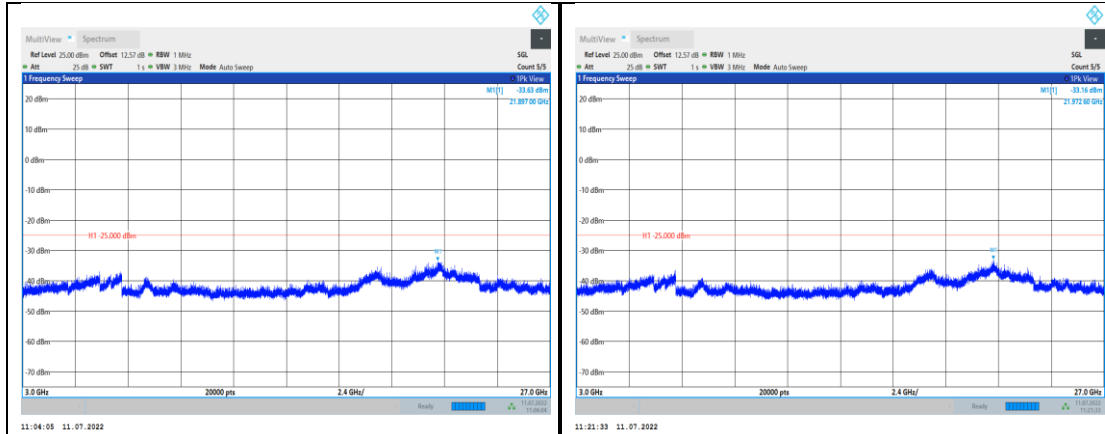
Band38-10MHz-16QAM-38000-1RB#0- Range3:3000~27000MHz
