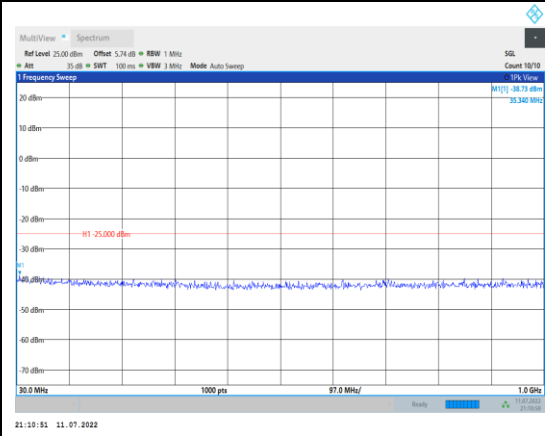
Band41-5MHz-QPSK-39675-1RB#0- Range1:30~1000MHz
