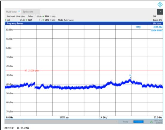
Band41-15MHz-16QAM-41515-1RB#0- Range3:3000~27000MHz
