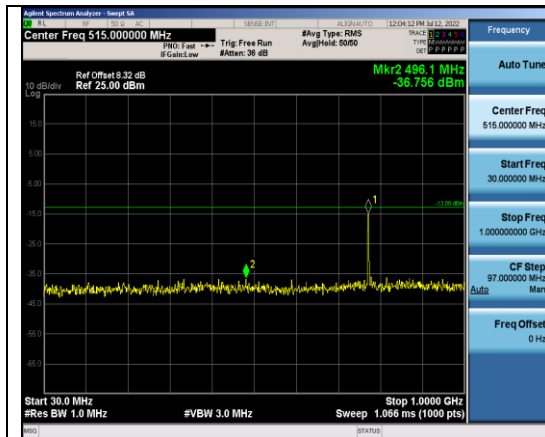
Band13-10MHz-QPSK-23230-1RB#0- Range1:30~1000MHz
