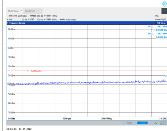
Band38-5MHz-16QAM-37775-1RB#0- Range2:1000~3000MHz
