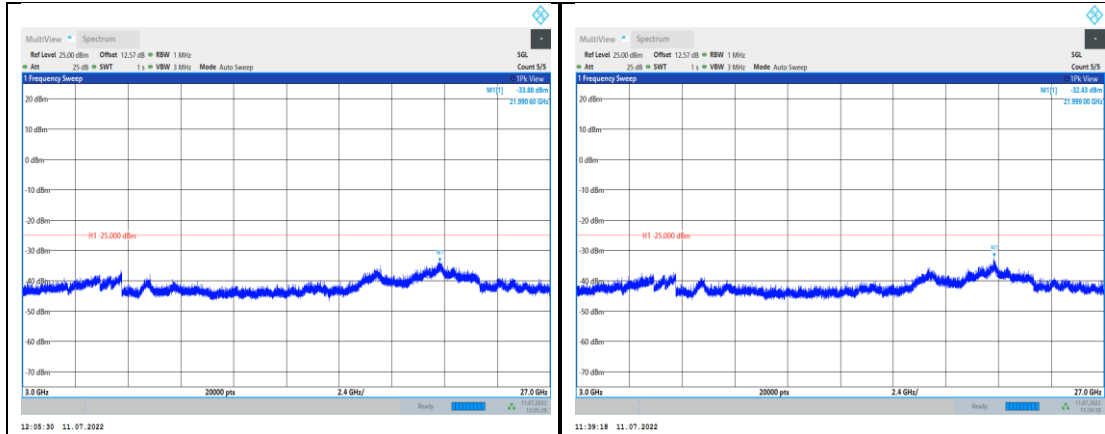
Band38-15MHz-QPSK-38175-1RB#0- Range3:3000~27000MHz
