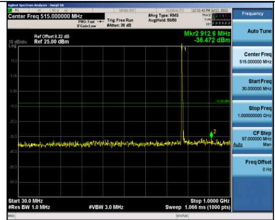
Band13-5MHz-16QAM-23205-1RB#0- Range1:30~1000MHz
