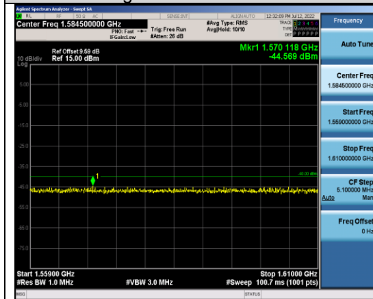
Band13-5MHz-16QAM-23205-1RB#0- Range3:1559~1610MHz
