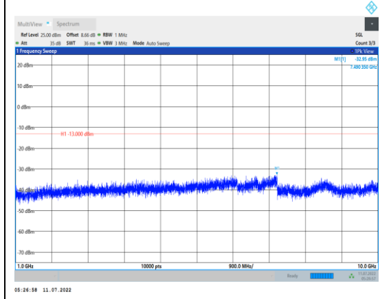
Band5-10MHz-QPSK-20450-1RB#0- Range2:1000~10000MHz
