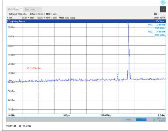
Band7-15MHz-16QAM-21100-1RB#0- Range2:1000~3000MHz
