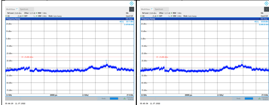
Band7-5MHz-16QAM-21100-1RB#0- Range3:3000~27000MHz
