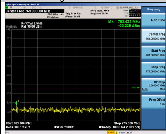
Band13-5MHz-QPSK-23255-1RB#0- Range4:763~775MHz
