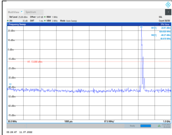
Band5-10MHz-QPSK-20450-1RB#0- Range1:30~1000MHz
