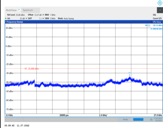
Band7-15MHz-QPSK-21100-1RB#0- Range3:3000~27000MHz
