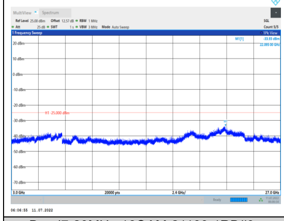
Band7-20MHz-16QAM-21100-1RB#0- Range3:3000~27000MHz
