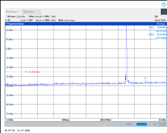
Band7-15MHz-16QAM-20825-1RB#0- Range2:1000~3000MHz
