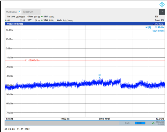
Band5-10MHz-16QAM-20525-1RB#0- Range2:1000~10000MHz
