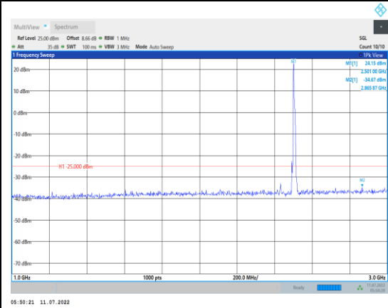
Band7-10MHz-16QAM-20800-1RB#0- Range2:1000~3000MHz
