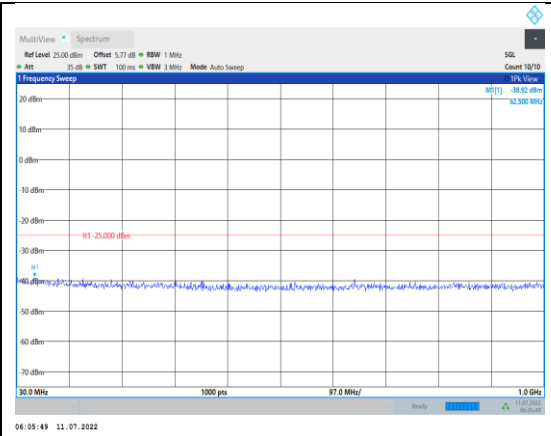
Band7-20MHz-QPSK-21100-1RB#0-Range1:30~1000MHz
