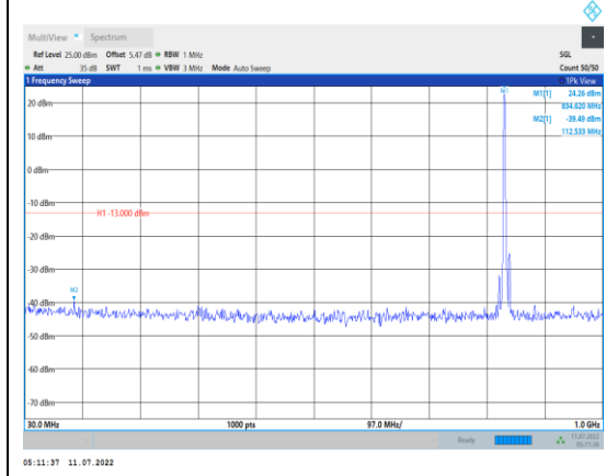
Band5-5MHz-16QAM-20525-1RB#0- Range1:30~1000MHz
