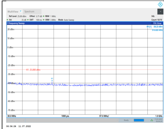
Band7-20MHz-QPSK-20850-1RB#0-Range1:30~1000MHz
