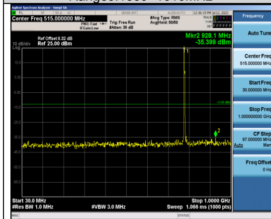
Band13-5MHz-16QAM-23255-1RB#0- Range1:30~1000MHz
