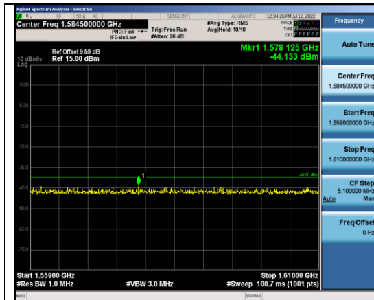
Band13-5MHz-16QAM-23230-1RB#0- Range3:1559~1610MHz
