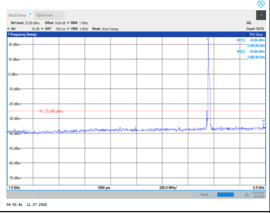
Band7-15MHz-16QAM-21375-1RB#0- Range2:1000~3000MHz
