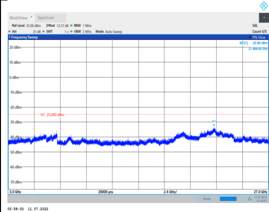
Band7-15MHz-16QAM-20825-1RB#0- Range3:3000~27000MHz
