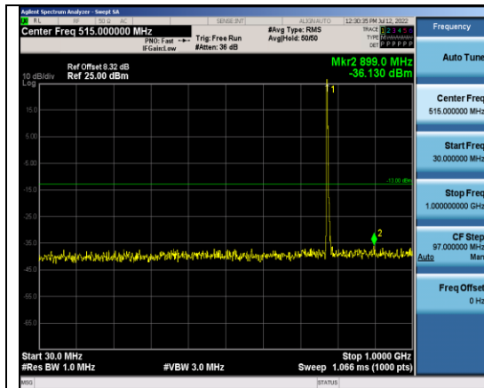
Band13-5MHz-QPSK-23205-1RB#0- Range1:30~1000MHz
