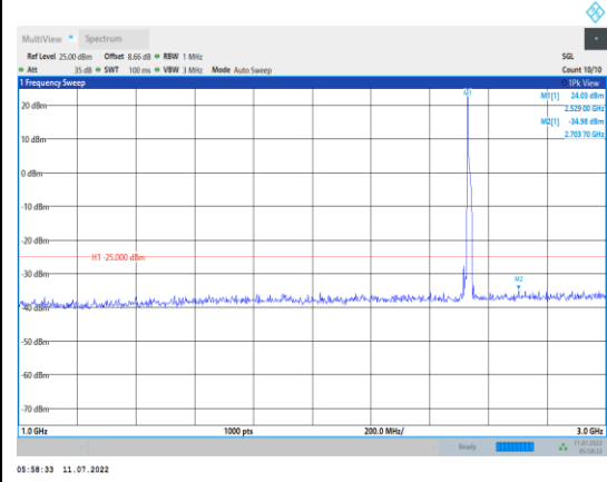
Band7-15MHz-QPSK-21100-1RB#0- Range2:1000~3000MHz
