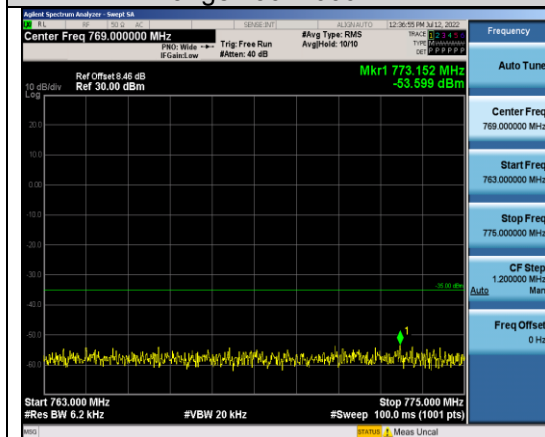
Band13-5MHz-16QAM-23255-1RB#0- Range4:763~775MHz
