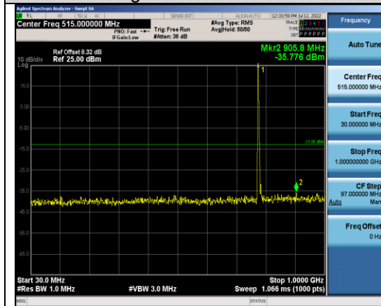
Band13-5MHz-16QAM-23230-1RB#0- Range1:30~1000MHz
