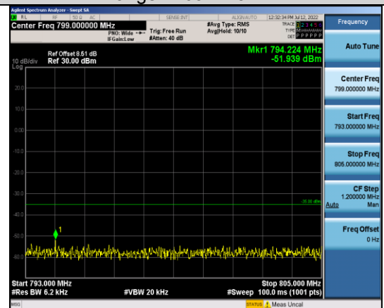
Band13-5MHz-16QAM-23205-1RB#0- Range5:793~805MHz
