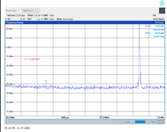
Band5-5MHz-16QAM-20625-1RB#0- Range1:30~1000MHz
