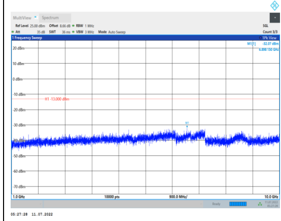
Band5-10MHz-16QAM-20450-1RB#0- Range2:1000~10000MHz
