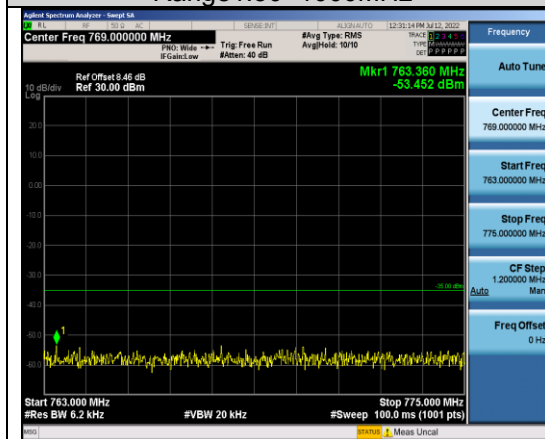
Band13-5MHz-QPSK-23205-1RB#0- Range4:763~775MHz
