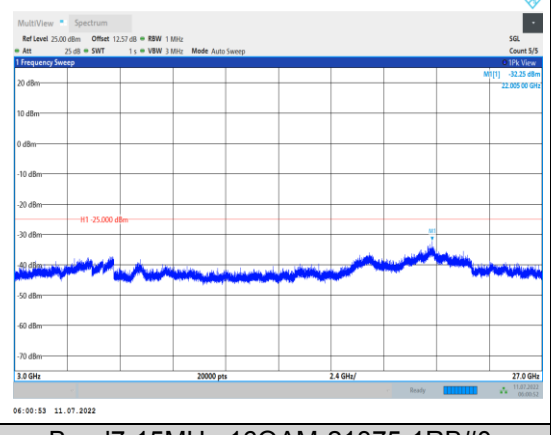
Band7-15MHz-16QAM-21375-1RB#0- Range3:3000~27000MHz
