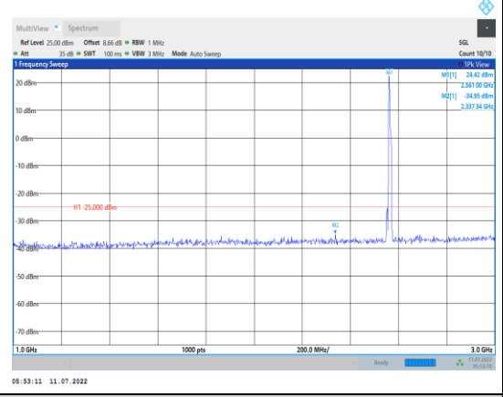
Band7-10MHz-16QAM-21400-1RB#0- Range2:1000~3000MHz
