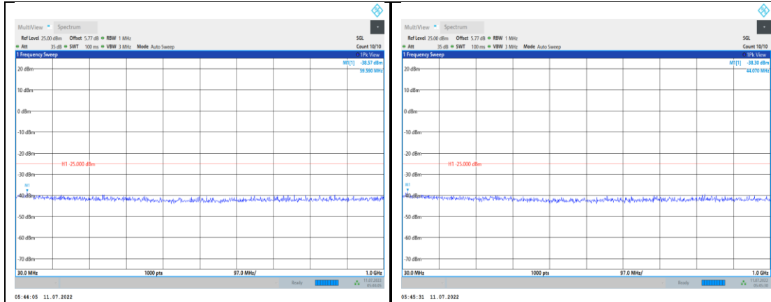
Band7-5MHz-16QAM-21100-1RB#0- Range1:30~1000MHz
