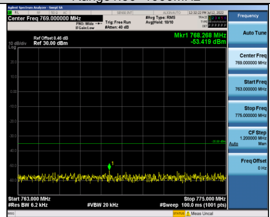
Band13-5MHz-16QAM-23205-1RB#0- Range4:763~775MHz
