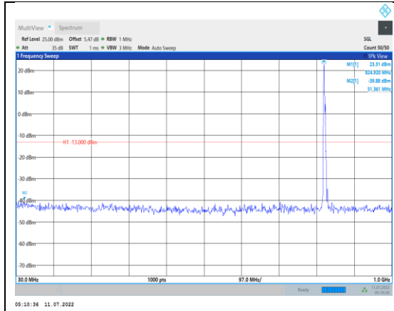
Band5-5MHz-16QAM-20425-1RB#0- Range1:30~1000MHz
