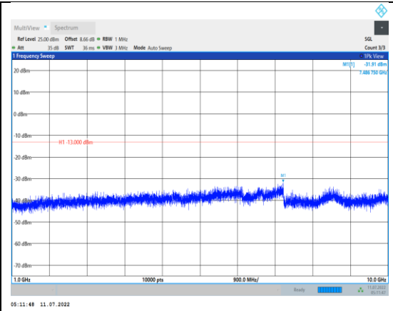
Band5-5MHz-16QAM-20525-1RB#0- Range2:1000~10000MHz
