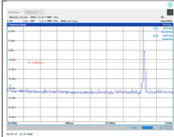
Band5-10MHz-16QAM-20450-1RB#0- Range1:30~1000MHz
