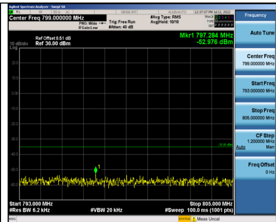
Band13-5MHz-16QAM-23255-1RB#0- Range5:793~805MHz
