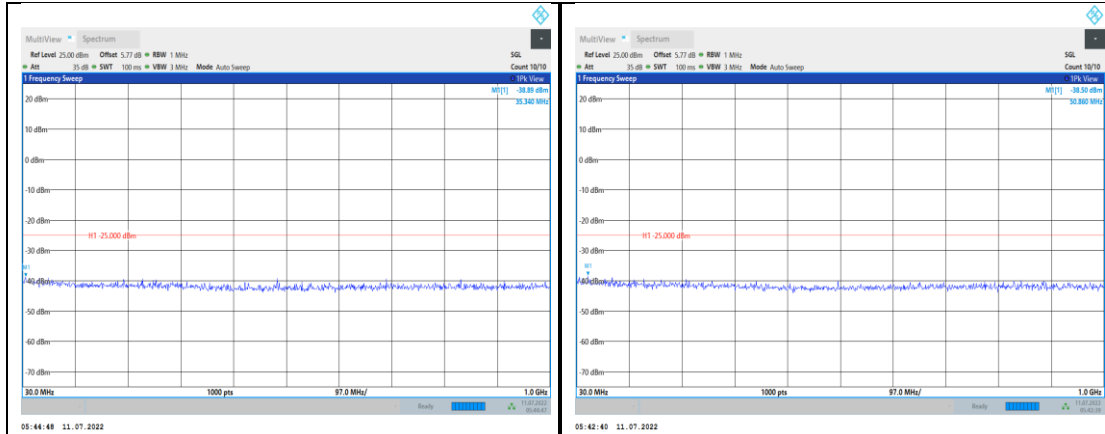
Band7-5MHz-QPSK-21425-1RB#0- Range1:30~1000MHz
