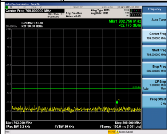
Band13-5MHz-16QAM-23230-1RB#0- Range5:793~805MHz
