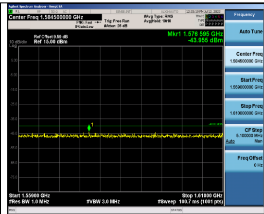
Band13-5MHz-QPSK-23230-1RB#0- Range3:1559~1610MHz
