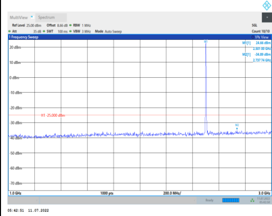
Band7-5MHz-16QAM-20775-1RB#0- Range2:1000~3000MHz
