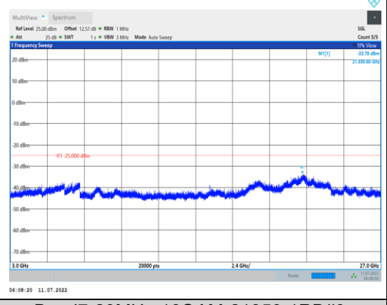
Band7-20MHz-16QAM-21350-1RB#0- Range3:3000~27000MHz
