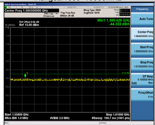
Band13-5MHz-QPSK-23205-1RB#0- Range3:1559~1610MHz
