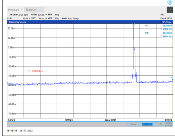
Band7-20MHz-16QAM-21100-1RB#0- Range2:1000~3000MHz
