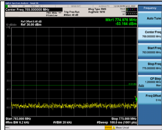
Band13-5MHz-16QAM-23230-1RB#0- Range4:763~775MHz
