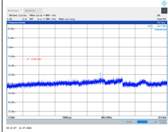
Band5-5MHz-16QAM-20425-1RB#0- Range2:1000~10000MHz
