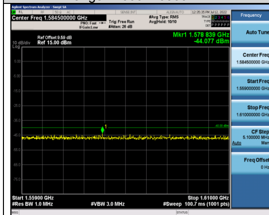
Band13-5MHz-QPSK-23255-1RB#0- Range3:1559~1610MHz
