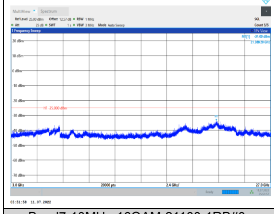
Band7-10MHz-16QAM-21100-1RB#0- Range3:3000~27000MHz
