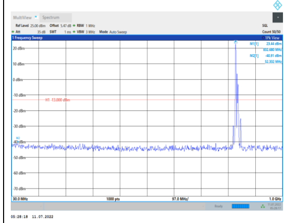
Band5-10MHz-16QAM-20525-1RB#0- Range1:30~1000MHz
