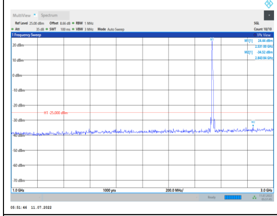
Band7-10MHz-16QAM-21100-1RB#0- Range2:1000~3000MHz
