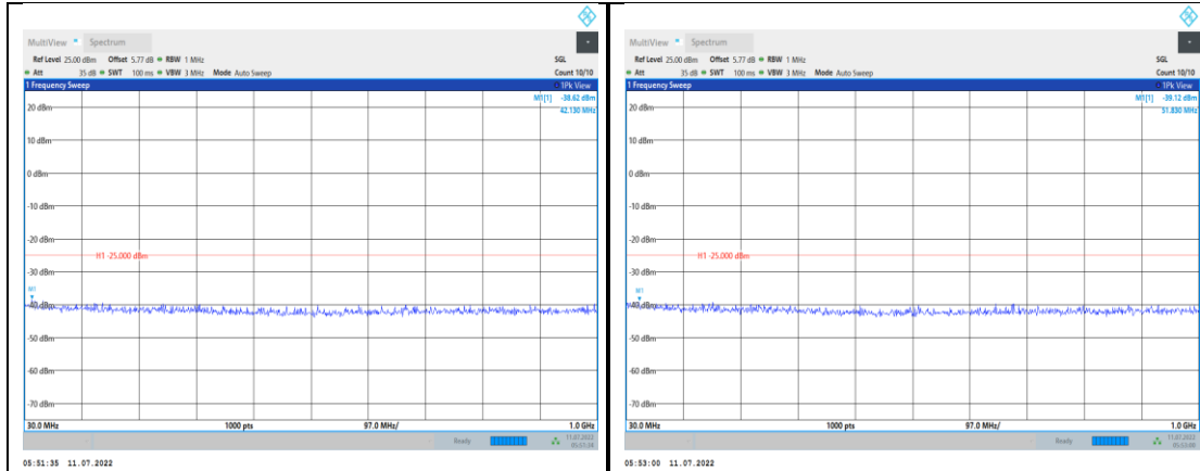
Band7-10MHz-16QAM-21100-1RB#0- Range1:30~1000MHz
