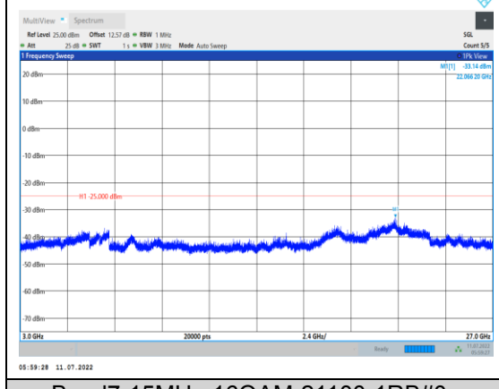
Band7-15MHz-16QAM-21100-1RB#0- Range3:3000~27000MHz
