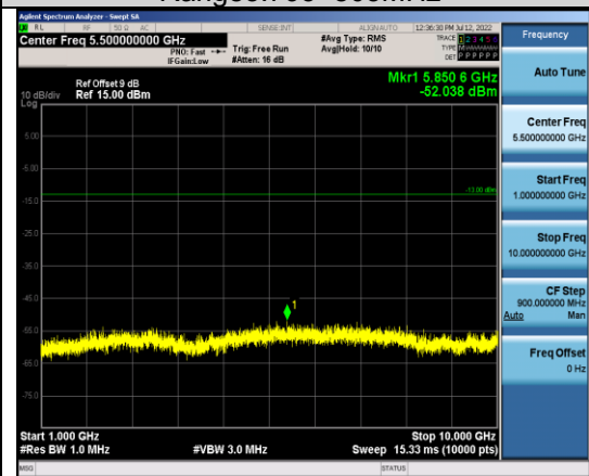
Band13-5MHz-16QAM-23255-1RB#0- Range2:1000~10000MHz
