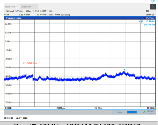
Band7-10MHz-16QAM-21400-1RB#0- Range3:3000~27000MHz
