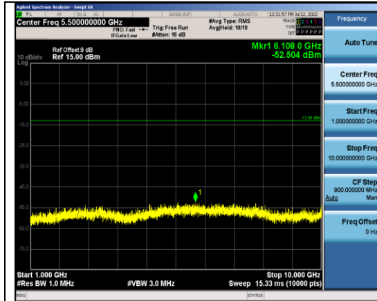
Band13-5MHz-16QAM-23205-1RB#0- Range2:1000~10000MHz
