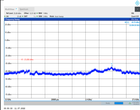
Band7-10MHz-16QAM-20800-1RB#0- Range3:3000~27000MHz
