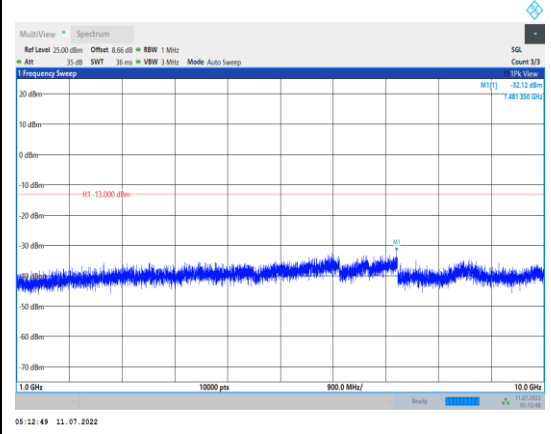
Band5-5MHz-16QAM-20625-1RB#0- Range2:1000~10000MHz
