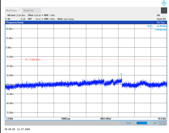
Band5-10MHz-16QAM-20600-1RB#0- Range2:1000~10000MHz
