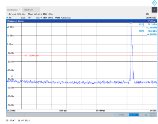
Band5-10MHz-QPSK-20525-1RB#0- Range1:30~1000MHz
