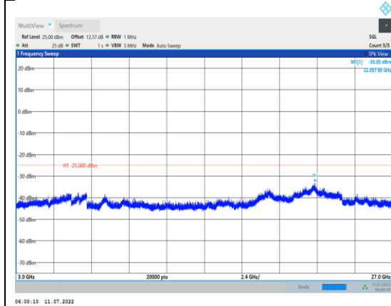
Band7-15MHz-QPSK-21375-1RB#0- Range3:3000~27000MHz
