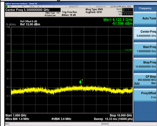
Band13-5MHz-16QAM-23230-1RB#0- Range2:1000~10000MHz
