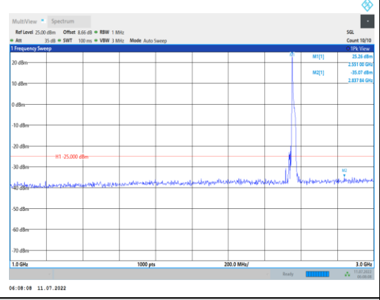
Band7-20MHz-16QAM-21350-1RB#0- Range2:1000~3000MHz
