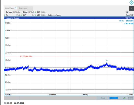
Band7-5MHz-16QAM-20775-1RB#0- Range3:3000~27000MHz
