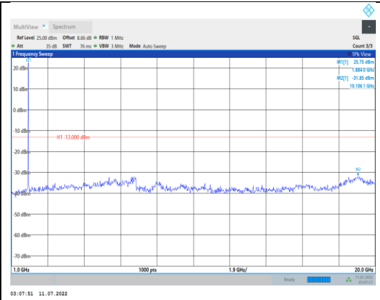
Band2-10MHz-QPSK-18900-1RB#0- Range2:1000~20000MHz
