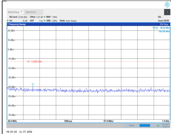
Band4-1.4MHz-16QAM-19957-1RB#0- Range1:30~1000MHz
