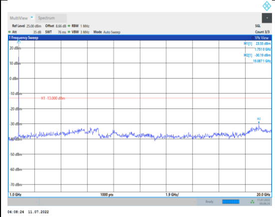
Band4-3MHz-16QAM-20385-1RB#0- Range2:1000~20000MHz
