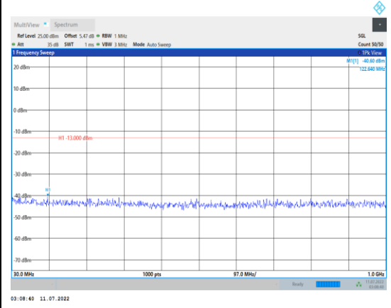
Band2-10MHz-QPSK-19150-1RB#0- Range1:30~1000MHz
