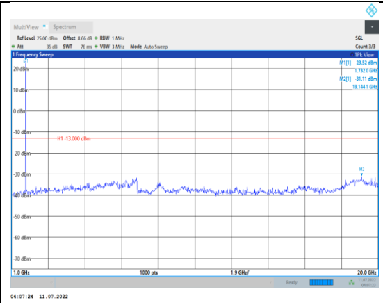
Band4-3MHz-16QAM-20175-1RB#0- Range2:1000~20000MHz
