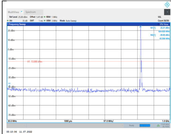
Band5-5MHz-QPSK-20425-1RB#0- Range1:30~1000MHz
