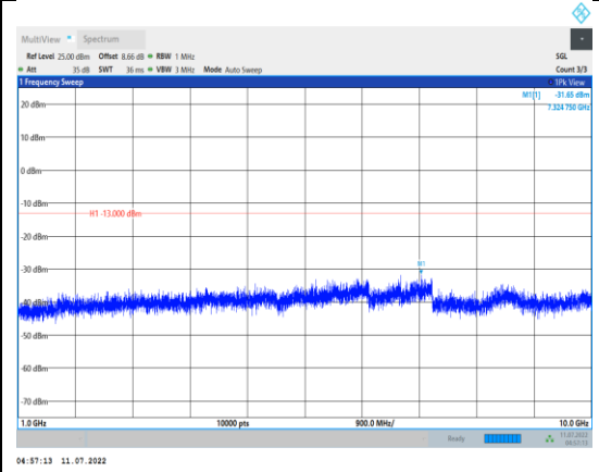
Band5-1.4MHz-16QAM-20643-1RB#0- Range2:1000~10000MHz
