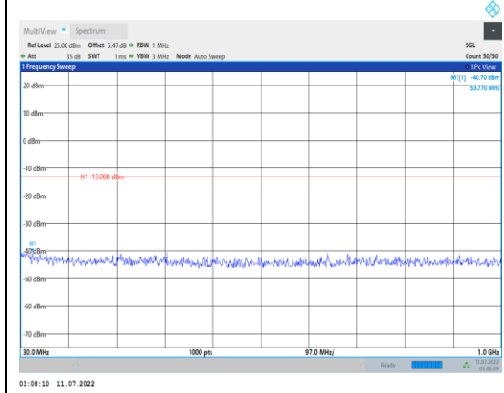
Band2-10MHz-16QAM-18900-1RB#0- Range1:30~1000MHz
