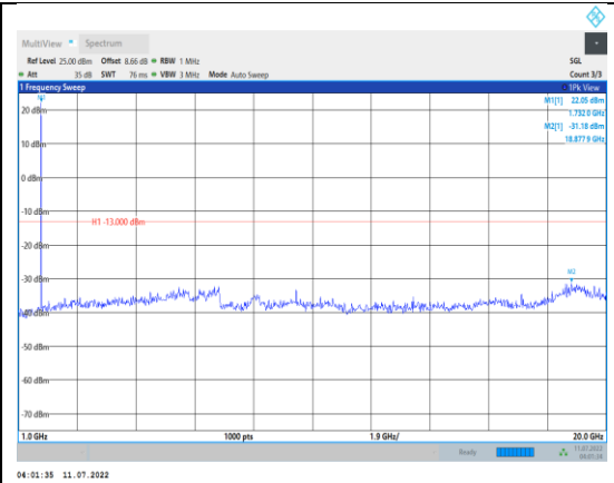
Band4-1.4MHz-16QAM-20175-1RB#0- Range2:1000~20000MHz
