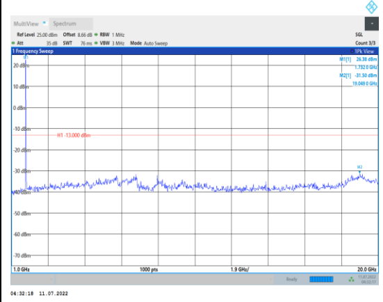
Band4-20MHz-16QAM-20300-1RB#0- Range2:1000~20000MHz
