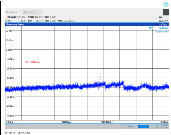
Band5-1.4MHz-QPSK-20525-1RB#0- Range2:1000~10000MHz
