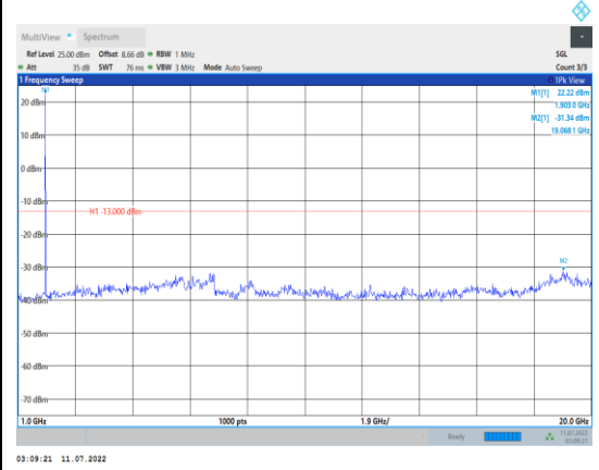
Band2-10MHz-16QAM-19150-1RB#0- Range2:1000~20000MHz
