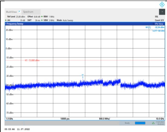
Band5-3MHz-16QAM-20525-1RB#0- Range2:1000~10000MHz
