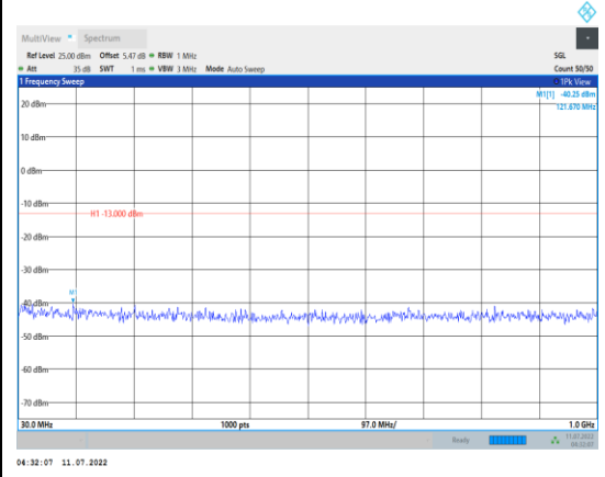
Band4-20MHz-16QAM-20300-1RB#0- Range1:30~1000MHz
