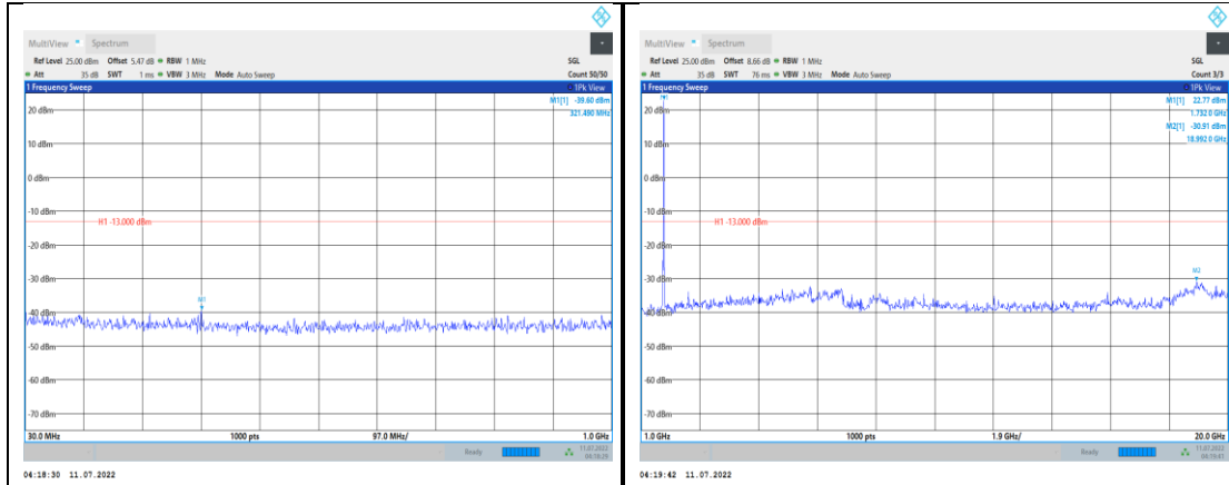
Band4-10MHz-16QAM-2000-1RB#0- Range1:30~1000MHz
