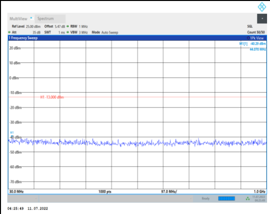
Band4-15MHz-QPSK-20325-1RB#0- Range1:30~1000MHz
