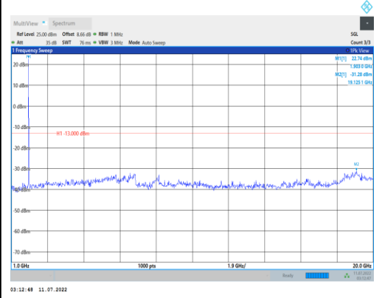
Band2-15MHz-16QAM-19125-1RB#0- Range2:1000~20000MHz
