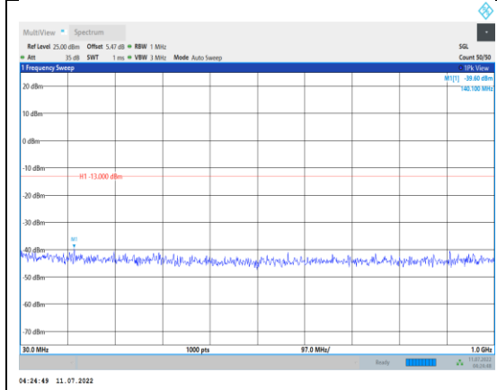
Band4-15MHz-QPSK-20175-1RB#0- Range1:30~1000MHz
