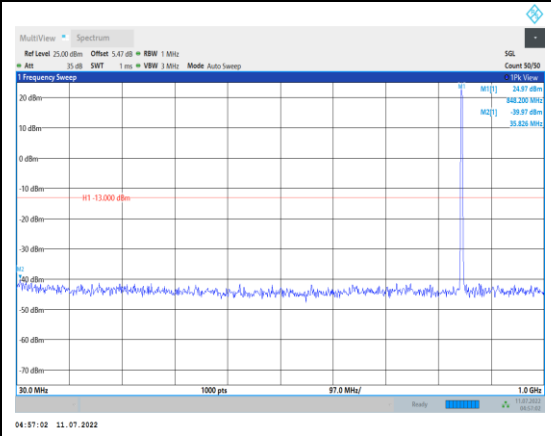
Band5-1.4MHz-16QAM-20643-1RB#0- Range1:30~1000MHz
