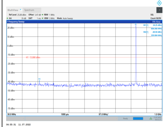
Band5-1.4MHz-QPSK-20525-1RB#0- Range1:30~1000MHz
