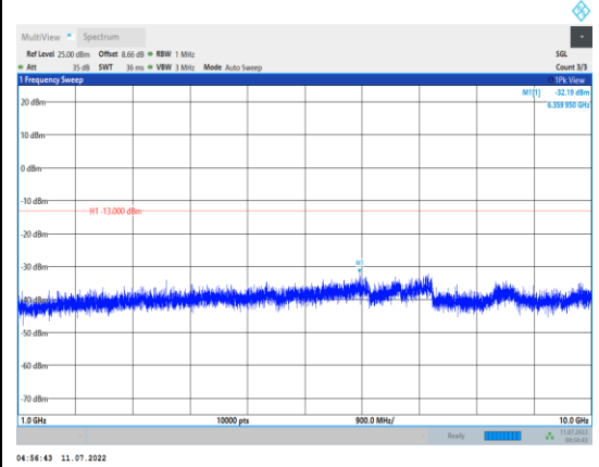
Band5-1.4MHz-QPSK-20643-1RB#0- Range2:1000~10000MHz
