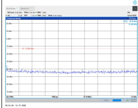
Band4-1.4MHz-16QAM-20175-1RB#0- Range1:30~1000MHz
