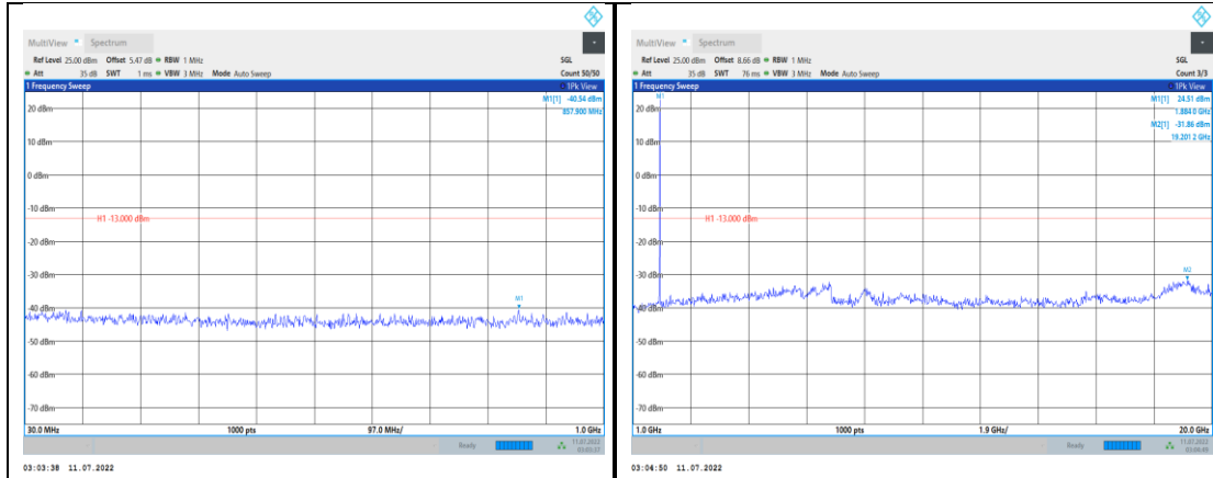
Band2-5MHz-16QAM-18625-1RB#0- Range1:30~1000MHz
