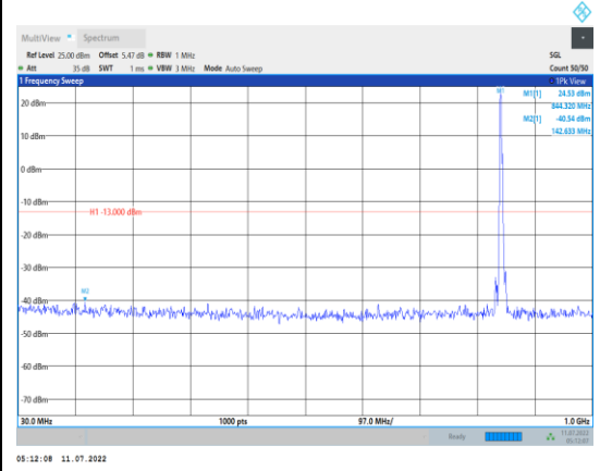
Band5-5MHz-QPSK-20625-1RB#0- Range1:30~1000MHz
