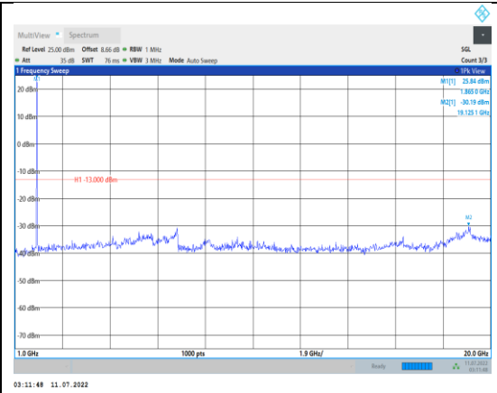
Band2-15MHz-16QAM-18900-1RB#0- Range2:1000~20000MHz
