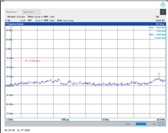
Band4-5MHz-16QAM-20175-1RB#0- Range2:1000~20000MHz
