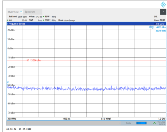
Band2-15MHz-16QAM-18675-1RB#0- Range1:30~1000MHz
