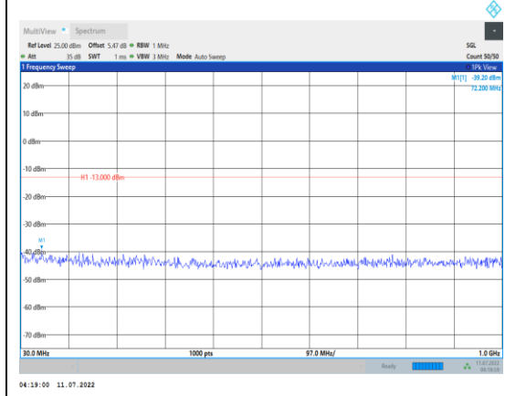
Band4-10MHz-QPSK-20175-1RB#0- Range1:30~1000MHz
