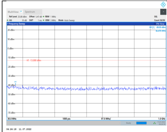
Band4-15MHz-16QAM-20025-1RB#0- Range1:30~1000MHz
