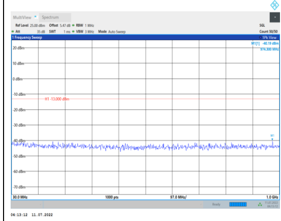
Band4-5MHz-QPSK-20175-1RB#0- Range1:30~1000MHz
