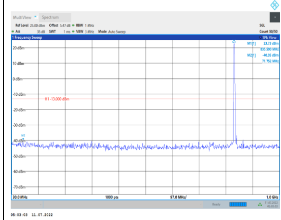
Band5-3MHz-QPSK-20525-1RB#0- Range1:30~1000MHz
