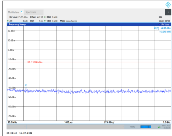
Band2-10MHz-QPSK-18650-1RB#0- Range1:30~1000MHz
