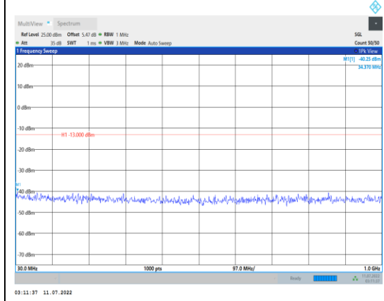
Band2-15MHz-16QAM-18900-1RB#0- Range1:30~1000MHz
