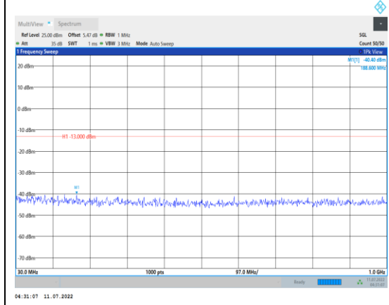
Band4-20MHz-16QAM-20175-1RB#0- Range1:30~1000MHz
