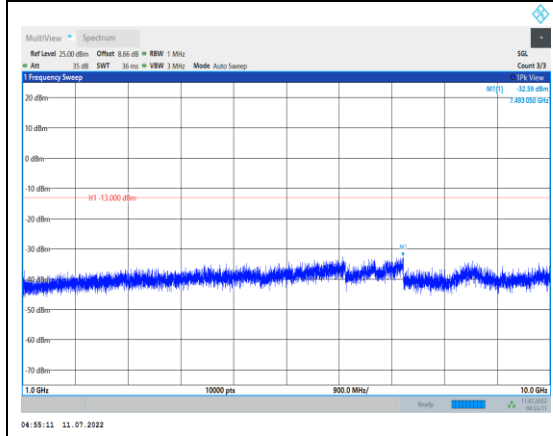
Band5-1.4MHz-16QAM-20407-1RB#0- Range2:1000~10000MHz
