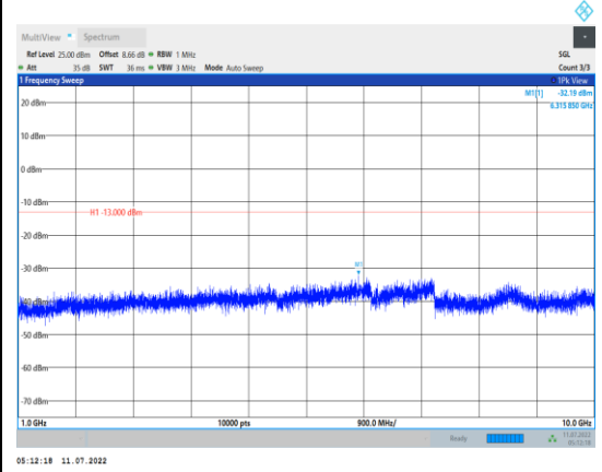
Band5-5MHz-QPSK-20625-1RB#0- Range2:1000~10000MHz
