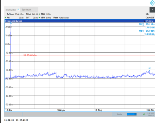
Band4-1.4MHz-16QAM-20393-1RB#0- Range2:1000~20000MHz
