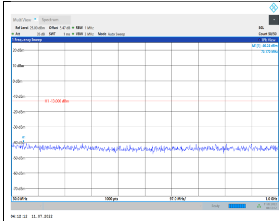
Band4-5MHz-QPSK-19975-1RB#0- Range1:30~1000MHz
