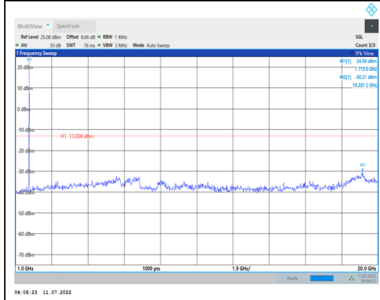
Band4-3MHz-16QAM-19965-1RB#0- Range2:1000~20000MHz
