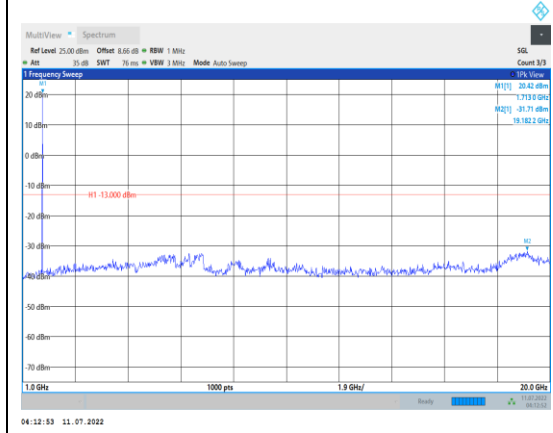
Band4-5MHz-16QAM-19975-1RB#0- Range2:1000~20000MHz
