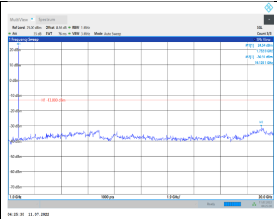
Band4-15MHz-16QAM-20175-1RB#0- Range2:1000~20000MHz
