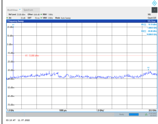
Band2-15MHz-16QAM-18675-1RB#0- Range2:1000~20000MHz
