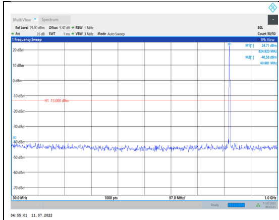
Band5-1.4MHz-16QAM-20407-1RB#0- Range1:30~1000MHz
