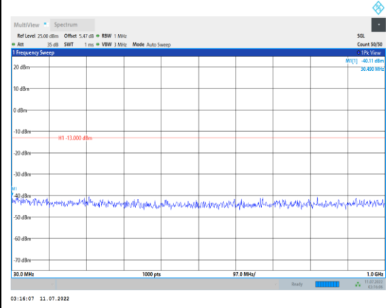
Band2-20MHz-16QAM-19100-1RB#0- Range1:30~1000MHz
