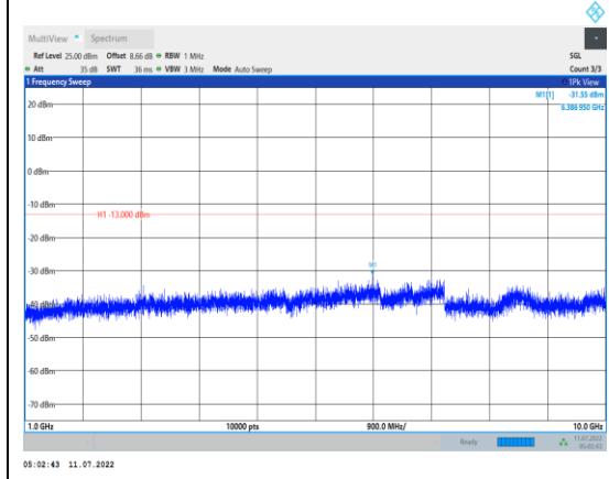
Band5-3MHz-16QAM-20415-1RB#0- Range2:1000~10000MHz
