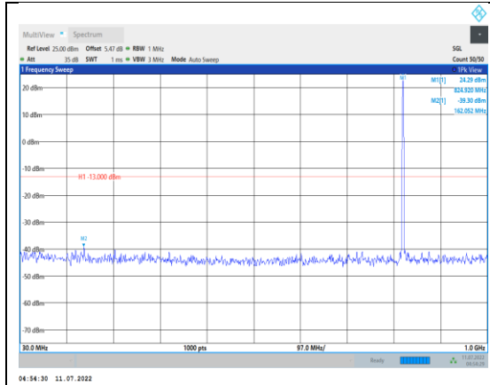
Band5-1.4MHz-QPSK-20407-1RB#0- Range1:30~1000MHz
