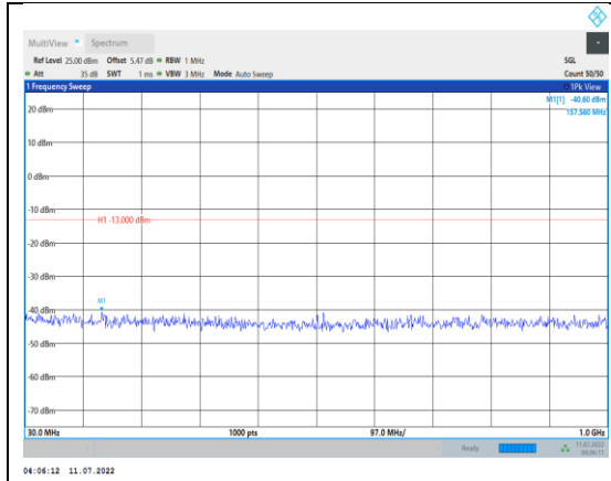
Band4-3MHz-16QAM-19965-1RB#0- Range1:30~1000MHz
