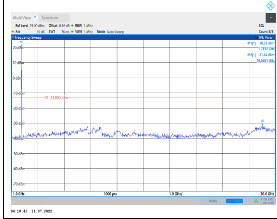
Band4-10MHz-16QAM-20000-1RB#0- Range2:1000~20000MHz
