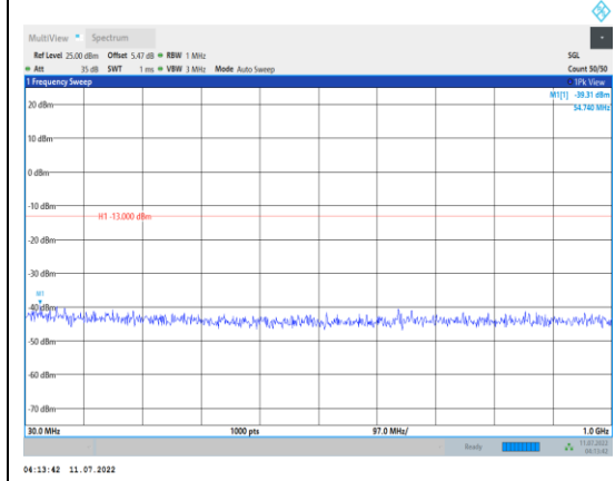
Band4-5MHz-16QAM-20175-1RB#0- Range1:30~1000MHz
