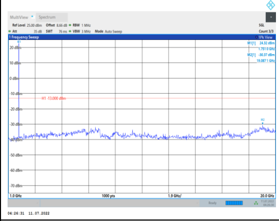
Band4-15MHz-16QAM-20325-1RB#0- Range2:1000~20000MHz
