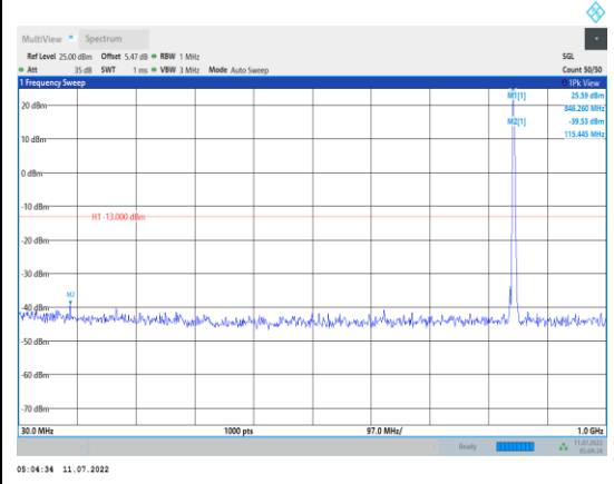
Band5-3MHz-16QAM-20635-1RB#0- Range1:30~1000MHz
