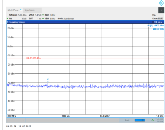
Band2-20MHz-16QAM-18900-1RB#0- Range1:30~1000MHz
