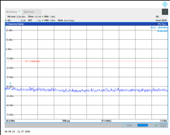
Band4-3MHz-16QAM-20385-1RB#0- Range1:30~1000MHz
