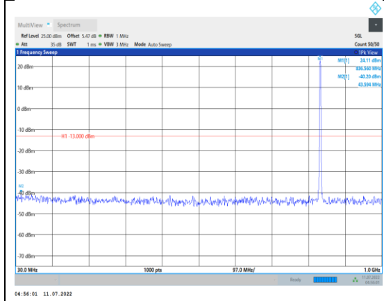
Band5-1.4MHz-16QAM-20525-1RB#0- Range1:30~1000MHz
