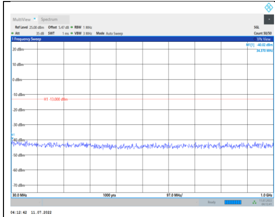
Band4-5MHz-16QAM-19975-1RB#0- Range1:30~1000MHz
