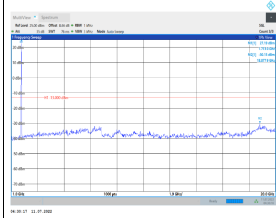
Band4-20MHz-16QAM-20050-1RB#0- Range2:1000~20000MHz
