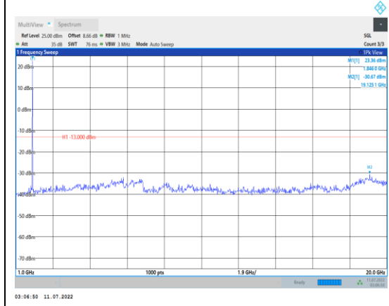
Band2-10MHz-QPSK-18650-1RB#0- Range2:1000~20000MHz
