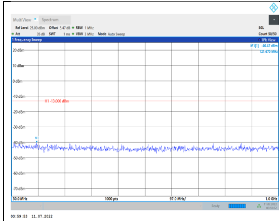
Band4-1.4MHz-QPSK-19957-1RB#0- Range1:30~1000MHz
