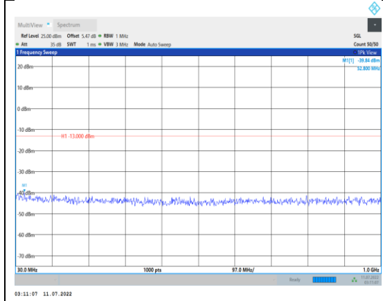
Band2-15MHz-QPSK-18900-1RB#0- Range1:30~1000MHz
