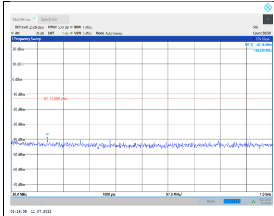
Band2-20MHz-16QAM-18700-1RB#0- Range1:30~1000MHz
