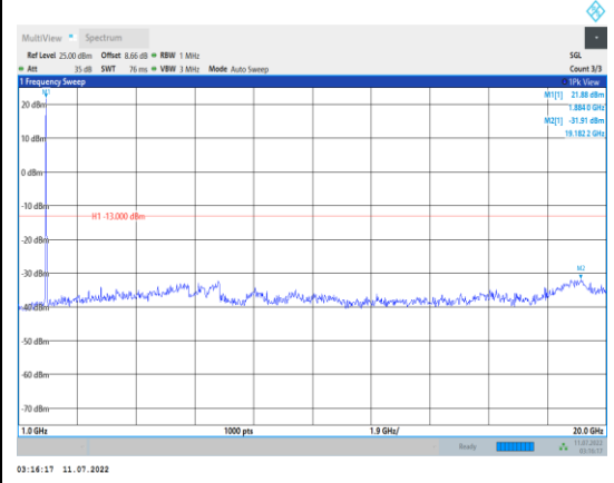
Band2-20MHz-16QAM-19100-1RB#0- Range2:1000~20000MHz
