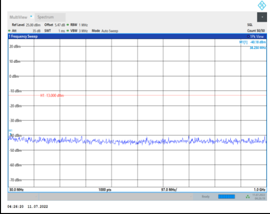
Band4-15MHz-16QAM-20325-1RB#0- Range1:30~1000MHz
