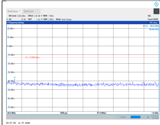
Band2-10MHz-16QAM-18650-1RB#0- Range1:30~1000MHz
