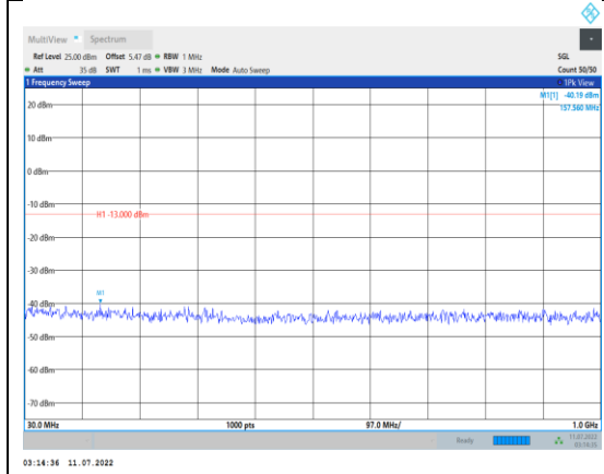
Band2-20MHz-QPSK-18900-1RB#0- Range1:30~1000MHz
