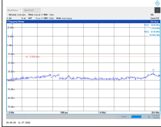
Band4-15MHz-16QAM-20025-1RB#0- Range2:1000~20000MHz
