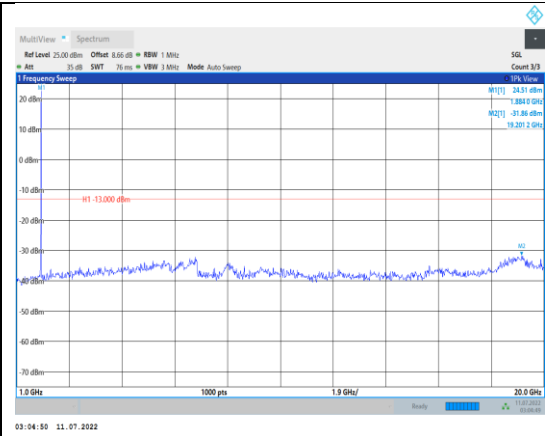
Band2-5MHz-16QAM-18900-1RB#0- Range2:1000~20000MHz
