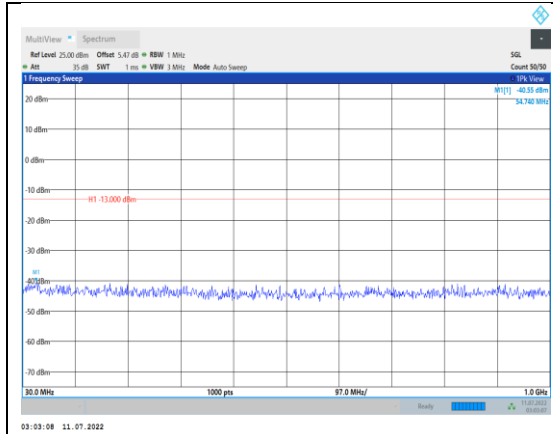
Band2-5MHz-QPSK-18625-1RB#0- Range1:30~1000MHz
