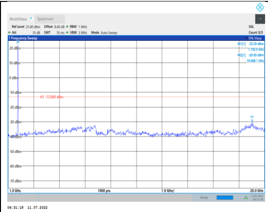
Band4-20MHz-16QAM-20175-1RB#0- Range2:1000~20000MHz
