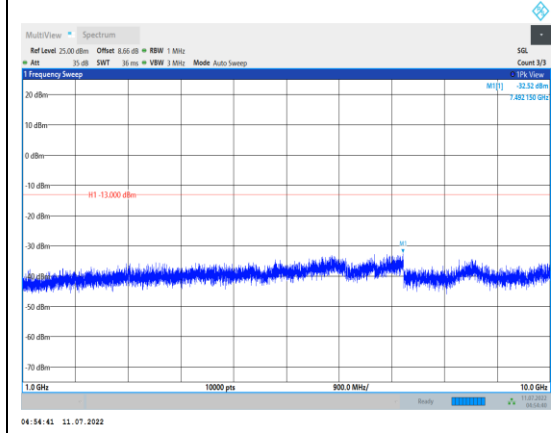
Band5-1.4MHz-QPSK-20407-1RB#0- Range2:1000~10000MHz
