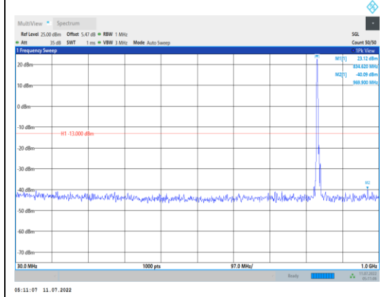
Band5-5MHz-QPSK-20525-1RB#0- Range1:30~1000MHz
