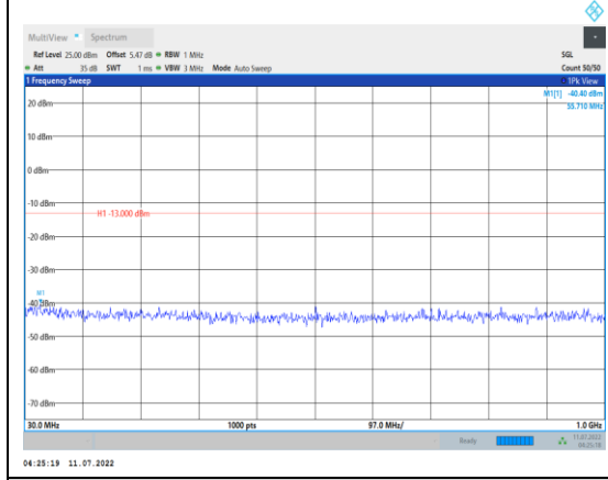
Band4-15MHz-16QAM-20175-1RB#0- Range1:30~1000MHz
