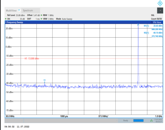
Band5-1.4MHz-QPSK-20643-1RB#0- Range1:30~1000MHz
