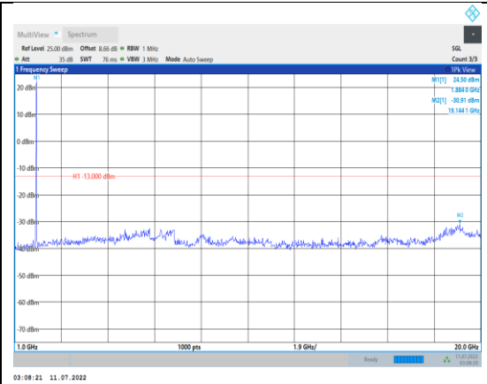
Band2-10MHz-16QAM-18900-1RB#0- Range2:1000~20000MHz
