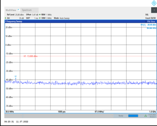
Band4-10MHz-16QAM-20350-1RB#0- Range1:30~1000MHz
