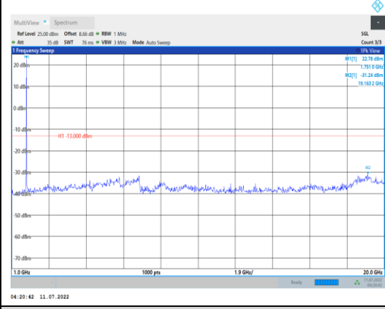
Band4-10MHz-16QAM-20350-1RB#0- Range2:1000~20000MHz
