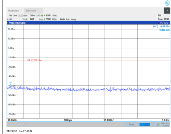
Band4-3MHz-QPSK-20175-1RB#0- Range1:30~1000MHz
