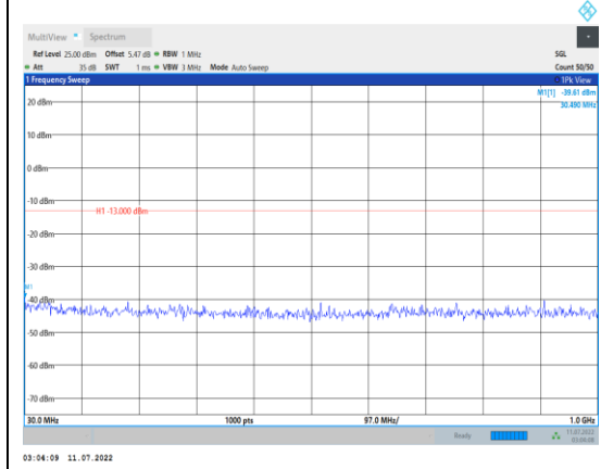
Band2-5MHz-QPSK-18900-1RB#0- Range1:30~1000MHz
