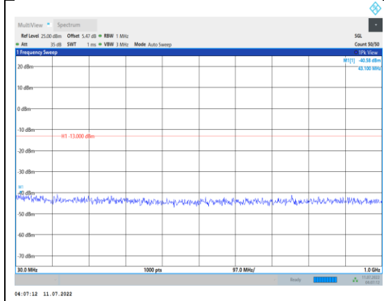
Band4-3MHz-16QAM-20175-1RB#0- Range1:30~1000MHz
