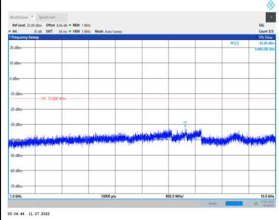
Band5-3MHz-16QAM-20635-1RB#0- Range2:1000~10000MHz
