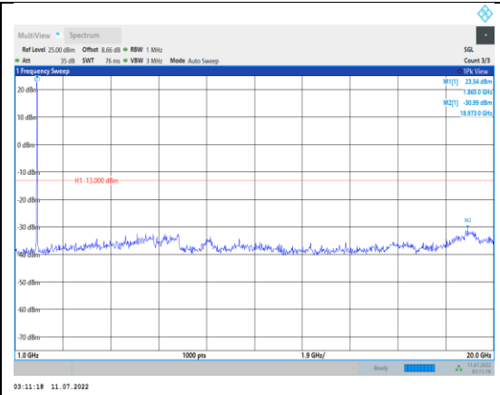
Band2-15MHz-QPSK-18900-1RB#0- Range2:1000~20000MHz
