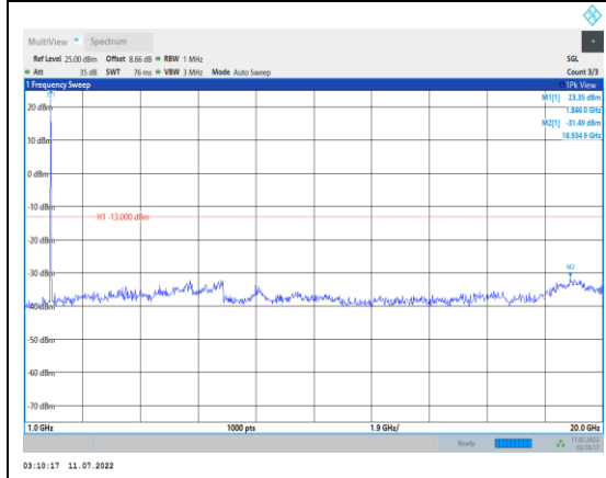
Band2-15MHz-QPSK-18675-1RB#0- Range2:1000~20000MHz
