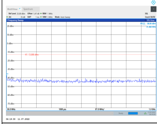
Band4-10MHz-16QAM-20175-1RB#0- Range1:30~1000MHz
