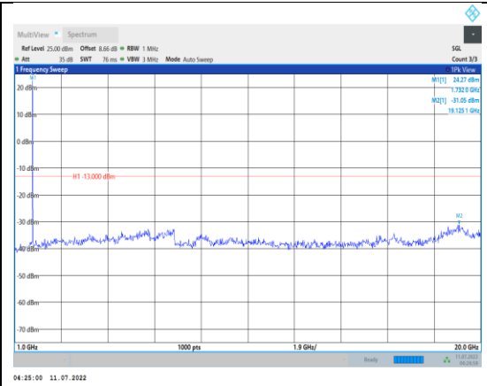
Band4-15MHz-QPSK-20175-1RB#0- Range2:1000~20000MHz
