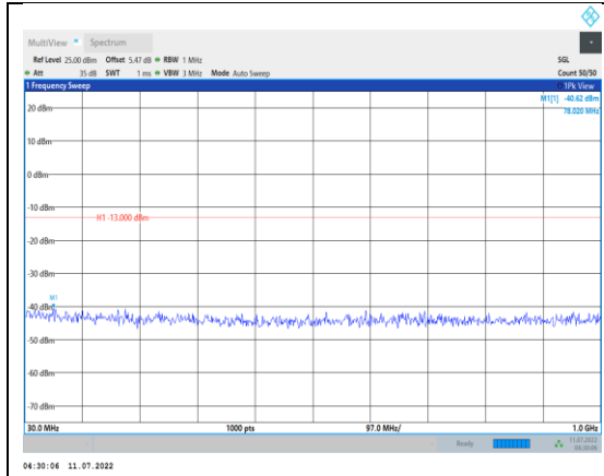
Band4-20MHz-16QAM-20050-1RB#0- Range1:30~1000MHz
