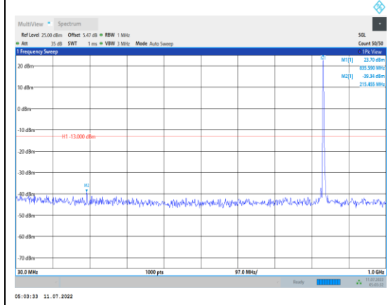
Band5-3MHz-16QAM-20525-1RB#0- Range1:30~1000MHz
