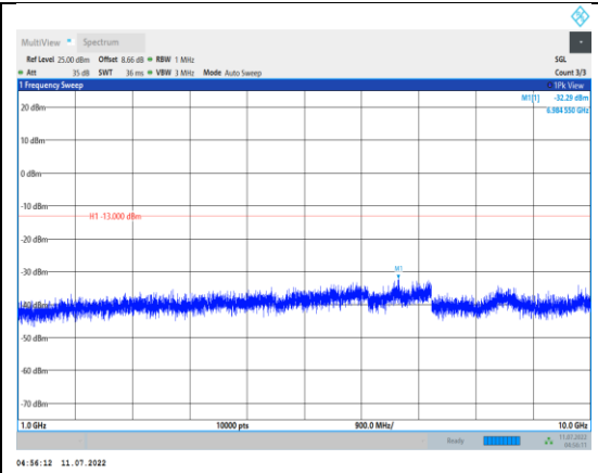
Band5-1.4MHz-16QAM-20525-1RB#0- Range2:1000~10000MHz
