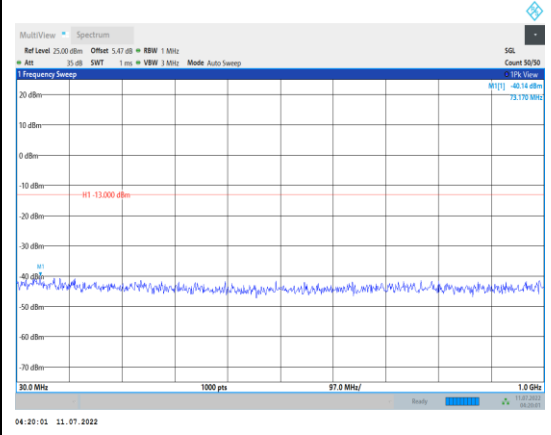
Band4-10MHz-QPSK-20350-1RB#0- Range1:30~1000MHz
