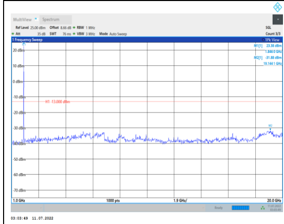
Band2-5MHz-16QAM-18625-1RB#0- Range2:1000~20000MHz
