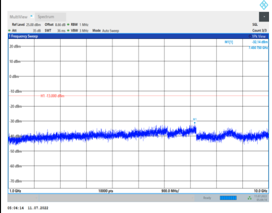
Band5-3MHz-QPSK-20635-1RB#0- Range2:1000~10000MHz
