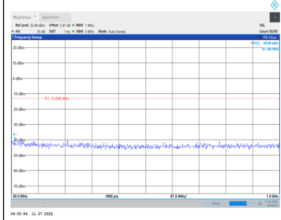
Band4-1.4MHz-QPSK-20175-1RB#0- Range1:30~1000MHz
