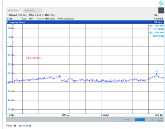
Band4-1.4MHz-16QAM-19957-1RB#0- Range2:1000~20000MHz
