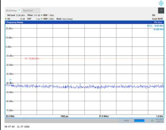
Band4-3MHz-QPSK-20385-1RB#0- Range1:30~1000MHz
