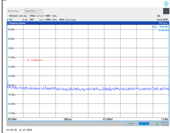
Band2-5MHz-16QAM-18900-1RB#0- Range1:30~1000MHz
