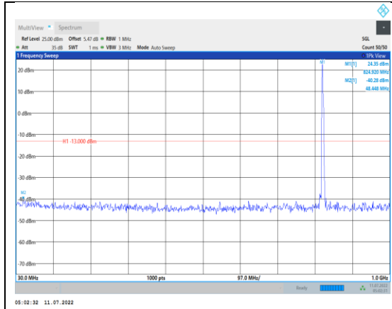
Band5-3MHz-16QAM-20415-1RB#0- Range1:30~1000MHz
