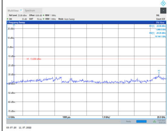
Band2-10MHz-16QAM-18650-1RB#0- Range2:1000~20000MHz
