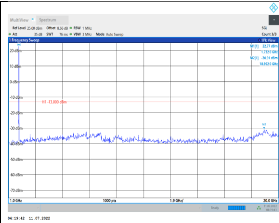
Band4-10MHz-16QAM-20175-1RB#0- Range2:1000~20000MHz
