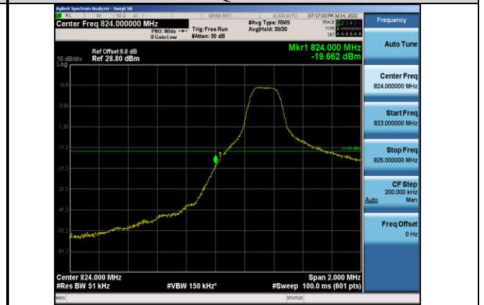
Band5-5MHz-QPSK-20425-1RB#0
