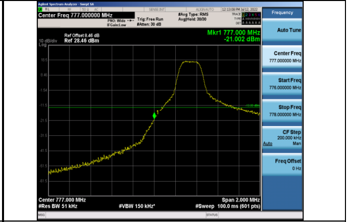
Band13-5MHz-QPSK-23205-1RB#0
