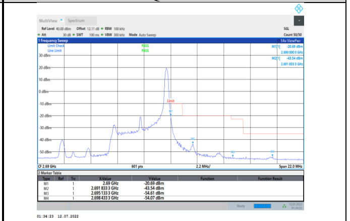
Band41-5MHz-QPSK-41565-1RB#24
