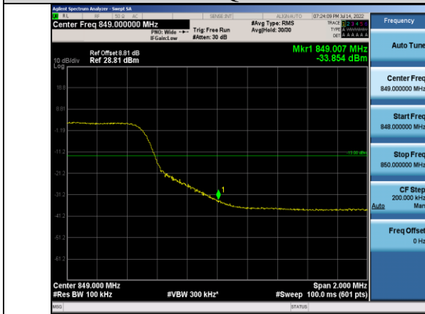
Band5-10MHz-16QAM-20600-50RB#0
