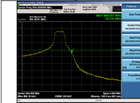
Band5-3MHz-16QAM-20635-1RB#14
