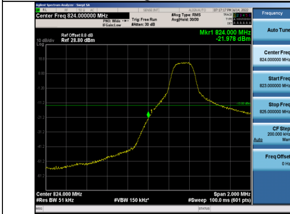
Band5-5MHz-16QAM-20425-1RB#0
