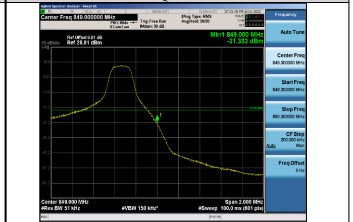
Band5-5MHz-16QAM-20625-1RB#24
