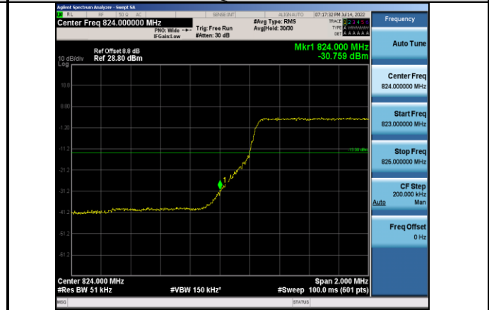
Band5-5MHz-QPSK-20425-25RB#0
