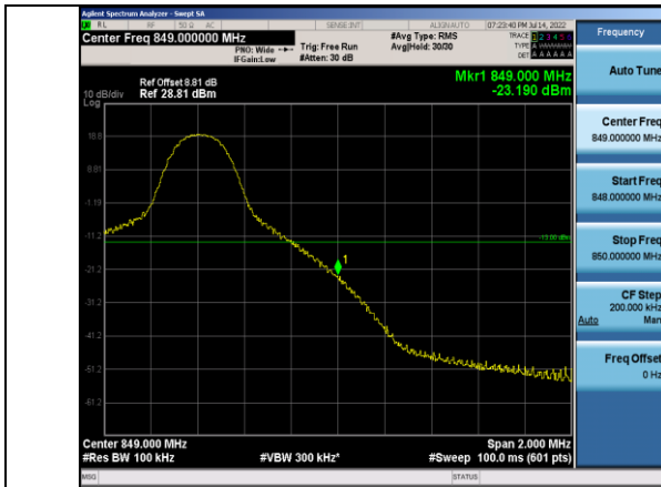
Band5-10MHz-16QAM-20600-1RB#49
