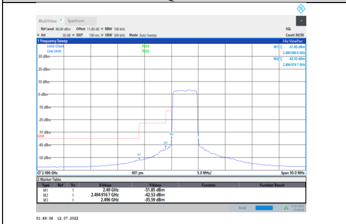
Band41-5MHz-16QAM-39675-25RB#0
