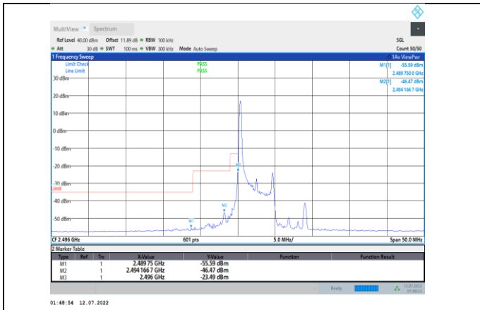
Band41-5MHz-16QAM-39675-1RB#0
