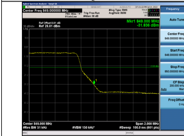
Band5-5MHz-QPSK-20625-25RB#0
