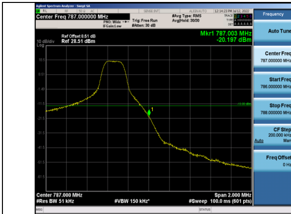
Band13-5MHz-QPSK-23255-1RB#24
