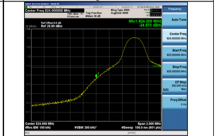
Band5-10MHz-16QAM-20450-1RB#0
