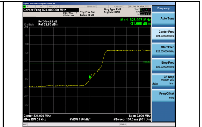
Band5-5MHz-16QAM-20425-25RB#0
