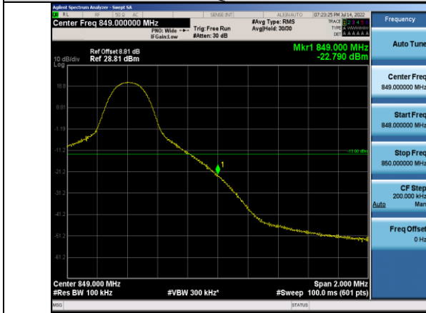
Band5-10MHz-QPSK-20600-1RB#49
