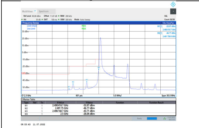
Band7-10MHz-16QAM-20800-1RB#0
