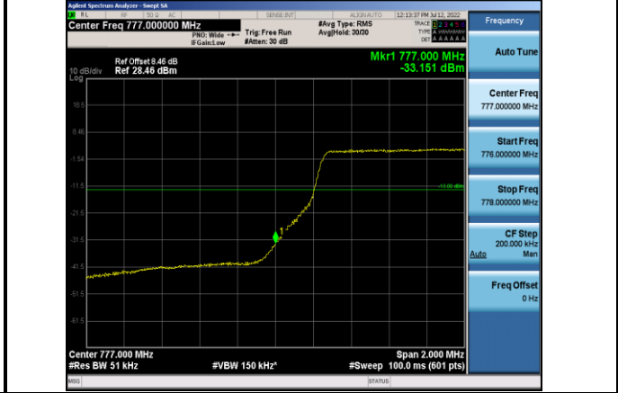
Band13-5MHz-QPSK-23205-25RB#0
