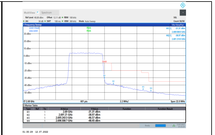
Band41-5MHz-16QAM-41565-25RB#0
