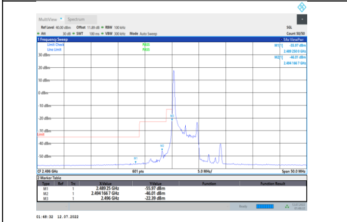
Band41-5MHz-QPSK-39675-1RB#0
