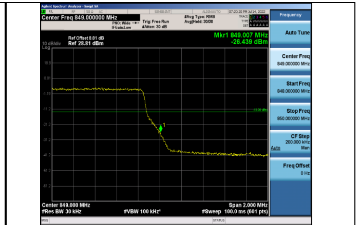
Band5-3MHz-16QAM-20635-15RB#0
