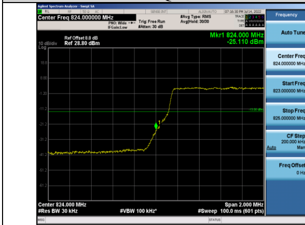
Band5-3MHz-16QAM-20415-15RB#0
