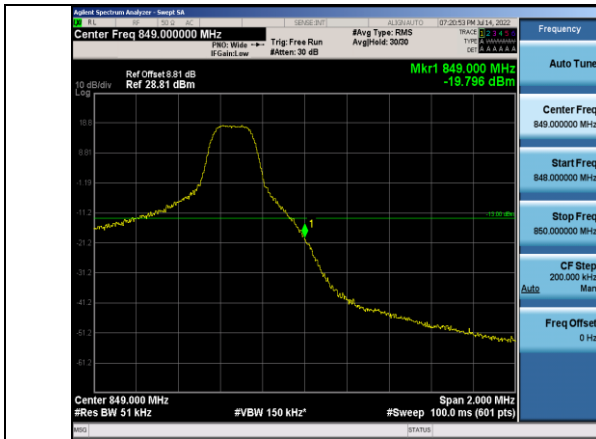
Band5-5MHz-QPSK-20625-1RB#24
