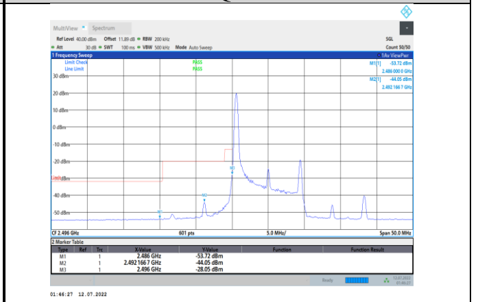
Band41-10MHz-QPSK-39700-1RB#0
