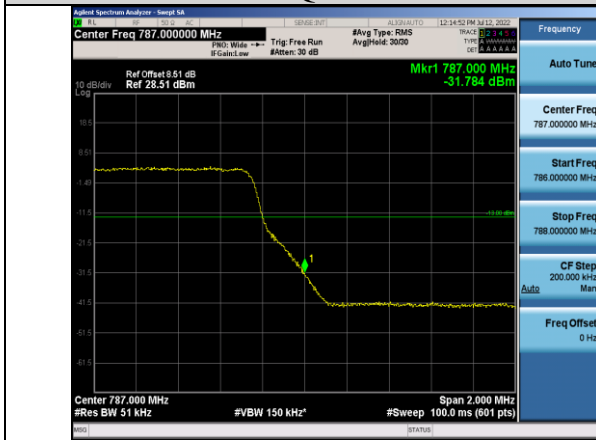
Band13-5MHz-QPSK-23255-25RB#0
