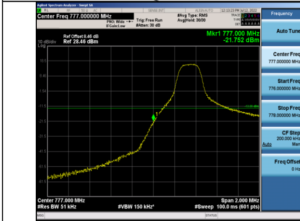
Band13-5MHz-16QAM-23205-1RB#0
