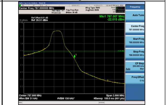
Band13-5MHz-16QAM-23255-1RB#24
