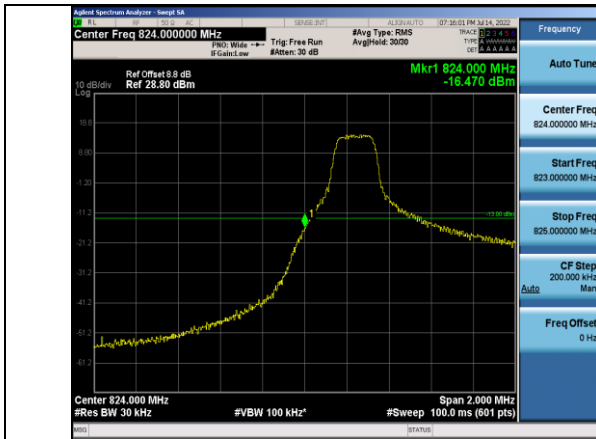
Band5-3MHz-16QAM-20415-1RB#0
