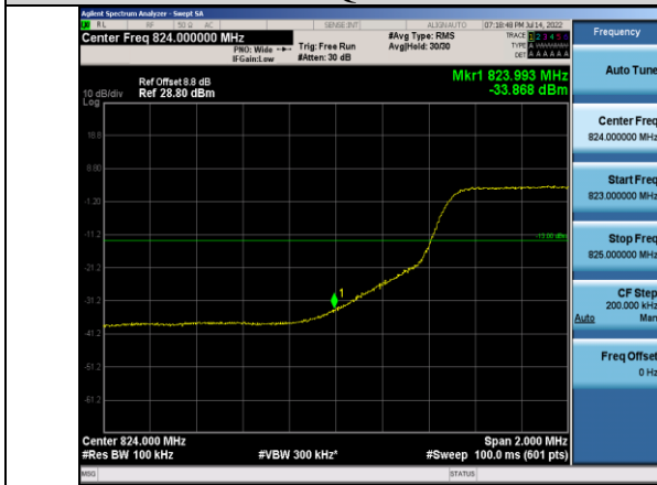
Band5-10MHz-QPSK-20450-50RB#0
