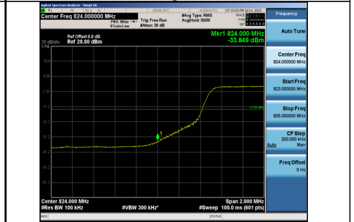
Band5-10MHz-16QAM-20450-50RB#0
