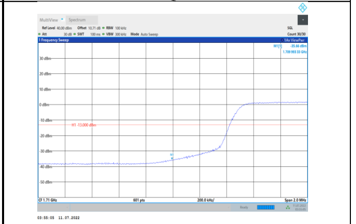
Band4-10MHz-16QAM-20000-50RB#0
