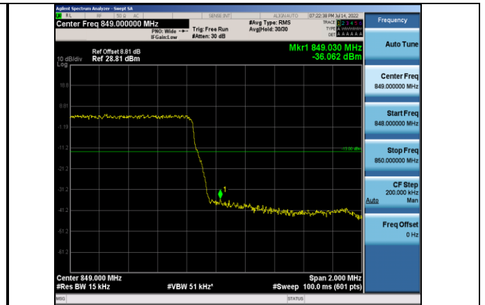
Band5-1.4MHz-QPSK-20643-6RB#0
