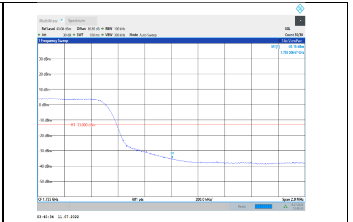
Band4-10MHz-QPSK-20350-50RB#0
