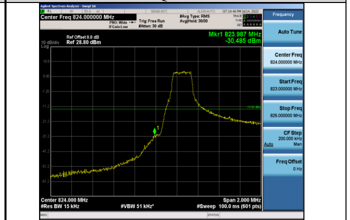
Band5-1.4MHz-16QAM-20407-1RB#0
