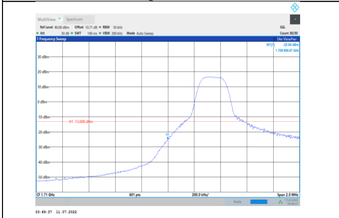
Band4-5MHz-16QAM-19975-1RB#0
