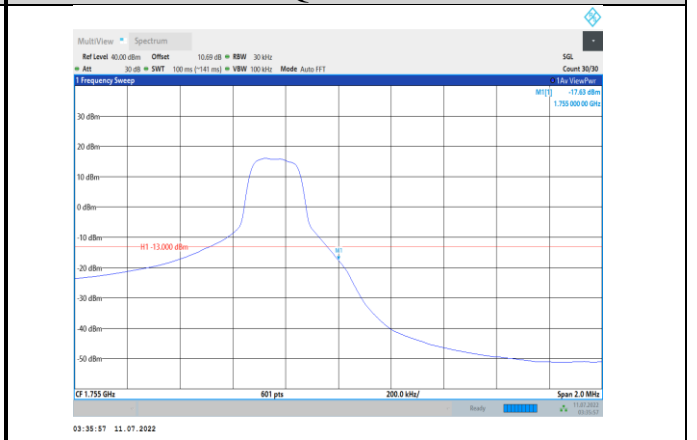
Band4-3MHz-QPSK-20385-1RB#14
