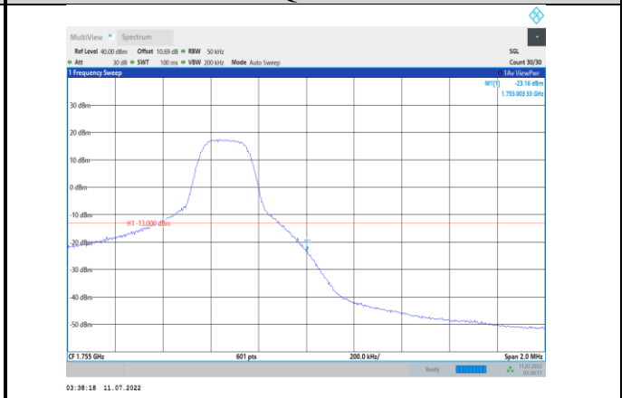
Band4-5MHz-16QAM-20375-1RB#24
