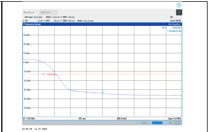
Band4-15MHz-16QAM-20325-75RB#0
