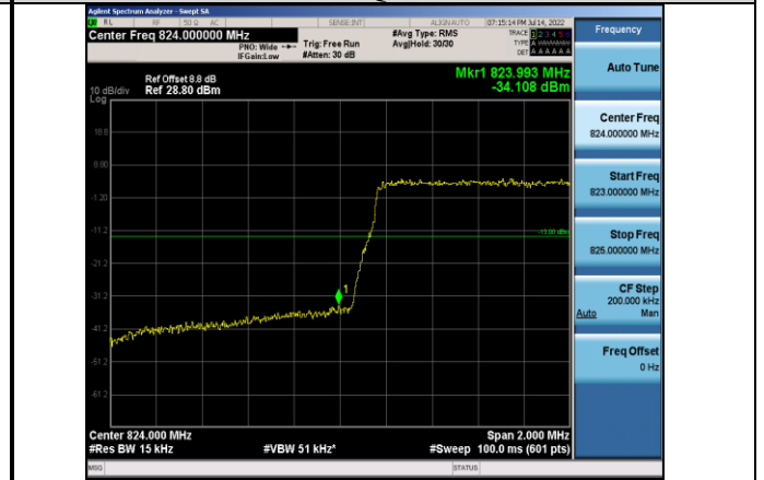
Band5-1.4MHz-16QAM-20407-6RB#0
