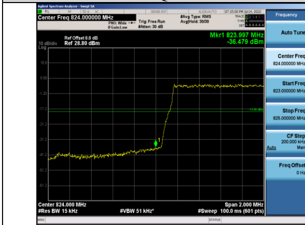
Band5-1.4MHz-QPSK-20407-6RB#0
