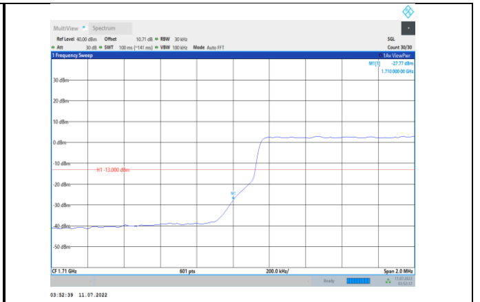
Band4-3MHz-QPSK-19965-15RB#0
