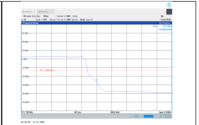
Band4-3MHz-16QAM-20385-15RB#0
