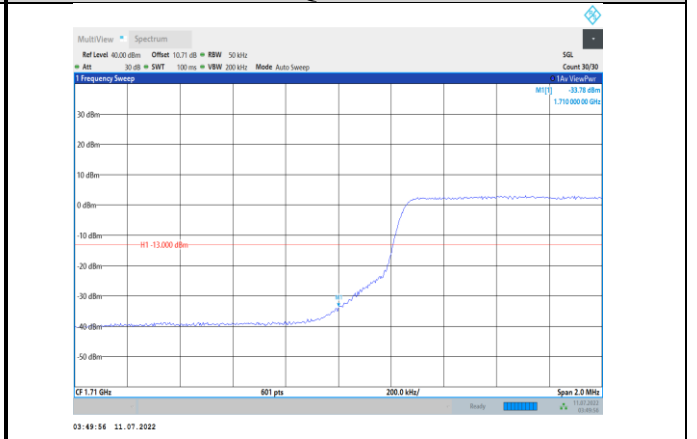
Band4-5MHz-QPSK-19975-25RB#0
