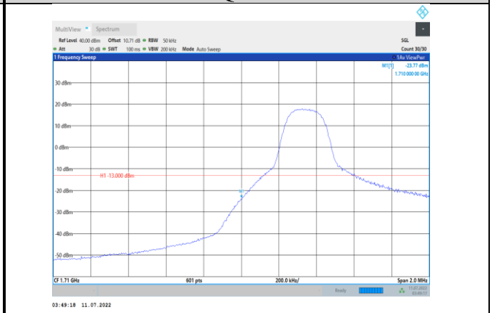
Band4-5MHz-QPSK-19975-1RB#0
