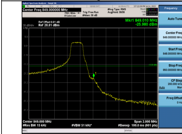
Band5-1.4MHz-QPSK-20643-1RB#5
