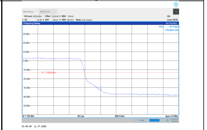
Band4-5MHz-16QAM-20375-25RB#0
