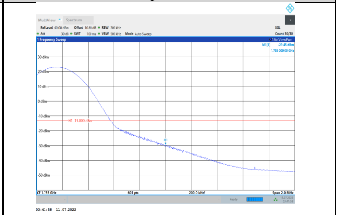
Band4-15MHz-QPSK-20325-1RB#74
