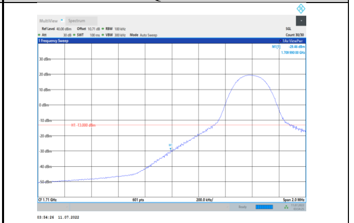
Band4-10MHz-16QAM-20000-1RB#0
