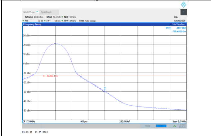
Band4-10MHz-QPSK-20350-1RB#49
