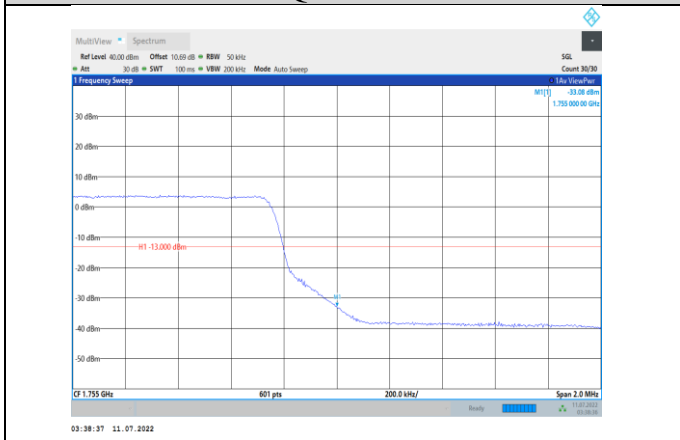
Band4-5MHz-QPSK-20375-25RB#0
