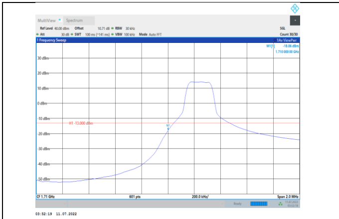
Band4-3MHz-16QAM-19965-1RB#0
