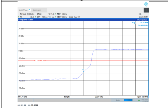
Band4-3MHz-16QAM-19965-15RB#0
