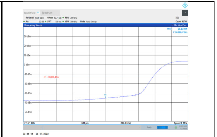
Band4-15MHz-QPSK-20025-75RB#0
