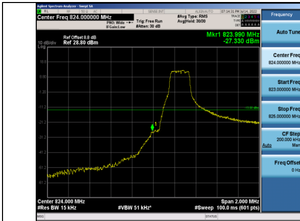
Band5-1.4MHz-QPSK-20407-1RB#0
