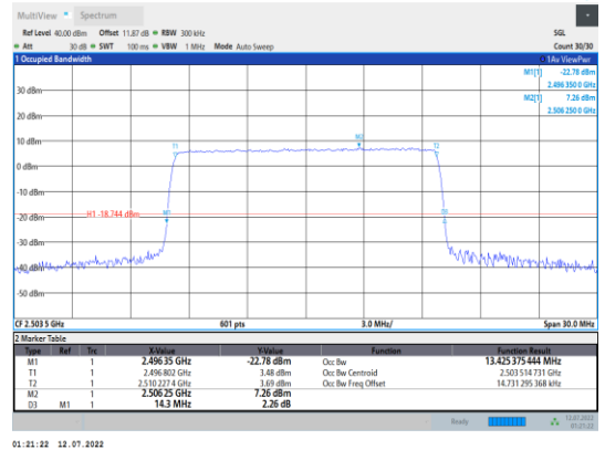
Band41-15MHz-16QAM-39725-75RB#0
