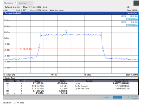
Band66-5MHz-16QAM-131997-25RB#0
