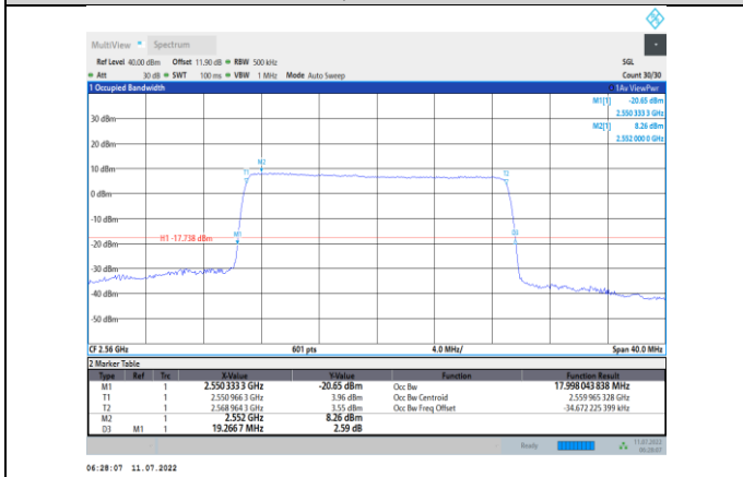
Band7-20MHz-QPSK-21350-100RB#0
