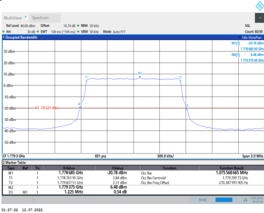
Band66-1.4MHz-QPSK-132665-6RB#0
