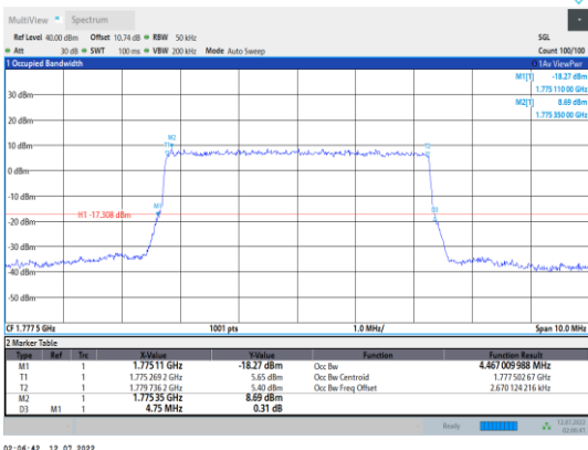
Band66-5MHz-QPSK-132647-25RB#0
