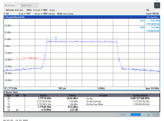
Band66-5MHz-16QAM-132647-25RB#0
