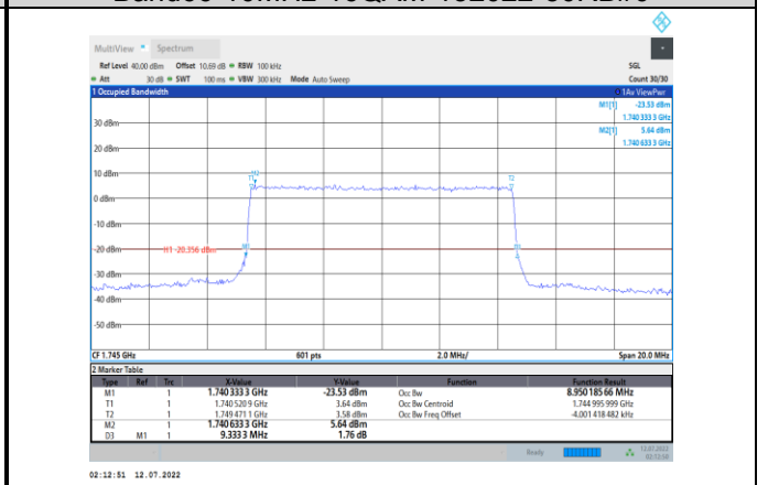
Band66-10MHz-16QAM-132322-50RB#0
