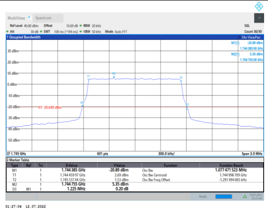
Band66-1.4MHz-16QAM-132322-6RB#0
