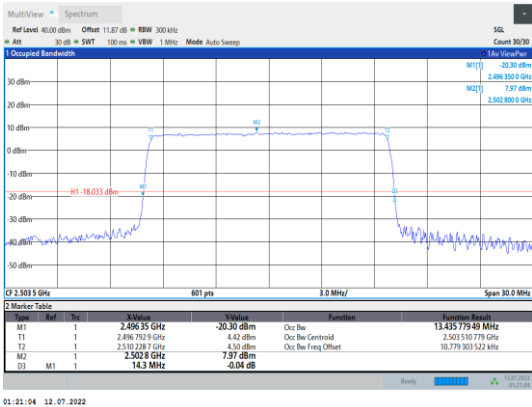
Band41-15MHz-QPSK-39725-75RB#0
