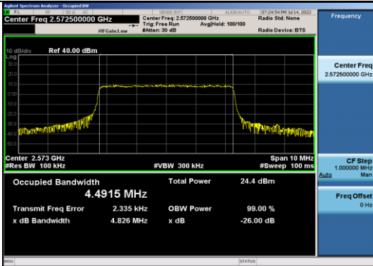
Band38-5MHz-QPSK-37775-25RB#0
