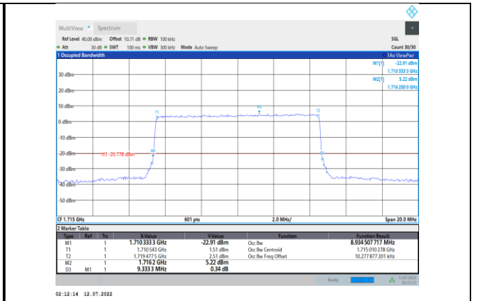
Band66-10MHz-16QAM-132022-50RB#0
