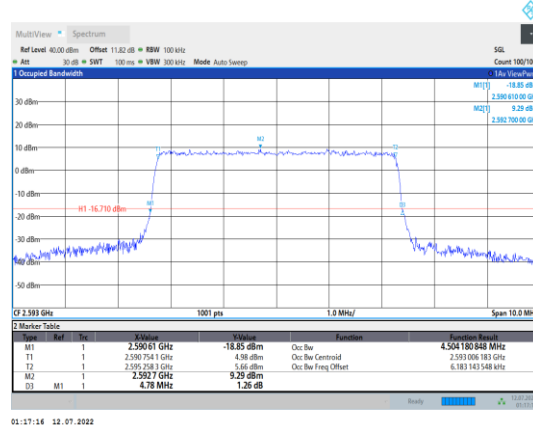
Band41-5MHz-16QAM-40620-25RB#0
