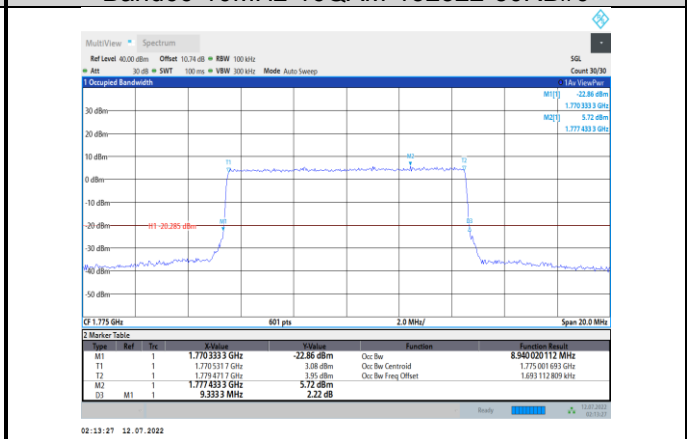
Band66-10MHz-16QAM-132622-50RB#0
