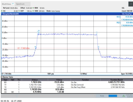
Band66-5MHz-QPSK-132322-25RB#0
