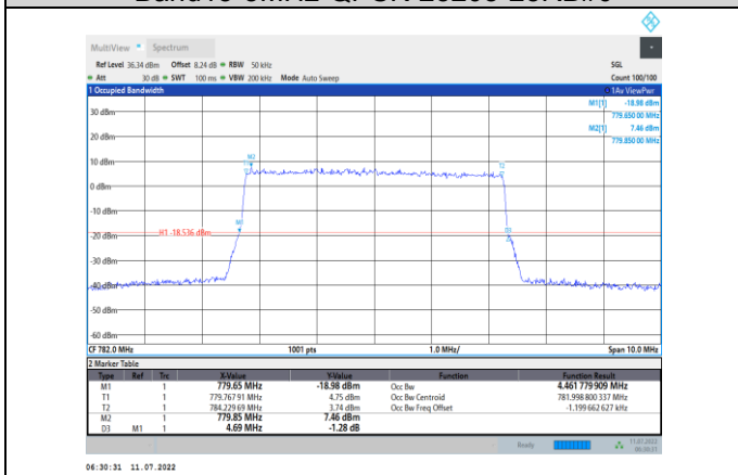
Band13-5MHz-QPSK-23230-25RB#0
