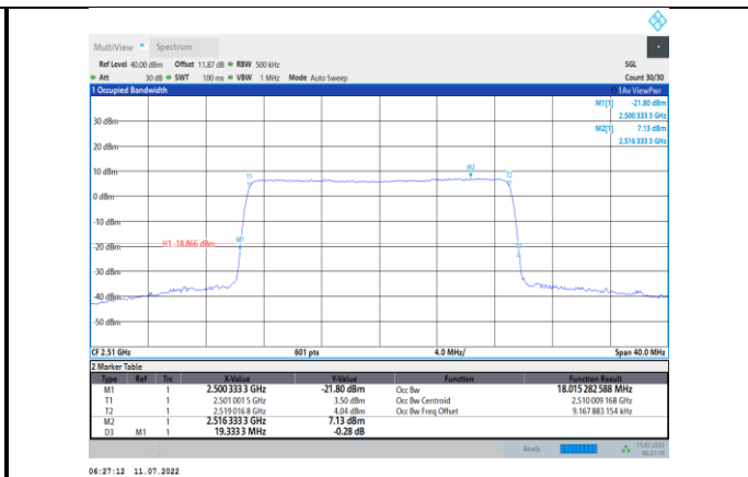
Band7-20MHz-16QAM-20850-100RB#0
