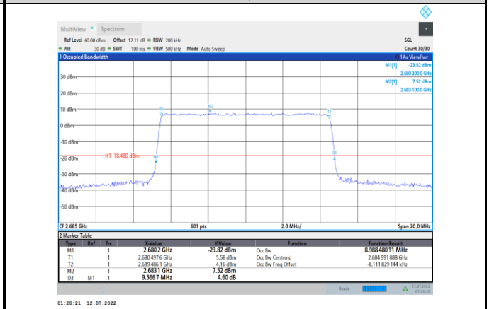
Band41-10MHz-16QAM-41540-50RB#0
