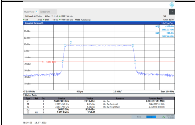
Band41-10MHz-QPSK-41540-50RB#0
