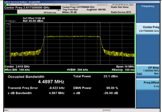
Band38-5MHz-16QAM-38225-25RB#0
