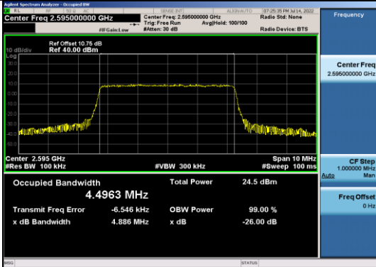
Band38-5MHz-QPSK-38000-25RB#0
