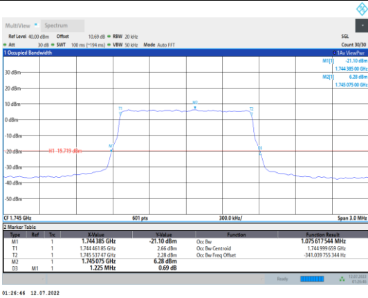
Band66-1.4MHz-QPSK-132322-6RB#0
