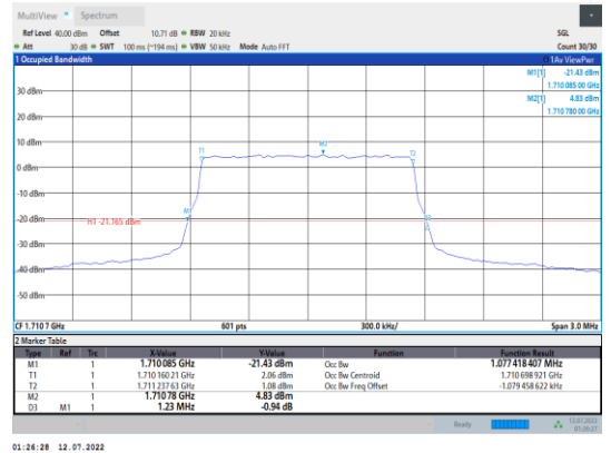
Band66-1.4MHz-16QAM-131979-6RB#0
