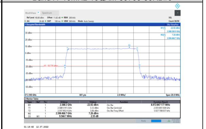
Band41-10MHz-16QAM-40620-50RB#0
