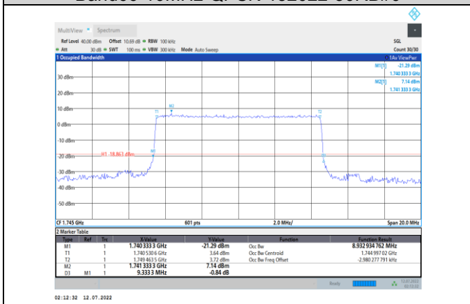
Band66-10MHz-QPSK-132322-50RB#0
