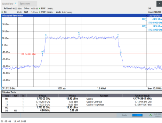
Band66-5MHz-QPSK-131997-25RB#0
