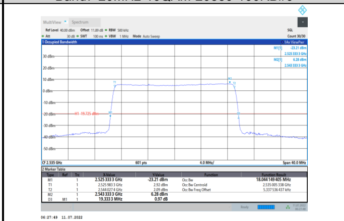
Band7-20MHz-16QAM-21100-100RB#0
