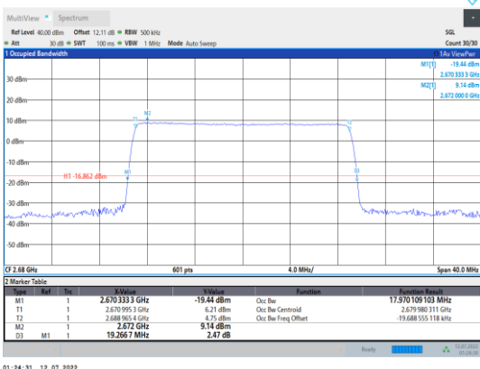
Band41-20MHz-QPSK-41490-100RB#0
