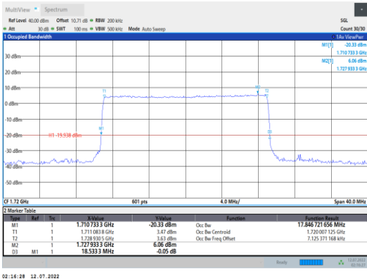
Band66-20MHz-QPSK-132072-100RB#0
