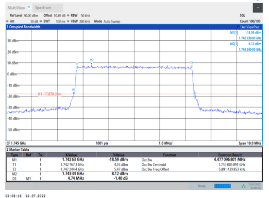
Band66-5MHz-16QAM-132322-25RB#0
