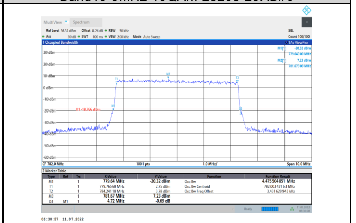
Band13-5MHz-16QAM-23230-25RB#0
