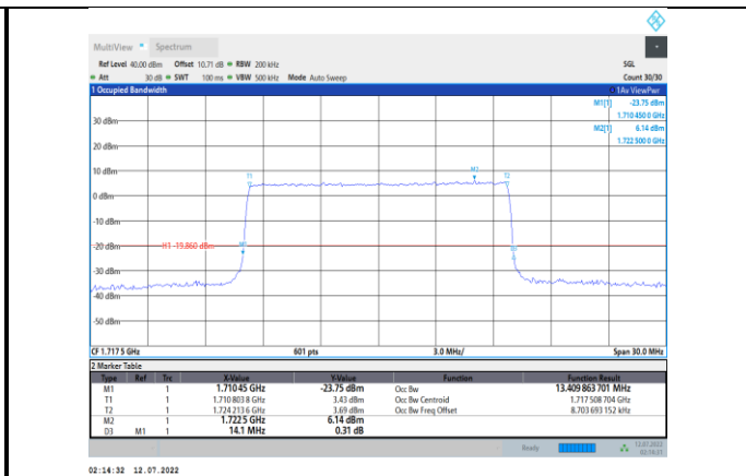
Band66-15MHz-16QAM-132047-75RB#0
