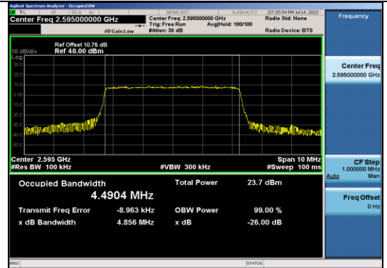
Band38-5MHz-16QAM-38000-25RB#0
