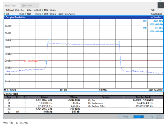
Band66-20MHz-16QAM-132322-100RB#0
