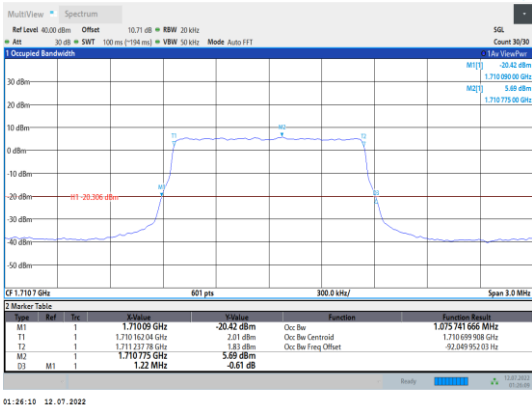
Band66-1.4MHz-QPSK-131979-6RB#0
