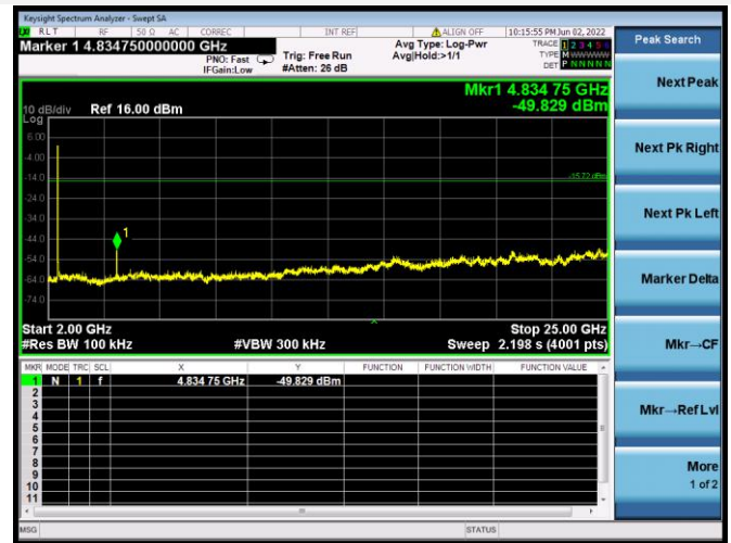
802.11b CHANNEL 2, SPURIOUS 2 GHz ~ 25 GHz
