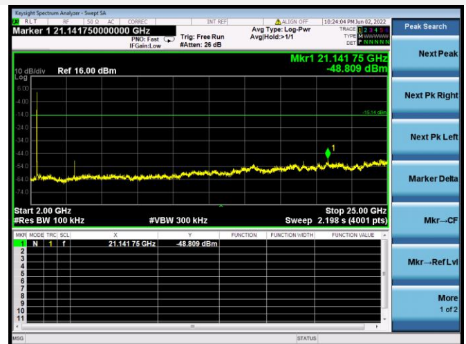
802.11b CHANNEL 3, SPURIOUS 2 GHz ~ 25 GHz
