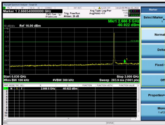
802.11b CHANNEL 3, SPURIOUS 30 MHz ~ 3 GHz
