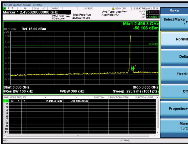
802.11b CHANNEL 5, SPURIOUS 30 MHz ~ 3 GHz
