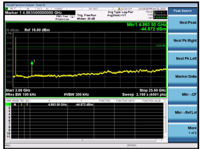
802.11b CHANNEL 5, SPURIOUS 2 GHz ~ 25 GHz
