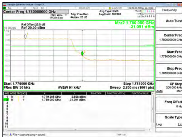
Band66 / 3MHz / High CH / QPSK / FULL RB
