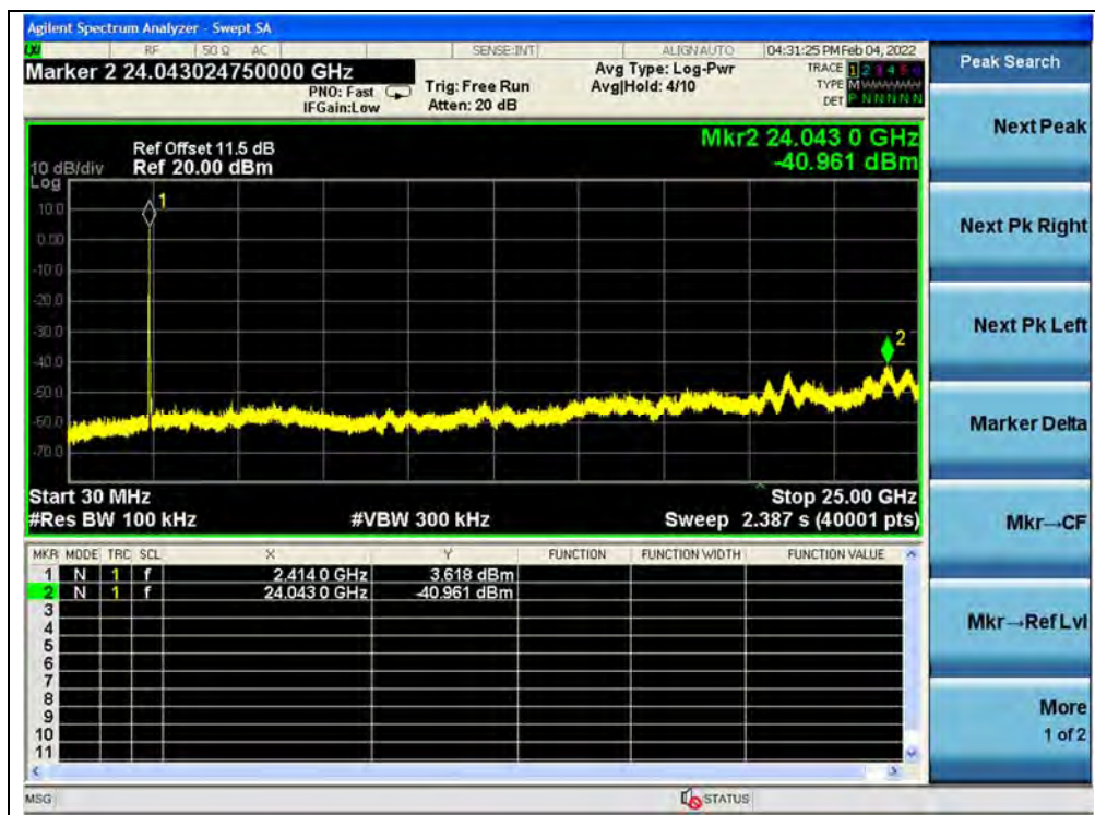
(30MHz to 25GHz, Channel 1, 802.11ac (VHT20))
