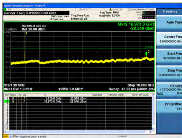
Band66 / 3MHz / Low CH / 64QAM
