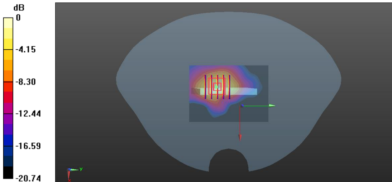
0 dB = 0.321 W/kg
