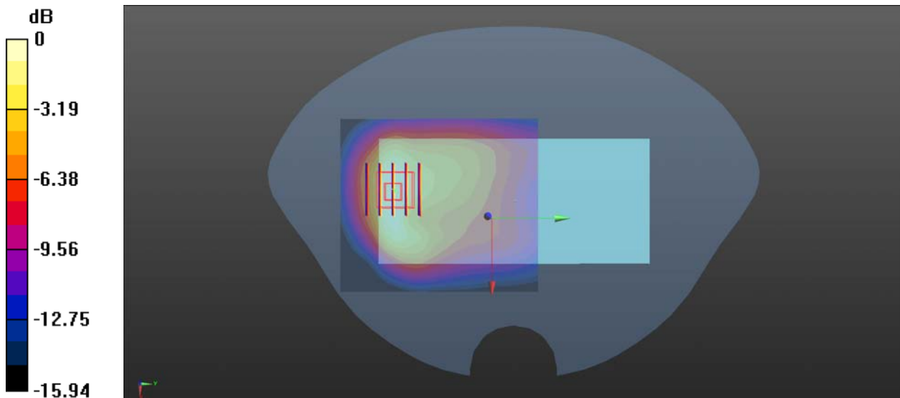
0 dB = 0.463 W/kg
