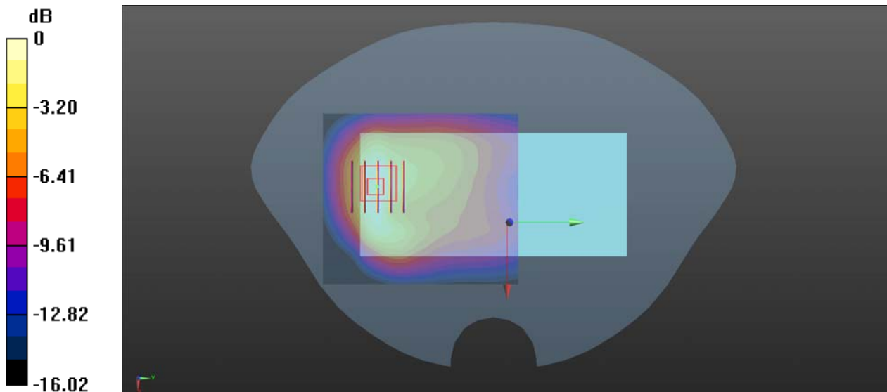
0 dB = 0.650 W/kg
