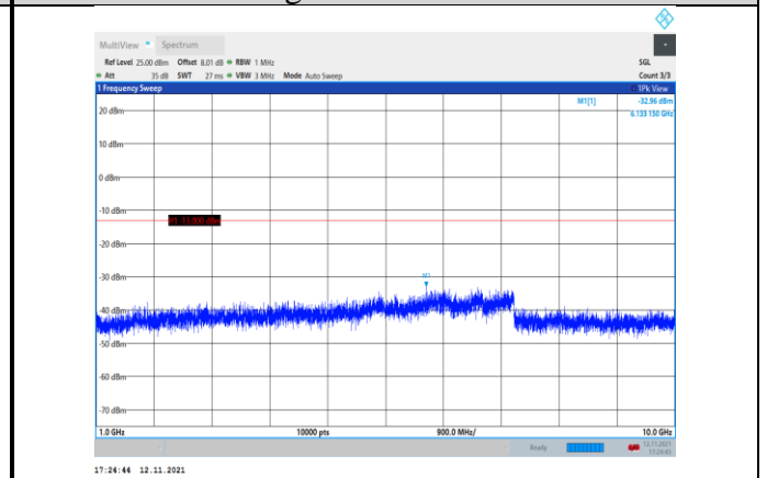
Band26-3MHz-16QAM-26775-1RB#0- Range2:1000~10000MHz
