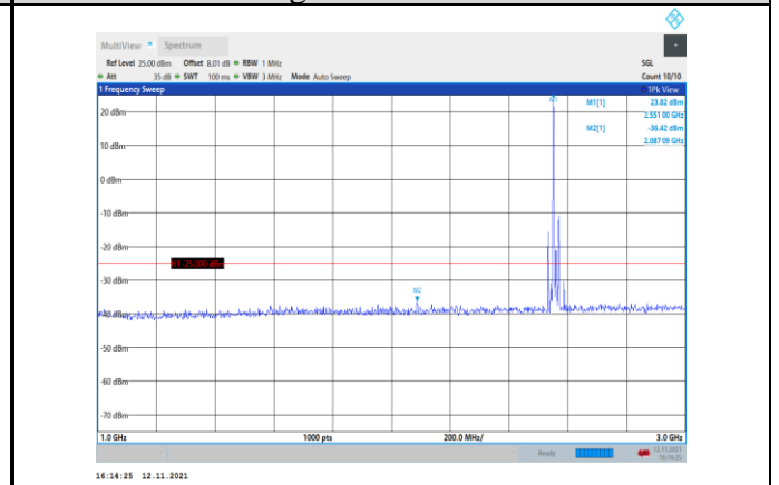
Band7-20MHz-16QAM-21350-1RB#0- Range2:1000~3000MHz
