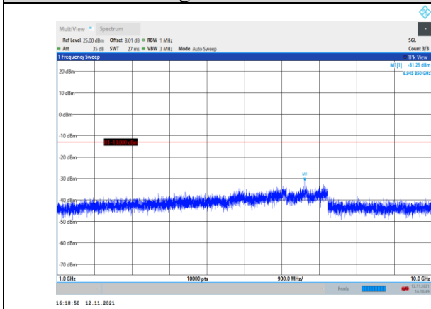
Band12-1.4MHz-16QAM-23017-1RB#0- Range2:1000~10000MHz
