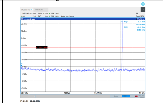
Band26-3MHz-16QAM-26775-1RB#0- Range1:30~1000MHz
