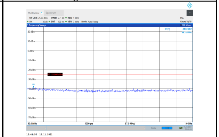
Band38-5MHz-16QAM-38000-1RB#0- Range1:30~1000MHz
