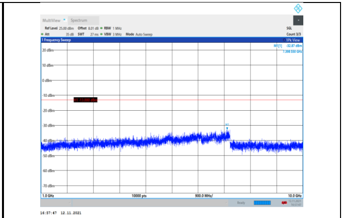
Band17-10MHz-16QAM-23790-1RB#0- Range2:1000~10000MHz
