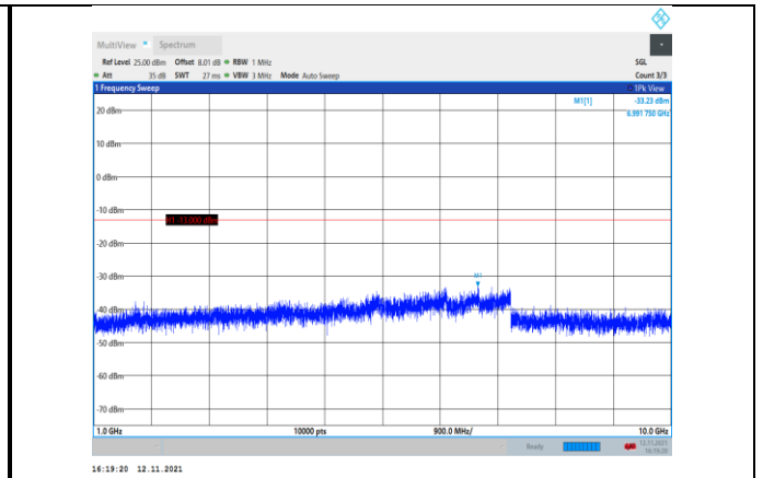
Band12-1.4MHz-QPSK-23095-1RB#0- Range2:1000~10000MHz
