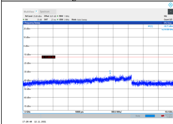
Band26-5MHz-16QAM-26715-1RB#0- Range2:1000~10000MHz
