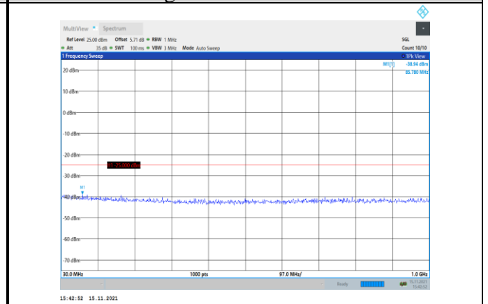
Band38-5MHz-QPSK-37775-1RB#0- Range1:30~1000MHz
