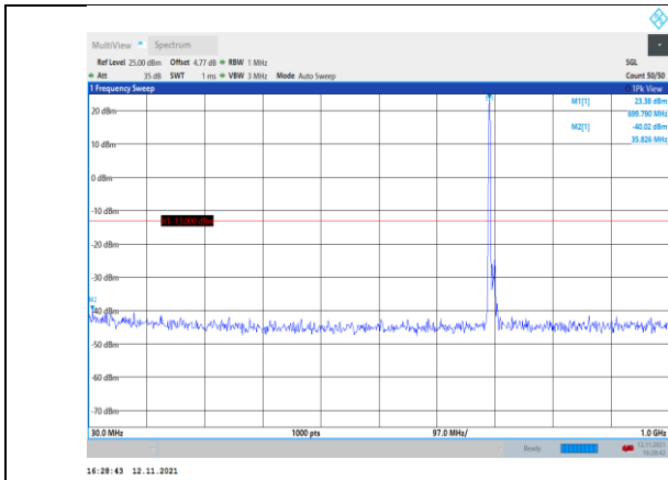
Band12-10MHz-16QAM-23060-1RB#0- Range1:30~1000MHz
