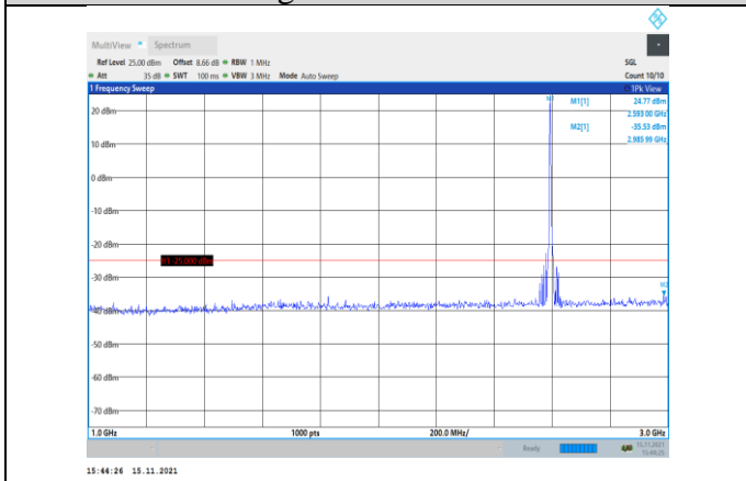
Band38-5MHz-QPSK-38000-1RB#0- Range2:1000~3000MHz
