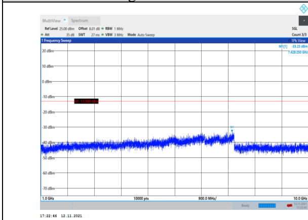
Band26-3MHz-16QAM-26705-1RB#0- Range2:1000~10000MHz
