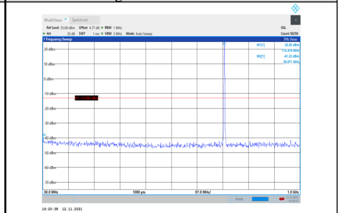
Band12-1.4MHz-16QAM-23173-1RB#0- Range1:30~1000MHz
