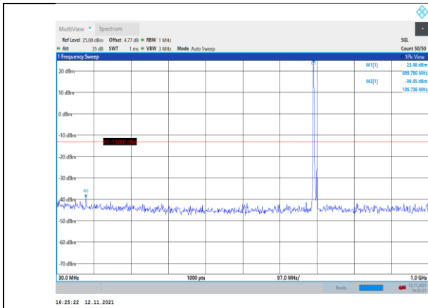
Band12-5MHz-16QAM-23035-1RB#0- Range1:30~1000MHz
