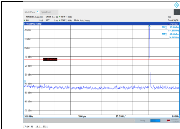
Band26-1.4MHz-16QAM-26697-1RB#0- Range1:30~1000MHz
