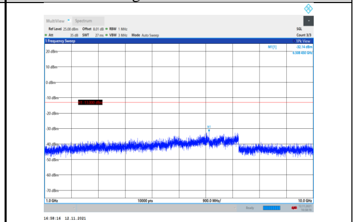
Band17-10MHz-QPSK-23800-1RB#0- Range2:1000~10000MHz
