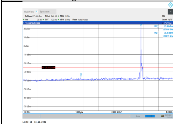
Band38-5MHz-16QAM-37775-1RB#0- Range2:1000~3000MHz
