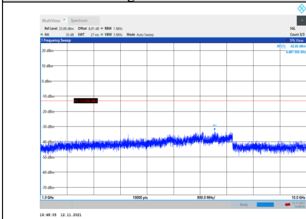
Band17-5MHz-QPSK-23755-1RB#0- Range2:1000~10000MHz
