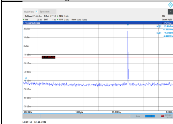
Band12-1.4MHz-QPSK-23095-1RB#0- Range1:30~1000MHz
