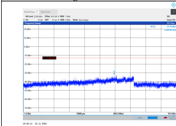
Band12-3MHz-16QAM-23025-1RB#0- Range2:1000~10000MHz
