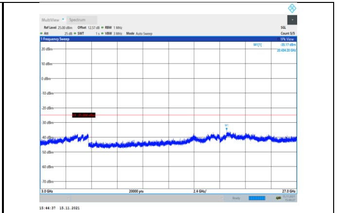
Band38-5MHz-QPSK-38000-1RB#0- Range3:3000~27000MHz
