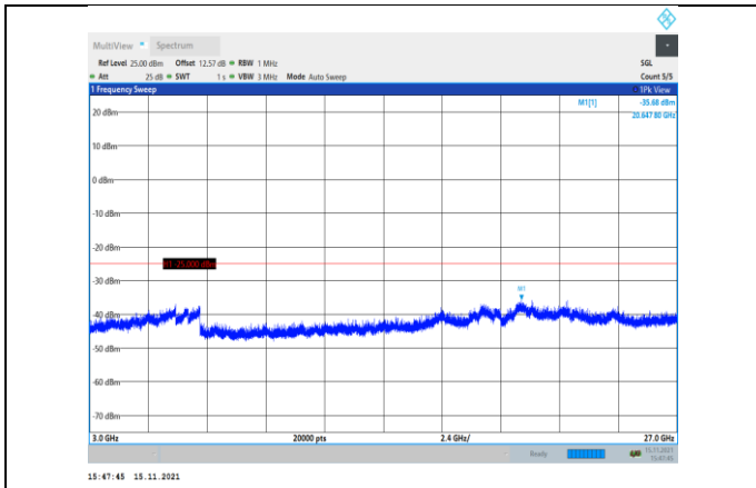
Band38-10MHz-QPSK-37800-1RB#0- Range3:3000~27000MHz
