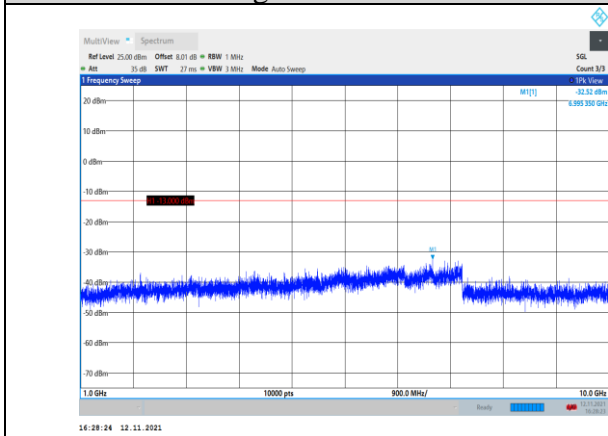
Band12-10MHz-QPSK-23060-1RB#0- Range2:1000~10000MHz
