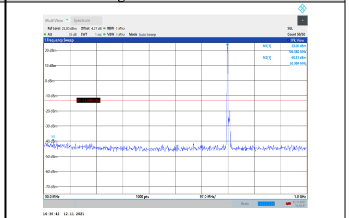
Band12-10MHz-16QAM-23130-1RB#0- Range1:30~1000MHz
