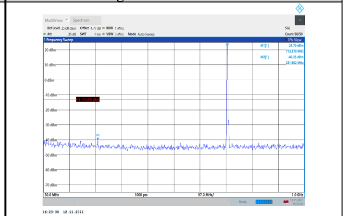
Band12-3MHz-QPSK-23165-1RB#0- Range1:30~1000MHz
