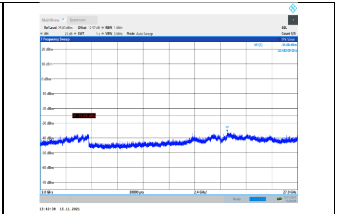
Band38-10MHz-QPSK-38000-1RB#0- Range3:3000~27000MHz
