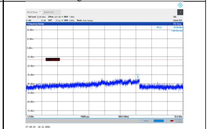
Band26-1.4MHz-QPSK-26783-1RB#0- Range2:1000~10000MHz
