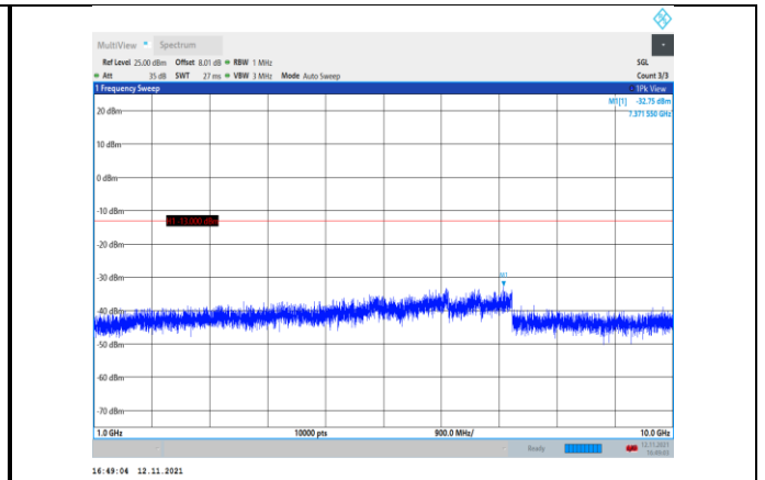
Band17-5MHz-QPSK-23790-1RB#0- Range2:1000~10000MHz
