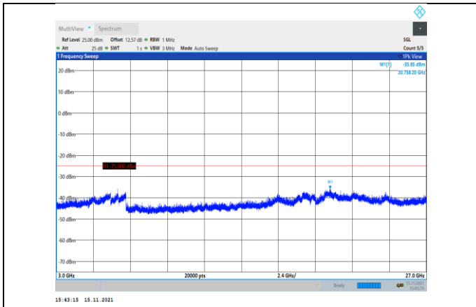
Band38-5MHz-QPSK-37775-1RB#0- Range3:3000~27000MHz
