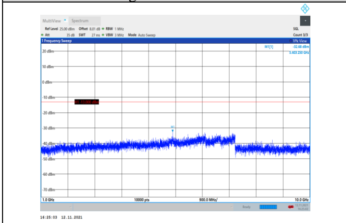
Band12-5MHz-QPSK-23035-1RB#0- Range2:1000~10000MHz
