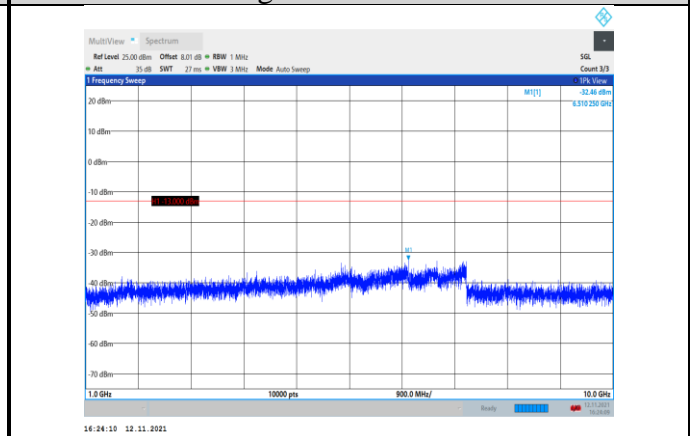
Band12-3MHz-16QAM-23165-1RB#0- Range2:1000~10000MHz
