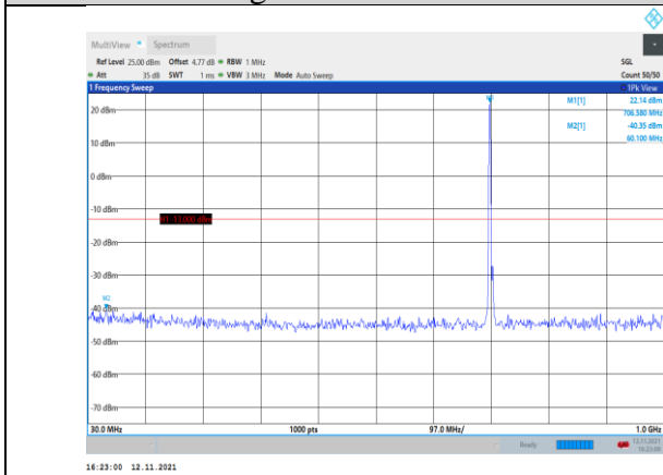
Band12-3MHz-16QAM-23095-1RB#0- Range1:30~1000MHz
