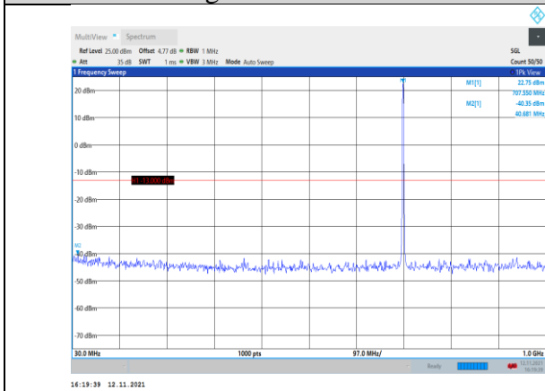
Band12-1.4MHz-16QAM-23095-1RB#0- Range1:30~1000MHz
