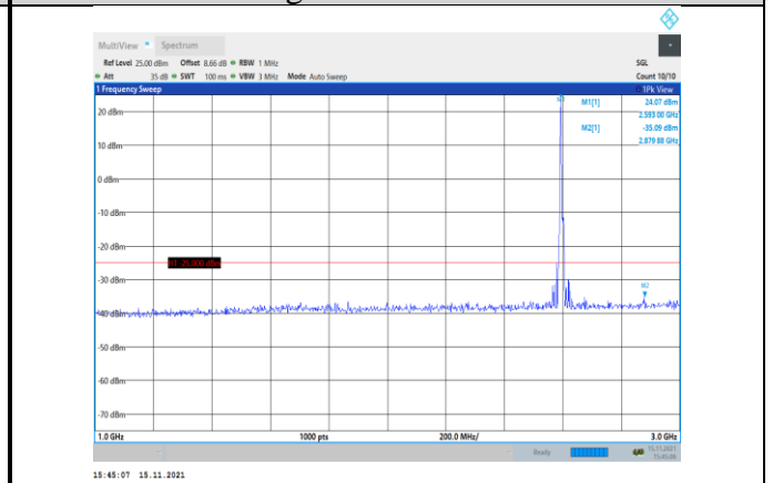
Band38-5MHz-16QAM-38000-1RB#0- Range2:1000~3000MHz
