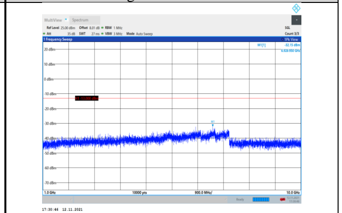
Band26-5MHz-16QAM-26765-1RB#0- Range2:1000~10000MHz
