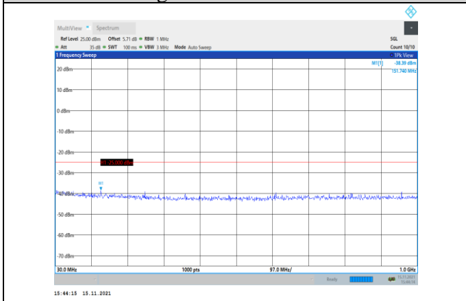
Band38-5MHz-QPSK-38000-1RB#0- Range1:30~1000MHz
