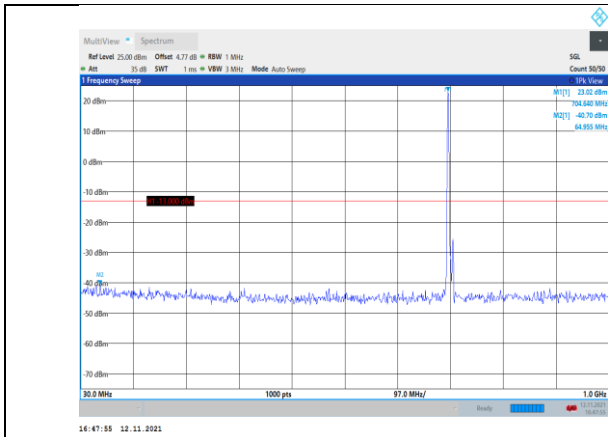
Band17-5MHz-QPSK-23755-1RB#0- Range1:30~1000MHz
