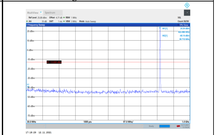
Band26-1.4MHz-16QAM-26783-1RB#0- Range1:30~1000MHz
