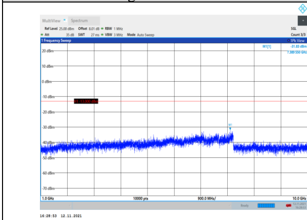
Band12-10MHz-16QAM-23060-1RB#0- Range2:1000~10000MHz
