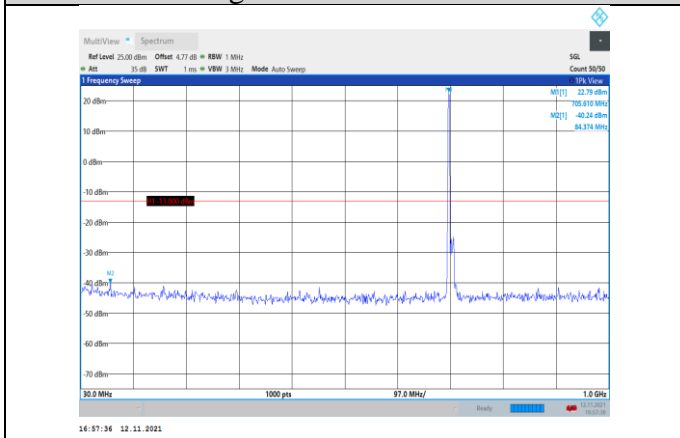
Band17-10MHz-16QAM-23790-1RB#0- Range1:30~1000MHz
