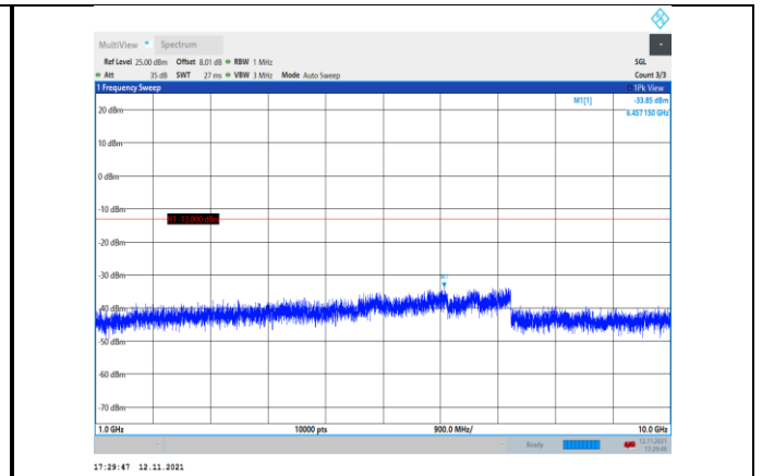
Band26-5MHz-16QAM-26740-1RB#0- Range2:1000~10000MHz
