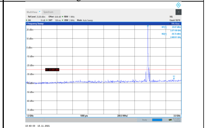
Band38-5MHz-QPSK-37775-1RB#0- Range2:1000~3000MHz
