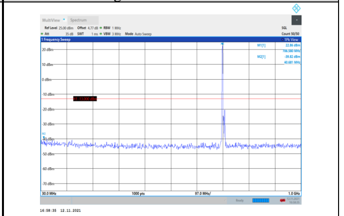
Band17-10MHz-16QAM-23800-1RB#0- Range1:30~1000MHz
