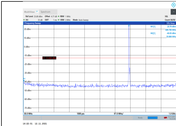
Band12-3MHz-16QAM-23025-1RB#0- Range1:30~1000MHz
