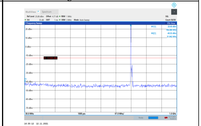
Band12-10MHz-QPSK-23130-1RB#0- Range1:30~1000MHz
