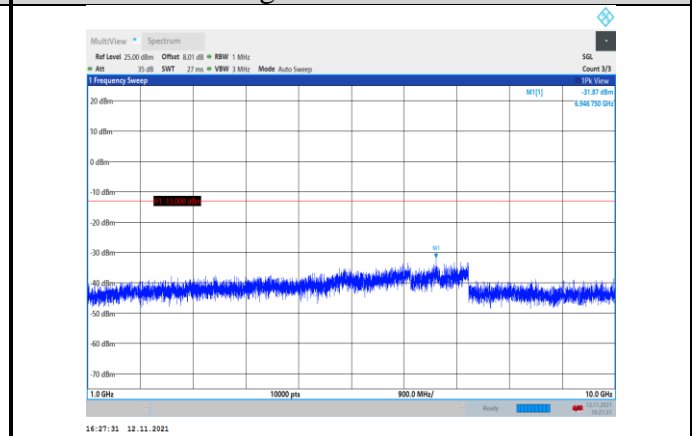
Band12-5MHz-16QAM-23155-1RB#0- Range2:1000~10000MHz
