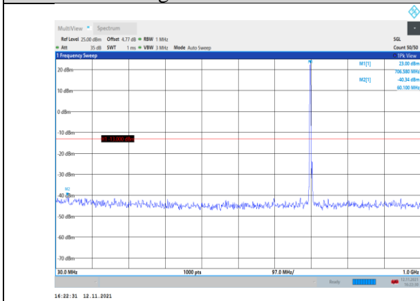
Band12-3MHz-QPSK-23095-1RB#0- Range1:30~1000MHz
