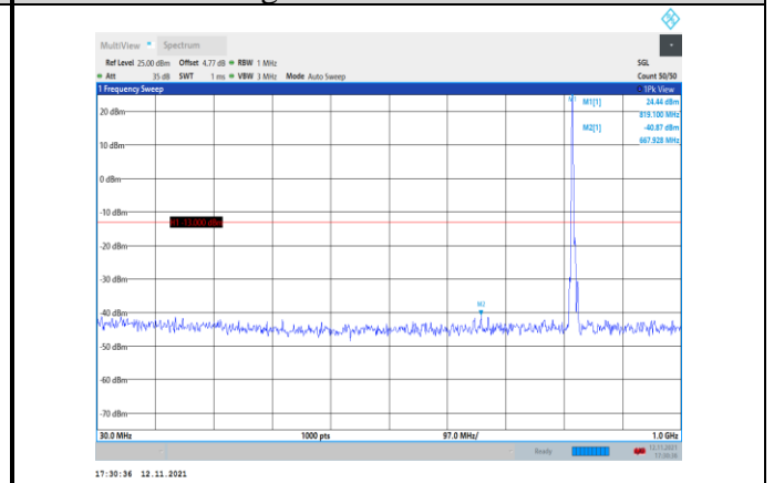
Band26-5MHz-16QAM-26765-1RB#0- Range1:30~1000MHz
