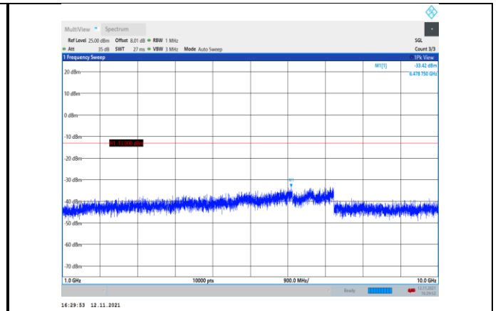
Band12-10MHz-16QAM-23095-1RB#0- Range2:1000~10000MHz
