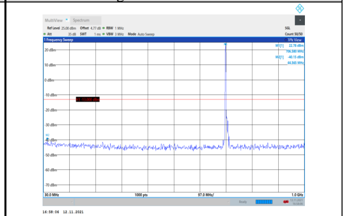
Band17-10MHz-QPSK-23800-1RB#0- Range1:30~1000MHz
