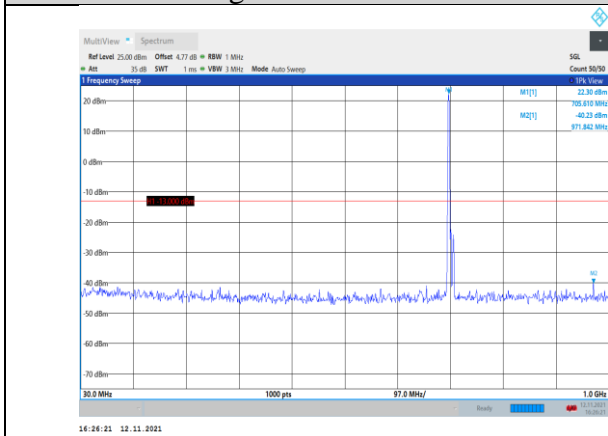
Band12-5MHz-16QAM-23095-1RB#0- Range1:30~1000MHz
