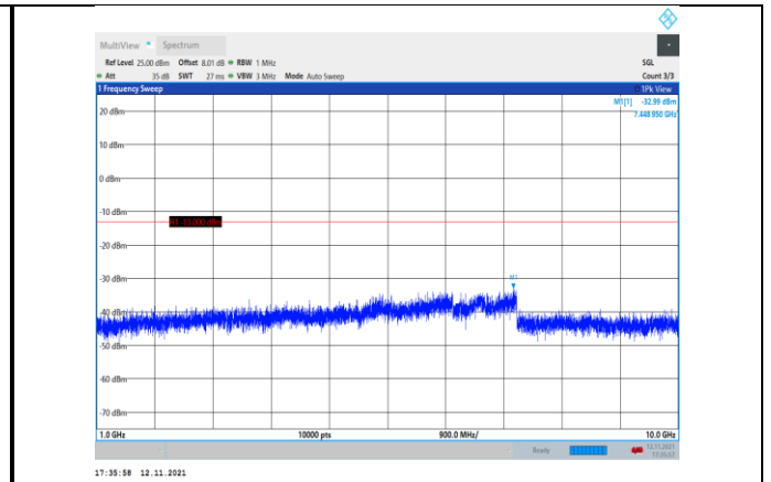
Band26-10MHz-16QAM-26740-1RB#0- Range2:1000~10000MHz
