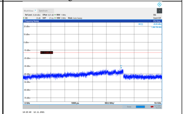
Band12-3MHz-QPSK-23165-1RB#0- Range2:1000~10000MHz
