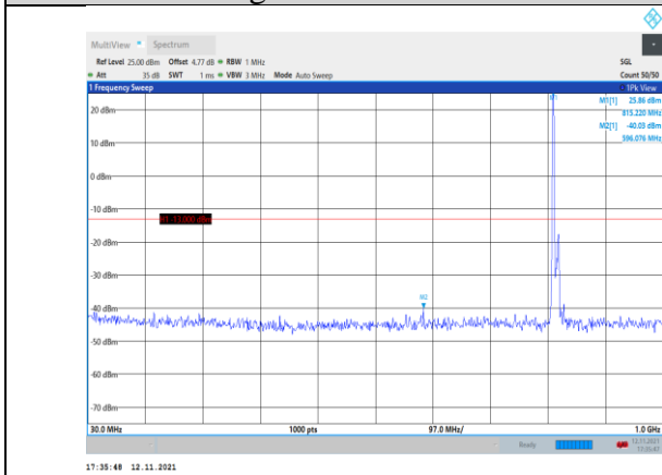
Band26-10MHz-16QAM-26740-1RB#0- Range1:30~1000MHz
