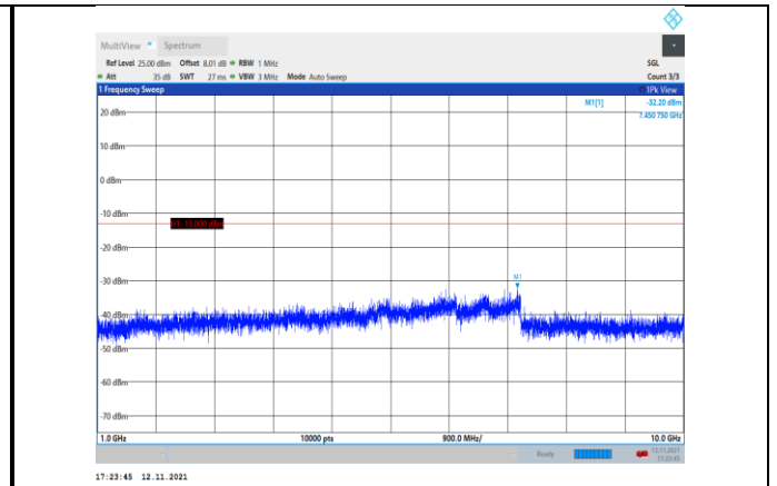
Band26-3MHz-16QAM-26740-1RB#0- Range2:1000~10000MHz
