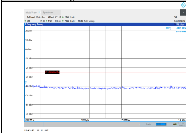
Band38-5MHz-16QAM-37775-1RB#0- Range1:30~1000MHz
