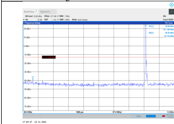
Band26-5MHz-16QAM-26740-1RB#0- Range1:30~1000MHz
