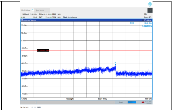
Band12-5MHz-QPSK-23095-1RB#0- Range2:1000~10000MHz
