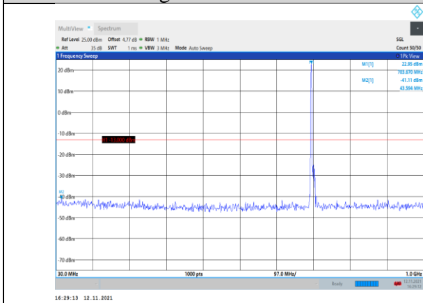
Band12-10MHz-QPSK-23095-1RB#0- Range1:30~1000MHz
