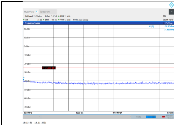
Band7-20MHz-16QAM-21100-1RB#0- Range1:30~1000MHz
