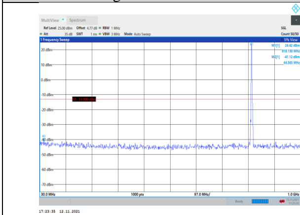
Band26-3MHz-16QAM-26740-1RB#0- Range1:30~1000MHz
