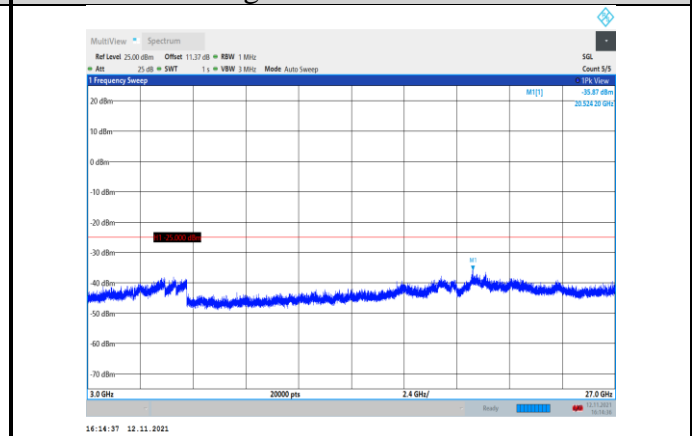
Band7-20MHz-16QAM-21350-1RB#0- Range3:3000~27000MHz
