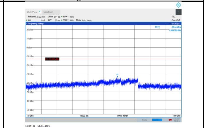
Band12-10MHz-16QAM-23130-1RB#0- Range2:1000~10000MHz
