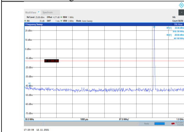
Band26-3MHz-QPSK-26740-1RB#0- Range1:30~1000MHz
