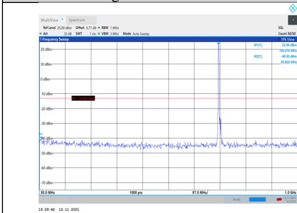
Band12-10MHz-16QAM-23095-1RB#0- Range1:30~1000MHz
