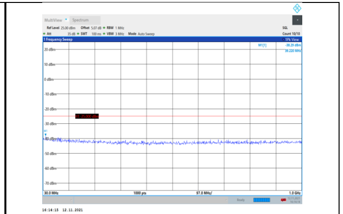
Band7-20MHz-16QAM-21350-1RB#0- Range1:30~1000MHz
