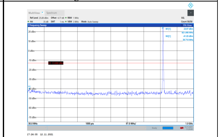
Band26-3MHz-QPSK-26775-1RB#0- Range1:30~1000MHz
