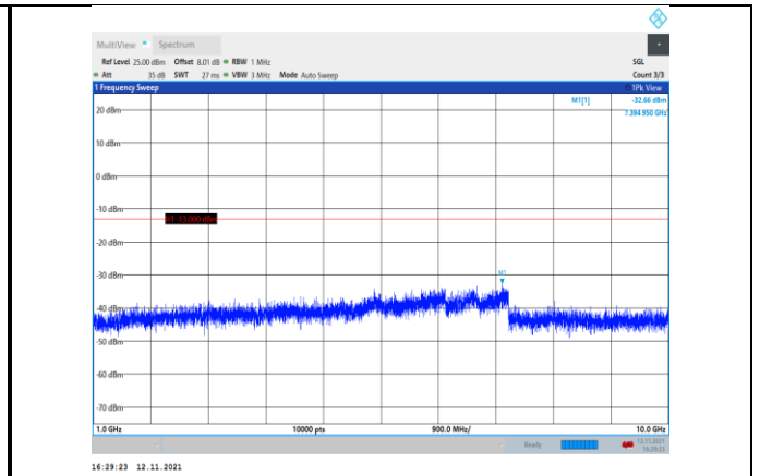
Band12-10MHz-QPSK-23095-1RB#0- Range2:1000~10000MHz
