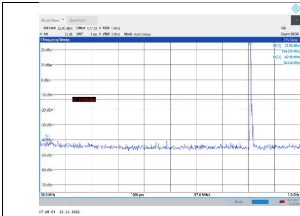
Band26-5MHz-QPSK-26715-1RB#0- Range1:30~1000MHz
