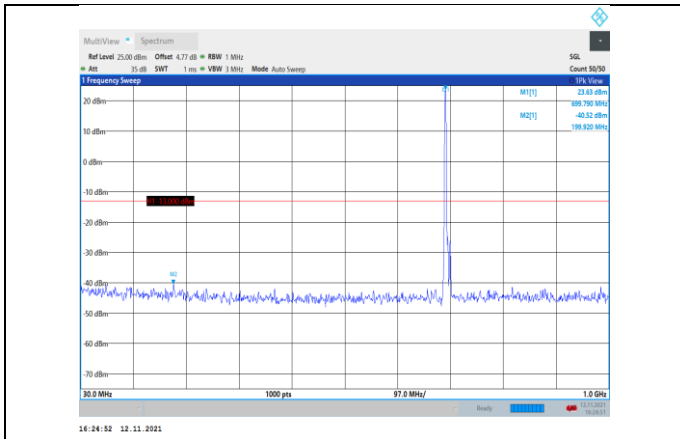
Band12-5MHz-QPSK-23035-1RB#0- Range1:30~1000MHz
