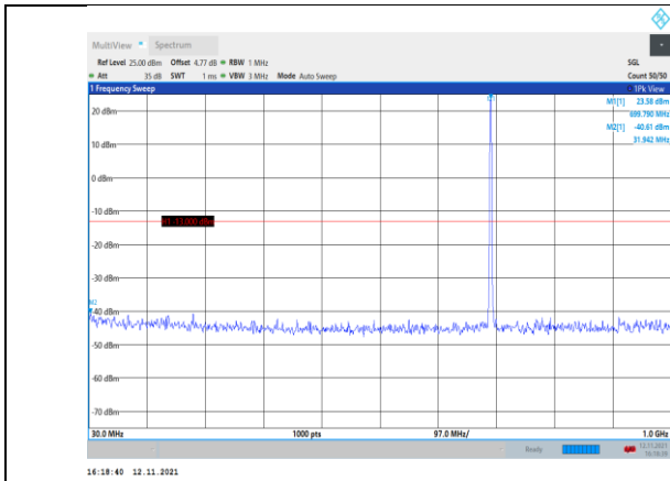
Band12-1.4MHz-16QAM-23017-1RB#0- Range1:30~1000MHz
