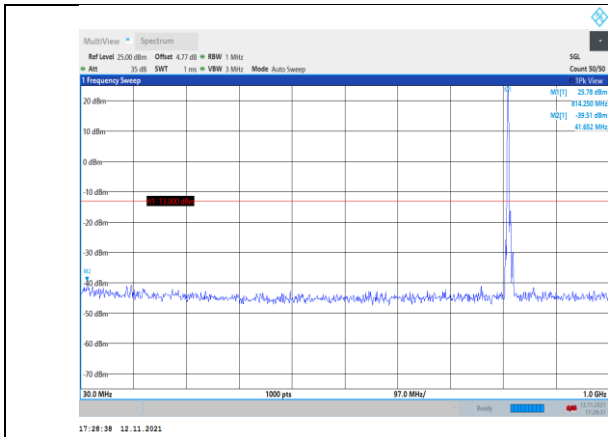
Band26-5MHz-16QAM-26715-1RB#0- Range1:30~1000MHz
