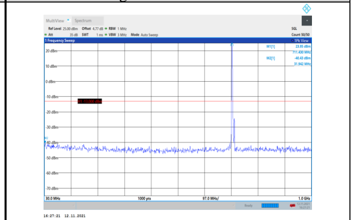
Band12-5MHz-16QAM-23155-1RB#0- Range1:30~1000MHz
