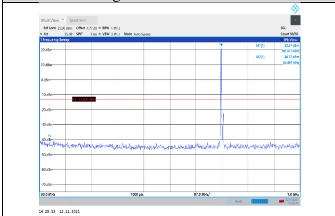
Band12-5MHz-QPSK-23095-1RB#0- Range1:30~1000MHz
