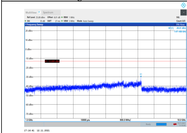
Band26-1.4MHz-16QAM-26697-1RB#0- Range2:1000~10000MHz
