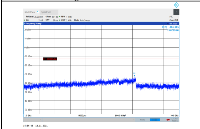
Band17-10MHz-16QAM-23780-1RB#0- Range2:1000~10000MHz
