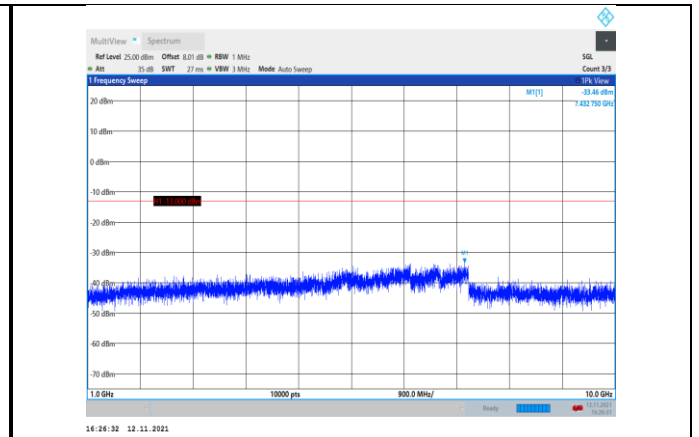
Band12-5MHz-16QAM-23095-1RB#0- Range2:1000~10000MHz
