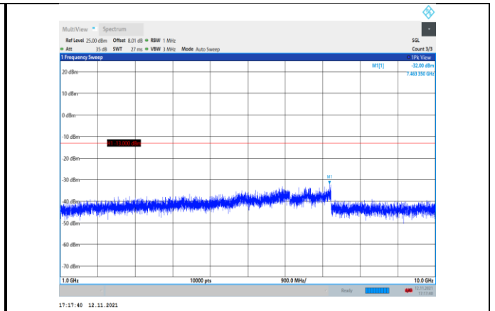
Band26-1.4MHz-16QAM-26740-1RB#0- Range2:1000~10000MHz
