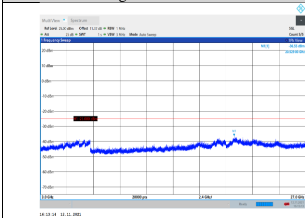
Band7-20MHz-16QAM-21100-1RB#0- Range3:3000~27000MHz
