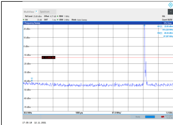
Band26-10MHz-QPSK-26740-1RB#0- Range1:30~1000MHz
