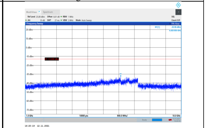
Band12-1.4MHz-QPSK-23173-1RB#0- Range2:1000~10000MHz
