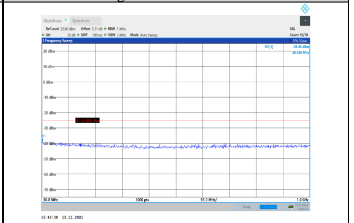
Band38-5MHz-QPSK-38225-1RB#0- Range1:30~1000MHz
