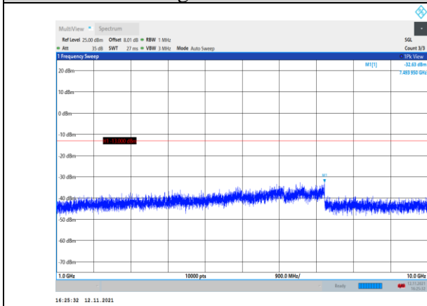
Band12-5MHz-16QAM-23035-1RB#0- Range2:1000~10000MHz
