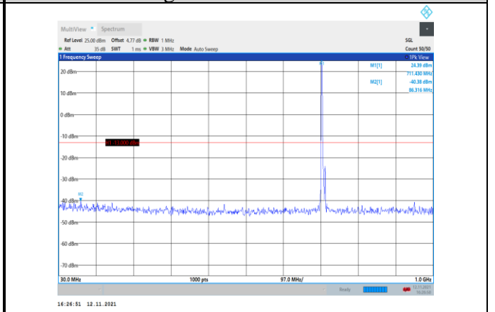
Band12-5MHz-QPSK-23155-1RB#0- Range1:30~1000MHz
