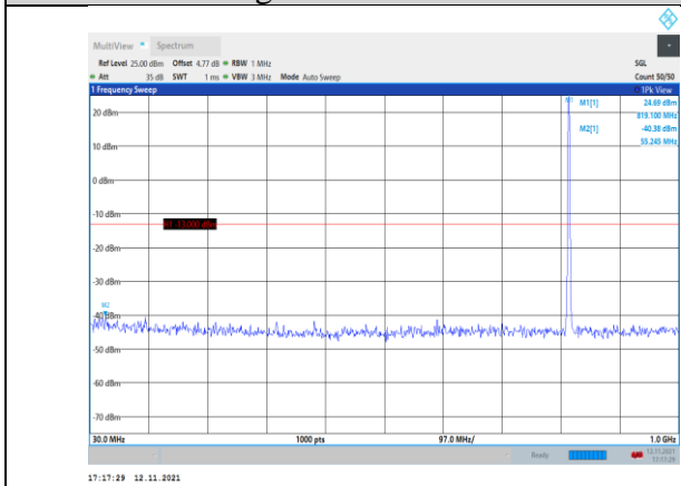
Band26-1.4MHz-16QAM-26740-1RB#0- Range1:30~1000MHz
