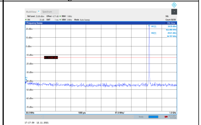
Band26-1.4MHz-QPSK-26783-1RB#0- Range1:30~1000MHz
