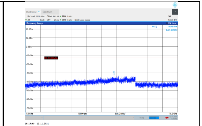
Band12-1.4MHz-16QAM-23095-1RB#0- Range2:1000~10000MHz
