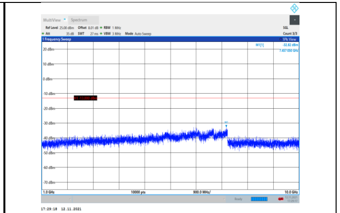
Band26-5MHz-QPSK-26740-1RB#0- Range2:1000~10000MHz
