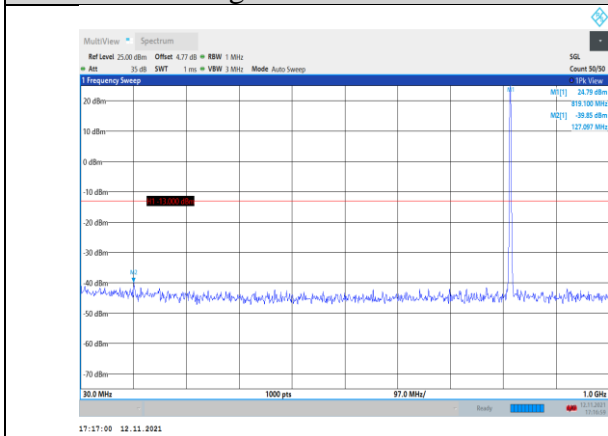
Band26-1.4MHz-QPSK-26740-1RB#0- Range1:30~1000MHz
