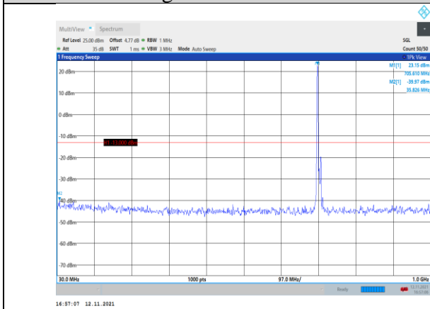
Band17-10MHz-QPSK-23790-1RB#0- Range1:30~1000MHz
