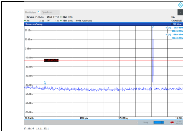
Band26-3MHz-16QAM-26705-1RB#0- Range1:30~1000MHz
