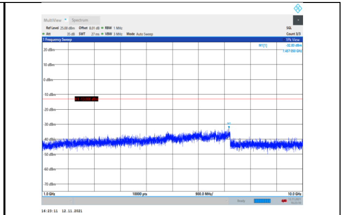
Band12-3MHz-16QAM-23095-1RB#0- Range2:1000~10000MHz
