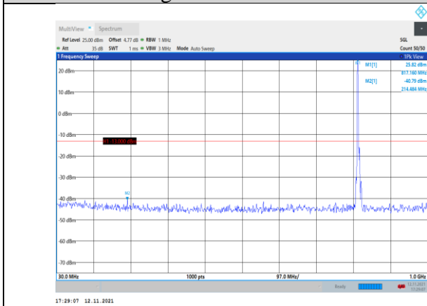
Band26-5MHz-QPSK-26740-1RB#0- Range1:30~1000MHz
