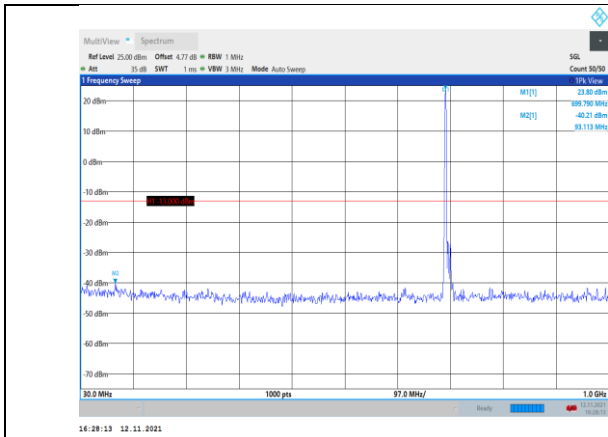
Band12-10MHz-QPSK-23060-1RB#0- Range1:30~1000MHz
