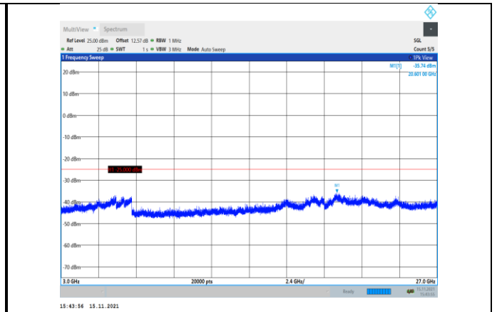
Band38-5MHz-16QAM-37775-1RB#0- Range3:3000~27000MHz
