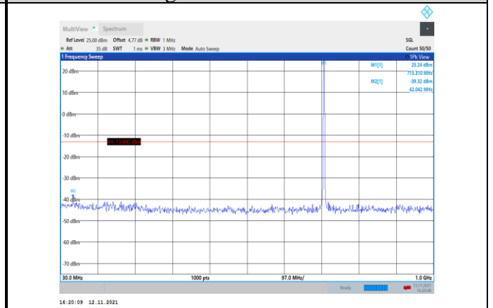
Band12-1.4MHz-QPSK-23173-1RB#0- Range1:30~1000MHz
