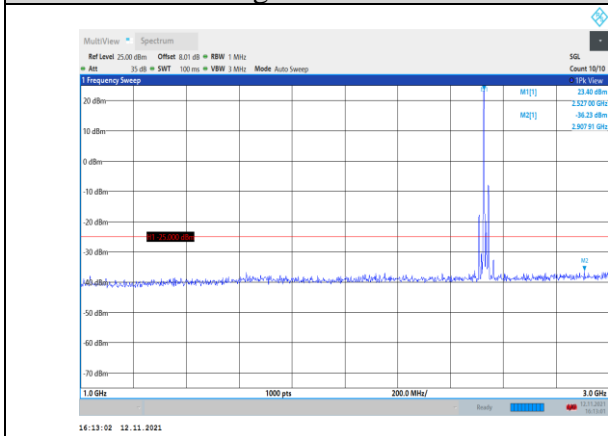
Band7-20MHz-16QAM-21100-1RB#0- Range2:1000~3000MHz
