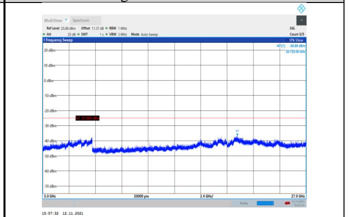
Band7-10MHz-16QAM-20800-1RB#0- Range3:3000~27000MHz
