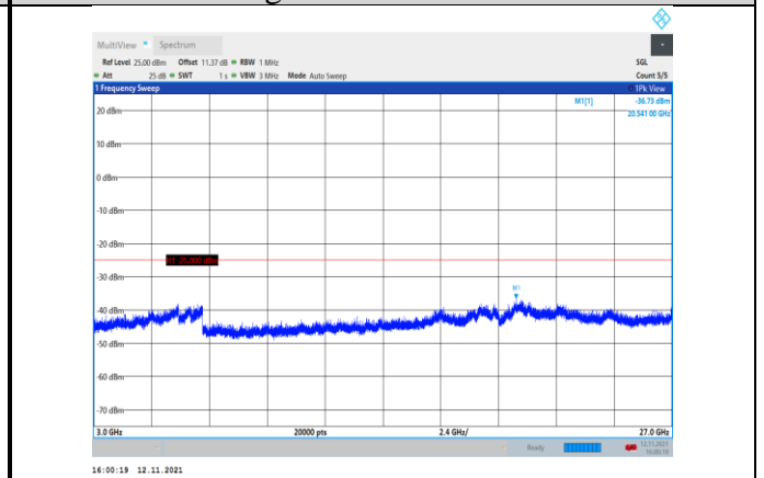
Band7-10MHz-16QAM-21400-1RB#0- Range3:3000~27000MHz
