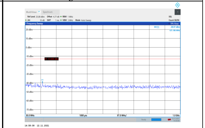
Band4-15MHz-QPSK-20325-1RB#0- Range1:30~1000MHz
