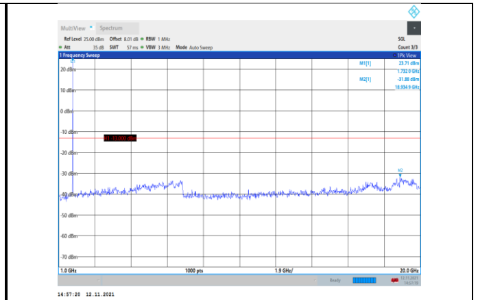
Band4-15MHz-QPSK-20175-1RB#0- Range2:1000~20000MHz
