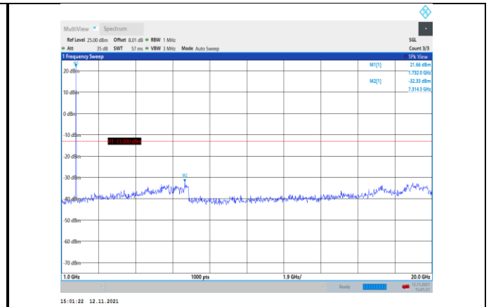
Band4-20MHz-16QAM-20175-1RB#0- Range2:1000~20000MHz
