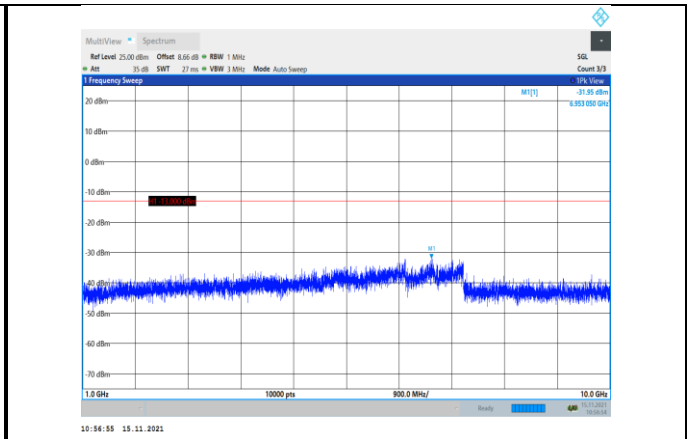
Band5-1.4MHz-QPSK-20525-1RB#0- Range2:1000~10000MHz
