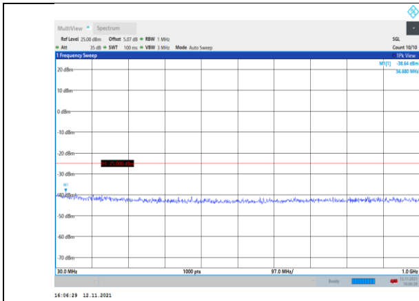
Band7-15MHz-QPSK-21375-1RB#0- Range1:30~1000MHz
