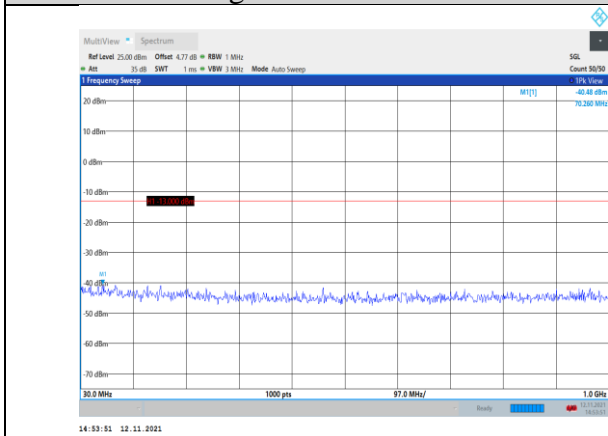
Band4-10MHz-16QAM-20175-1RB#0- Range1:30~1000MHz
