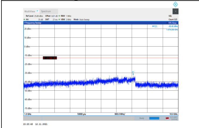
Band5-5MHz-16QAM-20425-1RB#0- Range2:1000~10000MHz
