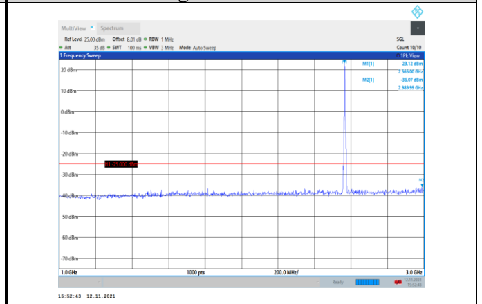
Band7-5MHz-16QAM-21425-1RB#0- Range2:1000~3000MHz
