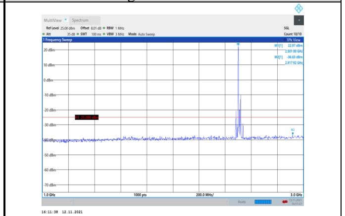
Band7-20MHz-16QAM-20850-1RB#0- Range2:1000~3000MHz
