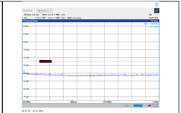
Band7-10MHz-QPSK-21100-1RB#0- Range1:30~1000MHz
