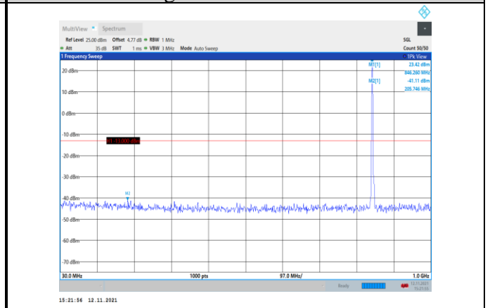
Band5-3MHz-16QAM-20635-1RB#0- Range1:30~1000MHz
