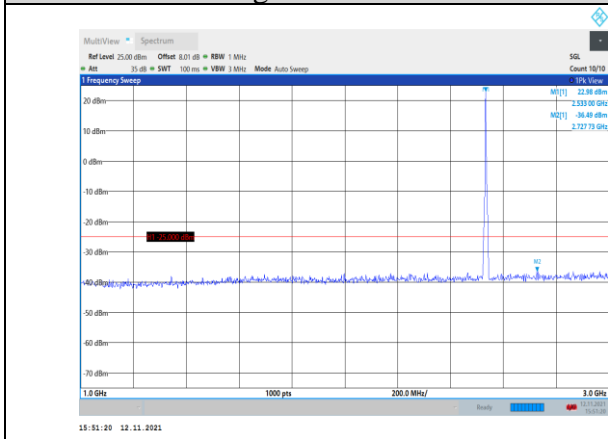
Band7-5MHz-16QAM-21100-1RB#0- Range2:1000~3000MHz
