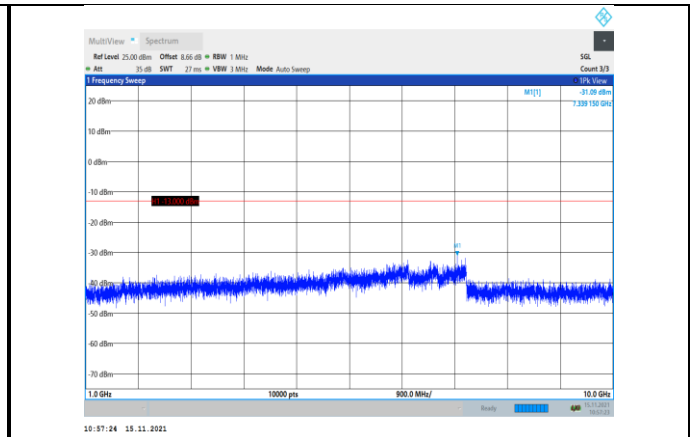
Band5-1.4MHz-16QAM-20525-1RB#0- Range2:1000~10000MHz
