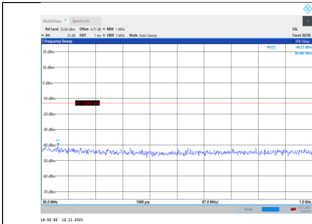
Band4-10MHz-16QAM-20000-1RB#0- Range1:30~1000MHz
