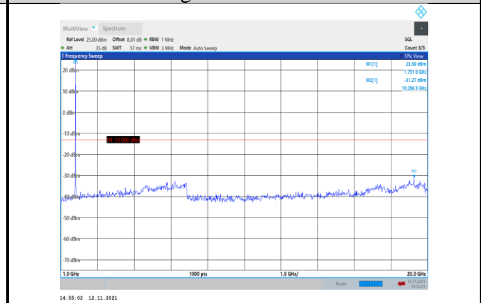
Band4-10MHz-16QAM-20350-1RB#0- Range2:1000~20000MHz
