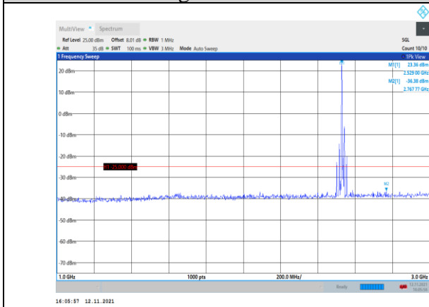
Band7-15MHz-16QAM-21100-1RB#0- Range2:1000~3000MHz
