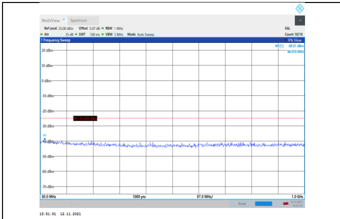
Band7-5MHz-QPSK-21425-1RB#0- Range1:30~1000MHz
