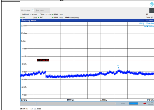
Band7-15MHz-QPSK-21375-1RB#0- Range3:3000~27000MHz
