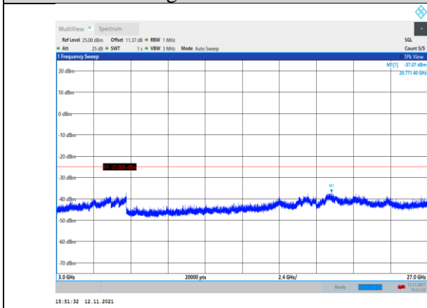
Band7-5MHz-16QAM-21100-1RB#0- Range3:3000~27000MHz
