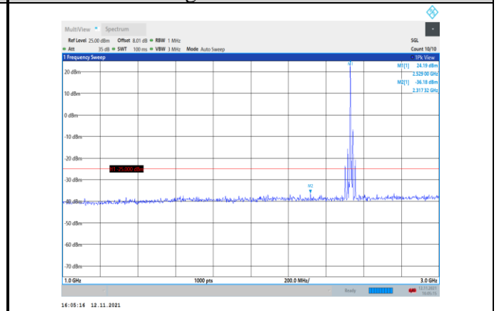
Band7-15MHz-QPSK-21100-1RB#0- Range2:1000~3000MHz
