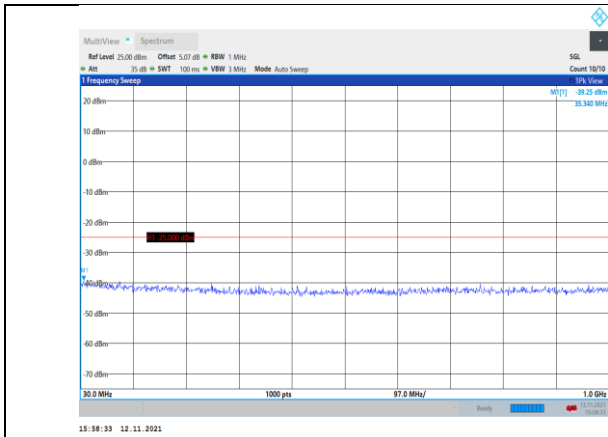
Band7-10MHz-16QAM-21100-1RB#0- Range1:30~1000MHz
