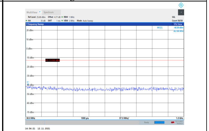
Band4-10MHz-QPSK-20350-1RB#0- Range1:30~1000MHz
