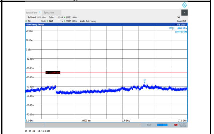
Band7-5MHz-16QAM-20775-1RB#0- Range3:3000~27000MHz
