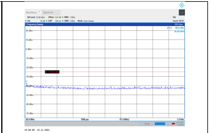
Band7-5MHz-16QAM-20775-1RB#0- Range1:30~1000MHz
