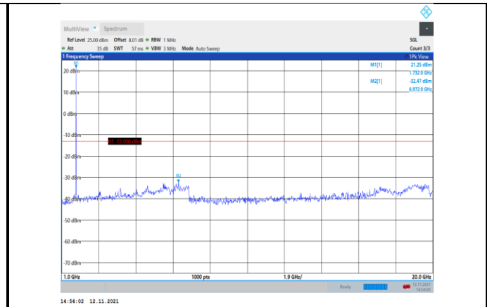
Band4-10MHz-16QAM-20175-1RB#0- Range2:1000~20000MHz
