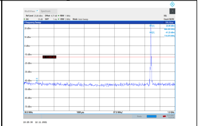
Band5-5MHz-16QAM-20625-1RB#0- Range1:30~1000MHz
