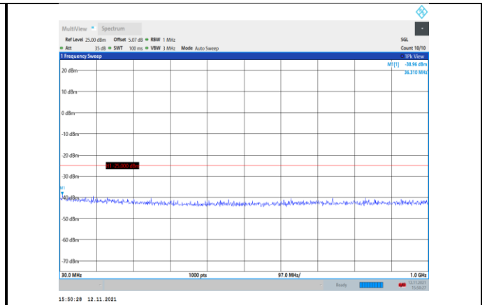
Band7-5MHz-QPSK-21100-1RB#0- Range1:30~1000MHz
