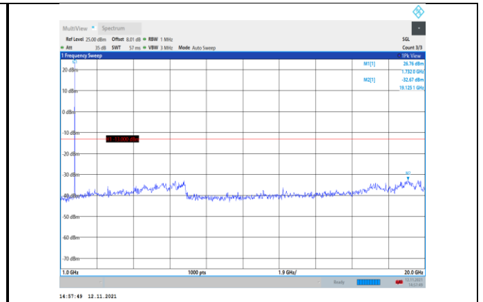
Band4-15MHz-16QAM-20175-1RB#0- Range2:1000~20000MHz
