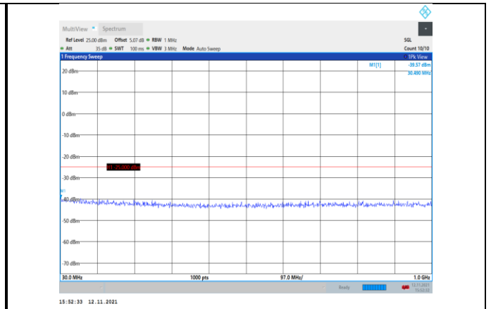
Band7-5MHz-16QAM-21425-1RB#0- Range1:30~1000MHz
