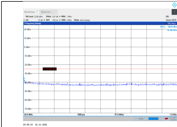
Band7-10MHz-QPSK-21400-1RB#0- Range1:30~1000MHz
