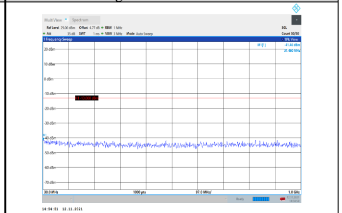
Band4-10MHz-16QAM-20350-1RB#0- Range1:30~1000MHz
