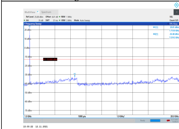
Band4-20MHz-16QAM-20050-1RB#0- Range2:1000~20000MHz
