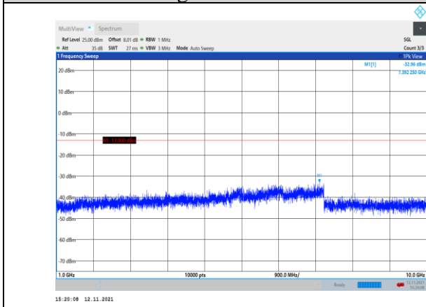
Band5-3MHz-16QAM-20415-1RB#0- Range2:1000~10000MHz
