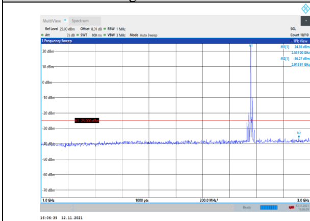
Band7-15MHz-QPSK-21375-1RB#0- Range2:1000~3000MHz
