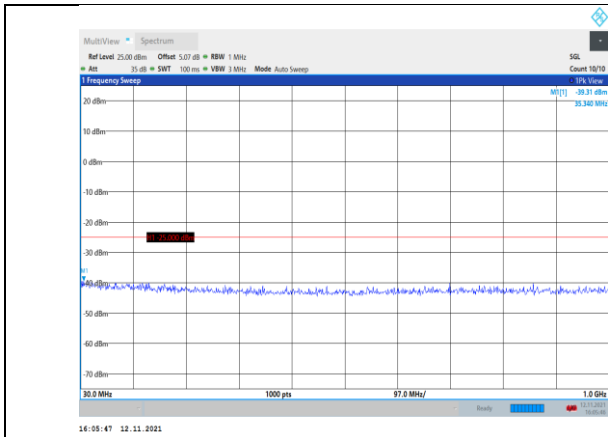
Band7-15MHz-16QAM-21100-1RB#0- Range1:30~1000MHz
