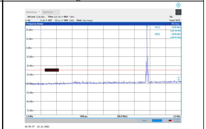
Band7-10MHz-16QAM-21400-1RB#0- Range2:1000~3000MHz
