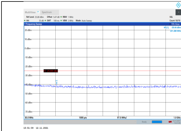
Band7-5MHz-16QAM-21100-1RB#0- Range1:30~1000MHz
