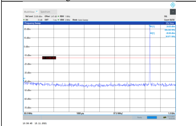
Band5-1.4MHz-QPSK-20525-1RB#0- Range1:30~1000MHz
