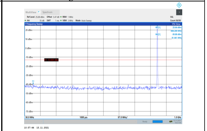
Band5-1.4MHz-QPSK-20643-1RB#0- Range1:30~1000MHz
