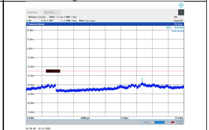
Band7-15MHz-16QAM-20825-1RB#0- Range3:3000~27000MHz
