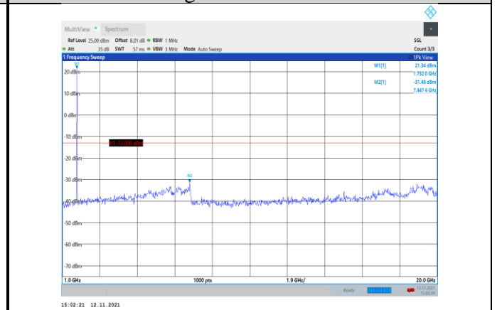
Band4-20MHz-16QAM-20300-1RB#0- Range2:1000~20000MHz
