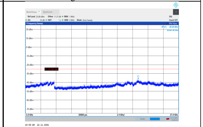
Band7-15MHz-QPSK-21100-1RB#0- Range3:3000~27000MHz
