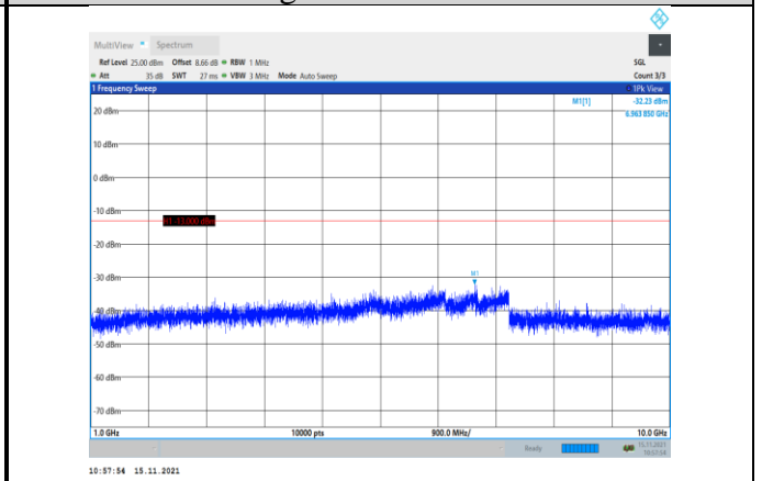
Band5-1.4MHz-QPSK-20643-1RB#0- Range2:1000~10000MHz
