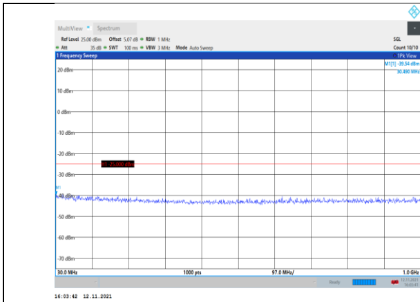
Band7-15MHz-QPSK-20825-1RB#0- Range1:30~1000MHz
