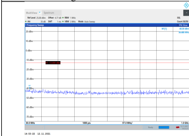
Band4-10MHz-QPSK-20175-1RB#0- Range1:30~1000MHz
