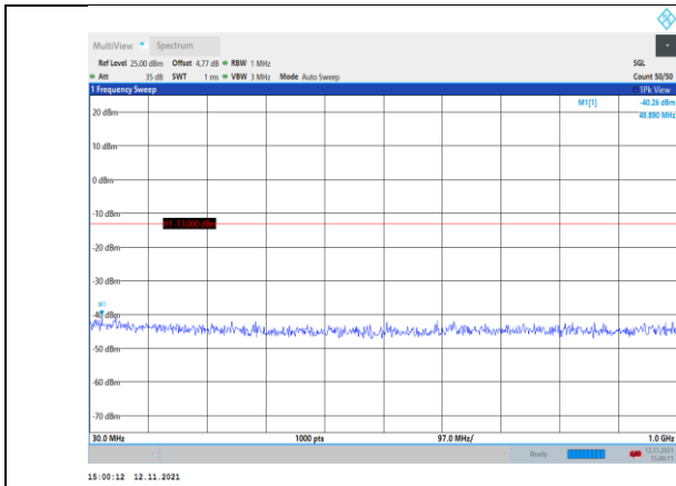
Band4-20MHz-16QAM-20050-1RB#0- Range1:30~1000MHz
