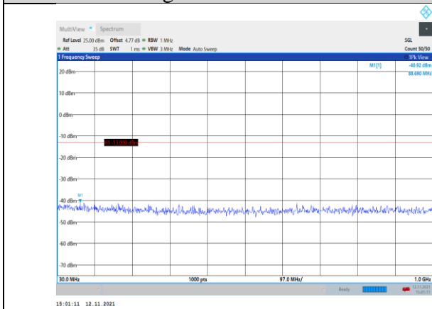
Band4-20MHz-16QAM-20175-1RB#0- Range1:30~1000MHz
