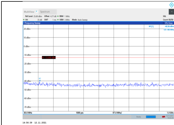
Band4-15MHz-16QAM-20025-1RB#0- Range1:30~1000MHz
