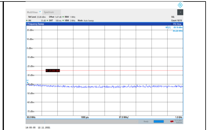
Band7-15MHz-QPSK-21100-1RB#0- Range1:30~1000MHz
