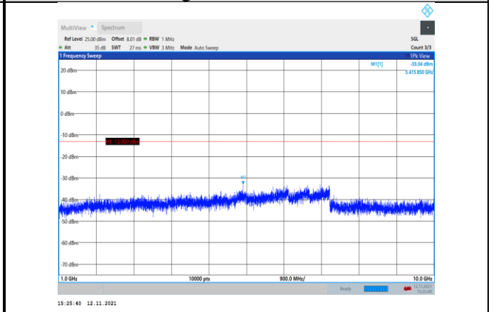
Band5-5MHz-16QAM-20625-1RB#0- Range2:1000~10000MHz
