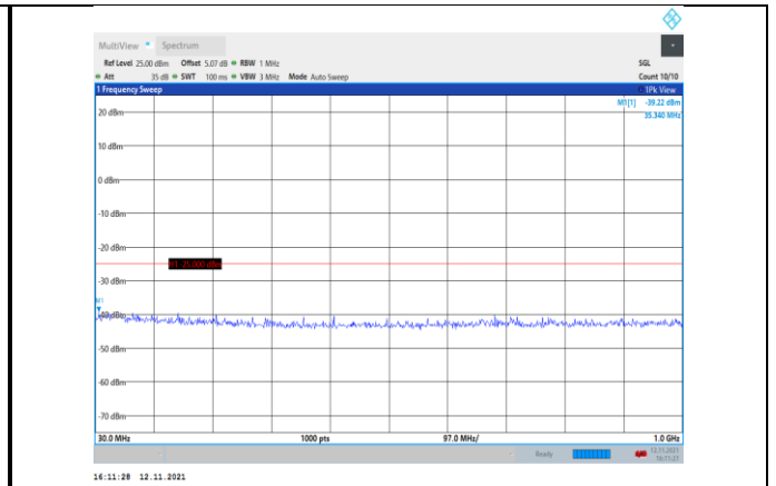
Band7-20MHz-16QAM-20850-1RB#0- Range1:30~1000MHz
