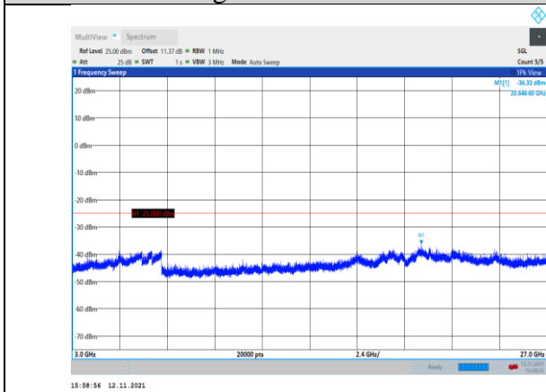
Band7-10MHz-16QAM-21100-1RB#0- Range3:3000~27000MHz
