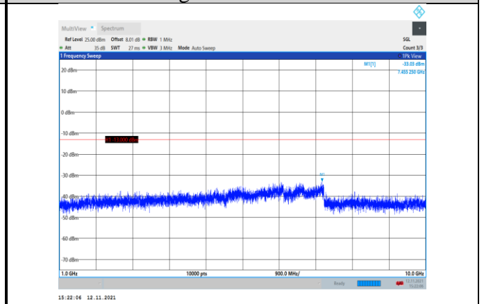
Band5-3MHz-16QAM-20635-1RB#0- Range2:1000~10000MHz
