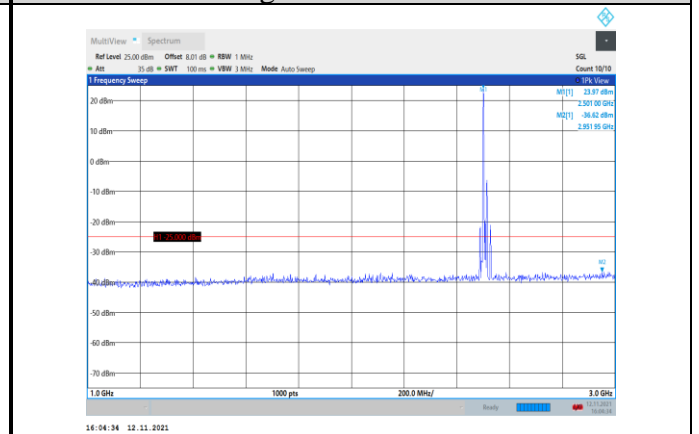
Band7-15MHz-16QAM-20825-1RB#0- Range2:1000~3000MHz
