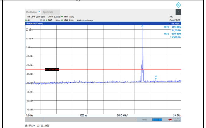
Band7-10MHz-16QAM-20800-1RB#0- Range2:1000~3000MHz
