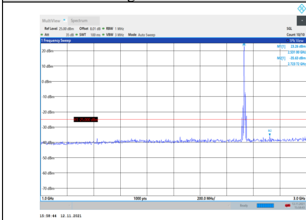
Band7-10MHz-16QAM-21100-1RB#0- Range2:1000~3000MHz
