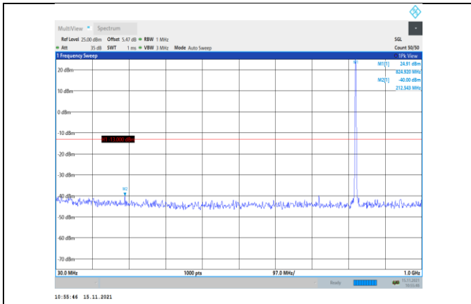
Band5-1.4MHz-QPSK-20407-1RB#0- Range1:30~1000MHz
