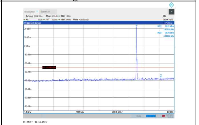
Band7-5MHz-16QAM-20775-1RB#0- Range2:1000~3000MHz
