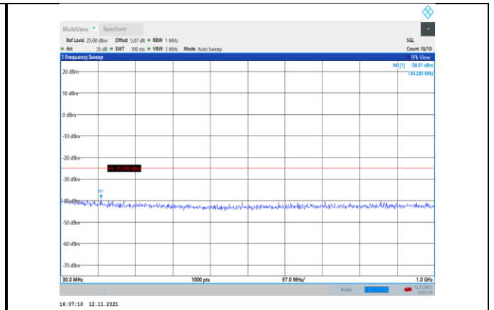
Band7-15MHz-16QAM-21375-1RB#0- Range1:30~1000MHz
