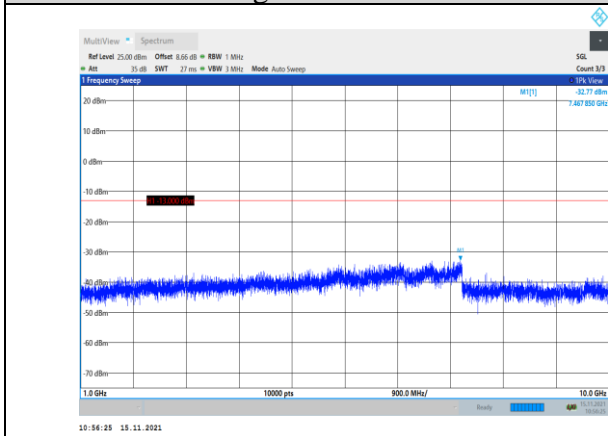
Band5-1.4MHz-16QAM-20407-1RB#0- Range2:1000~10000MHz
