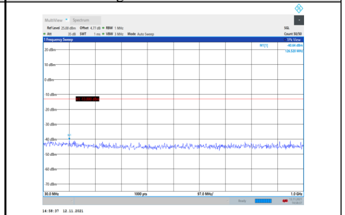
Band4-15MHz-16QAM-20325-1RB#0- Range1:30~1000MHz
