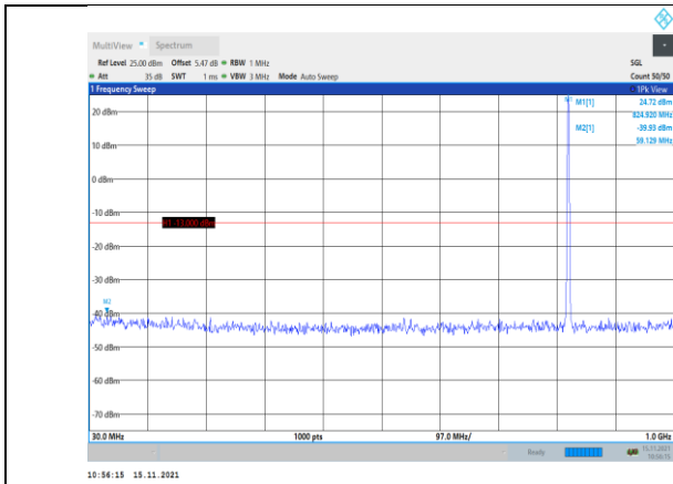
Band5-1.4MHz-16QAM-20407-1RB#0- Range1:30~1000MHz
