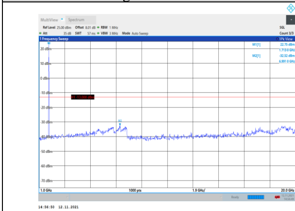
Band4-15MHz-16QAM-20025-1RB#0- Range2:1000~20000MHz
