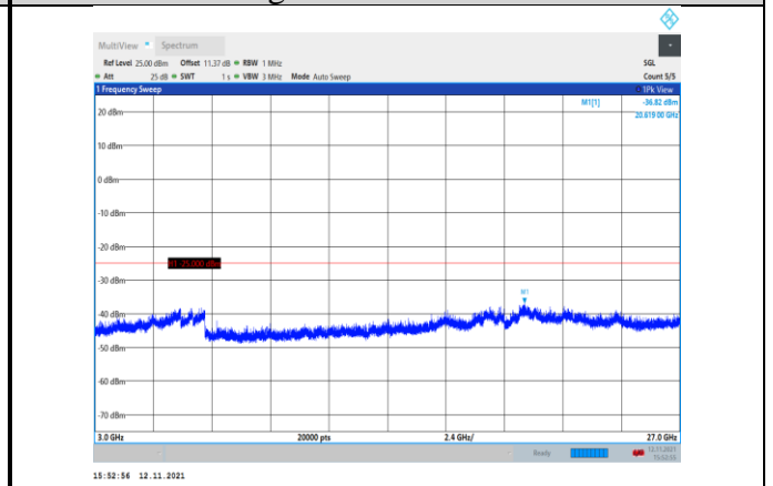
Band7-5MHz-16QAM-21425-1RB#0- Range3:3000~27000MHz
