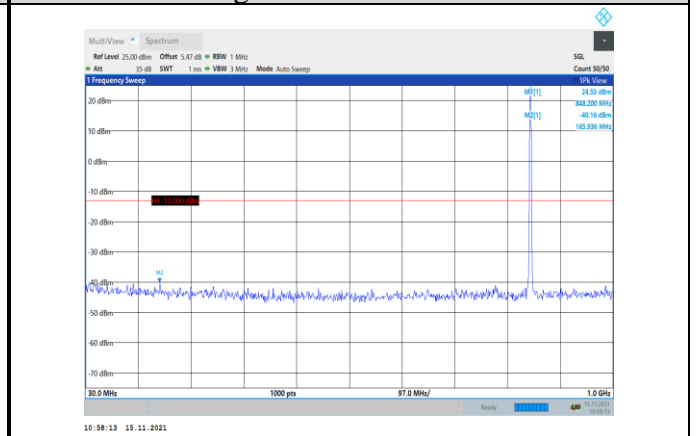
Band5-1.4MHz-16QAM-20643-1RB#0- Range1:30~1000MHz
