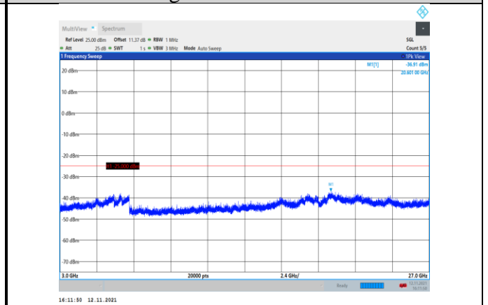
Band7-20MHz-16QAM-20850-1RB#0- Range3:3000~27000MHz
