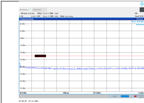
Band7-5MHz-QPSK-20775-1RB#0- Range1:30~1000MHz
