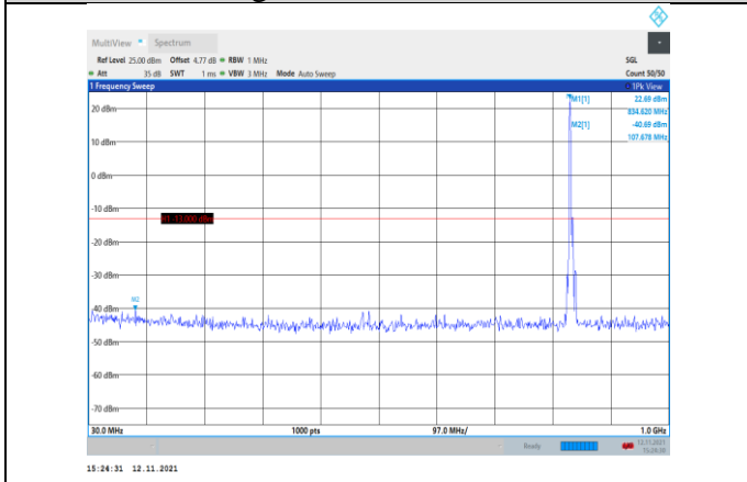
Band5-5MHz-16QAM-20525-1RB#0- Range1:30~1000MHz
