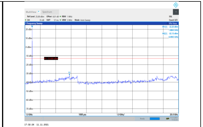
Band2-1.4MHz-16QAM-18900-1RB#0- Range2:1000~20000MHz
