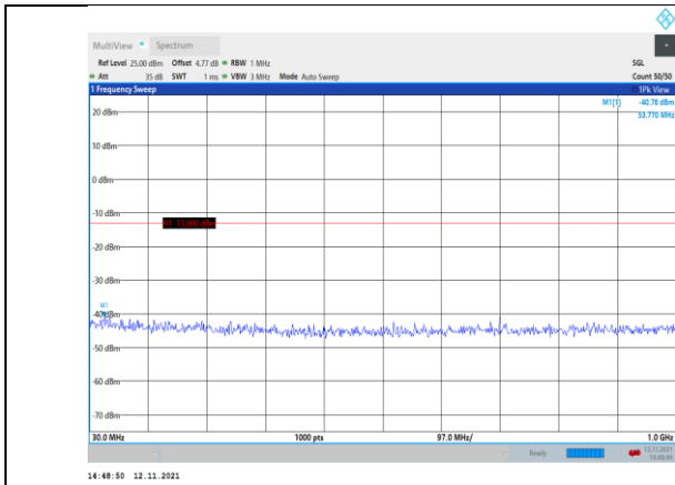
Band4-5MHz-QPSK-19975-1RB#0- Range1:30~1000MHz
