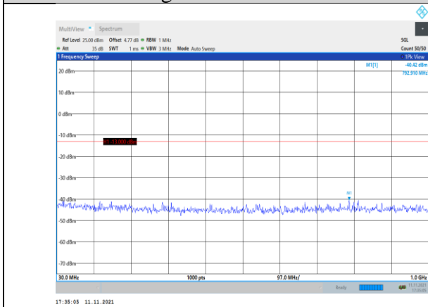
Band2-3MHz-QPSK-18900-1RB#0- Range1:30~1000MHz
