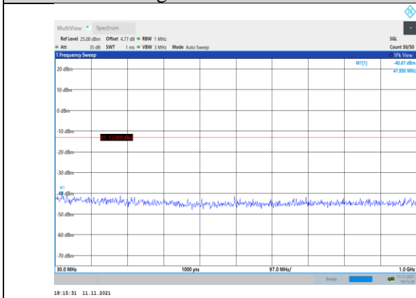
Band2-10MHz-16QAM-18900-1RB#0- Range1:30~1000MHz
