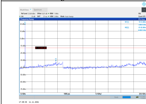
Band2-5MHz-16QAM-18625-1RB#0- Range2:1000~20000MHz
