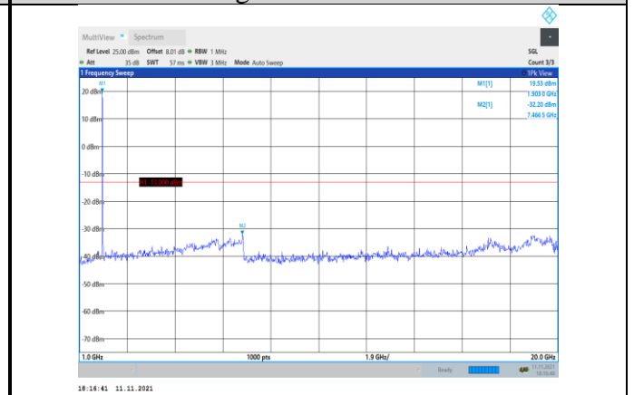
Band2-10MHz-16QAM-19150-1RB#0- Range2:1000~20000MHz
