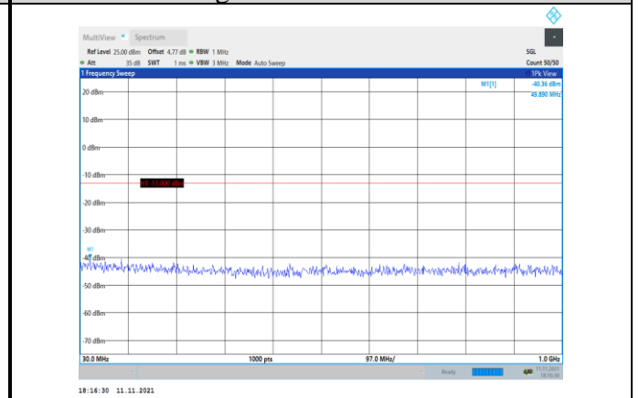
Band2-10MHz-16QAM-19150-1RB#0- Range1:30~1000MHz
