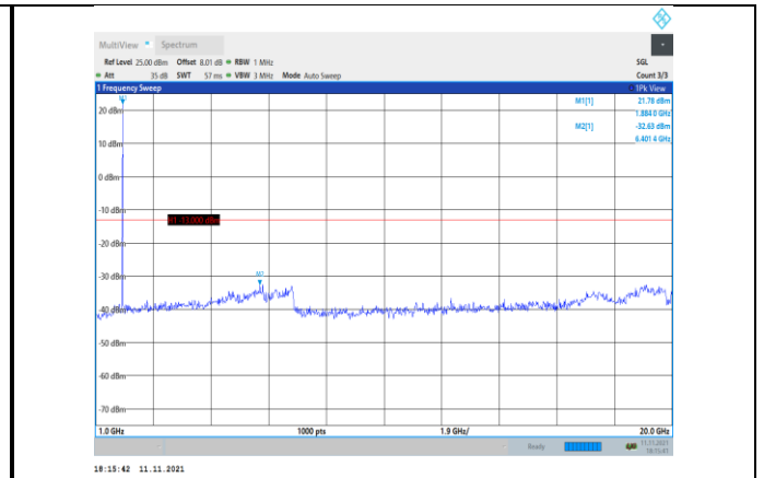
Band2-10MHz-16QAM-18900-1RB#0- Range2:1000~20000MHz
