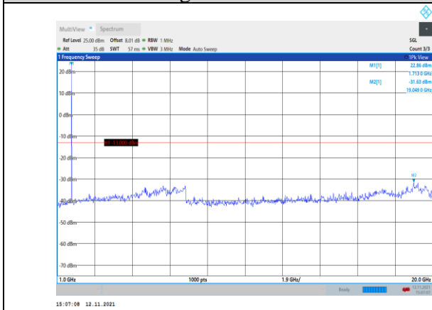
Band4-1.4MHz-16QAM-19957-1RB#0- Range2:1000~20000MHz
