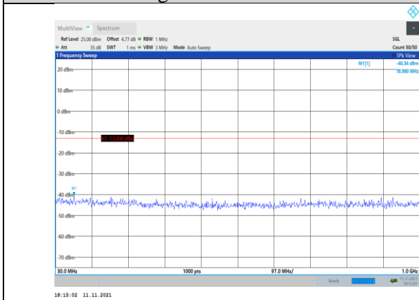
Band2-10MHz-QPSK-18900-1RB#0- Range1:30~1000MHz
