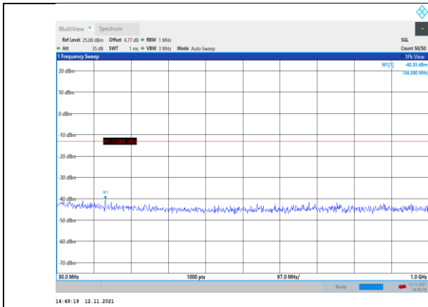
Band4-5MHz-16QAM-19975-1RB#0- Range1:30~1000MHz
