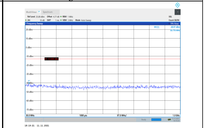
Band2-15MHz-QPSK-19125-1RB#0- Range1:30~1000MHz
