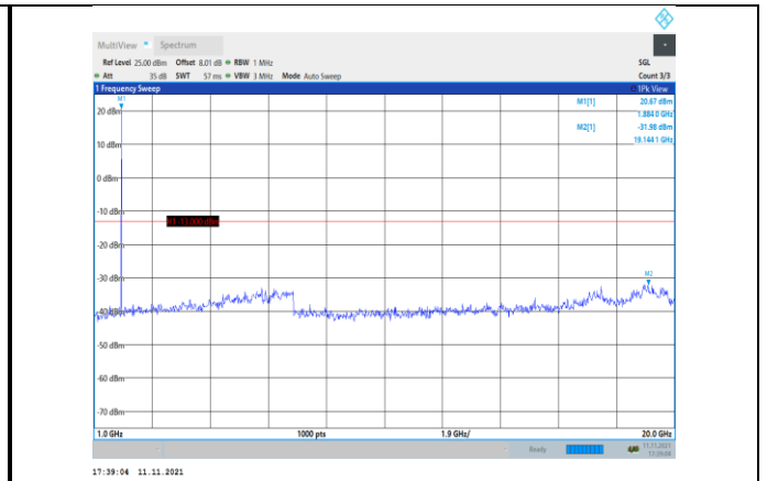
Band2-5MHz-16QAM-18900-1RB#0- Range2:1000~20000MHz
