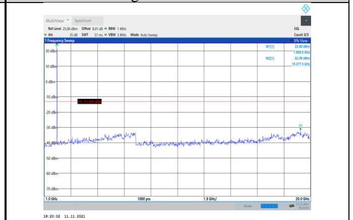
Band2-15MHz-16QAM-19125-1RB#0- Range2:1000~20000MHz
