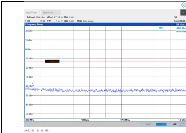
Band2-20MHz-16QAM-18700-1RB#0- Range1:30~1000MHz
