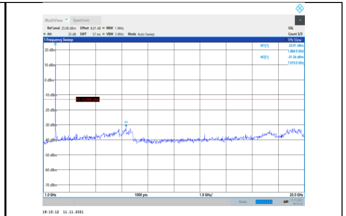
Band2-10MHz-QPSK-18900-1RB#0- Range2:1000~20000MHz
