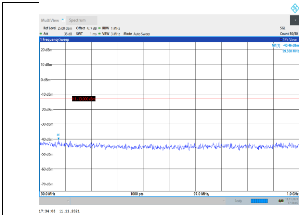
Band2-3MHz-QPSK-18615-1RB#0- Range1:30~1000MHz
