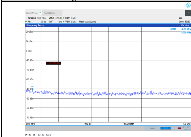
Band4-5MHz-16QAM-20175-1RB#0- Range1:30~1000MHz
