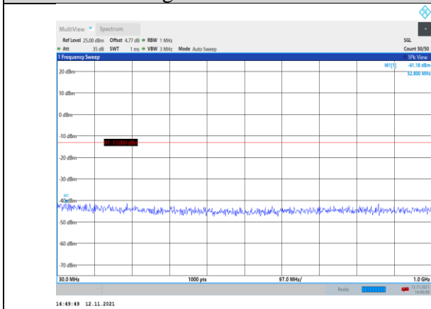
Band4-5MHz-QPSK-20175-1RB#0- Range1:30~1000MHz
