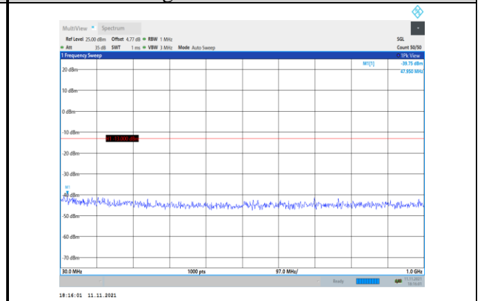
Band2-10MHz-QPSK-19150-1RB#0- Range1:30~1000MHz
