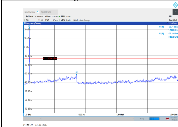
Band4-5MHz-16QAM-19975-1RB#0- Range2:1000~20000MHz
