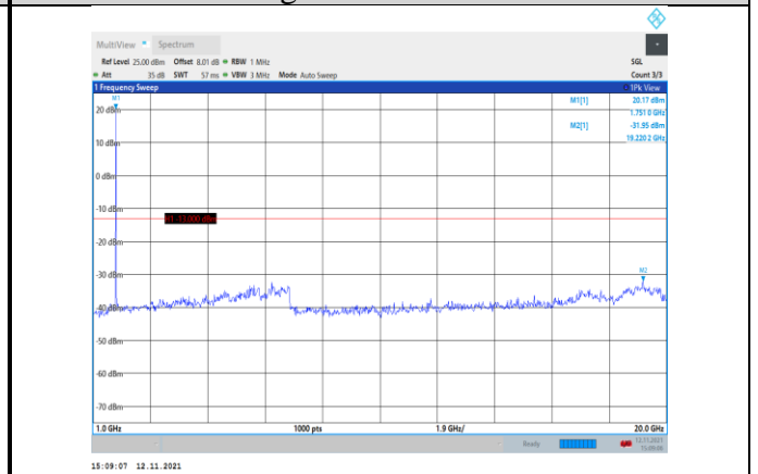
Band4-1.4MHz-16QAM-20393-1RB#0- Range2:1000~20000MHz
