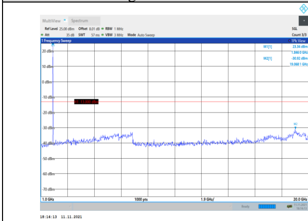
Band2-10MHz-QPSK-18650-1RB#0- Range2:1000~20000MHz
