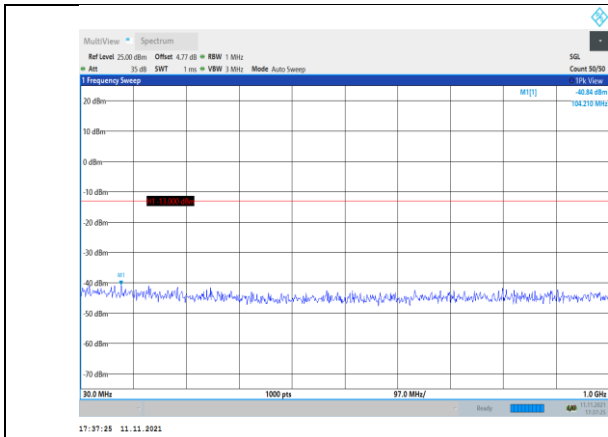
Band2-5MHz-QPSK-18625-1RB#0- Range1:30~1000MHz
