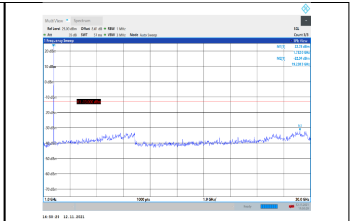
Band4-5MHz-16QAM-20175-1RB#0- Range2:1000~20000MHz
