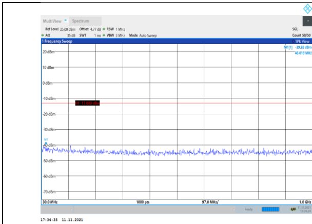
Band2-3MHz-16QAM-18615-1RB#0- Range1:30~1000MHz
