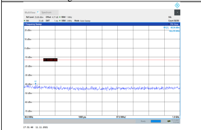
Band2-1.4MHz-QPSK-18900-1RB#0- Range1:30~1000MHz
