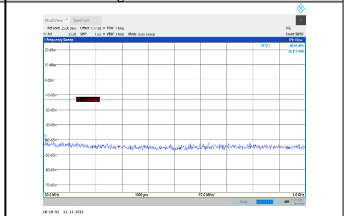
Band2-15MHz-16QAM-19125-1RB#0- Range1:30~1000MHz
