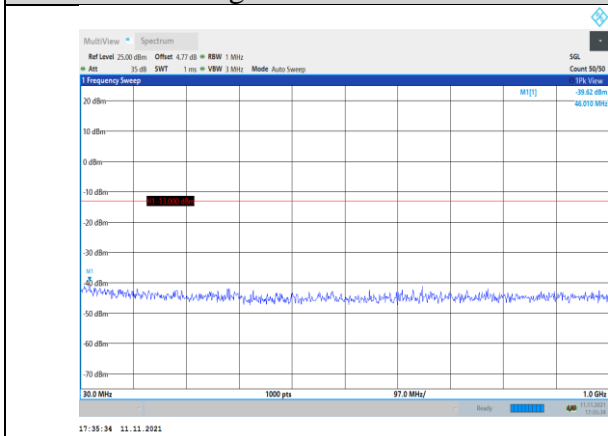
Band2-3MHz-16QAM-18900-1RB#0- Range1:30~1000MHz
