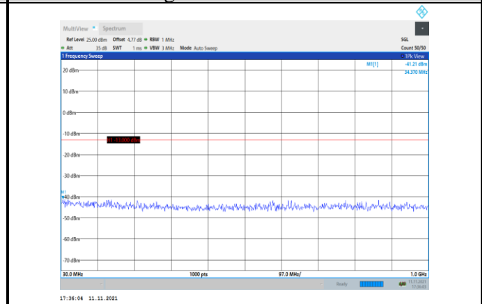
Band2-3MHz-QPSK-19185-1RB#0- Range1:30~1000MHz
