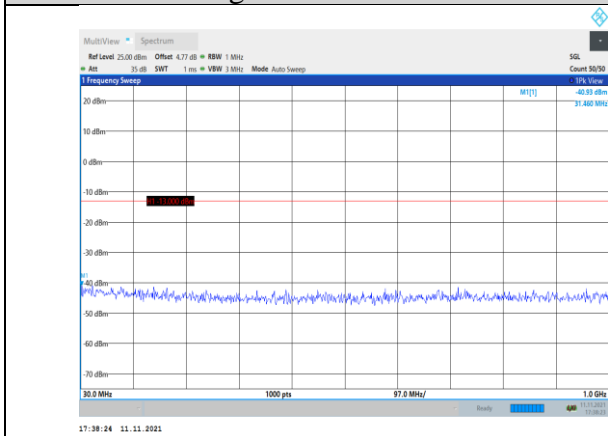
Band2-5MHz-QPSK-18900-1RB#0- Range1:30~1000MHz
