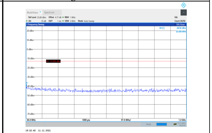
Band2-20MHz-QPSK-19100-1RB#0- Range1:30~1000MHz
