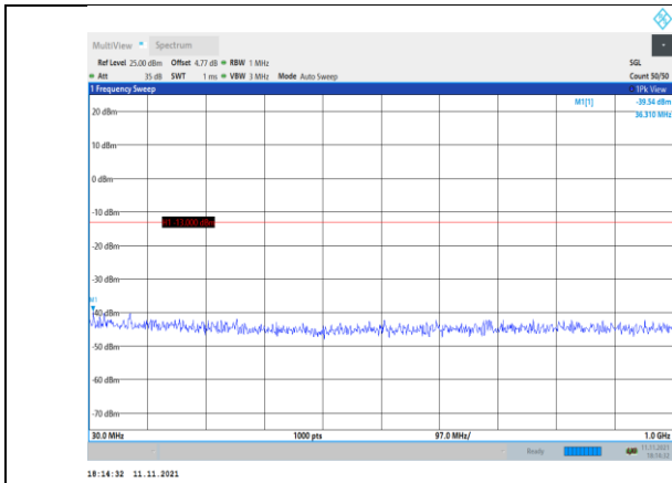
Band2-10MHz-16QAM-18650-1RB#0- Range1:30~1000MHz
