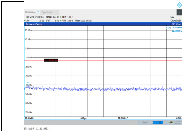
Band2-1.4MHz-16QAM-18607-1RB#0- Range1:30~1000MHz
