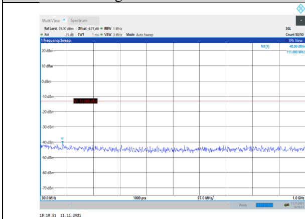
Band2-15MHz-16QAM-18900-1RB#0- Range1:30~1000MHz
