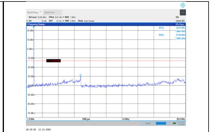
Band2-15MHz-16QAM-18900-1RB#0- Range2:1000~20000MHz
