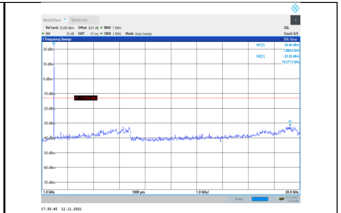
Band2-3MHz-16QAM-18900-1RB#0- Range2:1000~20000MHz
