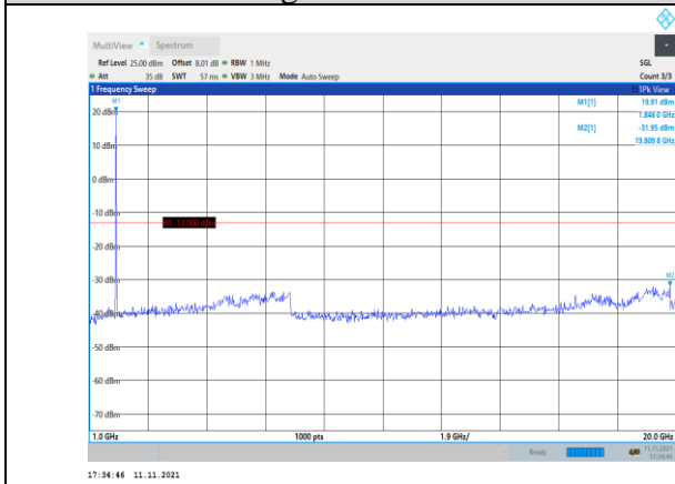
Band2-3MHz-16QAM-18615-1RB#0- Range2:1000~20000MHz
