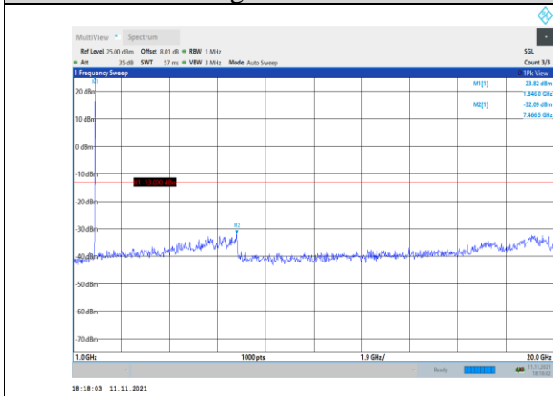
Band2-15MHz-16QAM-18675-1RB#0- Range2:1000~20000MHz
