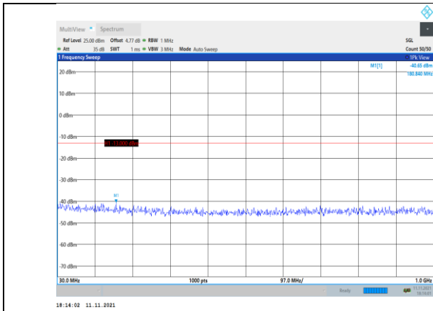
Band2-10MHz-QPSK-18650-1RB#0- Range1:30~1000MHz
