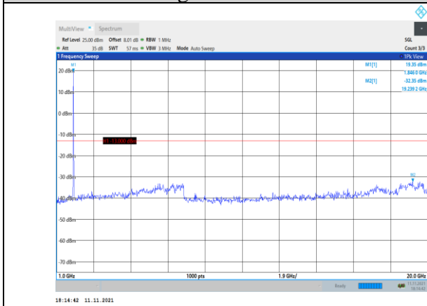
Band2-10MHz-16QAM-18650-1RB#0- Range2:1000~20000MHz
