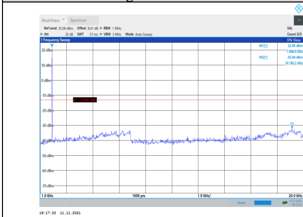
Band2-15MHz-QPSK-18675-1RB#0- Range2:1000~20000MHz
