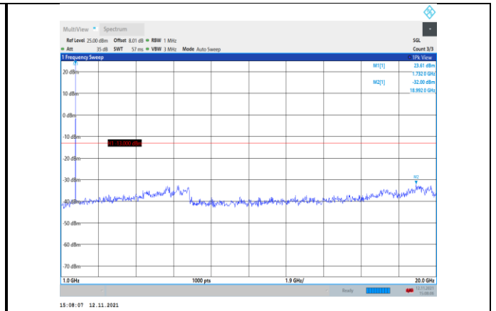
Band4-1.4MHz-16QAM-20175-1RB#0- Range2:1000~20000MHz
