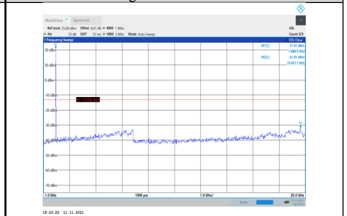
Band2-20MHz-16QAM-19100-1RB#0- Range2:1000~20000MHz
