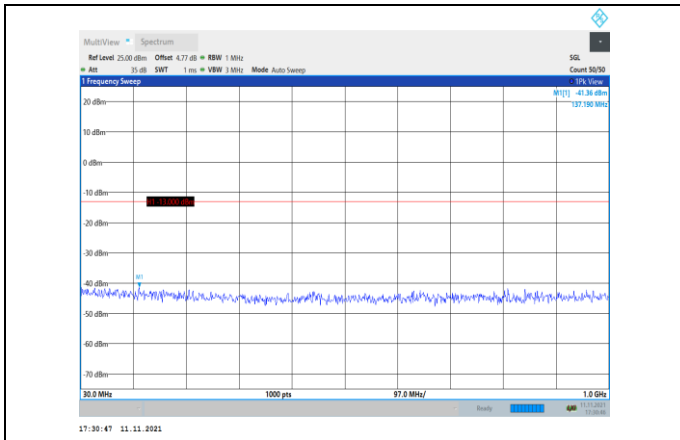
Band2-1.4MHz-QPSK-18607-1RB#0- Range1:30~1000MHz
