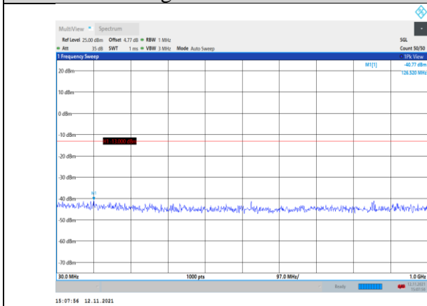
Band4-1.4MHz-16QAM-20175-1RB#0- Range1:30~1000MHz
