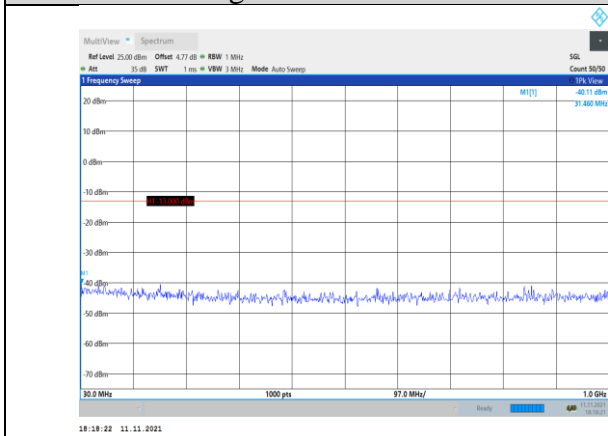
Band2-15MHz-QPSK-18900-1RB#0- Range1:30~1000MHz
