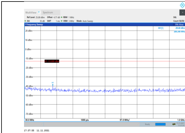
Band2-5MHz-16QAM-18625-1RB#0- Range1:30~1000MHz
