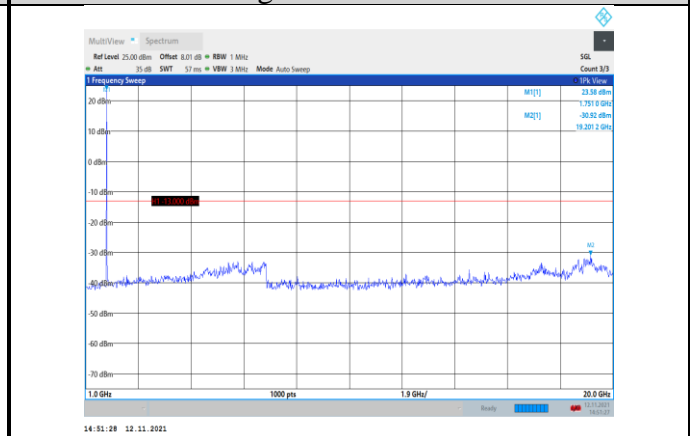
Band4-5MHz-16QAM-20375-1RB#0- Range2:1000~20000MHz
