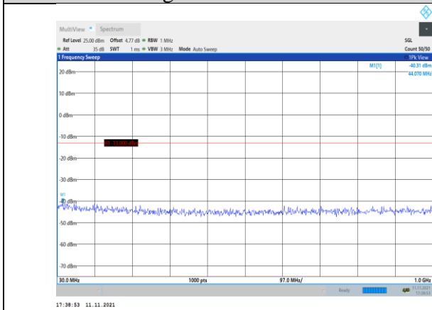
Band2-5MHz-16QAM-18900-1RB#0- Range1:30~1000MHz
