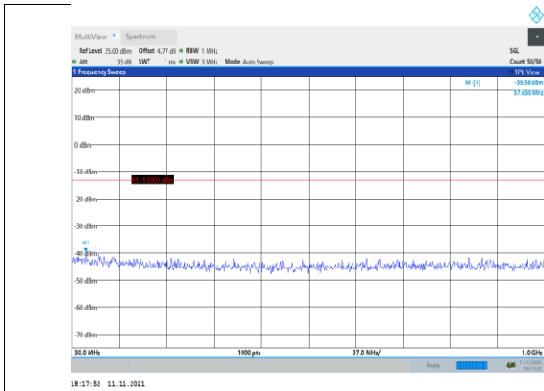
Band2-15MHz-16QAM-18675-1RB#0- Range1:30~1000MHz
