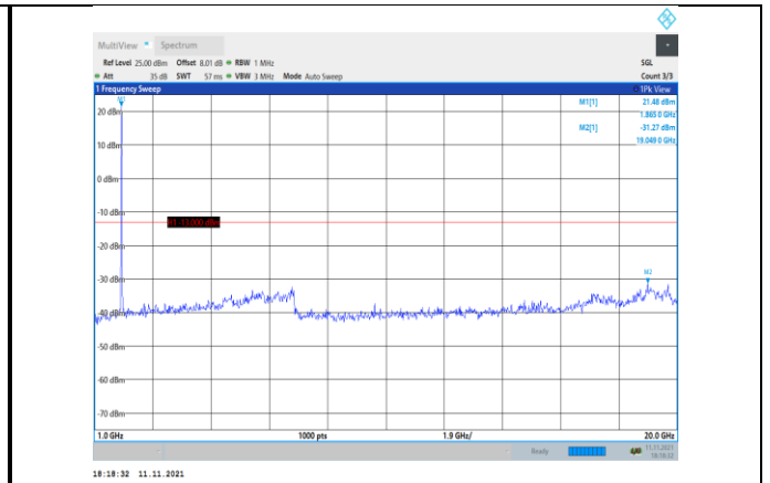
Band2-15MHz-QPSK-18900-1RB#0- Range2:1000~20000MHz
