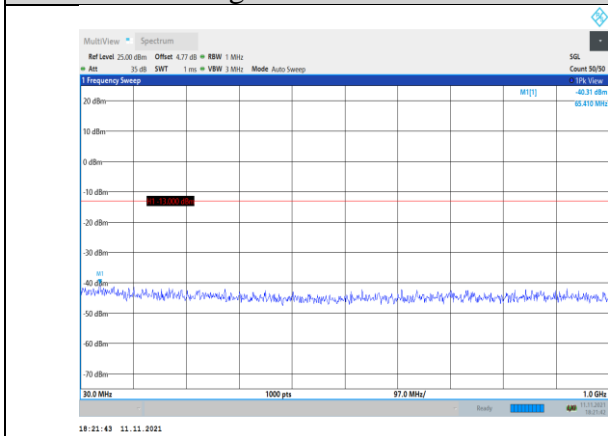
Band2-20MHz-QPSK-18900-1RB#0- Range1:30~1000MHz
