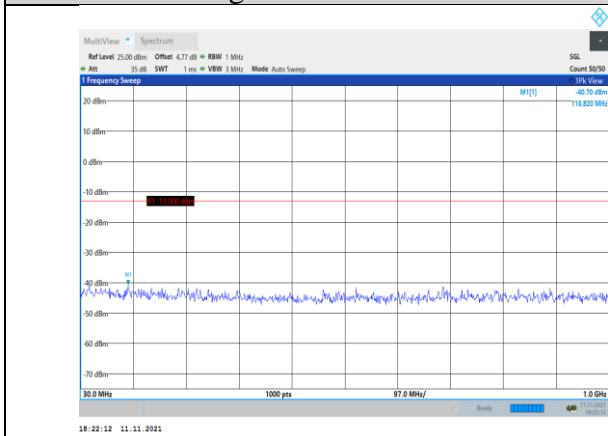
Band2-20MHz-16QAM-18900-1RB#0- Range1:30~1000MHz
