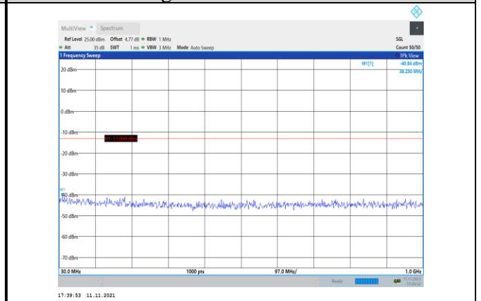
Band2-5MHz-16QAM-19175-1RB#0- Range1:30~1000MHz
