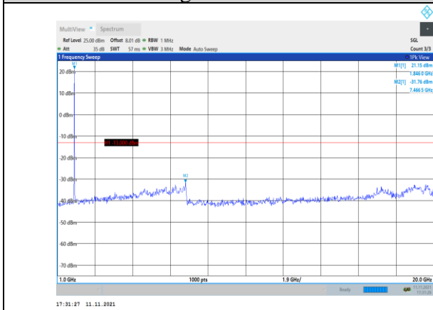
Band2-1.4MHz-16QAM-18607-1RB#0- Range2:1000~20000MHz
