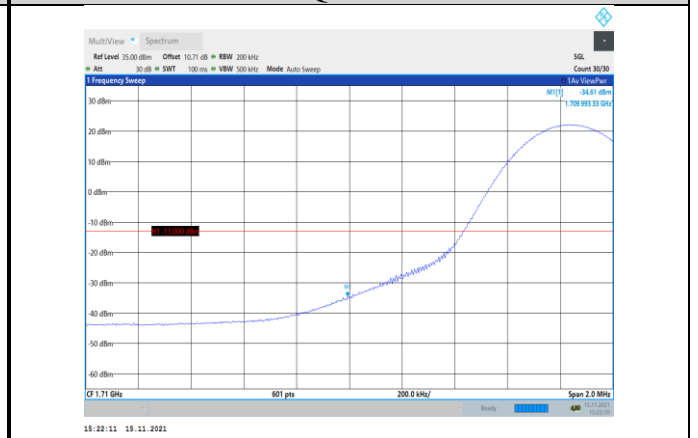
Band66-15MHz-16QAM-132047-1RB#0
