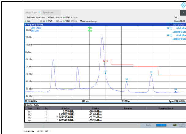
Band41-10MHz-QPSK-41190-1RB#49
