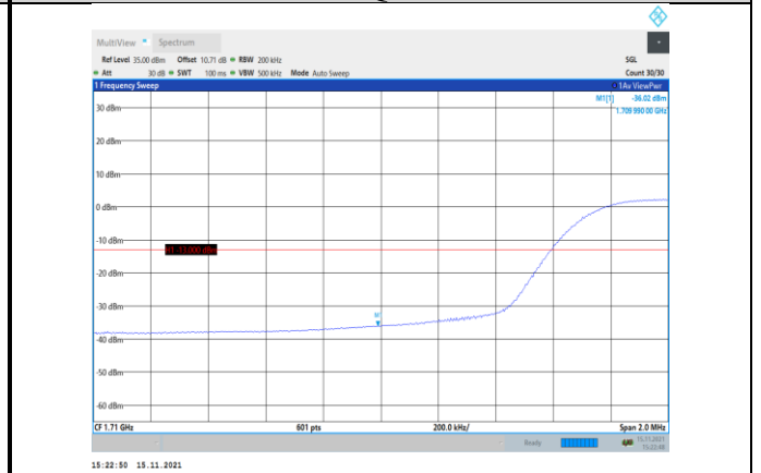
Band66-15MHz-16QAM-132047-75RB#0
