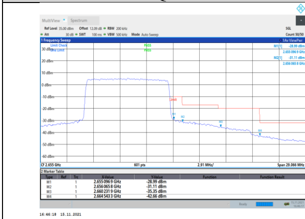
Band41-10MHz-QPSK-41190-50RB#0
