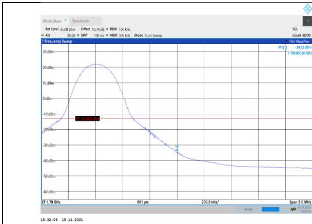
Band66-10MHz-QPSK-132622-1RB#49
