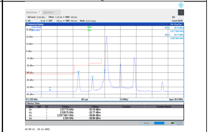
Band41-10MHz-QPSK-40090-1RB#0
