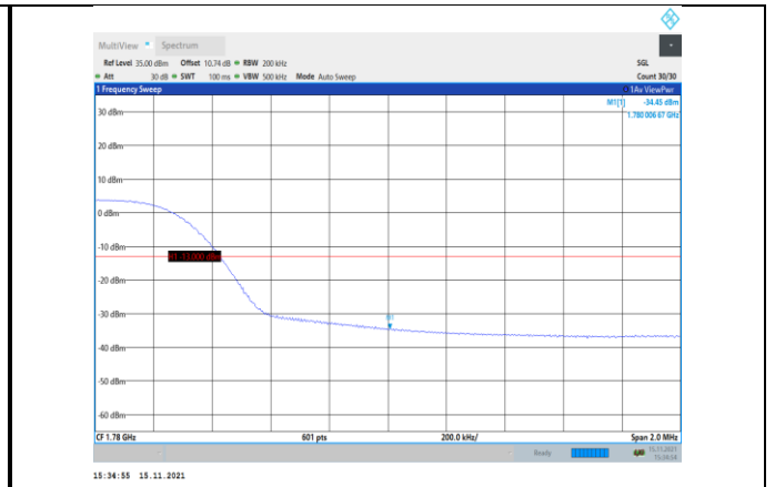
Band66-15MHz-QPSK-132597-75RB#0
