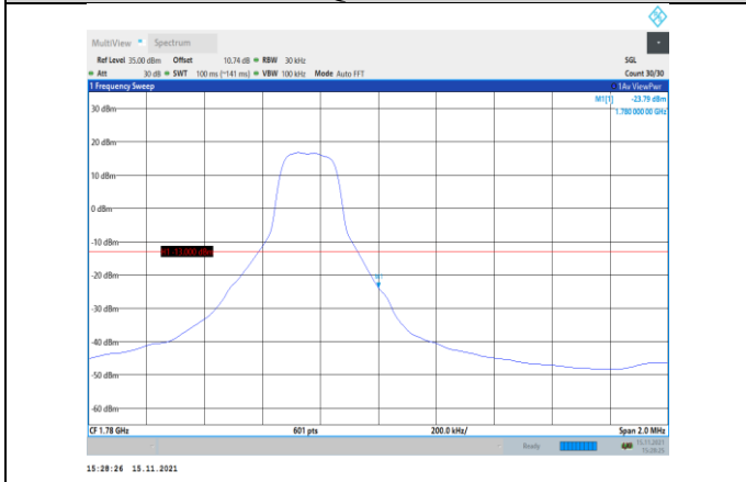
Band66-3MHz-QPSK-132657-1RB#14
