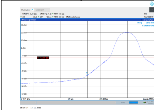
Band66-10MHz-16QAM-132022-1RB#0
