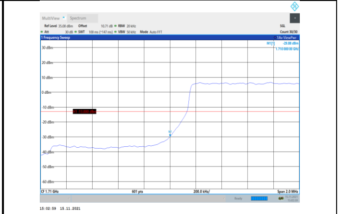
Band66-1.4MHz-QPSK-131979-6RB#0
