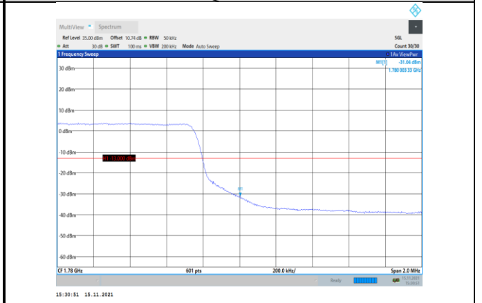
Band66-5MHz-QPSK-132647-25RB#0
