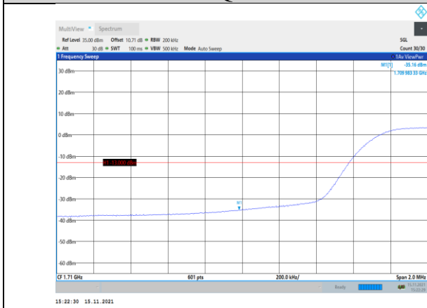
Band66-15MHz-QPSK-132047-75RB#0
