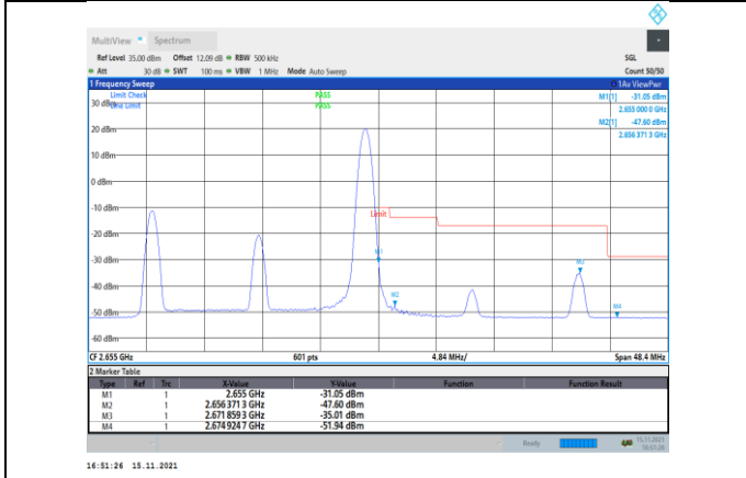
Band41-20MHz-16QAM-41140-1RB#99
