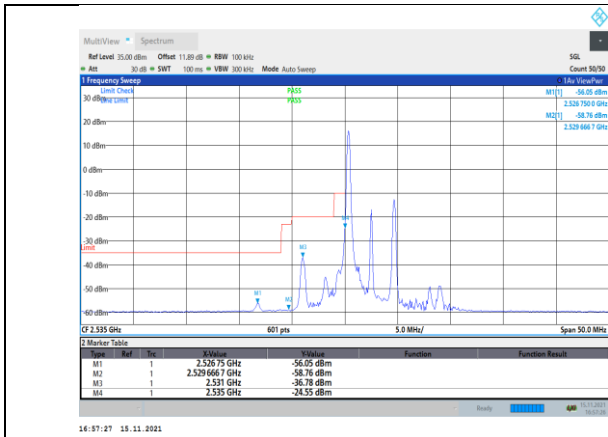
Band41-5MHz-16QAM-40065-1RB#0
