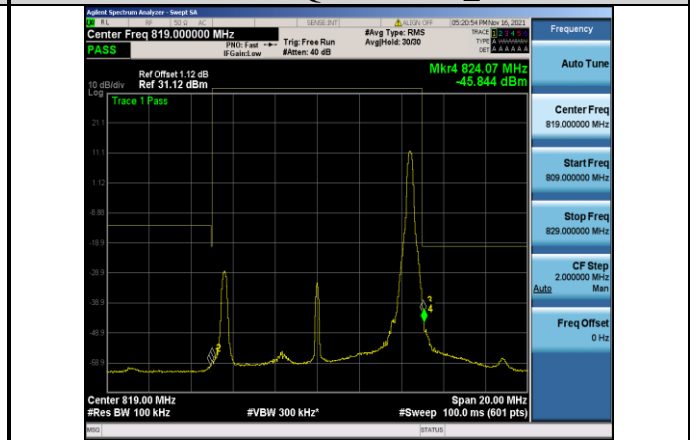
Band26-10MHz-16QAM-26740_Right-1RB#49
