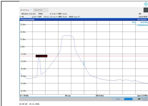
Band66-1.4MHz-QPSK-132665-1RB#5
