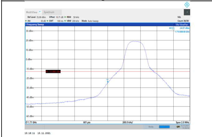
Band66-5MHz-QPSK-131997-1RB#0
