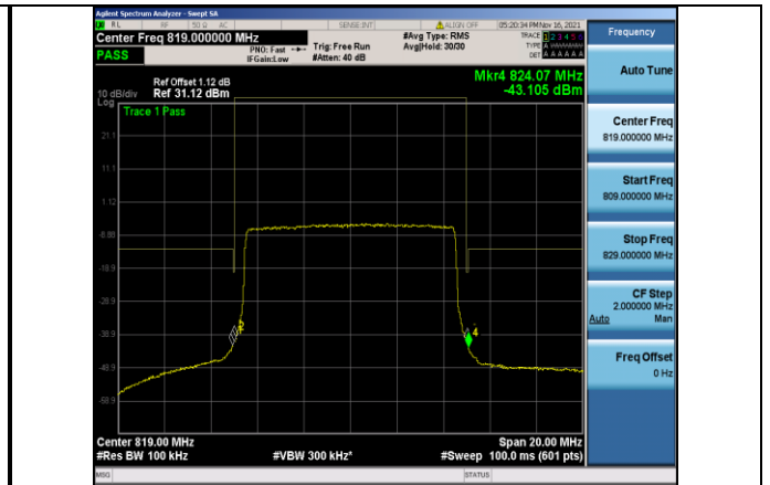
Band26-10MHz-16QAM-26740_Left-50RB#0
