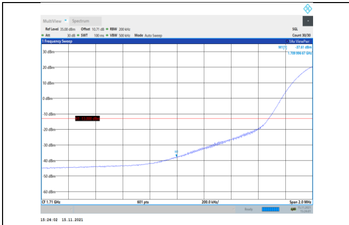
Band66-20MHz-16QAM-132072-1RB#0
