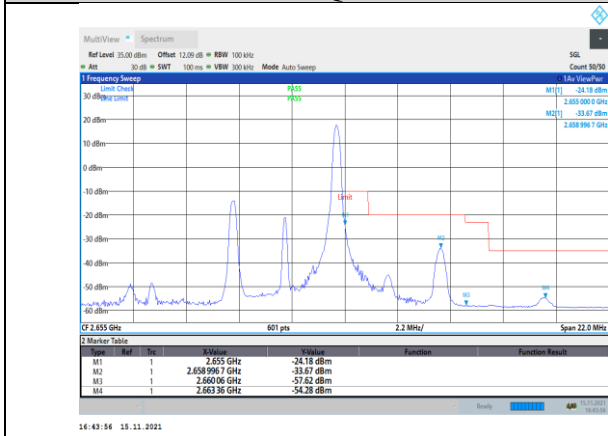
Band41-5MHz-16QAM-41215-1RB#24
