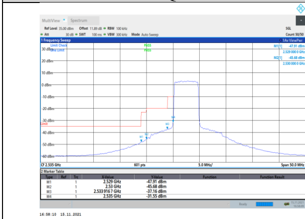
Band41-5MHz-16QAM-40065-25RB#0
