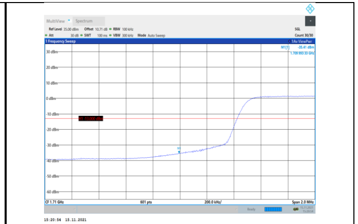
Band66-10MHz-16QAM-132022-50RB#0
