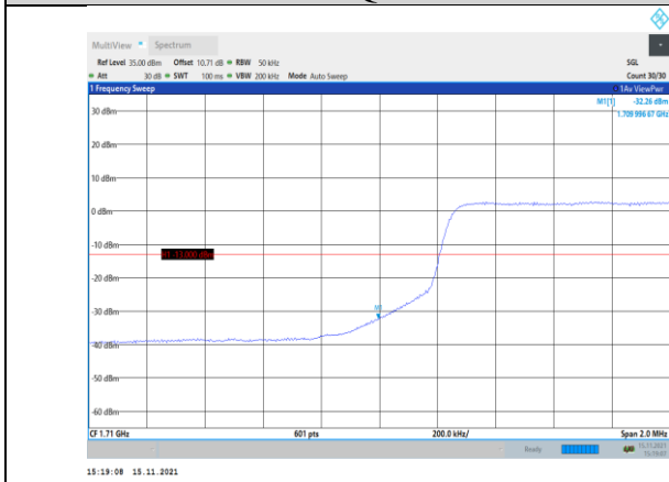
Band66-5MHz-16QAM-131997-25RB#0
