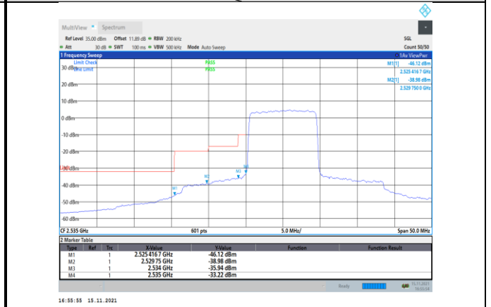
Band41-10MHz-QPSK-40090-50RB#0
