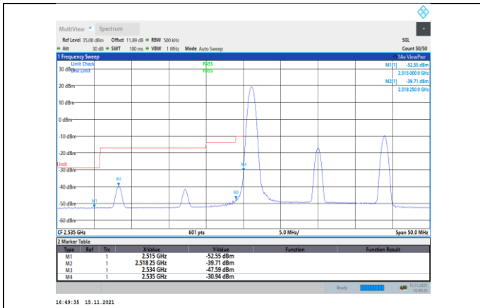
Band41-20MHz-16QAM-40140-1RB#0
