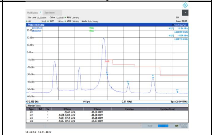
Band41-10MHz-16QAM-41190-1RB#49
