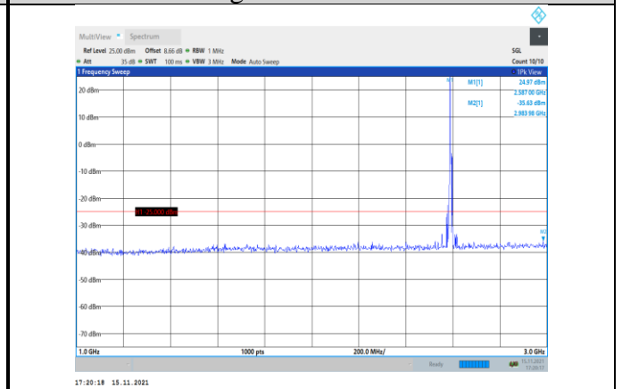
Band41-5MHz-16QAM-40590-1RB#0- Range2:1000~3000MHz
