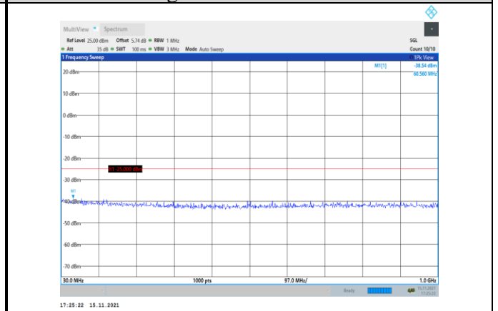
Band41-10MHz-QPSK-41190-1RB#0- Range1:30~1000MHz
