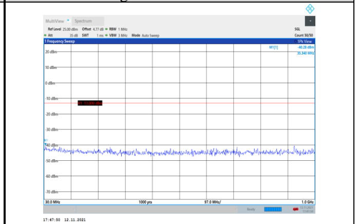
Band66-3MHz-16QAM-131987-1RB#0- Range1:30~1000MHz
