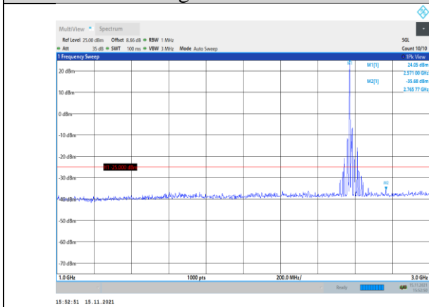
Band38-15MHz-16QAM-37825-1RB#0- Range2:1000~3000MHz
