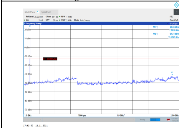
Band66-1.4MHz-QPSK-132322-1RB#0- Range2:1000~20000MHz
