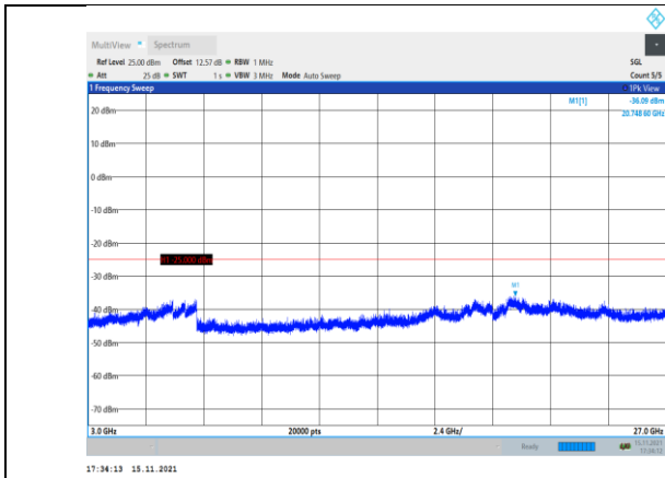
Band41-20MHz-16QAM-40590-1RB#0- Range3:3000~27000MHz
