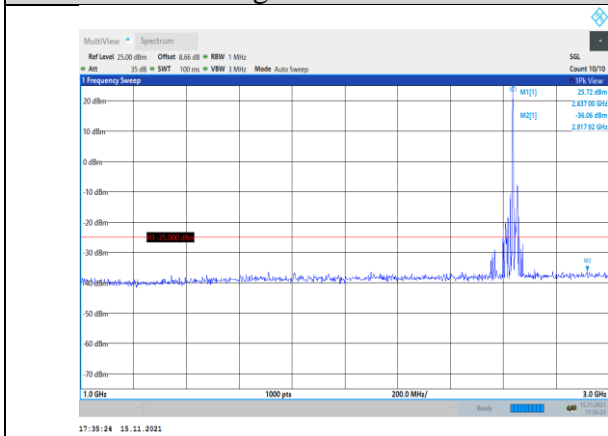
Band41-20MHz-16QAM-41140-1RB#0- Range2:1000~3000MHz
