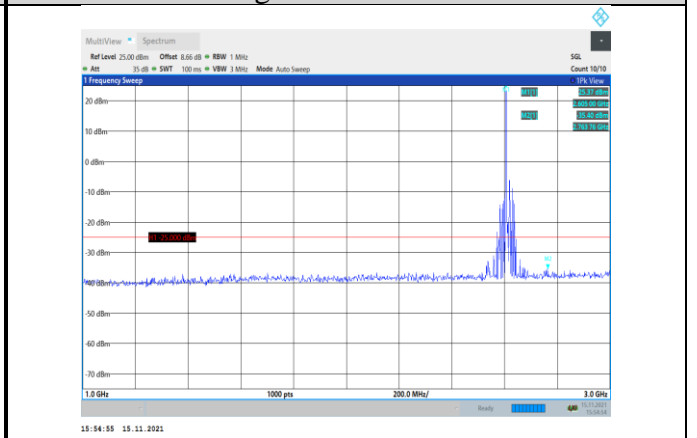
Band38-15MHz-QPSK-38175-1RB#0- Range2:1000~3000MHz
