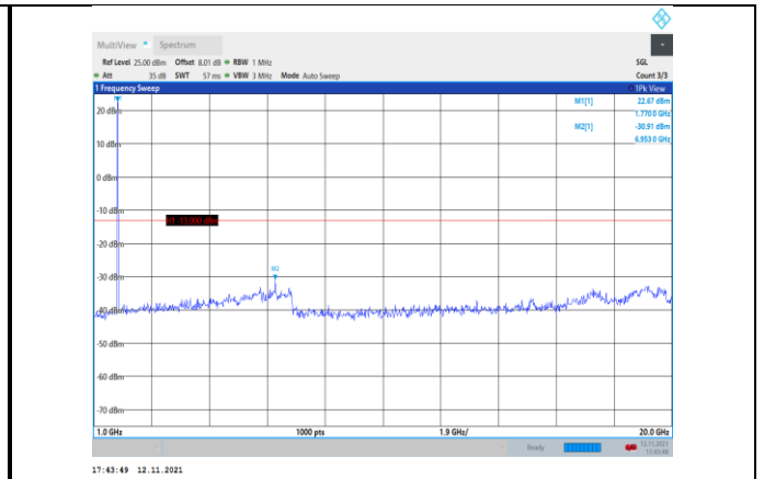
Band66-1.4MHz-QPSK-132665-1RB#0- Range2:1000~20000MHz
