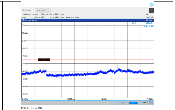
Band41-10MHz-16QAM-41190-1RB#0- Range3:3000~27000MHz
