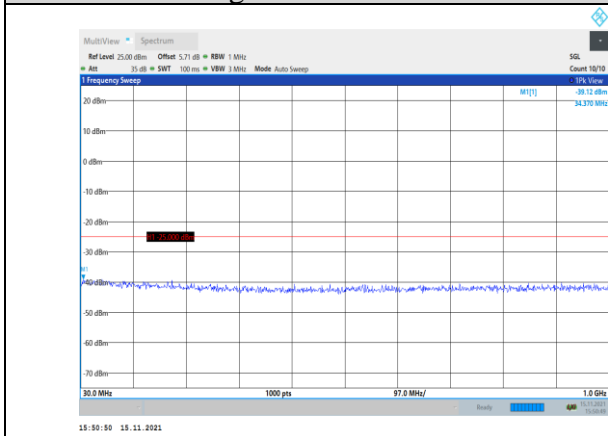
Band38-10MHz-16QAM-38200-1RB#0- Range1:30~1000MHz
