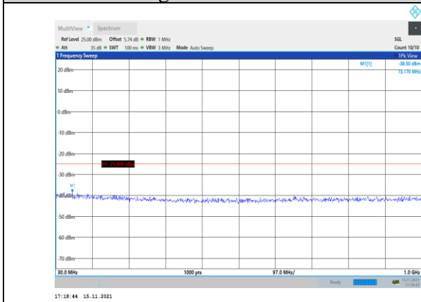
Band41-5MHz-16QAM-40065-1RB#0- Range1:30~1000MHz
