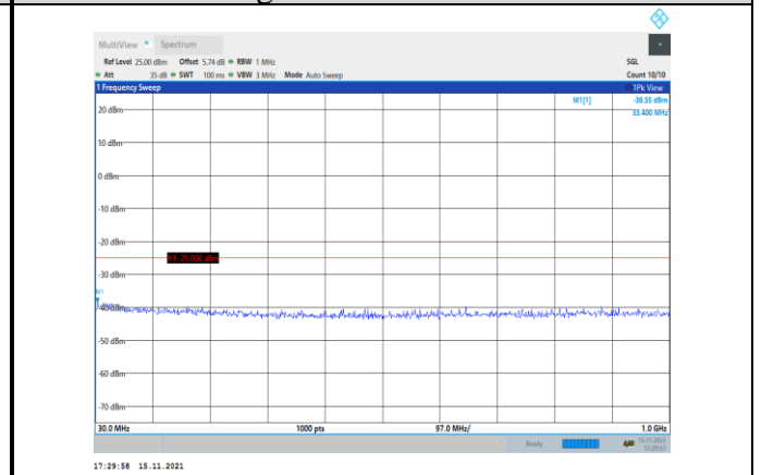
Band41-15MHz-QPSK-41165-1RB#0- Range1:30~1000MHz
