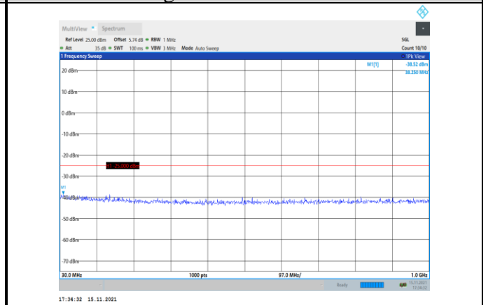
Band41-20MHz-QPSK-41140-1RB#0- Range1:30~1000MHz
