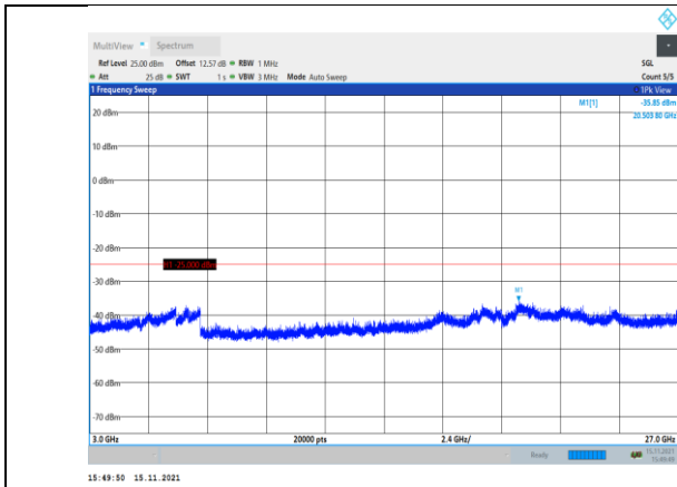
Band38-10MHz-16QAM-38000-1RB#0- Range3:3000~27000MHz
