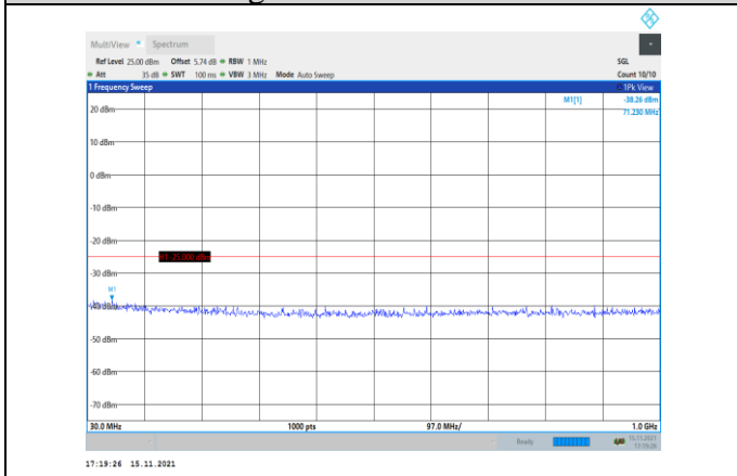
Band41-5MHz-QPSK-40590-1RB#0- Range1:30~1000MHz
