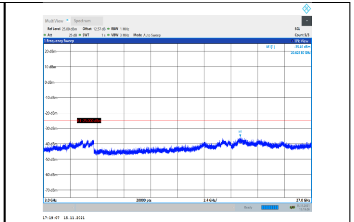
Band41-5MHz-16QAM-40065-1RB#0- Range3:3000~27000MHz
