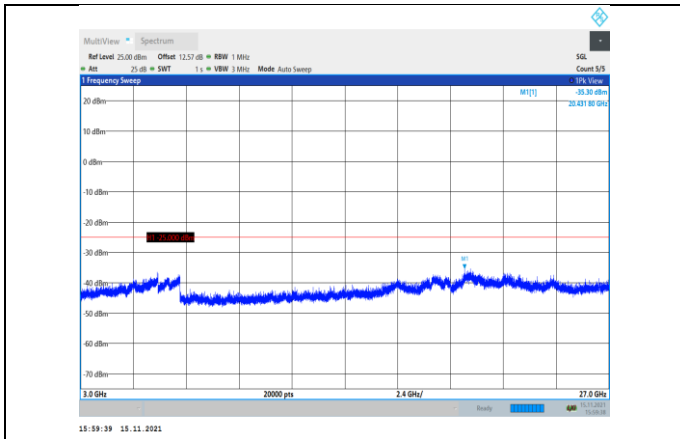
Band38-20MHz-QPSK-38150-1RB#0- Range3:3000~27000MHz
