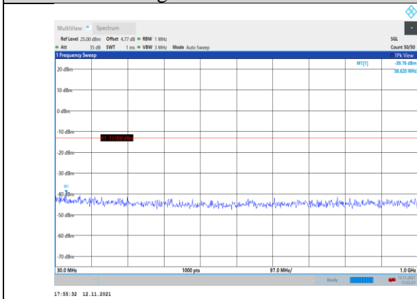
Band66-5MHz-QPSK-132647-1RB#0- Range1:30~1000MHz
