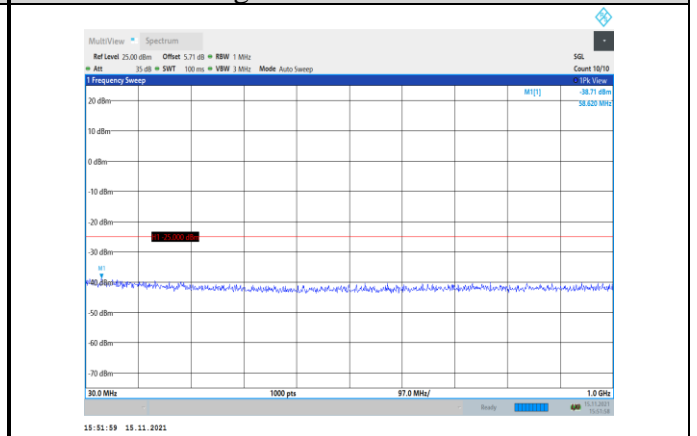
Band38-15MHz-QPSK-37825-1RB#0- Range1:30~1000MHz
