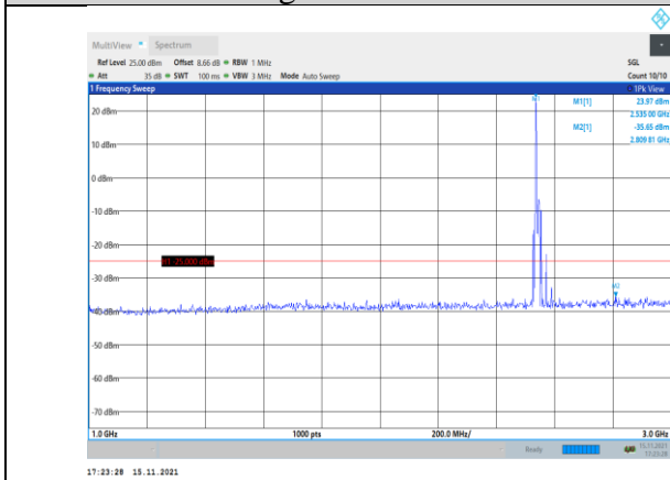
Band41-10MHz-16QAM-40090-1RB#0- Range2:1000~3000MHz
