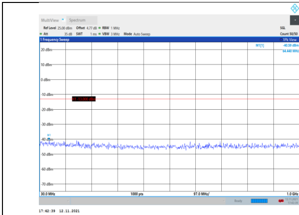
Band66-1.4MHz-QPSK-132322-1RB#0- Range1:30~1000MHz
