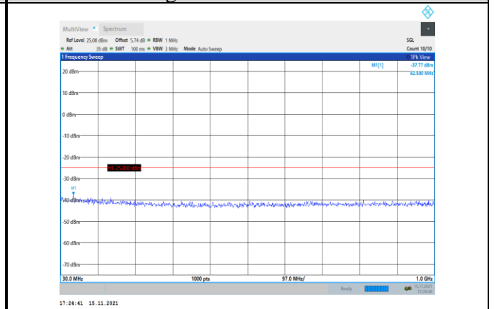
Band41-10MHz-16QAM-40590-1RB#0- Range1:30~1000MHz
