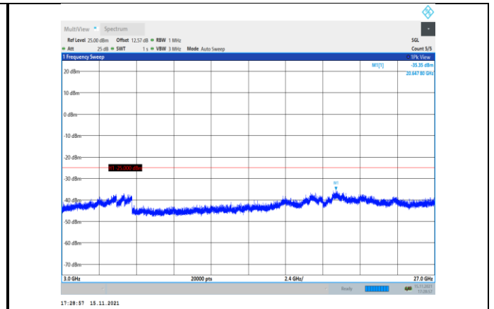
Band41-15MHz-QPSK-40590-1RB#0- Range3:3000~27000MHz
