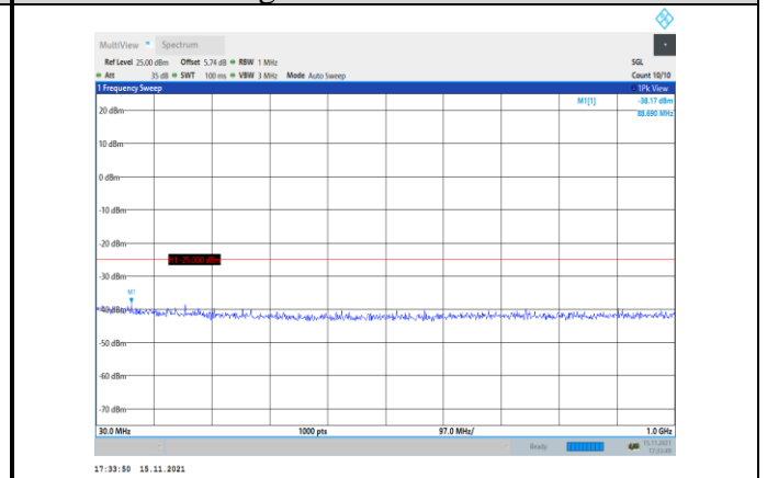
Band41-20MHz-16QAM-40590-1RB#0- Range1:30~1000MHz
