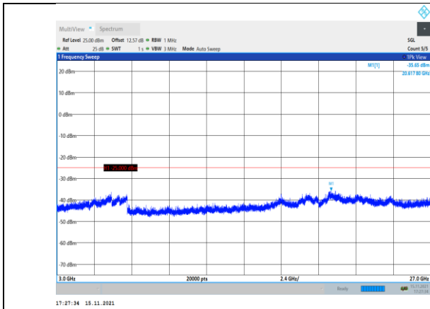
Band41-15MHz-QPSK-40115-1RB#0- Range3:3000~27000MHz
