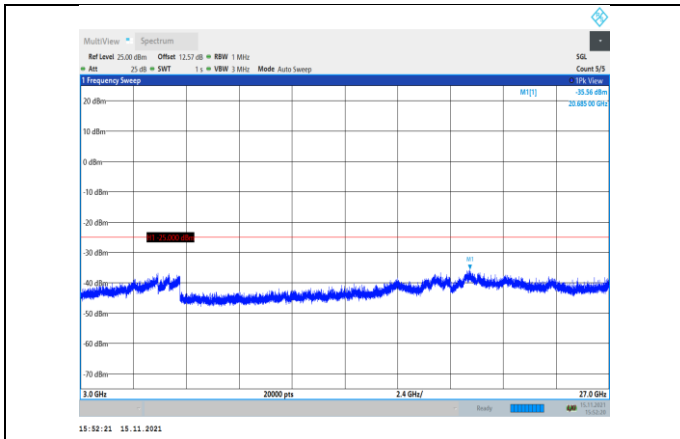
Band38-15MHz-QPSK-37825-1RB#0- Range3:3000~27000MHz
