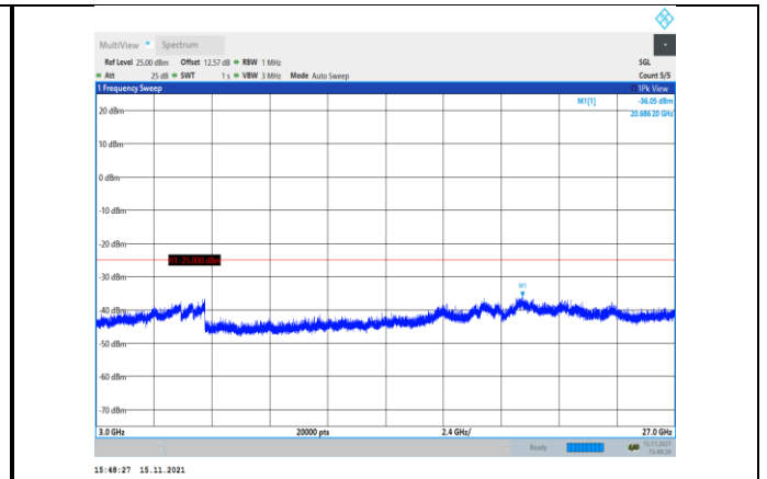
Band38-10MHz-16QAM-37800-1RB#0- Range3:3000~27000MHz
