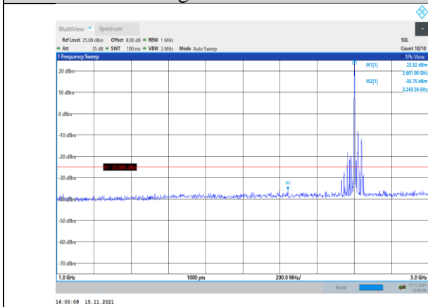
Band38-20MHz-16QAM-38150-1RB#0-Range2:1000~3000MHz
