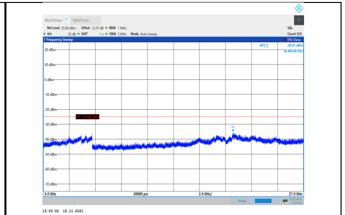
Band38-15MHz-16QAM-37825-1RB#0- Range3:3000~27000MHz
