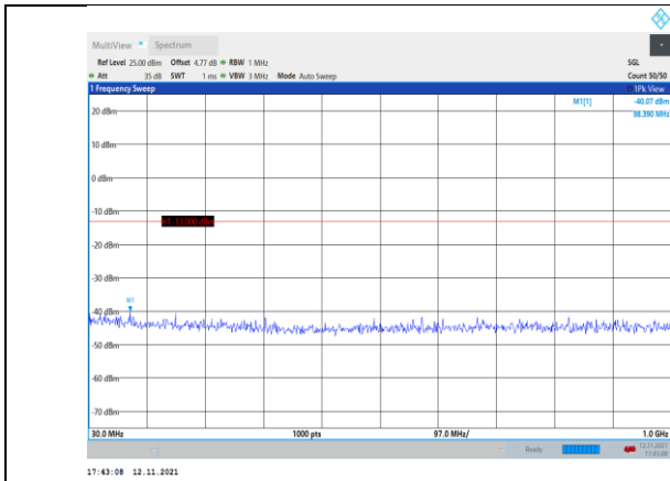
Band66-1.4MHz-16QAM-132322-1RB#0- Range1:30~1000MHz
