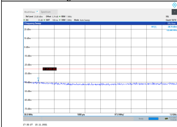
Band41-20MHz-16QAM-40140-1RB#0- Range1:30~1000MHz
