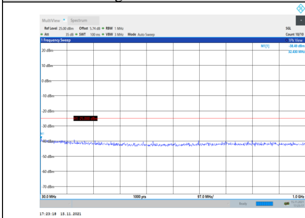
Band41-10MHz-16QAM-40090-1RB#0- Range1:30~1000MHz
