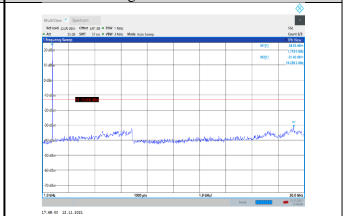
Band66-3MHz-16QAM-131987-1RB#0- Range2:1000~20000MHz
