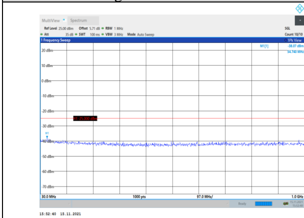
Band38-15MHz-16QAM-37825-1RB#0- Range1:30~1000MHz
