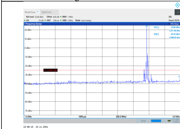
Band38-10MHz-16QAM-37800-1RB#0- Range2:1000~3000MHz
