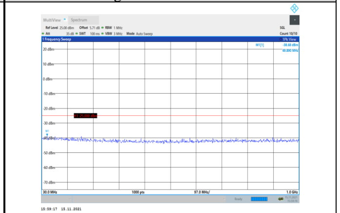
Band38-20MHz-QPSK-38150-1RB#0- Range1:30~1000MHz
