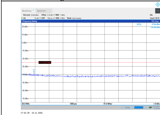
Band41-5MHz-16QAM-41215-1RB#0- Range1:30~1000MHz
