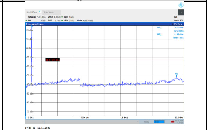
Band66-1.4MHz-QPSK-131979-1RB#0- Range2:1000~20000MHz
