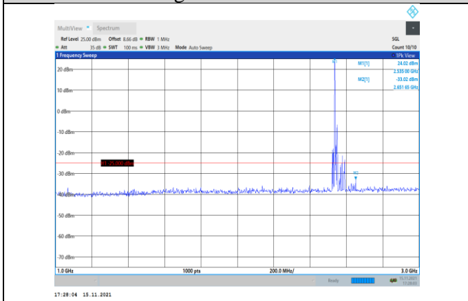
Band41-15MHz-16QAM-40115-1RB#0- Range2:1000~3000MHz
