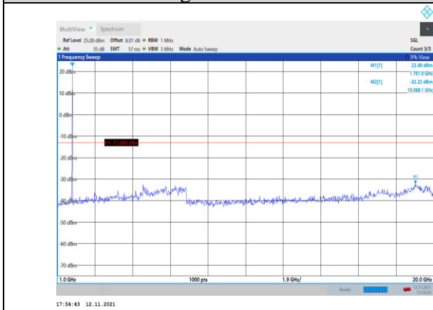
Band66-5MHz-QPSK-132322-1RB#0- Range2:1000~20000MHz
