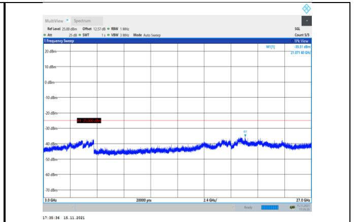
Band41-20MHz-16QAM-41140-1RB#0- Range3:3000~27000MHz
