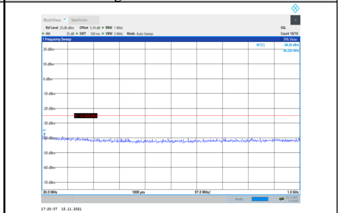
Band41-5MHz-16QAM-40590-1RB#0- Range1:30~1000MHz
