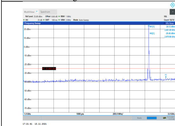
Band41-5MHz-16QAM-41215-1RB#0- Range2:1000~3000MHz
