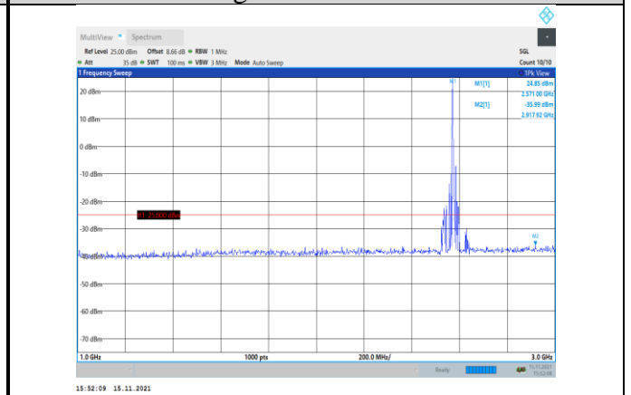
Band38-15MHz-QPSK-37825-1RB#0- Range2:1000~3000MHz
