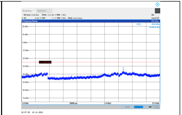
Band38-20MHz-16QAM-37850-1RB#0- Range3:3000~27000MHz
