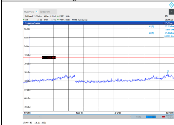
Band66-3MHz-QPSK-132322-1RB#0- Range2:1000~20000MHz
