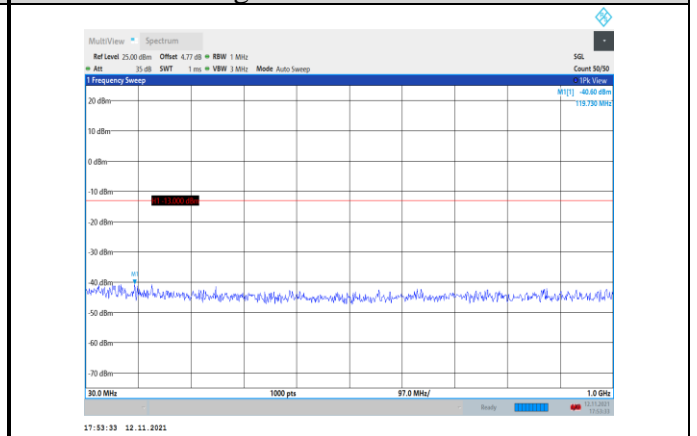
Band66-5MHz-QPSK-131997-1RB#0- Range1:30~1000MHz
