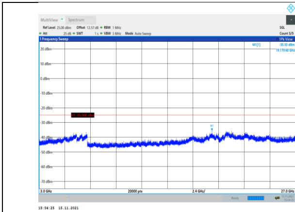
Band38-15MHz-16QAM-38000-1RB#0- Range3:3000~27000MHz
