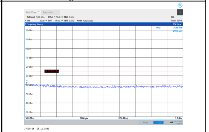
Band41-15MHz-16QAM-40590-1RB#0- Range1:30~1000MHz
