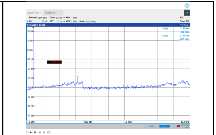
Band66-3MHz-16QAM-132657-1RB#0- Range2:1000~20000MHz
