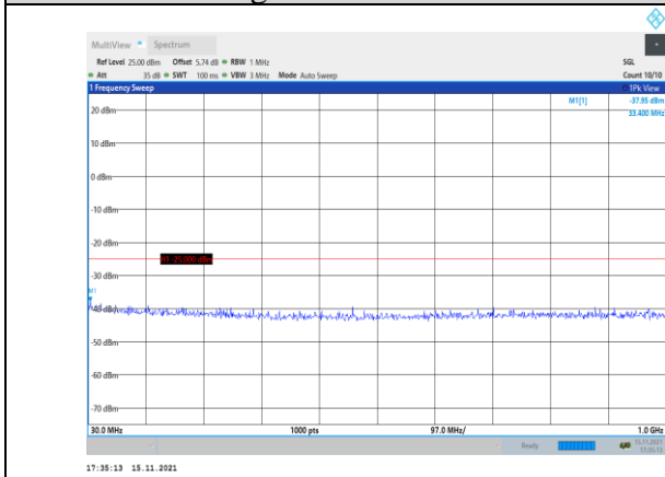
Band41-20MHz-16QAM-41140-1RB#0- Range1:30~1000MHz
