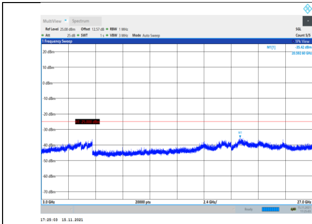
Band41-10MHz-16QAM-40590-1RB#0- Range3:3000~27000MHz
