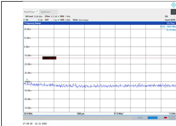
Band66-5MHz-QPSK-132322-1RB#0- Range1:30~1000MHz
