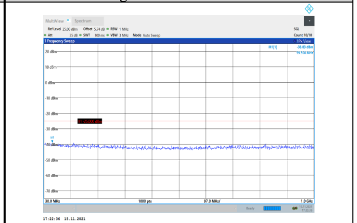
Band41-10MHz-QPSK-40090-1RB#0- Range1:30~1000MHz
