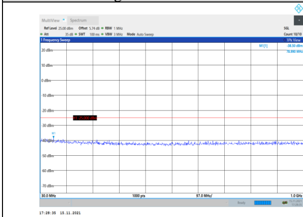
Band41-15MHz-QPSK-40590-1RB#0- Range1:30~1000MHz
