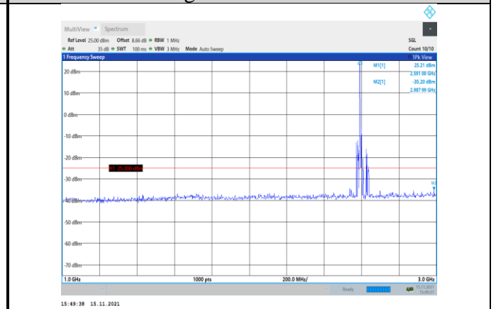
Band38-10MHz-16QAM-38000-1RB#0- Range2:1000~3000MHz
