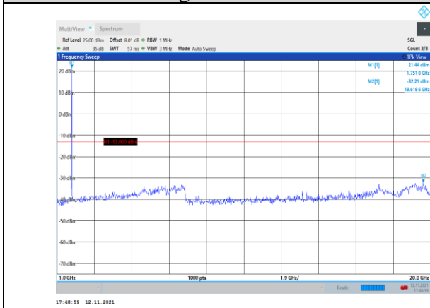
Band66-3MHz-16QAM-132322-1RB#0- Range2:1000~20000MHz
