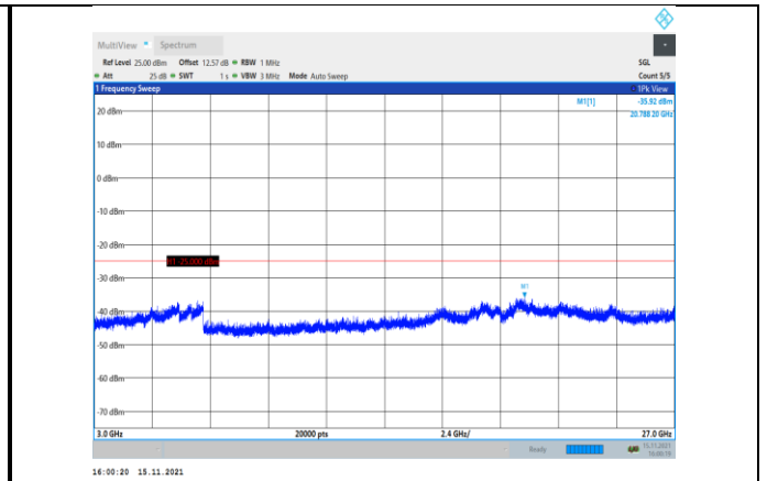
Band38-20MHz-16QAM-38150-1RB#0-Range3:3000~27000MHz
