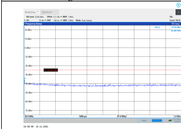
Band38-20MHz-16QAM-38150-1RB#0-Range1:30~1000MHz
