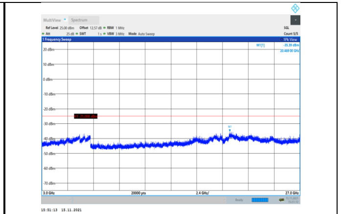
Band38-10MHz-16QAM-38200-1RB#0- Range3:3000~27000MHz
