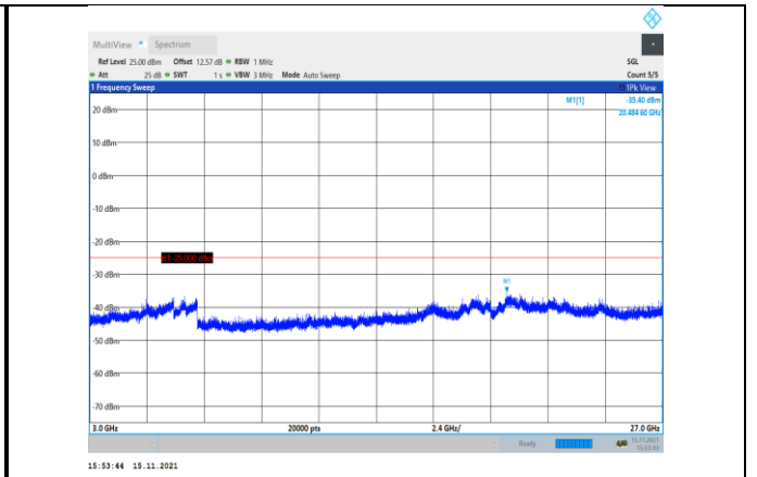
Band38-15MHz-QPSK-38000-1RB#0- Range3:3000~27000MHz
