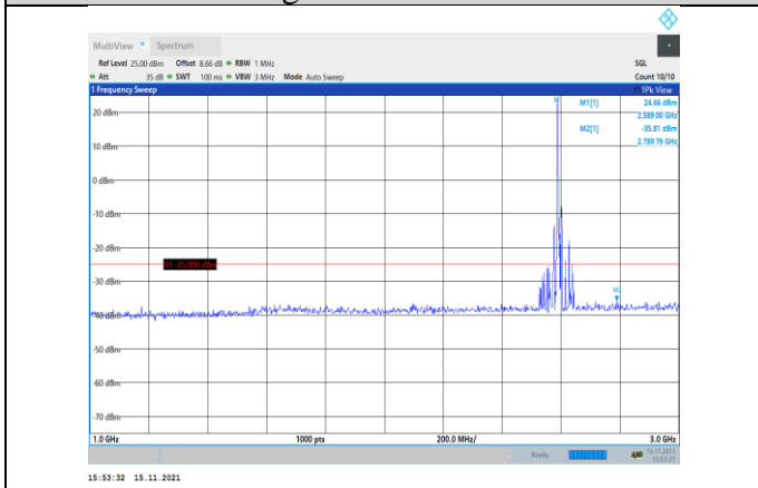
Band38-15MHz-QPSK-38000-1RB#0- Range2:1000~3000MHz
