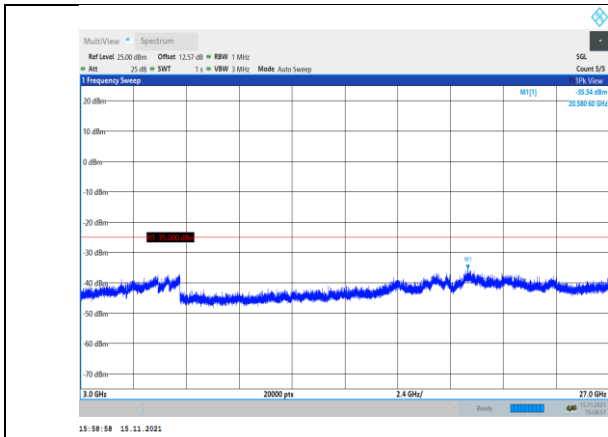
Band38-20MHz-16QAM-38000-1RB#0-Range3:3000~27000MHz
