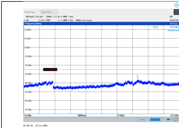
Band38-10MHz-QPSK-38200-1RB#0- Range3:3000~27000MHz
