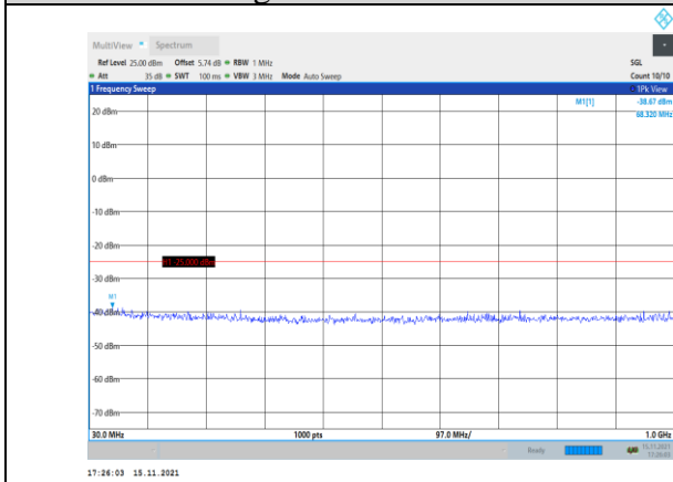
Band41-10MHz-16QAM-41190-1RB#0- Range1:30~1000MHz
