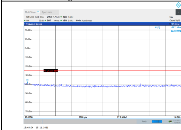
Band38-10MHz-16QAM-37800-1RB#0- Range1:30~1000MHz
