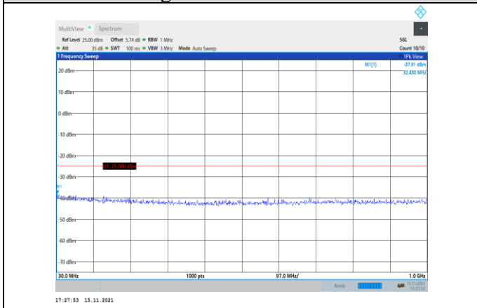
Band41-15MHz-16QAM-40115-1RB#0- Range1:30~1000MHz
