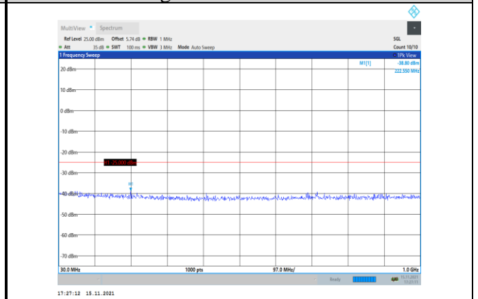
Band41-15MHz-QPSK-40115-1RB#0- Range1:30~1000MHz
