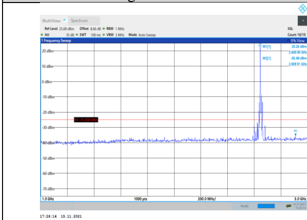
Band41-10MHz-16QAM-41190-1RB#0- Range2:1000~3000MHz
