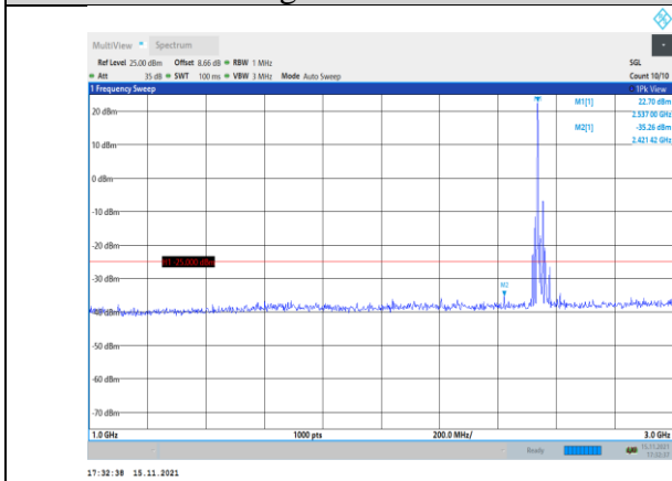
Band41-20MHz-16QAM-40140-1RB#0- Range2:1000~3000MHz
