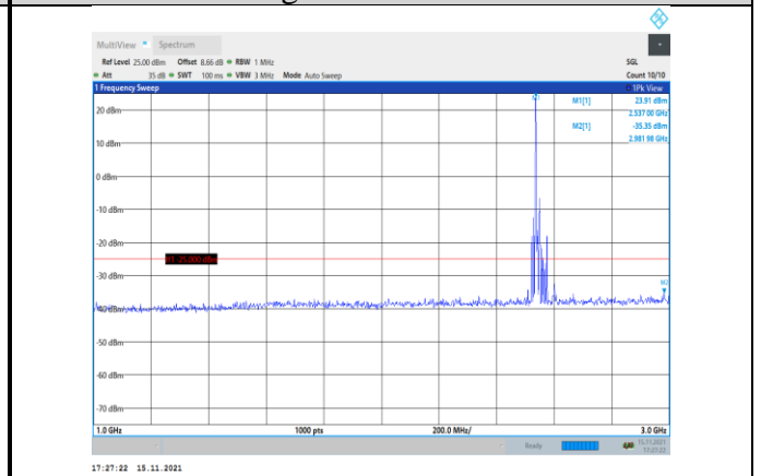
Band41-15MHz-QPSK-40115-1RB#0- Range2:1000~3000MHz
