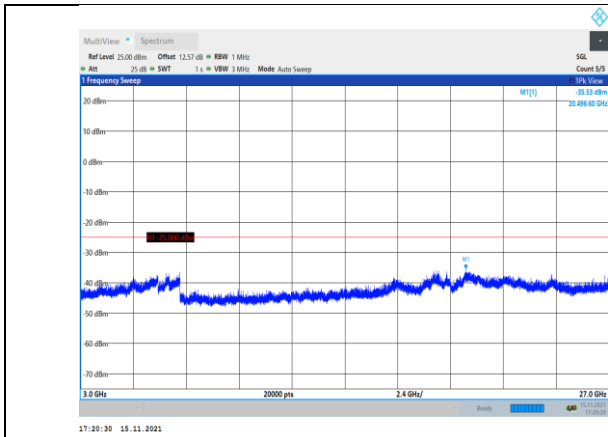
Band41-5MHz-16QAM-40590-1RB#0- Range3:3000~27000MHz
