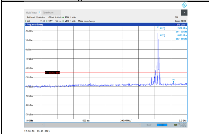
Band41-15MHz-16QAM-41165-1RB#0- Range2:1000~3000MHz
