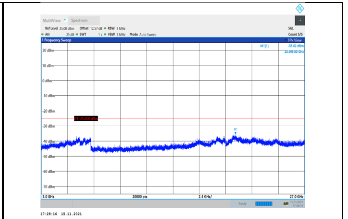
Band41-15MHz-16QAM-40115-1RB#0- Range3:3000~27000MHz
