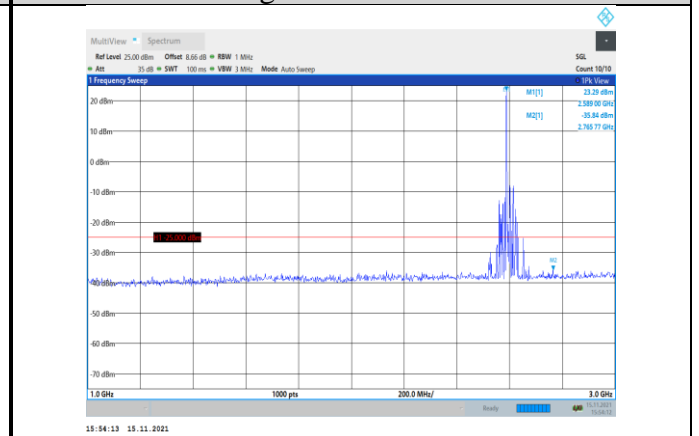
Band38-15MHz-16QAM-38000-1RB#0- Range2:1000~3000MHz
