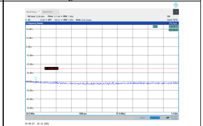
Band38-10MHz-16QAM-38000-1RB#0- Range1:30~1000MHz
