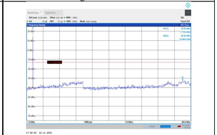
Band66-1.4MHz-16QAM-131979-1RB#0- Range2:1000~20000MHz
