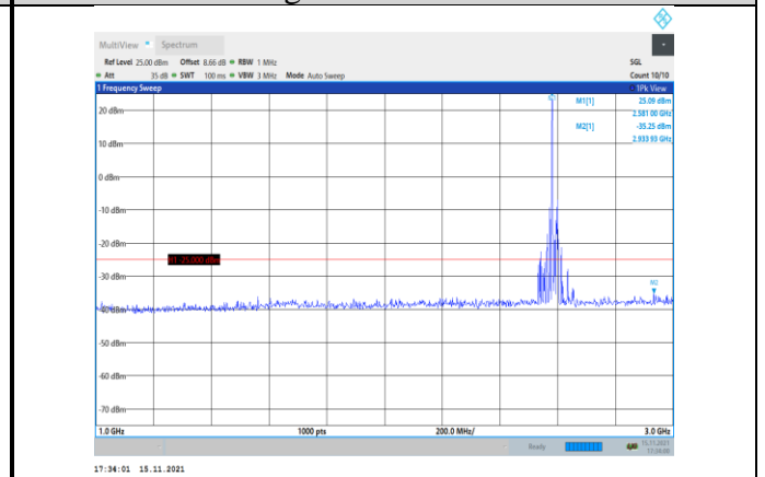
Band41-20MHz-16QAM-40590-1RB#0- Range2:1000~3000MHz
