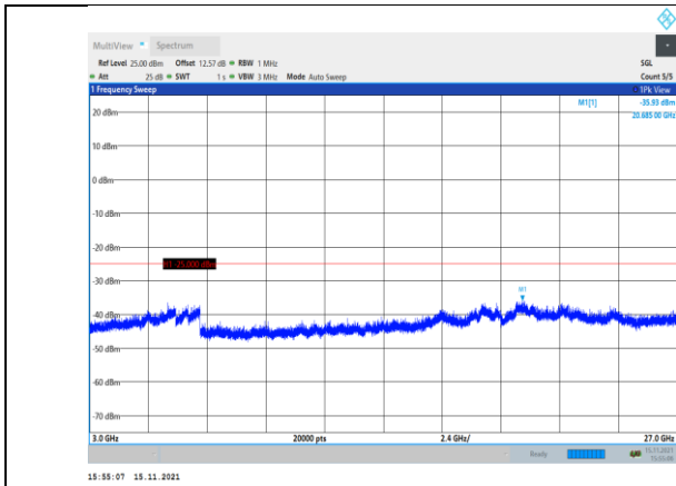
Band38-15MHz-QPSK-38175-1RB#0- Range3:3000~27000MHz
