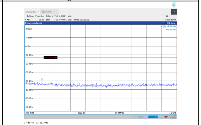
Band66-1.4MHz-QPSK-131979-1RB#0- Range1:30~1000MHz
