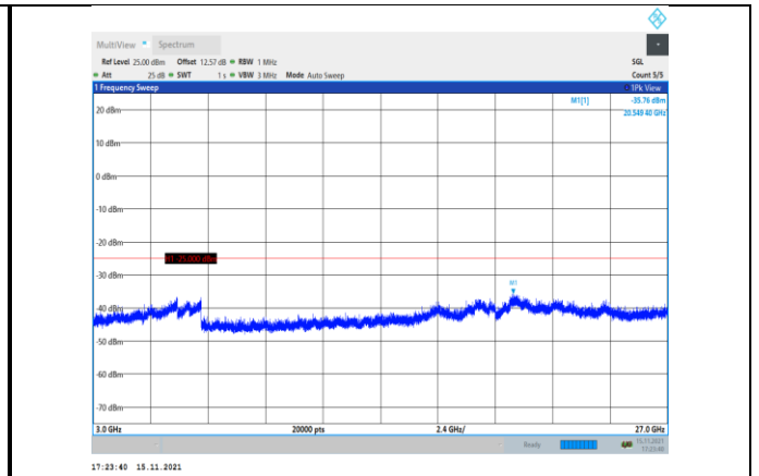
Band41-10MHz-16QAM-40090-1RB#0- Range3:3000~27000MHz
