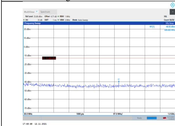
Band66-3MHz-16QAM-132657-1RB#0- Range1:30~1000MHz
