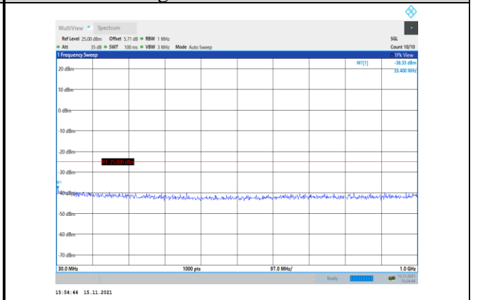
Band38-15MHz-QPSK-38175-1RB#0- Range1:30~1000MHz
