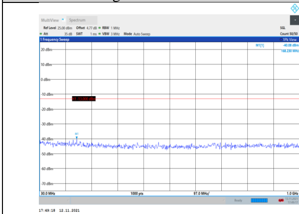
Band66-3MHz-QPSK-132657-1RB#0- Range1:30~1000MHz
