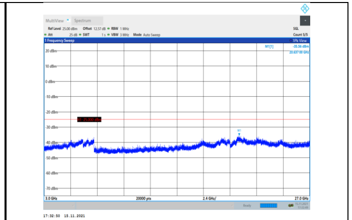
Band41-20MHz-16QAM-40140-1RB#0- Range3:3000~27000MHz
