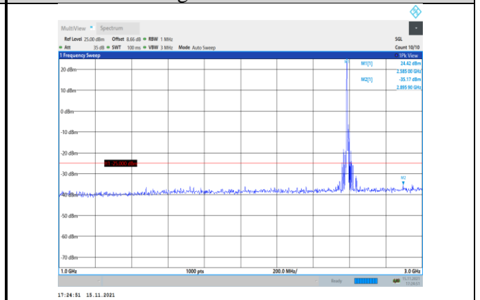
Band41-10MHz-16QAM-40590-1RB#0- Range2:1000~3000MHz
