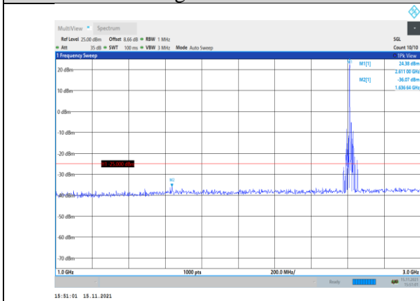
Band38-10MHz-16QAM-38200-1RB#0- Range2:1000~3000MHz
