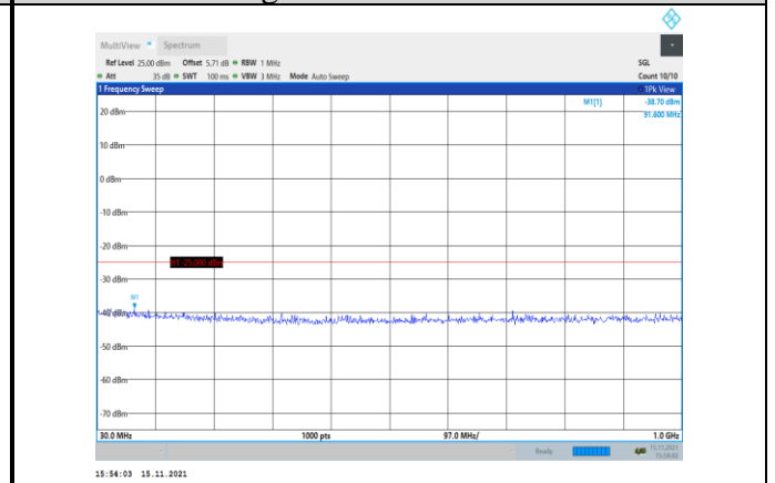
Band38-15MHz-16QAM-38000-1RB#0- Range1:30~1000MHz
