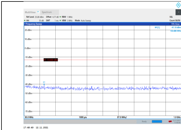
Band66-3MHz-16QAM-132322-1RB#0- Range1:30~1000MHz
